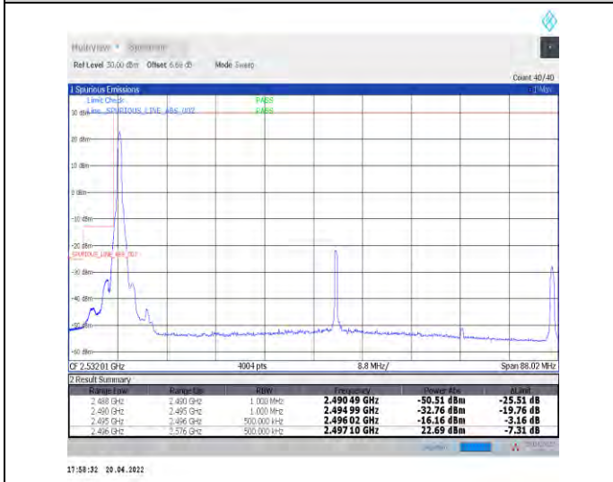
1-N41--30-80-L-4-CP-QPSK-Edge_1RB_Left-1@0-Ant0-PASS-see graph
