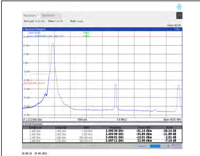
1-N41--30-40-L-1-DFT-PI2BPSK-Edge_1RB_Left-1@0-Ant0-PASS-see graph
