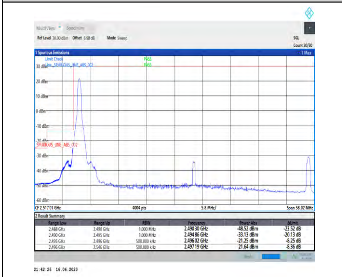
1-N41-PC1-30-50-L-4-CP-QPSK-Edge_1RB_Left-1@0-Ant0-1--PASS-see graph
