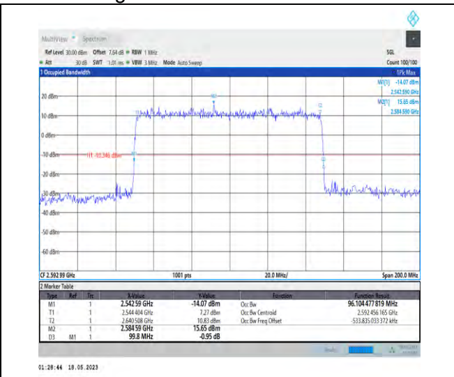
1-N41-PC1-30-100-M-1-DFT-QPSK-Outer_Full-270 @0-Ant0-96.104-99.800-≤100-PASS
