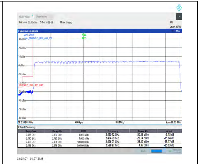
1-N41-PC1-30-80-L-3-DFT-PI2BPSK-Outer_Full-216@0-Ant0-1--PASS-see graph
