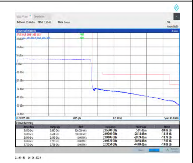
1-N41-PC1-30-40-H-6-CP-QPSK-Outer_Full-106@0-Ant0-1--PASS-see graph
