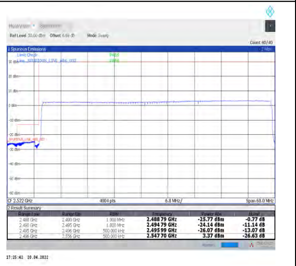
1-N41--30-60-L-6-CP-QPSK-Outer_Full-162@0-Ant0-PASS-see graph
