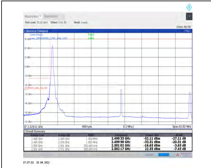
1-N41--30-70-L-1-DFT-PI2BPSK-Edge_1RB_Left-1@0-Ant0-PASS-see graph
