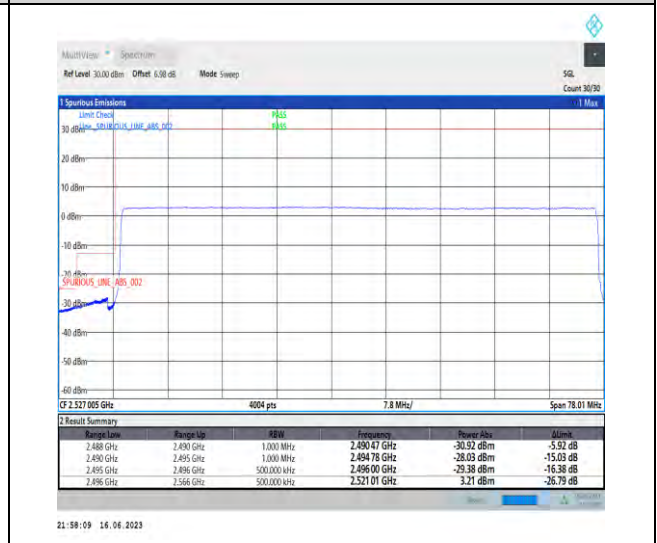
1-N41-PC1-30-70-L-6-CP-QPSK-Outer_Full-189@0-Ant0-1--PASS-see graph
