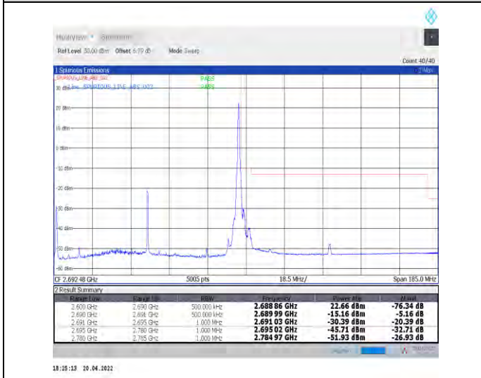
1-N41--30-90-H-5-CP-QPSK-Edge_1RB_Right-1@244-Ant0-PASS-see graph
