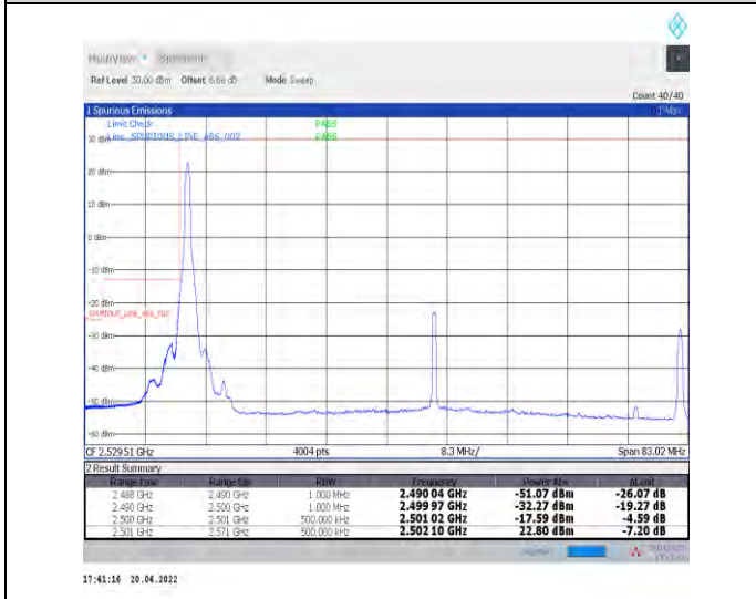
1-N41--30-70-L-4-CP-QPSK-Edge_1RB_Left-1@0-Ant0-PASS-see graph
