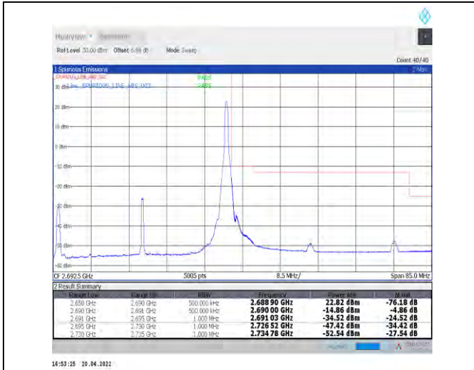
1-N41--30-40-H-2-DFT-PI2BPSK-Edge_1RB_Right-1@105-Ant0-PASS-see graph
