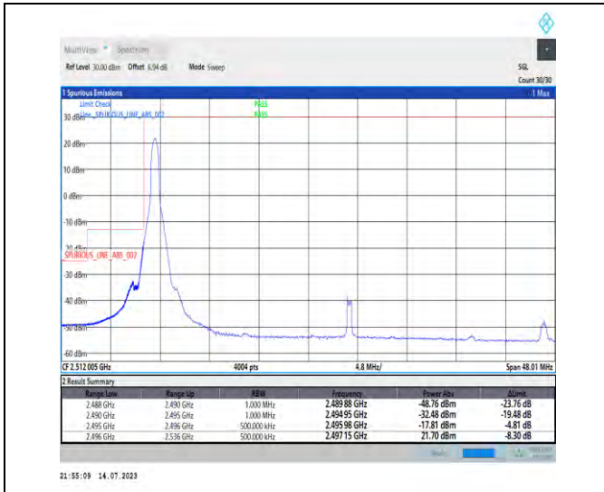
1-N41-PC1-30-40-L-1-DFT-PI2BPSK-Edge_1RB_Left-1@0-Ant0-1--PASS-see graph
