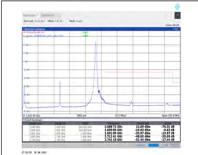
1-N41--30-50-H-2-DFT-PI2BPSK-Edge_1RB_Right-1@132-Ant0-PASS-see graph
