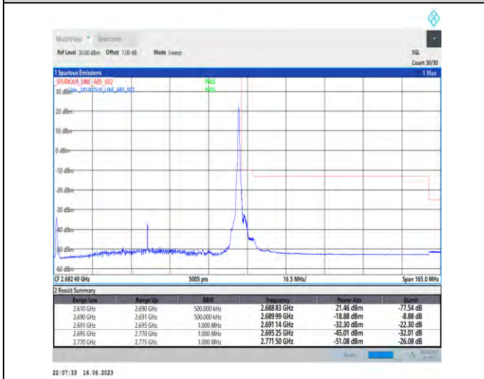
1-N41-PC1-30-80-H-5-CP-QPSK-Edge_1RB_Right-1@216-Ant0-1--PASS-see graph
