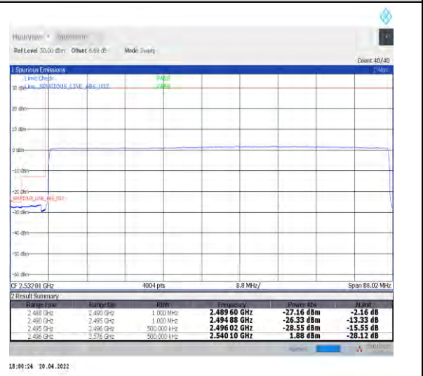
1-N41--30-80-L-6-CP-QPSK-Outer_Full-217@0-Ant0-PASS-see graph
