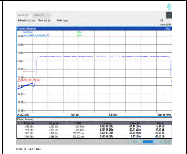
1-N41-PC1-30-60-L-3-DFT-PI2BPSK-Outer_Full-16 2@0-Ant0-1--PASS-see graph
