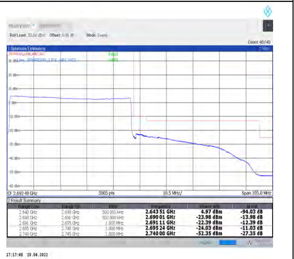
1-N41--30-50-H-6-CP-QPSK-Outer_Full-133@0-Ant0-PASS-see graph
