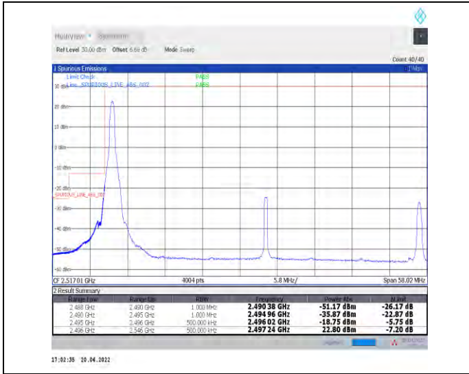
1-N41--30-50-L-1-DFT-PI2BPSK-Edge_1RB_Left-1@0-Ant0-PASS-see graph
