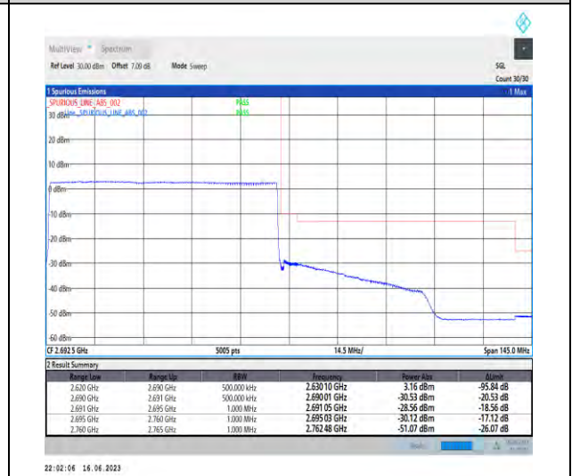
1-N41-PC1-30-70-H-6-CP-QPSK-Outer_Full-189@0-Ant0-1--PASS-see graph
