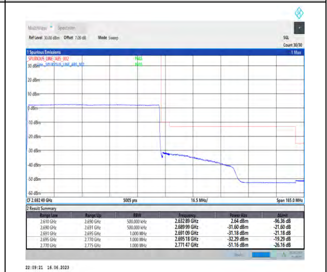
1-N41-PC1-30-80-H-6-CP-QPSK-Outer_Full-217@0-Ant0-1--PASS-see graph
