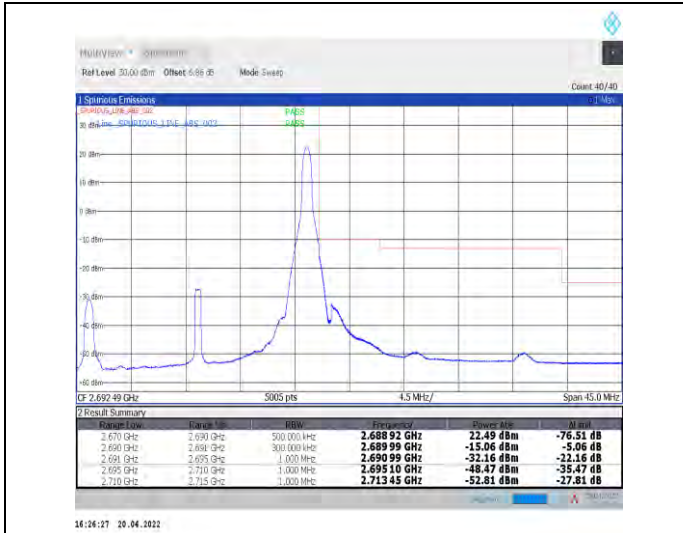
1-N41--30-20-H-2-DFT-PI2BPSK-Edge_1RB_Right-1@50-Ant0-PASS-see graph
