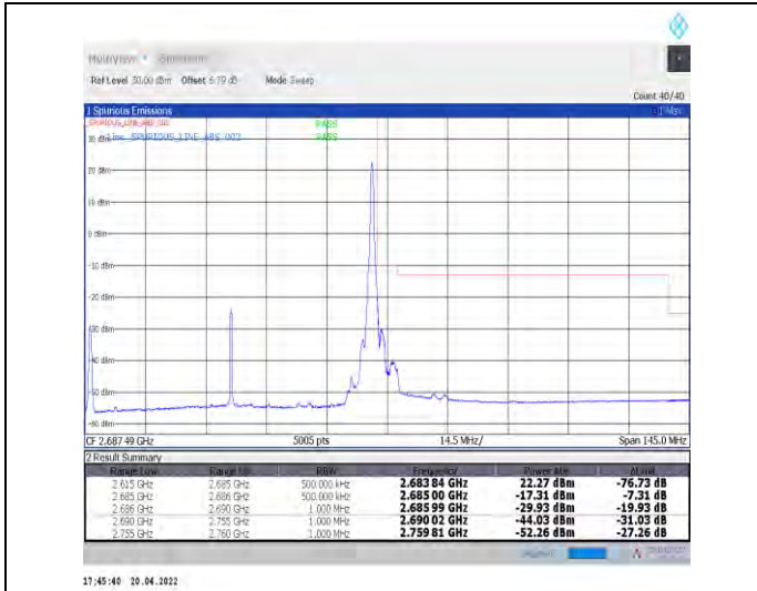
1-N41--30-70-H-2-DFT-PI2BPSK-Edge_1RB_Right-1@188-Ant0-PASS-see graph
