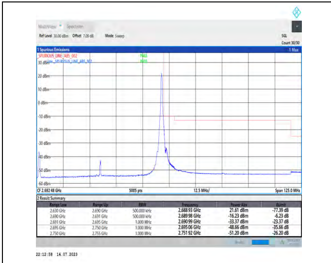
1-N41-PC1-30-60-H-2-DFT-PI2BPSK-Edge_1RB_Right-t-1@161-Ant0-1--PASS-see graph
