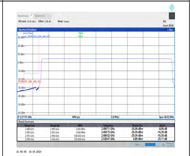
1-N41-PC1-30-50-L-6-CP-QPSK-Outer_Full-133@0-Ant0-1--PASS-see graph
