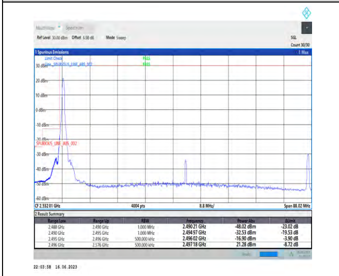
1-N41-PC1-30-80-L-4-CP-QPSK-Edge_1RB_Left-1@0-Ant0-1--PASS-see graph
