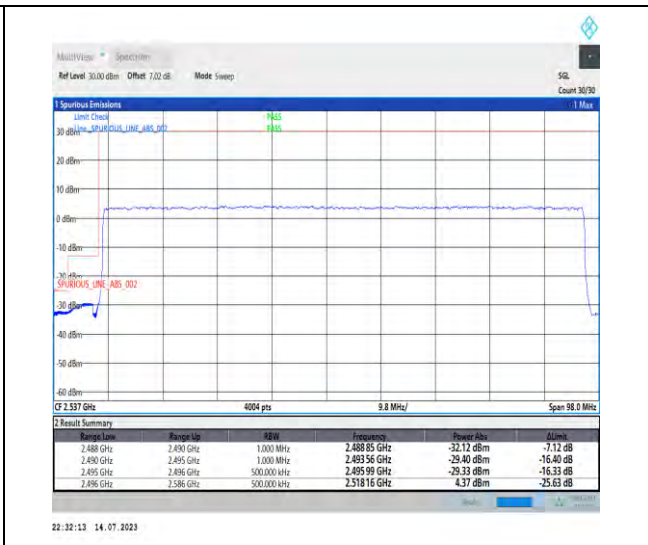
1-N41-PC1-30-90-L-3-DFT-PI2BPSK-Outer_Full-240@0-Ant0-1--PASS-see graph
