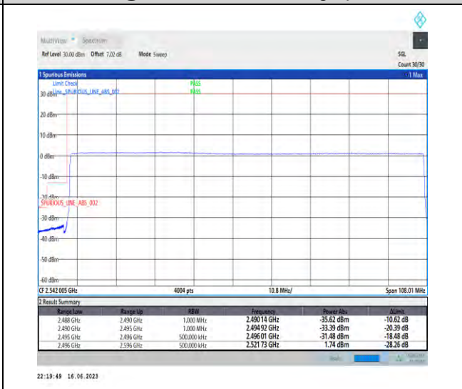
1-N41-PC1-30-100-L-6-CP-QPSK-Outer_Full-273@ 0-Ant0-1--PASS-see graph
