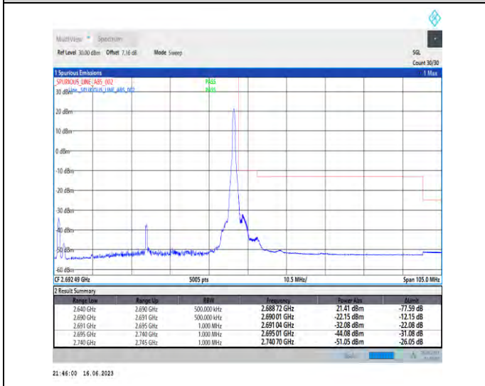
1-N41-PC1-30-50-H-5-CP-QPSK-Edge_1RB_Right-1@132-Ant0-1--PASS-see graph
