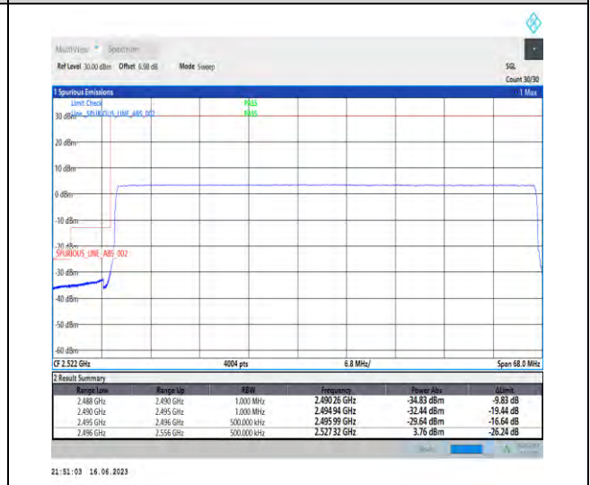
1-N41-PC1-30-60-L-6-CP-QPSK-Outer_Full-162@0-Ant0-1--PASS-see graph
