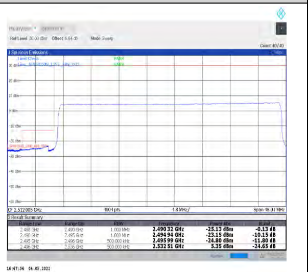
1-N41--30-40-L-6-CP-QPSK-Outer_Full-106@0-Ant0-PASS-see graph
