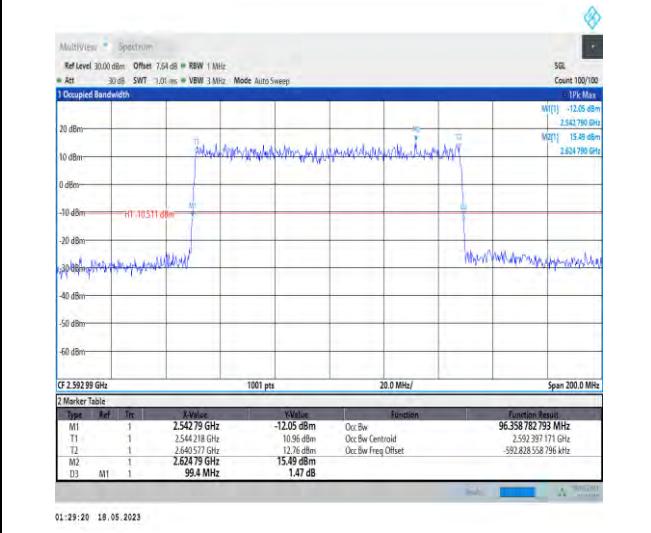
1-N41-PC1-30-100-M-3-DFT-16QAM-Outer_Full-270 @0-Ant0-96.359-99.400-≤100-PASS
