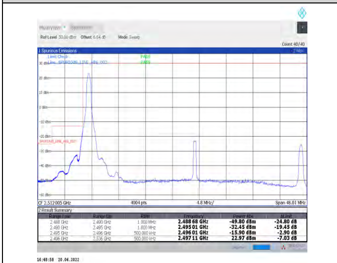
1-N41--30-40-L-4-CP-QPSK-Edge_1RB_Left-1@0-Ant0-PASS-see graph
