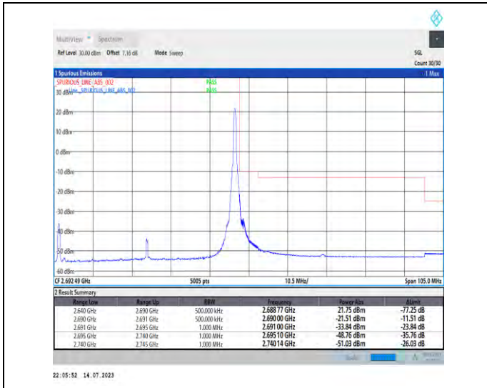
1-N41-PC1-30-50-H-2-DFT-PI2BPSK-Edge_1RB_Right-t-1@132-Ant0-1--PASS-see graph
