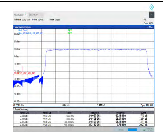
1-N41-PC1-30-30-L-3-DFT-PI2BPSK-Outer_Full-75@0-Ant0-1--PASS-see graph
