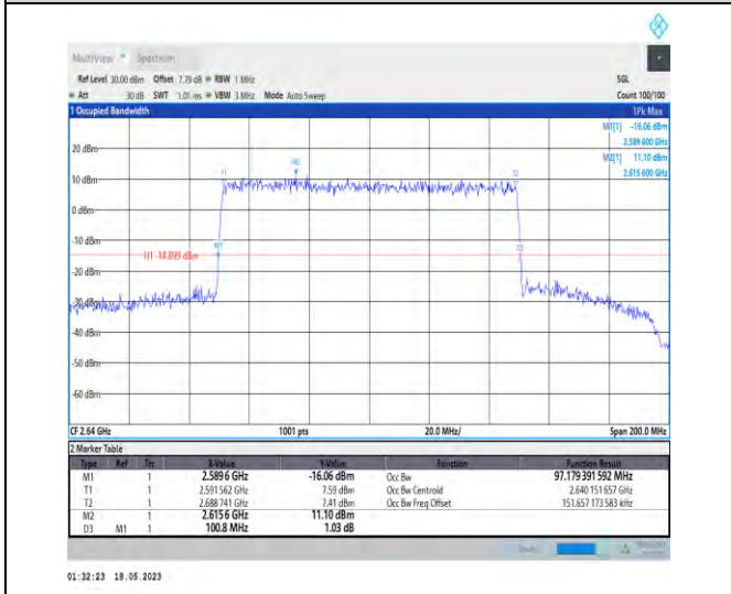
1-N41-PC1-30-100-H-9-CP-256QAM-Outer_Full-273 @0-Ant0-97.179-100.800-≤100-PASS
