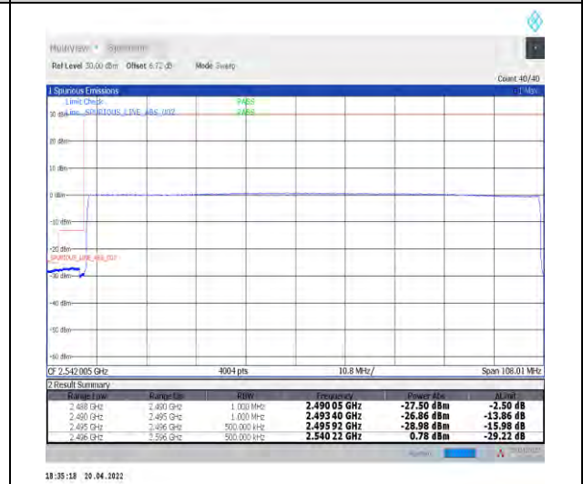
1-N41--30-100-L-6-CP-QPSK-Outer_Full-273@0-Ant0-PASS-see graph
