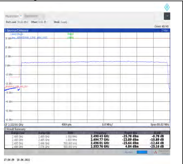
1-N41--30-80-L-3-DFT-PI2BPSK-Outer_Full-216@0-Ant0-PASS-see graph
