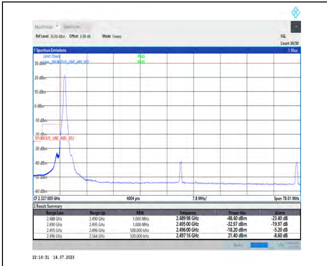
1-N41-PC1-30-70-L-1-DFT-PI2BPSK-Edge_1RB_Left-1@0-Ant0-1--PASS-see graph
