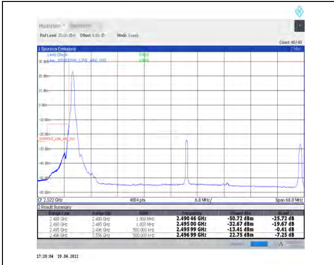
1-N41--30-60-L-1-DFT-PI2BPSK-Edge_1RB_Left-1@0-Ant0-PASS-see graph
