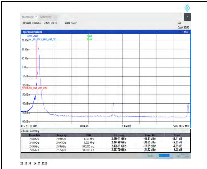
1-N41-PC1-30-80-L-1-DFT-PI2BPSK-Edge_1RB_Left-1@0-Ant0-1--PASS-see graph
