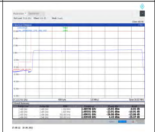
1-N41--30-50-L-6-CP-QPSK-Outer_Full-133@0-Ant0-PASS-see graph
