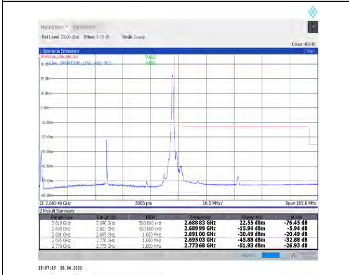
1-N41--30-80-H-5-CP-QPSK-Edge_1RB_Right-1@216 -Ant0-PASS-see graph
