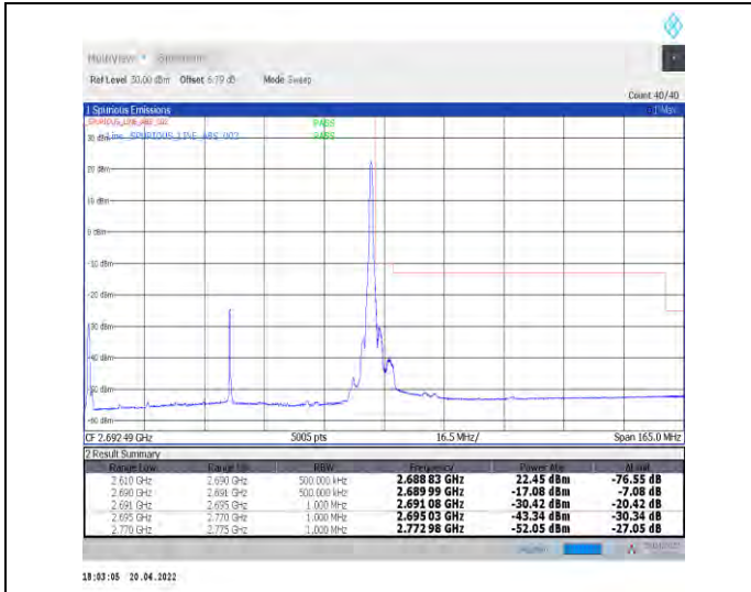
1-N41--30-80-H-2-DFT-PI2BPSK-Edge_1RB_Right-1@ 216-Ant0-PASS-see graph
