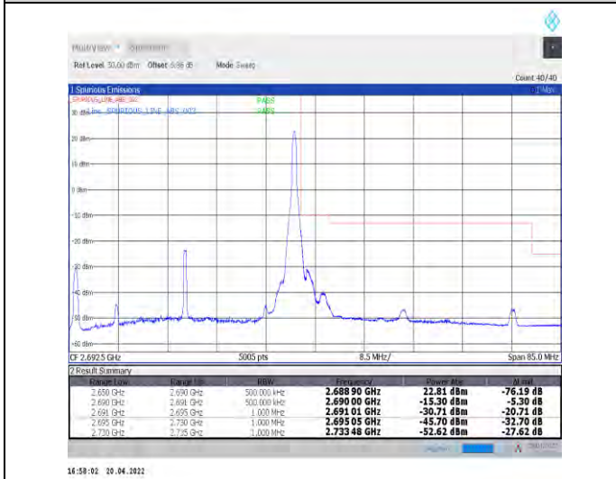
1-N41--30-40-H-5-CP-QPSK-Edge_1RB_Right-1@105-Ant0-PASS-see graph
