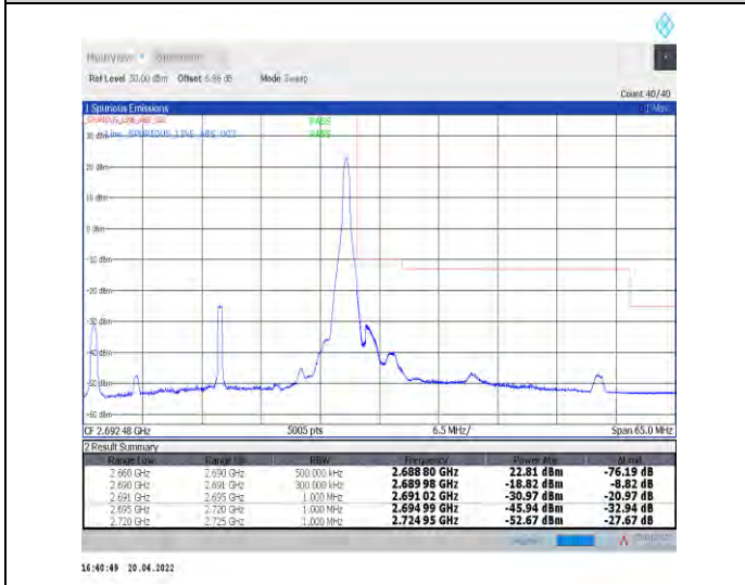
1-N41--30-30-H-5-CP-QPSK-Edge_1RB_Right-1@77-Ant0-PASS-see graph
