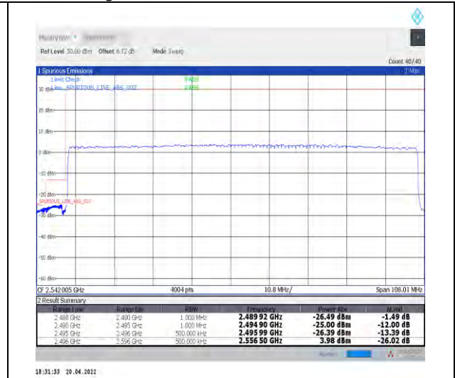
1-N41--30-100-L-3-DFT-PI2BPSK-Outer_Full-270@0-Ant0-PASS-see graph
