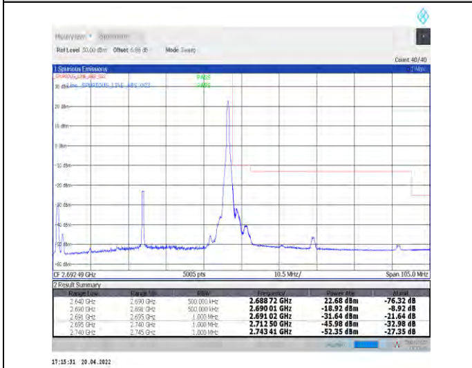
1-N41--30-50-H-5-CP-QPSK-Edge_1RB_Right-1@132-Ant0-PASS-see graph
