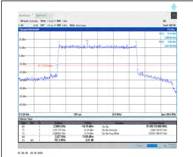
1-N41-PC1-30-100-H-7-CP-16QAM-Outer_Full-273 @0-Ant0-97.492-101.200-≤100-PASS
