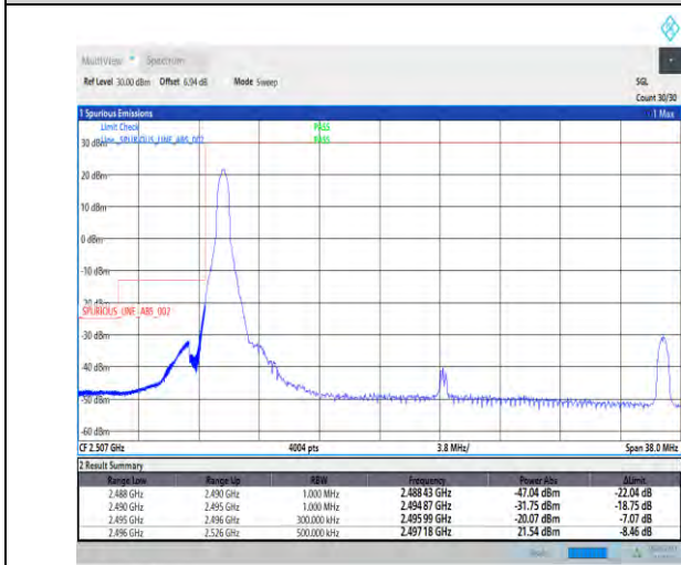
1-N41-PC1-30-30-L-1-DFT-PI2BPSK-Edge_1RB_Left-1@0-Ant0-1--PASS-see graph
