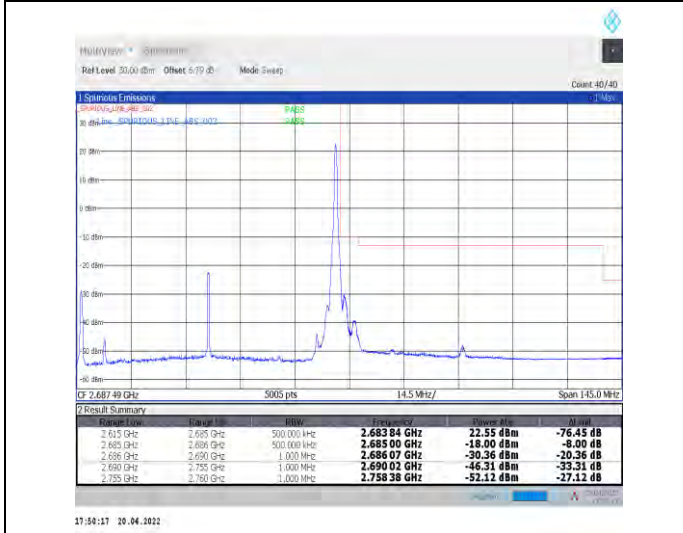
1-N41--30-70-H-5-CP-QPSK-Edge_1RB_Right-1@188-Ant0-PASS-see graph
