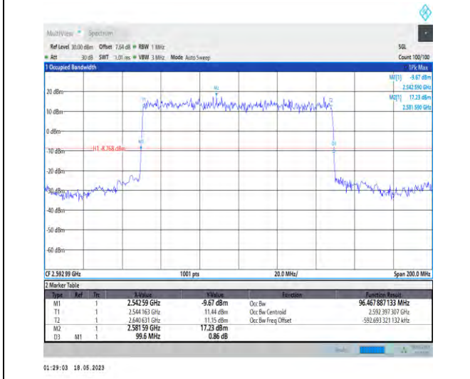
1-N41-PC1-30-100-M-2-DFT-PI2BPSK-Outer_Full-270 @0-Ant0-96.468-99.600-≤100-PASS
