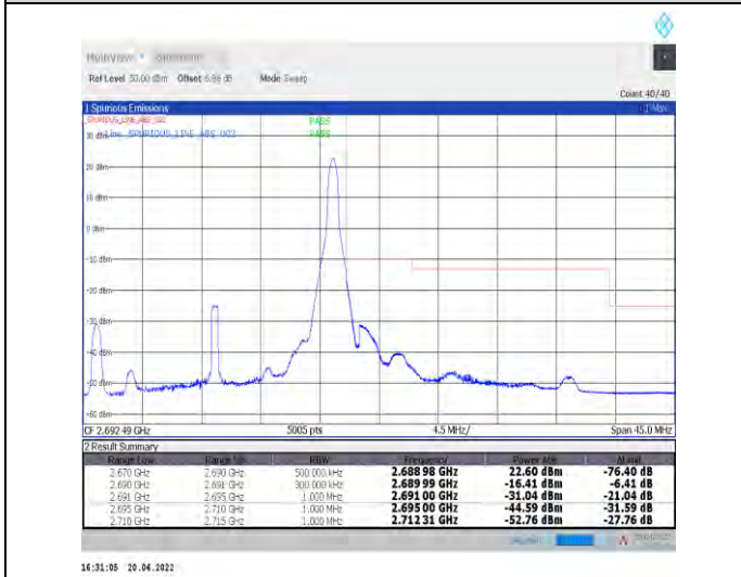
1-N41--30-20-H-5-CP-QPSK-Edge_1RB_Right-1@50-Ant0-PASS-see graph
