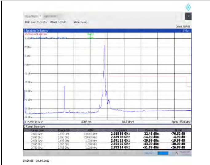
1-N41--30-90-H-2-DFT-PI2BPSK-Edge_1RB_Right-1@244-Ant0-PASS-see graph
