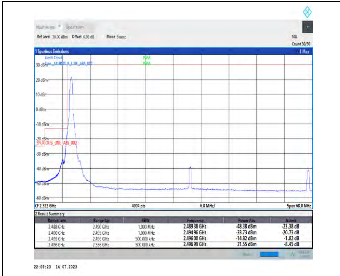
1-N41-PC1-30-60-L-1-DFT-PI2BPSK-Edge_1RB_Left-1@0-Ant0-1--PASS-see graph
