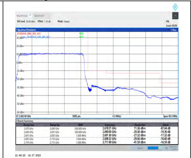
1-N41-PC1-30-20-H-3-DFT-PI2BPSK-Outer_Full-5 0@0-Ant0-1--PASS-see graph
