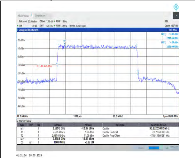
1-N41-PC1-30-100-H-4-DFT-64QAM-Outer_Full-270 @0-Ant0-96.233-100.000-≤100-PASS
