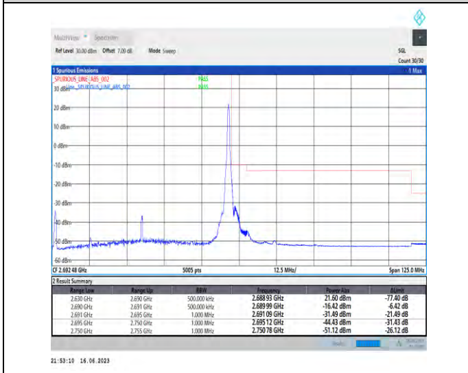
1-N41-PC1-30-60-H-5-CP-QPSK-Edge_1RB_Right-1@161-Ant0-1--PASS-see graph
