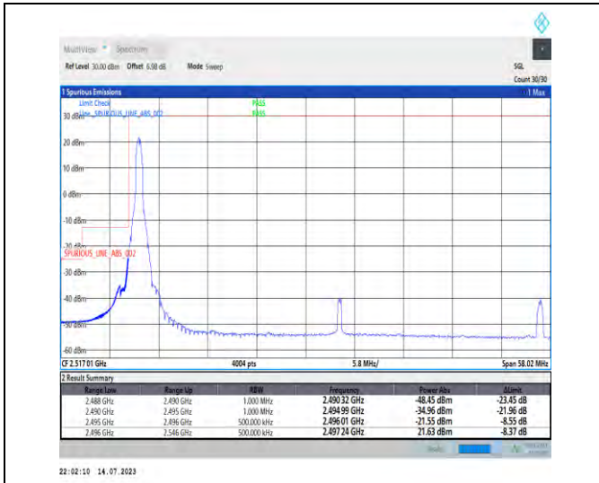
1-N41-PC1-30-50-L-1-DFT-PI2BPSK-Edge_1RB_Left-1@0-Ant0-1--PASS-see graph
