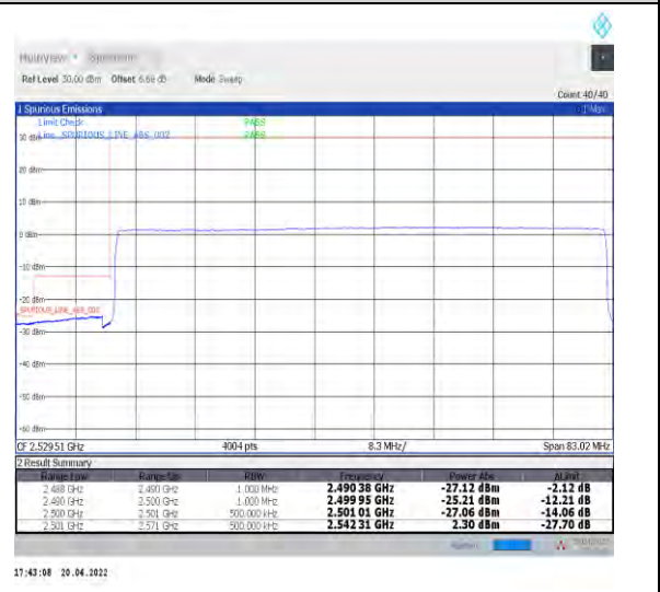
1-N41--30-70-L-6-CP-QPSK-Outer_Full-189@0-Ant0-PASS-see graph
