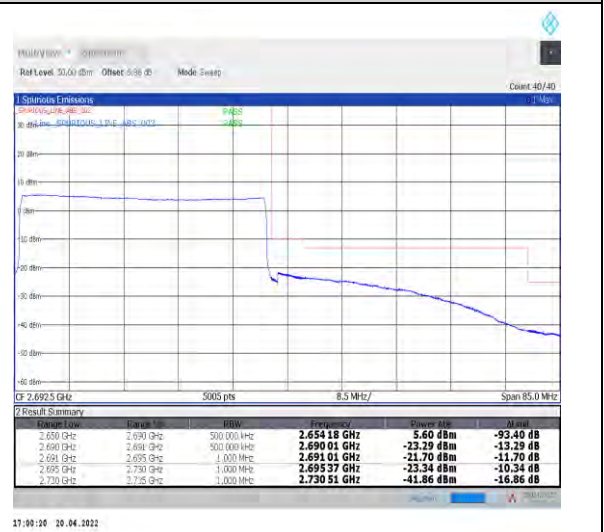
1-N41--30-40-H-6-CP-QPSK-Outer_Full-106@0-Ant0-PASS-see graph
