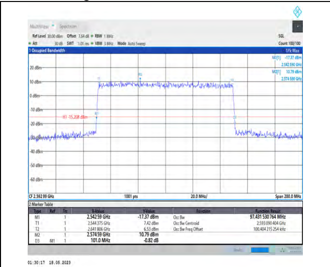
1-N41-PC1-30-100-M-9-CP-256QAM-Outer_Full-273 @0-Ant0-97.432-101.000-≤100-PASS
