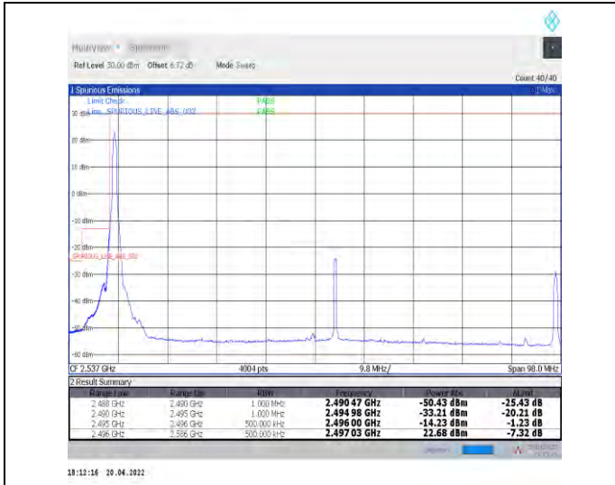
1-N41--30-90-L-1-DFT-PI2BPSK-Edge_1RB_Left-1@0-Ant0-PASS-see graph
