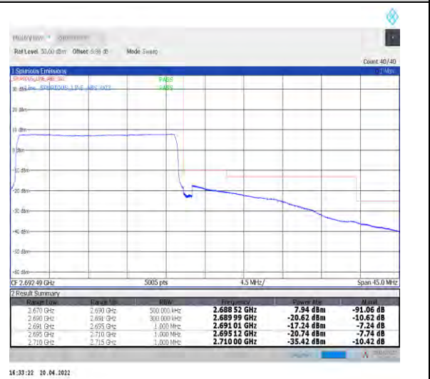
1-N41--30-20-H-6-CP-QPSK-Outer_Full-51@0-Ant0-PASS-see graph
