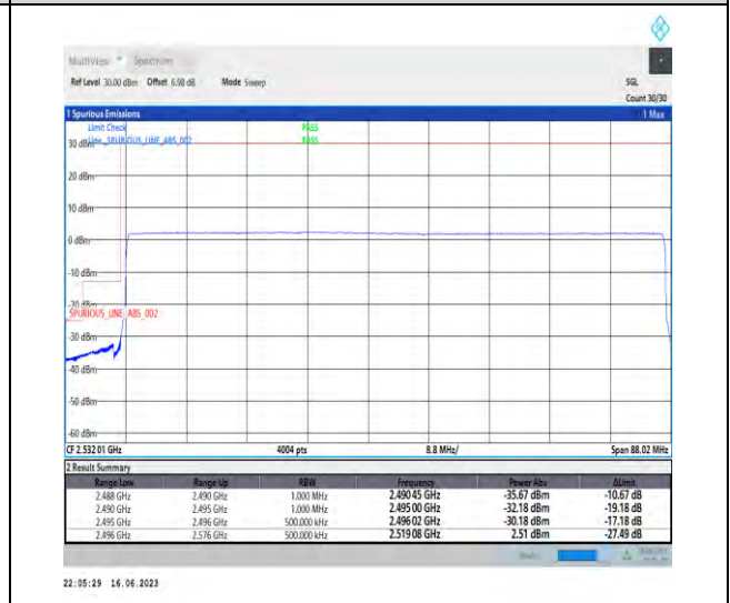
1-N41-PC1-30-80-L-6-CP-QPSK-Outer_Full-217@0-Ant0-1--PASS-see graph
