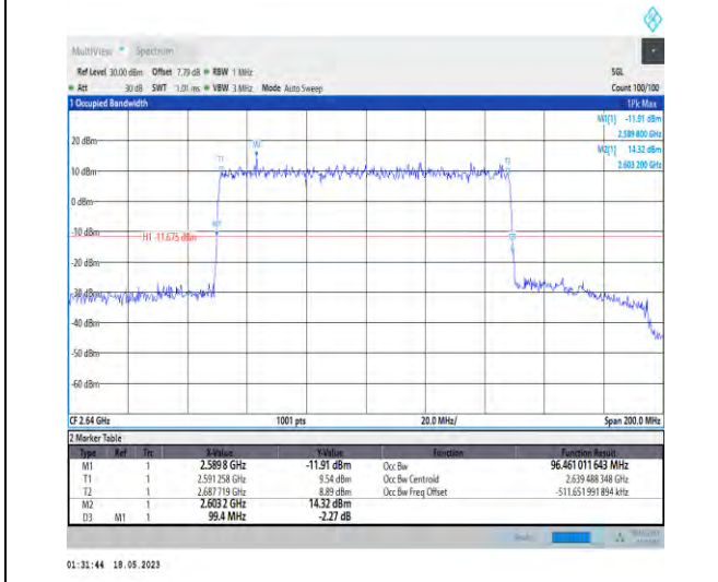
1-N41-PC1-30-100-H-5-DFT-256QAM-Outer_Full-270 @0-Ant0-96.461-99.400-≤100-PASS
