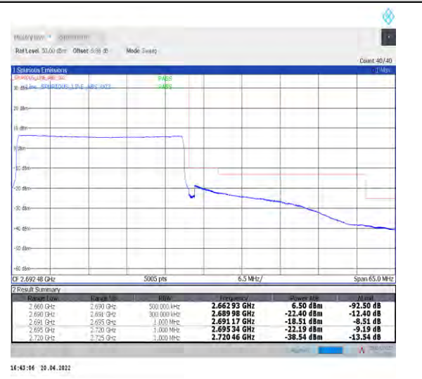
1-N41--30-30-H-6-CP-QPSK-Outer_Full-78@0-Ant0-PASS-see graph
