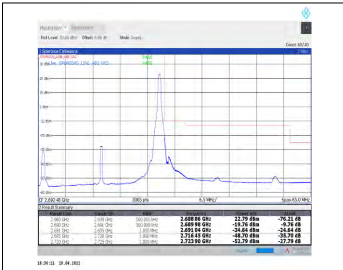
1-N41--30-30-H-2-DFT-PI2BPSK-Edge_1RB_Right-1@77-Ant0-PASS-see graph
