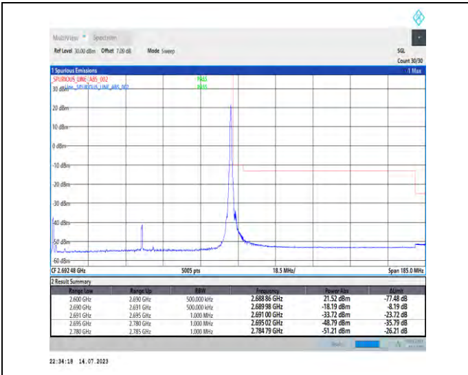
1-N41-PC1-30-90-H-2-DFT-PI2BPSK-Edge_1RB_Right-t-1@244-Ant0-1--PASS-see graph
