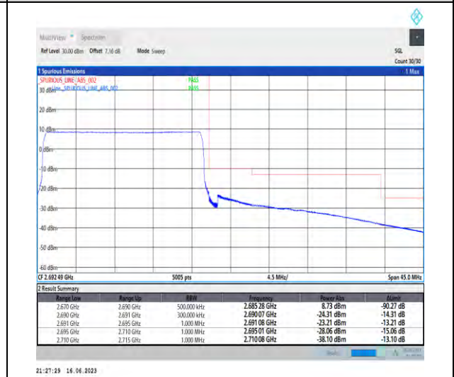
1-N41-PC1-30-20-H-6-CP-QPSK-Outer_Full-51 @0-Ant0-1--PASS-see graph
