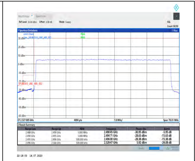
1-N41-PC1-30-70-L-3-DFT-PI2BPSK-Outer_Full-180@0-Ant0-1--PASS-see graph
