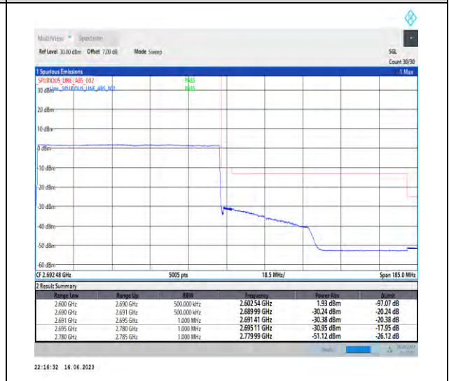
1-N41-PC1-30-90-H-6-CP-QPSK-Outer_Full-245@0-Ant0-1--PASS-see graph
