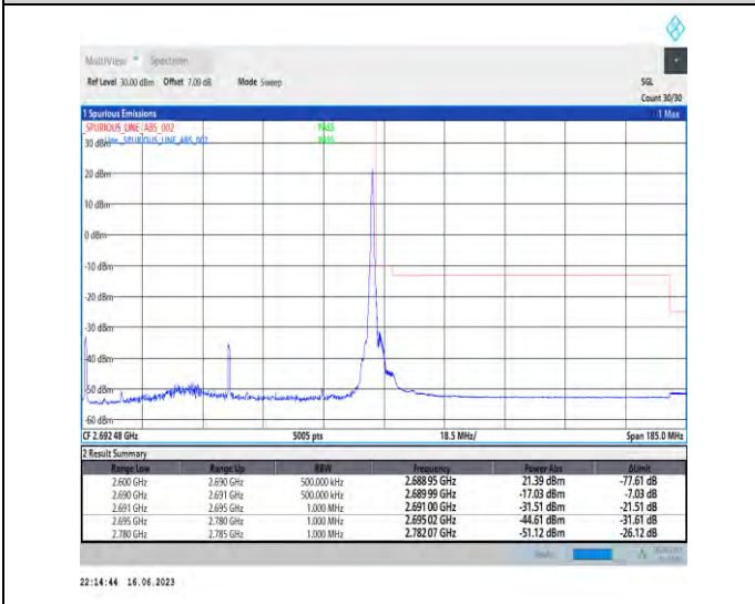
1-N41-PC1-30-90-H-5-CP-QPSK-Edge_1RB_Right-1@244-Ant0-1--PASS-see graph
