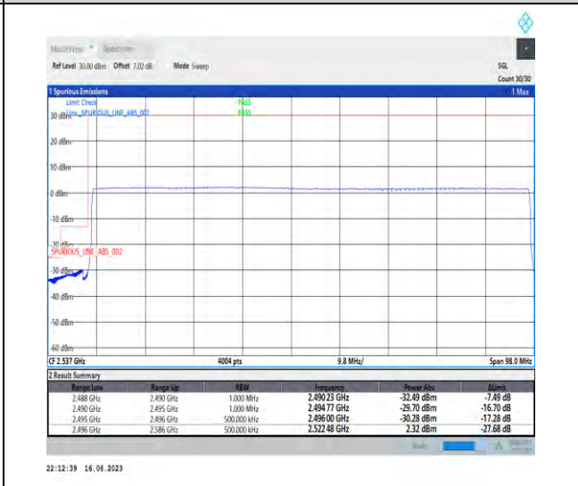
1-N41-PC1-30-90-L-6-CP-QPSK-Outer_Full-245@0-Ant0-1--PASS-see graph
