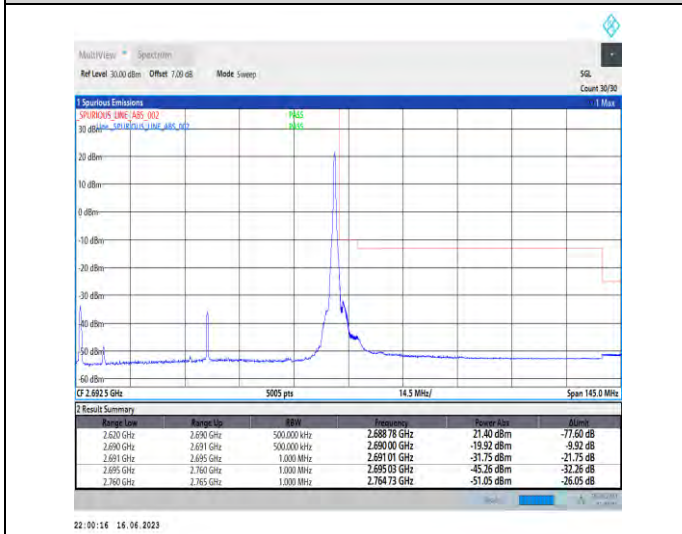
1-N41-PC1-30-70-H-5-CP-QPSK-Edge_1RB_Right-1@188-Ant0-1--PASS-see graph
