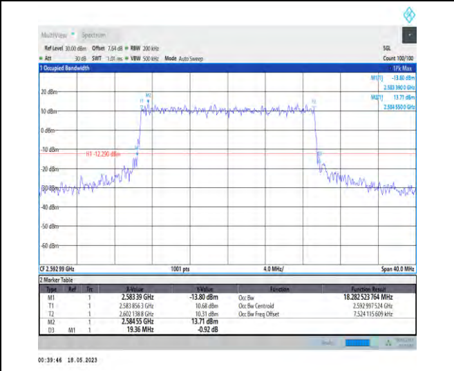
1-N41-PC1-30-20-M-7-CP-16QAM-Outer_Full-51@0- -Ant0-18.283-19.360-<=20-PASS
