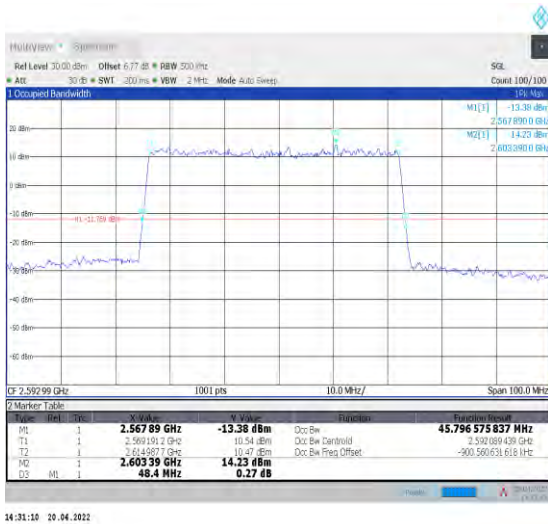
1-N41--30-50-M-5-DFT-256QAM-Outer_Full-128@0-Ant0-45.797-48.400-≤50-PASS
