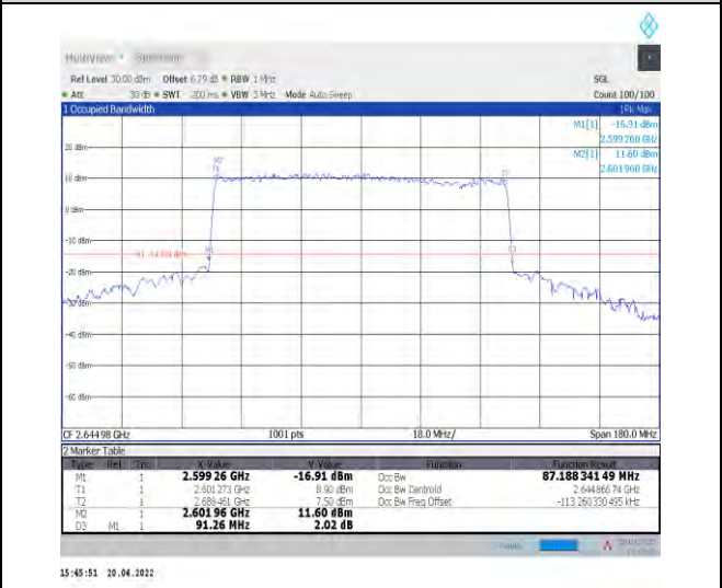
1-N41--30-90-H-9-CP-256QAM-Outer_Full-245@0-Ant t0-87.188-91.260-≤90-PASS
