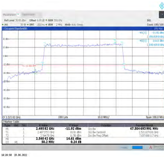
1-N41--30-50-L-6-CP-QPSK-Outer_Full-133@0-Ant0 -47.505-50.200-≤50-PASS
