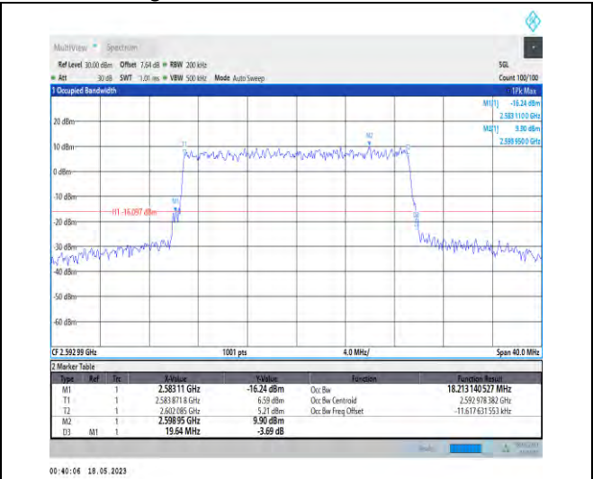
1-N41-PC1-30-20-M-9-CP-256QAM-Outer_Full-51@0 -Ant0-18.213-19.640-≤20-PASS
