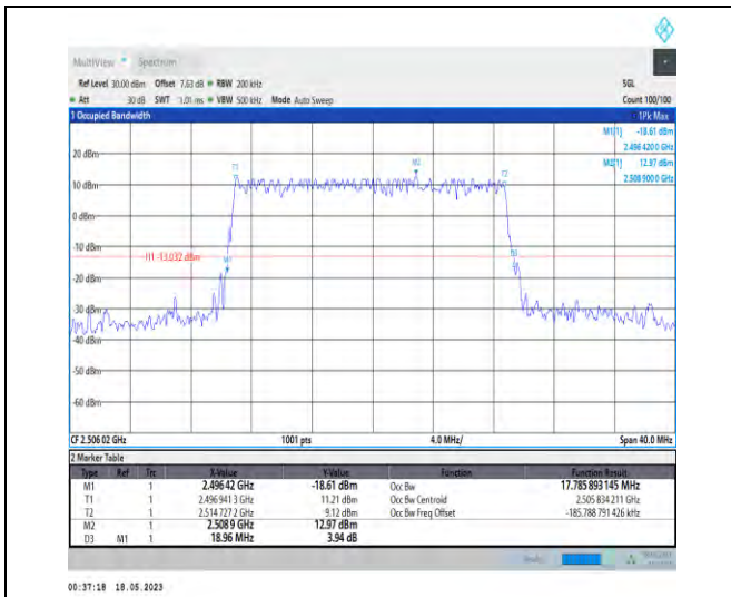
1-N41-PC1-30-20-L-5-DFT-256QAM-Outer_Full-50 @0-Ant0-17.786-18.960-≤20-PASS
