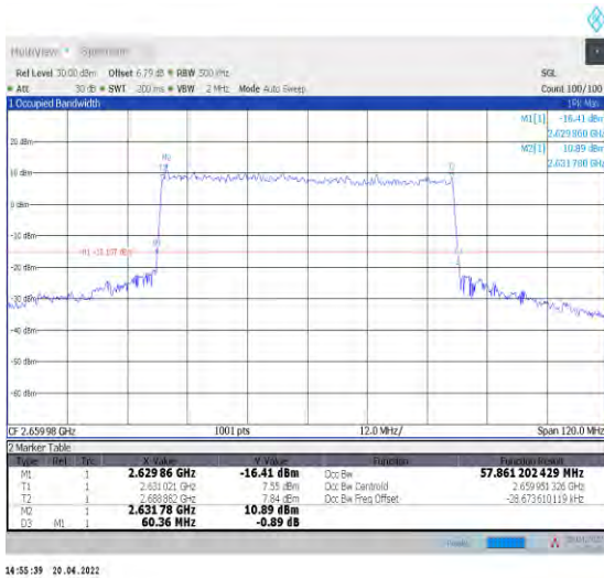
1-N41--30-60-H-9-CP-256QAM-Outer_Full-162@0-A nt0-57.861-60.360-≤60-PASS
