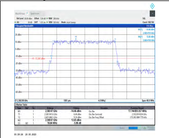
1-N41-PC1-30-20-M-5-DFT-256QAM-Outer_Full-50@ @0-Ant0-17.745-18.840-<=20-PASS
