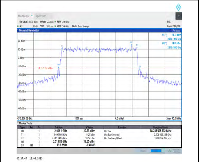
1-N41-PC1-30-20-L-8-CP-64QAM-Outer_Full-51@0-Ant0-18.237-19.800-≤20-PASS
