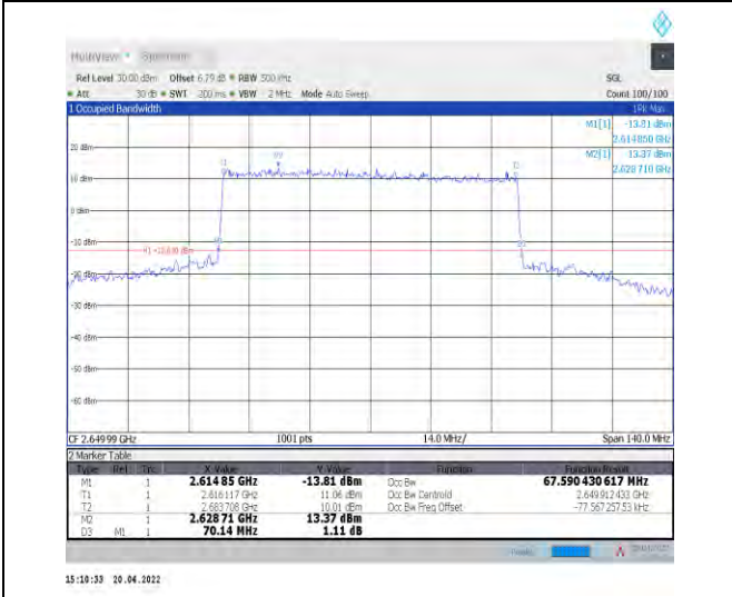
1-N41--30-70-H-6-CP-QPSK-Outer_Full-189@0-Ant0-67.59-70.140-≤70-PASS
