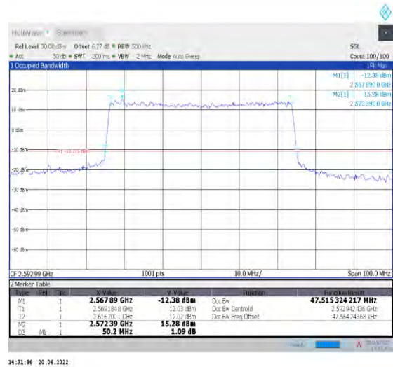
1-N41--30-50-M-6-CP-QPSK-Outer_Full-133@0-Ant0-47.515-50.200-≤50-PASS
