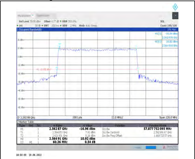
1-N41--30-60-M-9-CP-256QAM-Outer_Full-162@0-Ant0 t0-57.878-60.360-≤60-PASS
