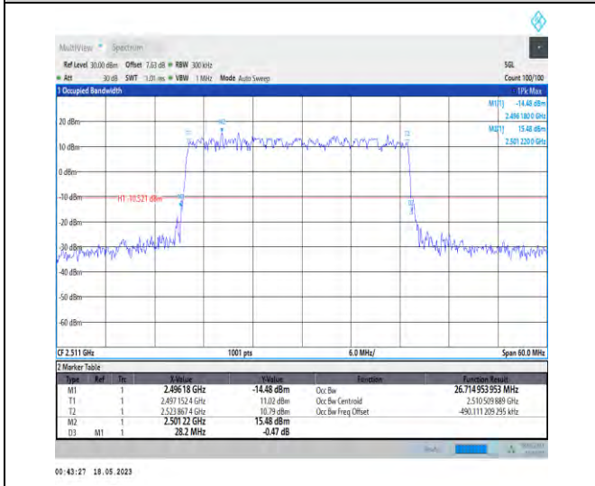
1-N41-PC1-30-30-L-4-DFT-64QAM-Outer_Full-75 @0-Ant0-26.715-28.200-≤30-PASS
