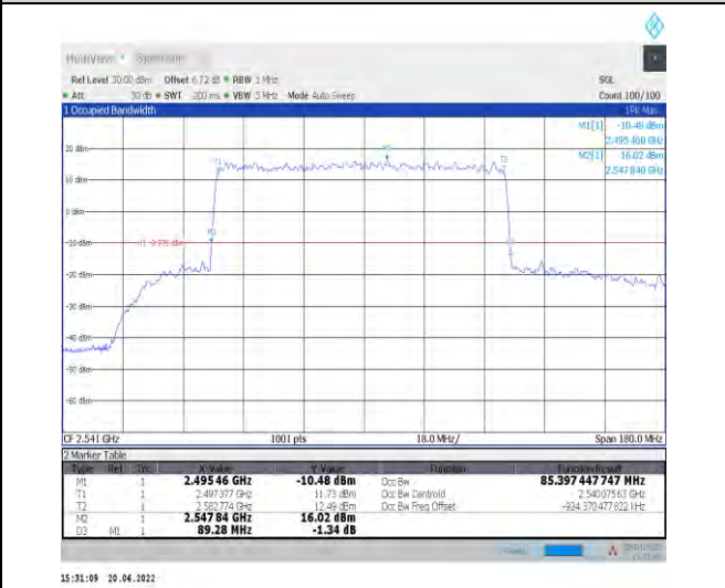
1-N41--30-90-L-3-DFT-16QAM-Outer_Full-240@0-A nt0-85.397-89.280-≤90-PASS
