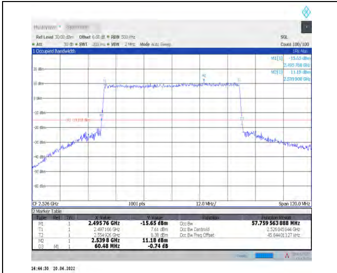
1-N41--30-60-L-9-CP-256QAM-Outer_Full-162@0-A nt0-57.76-60.480-≤60-PASS
