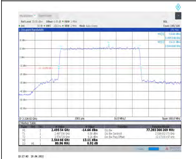
1-N41--30-80-L-9-CP-256QAM-Outer_Full-217@0-A nt0-77.393-80.960-≤80-PASS
