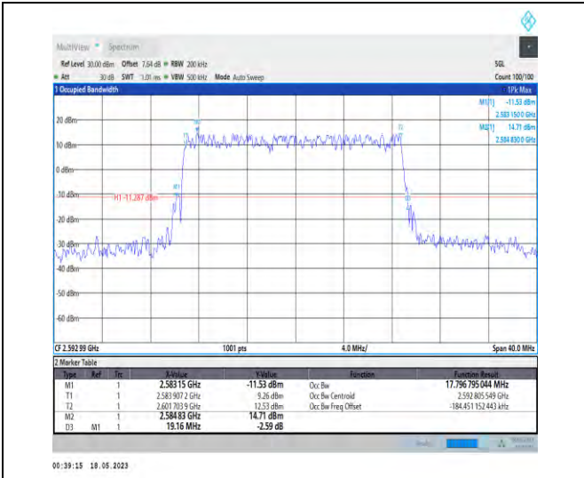
1-N41-PC1-30-20-M-4-DFT-64QAM-Outer_Full-50@ 0-Ant0-17.797-19.160-<=20-PASS
