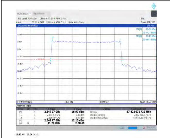
1-N41--30-90-M-9-CP-256QAM-Outer_Full-245@0-A nt0-87.423-91.260-<=90-PASS
