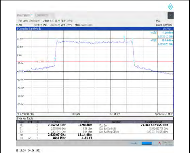
1-N41--30-80-M-1-DFT-QPSK-Outer_Full-216@0-An t0-77.343-80.800-≤80-PASS
