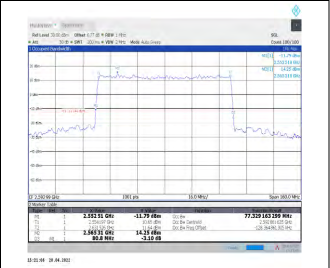
1-N41--30-80-M-5-DFT-256QAM-Outer_Full-216@0-Ant0-77.329-80.800-≤80-PASS
