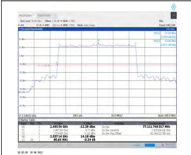
1-N41--30-80-L-5-DFT-256QAM-Outer_Full-216@0-A Ant0-77.112-80.640-<=80-PASS
