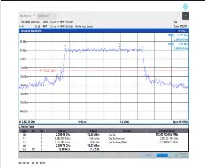
1-N41-PC1-30-20-M-6-CP-QPSK-Outer_Full-51@0- Ant0-18.241-19.480-<=20-PASS
