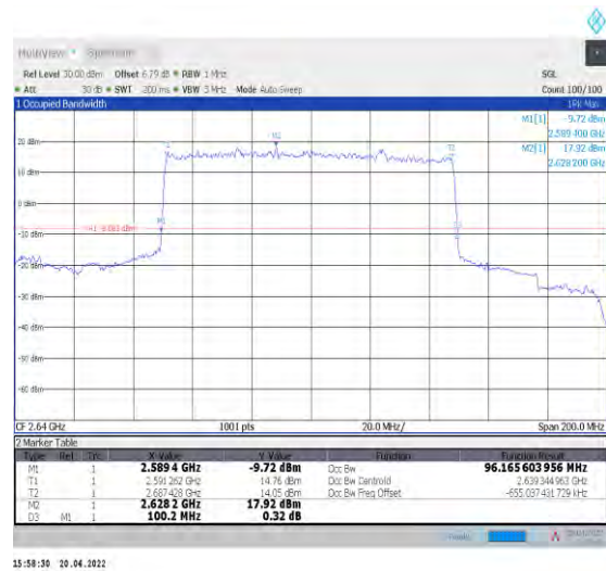
1-N41--30-100-H-2-DFT-PI2BPSK-Outer_Full-270@ 0-Ant0-96.166-100.200-≤100-PASS
