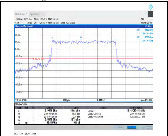
1-N41-PC1-30-20-L-6-CP-QPSK-Outer_Full-51@0-Ant0-18.145-19.440-≤20-PASS
