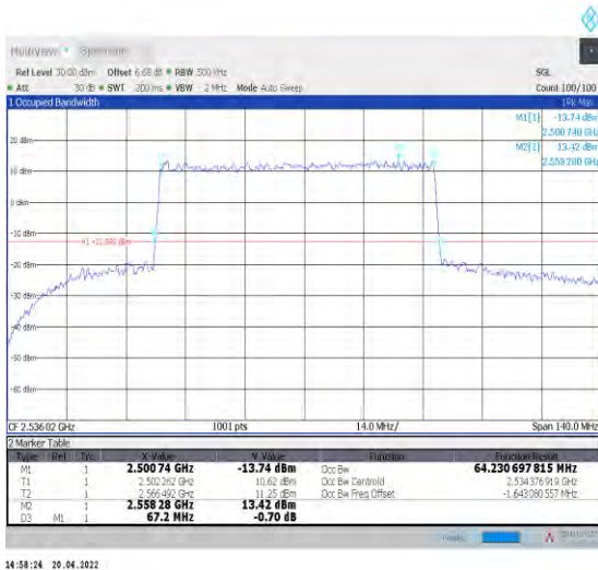
1-N41--30-70-L-4-DFT-64QAM-Outer_Full-180@0-Ant0-64.231-67.200-<=70-PASS
