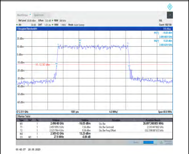
1-N41-PC1-30-30-L-5-DFT-256QAM-Outer_Full-75 @0-Ant0-26.697-27.900-≤30-PASS
