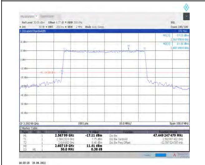
1-N41--30-50-M-9-CP-256QAM-Outer_Full-133@0-A nt0-47.449-50.000-<=50-PASS
