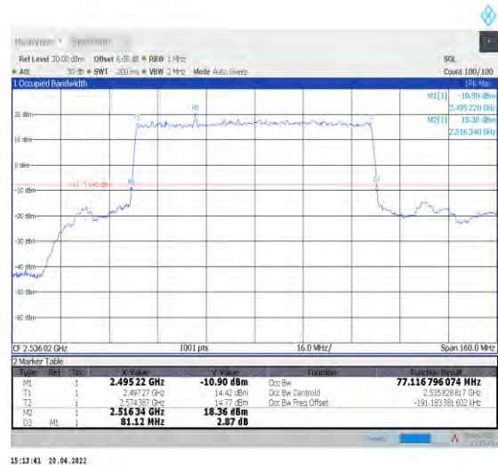
1-N41--30-80-L-2-DFT-PI2BPSK-Outer_Full-216@0-Ant 0-77.117-81.120-≤80-PASS
