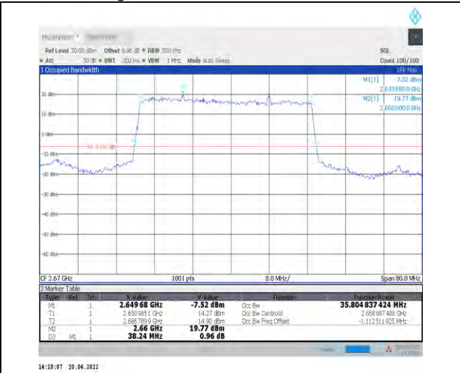
1-N41--30-40-H-2-DFT-PI2BPSK-Outer_Full-100@0-Ant0-35.805-38.240-≤40-PASS
