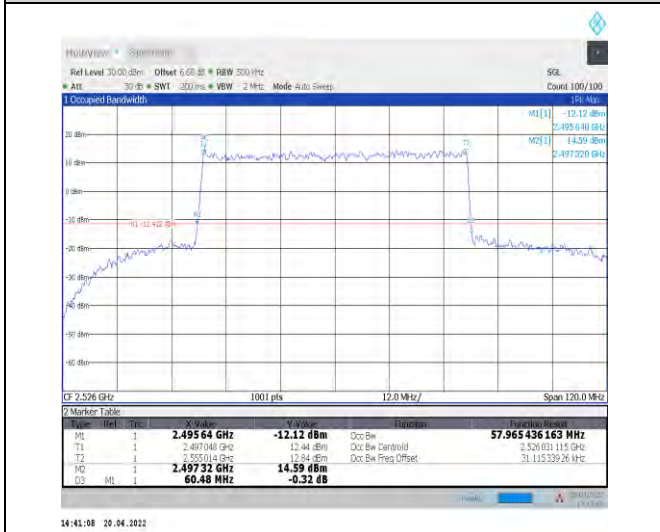
1-N41--30-60-L-3-DFT-16QAM-Outer_Full-162@0-A nt0-57.965-60.480-≤60-PASS
