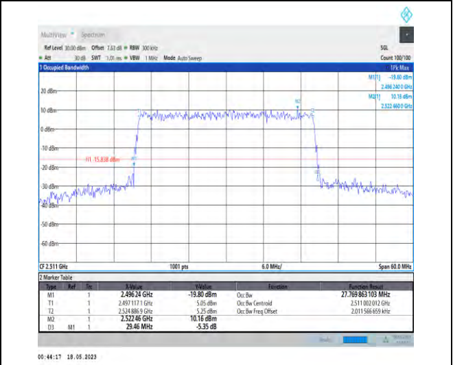
1-N41-PC1-30-30-L-9-CP-256QAM-Outer_Full-78@0-Ant0-27.77-29.460-≤30-PASS
