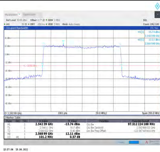
1-N41--30-100-M-9-CP-256QAM-Outer_Full-273@0- Ant0-97.512-101.200-≤100-PASS
