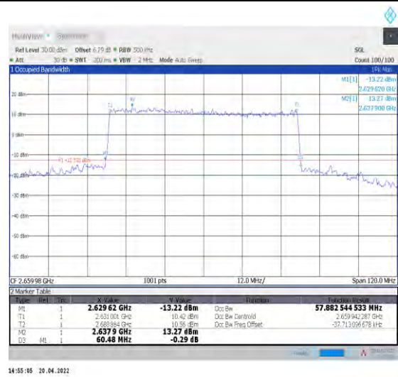
1-N41--30-60-H-8-CP-64QAM-Outer_Full-162@0-An t0-57.883-60.480-≤60-PASS
