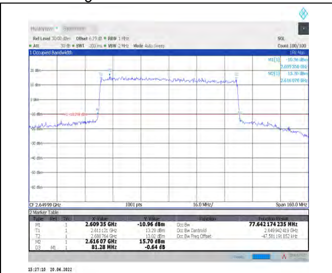
1-N41--30-80-H-6-CP-QPSK-Outer_Full-217@0-Ant 0-77.642-81.280-<math>\leq 80</math>-PASS
