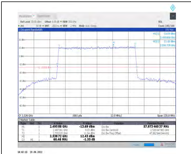
1-N41--30-60-L-5-DFT-256QAM-Outer_Full-162@0-Ant0-57.973-60.480-≤60-PASS
