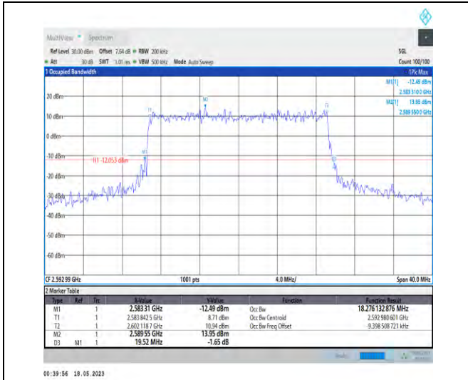
1-N41-PC1-30-20-M-8-CP-64QAM-Outer_Full-51@0 -Ant0-18.276-19.520-≤20-PASS
