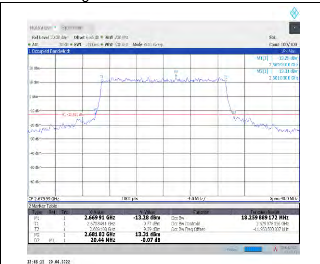
1-N41--30-20-H-8-CP-64QAM-Outer_Full-51@0-Ant 0-18.26-20.440-≤20-PASS
