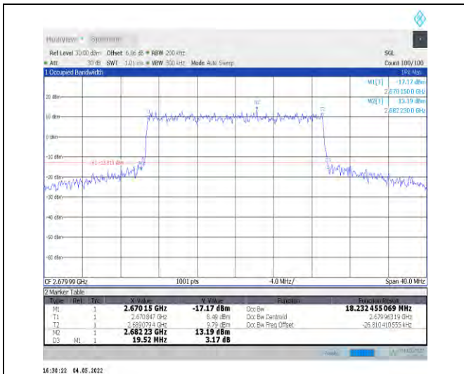
1-N41--30-20-H-7-CP-16QAM-Outer_Full-51@0-Ant 0-18.232-19.520-≤20-PASS
