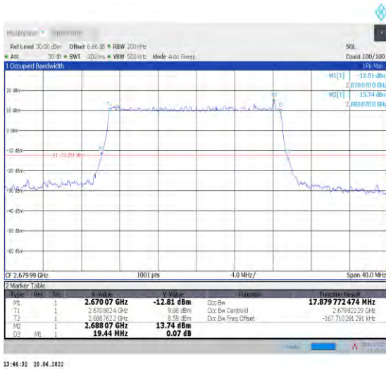
1-N41--30-20-H-5-DFT-256QAM-Outer_Full-50@0-A nt0-17.88-19.440-<=20-PASS
