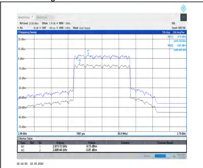
1-N41-PC1-30-100-H-2-CP-256QAM-Outer_Full-273@0-Ant0-9.96-19.56%-7.09-2.87-PASS-≤13
