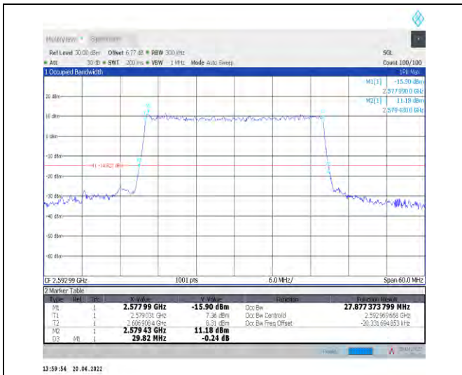
1-N41--30-30-M-9-CP-256QAM-Outer_Full-78@0-Ant t0-27.877-29.820-<30-PASS
