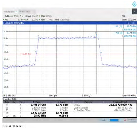
1-N41--30-30-L-5-DFT-256QAM-Outer_Full-75@0-A nt0-26.823-28.920-≤30-PASS
