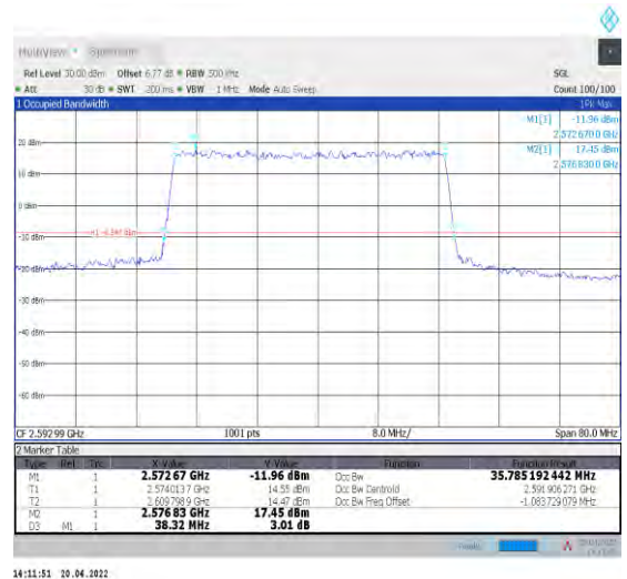
1-N41--30-40-M-1-DFT-QPSK-Outer_Full-100@0-An t0-35.785-38.320-≤40-PASS
