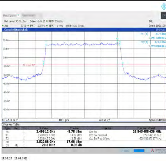
1-N41--30-30-L-2-DFT-PI2BPSK-Outer_Full-75@0-A nt0-26.845-28.800-≤30-PASS
