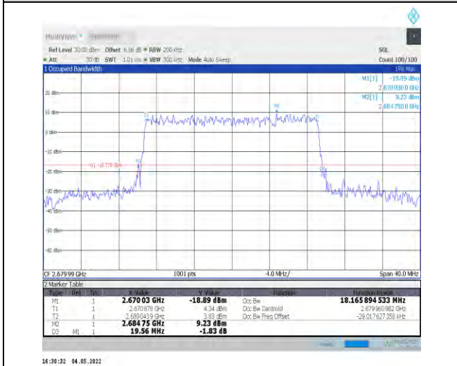
1-N41--30-20-H-9-CP-256QAM-Outer_Full-51@0-Ant t0-18.166-19.560-≤20-PASS
