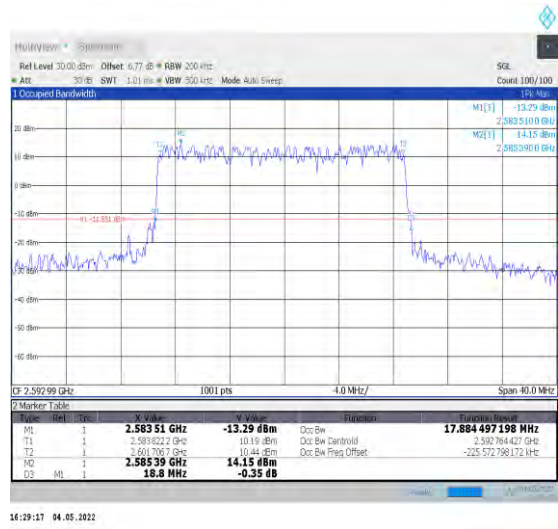
1-N41--30-20-M-3-DFT-16QAM-Outer_Full-50@0-Ant 0-17.884-18.800-≤20-PASS
