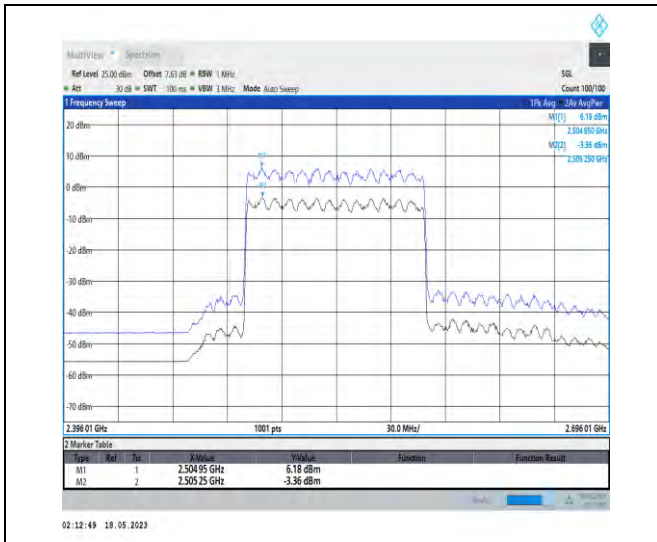
1-N41-PC1-30-100-L-1-DFT-256QAM-Outer_Full-270@0-Ant0-9.54-19.56%-7.09-2.45-PASS-≤13
