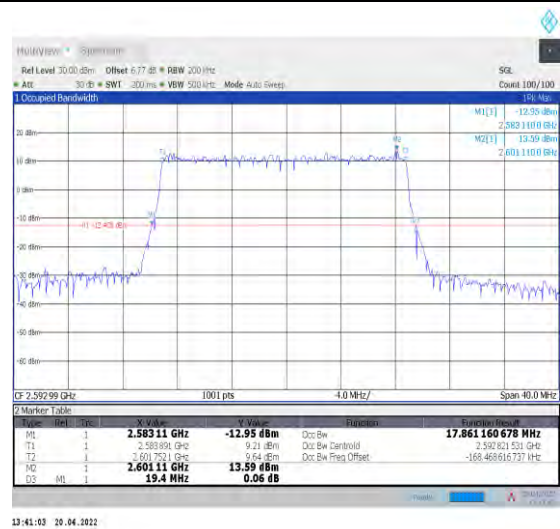
1-N41--30-20-M-5-DFT-256QAM-Outer_Full-50@0-Ant0-17.861-19.400-<=20-PASS
