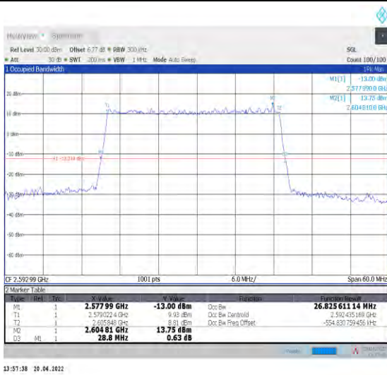
1-N41--30-30-M-5-DFT-256QAM-Outer_Full-75@0-A nt0-26.826-28.800-≤30-PASS
