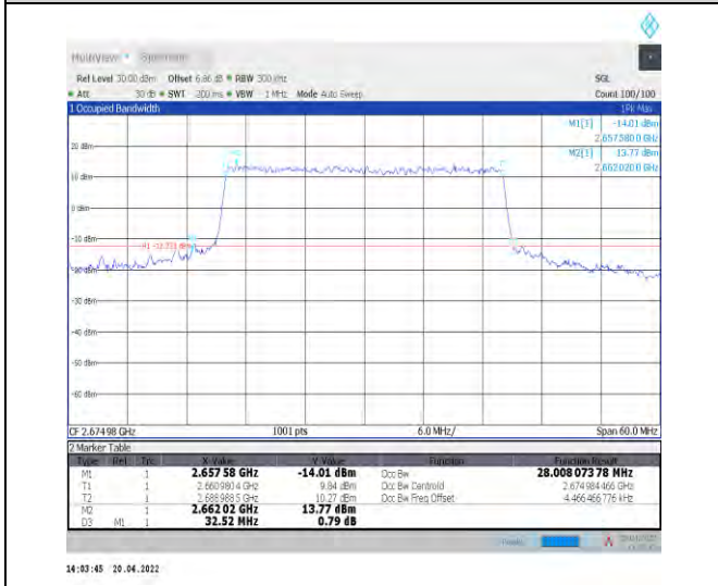
1-N41--30-30-H-6-CP-QPSK-Outer_Full-78@0-Ant-28.008-32.520-<30-PASS
