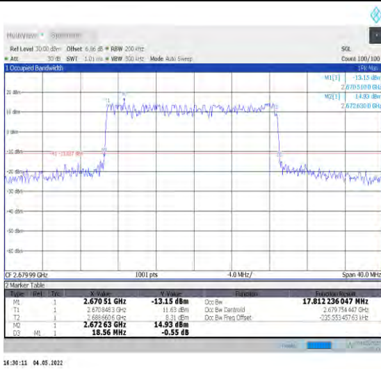
1-N41--30-20-H-3-DFT-16QAM-Outer_Full-50@0-An t0-17.812-18.560-<=20-PASS
