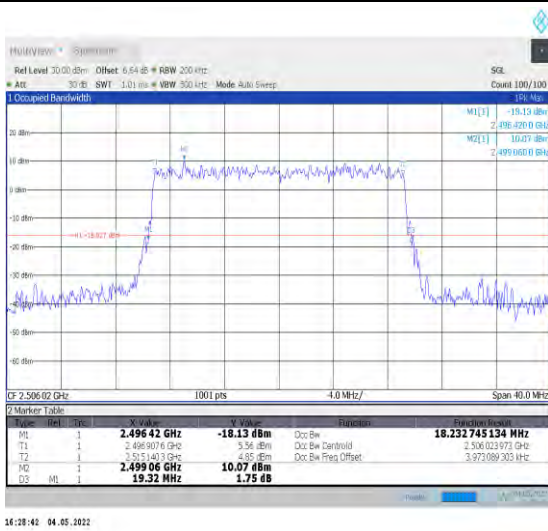
1-N41--30-20-L-9-CP-256QAM-Outer_Full-51@0-Ant 0-18.233-19.320-≤20-PASS
