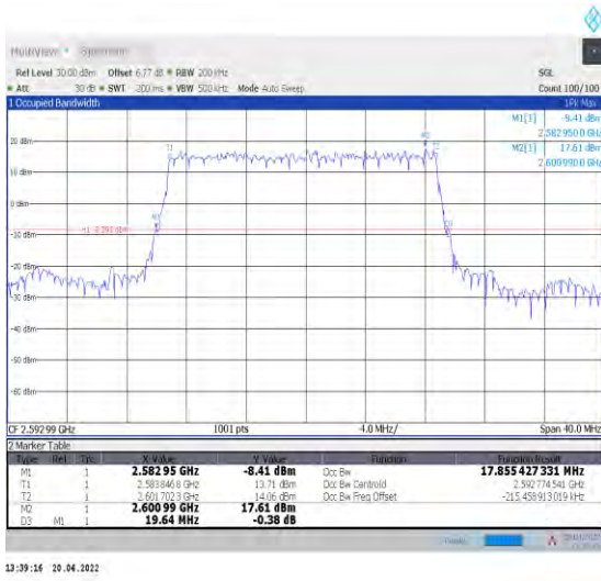
1-N41--30-20-M-2-DFT-16QAM-Outer_Full-50@0-Ant 0-17.855-19.640-≤20-PASS
