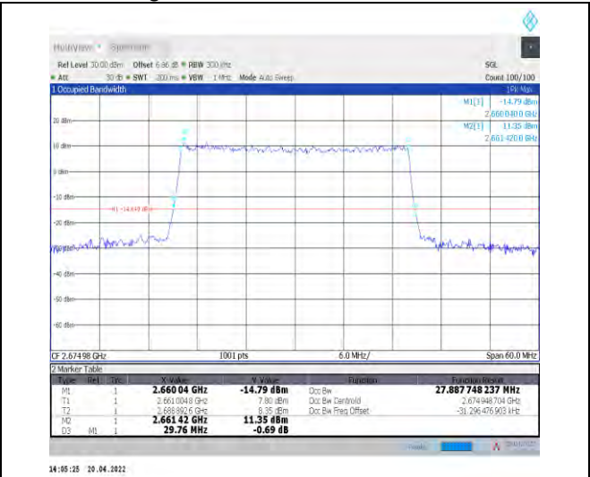
1-N41--30-30-H-9-CP-256QAM-Outer_Full-78@0-An t0-27.888-29.760-≤30-PASS
