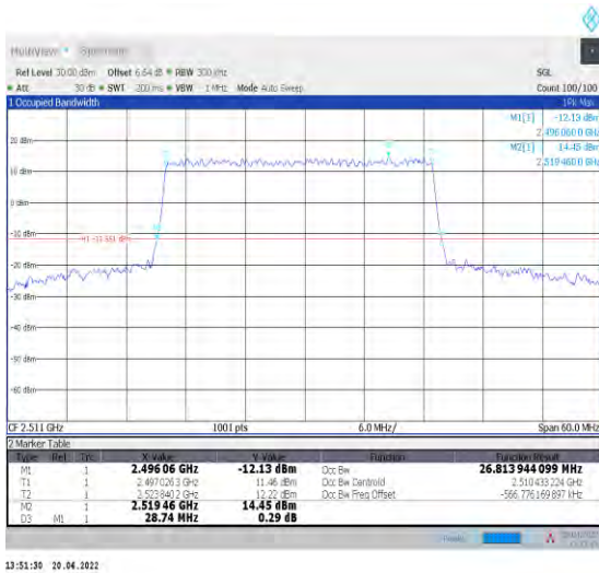
1-N41--30-30-L-4-DFT-64QAM-Outer_Full-75@0-Ant 0-26.814-28.740-≤30-PASS
