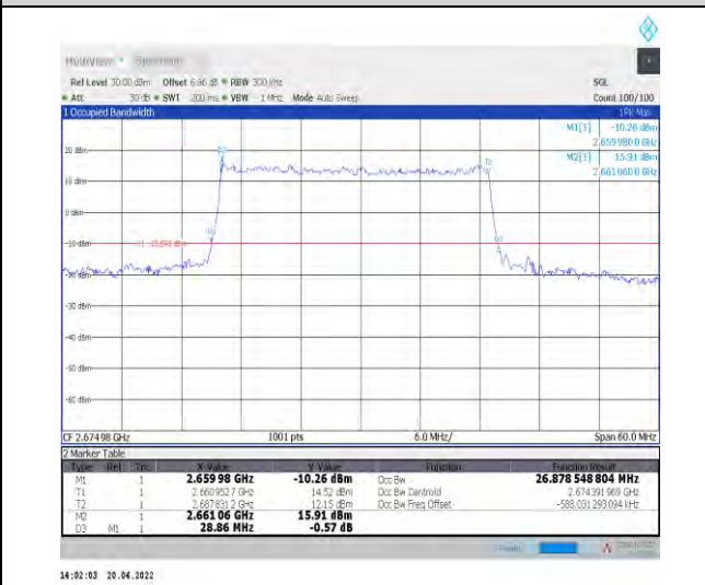
1-N41--30-30-H-3-DFT-16QAM-Outer_Full-75@0-Ant t0-26.879-28.860-<30-PASS
