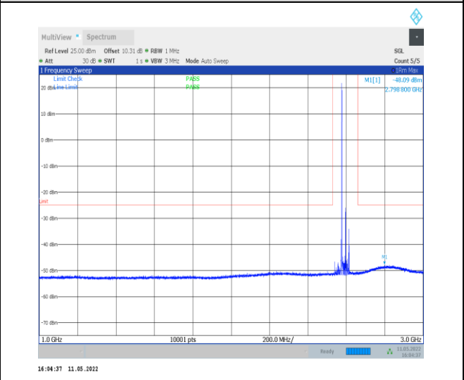
1-N38-PC2-30-40-M-1-DFT-QPSK-Edge_1RB_Left-1 @0-1000-3000-Ant0--48.09--25-PASS
