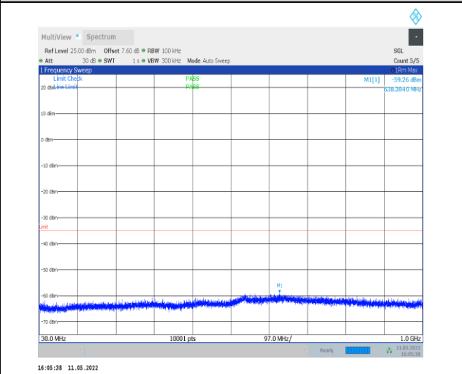
1-N38-PC2-30-40-H-1-DFT-QPSK-Edge_1RB_Left-1 @ 0-30-1000-Ant0--59.26--35-PASS
