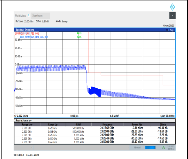
1-N38-PC2-30-30-H-6-CP-QPSK-Outer_Full-78@0-Ant0-PASS-see graph
