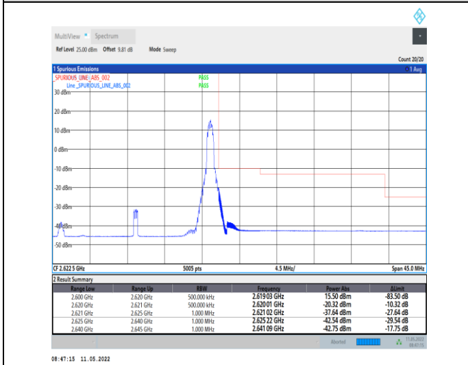
1-N38-PC2-30-20-H-5-CP-QPSK-Edge_1RB_Right-1@50-Ant0-PASS-see graph
