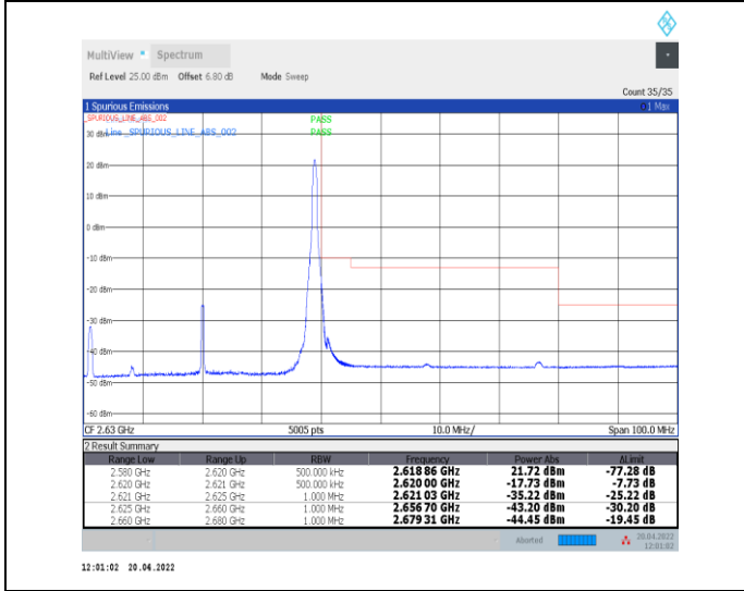
1-N38--30-40-H-5-CP-QPSK-Edge_1RB_Right-1@105-Ant0-PASS-see graph
