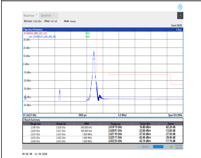
1-N38-PC2-30-30-H-5-CP-QPSK-Edge_1RB_Right-1@77-Ant0-PASS-see graph
