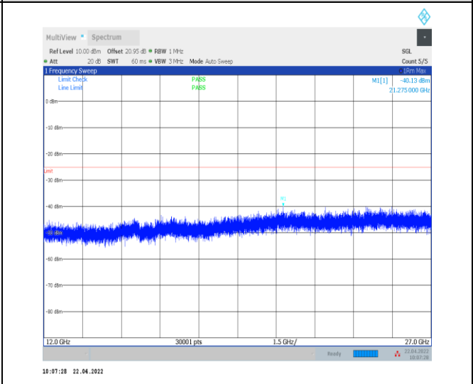
1-N38--30-40-M-1-DFT-PI2BPSK-Inner_1RB_Left-1 @ 1-12000-27000-Ant0--40.13--25-PASS
