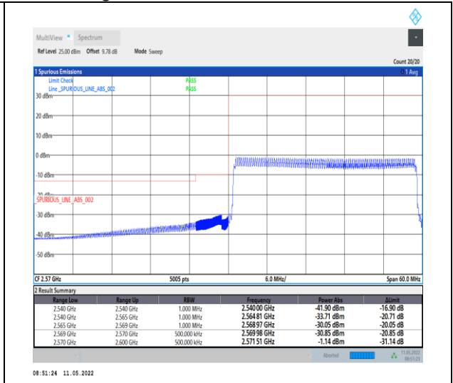
1-N38-PC2-30-30-L-6-CP-QPSK-Outer_Full-78@0-Ant0-PASS-see graph
