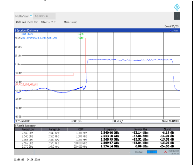
1-N38--30-40-L-3-DFT-PI2BPSK-Outer_Full-100@0-Ant0-PASS-see graph
