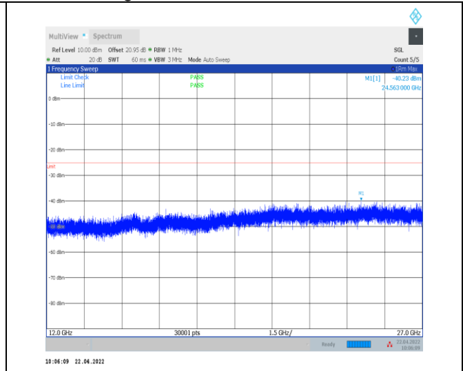
1-N38--30-40-L-1-DFT-PI2BPSK-Inner_1RB_Left-1 @ 1-12000-27000-Ant0--40.23--25-PASS
