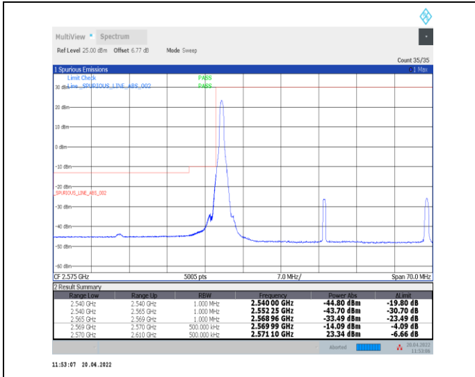
1-N38--30-40-L-1-DFT-PI2BPSK-Edge_1RB_Left-1@0-Ant0-PASS-see graph
