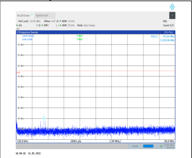
1-N38-PC2-30-40-M-1-DFT-QPSK-Edge_1RB_Left-1 @0-0.15-30-Ant0--92.36--45-PASS
