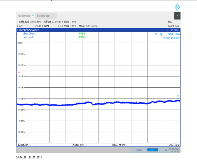
1-N38-PC2-30-40-M-1-DFT-QPSK-Edge_1RB_Left-1 @ 0-12000-20000-Ant0--50.83--25-PASS
