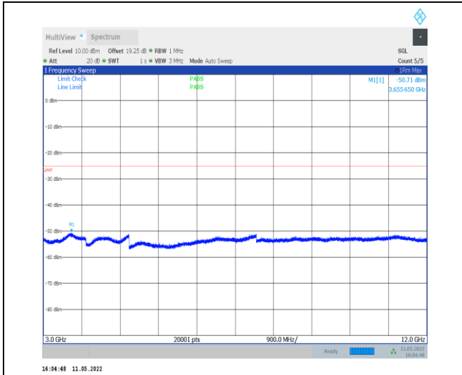
1-N38-PC2-30-40-M-1-DFT-QPSK-Edge_1RB_Left-1 @ 0-3000-12000-Ant0--50.71--25-PASS
