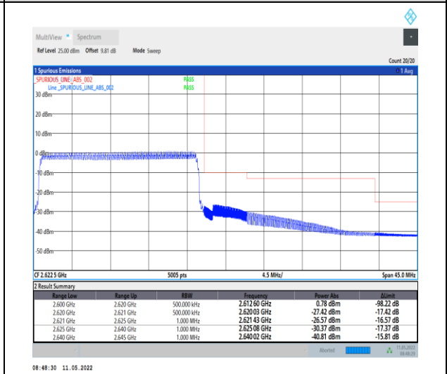
1-N38-PC2-30-20-H-6-CP-QPSK-Outer_Full-51@0-Ant0-PASS-see graph
