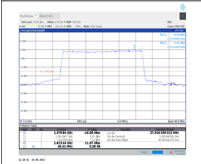
1-N38--30-40-H-9-CP-256QAM-Outer_Full-106@0-A nt0-37.92-40.320-≤40-PASS
