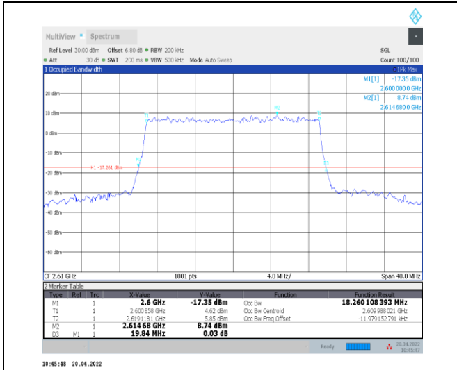
1-N38--30-20-H-9-CP-256QAM-Outer_Full-51@0-An t0-18.26-19.840-≤20-PASS
