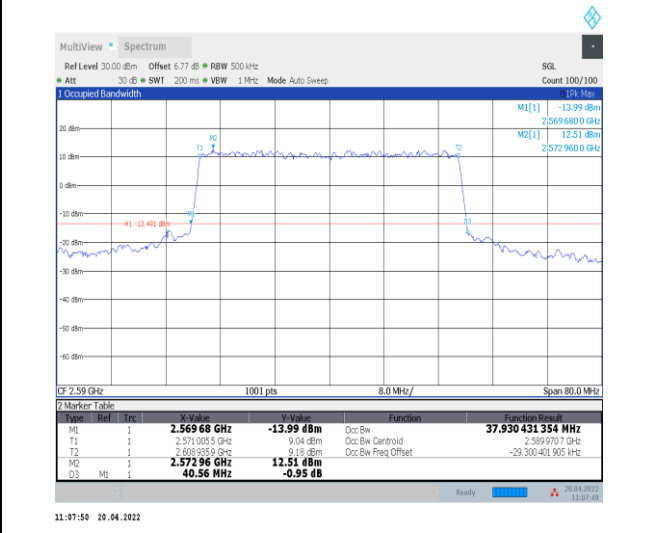
1-N38--30-40-L-8-CP-64QAM-Outer_Full-106@0-Ant t0-37.93-40.560-≤40-PASS
