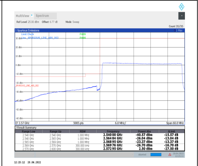
1-N38--30-30-L-6-CP-QPSK-Outer_Full-78@0-Ant0-PASS-see graph
