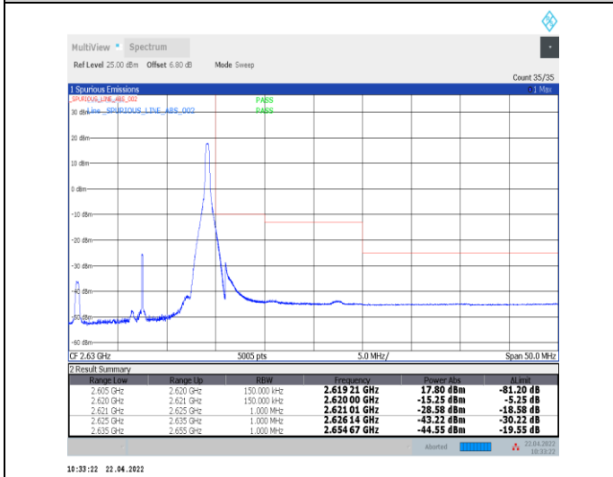
1-N38--30-15-H-5-CP-QPSK-Edge_1RB_Right-1@37-Ant0-PASS-see graph
