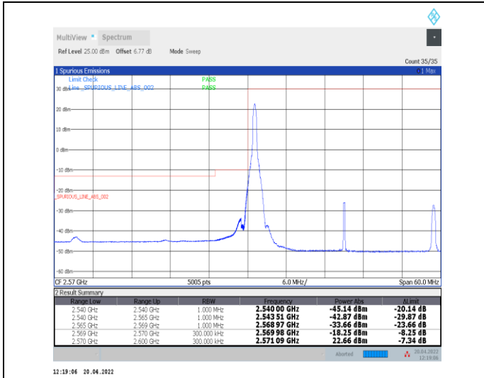
1-N38--30-30-L-1-DFT-PI2BPSK-Edge_1RB_Left-1@0-Ant0-PASS-see graph
