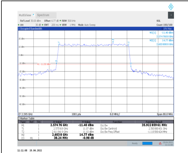
1-N38--30-40-M-4-DFT-64QAM-Outer_Full-100@0-A nt0-35.923-38.240-≤40-PASS
