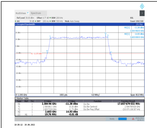
1-N38--30-20-M-2-DFT-PI2BPSK-Outer_Full-50@0-Ant0-17.858-19.760-≤20-PASS
