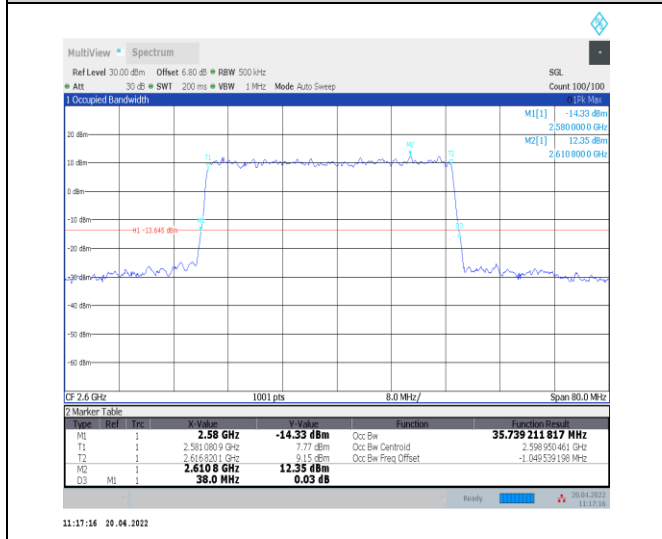
1-N38--30-40-H-5-DFT-256QAM-Outer_Full-100@0-A Ant0-35.739-38.000≤40-PASS
