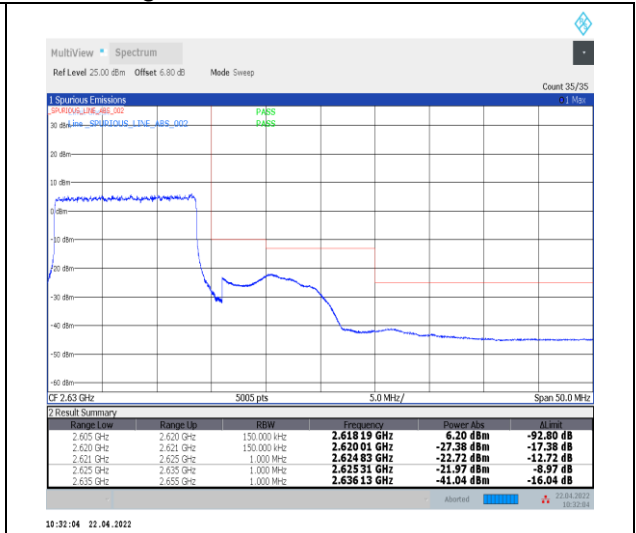
1-N38--30-15-H-3-DFT-PI2BPSK-Outer_Full-36@0-Ant0-PASS-see graph
