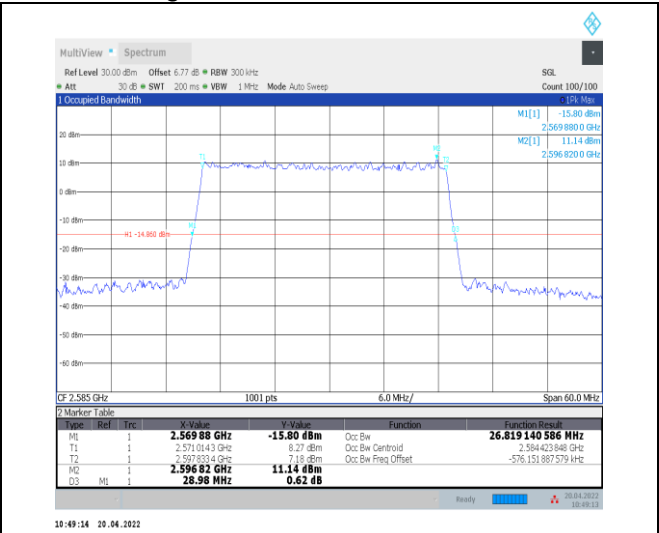
1-N38--30-30-L-5-DFT-256QAM-Outer_Full-75@0-Ant nt0-26.819-28.980-≤30-PASS
