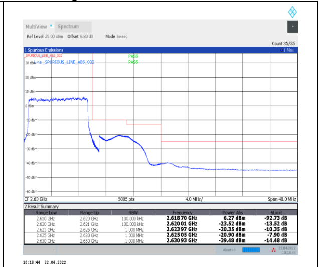
1-N38--30-10-H-3-DFT-PI2BPSK-Outer_Full-24@ 0-Ant0-PASS-see graph
