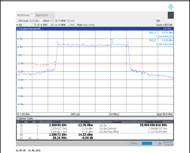
1-N38--30-40-L-4-DFT-64QAM-Outer_Full-100@0-A nt0-35.904-38.240-≤40-PASS
