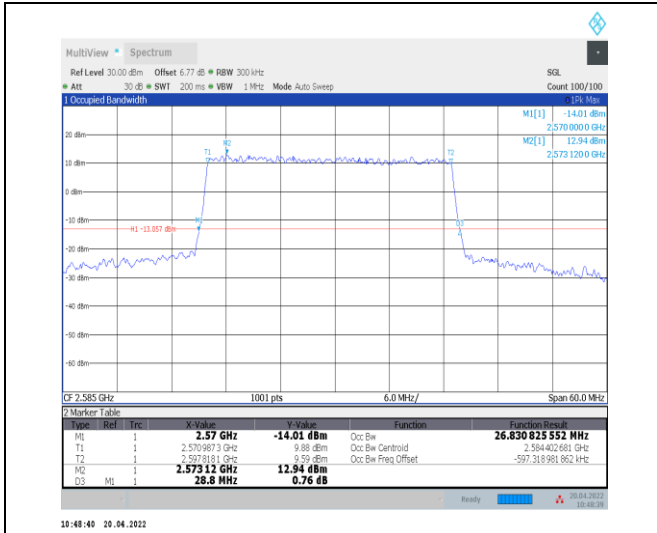
1-N38--30-30-L-4-DFT-64QAM-Outer_Full-75@0-Ant 0-26.831-28.800-≤30-PASS
