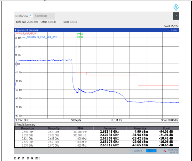
1-N38--30-30-H-3-DFT-PI2BPSK-Outer_Full-75@0-Ant0-PASS-see graph
