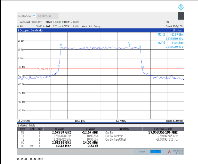
1-N38--30-40-H-6-CP-QPSK-Outer_Full-106@0-Ant 0-37.958-40.320≤40-PASS
