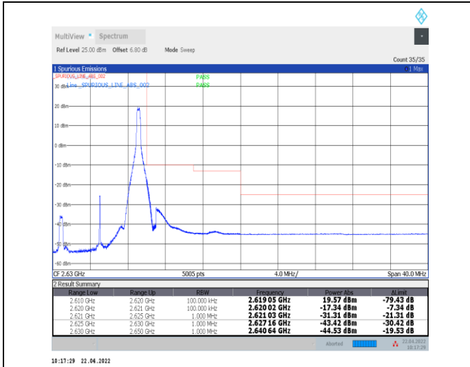
1-N38--30-10-H-2-DFT-PI2BPSK-Edge_1RB_Right-1@ 23-Ant0-PASS-see graph
