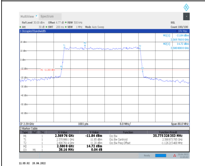
1-N38--30-40-L-3-DFT-16QAM-Outer_Full-100@0-A nt0-35.775-38.160-≤40-PASS
