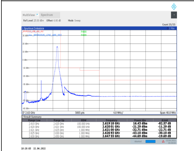
1-N38--30-10-H-5-CP-QPSK-Edge_1RB_Right-1@23- Ant0-PASS-see graph
