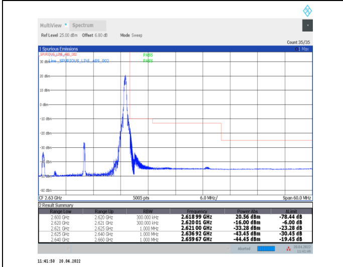
1-N38--30-20-H-5-CP-QPSK-Edge_1RB_Right-1@50-Ant0-PASS-see graph
