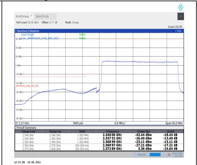
1-N38--30-30-L-3-DFT-PI2BPSK-Outer_Full-75@0-Ant0-PASS-see graph
