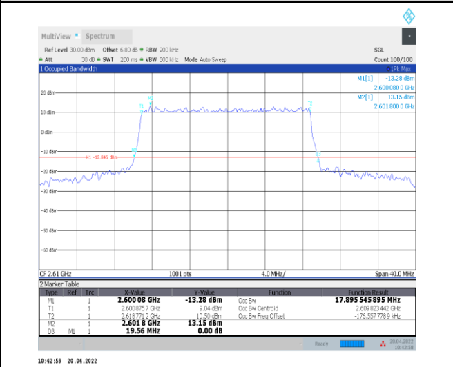
1-N38--30-20-H-4-DFT-64QAM-Outer_Full-50@0-Ant t0-17.896-19.560-≤20-PASS
