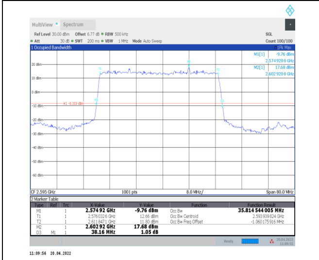
1-N38--30-40-M-2-DFT-PI2BPSK-Outer_Full-100@0 -Ant0-35.815-38.160-<math>\leq 40</math>-PASS
