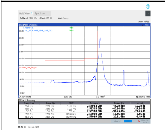
1-N38--30-20-L-4-CP-QPSK-Edge_1RB_Left-1@0-Ant0-PASS-see graph
