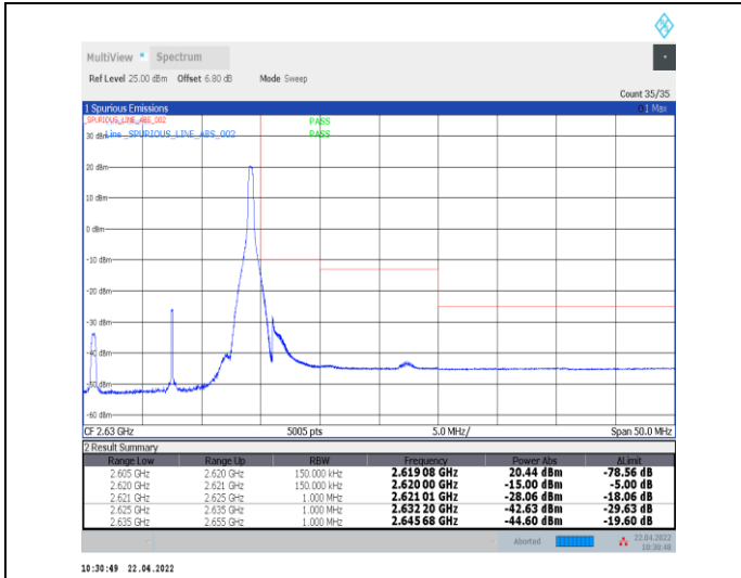
1-N38--30-15-H-2-DFT-PI2BPSK-Edge_1RB_Right-1@37-Ant0-PASS-see graph
