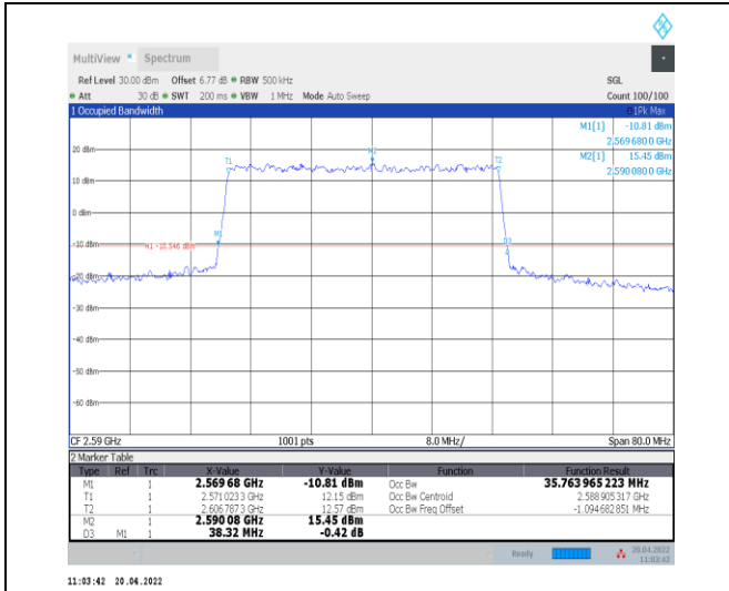
1-N38--30-40-L-1-DFT-QPSK-Outer_Full-100@0-Ant 0-35.764-38.320-≤40-PASS
