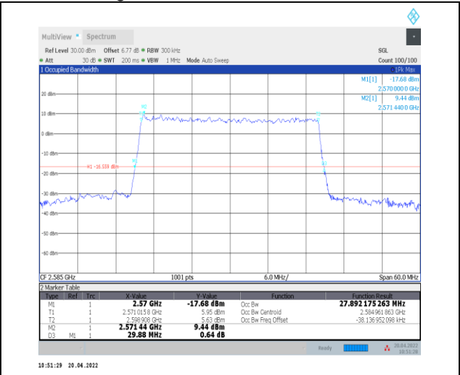
1-N38--30-30-L-9-CP-256QAM-Outer_Full-78@0-An t0-27.892-29.880-≤30-PASS
