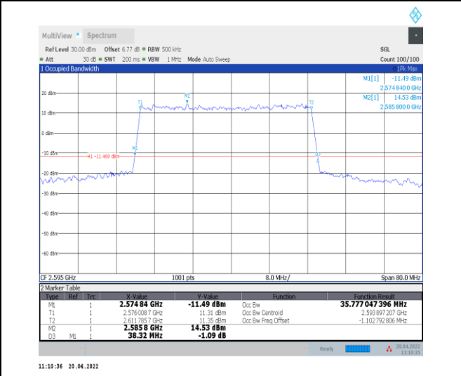
1-N38--30-40-M-3-DFT-16QAM-Outer_Full-100@0- Ant0-35.777-38.320-<math>\leq 40</math>-PASS
