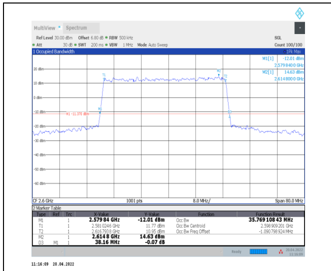
1-N38--30-40-H-3-DFT-16QAM-Outer_Full-100@0-A nt0-35.769-38.160≤40-PASS
