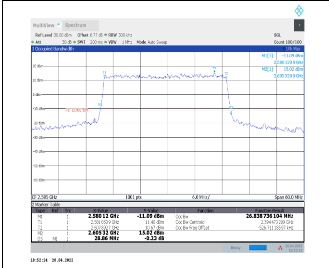
1-N38--30-30-M-1-DFT-QPSK-Outer_Full-75@0-Ant 0-26.839-28.860-≤30-PASS
