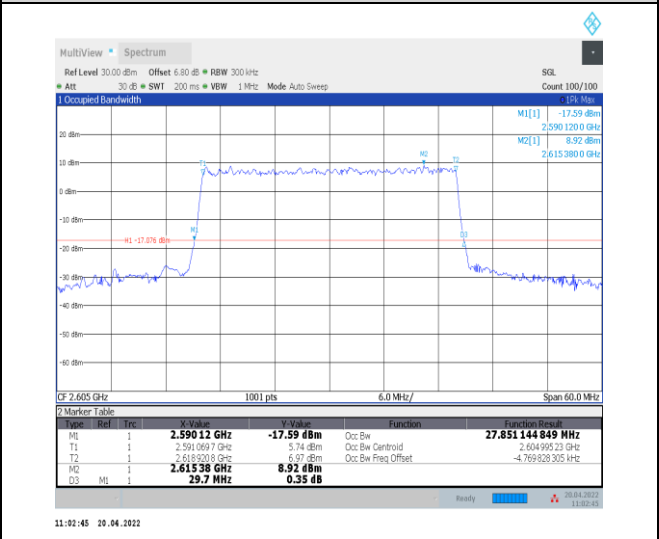
1-N38--30-30-H-9-CP-256QAM-Outer_Full-78@0-Ant0-27.851-29.700-≤30-PASS
