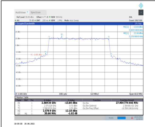
1-N38--30-30-L-8-CP-64QAM-Outer_Full-78@0-Ant0 -27.905-30.660-≤30-PASS
