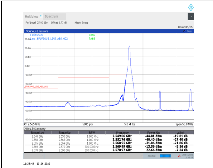
1-N38--30-20-L-1-DFT-PI2BPSK-Edge_1RB_Left-1@0-Ant0-PASS-see graph
