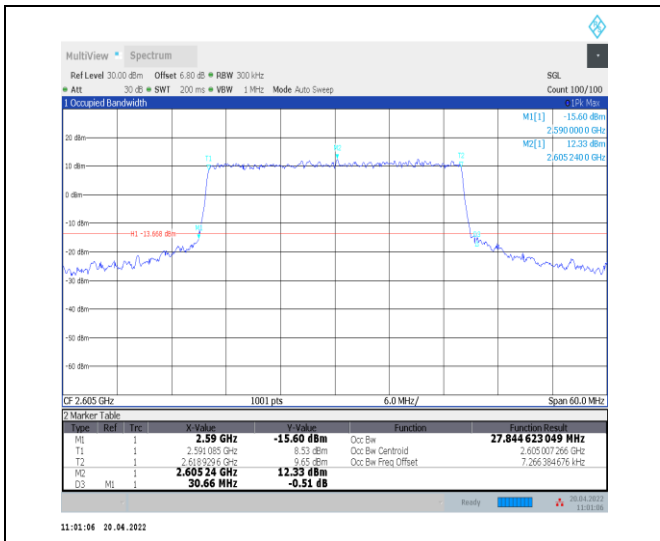
1-N38--30-30-H-6-CP-QPSK-Outer_Full-78@0-Ant0-27.845-30.660-≤30-PASS
