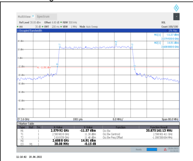
1-N38--30-40-H-4-DFT-64QAM-Outer_Full-100@0-A nt0-35.875-38.080≤40-PASS
