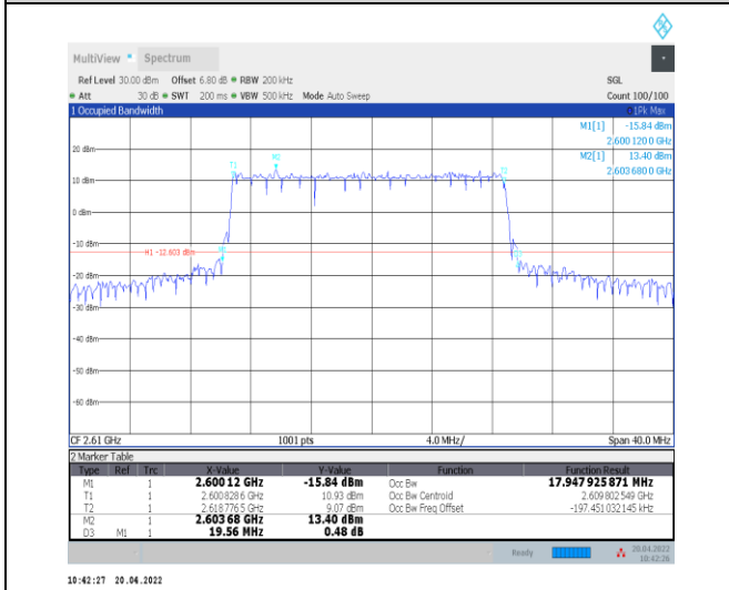
1-N38--30-20-H-3-DFT-16QAM-Outer_Full-50@0-Ant t0-17.948-19.560-≤20-PASS
