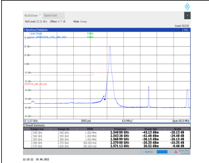
1-N38--30-30-L-4-CP-QPSK-Edge_1RB_Left-1@0-Ant0-PASS-see graph
