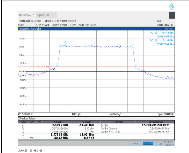
1-N38--30-30-L-6-CP-QPSK-Outer_Full-78@0-Ant 0-27.914-30.420-≤30-PASS
