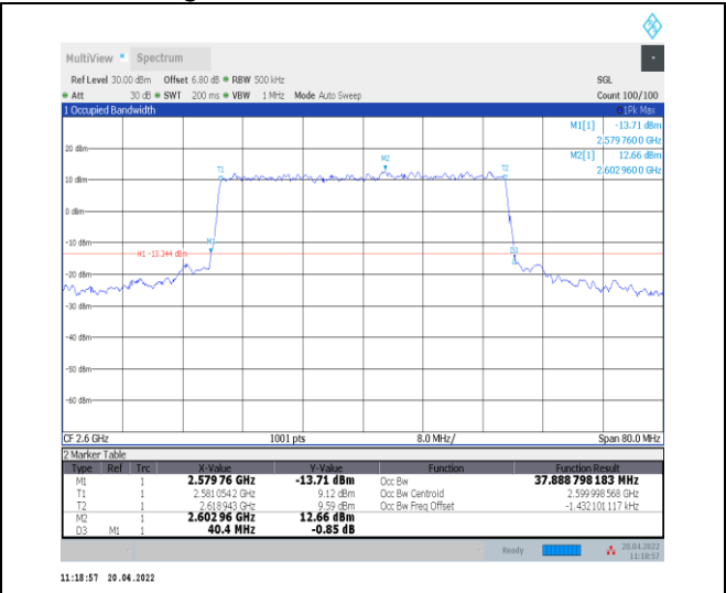
1-N38--30-40-H-8-CP-64QAM-Outer_Full-106@0-An t0-37.889-40.400-≤40-PASS
