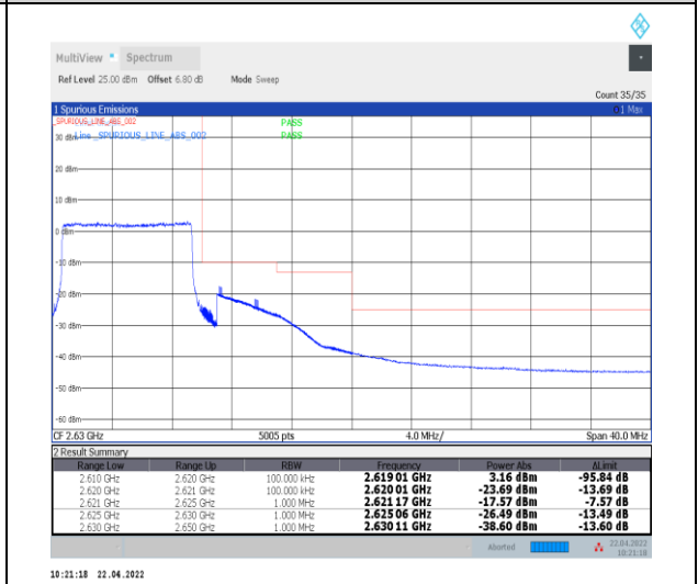
1-N38--30-10-H-6-CP-QPSK-Outer_Full-24@0-An t0-PASS-see graph
