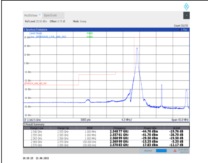
1-N38--30-15-L-4-CP-QPSK-Edge_1RB_Left-1@0-Ant0-PASS-see graph
