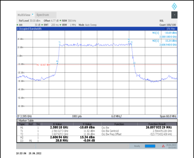
1-N38--30-30-M-2-DFT-PI2BPSK-Outer_Full-75@0- Ant0-26.898-28.800-≤30-PASS
