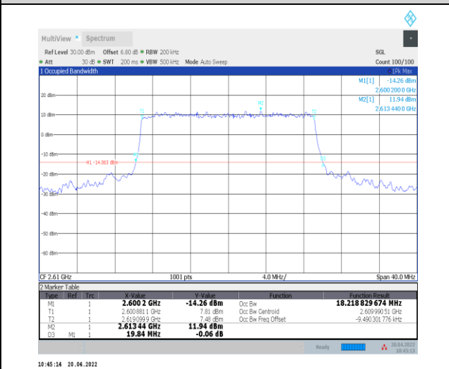
1-N38--30-20-H-8-CP-64QAM-Outer_Full-51@0-Ant 0-18.219-19.840-≤20-PASS
