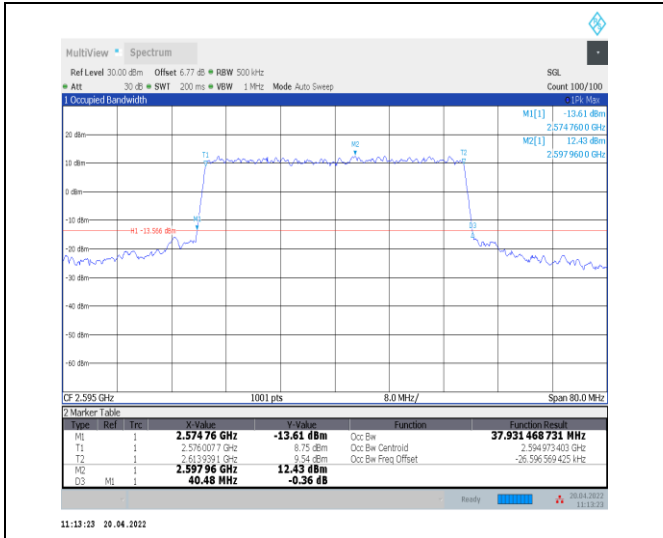
1-N38--30-40-M-8-CP-64QAM-Outer_Full-106@0-Ant0-37.931-40.480-≤40-PASS
