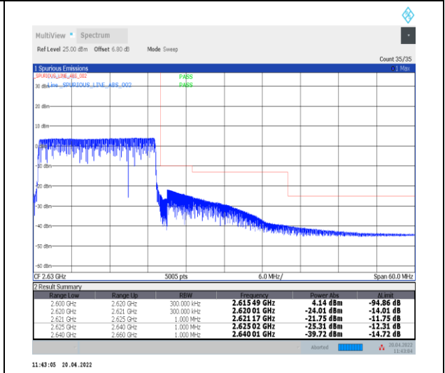
1-N38--30-20-H-6-CP-QPSK-Outer_Full-51@0-Ant0-PASS-see graph
