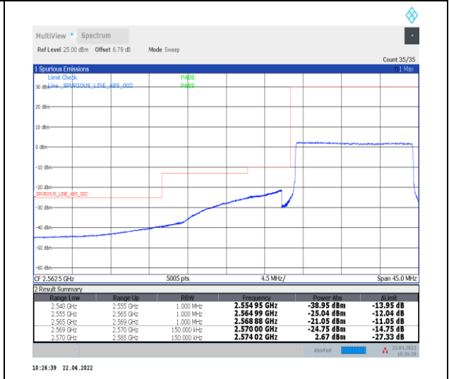
1-N38--30-15-L-6-CP-QPSK-Outer_Full-38@0-Ant0-PASS-see graph
