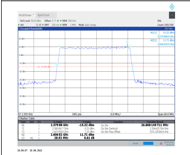
1-N38--30-30-M-5-DFT-256QAM-Outer_Full-75@0-Ant0-26.868-28.920-<=30-PASS
