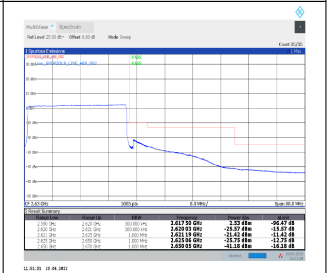
1-N38--30-30-H-6-CP-QPSK-Outer_Full-78@0-Ant0-PASS-see graph
