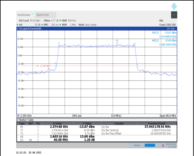
1-N38--30-40-M-7-CP-16QAM-Outer_Full-106@0-A nt0-37.943-40.480-≤40-PASS
