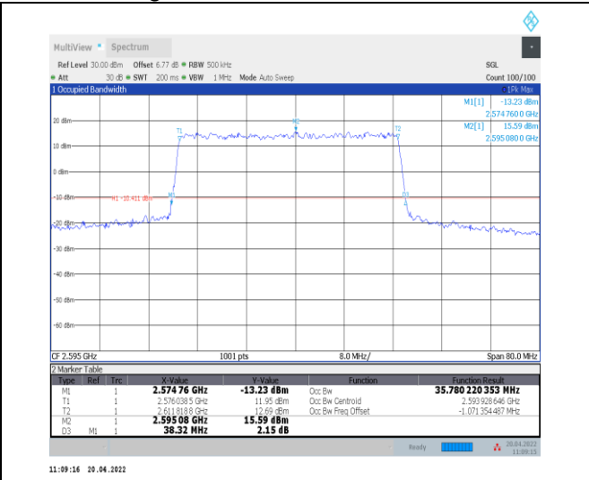
1-N38--30-40-M-1-DFT-QPSK-Outer_Full-100@0-An t0-35.78-38.320-<math>\leq 40</math>-PASS
