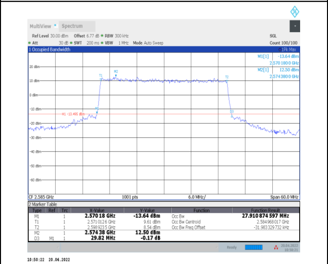
1-N38--30-30-L-7-CP-16QAM-Outer_Full-78@0-Ant 0-27.911-29.820-≤30-PASS
