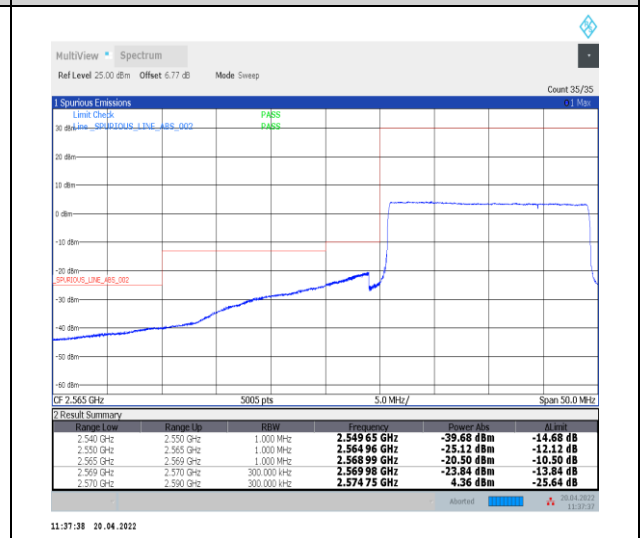
1-N38--30-20-L-6-CP-QPSK-Outer_Full-51@0-Ant0-PASS-see graph
