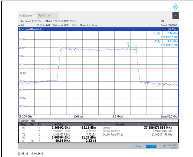
1-N38--30-40-L-9-CP-256QAM-Outer_Full-106@0-A nt0-37.89-40.160-<math>\leq 40</math>-PASS
