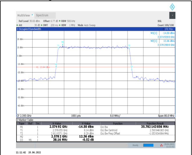
1-N38--30-40-M-5-DFT-256QAM-Outer_Full-100@0-A Ant0-35.782-38.160-≤40-PASS
