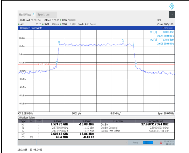
1-N38--30-40-M-6-CP-QPSK-Outer_Full-106@0-Ant 0-37.961-40.400-≤40-PASS
