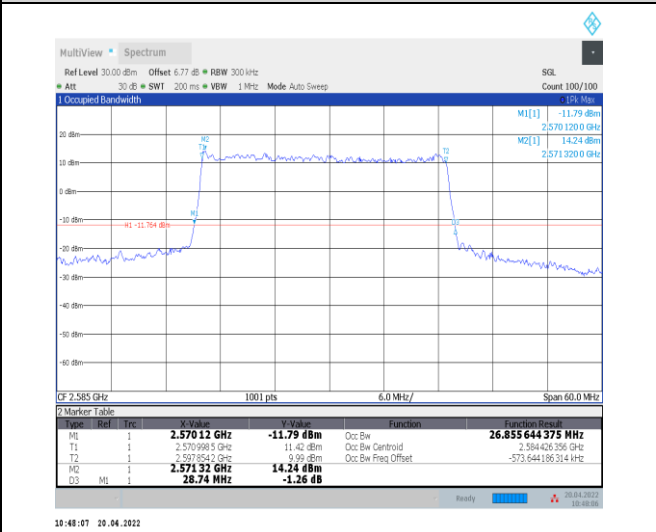
1-N38--30-30-L-3-DFT-16QAM-Outer_Full-75@0-An t0-26.856-28.740-≤30-PASS
