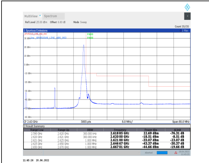
1-N38--30-30-H-2-DFT-PI2BPSK-Edge_1RB_Right-1@77-Ant0-PASS-see graph
