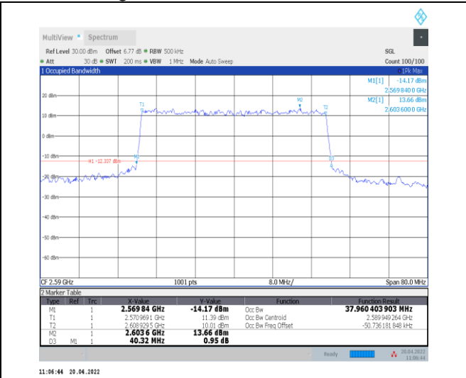
1-N38--30-40-L-6-CP-QPSK-Outer_Full-106@0-Ant 0-37.96-40.320-≤40-PASS
