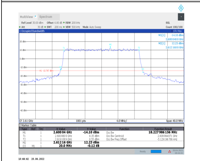
1-N38--30-20-H-7-CP-16QAM-Outer_Full-51@0-Ant 0-18.228-20.000-≤20-PASS
