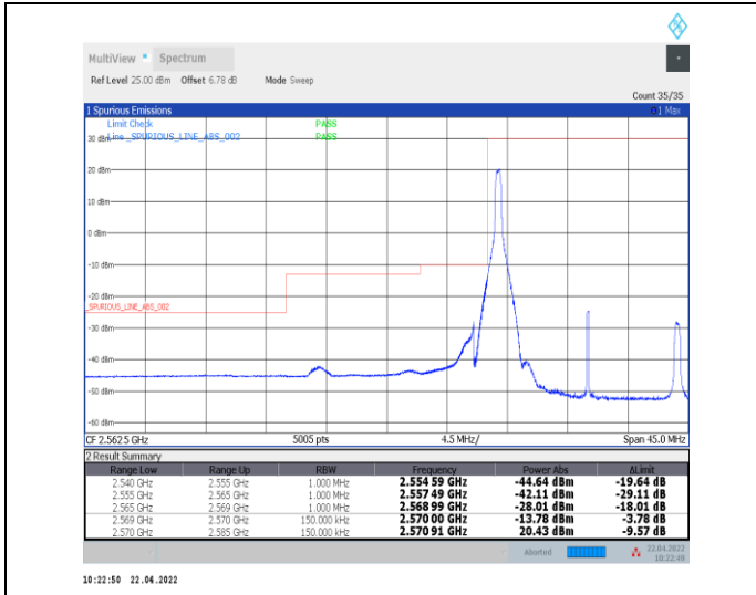
1-N38--30-15-L-1-DFT-PI2BPSK-Edge_1RB_Left-1@0-Ant0-PASS-see graph
