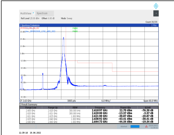
1-N38--30-20-H-2-DFT-PI2BPSK-Edge_1RB_Right-1@50-Ant0-PASS-see graph
