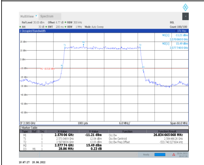
1-N38--30-30-L-2-DFT-PI2BPSK-Outer_Full-75@0-A nt0-26.835-28.860-≤30-PASS
