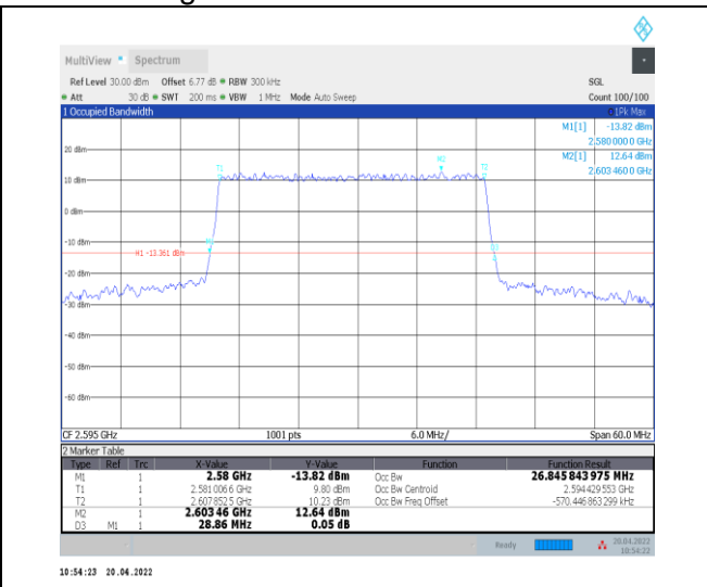
1-N38--30-30-M-4-DFT-64QAM-Outer_Full-75@0-Ant0-26.846-28.860-<=30-PASS
