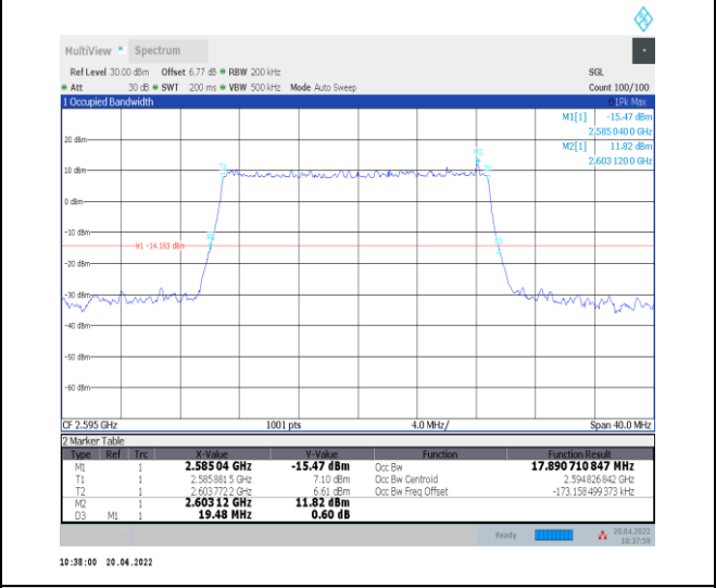
1-N38--30-20-M-5-DFT-256QAM-Outer_Full-50@0-Ant0-17.891-19.480-≤20-PASS
