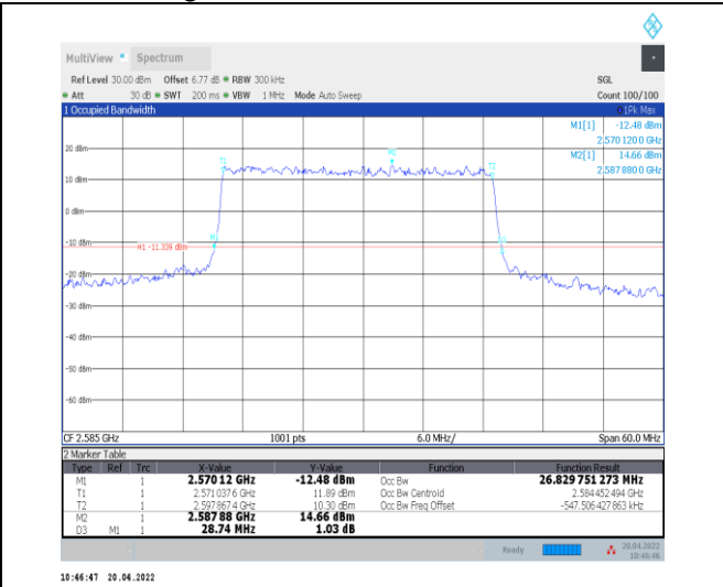
1-N38--30-30-L-1-DFT-QPSK-Outer_Full-75@0-Ant0 -26.83-28.740-≤30-PASS
