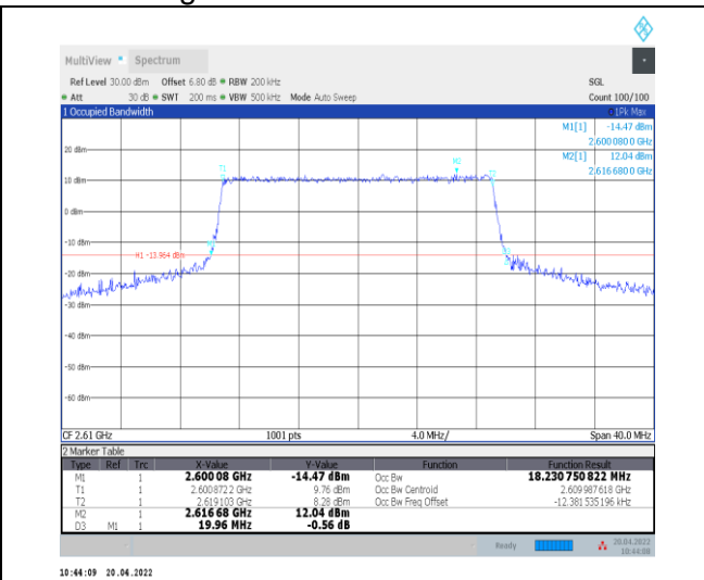
1-N38--30-20-H-6-CP-QPSK-Outer_Full-51@0-Ant0- 18.231-19.960-≤20-PASS
