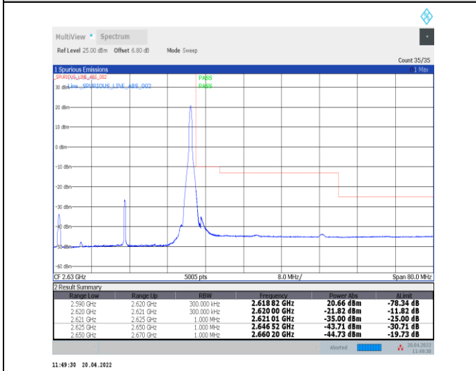
1-N38--30-30-H-5-CP-QPSK-Edge_1RB_Right-1@77-Ant0-PASS-see graph
