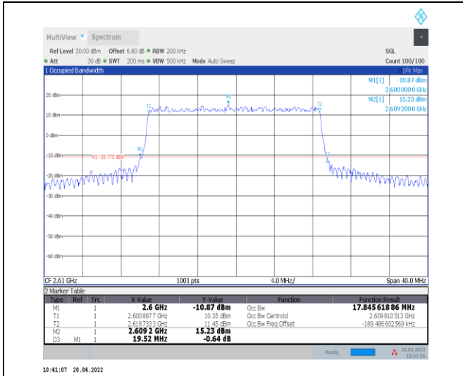
1-N38--30-20-H-1-DFT-QPSK-Outer_Full-50@0-Ant 0-17.846-19.520-≤20-PASS
