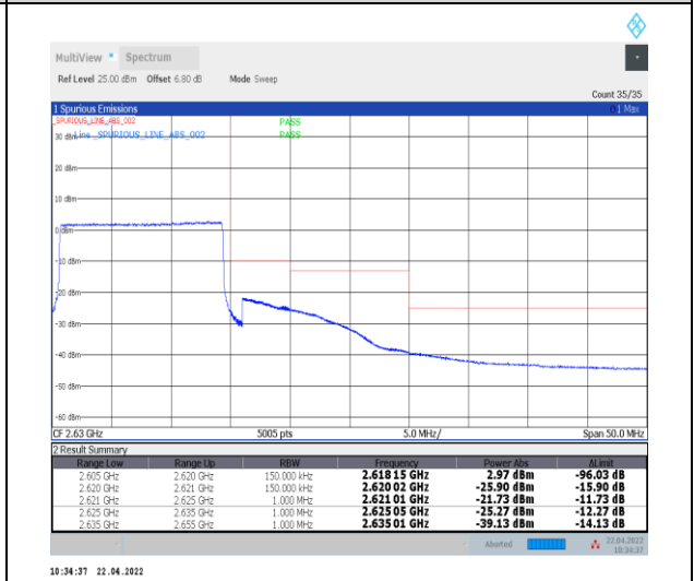
1-N38--30-15-H-6-CP-QPSK-Outer_Full-38@0-Ant0-PASS-see graph
