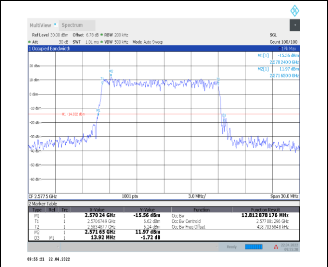
1-N38--30-15-L-5-DFT-256QAM-Outer_Full-36@0-A nt0-12.813-13.920-≤15-PASS
