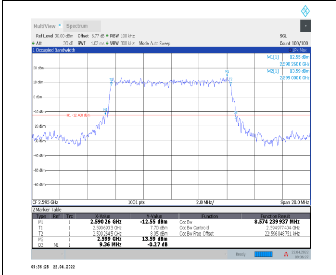
1-N38--30-10-M-2-DFT-PI2BPSK-Outer_Full-24@0-Ant 0-8.574-9.360-≤10-PASS
