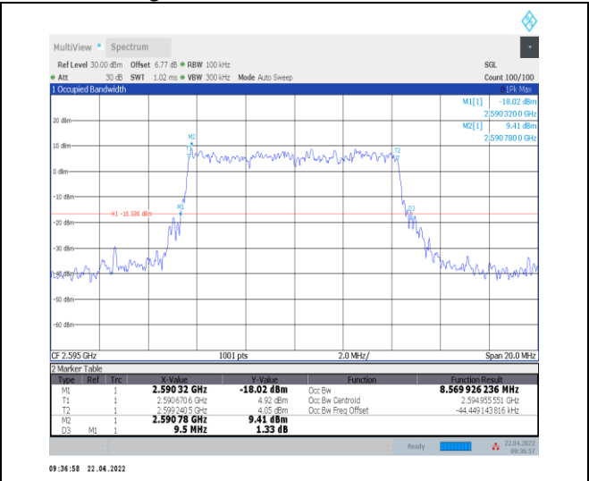
1-N38--30-10-M-5-DFT-256QAM-Outer_Full-24@0-Ant t0-8.57-9.500-≤10-PASS
