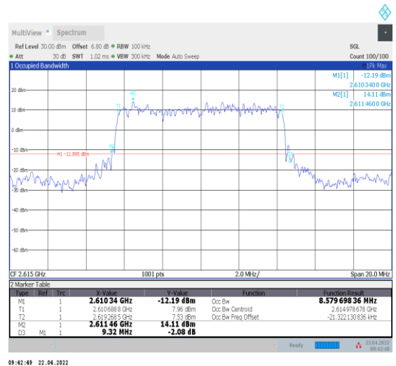
1-N38--30-10-H-2-DFT-PI2BPSK-Outer_Full-24@0-Ant 0-8.58-9.320-≤10-PASS
