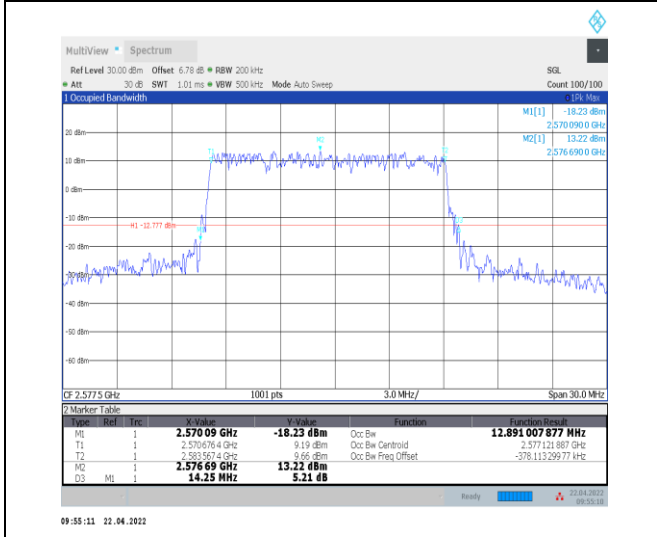
1-N38--30-15-L-4-DFT-64QAM-Outer_Full-36@0-Ant 0-12.891-14.250-≤15-PASS
