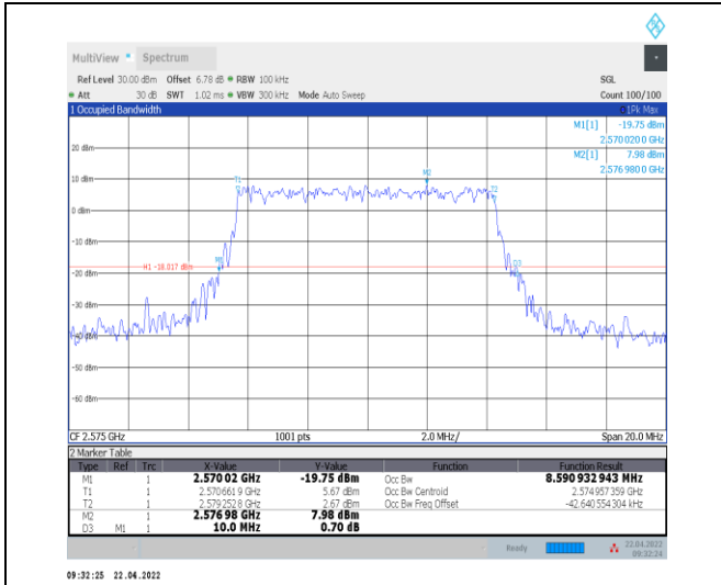
1-N38--30-10-L-5-DFT-256QAM-Outer_Full-24@0-A nt0-8.591-10.000-≤10-PASS
