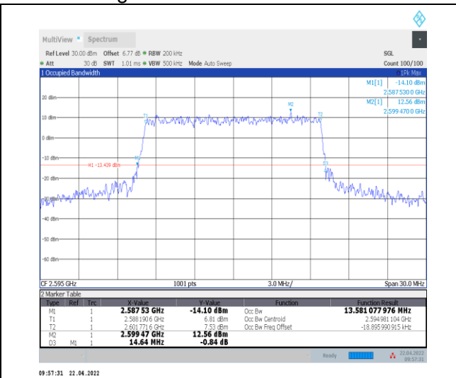
1-N38--30-15-M-6-CP-QPSK-Outer_Full-38@0-Ant0 -13.581-14.640-≤15-PASS
