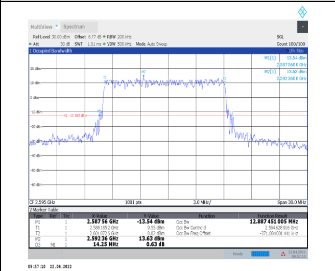
1-N38--30-15-M-4-DFT-64QAM-Outer_Full-36@0-Ant 0-12.887-14.250≤15-PASS
