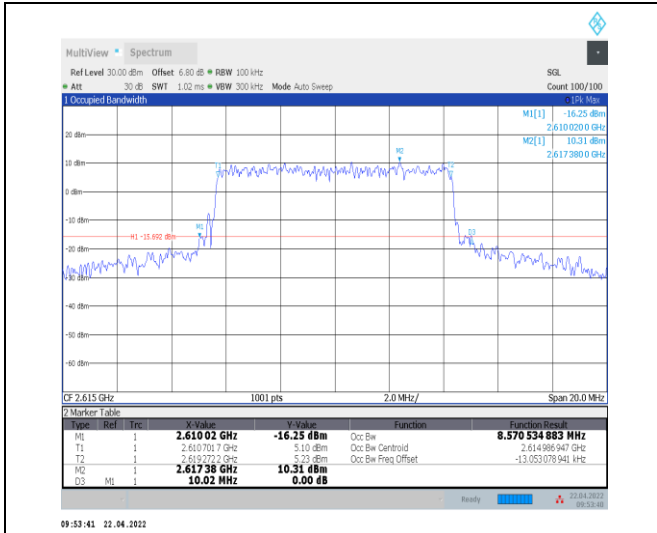
1-N38--30-10-H-7-CP-16QAM-Outer_Full-24@0-Ant 0-8.571-10.020-≤10-PASS
