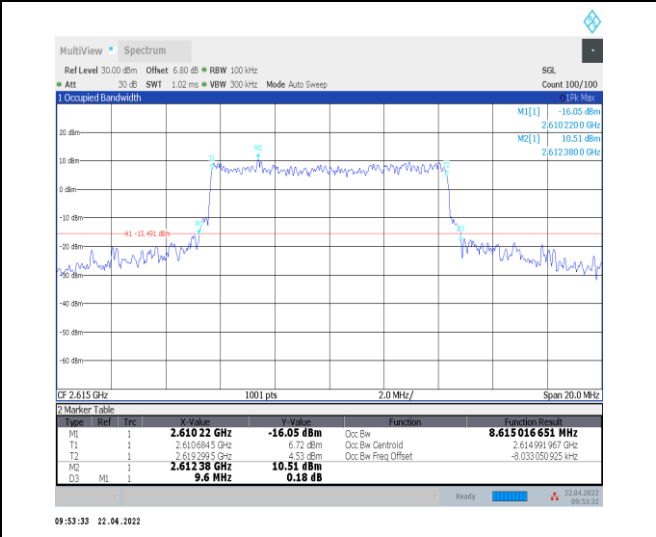
1-N38--30-10-H-6-CP-QPSK-Outer_Full-24@0-Ant0- 8.615-9.600-≤10-PASS
