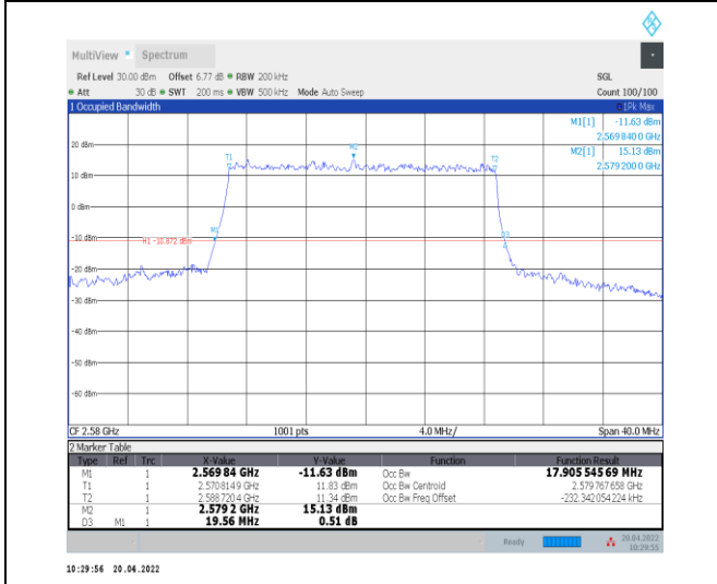
1-N38--30-20-L-1-DFT-QPSK-Outer_Full-50@0-Ant0 -17.906-19.560≤20-PASS
