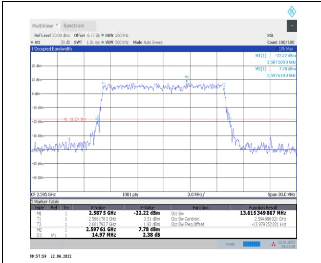
1-N38--30-15-M-9-CP-256QAM-Outer_Full-38@0-An t0-13.615-14.970-≤15-PASS
