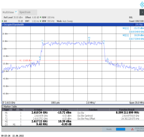
1-N38--30-10-H-1-DFT-QPSK-Outer_Full-24@0-Ant 0-8.599-9.480-≤10-PASS
