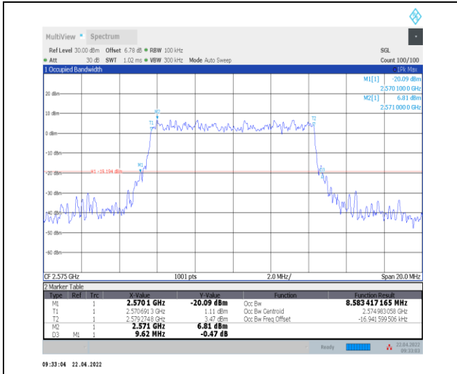
1-N38--30-10-L-9-CP-256QAM-Outer_Full-24@0-Ant 0-8.583-9.620-≤10-PASS
