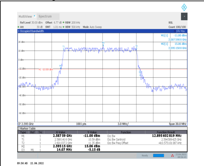
1-N38--30-15-M-2-DFT-PI2BPSK-Outer_Full-36@0-Ant 0-12.896-14.070≤15-PASS
