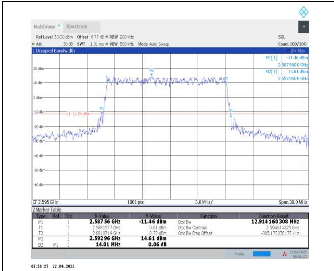
1-N38--30-15-M-1-DFT-QPSK-Outer_Full-36@0-Ant 0-12.914-14.010≤15-PASS
