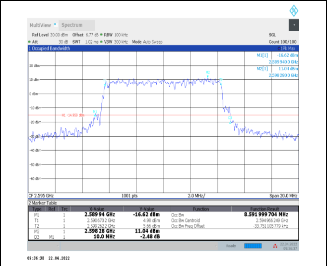
1-N38--30-10-M-3-DFT-16QAM-Outer_Full-24@0-Ant 0-8.592-10.000-≤10-PASS
