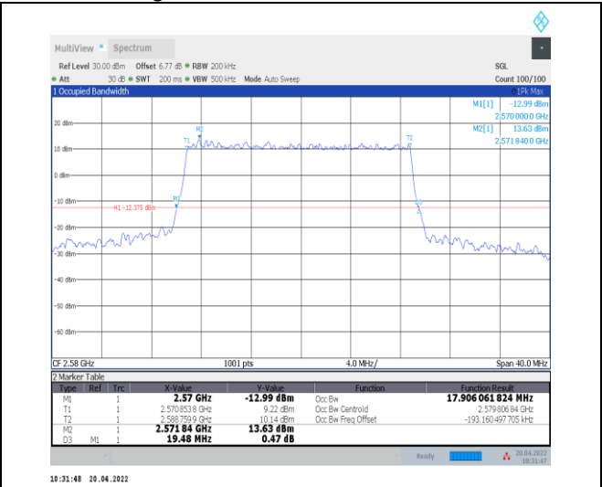
1-N38--30-20-L-4-DFT-64QAM-Outer_Full-50@0-Ant t0-17.906-19.480-≤20-PASS
