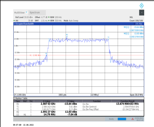
1-N38--30-15-M-8-CP-64QAM-Outer_Full-38@0-Ant 0-13.675-14.790-≤15-PASS
