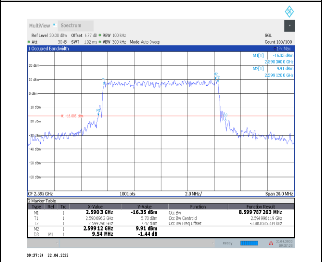
1-N38--30-10-M-7-CP-16QAM-Outer_Full-24@0-Ant t0-8.6-9.540-≤10-PASS
