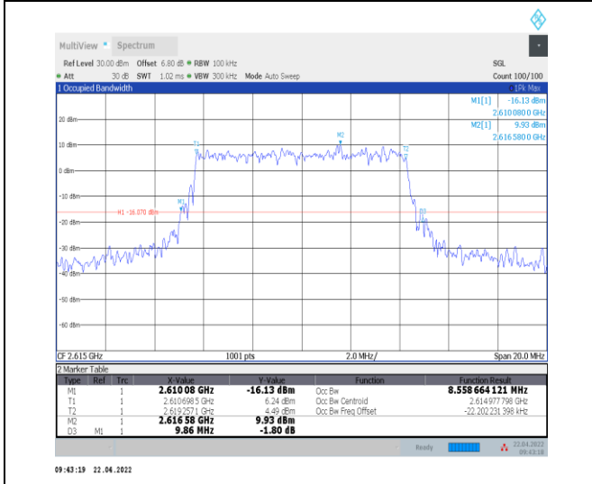
1-N38--30-10-H-5-DFT-256QAM-Outer_Full-24@0-A nt0-8.559-9.860-≤10-PASS
