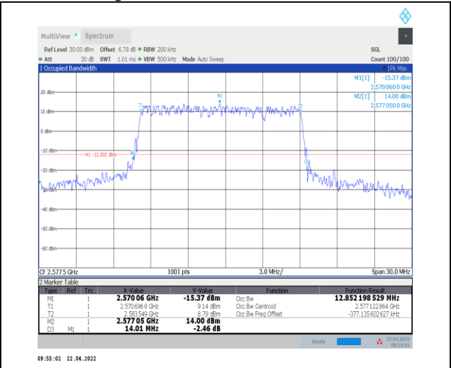
1-N38--30-15-L-3-DFT-16QAM-Outer_Full-36@0-An t0-12.852-14.010-≤15-PASS
