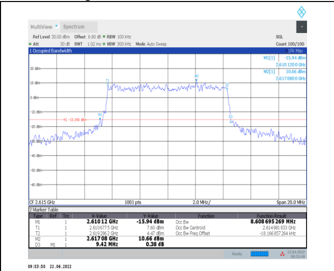
1-N38--30-10-H-8-CP-64QAM-Outer_Full-24@0-Ant 0-8.609-9.420-≤10-PASS
