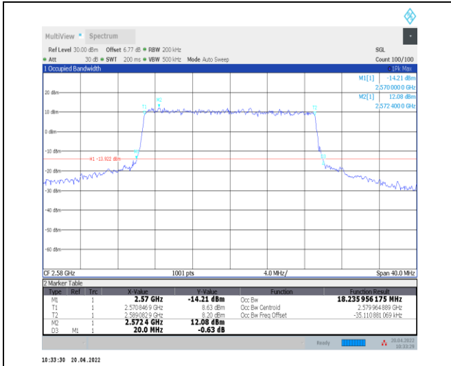
1-N38--30-20-L-7-CP-16QAM-Outer_Full-51@0-Ant0 -18.236-20.000-≤20-PASS
