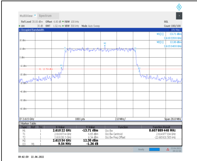
1-N38--30-10-H-3-DFT-16QAM-Outer_Full-24@0-An t0-8.608-9.540-≤10-PASS
