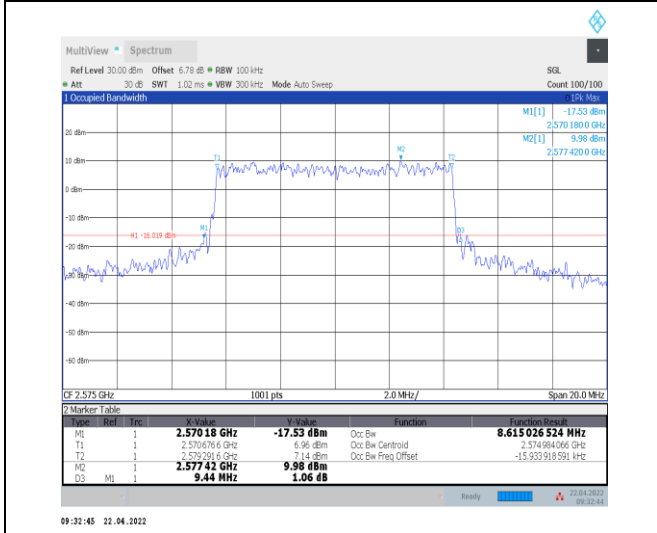
1-N38--30-10-L-7-CP-16QAM-Outer_Full-24@0-Ant0 -8.615-9.440-≤10-PASS
