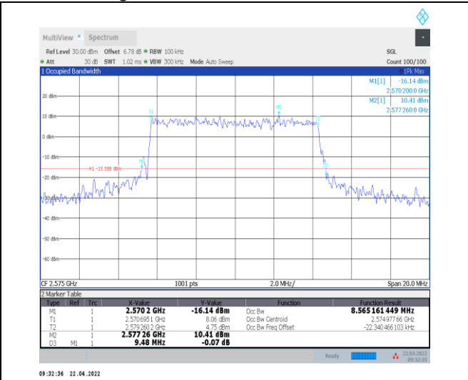
1-N38--30-10-L-6-CP-QPSK-Outer_Full-24@0-Ant0 8.565-9.480-≤10-PASS
