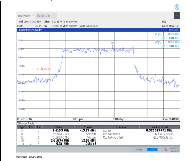
1-N38--30-10-H-4-DFT-64QAM-Outer_Full-24@0-An t0-8.594-9.360-≤10-PASS
