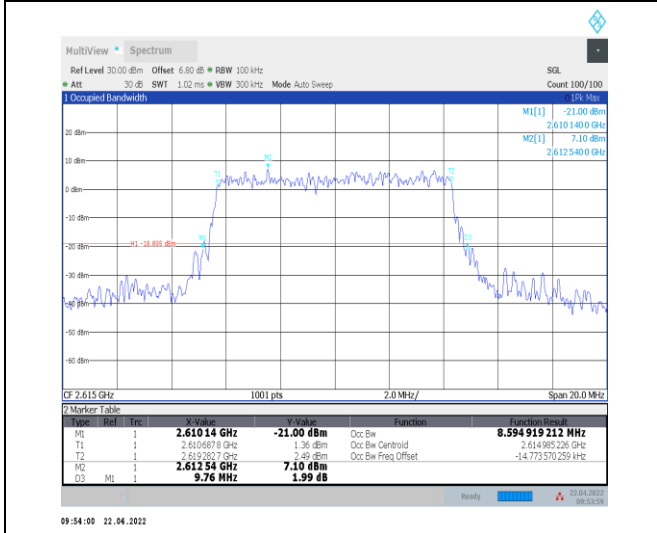
1-N38--30-10-H-9-CP-256QAM-Outer_Full-24@0-Ant t0-8.595-9.760-≤10-PASS
