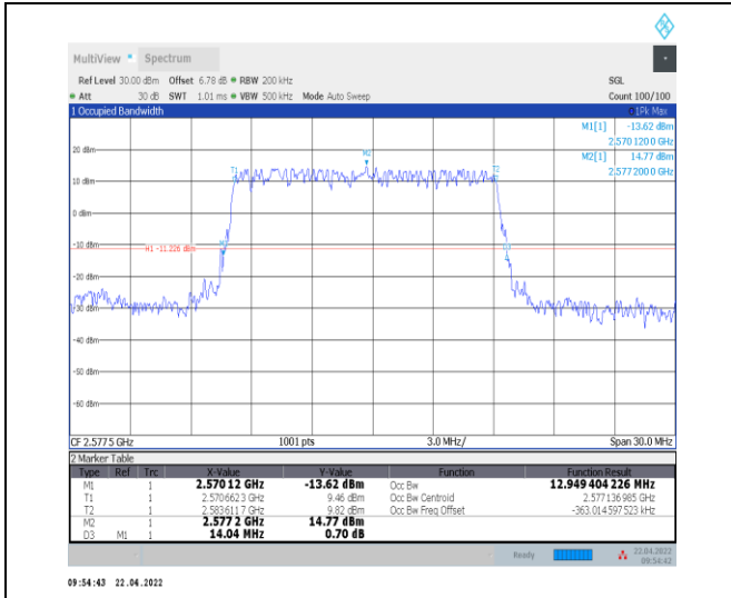
1-N38--30-15-L-2-DFT-PI2BPSK-Outer_Full-36@0-A nt0-12.949-14.040-≤15-PASS
