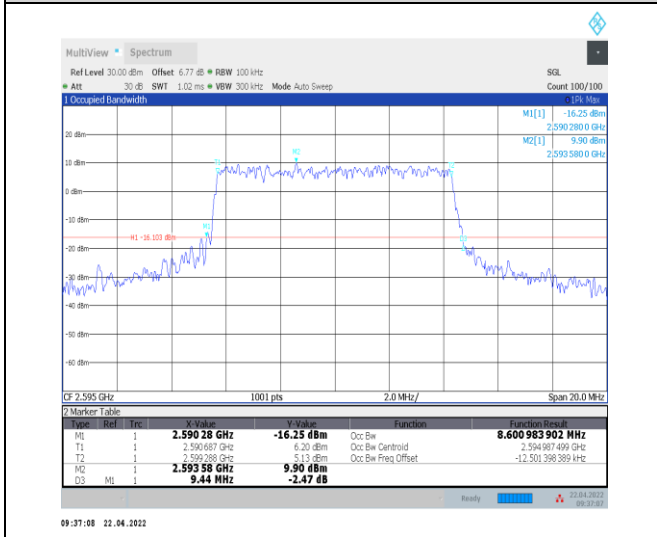
1-N38--30-10-M-6-CP-QPSK-Outer_Full-24@0-Ant t0-8.601-9.440-≤10-PASS
