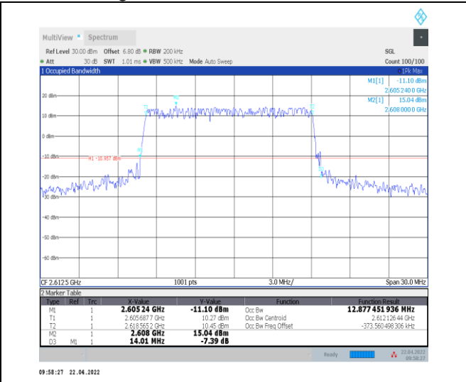
1-N38--30-15-H-1-DFT-QPSK-Outer_Full-36@0-Ant 0-12.877-14.010-≤15-PASS
