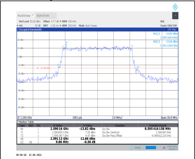
1-N38--30-10-M-1-DFT-QPSK-Outer_Full-24@0-Ant 0-8.595-9.860-≤10-PASS
