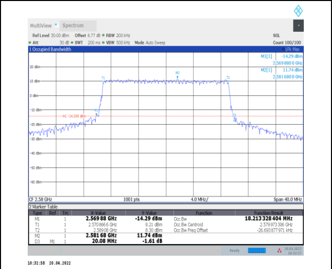
1-N38--30-20-L-6-CP-QPSK-Outer_Full-51@0-Ant t0-18.213-20.080-≤20-PASS
