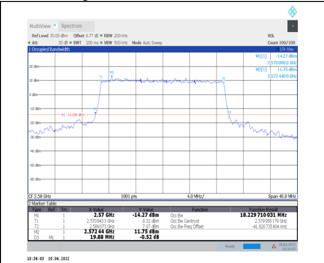
1-N38--30-20-L-8-CP-64QAM-Outer_Full-51@0-Ant0 0-18.23-19.880-≤20-PASS
