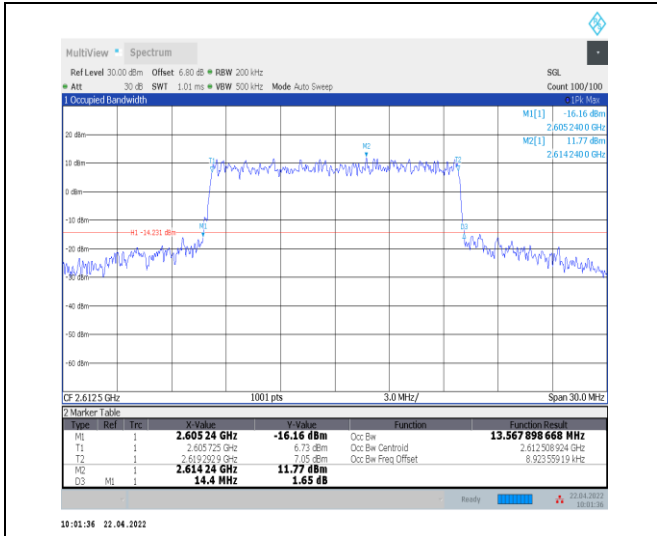
1-N38--30-15-H-8-CP-64QAM-Outer_Full-38@0-Ant 0-13.568-14.400≤15-PASS
