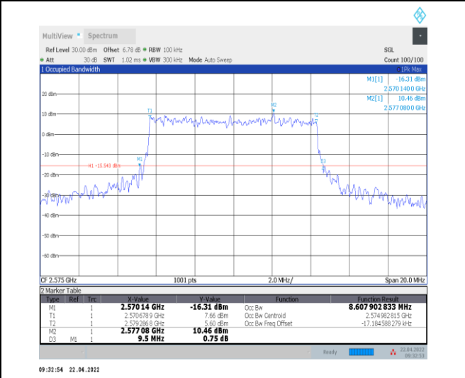
1-N38--30-10-L-8-CP-64QAM-Outer_Full-24@0-Ant 0-8.608-9.500-≤10-PASS
