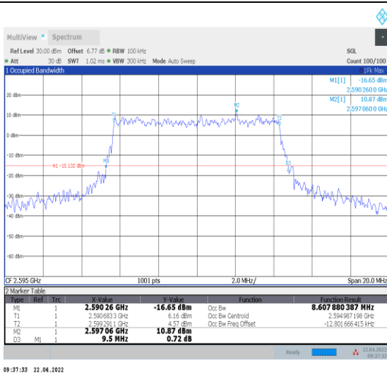
1-N38--30-10-M-8-CP-64QAM-Outer_Full-24@0-Ant 0-8.608-9.500-≤10-PASS
