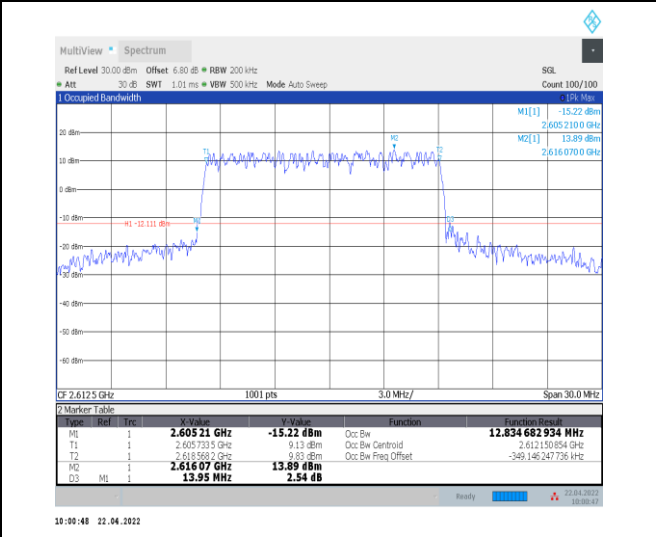
1-N38--30-15-H-3-DFT-16QAM-Outer_Full-36@0-An t0-12.835-13.950-≤15-PASS
