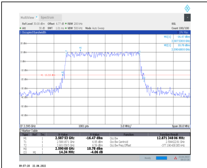
1-N38--30-15-M-5-DFT-256QAM-Outer_Full-36@0-A nt0-12.871-14.340-≤15-PASS
