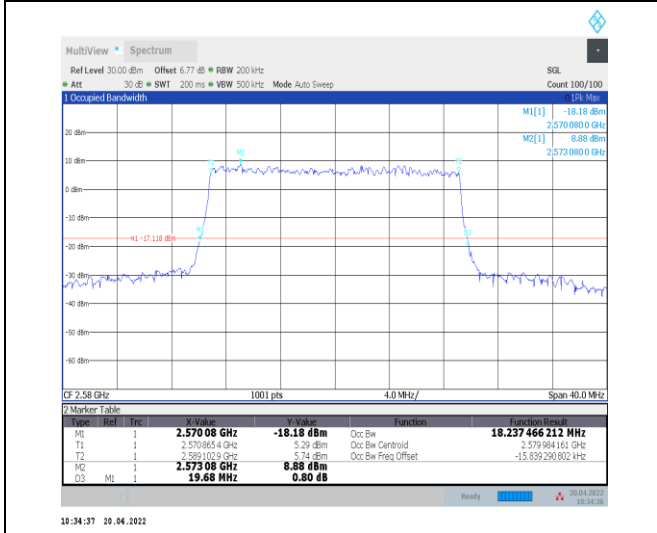
1-N38--30-20-L-9-CP-256QAM-Outer_Full-51@0-Ant0 0-18.237-19.680-≤20-PASS
