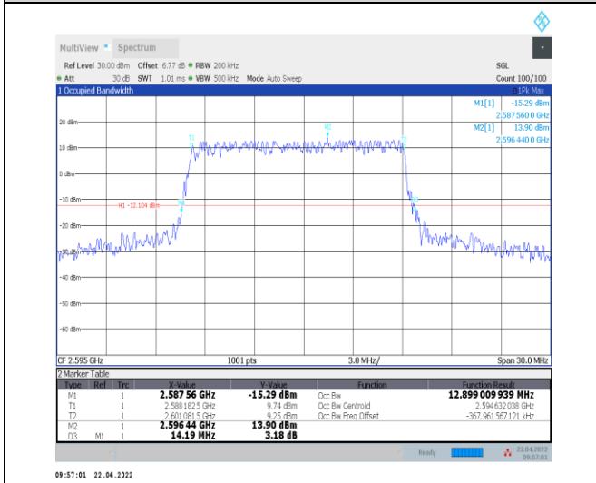
1-N38--30-15-M-3-DFT-16QAM-Outer_Full-36@0-Ant 0-12.899-14.190≤15-PASS
