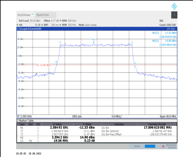
1-N38--30-20-M-1-DFT-QPSK-Outer_Full-50@0-Ant0 0-17.897-19.560-≤20-PASS
