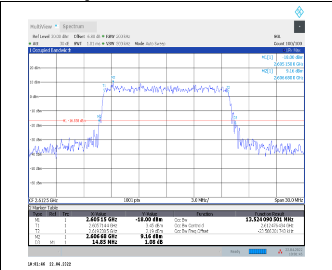
1-N38--30-15-H-9-CP-256QAM-Outer_Full-38@0-Ant t0-13.524-14.850≤15-PASS
