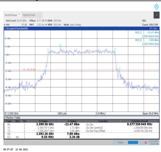
1-N38--30-10-M-9-CP-256QAM-Outer_Full-24@0-Ant 0-8.577-9.540-≤10-PASS
