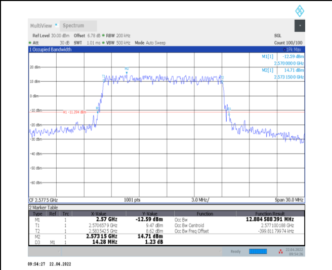
1-N38--30-15-L-1-DFT-QPSK-Outer_Full-36@0-Ant0 -12.885-14.280-≤15-PASS
