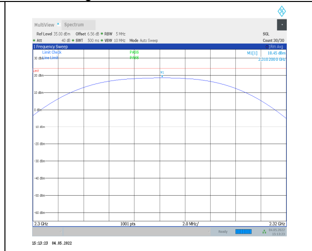
1-N30-PC3-15-10-H-3-DFT-PI2BPSK-Outer_Full-50 @0-2300-2320-Ant0-18.45-23.98-PASS
