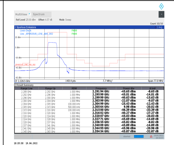
1-N30--30-10-L-6-CP-QPSK-Outer_Full-24@0-Ant0-PASS-see graph
