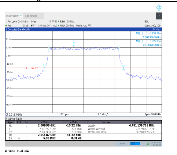
1-N30--15-5-H-4-DFT-64QAM-Outer_Full-25@0-Ant 0-4.481-5.080-≤5-PASS
