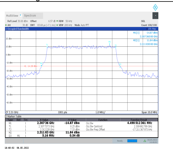
1-N30--15-5-M-1-DFT-QPSK-Outer_Full-25@0-Ant0- 4.491-5.160-<math>\leq</math>5-PASS
