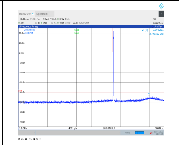
1-N30--15-10-H-1-DFT-PI2BPSK-Inner_1RB_Left-1 @1-1000-3000-Ant0--44.29--40-PASS
