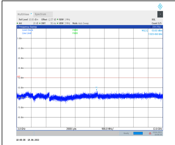
1-N30--30-15-L-1-DFT-PI2BPSK-Inner_1RB_Left-1 @1-3000-12000-Ant0--53.02--40-PASS
