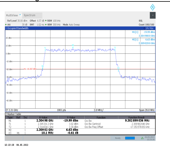
1-N30--15-10-H-9-CP-256QAM-Outer_Full-52@0-An t0-9.303-10.100-≤10-PASS
