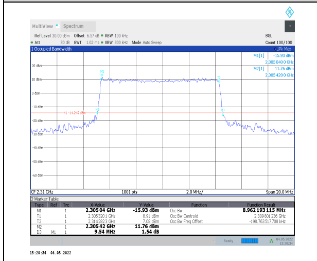
1-N30--15-10-M-3-DFT-16QAM-Outer_Full-50@0-A nt0-8.962-9.540-<=10-PASS
