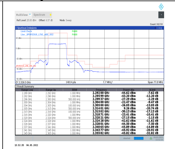
1-N30--15-10-H-3-DFT-PI2BPSK-Outer_Full-50@0-Ant0-PASS-see graph
