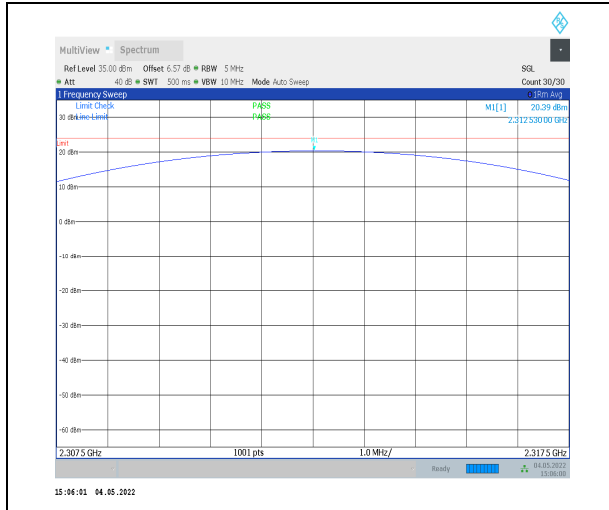
1-N30-PC3-15-5-H-3-DFT-PI2BPSK-Outter_Full-25 @0-2307.5-2317.5-Ant0-20.39-23.98-PASS
