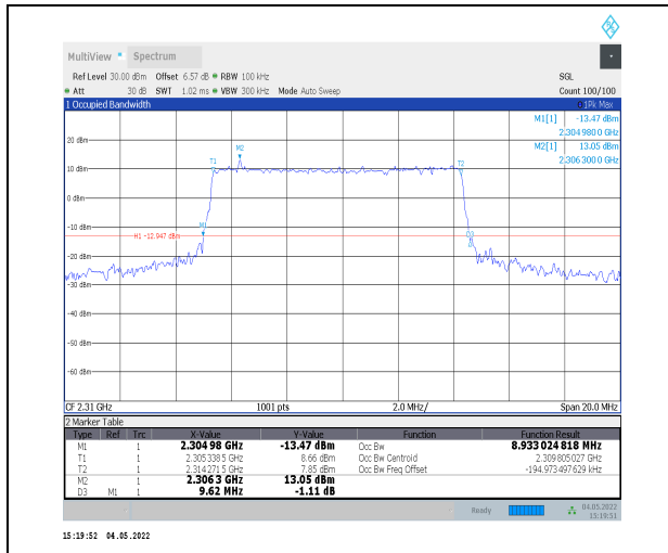
1-N30--15-10-M-1-DFT-QPSK-Outer_Full-50@0-Ant 0-8.933-9.620-<=10-PASS
