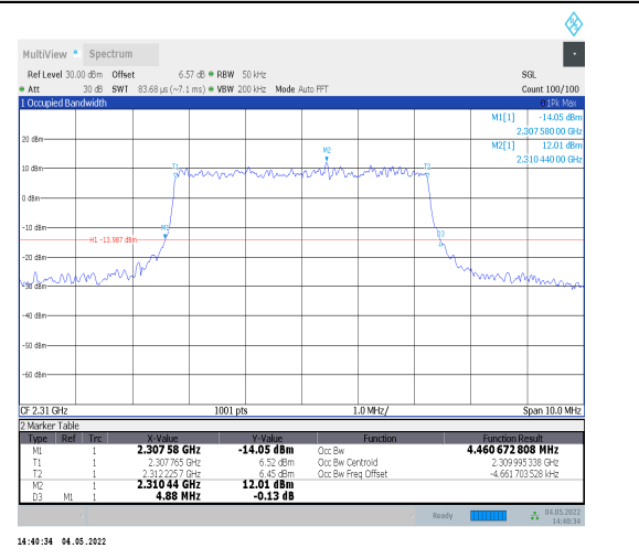
1-N30--15-5-M-3-DFT-16QAM-Outer_Full-25@0-Ant 0-4.461-4.880-<math>\leq</math>5-PASS
