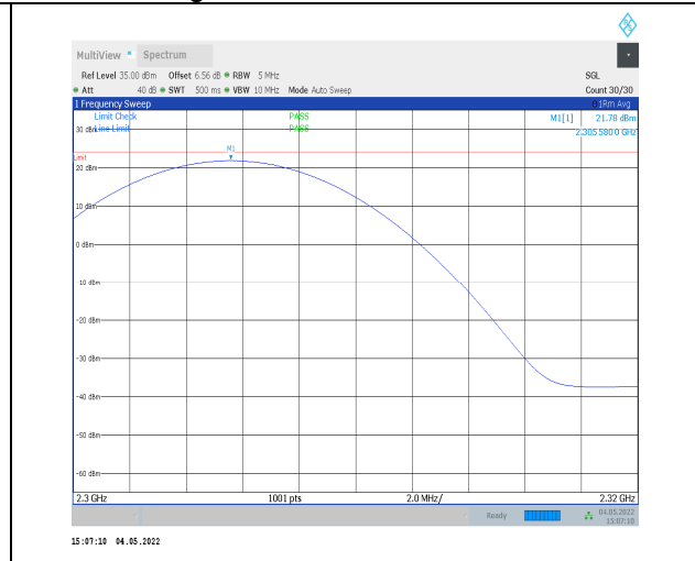
1-N30-PC3-15-10-L-1-DFT-PI2BPSK-Inner_1RB_Left -1@1-2300-2320-Ant0-21.78-23.98-PASS
