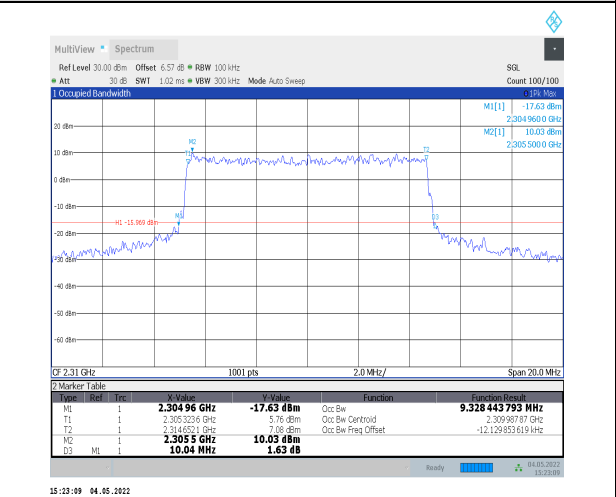
1-N30--15-10-H-7-CP-16QAM-Outer_Full-52@0-Ant 0-9.328-10.040-≤10-PASS
