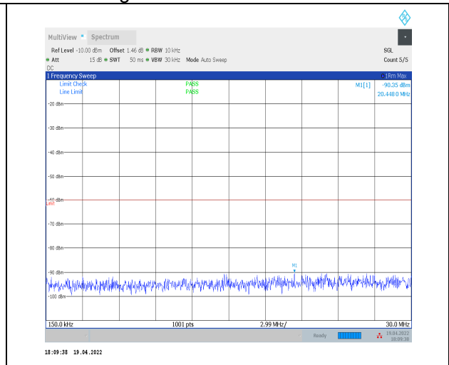
1-N30--15-10-H-1-DFT-PI2BPSK-Inner_1RB_Left-1 @1-0.15-30-Ant0--90.35--60-PASS
