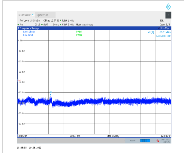
1-N30--15-10-H-1-DFT-PI2BPSK-Inner_1RB_Left-1 @1-3000-12000-Ant0--53.01--40-PASS
