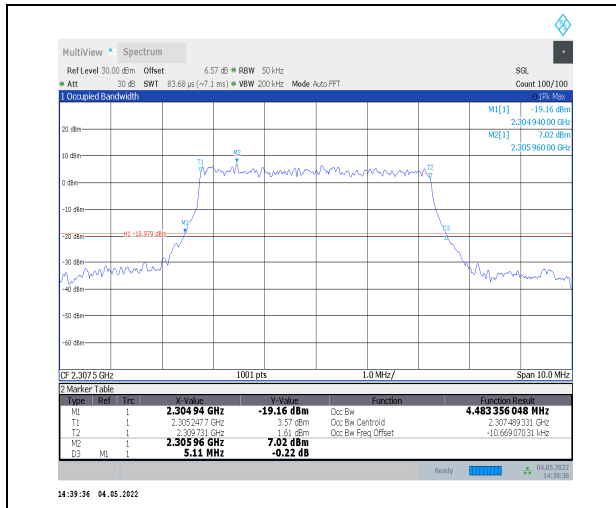
1-N30--15-5-L-9-CP-256QAM-Outer_Full-25@0-Ant 0-4.483-5.110-<math>\leq</math>5-PASS
