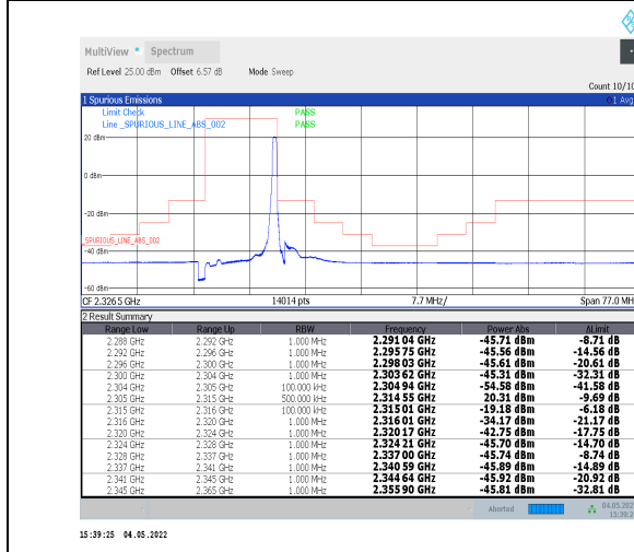
1-N30--15-10-H-5-CP-QPSK-Edge_1RB_Right-1@51-Ant0-PASS-see graph
