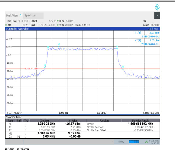
1-N30--15-5-H-6-CP-QPSK-Outer_Full-25@0-Ant0-4 .47-5.050-≤5-PASS
