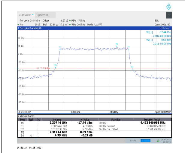
1-N30--15-5-M-8-CP-64QAM-Outer_Full-25@0-Ant0 -4.474-4.990-≤5-PASS
