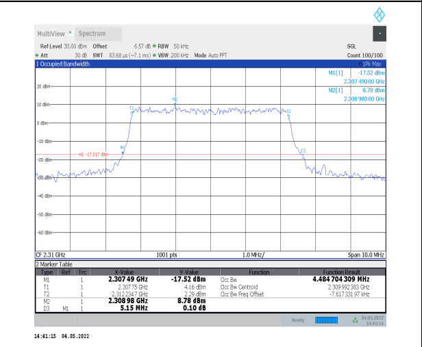
1-N30--15-5-M-7-CP-16QAM-Outer_Full-25@0-Ant0- -4.485-5.150-<math>\leq</math>5-PASS
