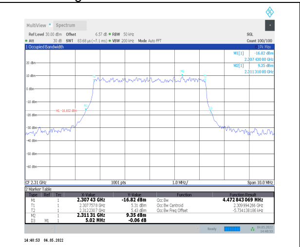
1-N30--15-5-M-5-DFT-256QAM-Outer_Full-25@0-An t0-4.473-5.020-<math>\leq</math>5-PASS
