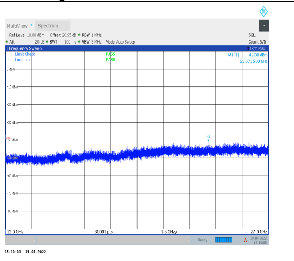
1-N30--15-10-H-1-DFT-PI2BPSK-Inner_1RB_Left-1 @1-12000-27000-Ant0--41.30--40-PASS
