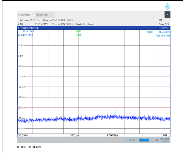
1-N30--15-10-H-1-DFT-PI2BPSK-Inner_1RB_Left-1 @1-30-1000-Ant0--55.75--50-PASS
