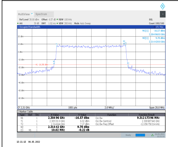
1-N30--15-10-M-7-CP-16QAM-Outer_Full-52@0-Ant0-9.312-10.020-≤10-PASS
