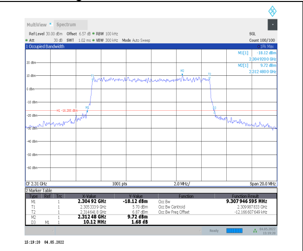
1-N30--15-10-L-7-CP-16QAM-Outer_Full-52@0-Ant0 -9.308-10.120≤10-PASS
