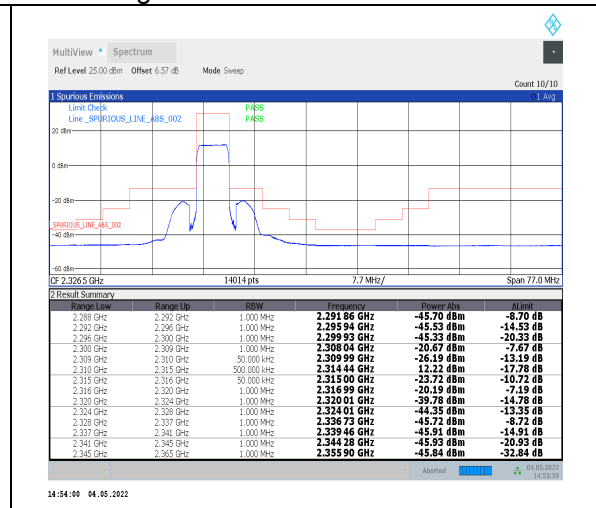
1-N30--15-5-H-3-DFT-PI2BPSK-Outer_Full-25@0 -Ant0-PASS-see graph
