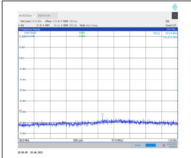
1-N30--15-10-M-1-DFT-PI2BPSK-Inner_1RB_Left-1 @1-30-1000-Ant0--55.24--50-PASS
