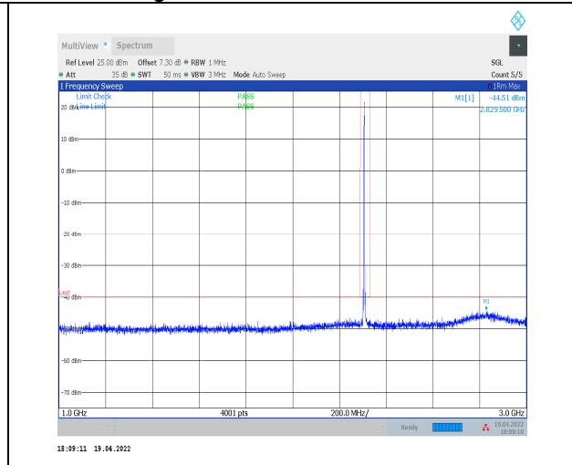
1-N30--15-10-M-1-DFT-PI2BPSK-Inner_1RB_Left-1 @1-1000-3000-Ant0--44.51--40-PASS
