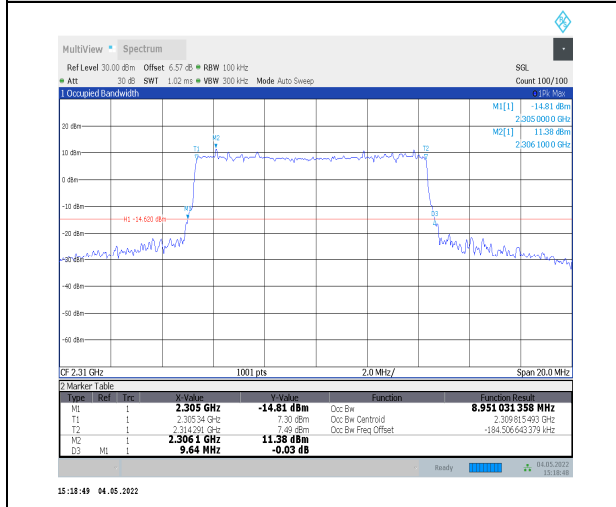
1-N30--15-10-L-4-DFT-64QAM-Outer_Full-50@0-A t0-8.951-9.640≤10-PASS
