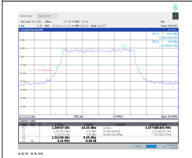
1-N30--15-5-H-5-DFT-256QAM-Outer_Full-25@0-Ant t0-4.477-5.160-≤5-PASS
