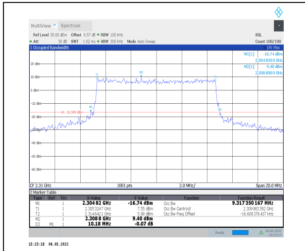
1-N30--15-10-H-8-CP-64QAM-Outer_Full-52@0-An 0-9.317-10.180-≤10-PASS
