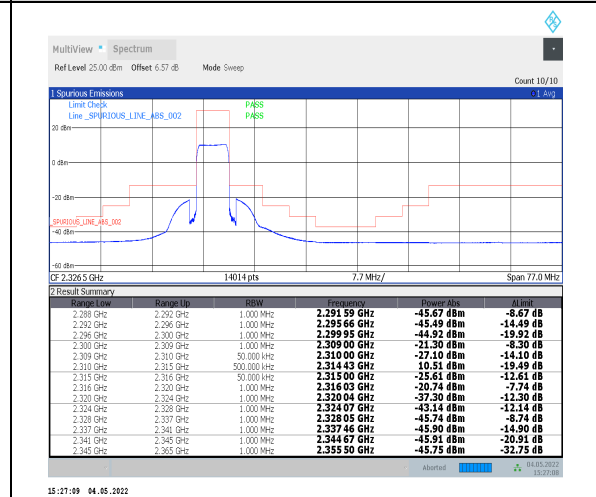
1-N30--15-5-H-6-CP-QPSK-Outer_Full-25@0-Ant 0-PASS-see graph
