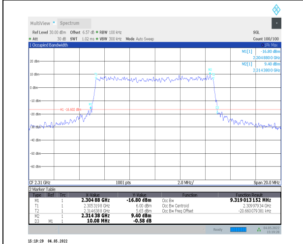
1-N30--15-10-L-8-CP-64QAM-Outer_Full-52@0-Ant 0-9.319-10.080≤10-PASS
