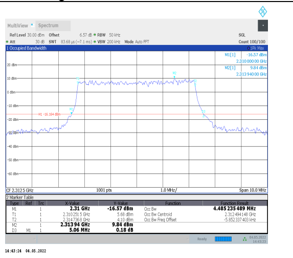
1-N30--15-5-H-8-CP-64QAM-Outer_Full-25@0-Ant0 4.485-5.060-≤5-PASS
