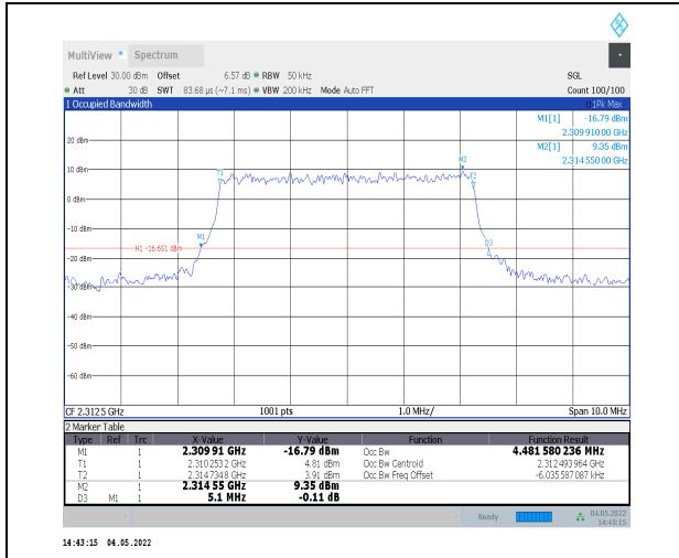
1-N30--15-5-H-7-CP-16QAM-Outer_Full-25@0-Ant0 -4.482-5.100-≤5-PASS
