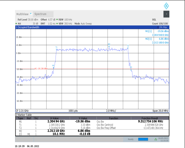
1-N30--15-10-L-9-CP-256QAM-Outer_Full-52@0-Ant 0-9.313-10.100≤10-PASS
