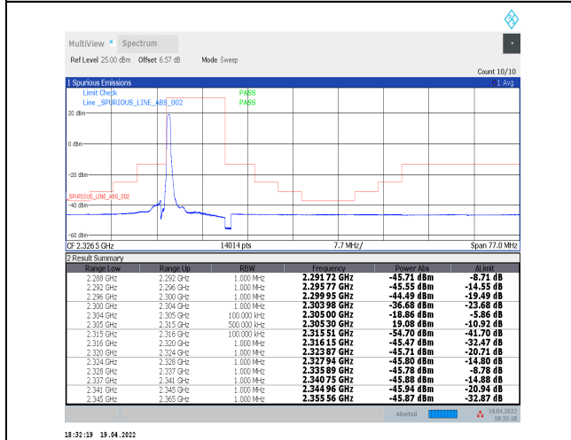
1-N30--30-10-L-4-CP-QPSK-Edge_1RB_Left-1@0-Ant0-PASS-see graph
