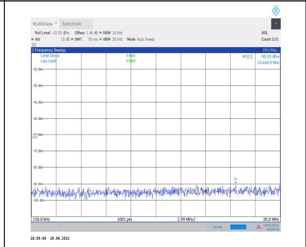
1-N30--15-10-M-1-DFT-PI2BPSK-Inner_1RB_Left-1 @1-0.15-30-Ant0--90.20--60-PASS
