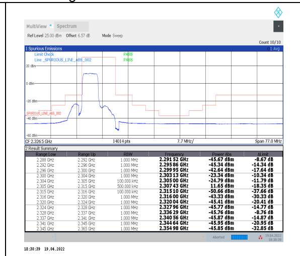
1-N30--30-10-L-3-DFT-PI2BPSK-Outer_Full-24@0-Ant0-PASS-see graph
