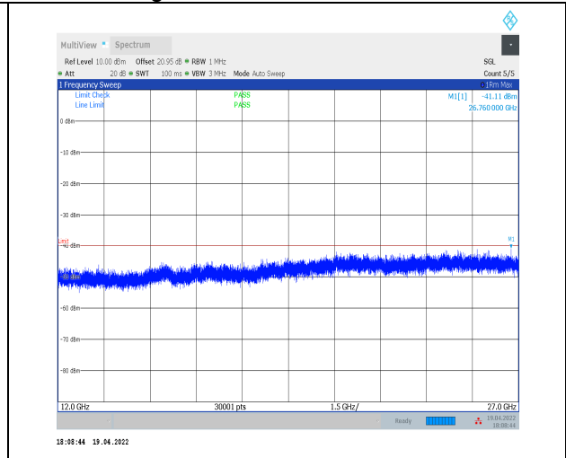
1-N30--15-10-L-1-DFT-PI2BPSK-Inner_1RB_Left-1 @1-12000-27000-Ant0--41.11--40-PASS
