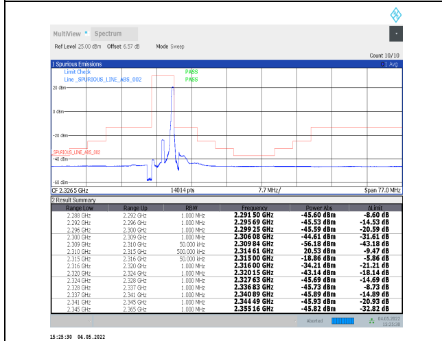
1-N30--15-5-H-5-CP-QPSK-Edge_1RB_Right-1@24-A nt0-PASS-see graph
