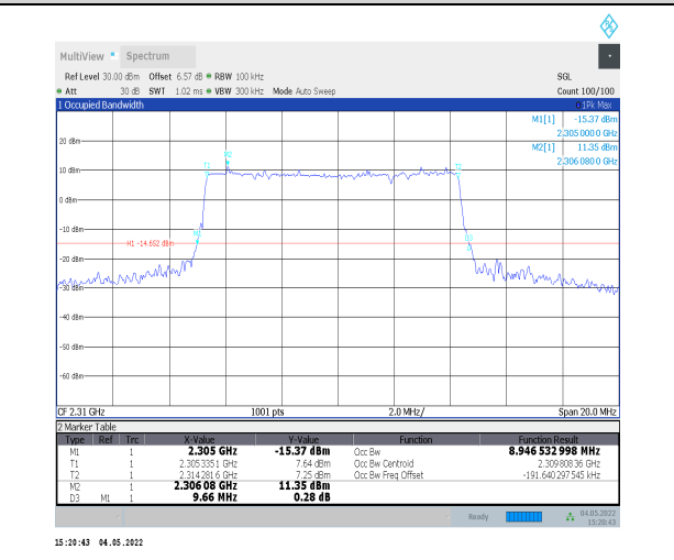
1-N30--15-10-M-4-DFT-64QAM-Outer_Full-50@0-An t0-8.947-9.660-<=10-PASS
