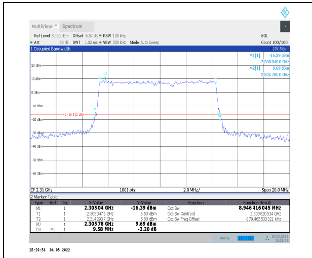
1-N30--15-10-M-5-DFT-256QAM-Outer_Full-50@0-Ant0-8.946-9.580-≤10-PASS
