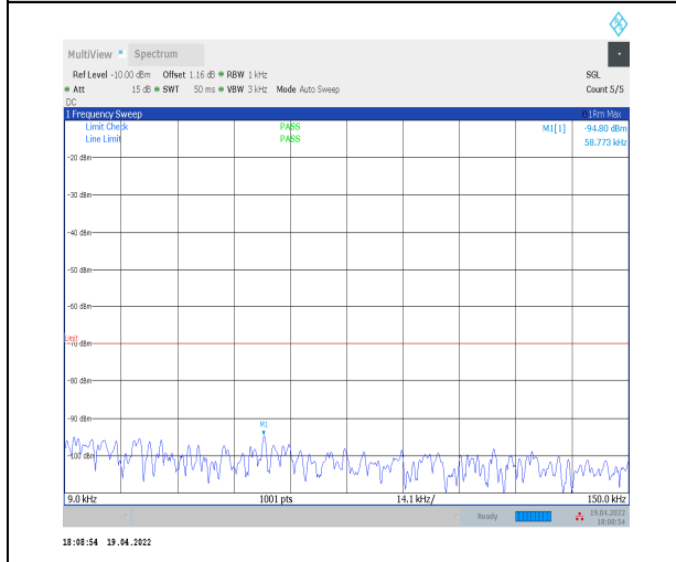
1-N30--15-10-M-1-DFT-PI2BPSK-Inner_1RB_Left-1 @1-0.009-0.15-Ant0--94.80--70-PASS
