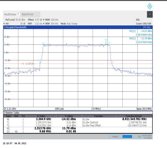
1-N30--15-10-L-1-DFT-QPSK-Outer_Full-50@0-Ant0 -8.922-9.680-≤10-PASS
