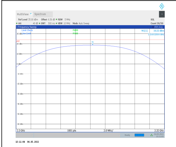
1-N30-PC3-15-10-M-3-DFT-PI2BPSK-Outer_Full-50 @0-2300-2320-Ant0-18.53-23.98-PASS
