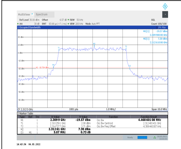
1-N30--15-5-H-9-CP-256QAM-Outer_Full-25@0-Ant 0-4.469-5.070-≤5-PASS
