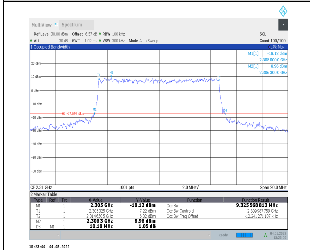
1-N30--15-10-H-6-CP-QPSK-Outer_Full-52@0-Ant0 9.326-10.180-≤10-PASS
