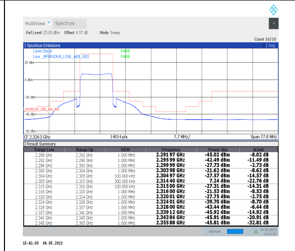
1-N30--15-10-H-6-CP-QPSK-Outer_Full-52@0-Ant0-PASS-see graph
