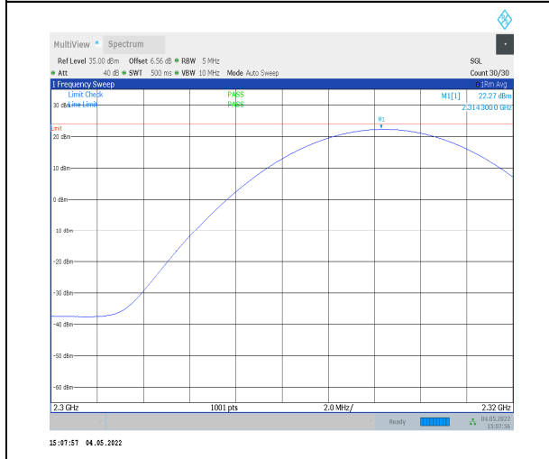
1-N30-PC3-15-10-L-2-DFT-PI2BPSK-Inner_1RB_Ri ght-1@50-2300-2320-Ant0-22.27-23.98-PASS
