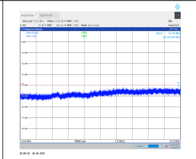
1-N30--15-10-M-1-DFT-PI2BPSK-Inner_1RB_Left-1 @1-12000-27000-Ant0--41.20--40-PASS
