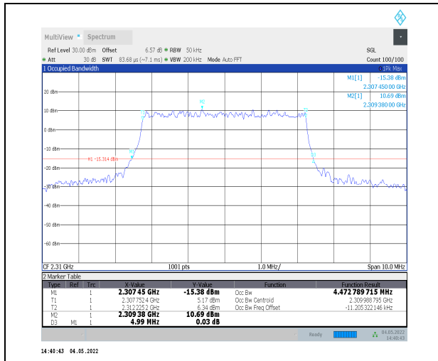
1-N30--15-5-M-4-DFT-64QAM-Outer_Full-25@0-Ant 0-4.473-4.990-<math>\leq</math>5-PASS
