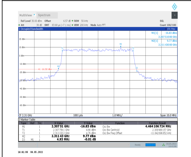
1-N30--15-5-M-6-CP-QPSK-Outer_Full-25@0-Ant0- 4.464-4.930-<math>\leq</math>5-PASS
