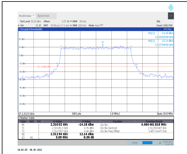
1-N30--15-5-H-3-DFT-16QAM-Outer_Full-25@0-Ant 0-4.484-5.090-≤5-PASS
