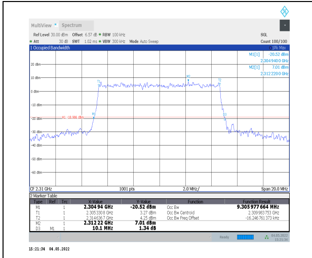
1-N30--15-10-M-9-CP-256QAM-Outer_Full-52@0-A nt0-9.306-10.100-<=10-PASS
