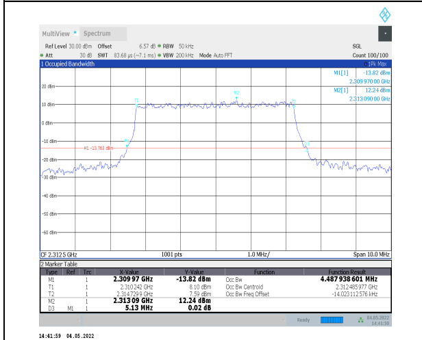
1-N30--15-5-H-1-DFT-QPSK-Outer_Full-25@0-Ant0 4.488-5.130-≤5-PASS
