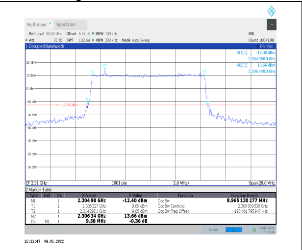
1-N30--15-10-H-1-DFT-QPSK-Outer_Full-50@0-Ant 0-8.965-9.580-<=10-PASS
