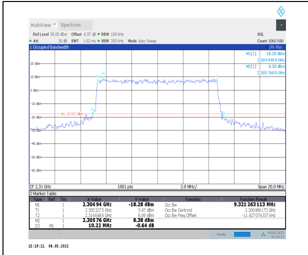
1-N30--15-10-L-6-CP-QPSK-Outer_Full-52@0-Ant0 9.321-10.220≤10-PASS
