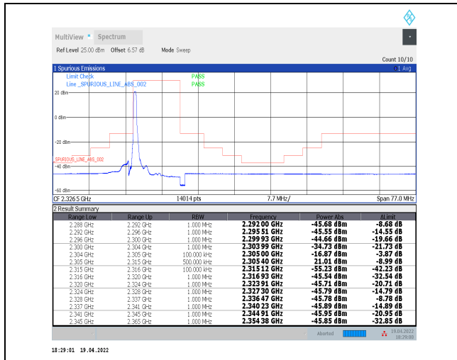
1-N30--30-10-L-1-DFT-PI2BPSK-Edge_1RB_Left-1@0-Ant0-PASS-see graph
