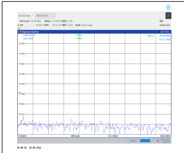
1-N30--15-10-H-1-DFT-PI2BPSK-Inner_1RB_Left-1 @1-0.009-0.15-Ant0--94.08--70-PASS
