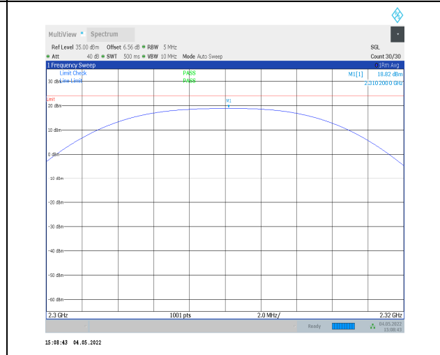
1-N30-PC3-15-10-L-3-DFT-PI2BPSK-Outter_Full-50 @0-2300-2320-Ant0-18.82-23.98-PASS
