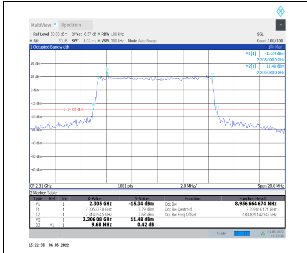
1-N30--15-10-H-4-DFT-64QAM-Outer_Full-50@0-Ant t0-8.957-9.680-≤10-PASS
