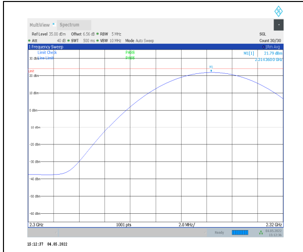
1-N30-PC3-15-10-H-2-DFT-PI2BPSK-Inner_1RB_Ri ght-1@50-2300-2320-Ant0-21.79-23.98-PASS
