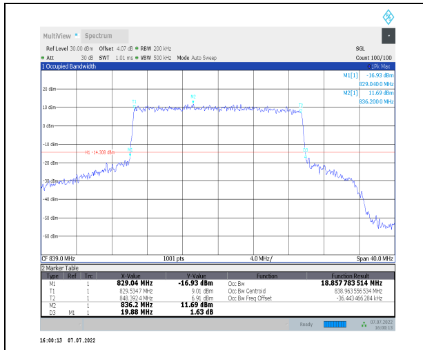
1-N26-824-849--15-20-H-6-CP-QPSK-Outer_Full-1 6@0-Ant0-18.858-19.880-≤20-PASS
