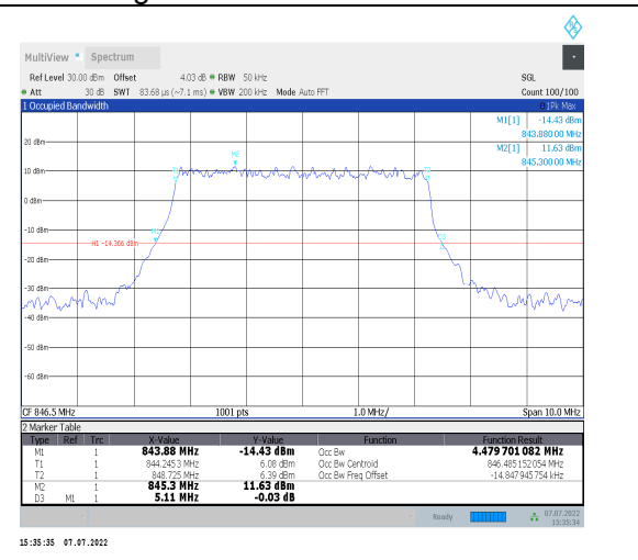
1-N26-824-849--15-5-H-4-DFT-64QAM-Outer_Full-2 5@0-Ant0-4.48-5.110-<math>\leq</math>5-PASS
