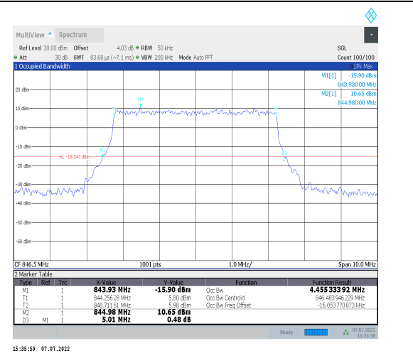
1-N26-824-849--15-5-H-6-CP-QPSK-Outer_Full-25 @0-Ant0-4.455-5.010-<math>\leq</math>5-PASS
