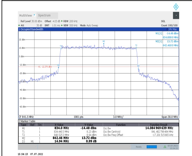
1-N26-824-849--15-15-H-7-CP-16QAM-Outer_Full-7 9@0-Ant0-14.085-14.940-<=15-PASS
