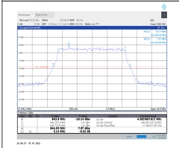
1-N26-824-849--15-5-H-9-CP-256QAM-Outer_Full-2 5@0-Ant0-4.504-5.140-<math>\leq</math>5-PASS
