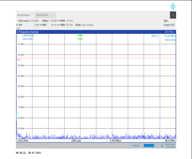
1-N26-824-849-PC3-15-20-H-1-DFT-PI2BPSK-Inner _1RB_Left-1@1-0.15-30-Ant0--78.48--33-PASS
