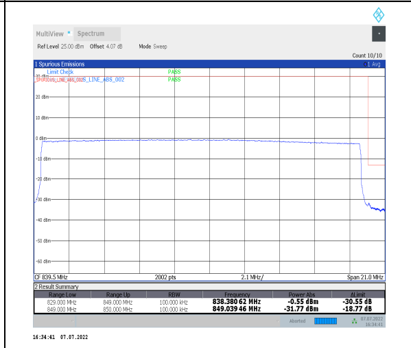
1-N26-824-849--15-20-H-6-CP-QPSK-Outer_Full-106@0-Ant0-seegraph-PASS-see graph
