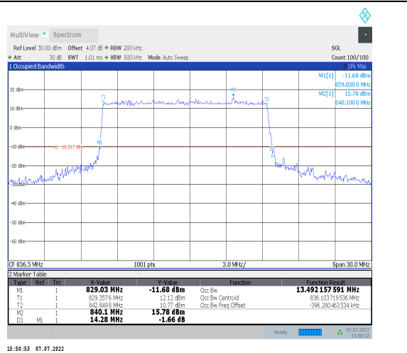
1-N26-824-849--15-15-M-1-DFT-QPSK-Outer_Full-7 5@0-Ant0-13.492-14.280-≤15-PASS
