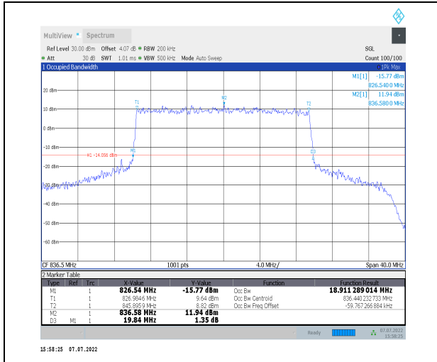
1-N26-824-849--15-20-M-7-CP-16QAM-Outer_Full-1 06@0-Ant0-18.911-19.840-≤20-PASS
