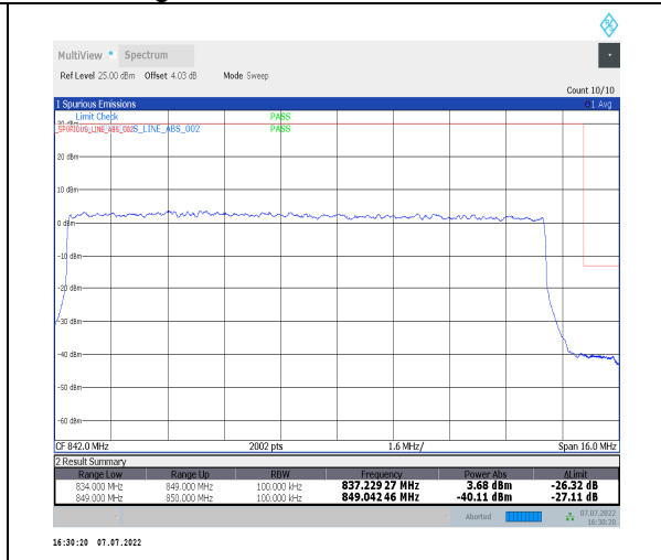
1-N26-824-849--15-15-H-3-DFT-PI2BPSK-Outer_Full-75@0-Ant0-seegraph-PASS-see graph
