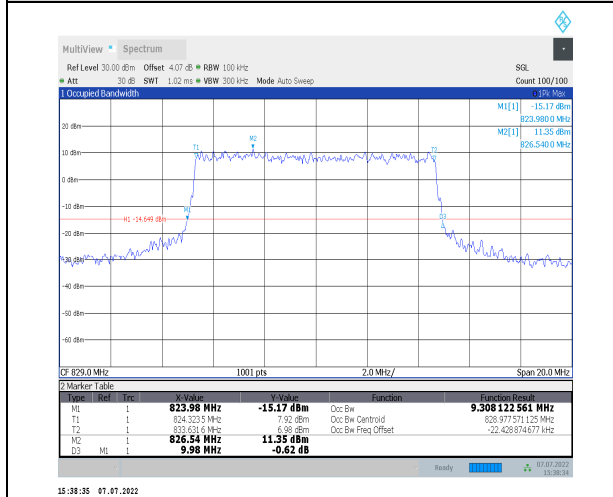
1-N26-824-849--15-10-L-8-CP-64QAM-Outer_Full-5 2@0-Ant0-9.308-9.980-≤10-PASS
