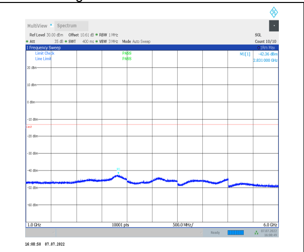
1-N26-824-849-PC3-15-20-H-1-DFT-PI2BPSK-Inner _1RB_Left-1@1-1000-6000-Ant0--42.36--13-PASS
