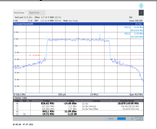
1-N26-824-849--15-20-M-8-CP-64QAM-Outer_Full-1 06@0-Ant0-18.87-19.720-≤20-PASS
