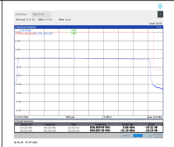
1-N26-824-849--15-15-H-6-CP-QPSK-Outer_Full-79@0-Ant0-seegraph-PASS-see graph
