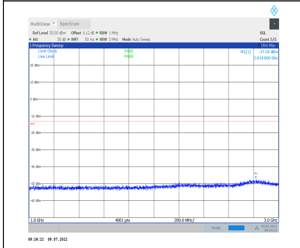
1-N26-824-849-PC3-15-20-H-1-DFT-PI2BPSK-Inner _1RB_Left-1@1-1000-3000-Ant0--47.20--13-PASS
