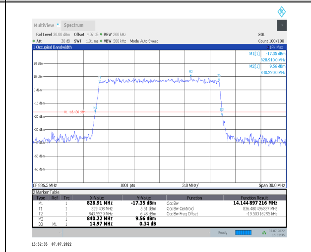
1-N26-824-849--15-15-M-9-CP-256QAM-Outer_Full-79 @0-Ant0-14.145-14.970-≤15-PASS
