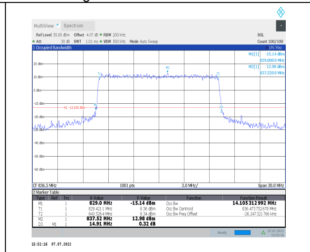
1-N26-824-849--15-15-M-7-CP-16QAM-Outer_Full-79 @0-Ant0-14.105-14.910-≤15-PASS
