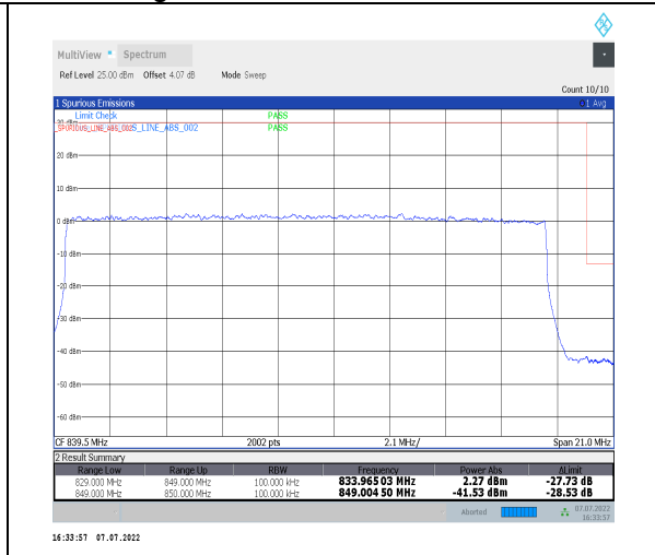
1-N26-824-849--15-20-H-3-DFT-PI2BPSK-Outer_Full-100@0-Ant0-seegraph-PASS-see graph
