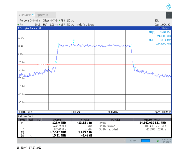
1-N26-824-849--15-15-L-7-CP-16QAM-Outer_Full-7 9@0-Ant0-14.142-15.210-≤15-PASS
