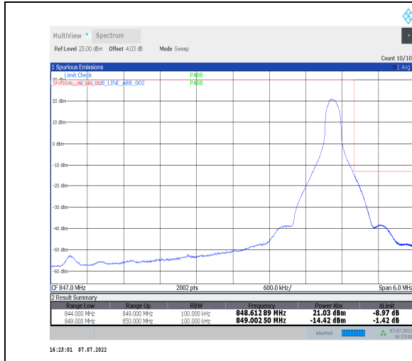
1-N26-824-849--15-5-H-2-DFT-PI2BPSK-Edge_1RB_Right-1@24-Ant0-seegraph-PASS-see graph
