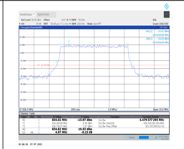
1-N26-824-849--15-5-M-7-CP-16QAM-Outer_Full-25 @0-Ant0-4.479-4.970-<5-PASS
