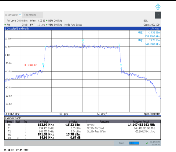
1-N26-824-849--15-15-H-8-CP-64QAM-Outer_Full-7 9@0-Ant0-14.147-14.910-<=15-PASS
