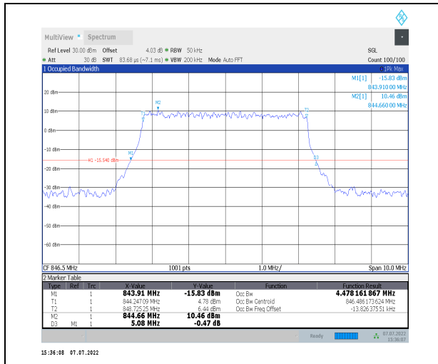
1-N26-824-849--15-5-H-7-CP-16QAM-Outer_Full-25 @0-Ant0-4.478-5.080-<math>\leq</math>5-PASS
