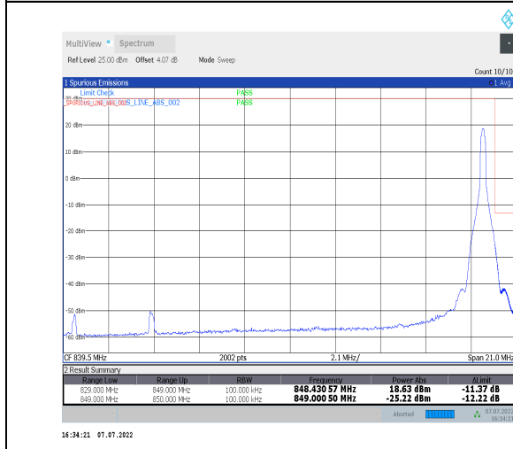
1-N26-824-849--15-20-H-5-CP-QPSK-Edge_1RB_Right-1@105-Ant0-seegraph-PASS-see graph
