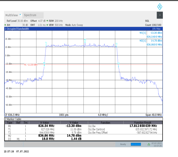
1-N26-824-849--15-20-M-2-DFT-PI2BPSK-Outer_Ful I-100@0-Ant0-17.813-18.800-<math>\leq 20</math>-PASS
