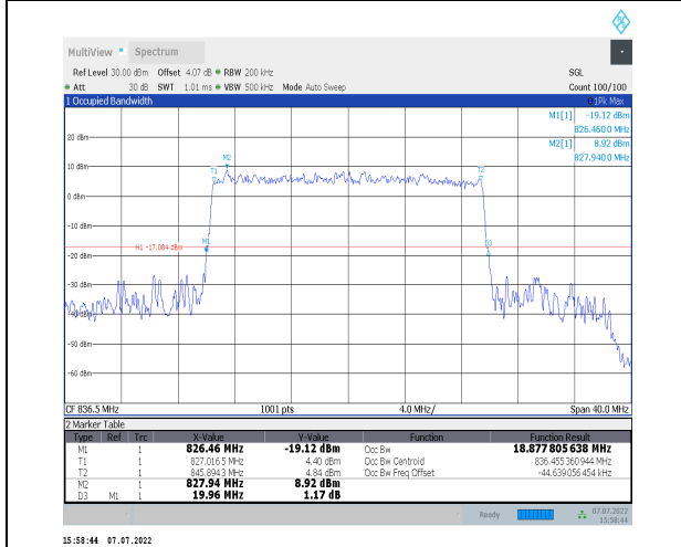
1-N26-824-849--15-20-M-9-CP-256QAM-Outer_Full-1 106@0-Ant0-18.878-19.960-≤20-PASS
