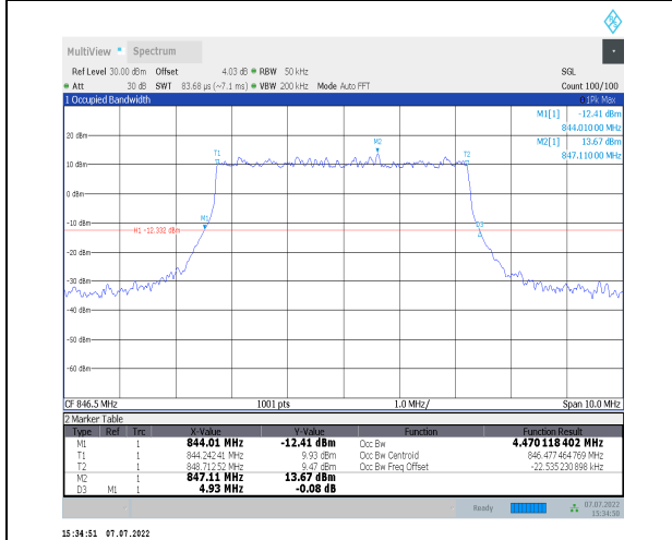
1-N26-824-849--15-5-H-1-DFT-QPSK-Outer_Full-25 @0-Ant0-4.47-4.930-<math>\leq</math>5-PASS
