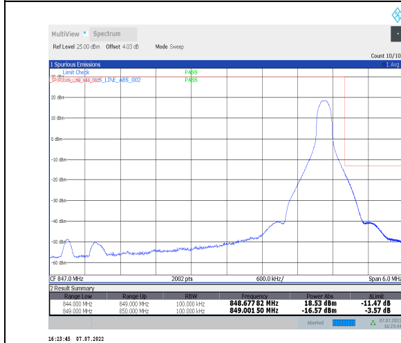
1-N26-824-849--15-5-H-5-CP-QPSK-Edge_1RB_Right-1@24-Ant0-seegraph-PASS-see graph
