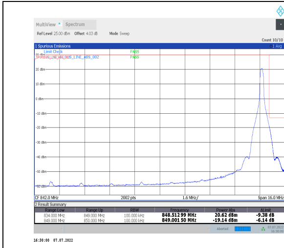
1-N26-824-849--15-15-H-2-DFT-PI2BPSK-Edge_1RB_Right-1@78-Ant0-seegraph-PASS-see graph
