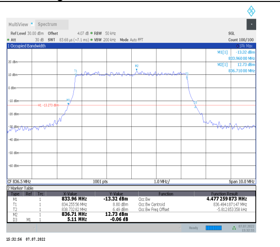
1-N26-824-849--15-5-M-1-DFT-QPSK-Outer_Full-25 @0-Ant0-4.477-5.110-<5-PASS
