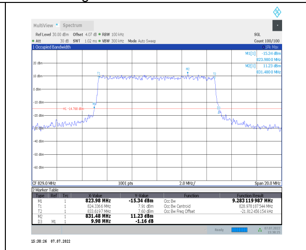
1-N26-824-849--15-10-L-7-CP-16QAM-Outer_Full-5 2@0-Ant0-9.283-9.980-≤10-PASS
