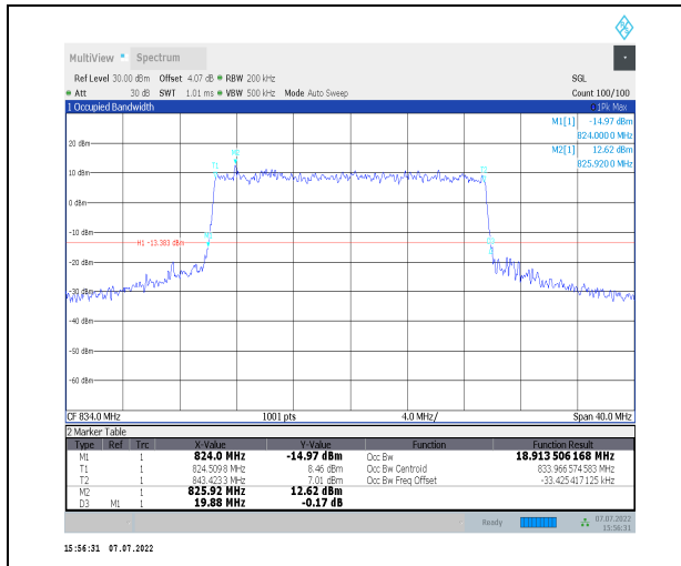
1-N26-824-849--15-20-L-8-CP-64QAM-Outer_Full-1 06@0-Ant0-18.914-19.880-<math>\leq 20</math>-PASS
