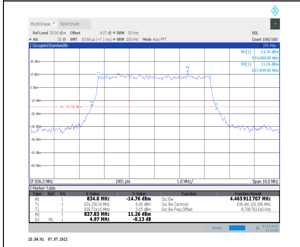
1-N26-824-849--15-5-M-6-CP-QPSK-Outer_Full-25 @0-Ant0-4.466-4.970-<5-PASS
