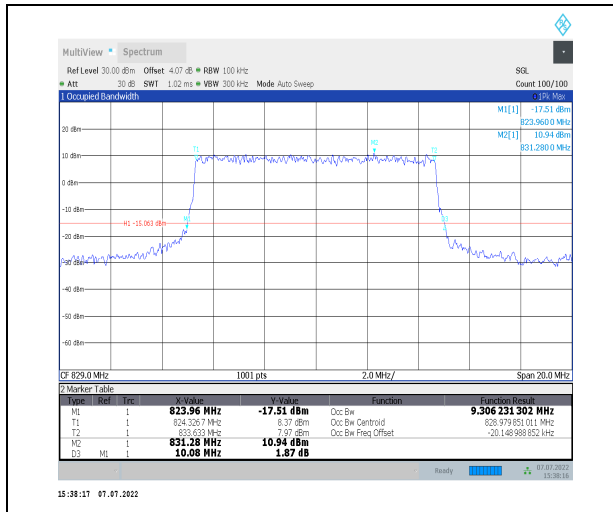
1-N26-824-849--15-10-L-6-CP-QPSK-Outer_Full-52 @0-Ant0-9.306-10.080-≤10-PASS
