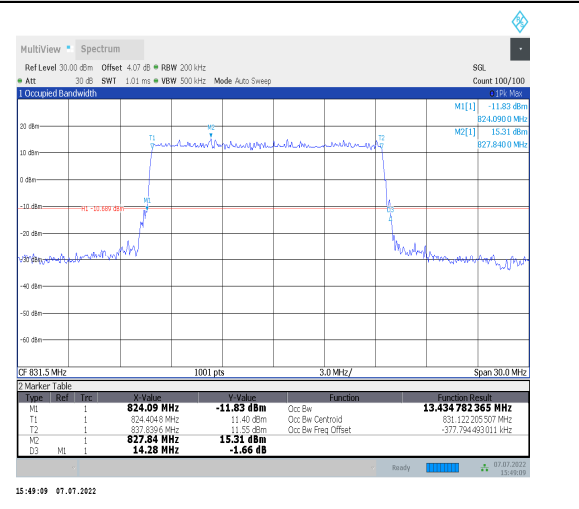
1-N26-824-849--15-15-L-2-DFT-PI2BPSK-Outer_Full7 5@0-Ant0-13.435-14.280-<=15-PASS
