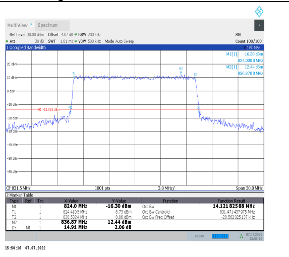
1-N26-824-849--15-15-L-8-CP-64QAM-Outer_Full-7 9@0-Ant0-14.122-14.910-≤15-PASS
