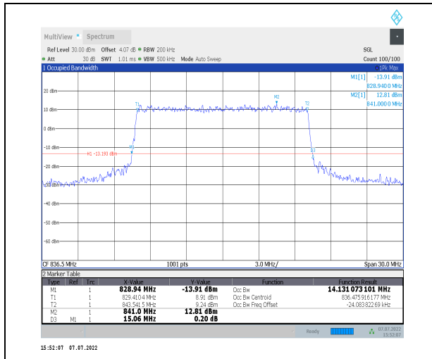
1-N26-824-849--15-15-M-6-CP-QPSK-Outer_Full-79 @0-Ant0-14.131-15.060-≤15-PASS
