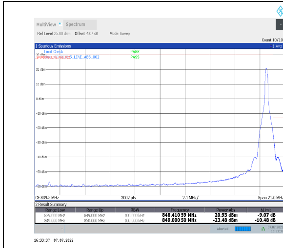
1-N26-824-849--15-20-H-2-DFT-PI2BPSK-Edge_1RB_Right-1@105-Ant0-seegraph-PASS-see graph
