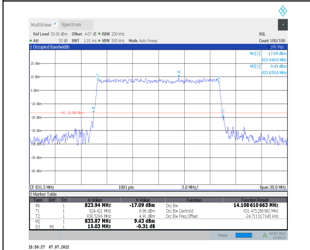
1-N26-824-849--15-15-L-9-CP-256QAM-Outer_Full-7 79@0-Ant0-14.109-15.030-≤15-PASS
