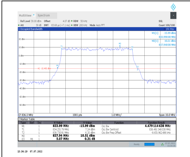
1-N26-824-849--15-5-M-8-CP-64QAM-Outer_Full-25 @0-Ant0-4.479-5.070-<math>\leq</math>5-PASS
