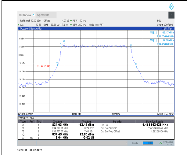
1-N26-824-849--15-5-M-2-DFT-PI2BPSK-Outer_Full-25 -25@0-Ant0-4.465-5.040-<5-PASS
