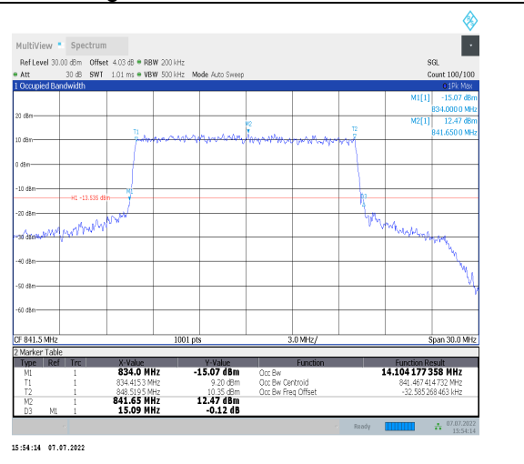
1-N26-824-849--15-15-H-6-CP-QPSK-Outer_Full-79 @0-Ant0-14.104-15.090-<=15-PASS
