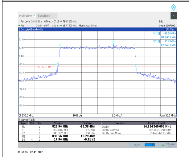
1-N26-824-849--15-15-M-8-CP-64QAM-Outer_Full-79 @0-Ant0-14.154-14.940-≤15-PASS
