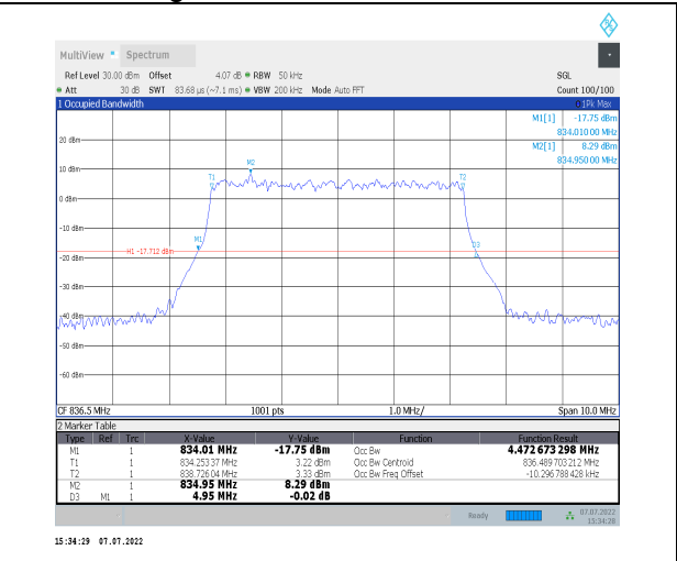
1-N26-824-849--15-5-M-9-CP-256QAM-Outer_Full-2 5@0-Ant0-4.473-4.950-<math>\leq</math>5-PASS
