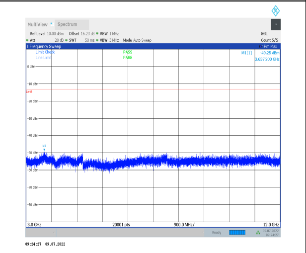
1-N26-824-849-PC3-15-20-H-1-DFT-PI2BPSK-Inner _1RB_Left-1@1-3000-12000-Ant0--49.25--13-PASS
