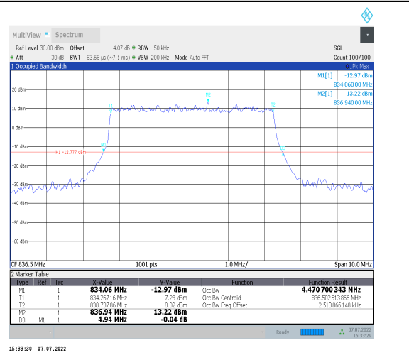
1-N26-824-849--15-5-M-3-DFT-16QAM-Outer_Full-2 5@0-Ant0-4.471-4.940-<5-PASS
