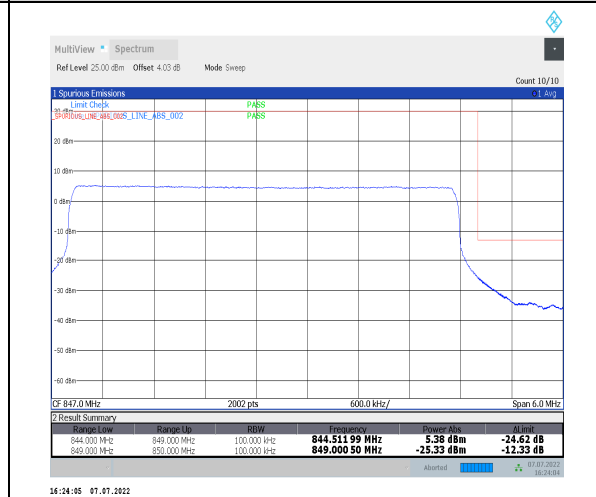
1-N26-824-849--15-5-H-6-CP-QPSK-Outer_Full-25@0-Ant0-seegraph-PASS-see graph
