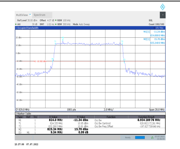
1-N26-824-849--15-10-L-1-DFT-QPSK-Outer_Full-50 @0-Ant0-8.934-9.540-<math>\leq</math>10-PASS
