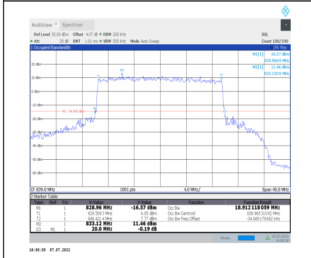
1-N26-824-849--15-20-H-8-CP-64QAM-Outer_Full-1 06@0-Ant0-18.912-20.000-≤20-PASS
