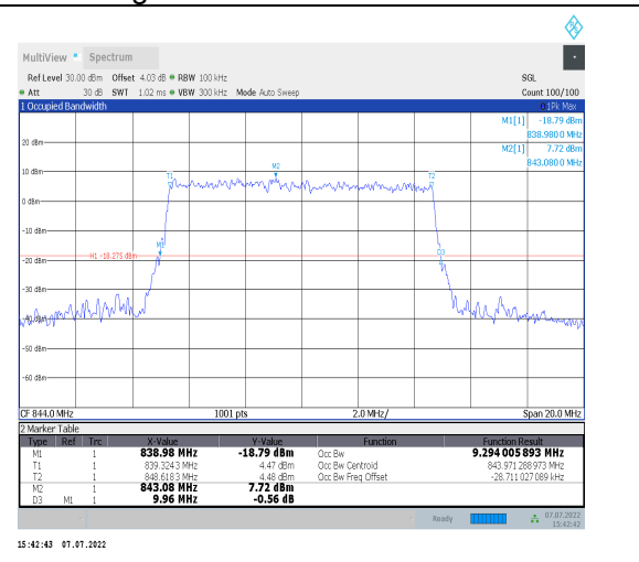
1-N26-824-849--15-10-H-9-CP-256QAM-Outer_Full5 2@0-Ant0-9.294-9.960-<=10-PASS
