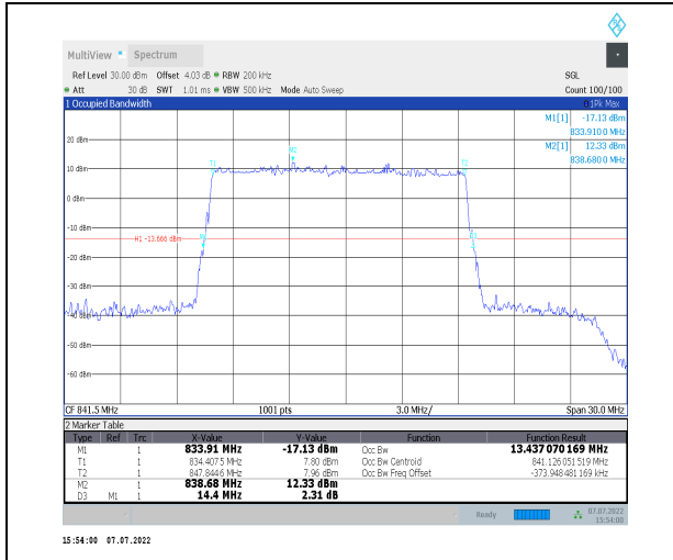
1-N26-824-849--15-15-H-5-DFT-256QAM-Outer_Full -75@0-Ant0-13.437-14.400-<=15-PASS
