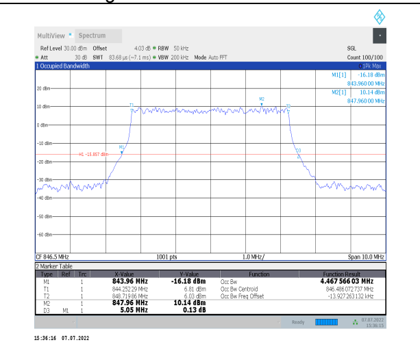
1-N26-824-849--15-5-H-8-CP-64QAM-Outer_Full-25 @0-Ant0-4.468-5.050-<math>\leq</math>5-PASS
