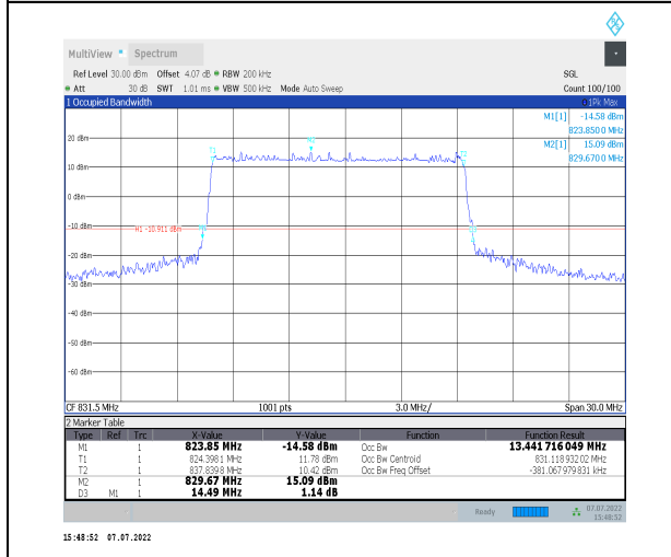
1-N26-824-849--15-15-L-1-DFT-QPSK-Outer_Full7 5@0-Ant0-13.442-14.490-<=15-PASS
