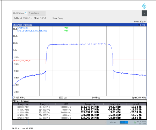
1-N26-814-824--15-10-M-6-CP-QPSK-Outer_Full-52@0-Ant0-PASS-see graph
