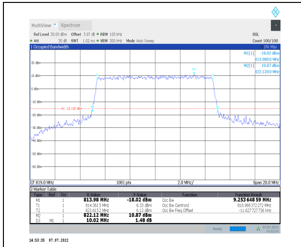
1-N26-814-824--15-10-M-6-CP-QPSK-Outer_Full-52 @0-Ant0-9.254-10.020-≤10-PASS
