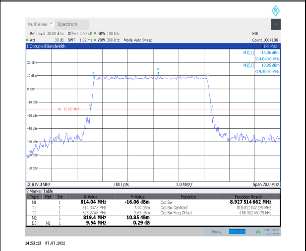
1-N26-814-824--15-10-M-5-DFT-256QAM-Outer_Full I-50@0-Ant0-8.928-9.540-≤10-PASS
