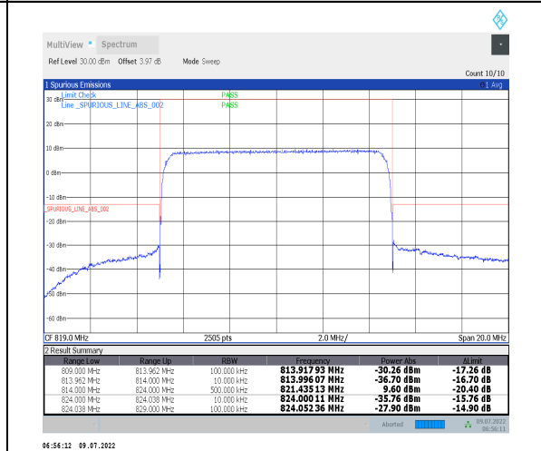
1-N26-814-824--15-10-M-6-CP-QPSK-Outer_Full-52@0-Ant0-PASS-see graph
