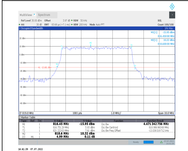
1-N26-814-824--15-5-M-6-CP-QPSK-Outer_Full-25@0-Ant0-4.471-4.990-≤5-PASS
