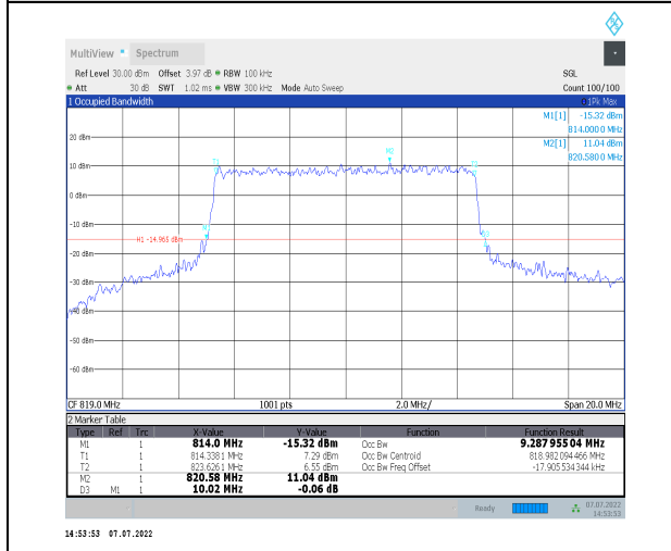
1-N26-814-824--15-10-M-8-CP-64QAM-Outer_Full-5 2@0-Ant0-9.288-10.020-≤10-PASS
