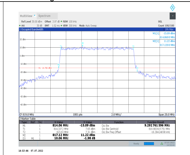
1-N26-814-824--15-10-M-7-CP-16QAM-Outer_Full-5 2@0-Ant0-9.293-10.060-≤10-PASS
