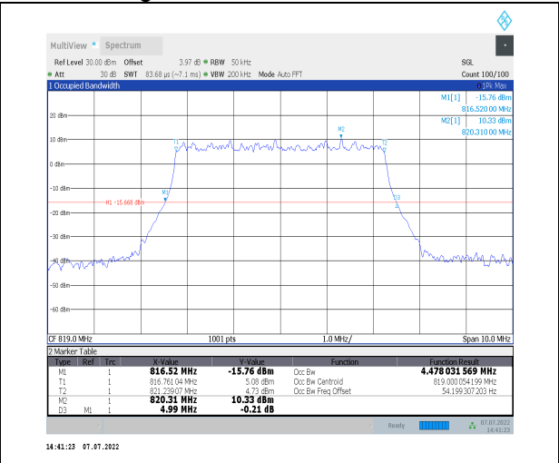
1-N26-814-824--15-5-M-5-DFT-256QAM-Outer_Full-25@0-Ant0-4.478-4.990-≤5-PASS
