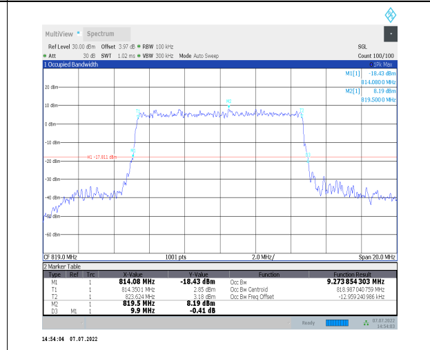
1-N26-814-824--15-10-M-9-CP-256QAM-Outer_Full- 52@0-Ant0-9.274-9.900-≤10-PASS
