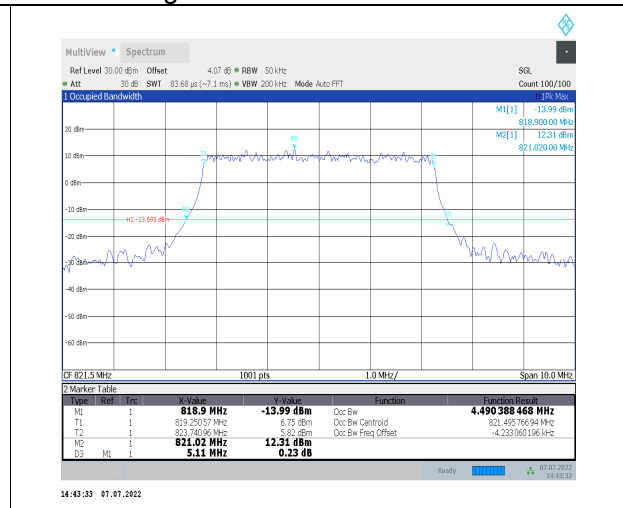
1-N26-814-824--15-5-H-4-DFT-64QAM-Outer_Full-2 5@0-Ant0-4.49-5.110-≤5-PASS
