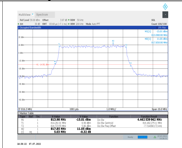
1-N26-814-824--15-5-L-6-CP-QPSK-Outer_Full-25@ 0-Ant0-4.463-5.030-≤5-PASS
