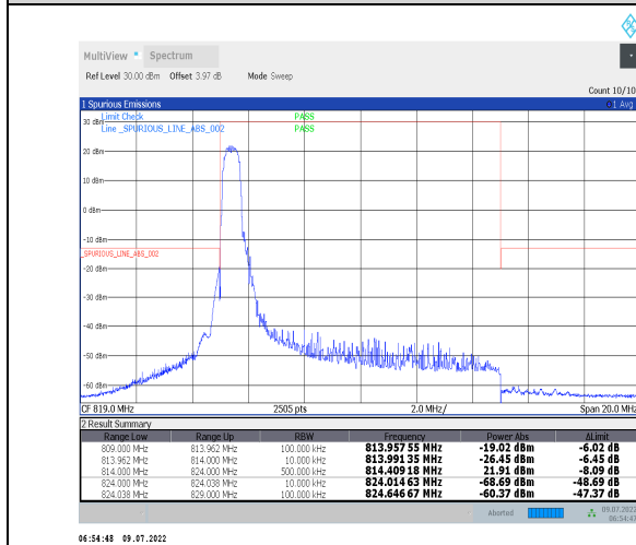
1-N26-814-824--15-10-M-4-CP-QPSK-Edge_1RB_Left-1@0-Ant0-PASS-see graph
