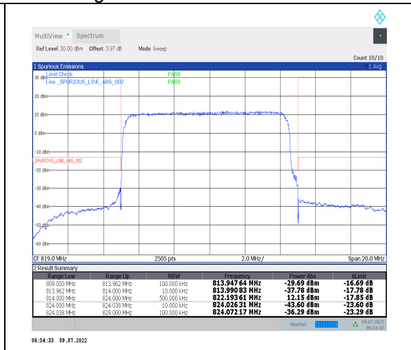
1-N26-814-824--15-10-M-3-DFT-PI2BPSK-Outer_Full-50@0-Ant0-PASS-see graph
