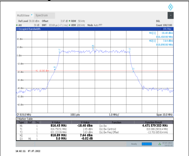
1-N26-814-824--15-5-M-9-CP-256QAM-Outer_Full-2 5@0-Ant0-4.472-5.000-<math>\leq</math>5-PASS
