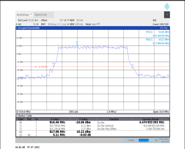
1-N26-814-824--15-5-M-7-CP-16QAM-Outer_Full-25@0-Ant0-4.475-5.110-≤5-PASS
