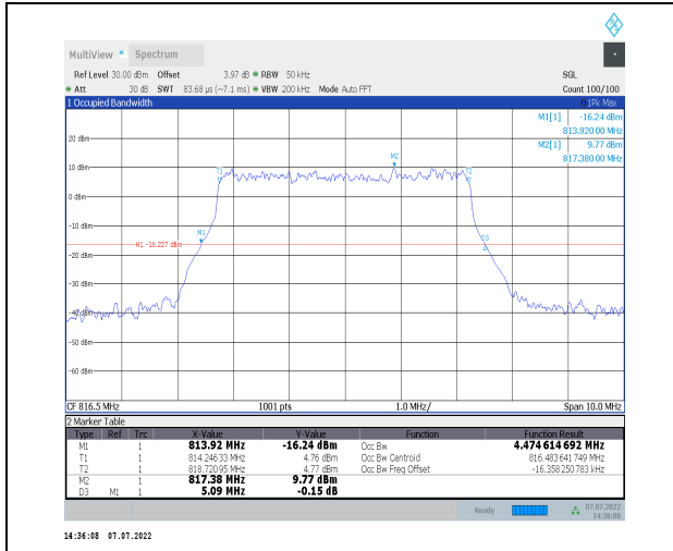
1-N26-814-824--15-5-L-5-DFT-256QAM-Outer_Full-2 @0-Ant0-4.475-5.090-≤5-PASS
