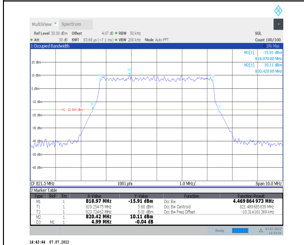
1-N26-814-824--15-5-H-5-DFT-256QAM-Outer_Full-2 25@0-Ant0-4.47-4.990-≤5-PASS
