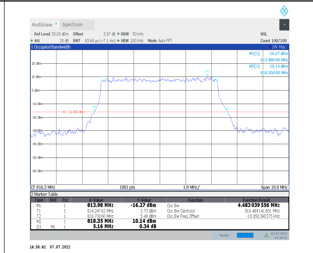
1-N26-814-824--15-5-L-8-CP-64QAM-Outer_Full-25 @0-Ant0-4.483-5.160-≤5-PASS
