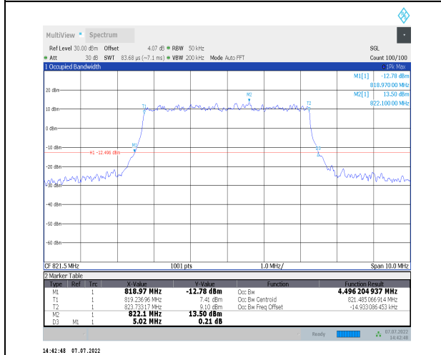
1-N26-814-824--15-5-H-1-DFT-QPSK-Outer_Full-25 @0-Ant0-4.496-5.020-<math>\leq</math>5-PASS
