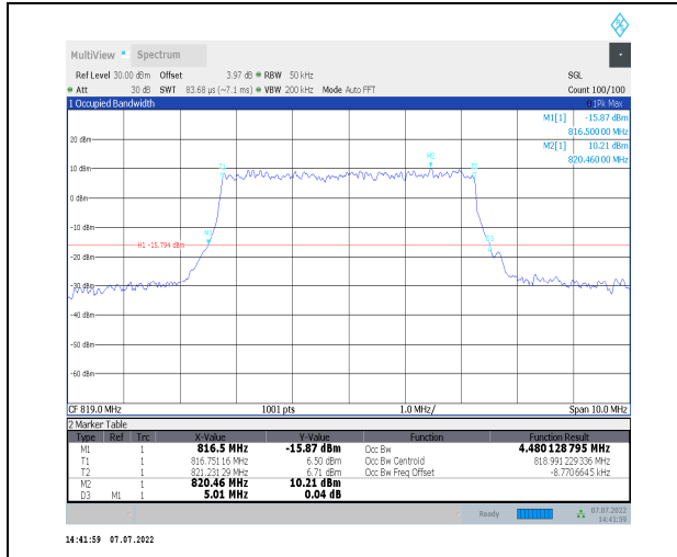
1-N26-814-824--15-5-M-8-CP-64QAM-Outer_Full-25 @0-Ant0-4.48-5.010-<math>\leq</math>5-PASS
