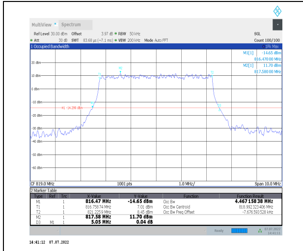
1-N26-814-824--15-5-M-4-DFT-64QAM-Outer_Full-2 5@0-Ant0-4.467-5.050-≤5-PASS
