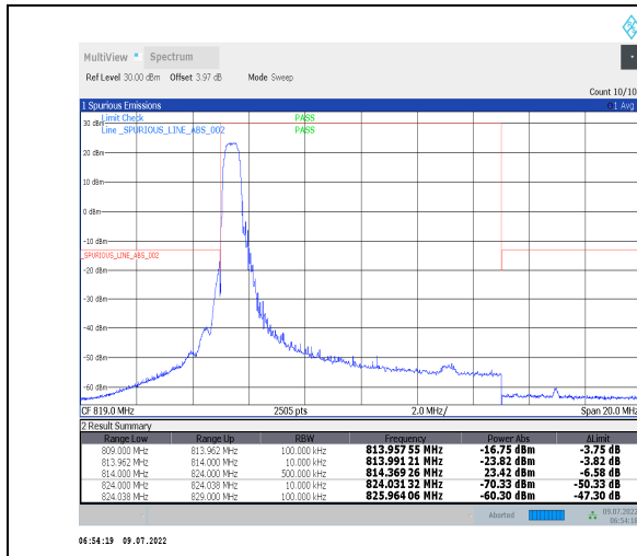
1-N26-814-824--15-10-M-1-DFT-PI2BPSK-Edge_1RB_Left-1@0-Ant0-PASS-see graph
