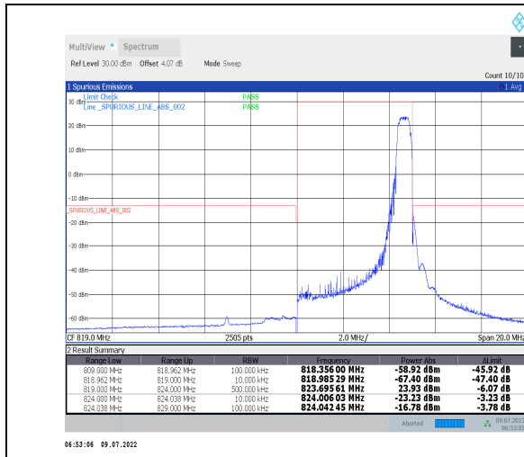
1-N26-814-824--15-5-H-2-DFT-PI2BPSK-Edge_1RB_Right-1@24-Ant0-PASS-see graph
