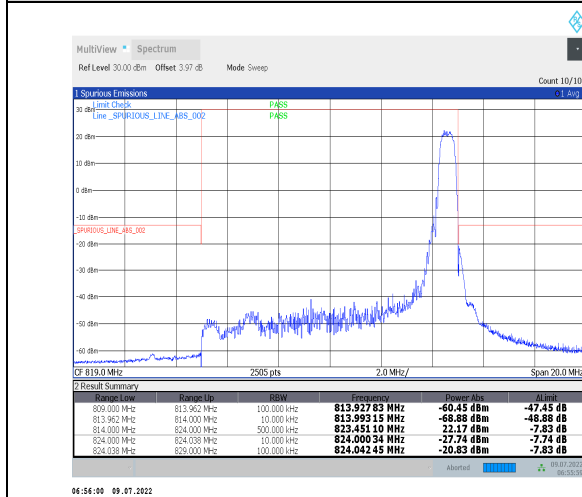
1-N26-814-824--15-10-M-5-CP-QPSK-Edge_1RB_Right-1@51-Ant0-PASS-see graph
