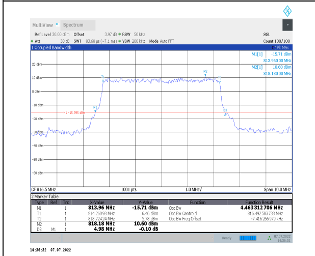
1-N26-814-824--15-5-L-7-CP-16QAM-Outer_Full-25 @0-Ant0-4.463-4.980-≤5-PASS
