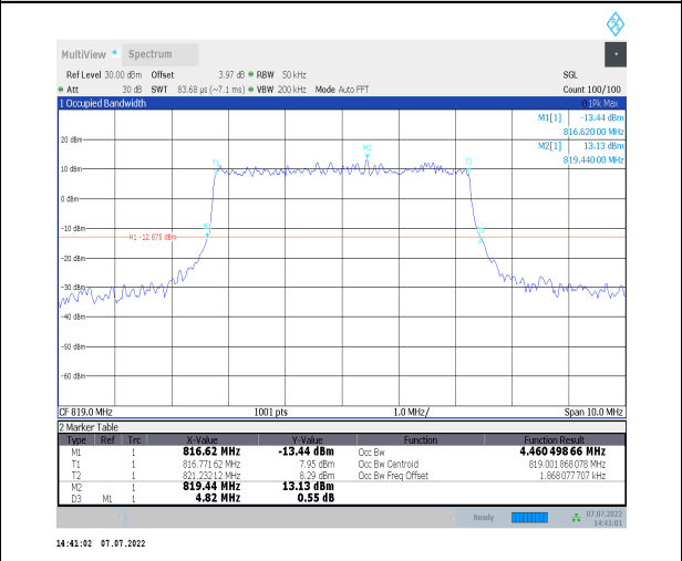
1-N26-814-824--15-5-M-3-DFT-16QAM-Outer_Full-25@0-Ant0-4.46-4.820-≤5-PASS
