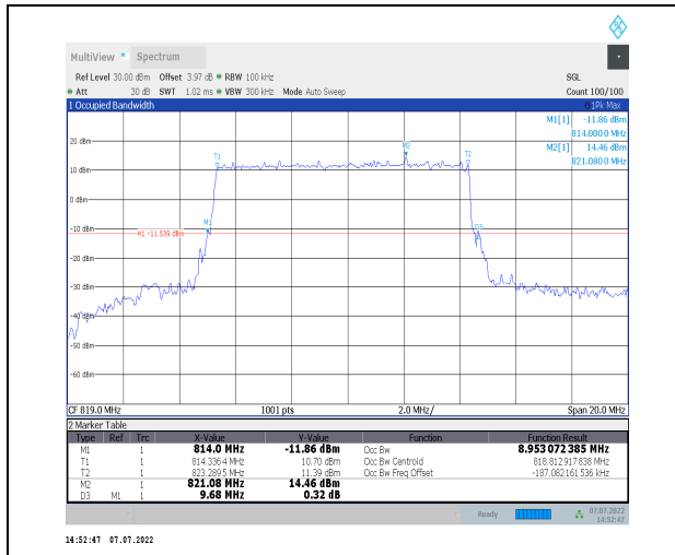
1-N26-814-824--15-10-M-2-DFT-PI2BPSK-Outer_Full I-50@0-Ant0-8.953-9.680-≤10-PASS
