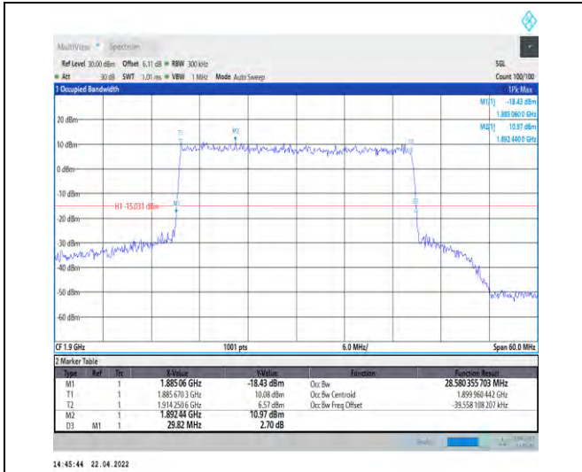
1-N25--15-30-H-4-DFT-64QAM-Outer_Full-160@0-A nt0-28.58-29.820-≤30-PASS
