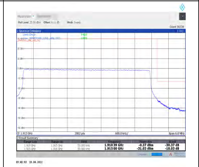
1-N25--15-5-H-6-CP-QPSK-Outer_Full-25@0-Ant0-seegraph-PASS-see graph
