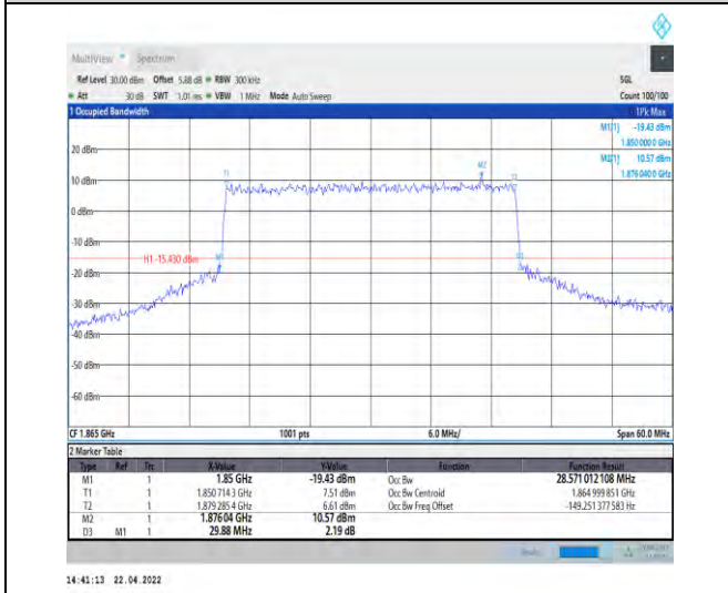
1-N25--15-30-L-8-CP-64QAM-Outer_Full-160@0-Ant0 -28.571-29.880-≤30-PASS
