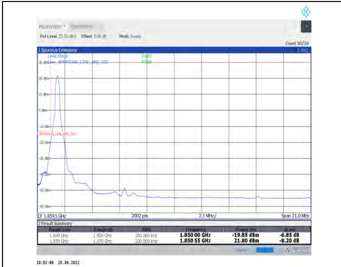
1-N25--15-20-L-1-DFT-PI2BPSK-Edge_1RB_Left-1@0-Ant0-seegraph-PASS-see graph
