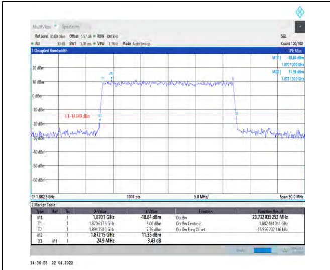
1-N25--15-25-M-8-CP-64QAM-Outer_Full-133@0-A nt0-23.733-24.900-<math>\leq 25</math>-PASS
