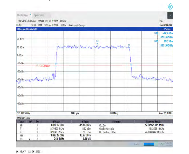
1-N25--15-25-M-1-DFT-QPSK-Outer_Full-128@0-An t0-22.89-24.000-<25-PASS
