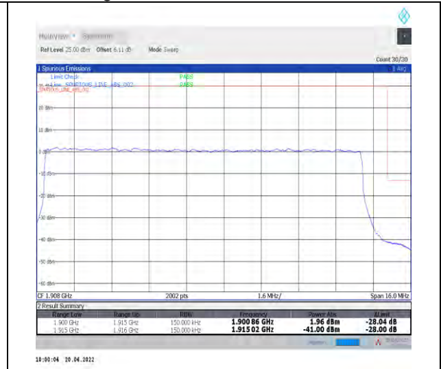
1-N25--15-15-H-3-DFT-PI2BPSK-Outer_Full-75@0-Ant0-seegraph-PASS-see graph
