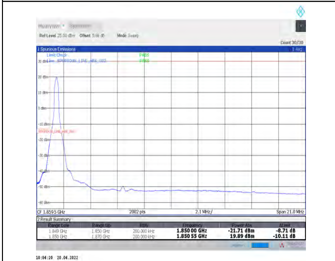
1-N25--15-20-L-4-CP-QPSK-Edge_1RB_Left-1@0-Ant0-seegraph-PASS-see graph
