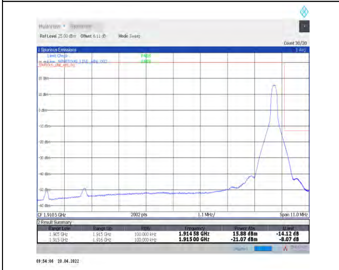
1-N25--15-10-H-5-CP-QPSK-Edge_1RB_Right-1@51-Ant0-seegraph-PASS-see graph
