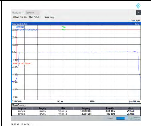
1-N25--15-25-L-6-CP-QPSK-Outer_Full-133@0-Ant0-seegraph-PASS-see graph
