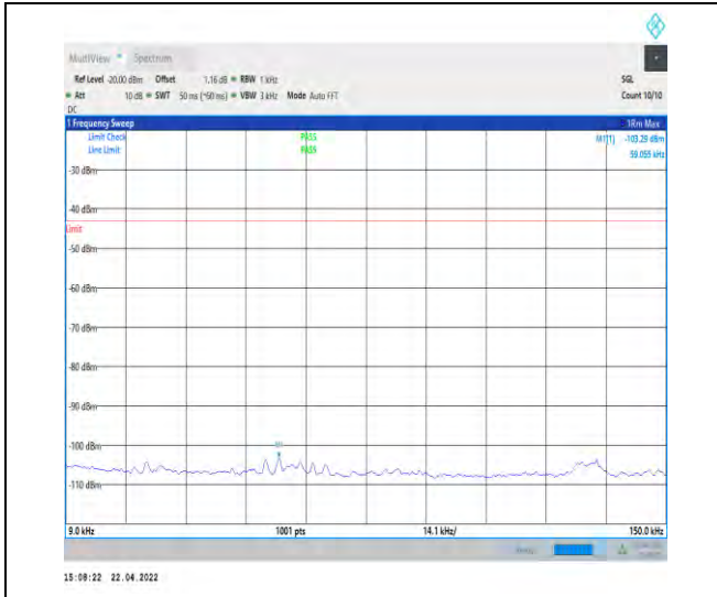
1-N25--15-40-H-1-DFT-PI2BPSK-Inner_1RB_Left-1 @1-0.009-0.15-Ant0--103.29--43-PASS
