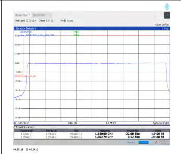
1-N25--15-15-L-6-CP-QPSK-Outer_Full-79@0-Ant0-seegraph-PASS-see graph
