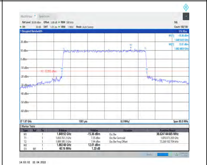
1-N25--15-40-L-6-CP-QPSK-Outer_Full-216@0-A nt0-38.624-40.160-<math>\leq 40</math>-PASS
