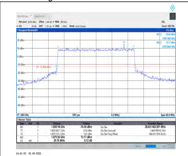
1-N25--15-30-L-7-CP-16QAM-Outer_Full-160@0-Ant0 -28.631-29.760-≤30-PASS
