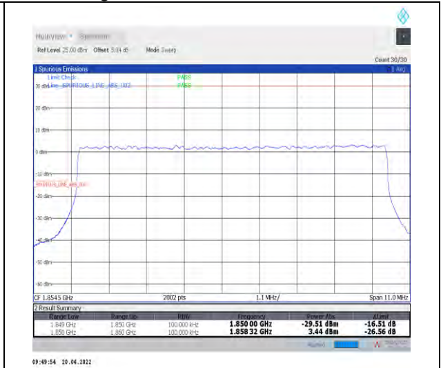
1-N25--15-10-L-3-DFT-PI2BPSK-Outer_Full-50@0-Ant0-seegraph-PASS-see graph
