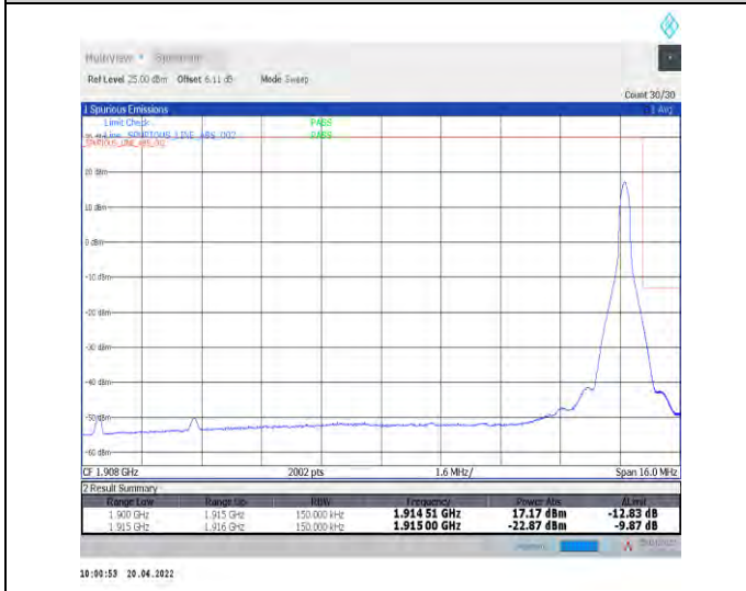
1-N25--15-15-H-5-CP-QPSK-Edge_1RB_Right-1@78-Ant0-seegraph-PASS-see graph
