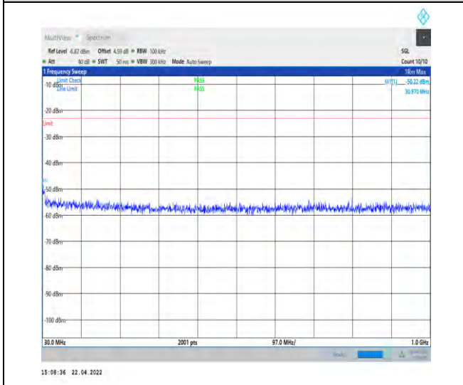
1-N25--15-40-H-1-DFT-PI2BPSK-Inner_1RB_Left-1 @1-30-1000-Ant0--50.22--23-PASS
