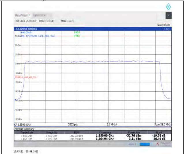
1-N25--15-20-L-3-DFT-PI2BPSK-Outer_Full-100@0-Ant0-seegraph-PASS-see graph
