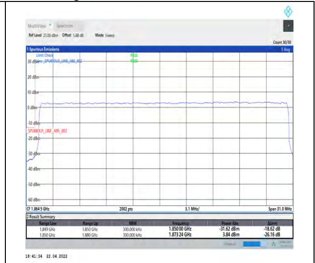
1-N25--15-30-L-3-DFT-PI2BPSK-Outer_Full-160@0-Ant0-seegraph-PASS-see graph
