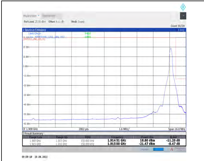
1-N25--15-15-H-2-DFT-PI2BPSK-Edge_1RB_Right-1@78-Ant0-seegraph-PASS-see graph
