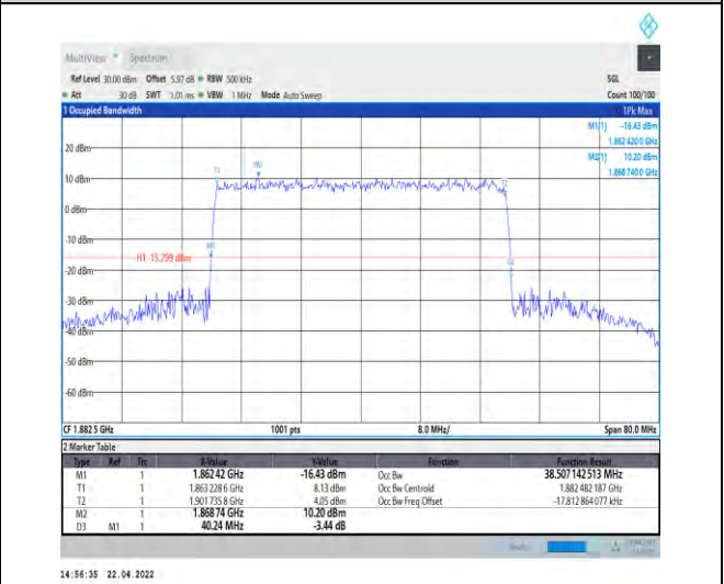
1-N25--15-40-M-5-DFT-256QAM-Outer_Full-216@0-Ant0-38.507-40.240-≤40-PASS
