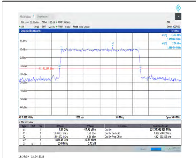
1-N25--15-25-M-6-CP-QPSK-Outer_Full-133@0-Ant 0-23.735-25.000-≤25-PASS
