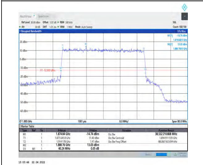
1-N25--15-40-H-3-DFT-16QAM-Outer_Full-216@0-A nt0-38.532-40.240-<math>\leq 40</math>-PASS
