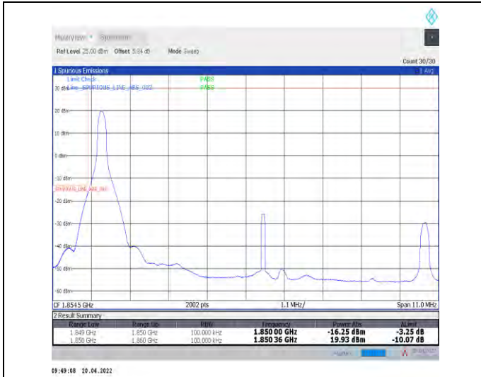
1-N25--15-10-L-1-DFT-PI2BPSK-Edge_1RB_Left-1@0-Ant0-seegraph-PASS-see graph
