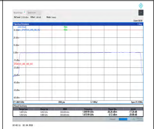
1-N25--15-30-L-6-CP-QPSK-Outer_Full-160@0-Ant0-seegraph-PASS-see graph
