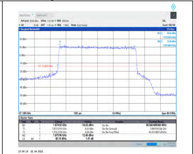
1-N25--15-40-H-6-CP-QPSK-Outer_Full-216@0-Ant0-38.56-40.160-<math>\leq 40</math>-PASS
