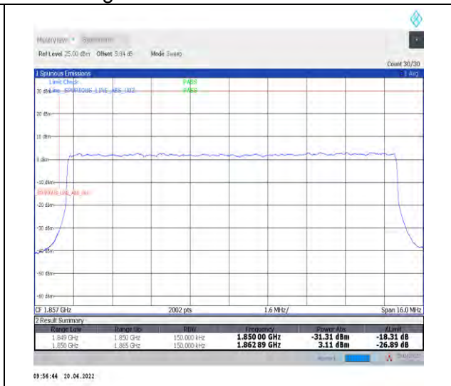
1-N25--15-15-L-3-DFT-PI2BPSK-Outer_Full-75@0-Ant0-seegraph-PASS-see graph
