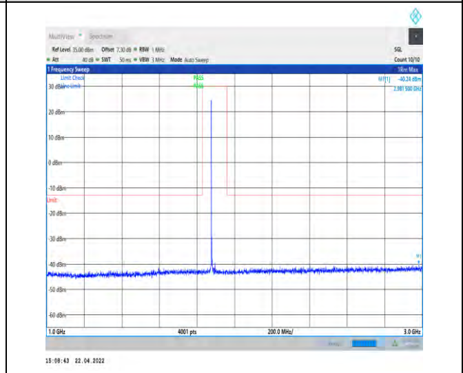
1-N25--15-40-H-1-DFT-PI2BPSK-Inner_1RB_Left-1 @1-1000-3000-Ant0--40.24--13-PASS
