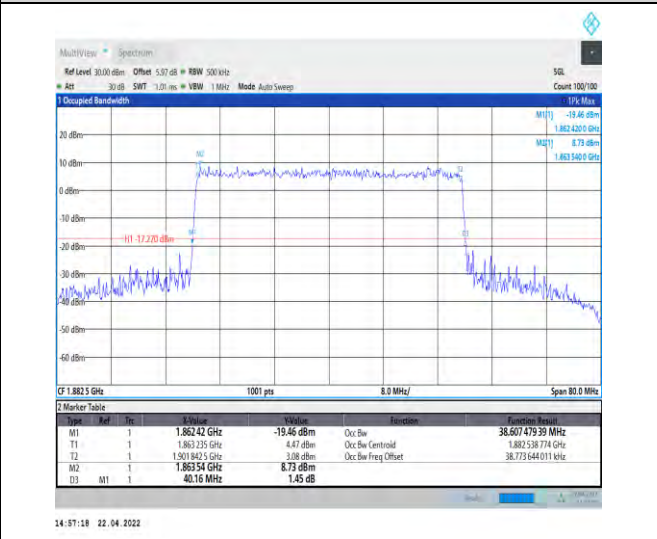
1-N25--15-40-M-9-CP-256QAM-Outer_Full-216@0-A Ant0-38.607-40.160-≤40-PASS
