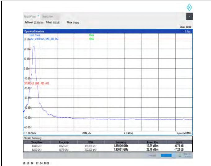
1-N25--15-25-L-1-DFT-PI2BPSK-Edge_1RB_Left-1@0-Ant0-seegraph-PASS-see graph
