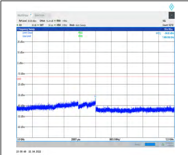
1-N25--15-40-H-1-DFT-PI2BPSK-Inner_1RB_Left-1 @1-3000-12000-Ant0--34.82--13-PASS
