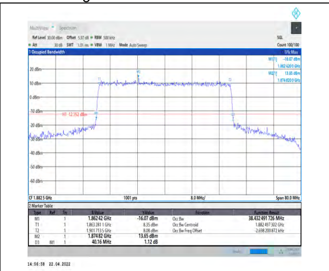
1-N25--15-40-M-7-CP-16QAM-Outer_Full-216@0-A nt0-38.432-40.160-≤40-PASS
