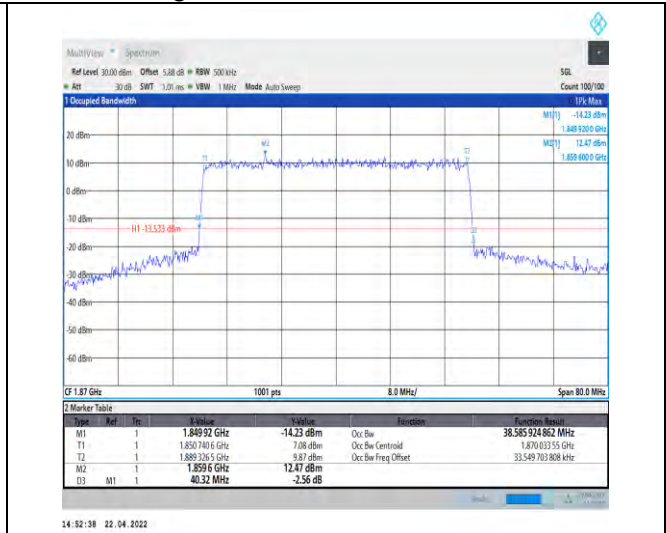
1-N25--15-40-L-4-DFT-64QAM-Outer_Full-216@0-A nt0-38.586-40.320-<math>\leq 40</math>-PASS
