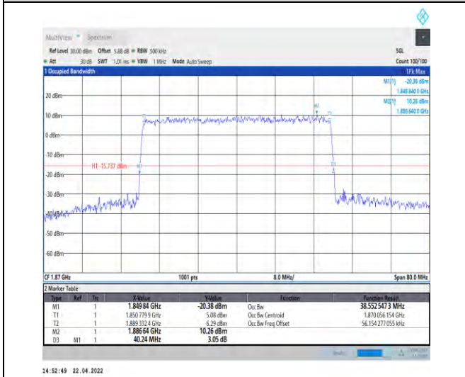
1-N25--15-40-L-5-DFT-256QAM-Outer_Full-216@0-A Ant0-38.553-40.240-<math>\leq 40</math>-PASS
