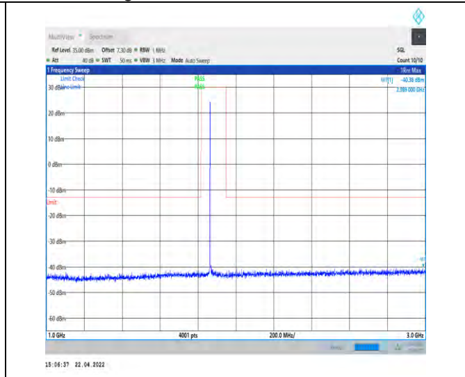
1-N25--15-40-M-1-DFT-PI2BPSK-Inner_1RB_Left-1 @1-1000-3000-Ant0--40.38--13-PASS
