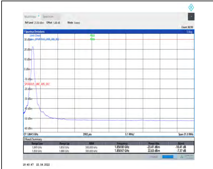
1-N25--15-30-L-1-DFT-PI2BPSK-Edge_1RB_Left-1@0-Ant0-seegraph-PASS-see graph
