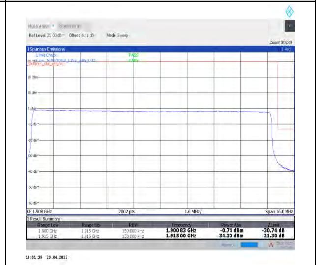
1-N25--15-15-H-6-CP-QPSK-Outer_Full-79@0-Ant0-seegraph-PASS-see graph
