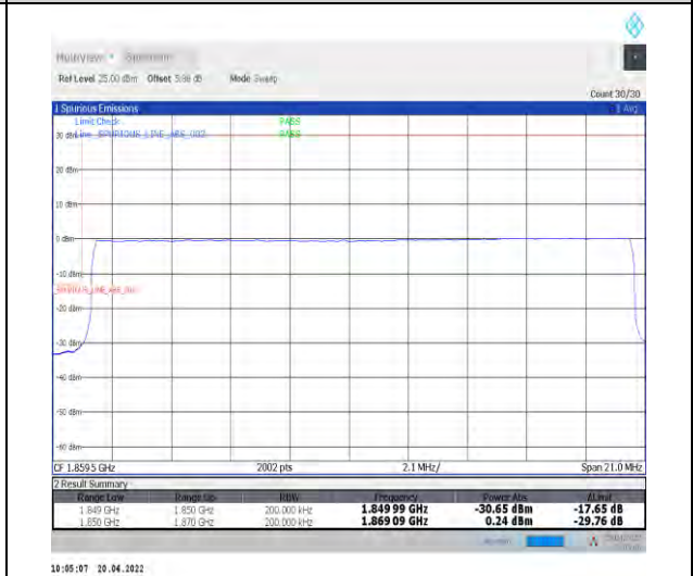
1-N25--15-20-L-6-CP-QPSK-Outer_Full-106@0-Ant0-seegraph-PASS-see graph
