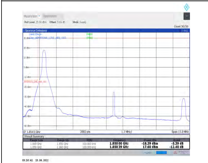
1-N25--15-10-L-4-CP-QPSK-Edge_1RB_Left-1@0-Ant0-seegraph-PASS-see graph
