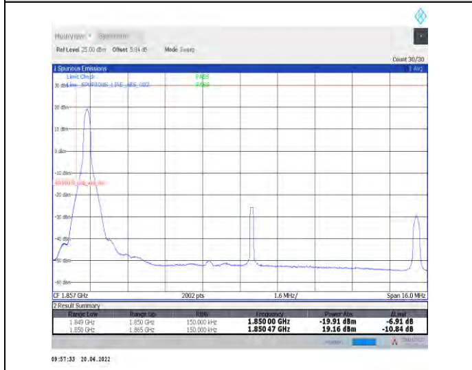
1-N25--15-15-L-4-CP-QPSK-Edge_1RB_Left-1@0-Ant0-seegraph-PASS-see graph
