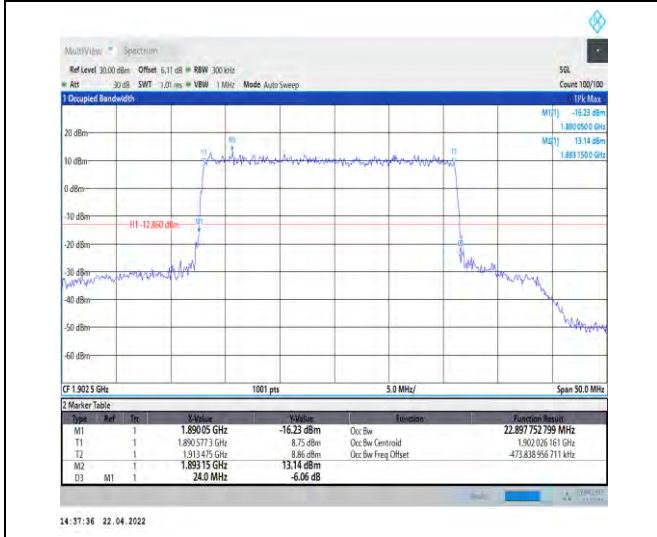
1-N25--15-25-H-1-DFT-QPSK-Outer_Full-128@0-An t0-22.898-24.000-<math>\leq 25</math>-PASS
