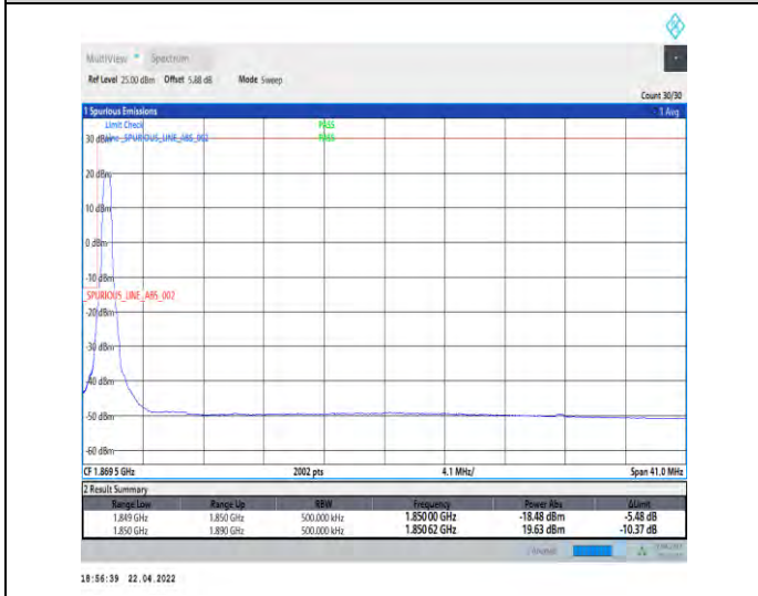
1-N25--15-40-L-4-CP-QPSK-Edge_1RB_Left-1@0-Ant0-seegraph-PASS-see graph
