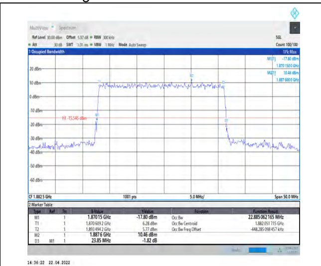
1-N25--15-25-M-5-DFT-256QAM-Outer_Full-128@0-A Ant0-22.885-23.850-≤25-PASS
