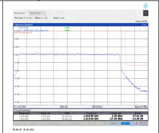
1-N25--15-5-H-3-DFT-PI2BPSK-Outer_Full-25@0-Ant0-seegraph-PASS-see graph
