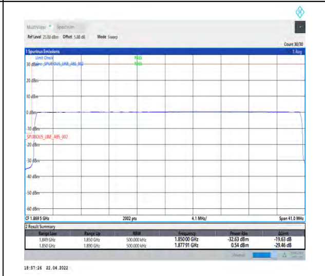
1-N25--15-40-L-6-CP-QPSK-Outer_Full-216@0-Ant0-seegraph-PASS-see graph
