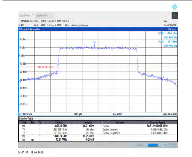
1-N25--15-40-M-8-CP-64QAM-Outer_Full-216@0-A nt0-38.512-40.240-≤40-PASS
