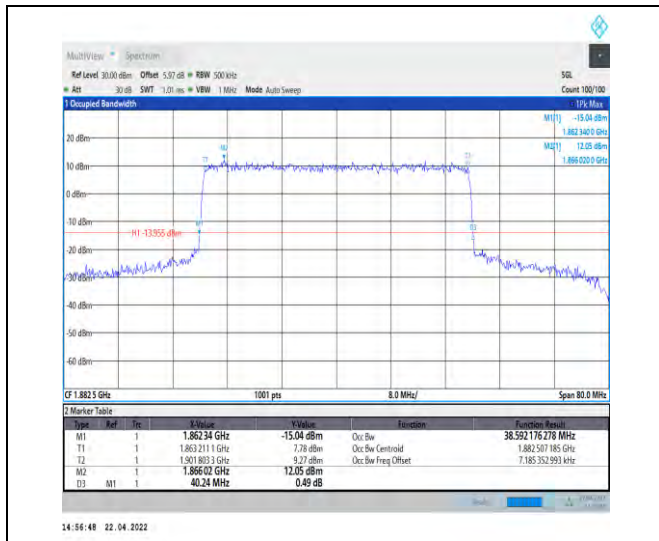
1-N25--15-40-M-6-CP-QPSK-Outer_Full-216@0-Ant 0-38.592-40.240-≤40-PASS
