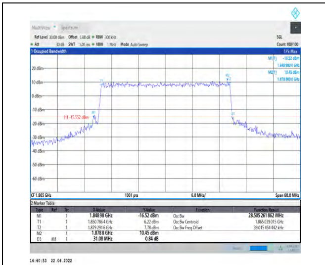
1-N25--15-30-L-6-CP-QPSK-Outer_Full-160@0-Ant0 -28.505-31.080-≤30-PASS
