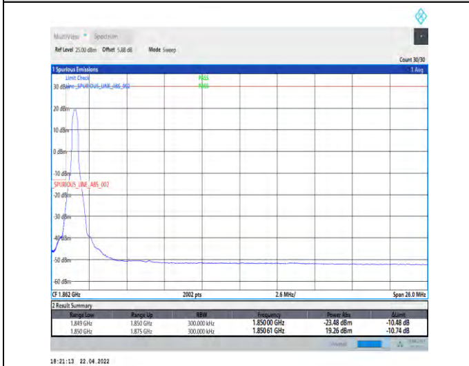
1-N25--15-25-L-4-CP-QPSK-Edge_1RB_Left-1@0-Ant0-seegraph-PASS-see graph
