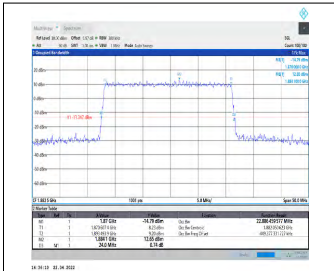
1-N25--15-25-M-4-DFT-64QAM-Outer_Full-128@0-A nt0-22.886-24.000-≤25-PASS
