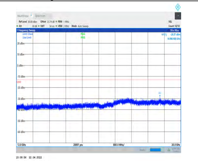
1-N25--15-40-H-1-DFT-PI2BPSK-Inner_1RB_Left-1 @1-12000-20000-Ant0--28.37--13-PASS
