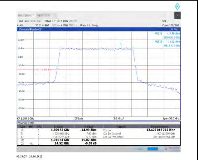
1-N25--15-15-H-4-DFT-64QAM-Outer_Full-75@0-Ant t0-13.427-14.520-≤15-PASS
