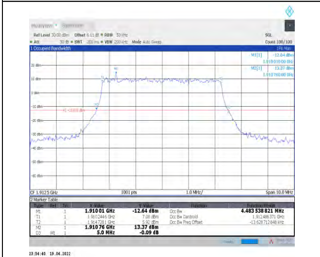
1-N25--15-5-H-1-DFT-QPSK-Outer_Full-25@0-Ant0 4.484-5.000-≤5-PASS
