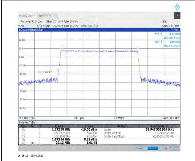
1-N25--15-20-M-9-CP-256QAM-Outer_Full-106@0-A Ant0-18.948-20.120-<=20-PASS
