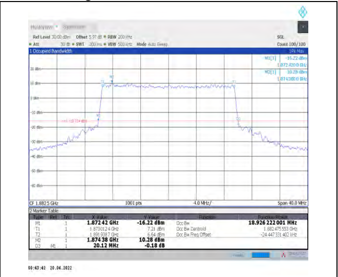
1-N25--15-20-M-8-CP-64QAM-Outer_Full-106@0-A nt0-18.926-20.120-<=20-PASS
