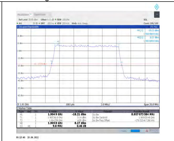
1-N25--15-10-H-5-DFT-256QAM-Outer_Full-50@0-Ant nt0-8.957-9.800-≤10-PASS
