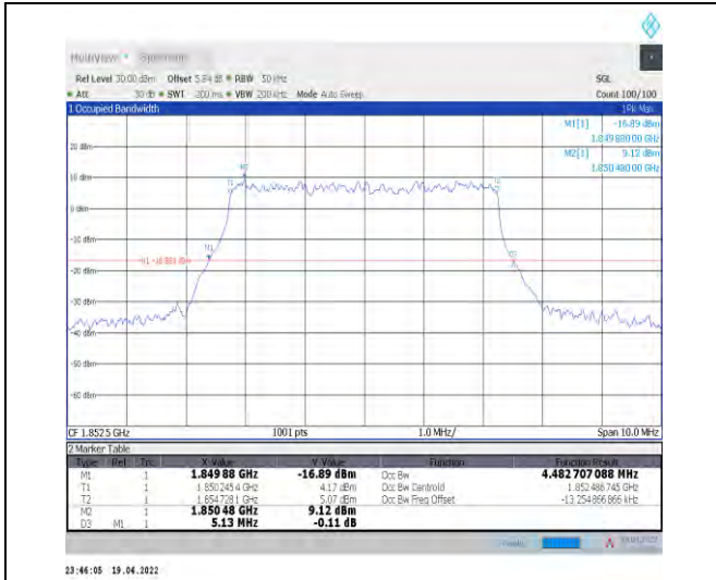
1-N25--15-5-L-5-DFT-256QAM-Outer_Full-25@0-Ant 0-4.483-5.130-≤5-PASS
