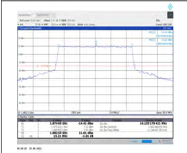
1-N25--15-15-M-8-CP-64QAM-Outer_Full-79@0-Ant0 0-14.153-15.210-≤15-PASS
