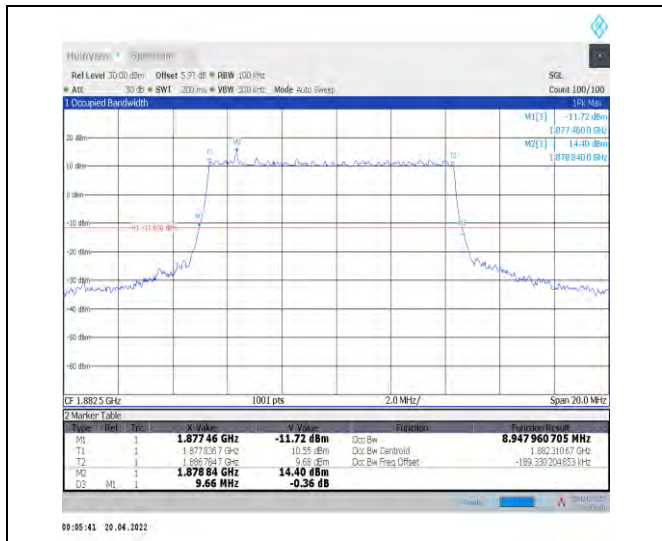
1-N25--15-10-M-1-DFT-QPSK-Outer_Full-50@0-Ant 0-8.948-9.660-≤10-PASS
