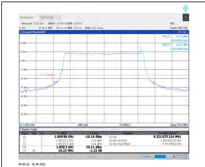
1-N25--15-10-L-6-CP-QPSK-Outer_Full-52@0-Ant0 9.321-10.320-≤10-PASS
