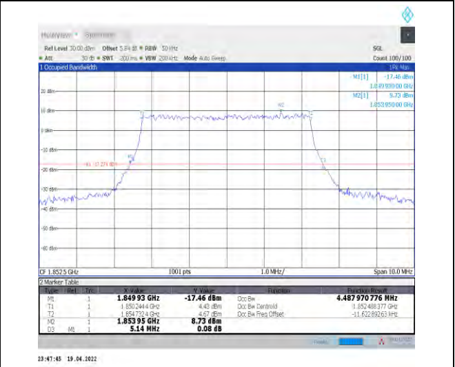
1-N25--15-5-L-8-CP-64QAM-Outer_Full-25@0-Ant0- 4.488-5.140-≤5-PASS
