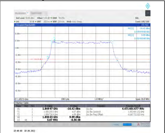
1-N25--15-5-L-6-CP-QPSK-Outer_Full-25@0-Ant0-4 .472-5.070-≤5-PASS
