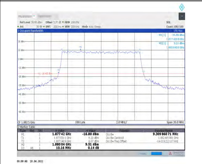
1-N25--15-10-M-8-CP-64QAM-Outer_Full-52@0-Ant 0-9.31-10.160-≤10-PASS
