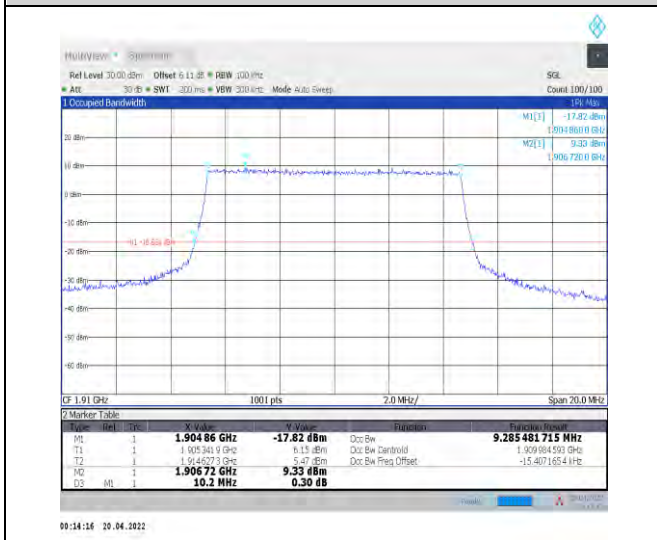
1-N25--15-10-H-6-CP-QPSK-Outer_Full-52@0-Ant0 9.285-10.200-≤10-PASS
