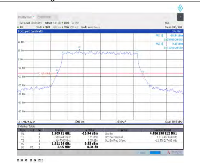
1-N25--15-5-H-4-DFT-64QAM-Outer_Full-25@0-Ant 0-4.486-5.150-≤5-PASS
