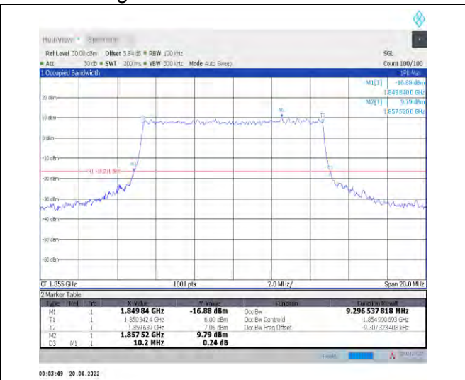
1-N25--15-10-L-7-CP-16QAM-Outer_Full-52@0-Ant 0-9.297-10.200-≤10-PASS
