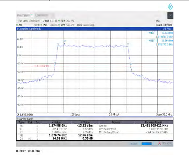
1-N25--15-15-M-3-DFT-16QAM-Outer_Full-75@0-An t0-13.452-14.520-≤15-PASS
