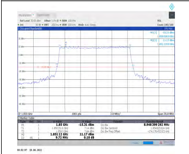
1-N25--15-10-L-4-DFT-64QAM-Outer_Full-50@0-Ant 0-8.948-9.720-≤10-PASS
