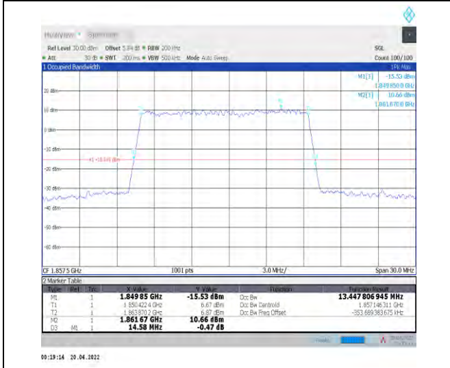
1-N25--15-15-L-5-DFT-256QAM-Outer_Full-75@0-A nt0-13.448-14.580-≤15-PASS
