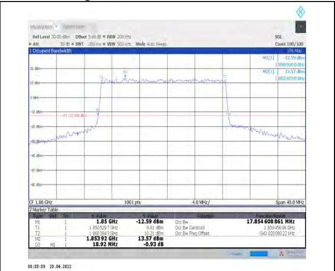
1-N25--15-20-L-1-DFT-QPSK-Outer_Full-100@0-Ant 0-17.855-18.920-<=20-PASS
