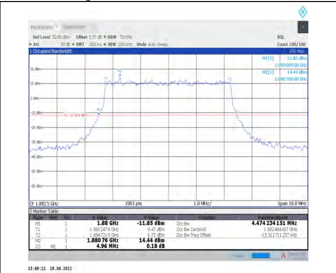
1-N25--15-5-M-1-DFT-QPSK-Outer_Full-25@0-Ant0 4.474-4.960-≤5-PASS
