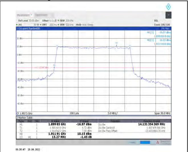
1-N25--15-15-H-6-CP-QPSK-Outer_Full-79@0-Ant0- 14.131-15.270-≤15-PASS
