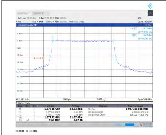
1-N25--15-10-M-3-DFT-16QAM-Outer_Full-50@0-Ant t0-8.947-9.680-≤10-PASS
