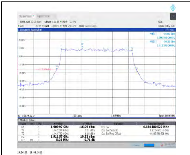
1-N25--15-5-H-3-DFT-16QAM-Outer_Full-25@0-Ant 0-4.484-5.050-≤5-PASS
