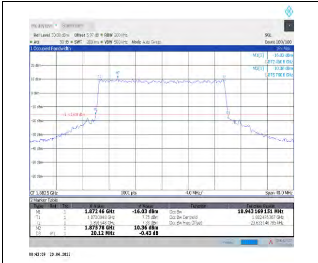
1-N25--15-20-M-7-CP-16QAM-Outer_Full-106@0-A nt0-18.943-20.120-<=20-PASS
