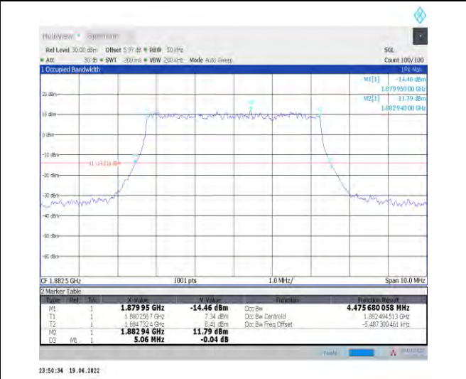
1-N25--15-5-M-3-DFT-16QAM-Outer_Full-25@0-Ant 0-4.476-5.060-≤5-PASS
