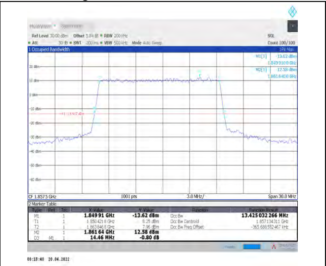
1-N25--15-15-L-4-DFT-64QAM-Outer_Full-75@0-Ant 0-13.425-14.460-≤15-PASS
