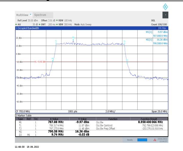
1-N14--15-10-M-2-DFT-PI2BPSK-Outer_Full-50@0-Ant 0-8.958-9.740-≤10-PASS
