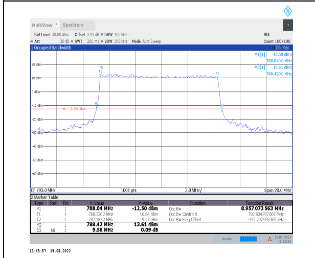
1-N14--15-10-M-3-DFT-16QAM-Outer_Full-50@0-Ant 0-8.957-9.580-≤10-PASS
