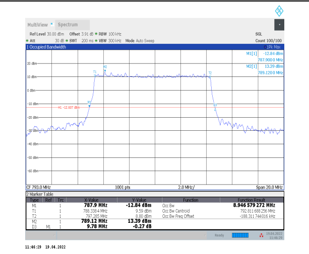
1-N14--15-10-M-4-DFT-64QAM-Outer_Full-50@0-Ant 0-8.947-9.780-≤10-PASS
