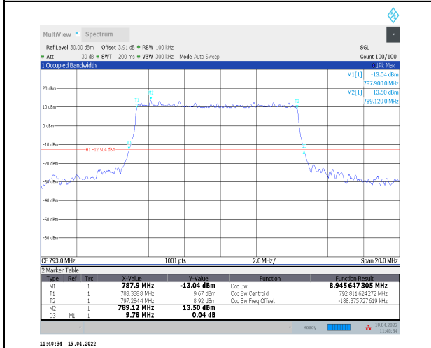
1-N14--15-10-L-4-DFT-64QAM-Outer_Full-50@0-A t0-8.946-9.780≤10-PASS
