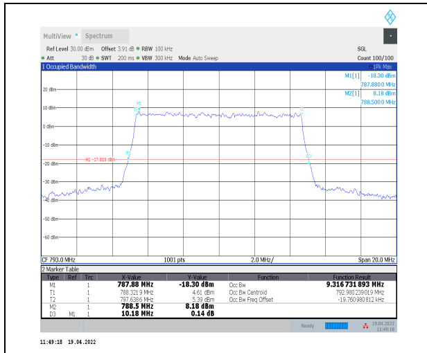
1-N14--15-10-M-9-CP-256QAM-Outer_Full-52@0-A nt0-9.317-10.180-<=10-PASS
