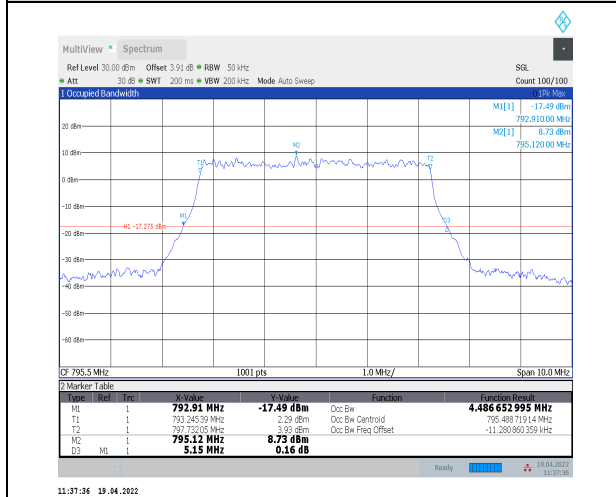
1-N14--15-5-H-9-CP-256QAM-Outer_Full-25@0-Ant 0-4.487-5.150-≤5-PASS
