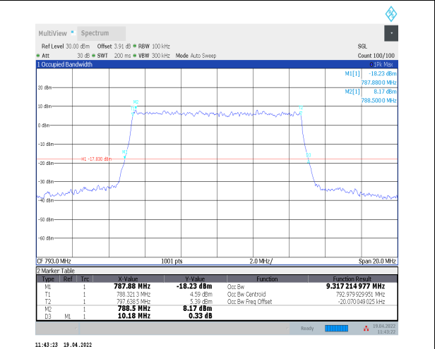
1-N14--15-10-L-9-CP-256QAM-Outer_Full-52@0-Ant 0-9.317-10.180≤10-PASS
