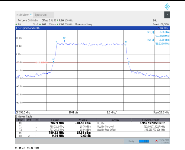
1-N14--15-10-L-1-DFT-QPSK-Outer_Full-50@0-Ant0 -8.96-9.740-≤10-PASS
