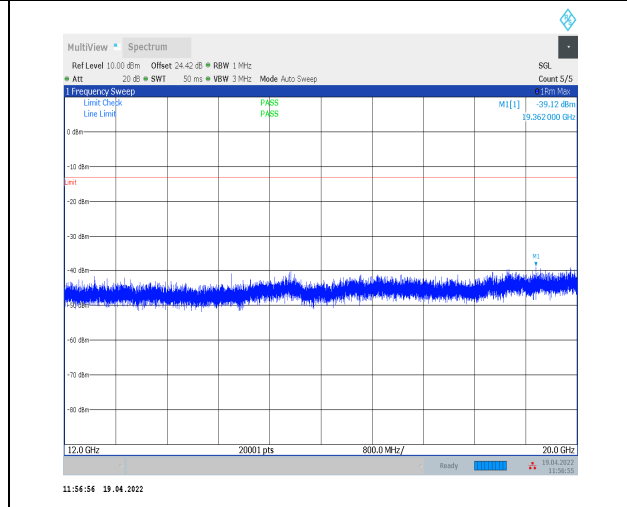
1-N14--15-10-M-1-DFT-PI2BPSK-Inner_1RB_Left-1 @1-12000-20000-Ant0--39.12--13-PASS
