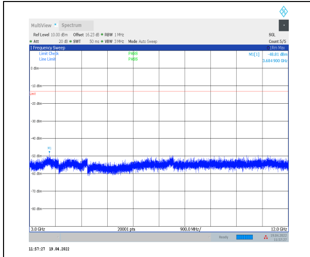
1-N14--15-10-H-1-DFT-PI2BPSK-Inner_1RB_Left-1 @1-3000-12000-Ant0--48.81--13-PASS
