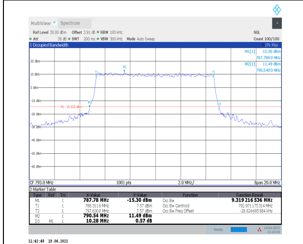
1-N14--15-10-L-8-CP-64QAM-Outer_Full-52@0-Ant 0-9.319-10.280≤10-PASS
