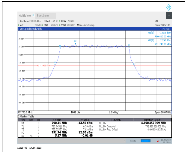
1-N14--15-5-M-4-DFT-64QAM-Outer_Full-25@0-Ant 0-4.49-5.170-<math>\leq</math>5-PASS
