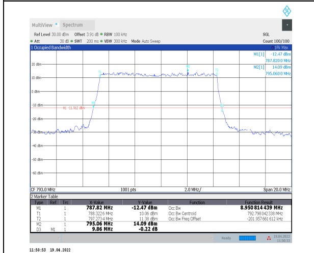
1-N14--15-10-H-2-DFT-PI2BPSK-Outer_Full-50@0- Ant0-8.951-9.860-<=10-PASS
