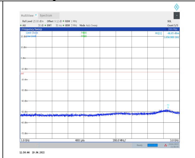
1-N14--15-10-M-1-DFT-PI2BPSK-Inner_1RB_Left-1 @1-1000-3000-Ant0--46.85--13-PASS
