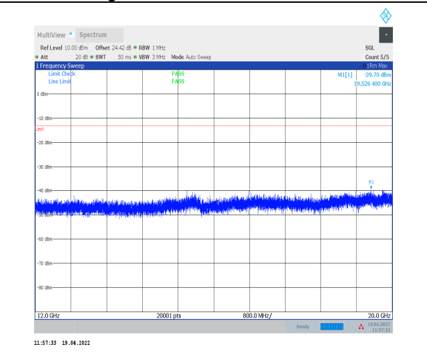
1-N14--15-10-H-1-DFT-PI2BPSK-Inner_1RB_Left-1 @1-12000-20000-Ant0--39.70--13-PASS
