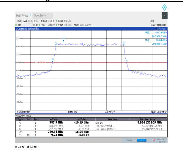
1-N14--15-10-H-1-DFT-QPSK-Outer_Full-50@0-Ant 0-8.954-9.740-<=10-PASS
