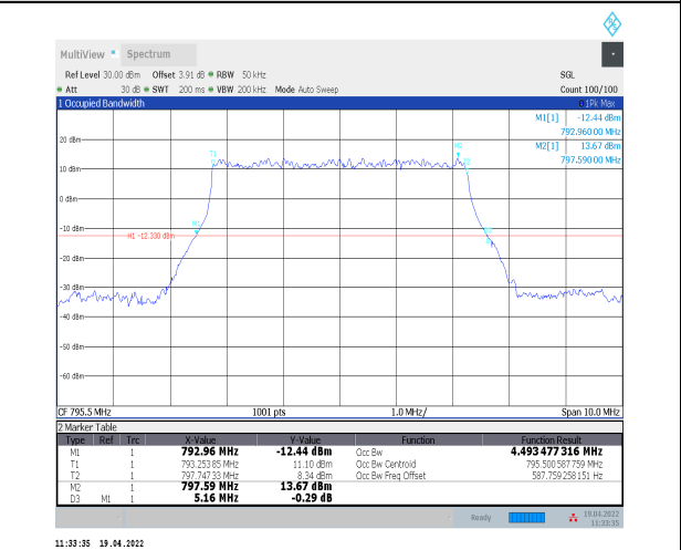
1-N14--15-5-H-2-DFT-PI2BPSK-Outer_Full-25@0-Ant0 0-4.493-5.160-≤5-PASS
