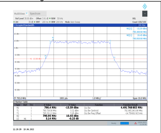
1-N14--15-5-M-5-DFT-256QAM-Outer_Full-25@0-An t0-4.492-5.140-<math>\leq</math>5-PASS
