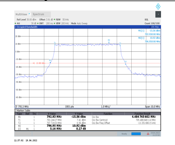
1-N14--15-5-H-8-CP-64QAM-Outer_Full-25@0-Ant0- 4.485-5.160-≤5-PASS
