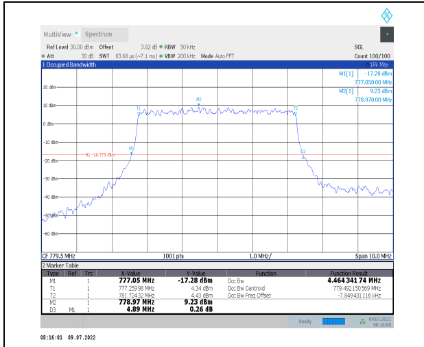
1-N13--15-5-L-5-DFT-256QAM-Outer_Full-25@0-Ant0-4.464-4.890-<math>\leq 5</math>-PASS
