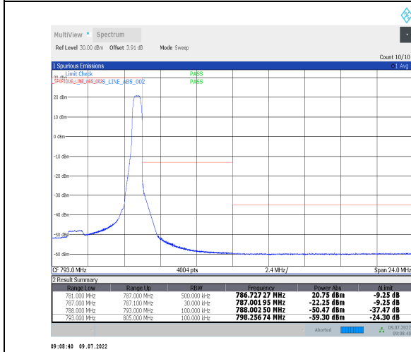
1-N13-PC3-15-5-H-5-CP-QPSK-Edge_1RB_Right-1@24-Ant0-PASS-see graph
