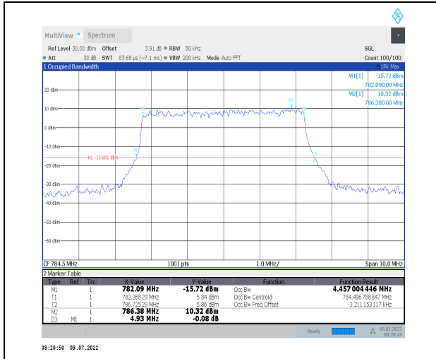
1-N13--15-5-H-7-CP-16QAM-Outer_Full-25@0-Ant0- 4.457-4.930-≤5-PASS
