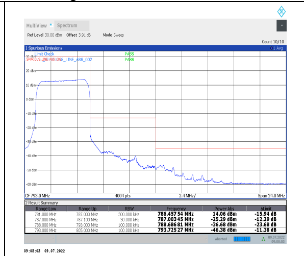
1-N13-PC3-15-5-H-3-DFT-PI2BPSK-Outer_Full-25@0-Ant0-PASS-see graph
