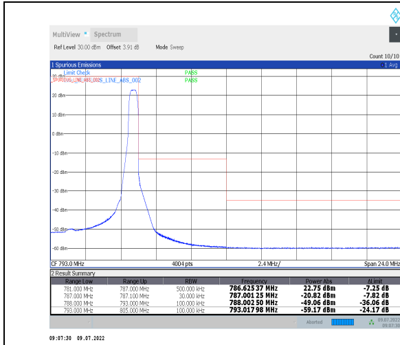
1-N13-PC3-15-5-H-2-DFT-PI2BPSK-Edge_1RB_Right-1@24-Ant0-PASS-see graph
