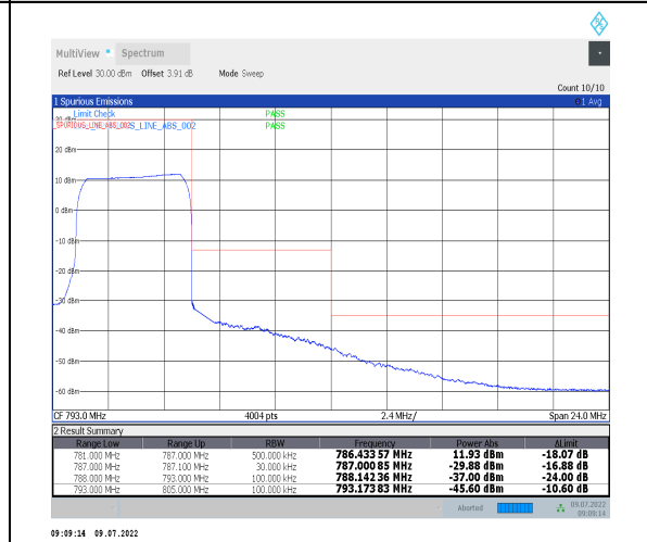
1-N13-PC3-15-5-H-6-CP-QPSK-Outer_Full-25@0-Ant0-PASS-see graph
