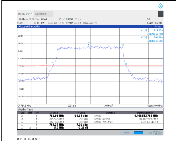
1-N13--15-5-H-9-CP-256QAM-Outer_Full-25@0-Ant 0-4.469-5.000-≤5-PASS
