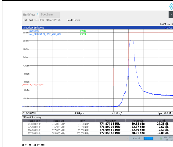
1-N13-PC3-15-10-L-4-CP-QPSK-Edge_1RB_Left-1@0-Ant0-PASS-see graph
