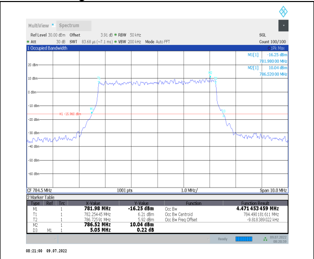
1-N13--15-5-H-8-CP-64QAM-Outer_Full-25@0-Ant0 -4.471-5.050-≤5-PASS
