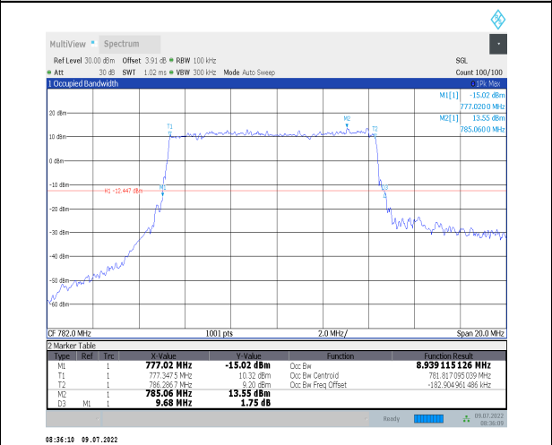
1-N13--15-10-M-1-DFT-QPSK-Outer_Full-50@0-Ant 0-8.939-9.680-≤10-PASS
