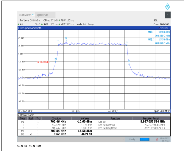
1-N12--15-10-M-1-DFT-QPSK-Outer_Full-50@0-Ant 0-8.937-9.620-<=10-PASS
