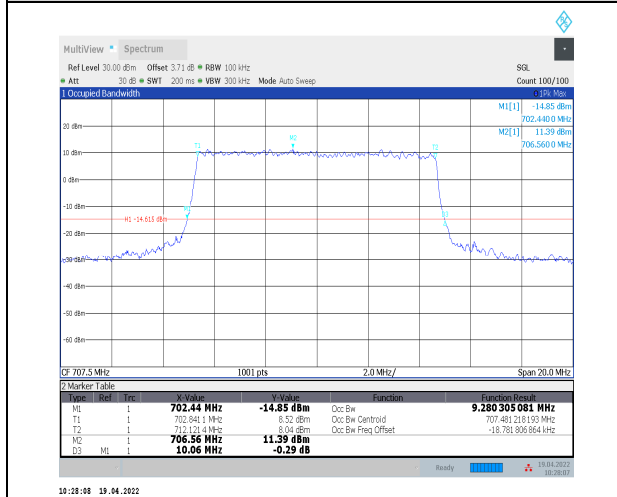
1-N12--15-10-M-7-CP-16QAM-Outer_Full-52@0-Ant 0-9.28-10.060-≤10-PASS
