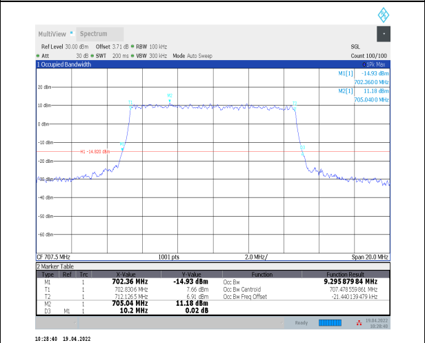
1-N12--15-10-M-8-CP-64QAM-Outer_Full-52@0-Ant 0-9.296-10.200-≤10-PASS
