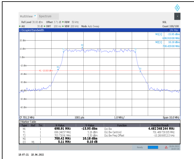
1-N12--15-5-L-5-DFT-256QAM-Outer_Full-25@0-Ant 0-4.482-5.110-<math>\leq</math>5-PASS
