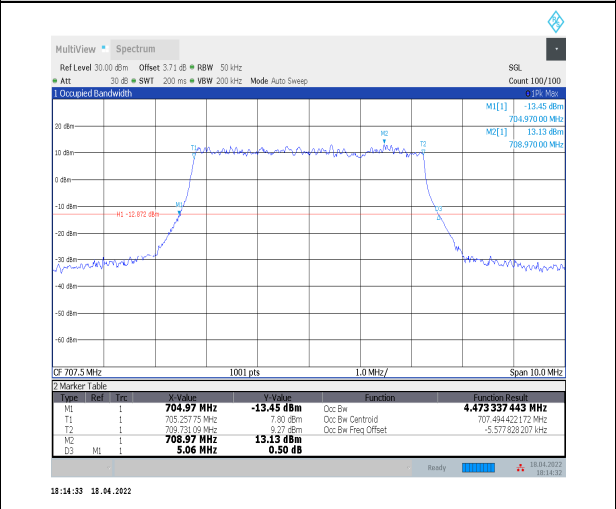
1-N12--15-5-M-3-DFT-16QAM-Outer_Full-25@0-Ant 0-4.473-5.060-≤5-PASS
