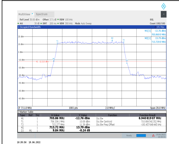
1-N12--15-10-H-2-DFT-PI2BPSK-Outer_Full-50@0-Ant Ant0-8.941-9.840≤10-PASS
