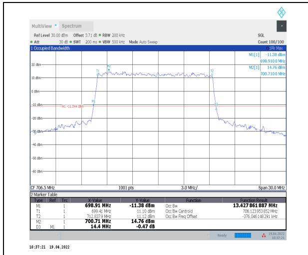
1-N12--15-15-L-3-DFT-16QAM-Outer_Full-75@0-Ant 0-13.428-14.400≤15-PASS
