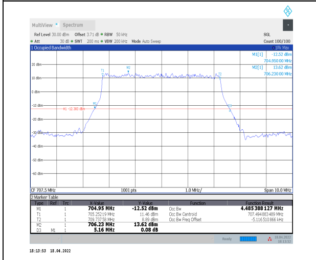
1-N12--15-5-M-2-DFT-PI2BPSK-Outer_Full-25@0-A nt0-4.485-5.160-≤5-PASS
