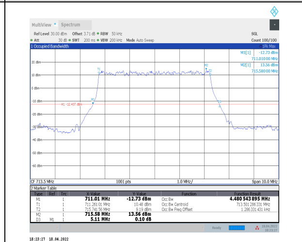
1-N12--15-5-H-2-DFT-PI2BPSK-Outer_Full-25@0-Ant0 4.481-5.110-≤5-PASS
