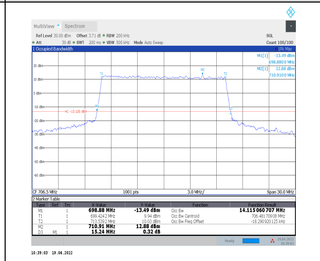
1-N12--15-15-L-6-CP-QPSK-Outer_Full-79@0-Ant0 14.115-15.240≤15-PASS
