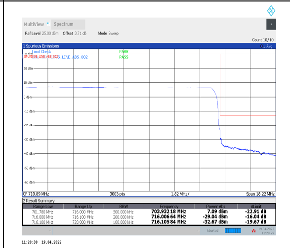
1-N12--15-15-H-6-CP-QPSK-Outer_Full-79@0-Ant0-PASS-see graph
