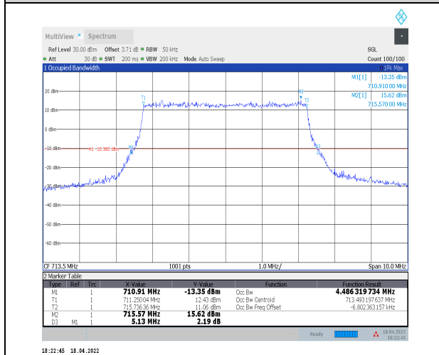
1-N12--15-5-H-1-DFT-QPSK-Outer_Full-25@0-Ant0 4.486-5.130-≤5-PASS
