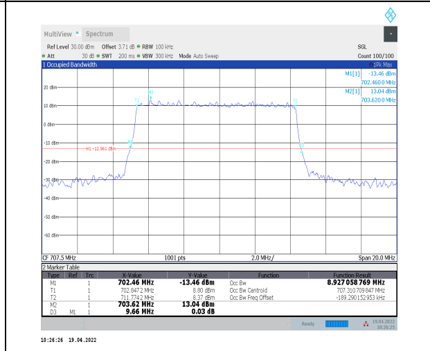
1-N12--15-10-M-4-DFT-64QAM-Outer_Full-50@0-A nt0-8.927-9.660-<=10-PASS
