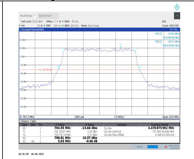
1-N12--15-5-M-5-DFT-256QAM-Outer_Full-25@0-A nt0-4.477-5.050-≤5-PASS
