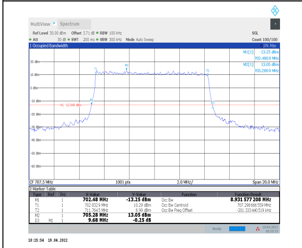
1-N12--15-10-M-3-DFT-16QAM-Outer_Full-50@0-Ant t0-8.932-9.680-<=10-PASS
