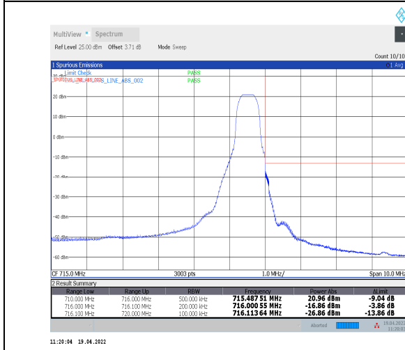
1-N12--15-15-H-5-CP-QPSK-Edge_1RB_Right-1@78-Ant0-PASS-see graph
