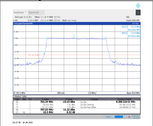
1-N12--15-10-M-6-CP-QPSK-Outer_Full-52@0-Ant0 -9.3-10.300-≤10-PASS
