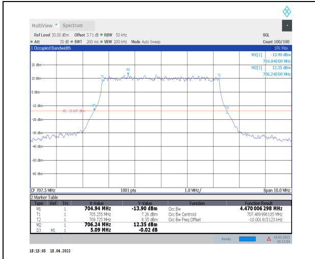
1-N12--15-5-M-4-DFT-64QAM-Outer_Full-25@0-Ant 0-4.47-5.090-≤5-PASS
