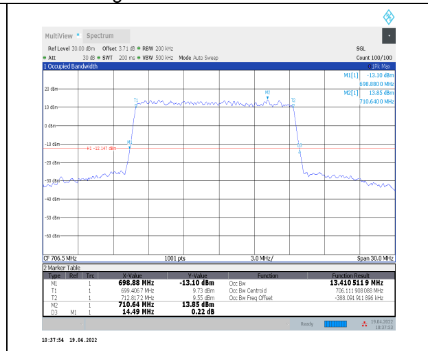
1-N12--15-15-L-4-DFT-64QAM-Outer_Full-75@0-An t0-13.411-14.490≤15-PASS
