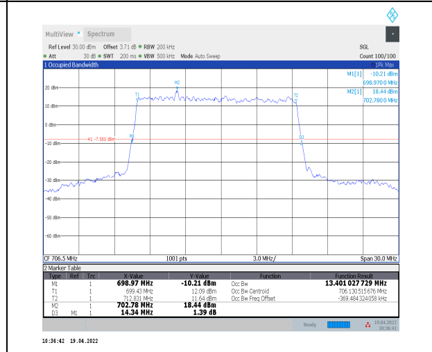
1-N12--15-15-L-2-DFT-PI2BPSK-Outer_Full-75@0-A n0-13.401-14.340-≤15-PASS
