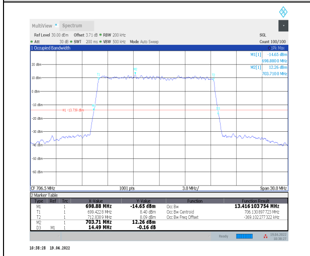
1-N12--15-15-L-5-DFT-256QAM-Outer_Full-75@0-A nt0-13.416-14.490≤15-PASS
