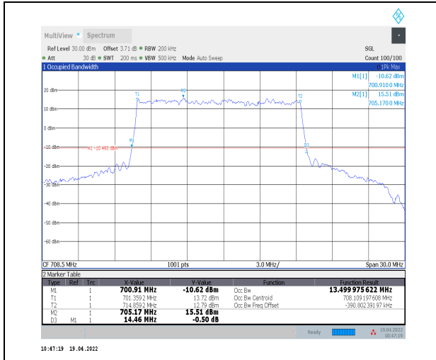
1-N12--15-15-H-1-DFT-QPSK-Outer_Full-75@0-Ant 0-13.5-14.460≤15-PASS
