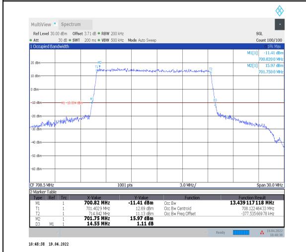
1-N12--15-15-H-3-DFT-16QAM-Outer_Full-75@0-An t0-13.439-14.550≤15-PASS
