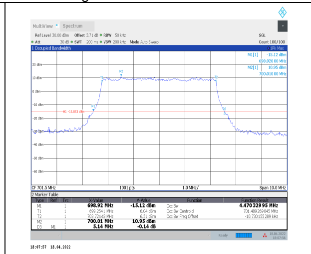
1-N12--15-5-L-6-CP-QPSK-Outer_Full-25@0-Ant0-4 .47-5.140-<math>\leq</math>5-PASS
