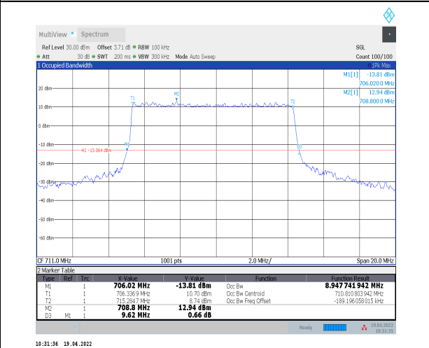
1-N12--15-10-H-3-DFT-16QAM-Outer_Full-50@0-Ant t0-8.948-9.620≤10-PASS
