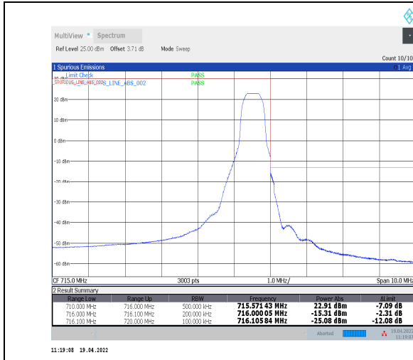
1-N12--15-15-H-2-DFT-PI2BPSK-Edge_1RB_Right-1@78-Ant0-PASS-see graph
