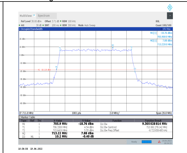
1-N12--15-10-H-9-CP-256QAM-Outer_Full-52@0-An 10-9.305-10.200-≤10-PASS
