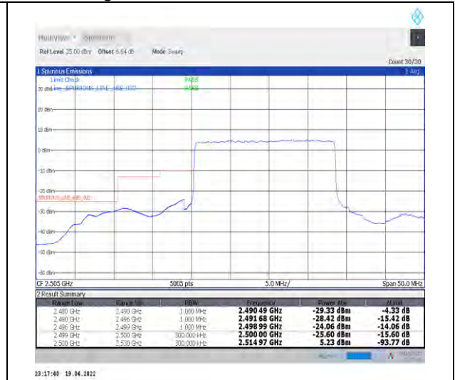
1-N7--15-20-L-3-DFT-PI2BPSK-Outer_Full-100@0-Ant0-PASS-see graph
