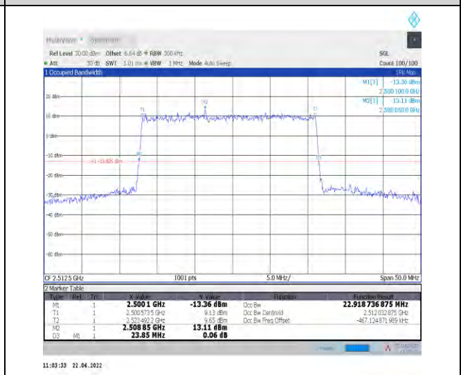
1-N7--15-25-L-4-DFT-64QAM-Outer_Full-128@0-Ant0 0-22.919-23.850-≤25-PASS
