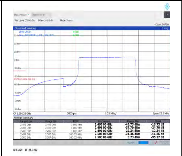
1-N7--15-5-L-6-CP-QPSK-Outer_Full-25@0-Ant0 PASS-see graph
