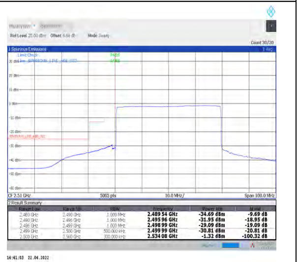
1-N7--15-40-L-6-CP-QPSK-Outer_Full-216@0-Ant0-PASS-see graph
