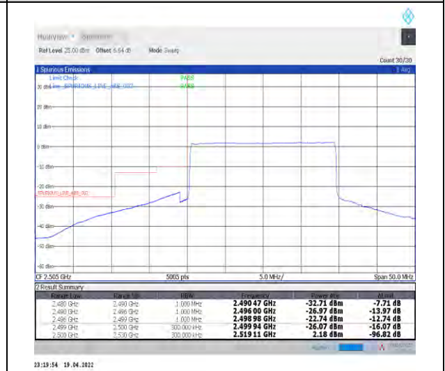
1-N7--15-20-L-6-CP-QPSK-Outer_Full-106@0-Ant0-PASS-see graph
