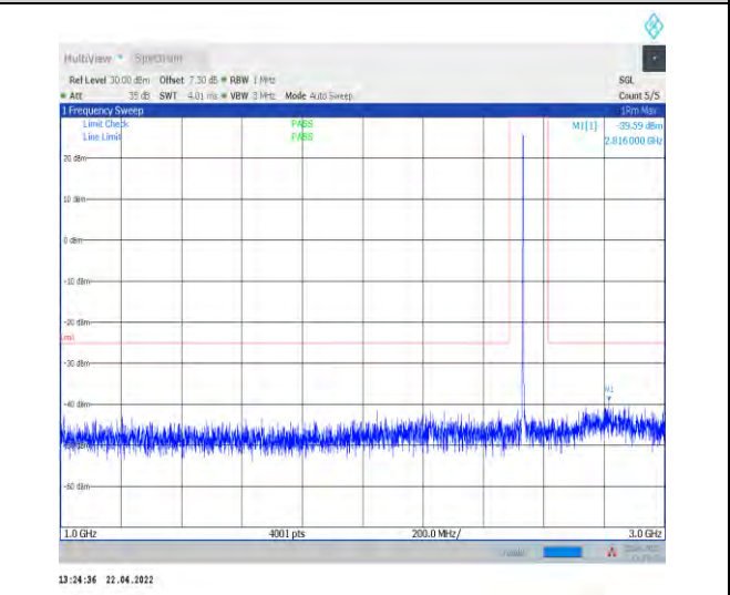
1-N7--15-40-H-1-DFT-PI2BPSK-Inner_1RB_Left-1@ 1-1000-3000-Ant0--39.59--25-PASS
