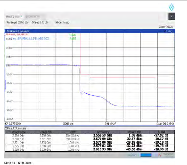
1-N7--15-40-H-6-CP-QPSK-Outer_Full-216@0-An t0-PASS-see graph
