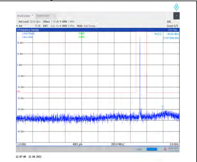
1-N7--15-40-M-1-DFT-PI2BPSK-Inner_1RB_Left-1@ 1-1000-3000-Ant0--40.60--25-PASS
