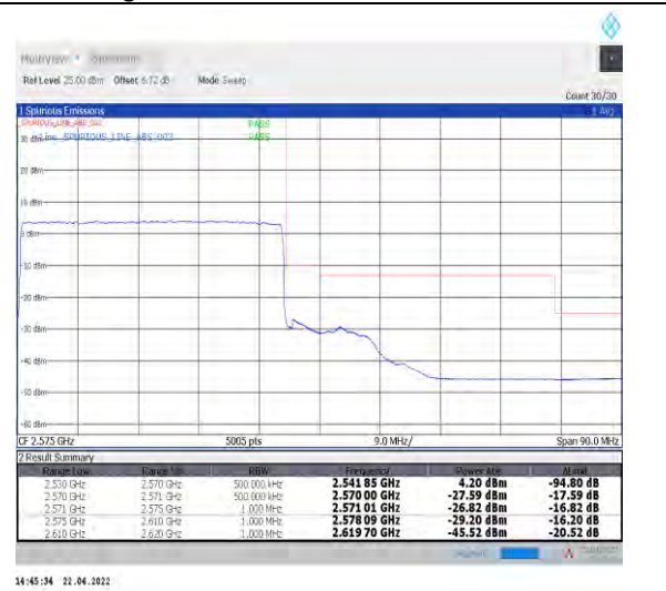
1-N7--15-40-H-3-DFT-PI2BPSK-Outer_Full-216@ 0-Ant0-PASS-see graph
