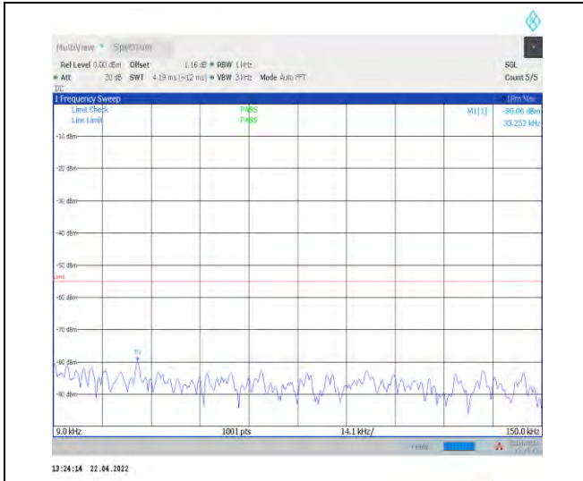
1-N7--15-40-H-1-DFT-PI2BPSK-Inner_1RB_Left-1@ 1-0.009-0.15-Ant0--80.06--55-PASS
