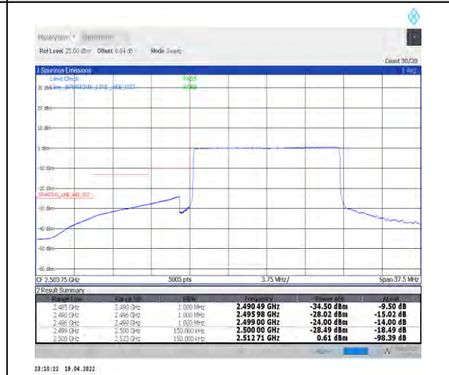
1-N7--15-15-L-6-CP-QPSK-Outer_Full-79@0-Ant0-PASS-see graph
