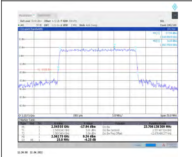
1-N7--15-25-H-9-CP-256QAM-Outer_Full-133@0-Ant t0-23.706-25.000-≤25-PASS
