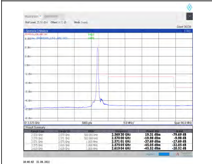
1-N7--15-40-H-5-CP-QPSK-Edge_1RB_Right-1@215- Ant0-PASS-see graph
