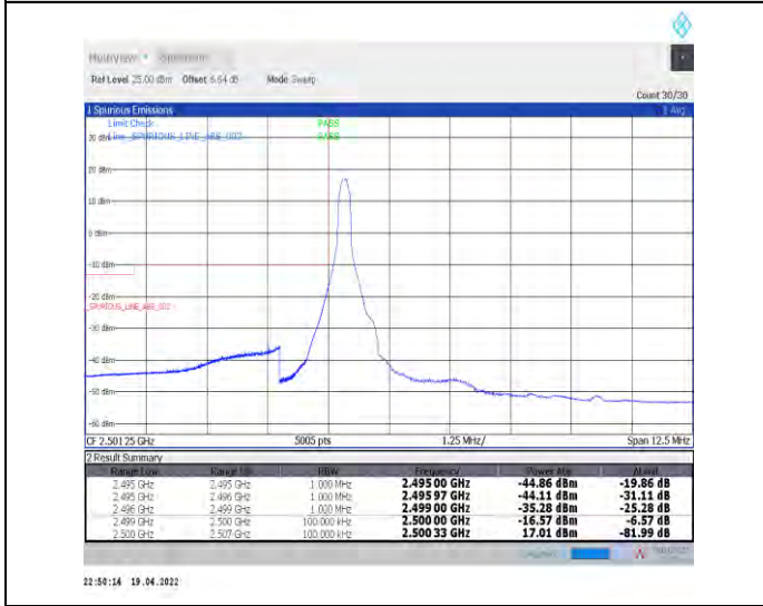
1-N7--15-5-L-4-CP-QPSK-Edge_1RB_Left-1@0-Ant0-P ASS-see graph
