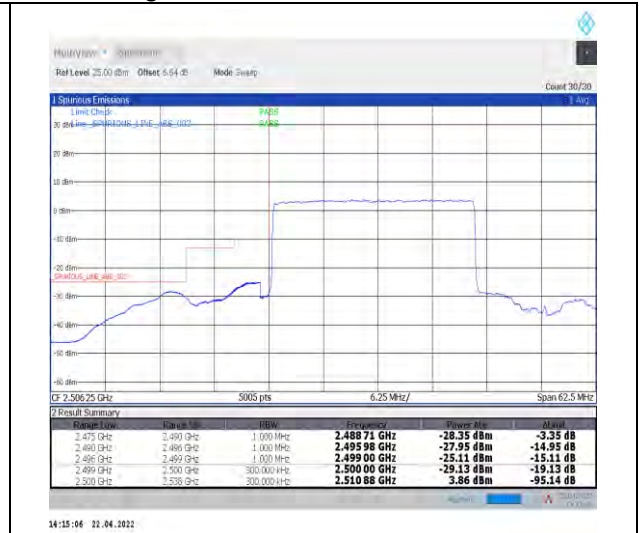
1-N7--15-25-L-3-DFT-PI2BPSK-Outer_Full-128@0-Ant0-PASS-see graph
