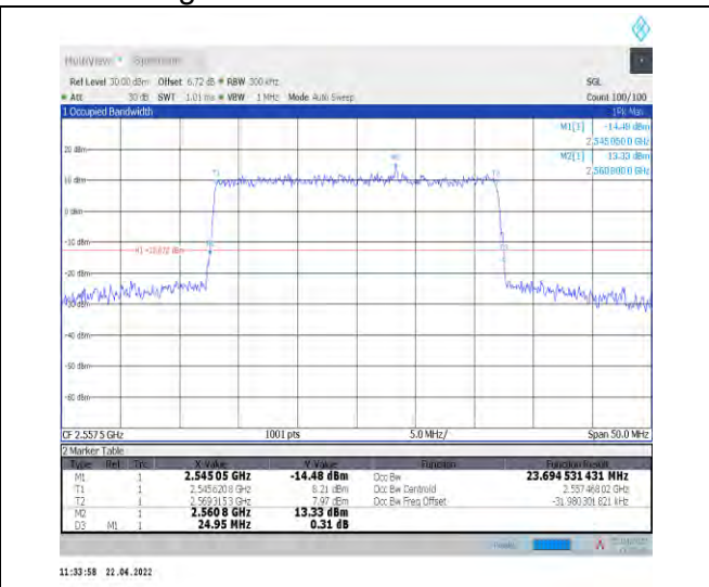
1-N7--15-25-H-8-CP-64QAM-Outer_Full-133@0-Ant 0-23.695-24.950-≤25-PASS
