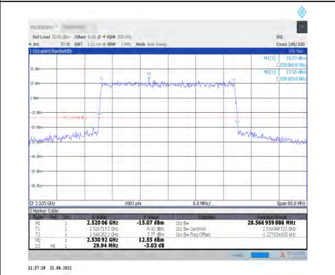
1-N7--15-30-M-4-DFT-64QAM-Outer_Full-160@0-Ant 0-28.567-29.940-≤30-PASS
