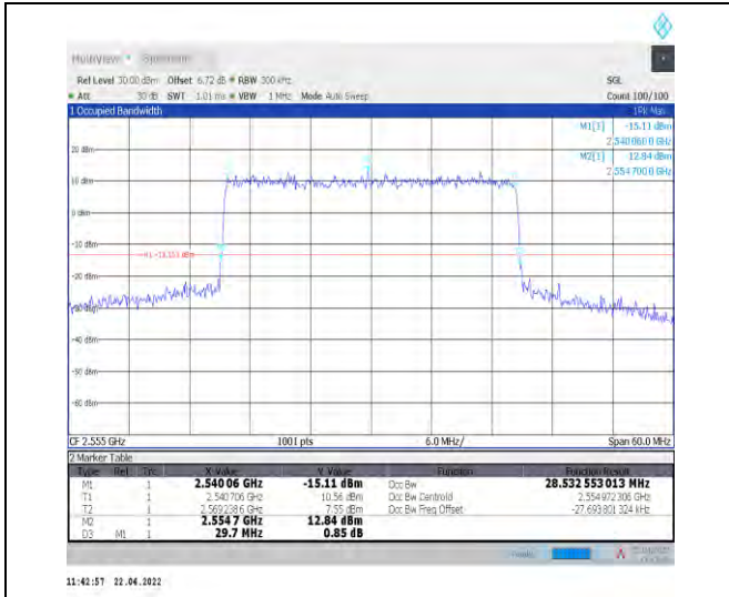
1-N7--15-30-H-4-DFT-64QAM-Outer_Full-160@0-Ant t0-28.533-29.700-<30-PASS
