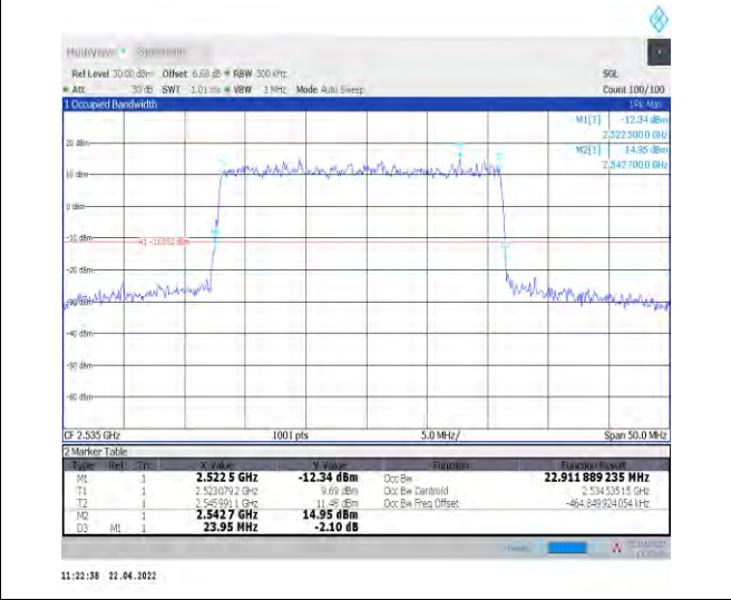
1-N7--15-25-M-3-DFT-16QAM-Outer_Full-128@0-Ant t0-22.912-23.950-<25-PASS
