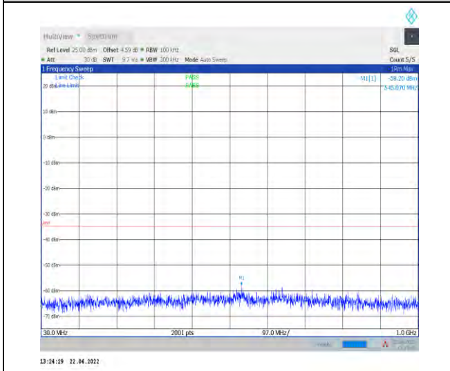
1-N7--15-40-H-1-DFT-PI2BPSK-Inner_1RB_Left-1@ 1-30-1000-Ant0--58.20--35-PASS
