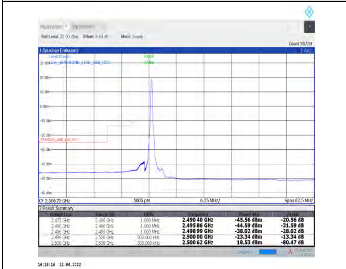
1-N7--15-25-L-4-CP-QPSK-Edge_1RB_Left-1@0-Ant0-PASS-see graph
