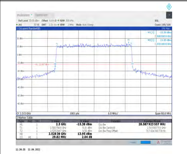
1-N7--15-30-L-1-DFT-QPSK-Outer_Full-160@0-Ant0 -28.589-29.820-≤30-PASS
