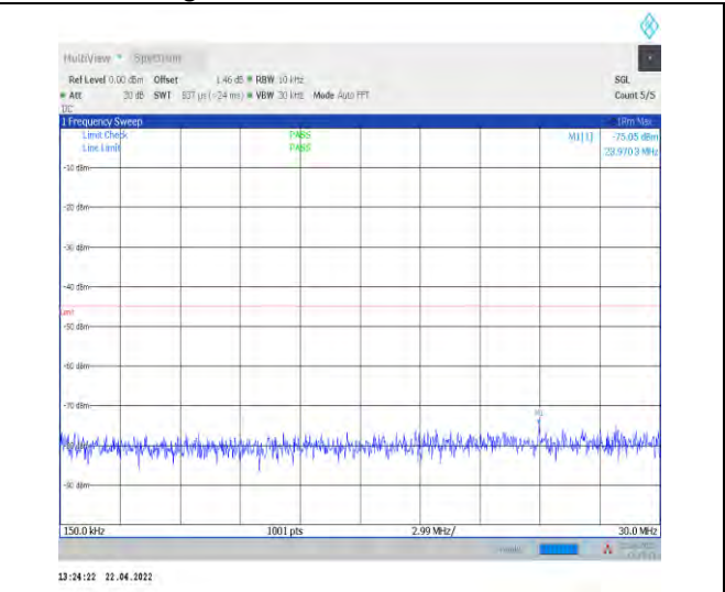
1-N7--15-40-H-1-DFT-PI2BPSK-Inner_1RB_Left-1@ 1-0.15-30-Ant0--75.05--45-PASS
