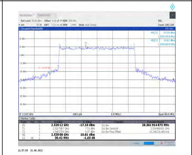
1-N7--15-30-M-8-CP-64QAM-Outer_Full-160@0-Ant 0-28.563-30.420-≤30-PASS
