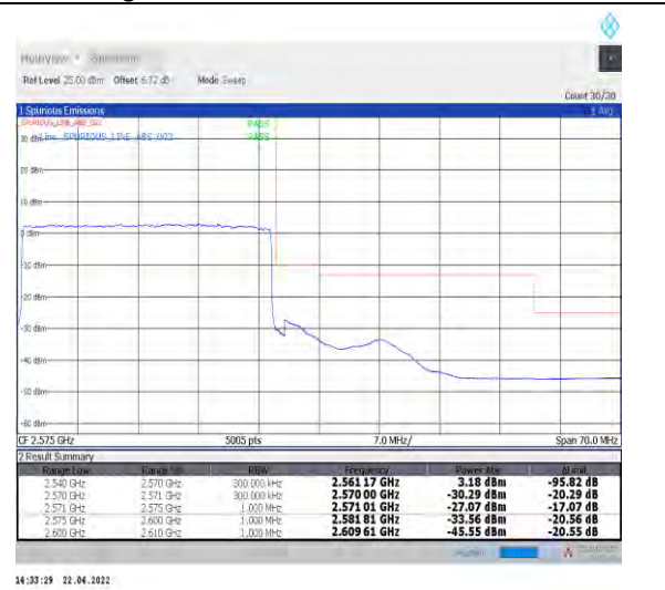
1-N7--15-30-H-3-DFT-PI2BPSK-Outer_Full-160@0-Ant0-PASS-see graph
