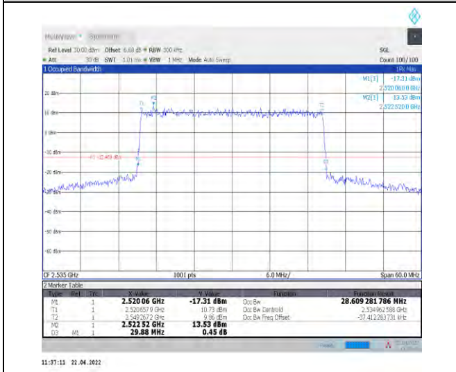
1-N7--15-30-M-3-DFT-16QAM-Outer_Full-160@0-Ant 0-28.61-29.880-≤30-PASS
