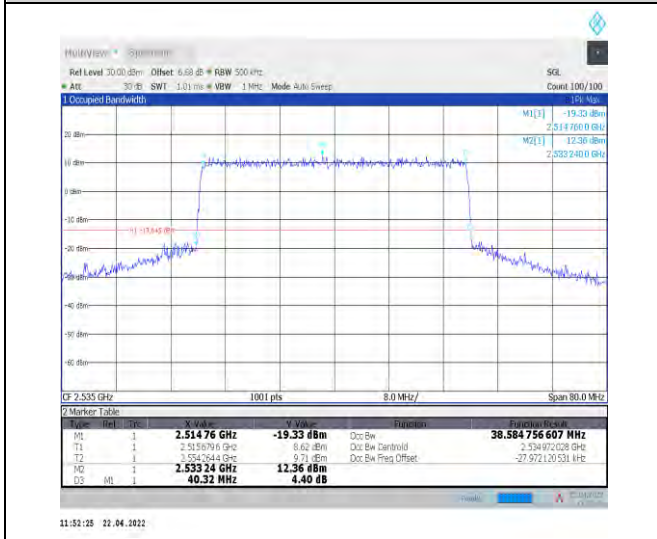
1-N7--15-40-M-8-CP-64QAM-Outer_Full-216@0-Ant0 0-38.585-40.320-≤40-PASS
