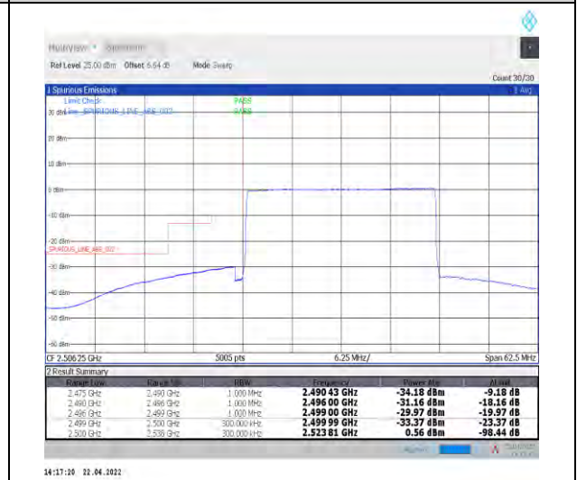
1-N7--15-25-L-6-CP-QPSK-Outer_Full-133@0-Ant0-PASS-see graph
