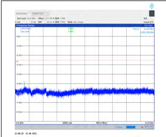
1-N7--15-40-L-1-DFT-PI2BPSK-Inner_1RB_Left-1@ 1-3000-12000-Ant0--51.69--25-PASS
