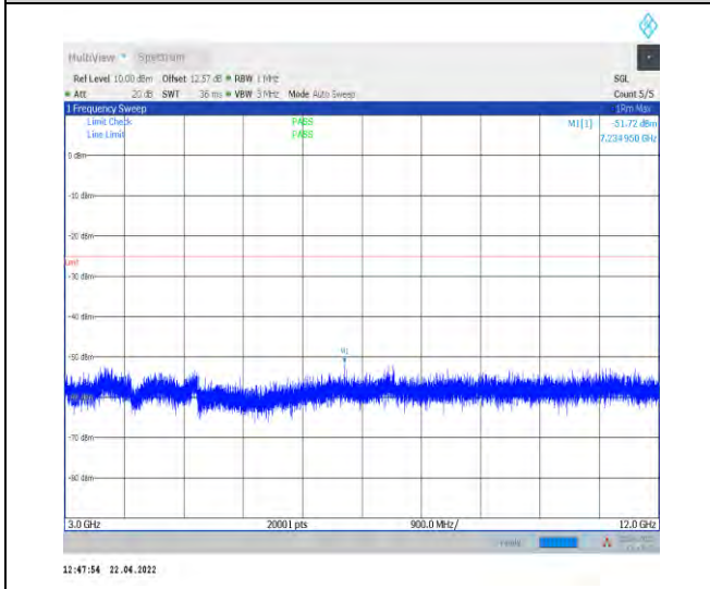
1-N7--15-40-M-1-DFT-PI2BPSK-Inner_1RB_Left-1 @1-3000-12000-Ant0--51.72--25-PASS
