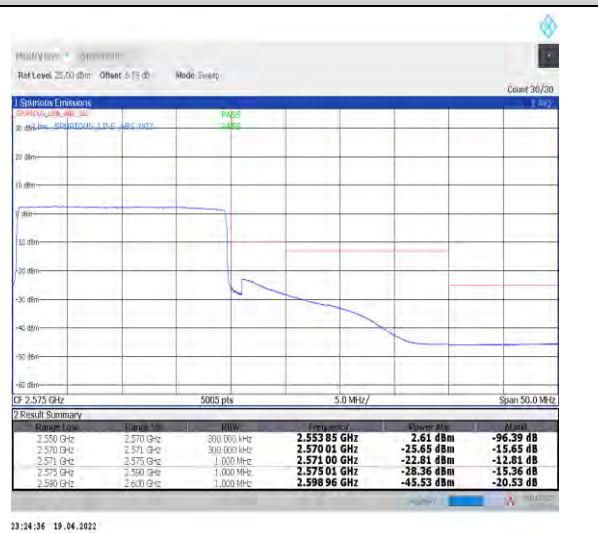
1-N7--15-20-H-6-CP-QPSK-Outer_Full-106@0-Ant0- PASS-see graph
