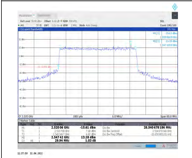
1-N7--15-30-M-7-CP-16QAM-Outer_Full-160@0-Ant 0-28.541-29.940-≤30-PASS
