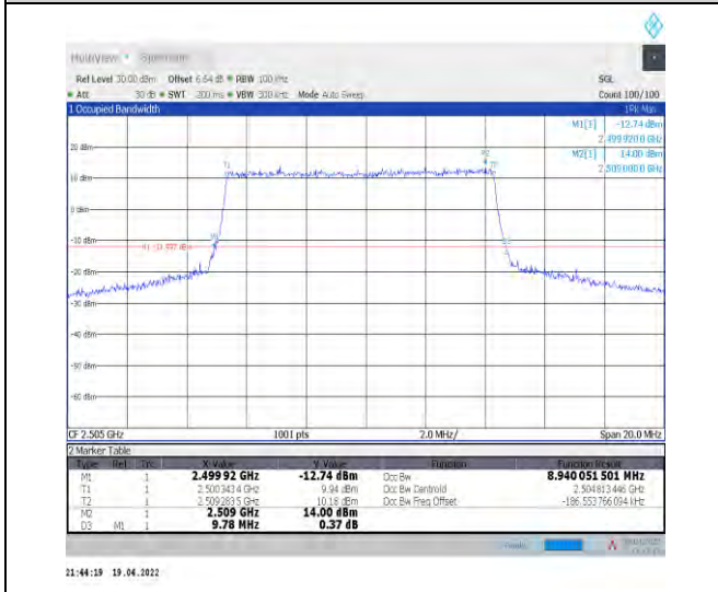
1-N7--15-10-L-4-DFT-64QAM-Outer_Full-50@0-Ant0 -8.94-9.780-<=10-PASS
