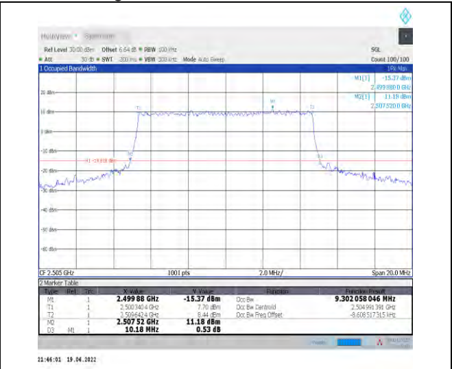
1-N7--15-10-L-7-CP-16QAM-Outer_Full-52@0-Ant0-9 9.302-10.180-≤10-PASS
