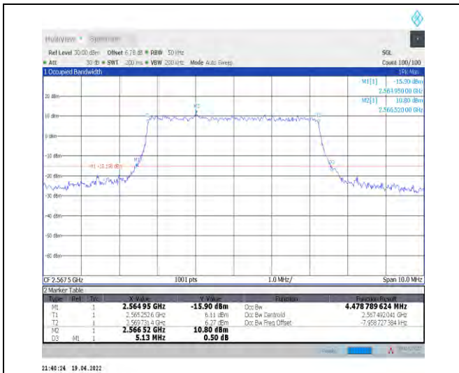
1-N7--15-5-H-7-CP-16QAM-Outer_Full-25@0-Ant0-4 .479-5.130-≤5-PASS
