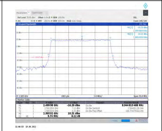
1-N7--15-10-L-5-DFT-256QAM-Outer_Full-50@0-Ant 0-8.945-9.740-<=10-PASS
