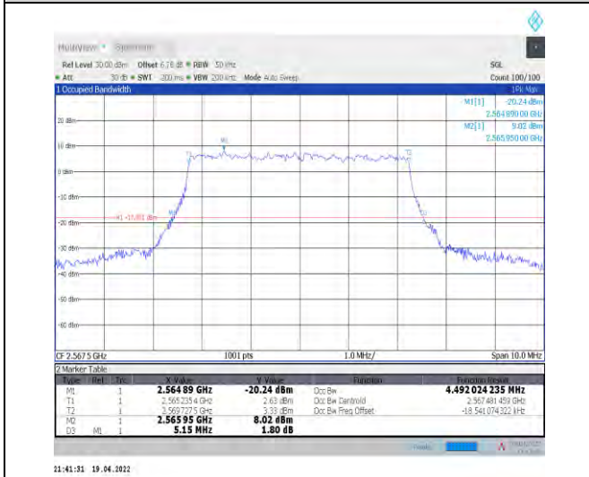
1-N7--15-5-H-9-CP-256QAM-Outer_Full-25@0-Ant0-4 4.492-5.150-≤5-PASS
