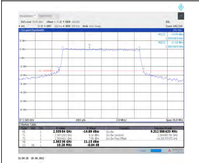
1-N7--15-10-H-6-CP-QPSK-Outer_Full-52@0-Ant0-9 .313-10.280-≤10-PASS
