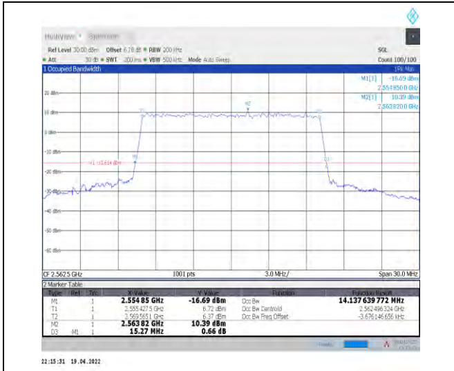
1-N7--15-15-H-9-CP-256QAM-Outer_Full-79@0-Ant 0-14.138-15.270-≤15-PASS
