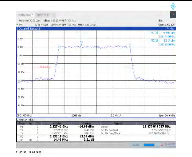
1-N7--15-15-M-5-DFT-256QAM-Outer_Full-75@0-Ant t0-13.43-14.460-≤15-PASS
