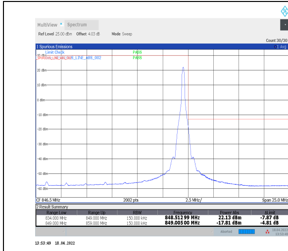
1-N5--15-15-H-2-DFT-PI2BPSK-Edge_1RB_Right-1@78-Ant0-seegraph-PASS-see graph
