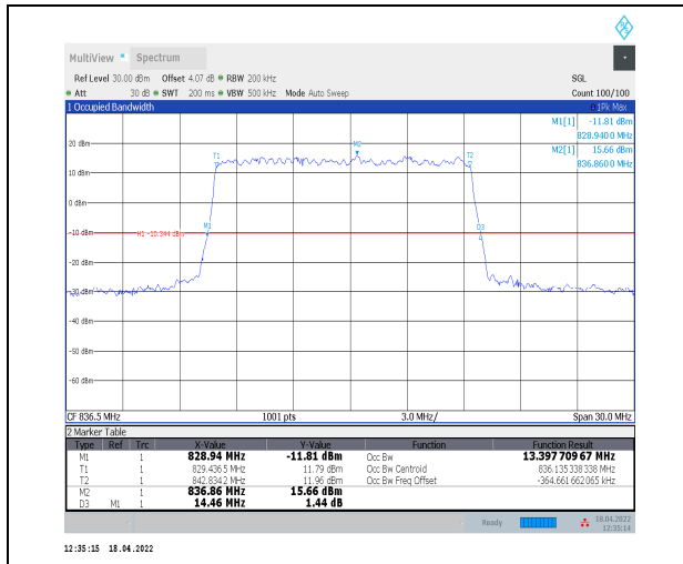
1-N5--15-15-M-2-DFT-PI2BPSK-Outer_Full-75@0-A nt0-13.398-14.460-≤15-PASS
