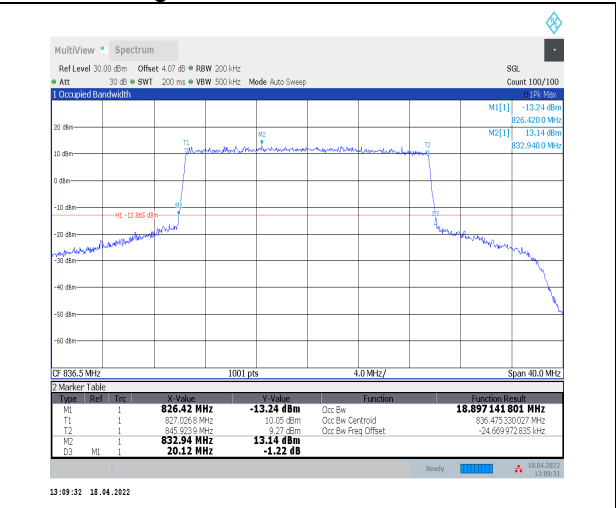
1-N5--15-20-M-8-CP-64QAM-Outer_Full-106@0-Ant 0-18.897-20.120-≤20-PASS
