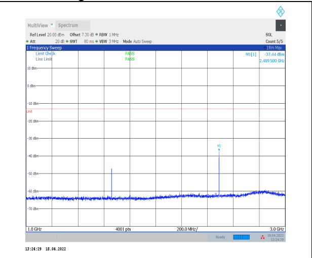
1-N5--15-20-H-1-DFT-PI2BPSK-Inner_1RB_Left-1@ 1-1000-3000-Ant0--37.44--13-PASS
