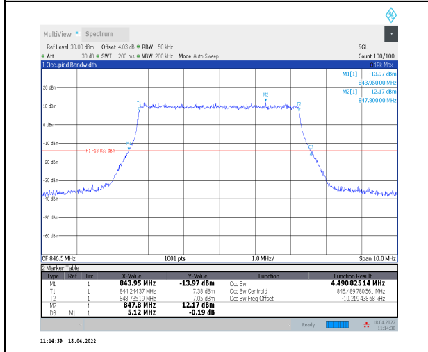
1-N5--15-5-H-5-DFT-256QAM-Outer_Full-25@0-Ant0-0-4.491-5.120-≤5-PASS
