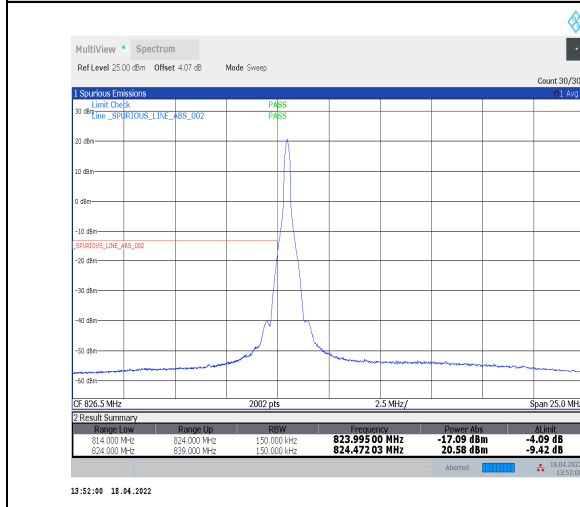
1-N5--15-15-L-4-CP-QPSK-Edge_1RB_Left-1@0-Ant0-seegraph-PASS-see graph
