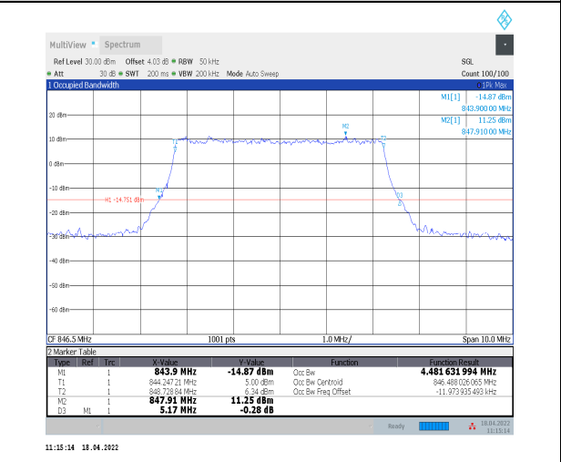
1-N5--15-5-H-6-CP-QPSK-Outer_Full-25@0-Ant0-4.482-5.170-≤5-PASS
