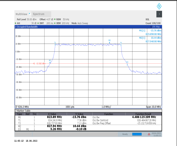
1-N5--15-5-L-8-CP-64QAM-Outer_Full-25@0-Ant0-4 .486-5.260-≤5-PASS
