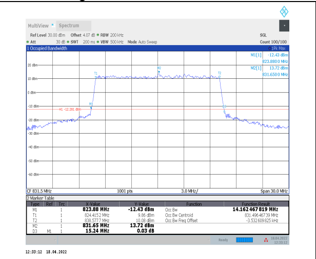
1-N5--15-15-L-8-CP-64QAM-Outer_Full-79@0-Ant0-14.162-15.240-<=15-PASS
