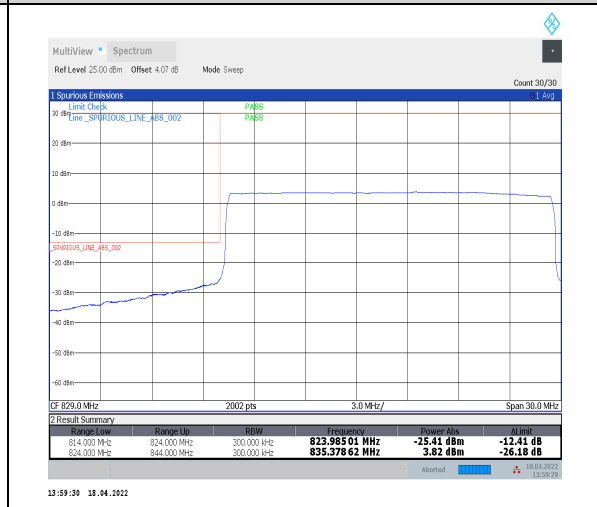
1-N5--15-20-L-6-CP-QPSK-Outer_Full-106@0-Ant0-seegraph-PASS-see graph
