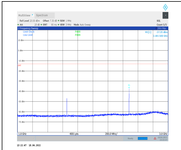
1-N5--15-20-M-1-DFT-PI2BPSK-Inner_1RB_Left-1@ 1-1000-3000-Ant0--37.35--13-PASS
