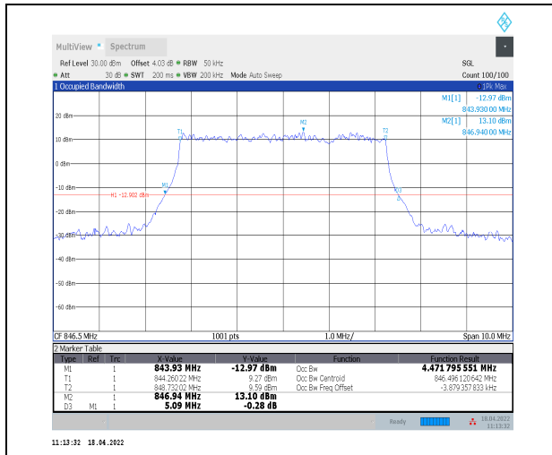
1-N5--15-5-H-3-DFT-16QAM-Outer_Full-25@0-Ant0-4.472-5.090-≤5-PASS
