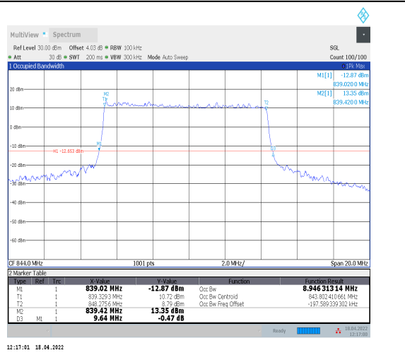
1-N5--15-10-H-3-DFT-16QAM-Outer_Full-50@0-Ant 0-8.946-9.640-≤10-PASS
