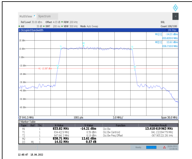
1-N5--15-15-H-5-DFT-256QAM-Outer_Full-75@0-Ant t0-13.418-14.520-<=15-PASS
