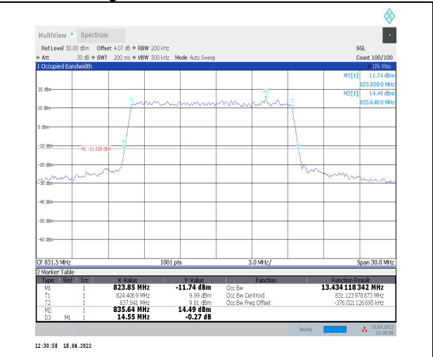
1-N5--15-15-L-4-DFT-64QAM-Outer_Full-75@0-Ant0 -13.434-14.550≤15-PASS
