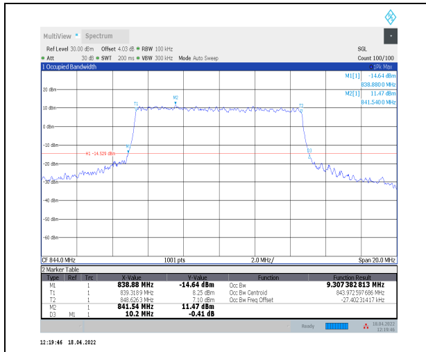
1-N5--15-10-H-8-CP-64QAM-Outer_Full-52@0-Ant0 -9.307-10.200≤10-PASS
