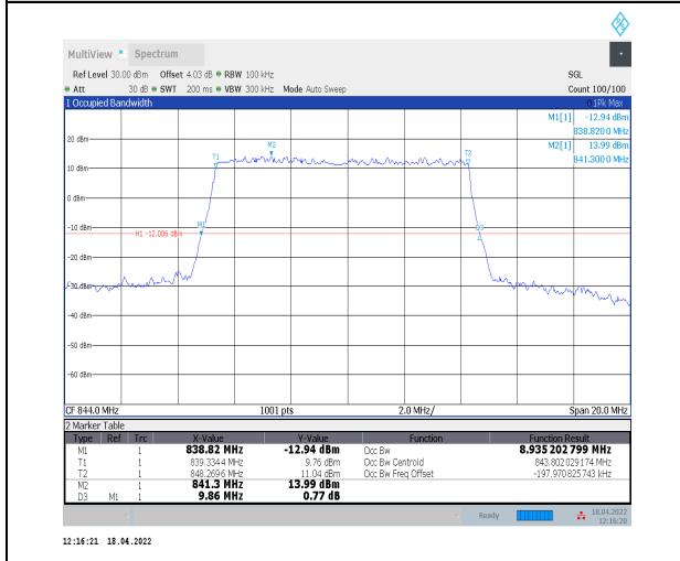
1-N5--15-10-H-2-DFT-PI2BPSK-Outer_Full-50@0-A nt0-8.935-9.860-≤10-PASS
