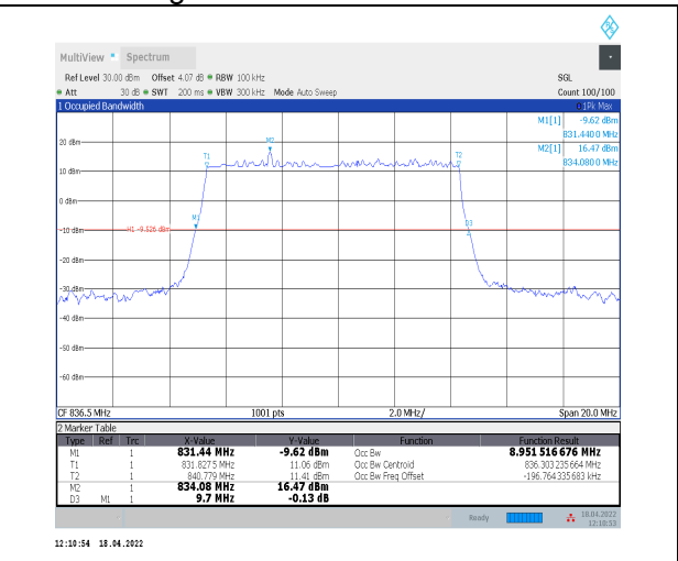
1-N5--15-10-M-2-DFT-PI2BPSK-Outer_Full-50@0-Ant0 -8.952-9.700-≤10-PASS
