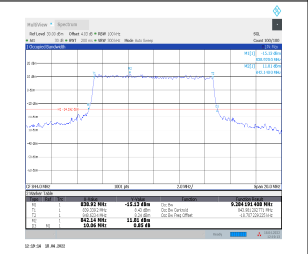
1-N5--15-10-H-7-CP-16QAM-Outer_Full-52@0-Ant0-9 9.284-10.060-<=10-PASS
