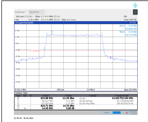
1-N5--15-15-L-3-DFT-16QAM-Outer_Full-75@0-Ant 0-13.446-14.490≤15-PASS
