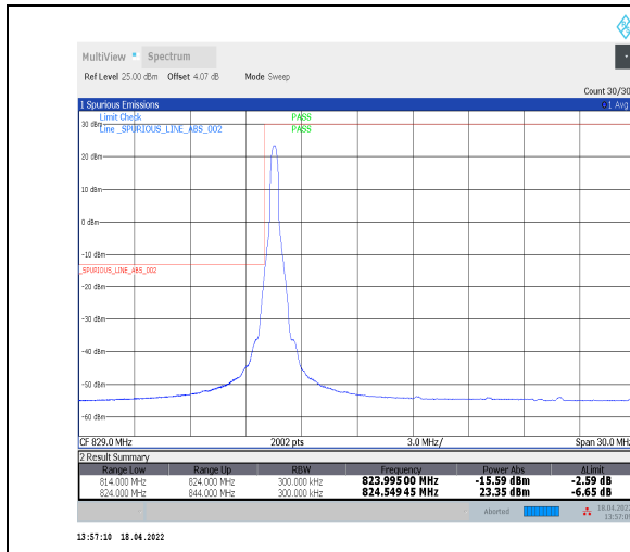
1-N5--15-20-L-1-DFT-PI2BPSK-Edge_1RB_Left-1@0-Ant0-seegraph-PASS-see graph
