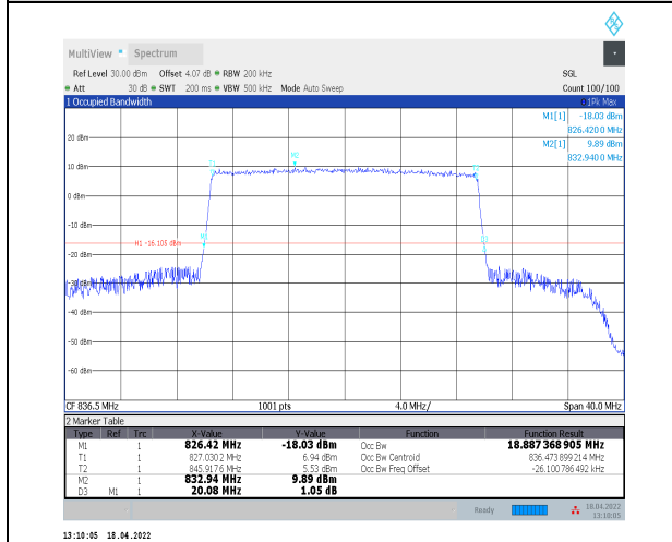
1-N5--15-20-M-9-CP-256QAM-Outer_Full-106@0-A nt0-18.887-20.080-≤20-PASS
