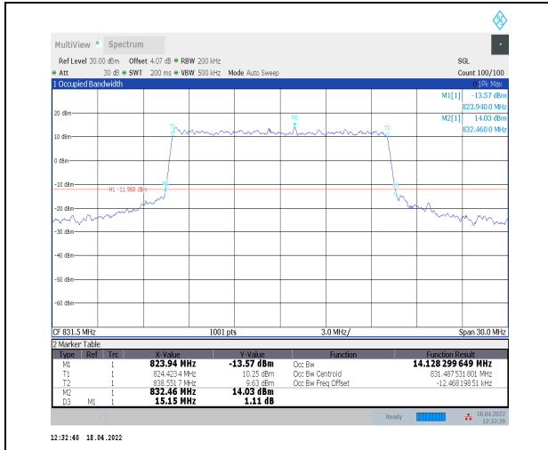
1-N5--15-15-L-7-CP-16QAM-Outer_Full-79@0-Ant0-14.128-15.150-<=15-PASS
