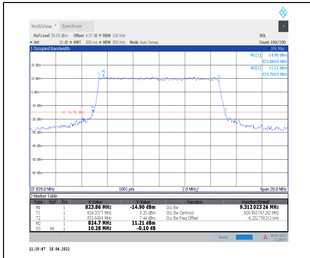
1-N5--15-10-L-6-CP-QPSK-Outer_Full-52@0-Ant0-9 9.312-10.280-≤10-PASS
