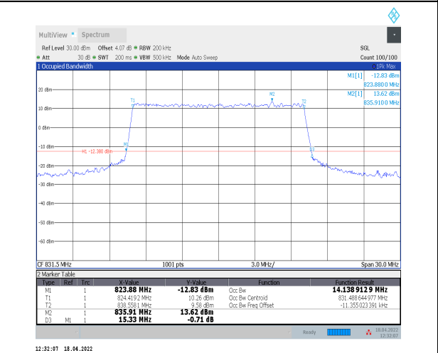
1-N5--15-15-L-6-CP-QPSK-Outer_Full-79@0-Ant0-1 4.139-15.330≤15-PASS
