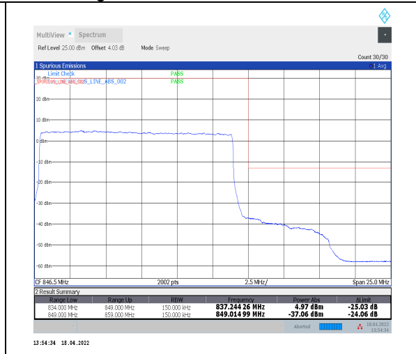
1-N5--15-15-H-3-DFT-PI2BPSK-Outer_Full-75@0-Ant0-seegraph-PASS-see graph
