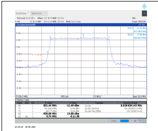
1-N5--15-10-M-1-DFT-QPSK-Outer_Full-50@0-Ant0 -8.929-9.740-≤10-PASS
