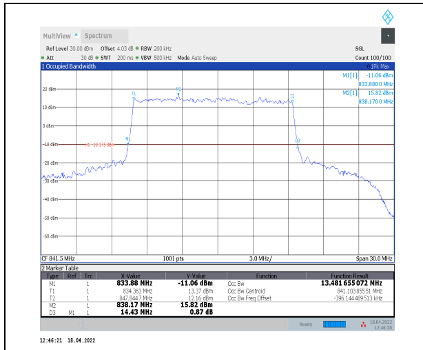
1-N5--15-15-H-1-DFT-QPSK-Outer_Full-75@0-Ant-0 13.482-14.430≤15-PASS
