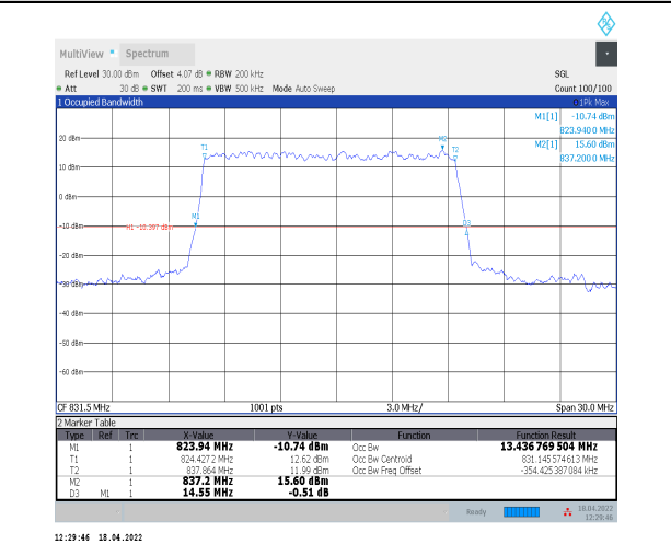
1-N5--15-15-L-2-DFT-PI2BPSK-Outer_Full-75@0-An t0-13.437-14.550≤15-PASS
