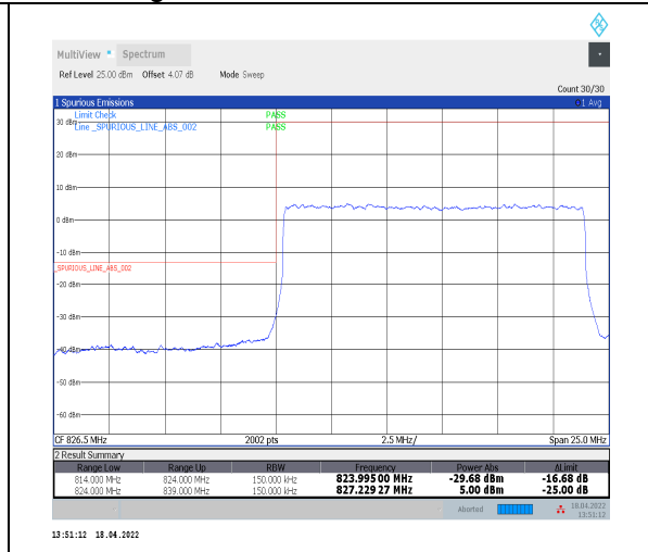
1-N5--15-15-L-3-DFT-PI2BPSK-Outer_Full-75@0-Ant0-seegraph-PASS-see graph
