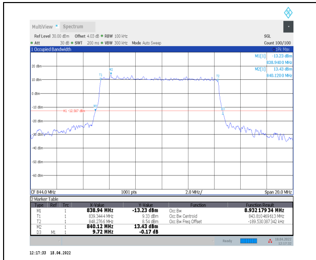
1-N5--15-10-H-4-DFT-64QAM-Outer_Full-50@0-Ant 0-8.932-9.720-<=10-PASS
