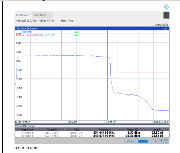
1-N5--15-20-H-3-DFT-PI2BPSK-Outer_Full-100@0-Ant0-seegraph-PASS-see graph
