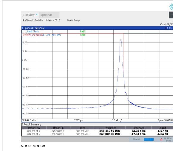
1-N5--15-20-H-2-DFT-PI2BPSK-Edge_1RB_Right-1@105-Ant0-seegraph-PASS-see graph
