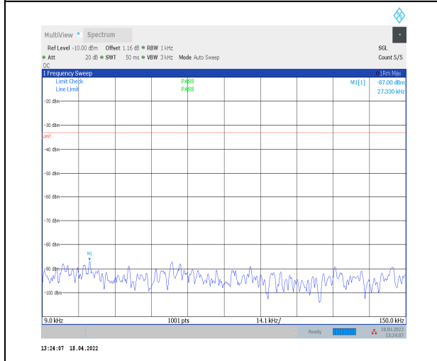
1-N5--15-20-H-1-DFT-PI2BPSK-Inner_1RB_Left-1@ 1-0.009-0.15-Ant0--87.00--33-PASS
