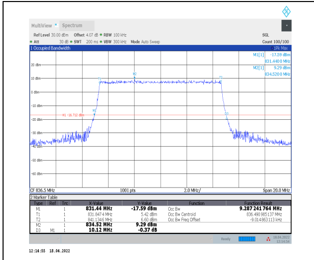
1-N5--15-10-M-9-CP-256QAM-Outer_Full-52@0-Ant 0-9.287-10.120-≤10-PASS
