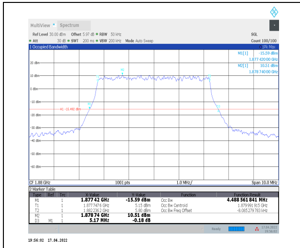
1-N2--15-5-M-4-DFT-64QAM-Outer_Full-25@0-Ant0 -4.489-5.170≤5-PASS
