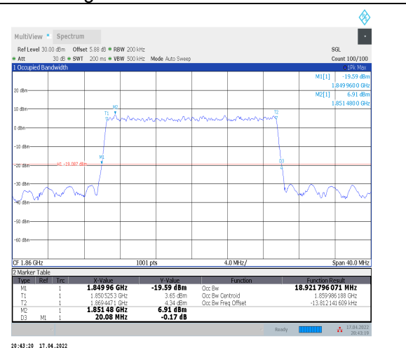
1-N2--15-20-L-9-CP-256QAM-Outer_Full-106@0-Ant 0-18.922-20.080-≤20-PASS
