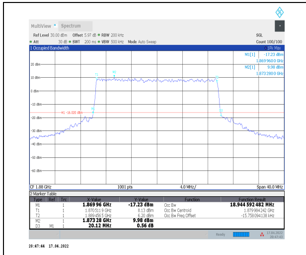
1-N2--15-20-M-7-CP-16QAM-Outer_Full-106@0-Ant 0-18.945-20.120-≤20-PASS
