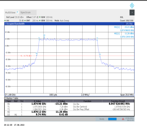
1-N2--15-10-M-4-DFT-64QAM-Outer_Full-50@0-Ant0 0-8.948-9.740-≤10-PASS
