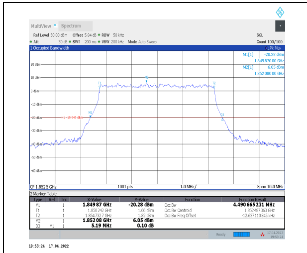
1-N2--15-5-L-9-CP-256QAM-Outer_Full-25@0-Ant0-4.491-5.190-<=5-PASS
