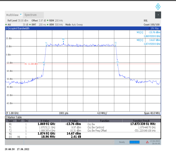
1-N2--15-20-M-2-DFT-PI2BPSK-Outer_Full-100@0-Ant 0-17.873-18.960-≤20-PASS
