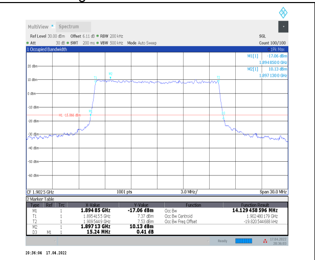
1-N2--15-15-H-6-CP-QPSK-Outer_Full-79@0-Ant0-1 4.129-15.240-<=15-PASS
