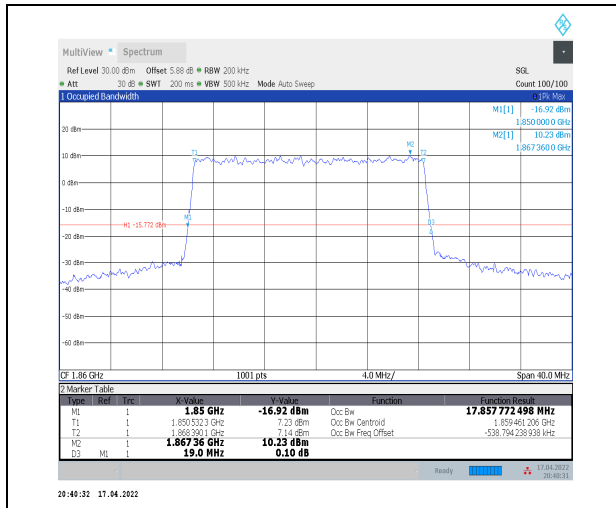
1-N2--15-20-L-4-DFT-64QAM-Outer_Full-100@0-An t0-17.858-19.000-<math>\leq 20</math>-PASS
