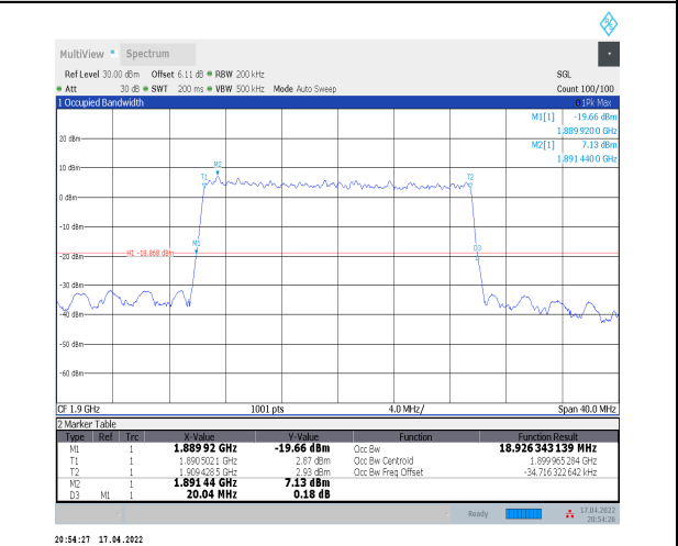
1-N2--15-20-H-9-CP-256QAM-Outer_Full-106@0-Ant t0-18.926-20.040-≤20-PASS
