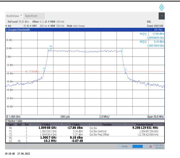
1-N2--15-10-H-7-CP-16QAM-Outer_Full-52@0-Ant0- 9.298-10.200-<=10-PASS
