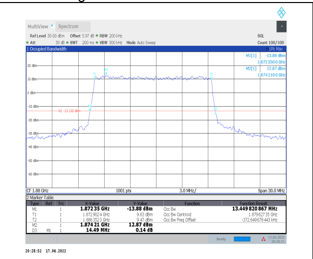
1-N2--15-15-M-3-DFT-16QAM-Outer_Full-75@0-Ant 0-13.45-14.490-≤15-PASS
