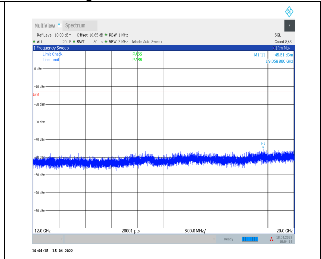
1-N2--15-20-H-1-DFT-PI2BPSK-Inner_1RB_Left-1@ 1-12000-20000-Ant0--45.51--13-PASS
