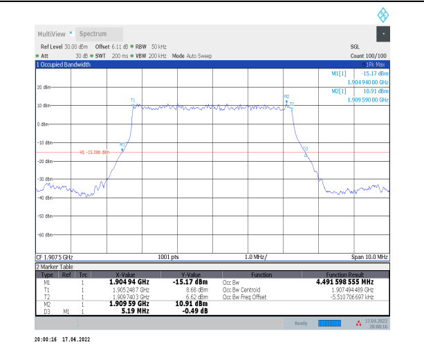
1-N2--15-5-H-2-DFT-PI2BPSK-Outer_Full-25@0-Ant0-4.492-5.190-≤5-PASS
