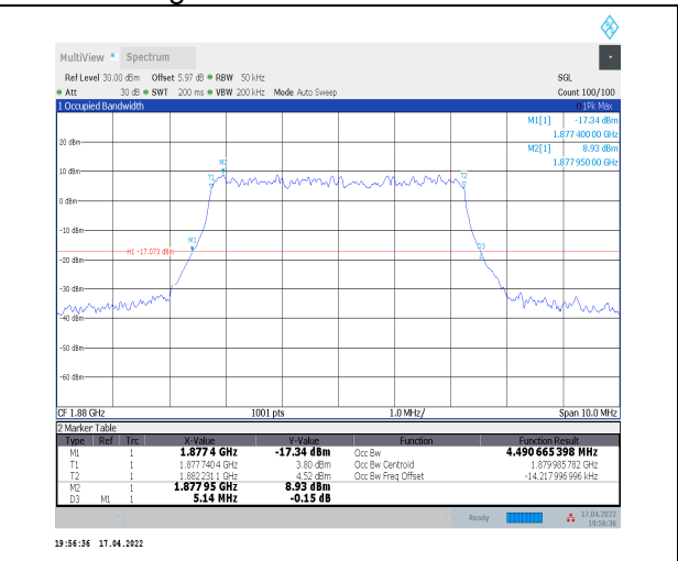
1-N2--15-5-M-5-DFT-256QAM-Outer_Full-25@0-Ant 0-4.491-5.140≤5-PASS
