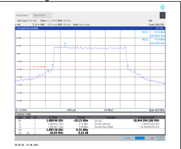
1-N2--15-20-H-7-CP-16QAM-Outer_Full-106@0-Ant 0-18.945-20.040-≤20-PASS
