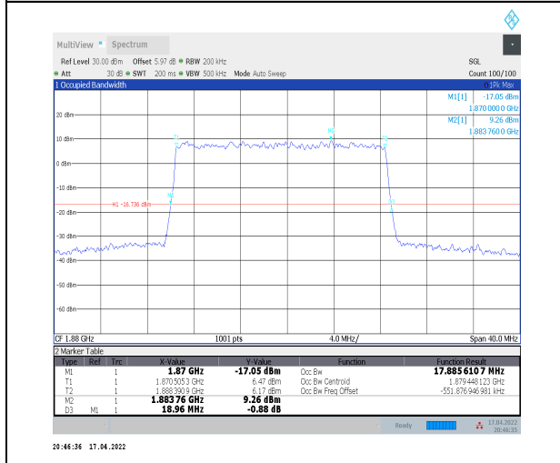
1-N2--15-20-M-5-DFT-256QAM-Outer_Full-100@0-A Ant0-17.886-18.960-≤20-PASS
