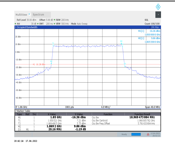
1-N2--15-20-L-7-CP-16QAM-Outer_Full-106@0-Ant0- -18.969-20.160-<math>\leq 20</math>-PASS
