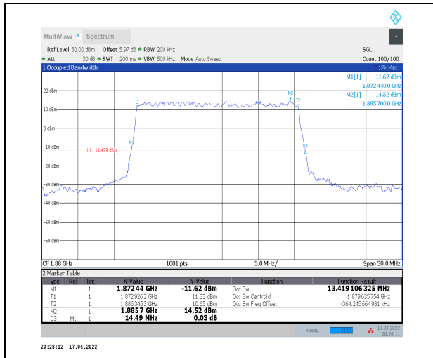
1-N2--15-15-M-2-DFT-PI2BPSK-Outer_Full-75@0-A nt0-13.419-14.490-≤15-PASS
