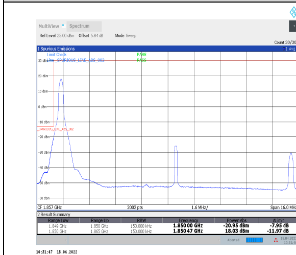
1-N2--15-15-L-4-CP-QPSK-Edge_1RB_Left-1@0-Ant0-seegraph-PASS-see graph
