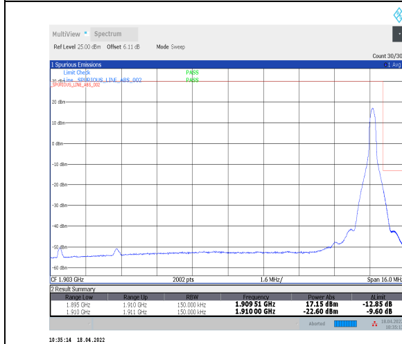
1-N2--15-15-H-5-CP-QPSK-Edge_1RB_Right-1@78-Ant0-seegraph-PASS-see graph
