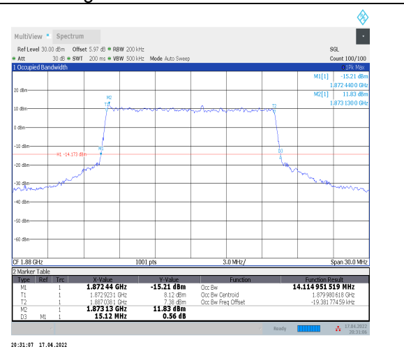
1-N2--15-15-M-7-CP-16QAM-Outer_Full-79@0-Ant0 -14.115-15.120≤15-PASS
