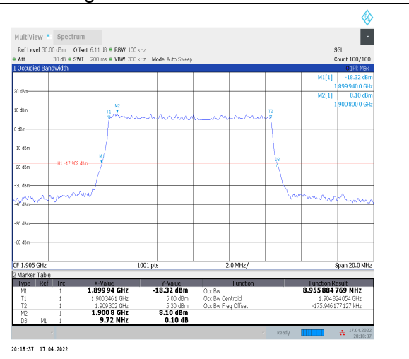
1-N2--15-10-H-5-DFT-256QAM-Outer_Full-50@0-An t0-8.956-9.720-<=10-PASS
