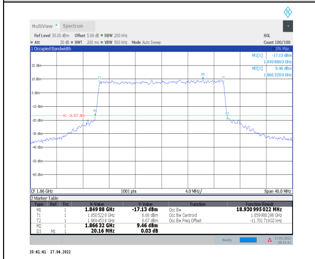
1-N2--15-20-L-6-CP-QPSK-Outer_Full-106@0-Ant0- 18.931-20.160-<math>\leq 20</math>-PASS
