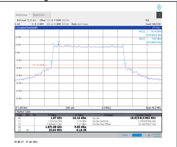
1-N2--15-20-M-8-CP-64QAM-Outer_Full-106@0-Ant 0-18.926-20.040-≤20-PASS
