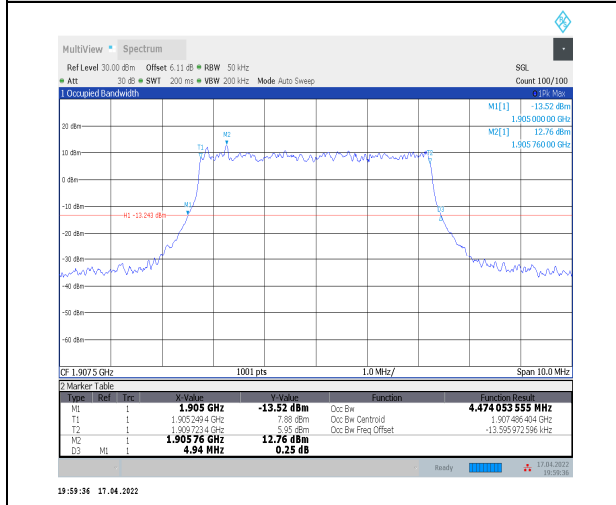
1-N2--15-5-H-1-DFT-QPSK-Outer_Full-25@0-Ant0-4.474-4.940-≤5-PASS
