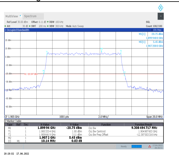
1-N2--15-10-H-9-CP-256QAM-Outer_Full-52@0-Ant 0-9.308-10.140≤10-PASS
