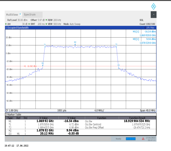
1-N2--15-20-M-6-CP-QPSK-Outer_Full-106@0-Ant0- 18.93-20.120-≤20-PASS
