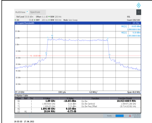
1-N2--15-20-H-8-CP-64QAM-Outer_Full-106@0-Ant 0-18.923-20.040-≤20-PASS
