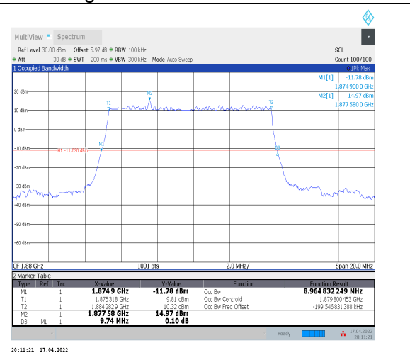
1-N2--15-10-M-2-DFT-PI2BPSK-Outer_Full-50@0-Ant0 -8.965-9.740-≤10-PASS
