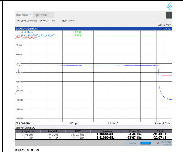
1-N2--15-15-H-6-CP-QPSK-Outer_Full-79@0-Ant0-seegraph-PASS-see graph
