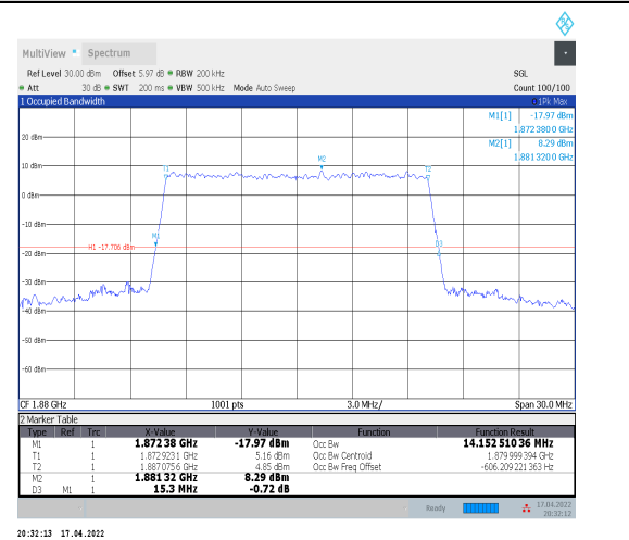
1-N2--15-15-M-9-CP-256QAM-Outer_Full-79@0-Ant 0-14.153-15.300≤15-PASS
