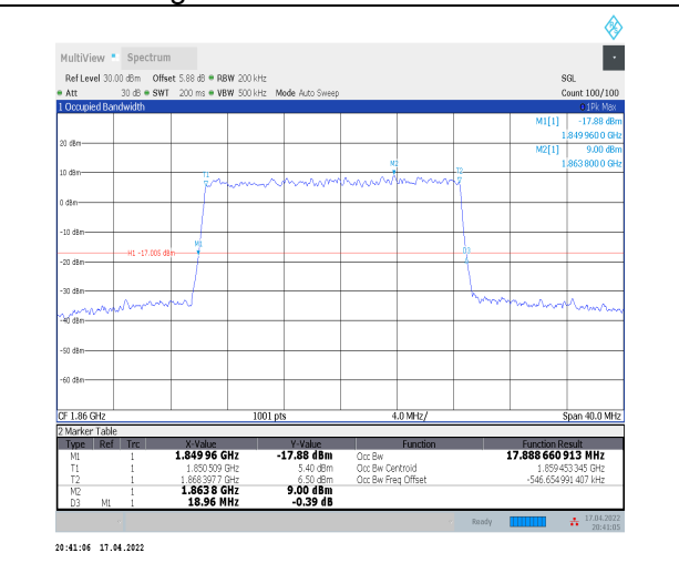
1-N2--15-20-L-5-DFT-256QAM-Outer_Full-100@0-A nt0-17.889-18.960-<math>\leq 20</math>-PASS
