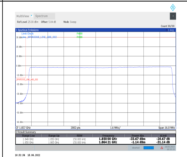
1-N2--15-15-L-6-CP-QPSK-Outer_Full-79@0-Ant0-seegraph-PASS-see graph
