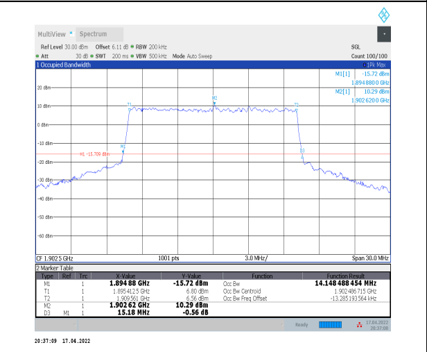
1-N2--15-15-H-8-CP-64QAM-Outer_Full-79@0-Ant0-1 14.148-15.180-<=15-PASS
