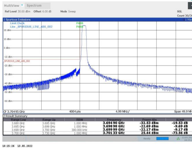
43-43-10MHz-20MHz-QPSK-QPSK-44645-44789-50RB#0-100RB#0
