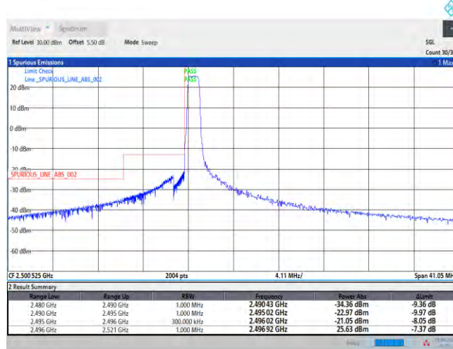
41-41-10MHz-15MHz-QPSK-QPSK-39703-39823-1RB#0-0RB#0
