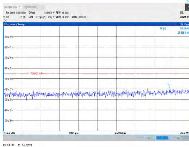
41-41-20MHz-20MHz-QPSK-QPSK-39750-39948-1RB#0-0RB#0-0.15~30MHz
