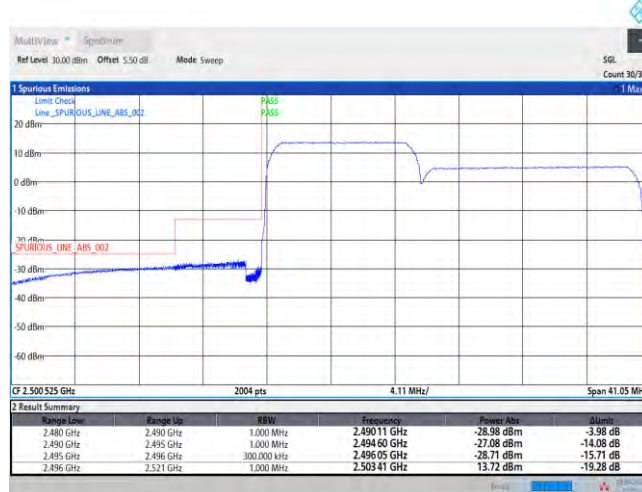
41-41-10MHz-15MHz-QPSK-QPSK-39703-39823-50RB#0-75RB#0
