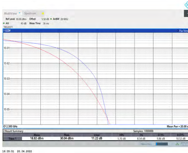
41-41-20MHz-20MHz-QPSK-QPSK-40521-40719-100RB#0-100RB#0
