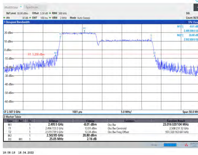
41-41-10MHz-15MHz-QPSK-QPSK-40549-40669-50RB#0-75RB#0
