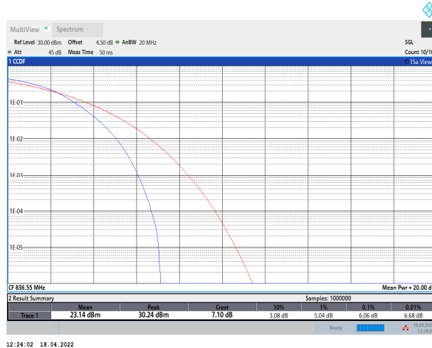
5-5-10MHz-10MHz-QPSK-QPSK-20476-20575-50RB#0-50RB#0
