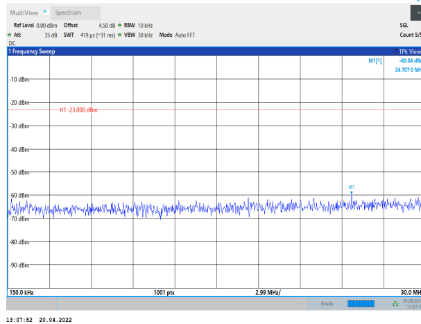
5-5-10MHz-10MHz-QPSK-QPSK-20450-20549-1RB#0-0RB#0-0.15~30MHz
