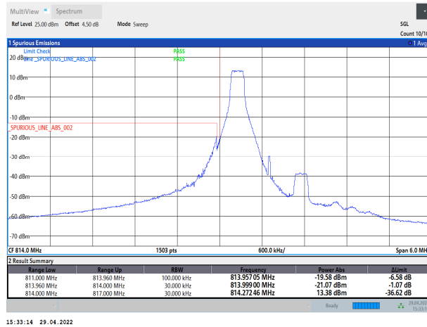
Band26-1.4MHz-QPSK-26697-6RB#0
