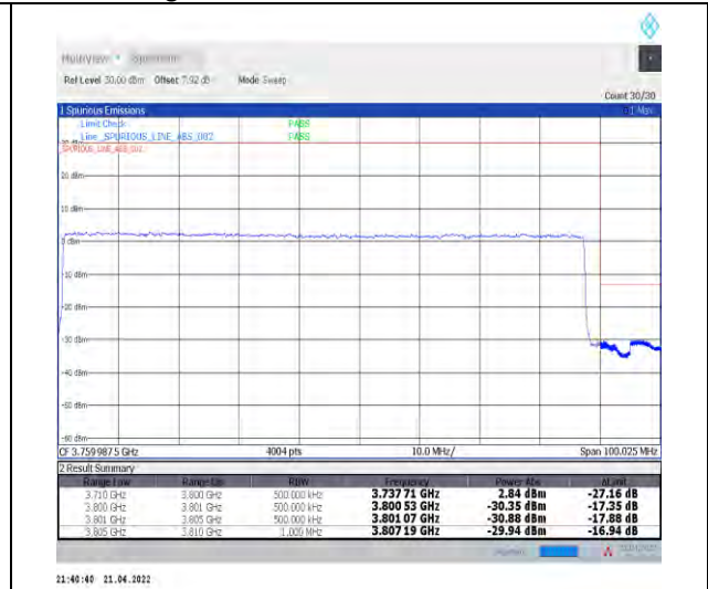
1-N78-3700-3800--30-90-H-3-DFT-PI2BPSK-Outer_Full-240@0-Ant1-PASS-see graph
