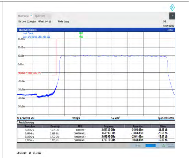
1-N78-3700-3800-PC1-30-30-L-3-DFT-PI2BPSK-Outer_Full-75@0-Ant1-1--PASS-see graph
