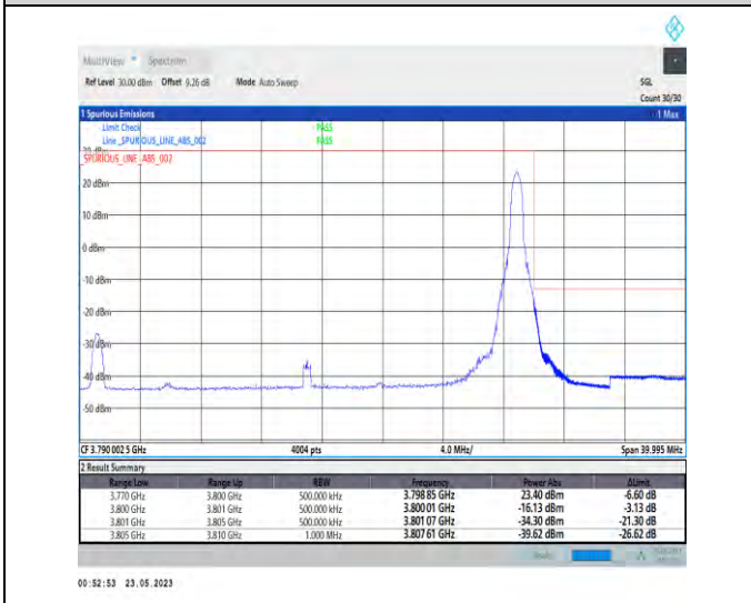
1-N78-3700-3800-PC1-30-30-H-5-CP-QPSK-Edge_1RB_Right-1@77-Ant1-1--PASS-see graph
