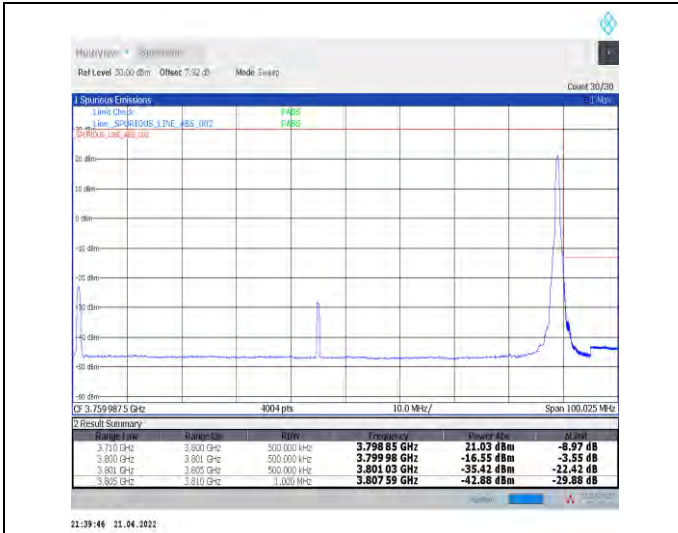
1-N78-3700-3800--30-90-H-2-DFT-PI2BPSK-Edge_1R_B_Right-1@244-Ant1-PASS-see graph
