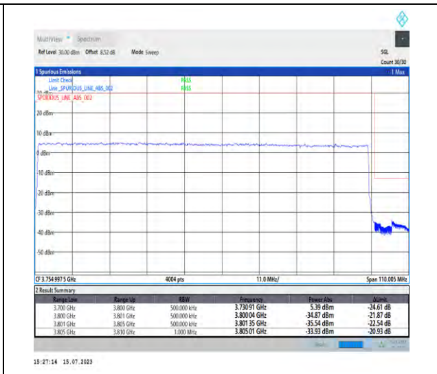
1-N78-3700-3800-PC1-30-100-H-3-DFT-PI2BPSK-Outer_Full-270@0-Ant1-1--PASS-see graph
