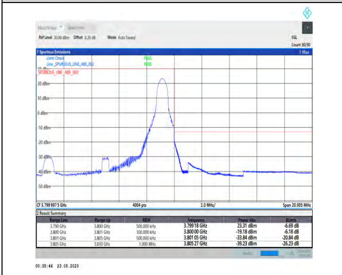
1-N78-3700-3800-PC1-30-10-H-5-CP-QPSK-Edge_1RB_Right-1@23-Ant1-1--PASS-see graph
