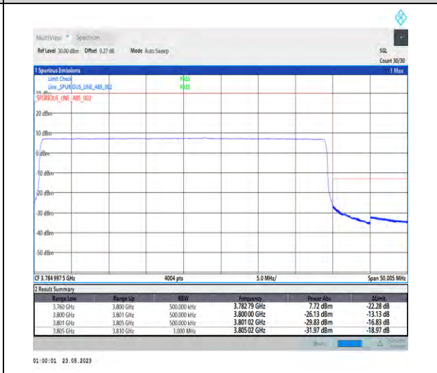
1-N78-3700-3800-PC1-30-40-H-6-CP-QPSK-Outer_Full-106@0-Ant1-1--PASS-see graph
