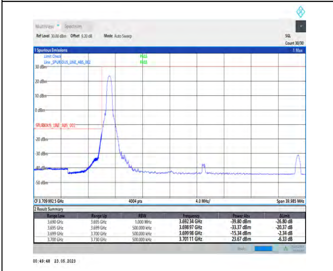
1-N78-3700-3800-PC1-30-30-L-4-CP-QPSK-Edge_1_RB_Left-1@0-Ant1-1--PASS-see graph
