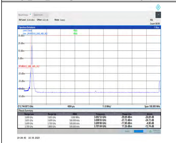
1-N78-3700-3800-PC1-30-100-L-4-CP-QPSK-Edge_1RB_Left-1@0-Ant1-1--PASS-see graph
