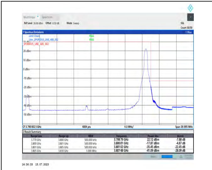
1-N78-3700-3800-PC1-30-30-H-2-DFT-PI2BPSK-Edge_1RB_Right-1@77-Ant1-1--PASS-see graph
