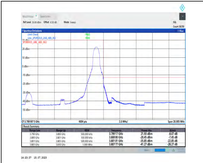
1-N78-3700-3800-PC1-30-10-H-2-DFT-PI2BPSK-Edge_1RB_Right-1@23-Ant1-1--PASS-see graph
