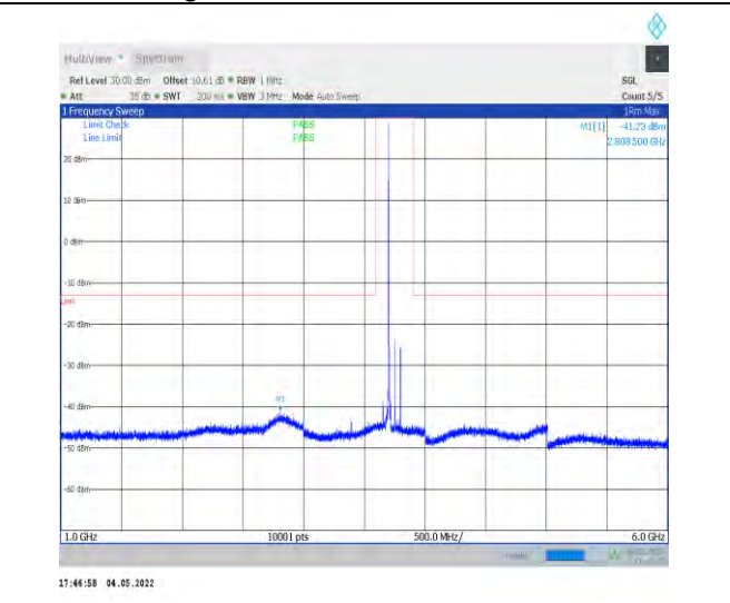
1-N78-3700-3800--30-100-M-1-DFT-PI2BPSK-Inner_ 1RB_Left-1@1-1000-6000-Ant1--41.23--13-PASS
