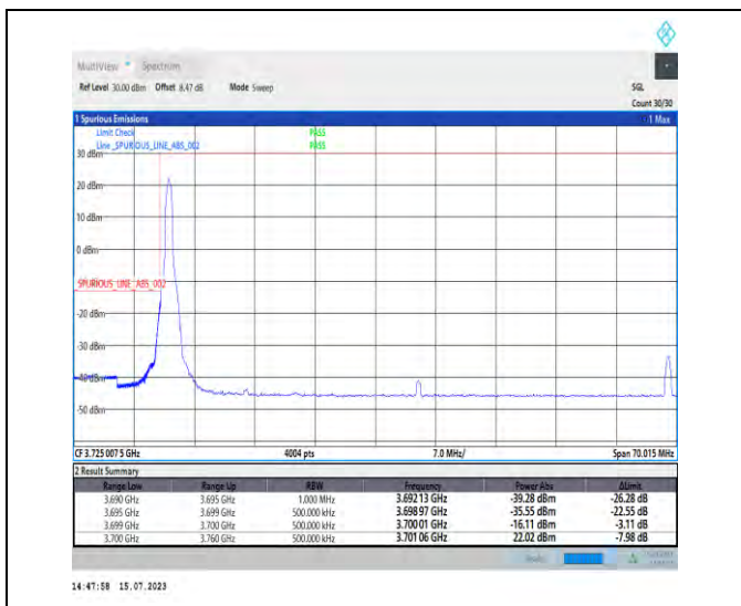
1-N78-3700-3800-PC1-30-60-L-1-DFT-PI2BPSK-Edge_1_RB_Left-1@0-Ant1-1--PASS-see graph
