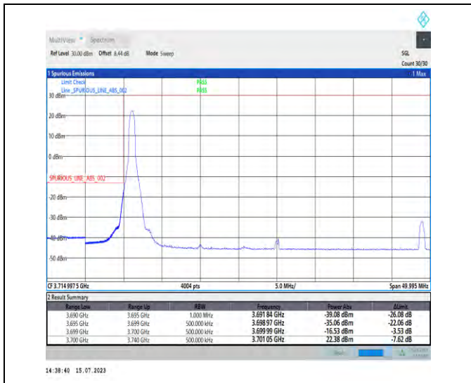
1-N78-3700-3800-PC1-30-40-L-1-DFT-PI2BPSK-Edge_1_RB_Left-1@0-Ant1-1--PASS-see graph
