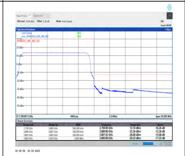
1-N78-3700-3800-PC1-30-10-H-6-CP-QPSK-Outer_Full-24@0-Ant1-1--PASS-see graph
