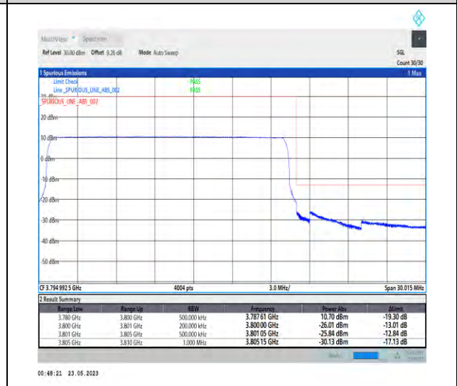
1-N78-3700-3800-PC1-30-20-H-6-CP-QPSK-Outer_Full-51@0-Ant1-1--PASS-see graph
