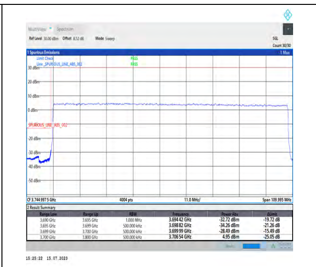
1-N78-3700-3800-PC1-30-100-L-3-DFT-PI2BPSK-Outer_Full-270@0-Ant1-1--PASS-see graph
