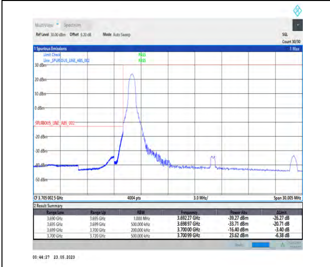
1-N78-3700-3800-PC1-30-20-L-4-CP-QPSK-Edge_1_RB_Left-1@0-Ant1-1--PASS-see graph
