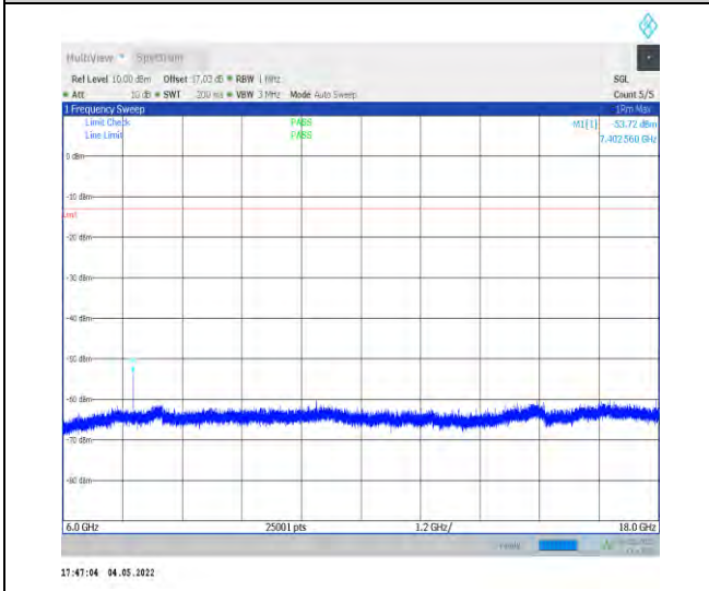
1-N78-3700-3800--30-100-M-1-DFT-PI2BPSK-Inner _1RB_Left-1@1-6000-18000-Ant1--53.72--13-PASS
