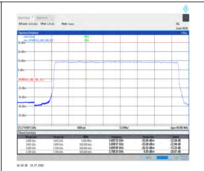
1-N78-3700-3800-PC1-30-40-L-3-DFT-PI2BPSK-Outer_Full-100@0-Ant1-1--PASS-see graph
