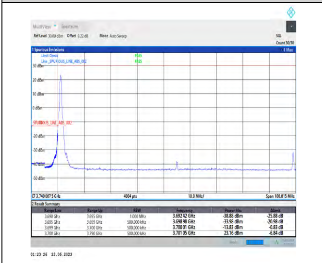
1-N78-3700-3800-PC1-30-90-L-4-CP-QPSK-Edge_1_RB_Left-1@0-Ant1-1--PASS-see graph
