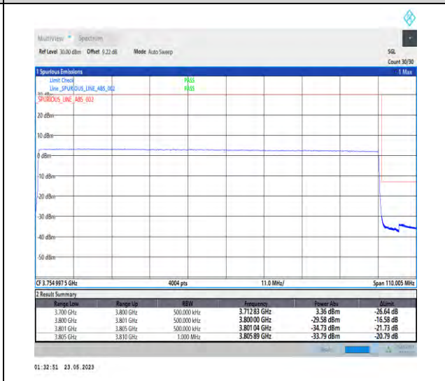
1-N78-3700-3800-PC1-30-100-H-6-CP-QPSK-Outer_Full-273@0-Ant1-1--PASS-see graph
