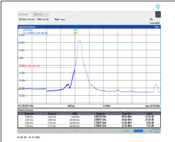
1-N78-3700-3800-PC1-30-15-L-1-DFT-PI2BPSK-Edge_1_RB_Left-1@0-Ant1-1--PASS-see graph
