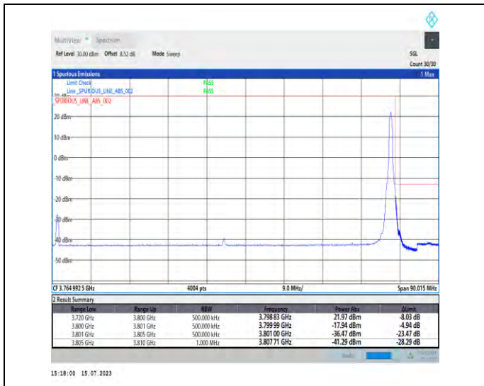
1-N78-3700-3800-PC1-30-80-H-2-DFT-PI2BPSK-Edge_1RB_Right-1@216-Ant1-1--PASS-see graph
