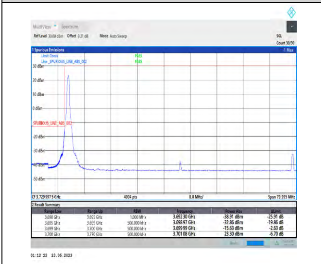
1-N78-3700-3800-PC1-30-70-L-4-CP-QPSK-Edge_1_RB_Left-1@0-Ant1-1--PASS-see graph
