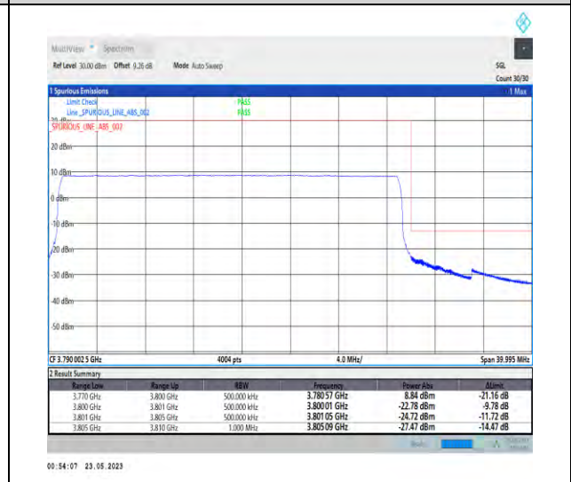
1-N78-3700-3800-PC1-30-30-H-6-CP-QPSK-Outer_Full-78@0-Ant1-1--PASS-see graph
