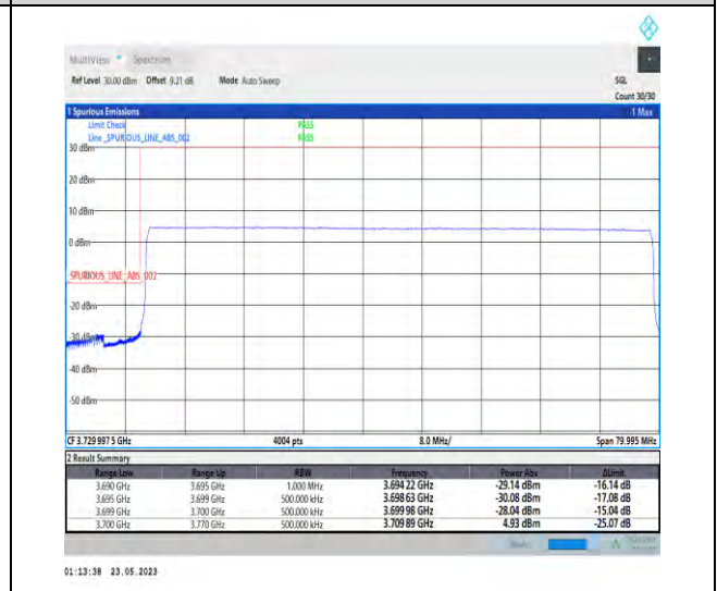
1-N78-3700-3800-PC1-30-70-L-6-CP-QPSK-Outer_Full-189@0-Ant1-1--PASS-see graph
