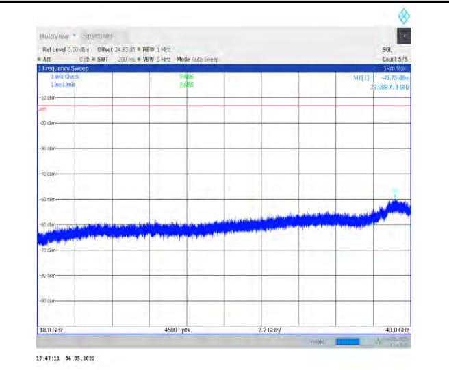
1-N78-3700-3800--30-100-M-1-DFT-PI2BPSK-Inner_ 1RB_Left-1@1-18000-40000-Ant1--49.75--13-PASS
