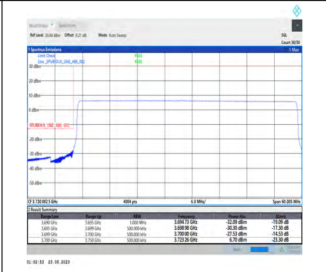
1-N78-3700-3800-PC1-30-50-L-6-CP-QPSK-Outer_Full-133@0-Ant1-1--PASS-see graph
