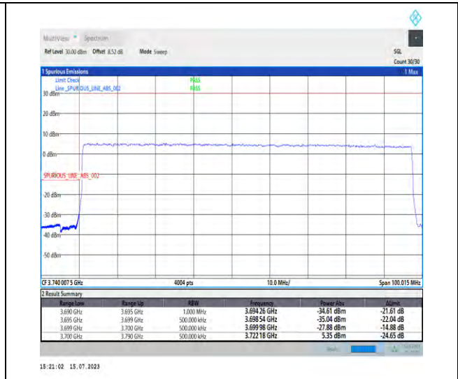
1-N78-3700-3800-PC1-30-90-L-3-DFT-PI2BPSK-Outer_Full-240@0-Ant1-1--PASS-see graph
