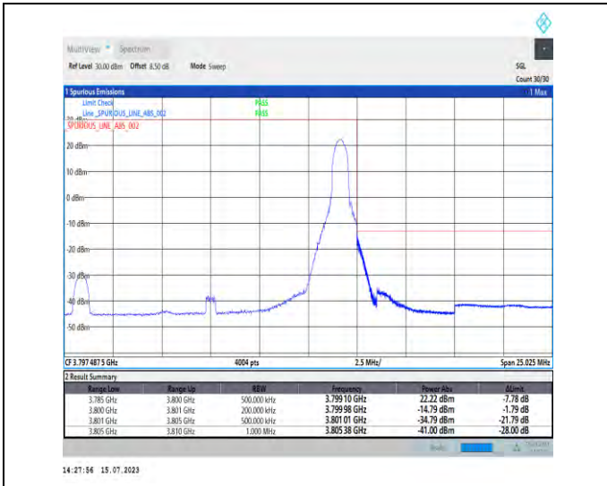
1-N78-3700-3800-PC1-30-15-H-2-DFT-PI2BPSK-Edge_1RB_Right-1@37-Ant1-1--PASS-see graph
