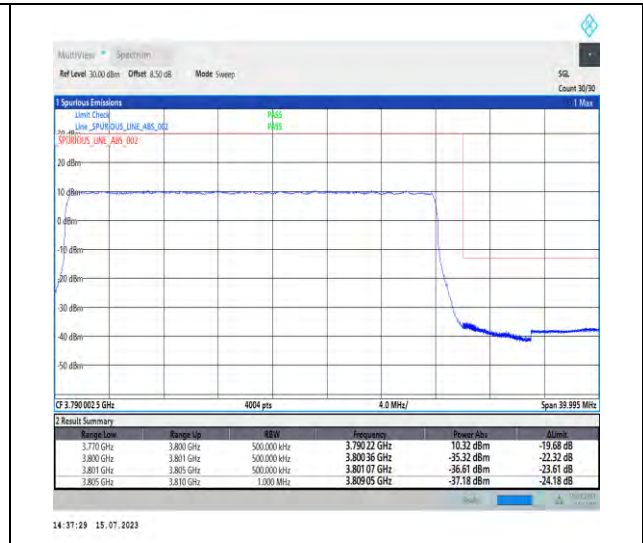
1-N78-3700-3800-PC1-30-30-H-3-DFT-PI2BPSK-Outer_Full-75@0-Ant1-1--PASS-see graph
