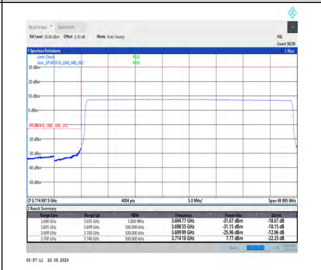
1-N78-3700-3800-PC1-30-40-L-6-CP-QPSK-Outer_Full-106@0-Ant1-1--PASS-see graph
