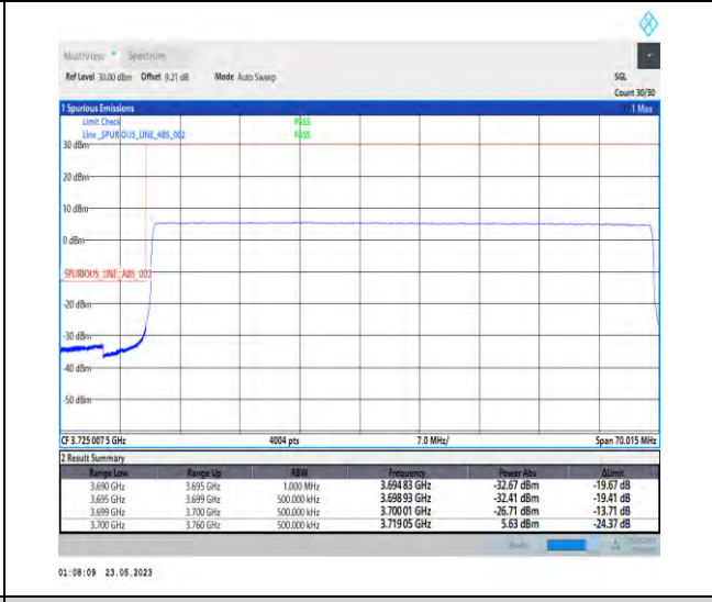
1-N78-3700-3800-PC1-30-60-L-6-CP-QPSK-Outer_Full-162@0-Ant1-1--PASS-see graph
