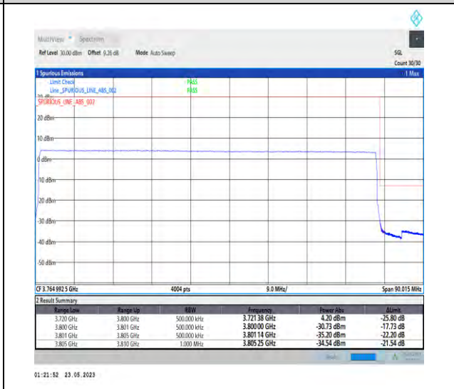
1-N78-3700-3800-PC1-30-80-H-6-CP-QPSK-Outer_Full-217@0-Ant1-1--PASS-see graph
