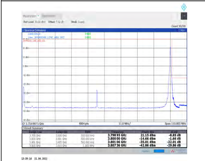
1-N78-3700-3800--30-100-H-5-CP-QPSK-Edge_1RB_Right-1@272-Ant1-PASS-see graph
