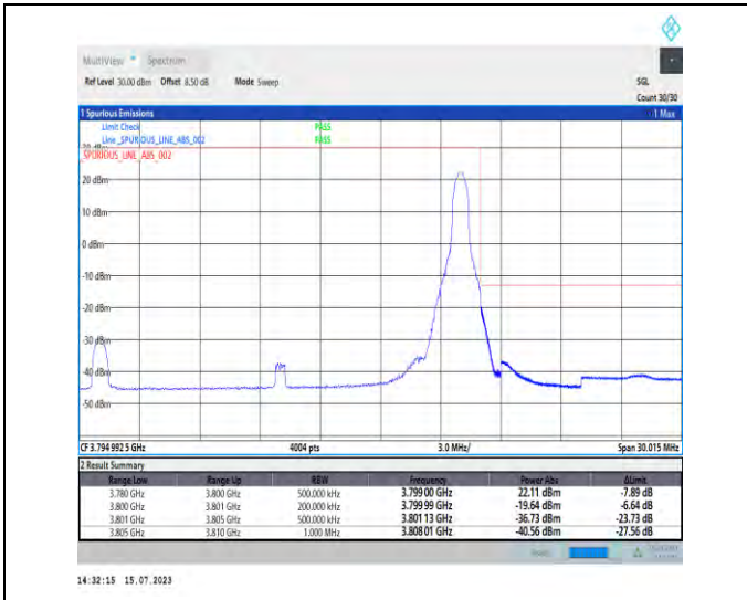
1-N78-3700-3800-PC1-30-20-H-2-DFT-PI2BPSK-Edge_1RB_Right-1@50-Ant1-1--PASS-see graph
