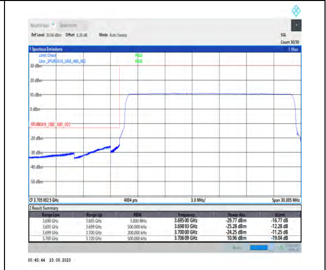
1-N78-3700-3800-PC1-30-20-L-6-CP-QPSK-Outer_Full-51@0-Ant1-1--PASS-see graph
