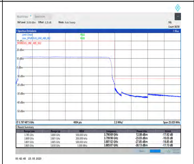
1-N78-3700-3800-PC1-30-15-H-6-CP-QPSK-Outer_Full-38@0-Ant1-1--PASS-see graph
