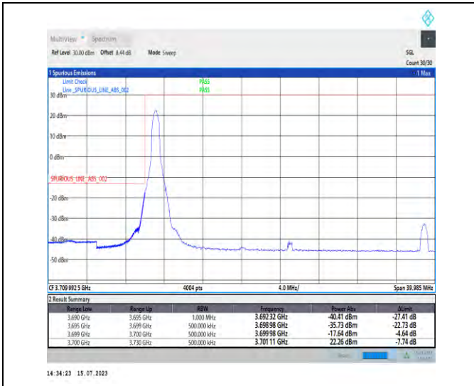
1-N78-3700-3800-PC1-30-30-L-1-DFT-PI2BPSK-Edge_1_RB_Left-1@0-Ant1-1--PASS-see graph
