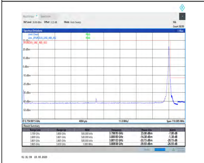
1-N78-3700-3800-PC1-30-100-H-5-CP-QPSK-Edge_1RB_Right-1@272-Ant1-1--PASS-see graph
