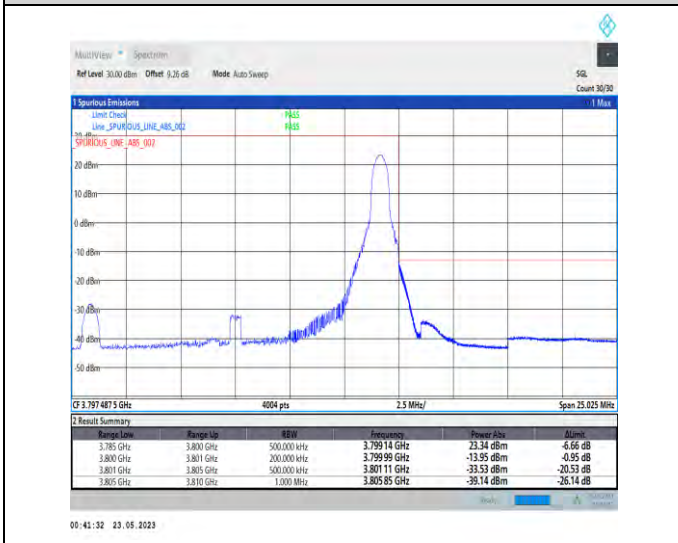
1-N78-3700-3800-PC1-30-15-H-5-CP-QPSK-Edge_1RB_Right-1@37-Ant1-1--PASS-see graph
