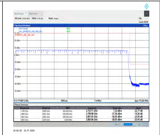
1-N78-3700-3800-PC1-30-60-H-3-DFT-PI2BPSK-Outer_Full-162@0-Ant1-1--PASS-see graph
