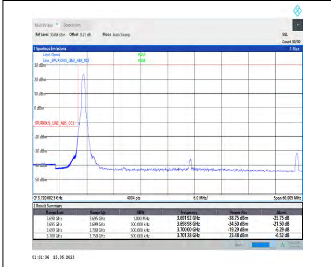
1-N78-3700-3800-PC1-30-50-L-4-CP-QPSK-Edge_1RB_Left-1@0-Ant1-1--PASS-see graph
