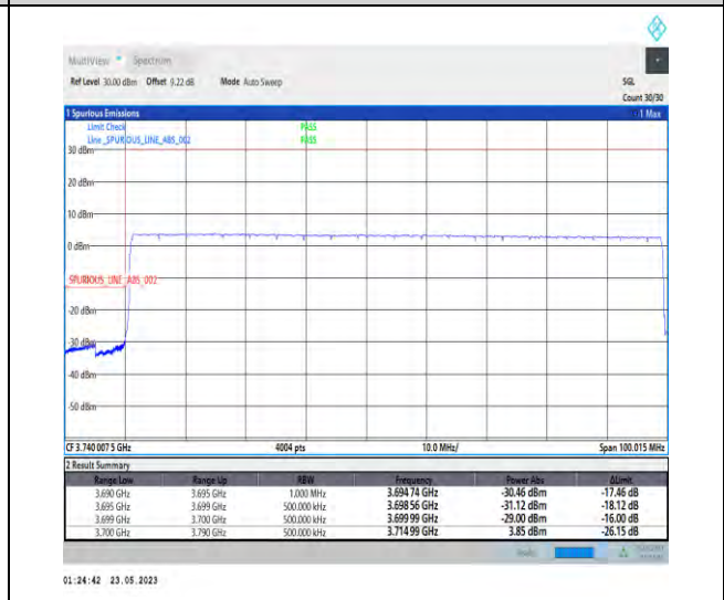
1-N78-3700-3800-PC1-30-90-L-6-CP-QPSK-Outer_Full-245@0-Ant1-1--PASS-see graph
