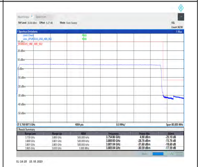
1-N78-3700-3800-PC1-30-70-H-6-CP-QPSK-Outer_Full-189@0-Ant1-1--PASS-see graph
