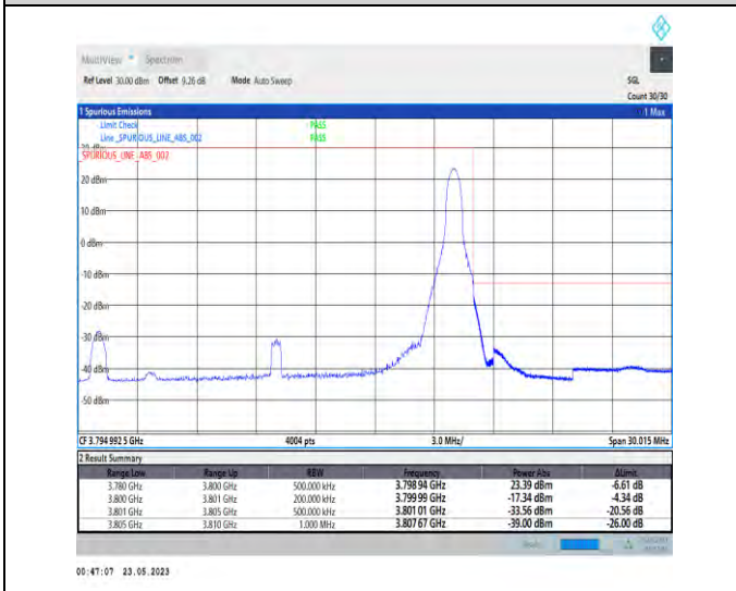
1-N78-3700-3800-PC1-30-20-H-5-CP-QPSK-Edge_1RB_Right-1@50-Ant1-1--PASS-see graph
