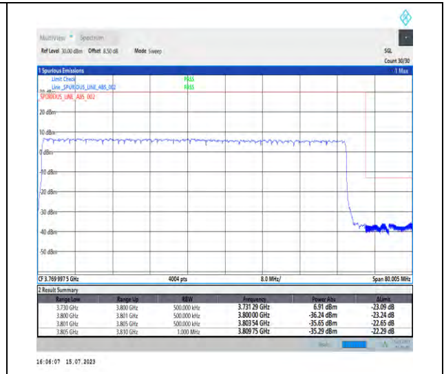
1-N78-3700-3800-PC1-30-70-H-3-DFT-PI2BPSK-Outer_Full-180@0-Ant1-1--PASS-see graph
