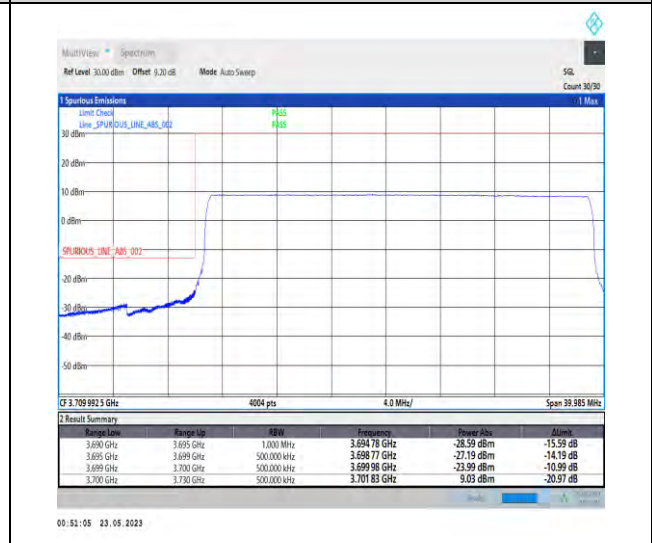
1-N78-3700-3800-PC1-30-30-L-6-CP-QPSK-Outer_Full-78@0-Ant1-1--PASS-see graph
