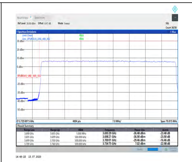
1-N78-3700-3800-PC1-30-60-L-3-DFT-PI2BPSK-Outer_Full-162@0-Ant1-1--PASS-see graph
