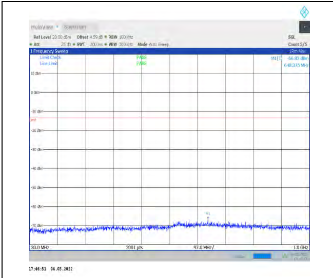
1-N78-3700-3800--30-100-M-1-DFT-PI2BPSK-Inner _1RB_Left-1@1-30-1000-Ant1--66.82--13-PASS
