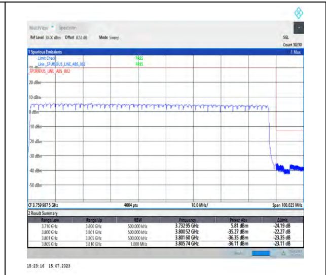
1-N78-3700-3800-PC1-30-90-H-3-DFT-PI2BPSK-Outer_Full-240@0-Ant1-1--PASS-see graph
