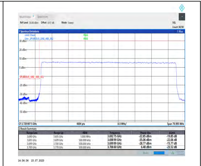
1-N78-3700-3800-PC1-30-70-L-3-DFT-PI2BPSK-Outer_Full-180@0-Ant1-1--PASS-see graph
