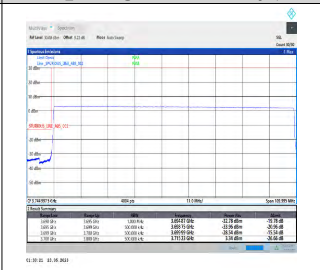
1-N78-3700-3800-PC1-30-100-L-6-CP-QPSK-Outer_Full-273@0-Ant1-1--PASS-see graph
