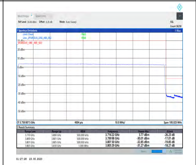
1-N78-3700-3800-PC1-30-90-H-6-CP-QPSK-Outer_Full-245@0-Ant1-1--PASS-see graph
