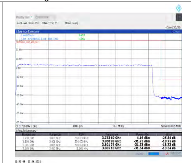
1-N78-3700-3800--30-70-H-3-DFT-PI2BPSK-Outer_Full-180@0-Ant1-PASS-see graph
