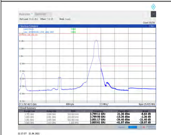
1-N78-3700-3800--30-15-H-5-CP-QPSK-Edge_1RB_R ight-1@37-Ant1-PASS-see graph
