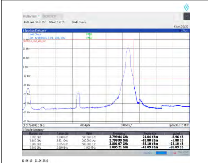
1-N78-3700-3800--30-20-H-5-CP-QPSK-Edge_1RB_R ight-1@50-Ant1-PASS-see graph
