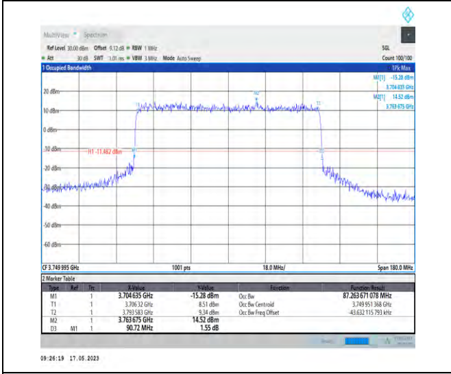
1-N78-3700-3800-PC1-30-90-M-7-CP-16QAM-Outer _Full-245@0-Ant1-87.264-90.720-<90-PASS
