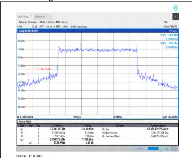
1-N78-3700-3800-PC1-30-70-H-7-CP-16QAM-Outer_Full-189@0-Ant1-67.358-69.580-≤70-PASS
