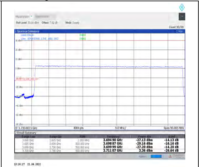
1-N78-3700-3800--30-80-L-3-DFT-PI2BPSK-Outer_Full-216@0-Ant1-PASS-see graph
