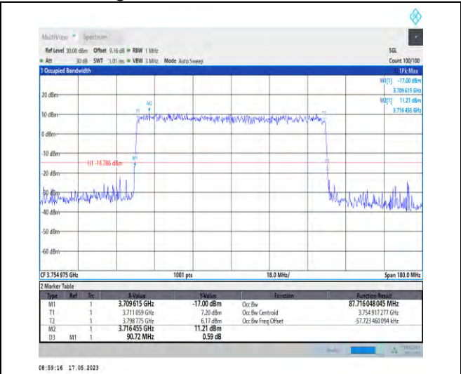
1-N78-3700-3800-PC1-30-90-H-9-CP-256QAM-Outer_Full-245@0-Ant1-87.716-90.720-≤90-PASS
