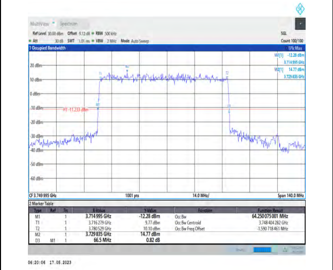
1-N78-3700-3800-PC1-30-70-M-2-DFT-PI2BPSK-Outer_Full-180@0-Ant1-64.25-66.500-≤70-PASS
