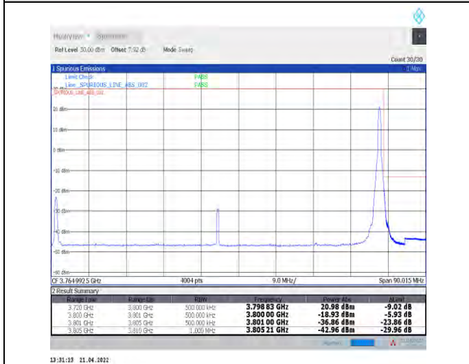
1-N78-3700-3800--30-80-H-5-CP-QPSK-Edge_1RB_R ight-1@216-Ant1-PASS-see graph
