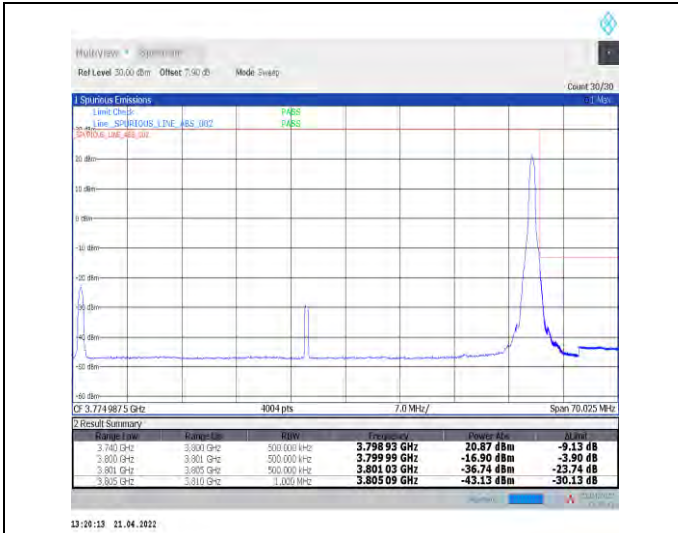
1-N78-3700-3800--30-60-H-2-DFT-PI2BPSK-Edge_1R_B_Right-1@161-Ant1-PASS-see graph
