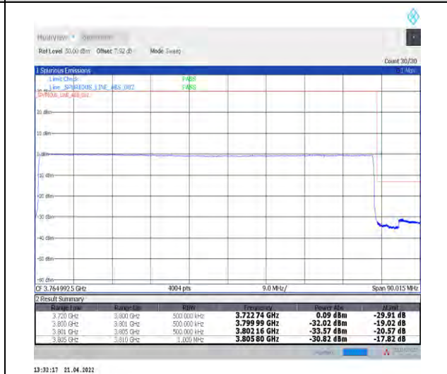
1-N78-3700-3800--30-80-H-6-CP-QPSK-Outer_Fu ll-217@0-Ant1-PASS-see graph
