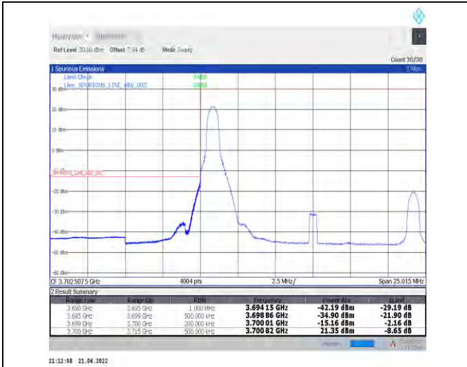
1-N78-3700-3800--30-15-L-1-DFT-PI2BPSK-Edge_1R_B_Left-1@0-Ant1-PASS-see graph
