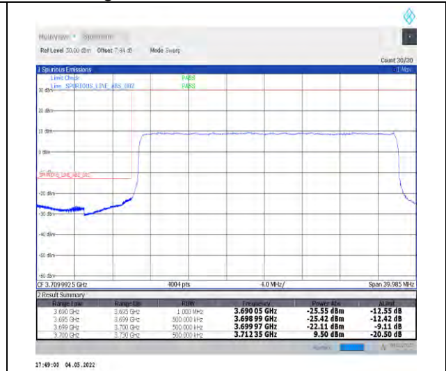
1-N78-3700-3800--30-30-L-3-DFT-PI2BPSK-Outer_Full-75@0-Ant1-PASS-see graph
