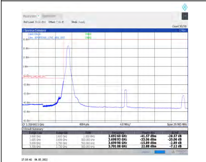
1-N78-3700-3800--30-30-L-4-CP-QPSK-Edge_1RB_L_eff-1@0-Ant1-PASS-see graph
