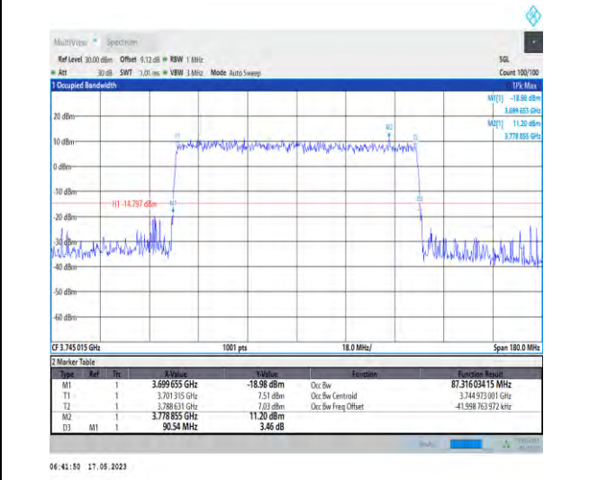
1-N78-3700-3800-PC1-30-90-L-9-CP-256QAM-Outer_Full-245@0-Ant1-87.316-90.540≤90-PASS
