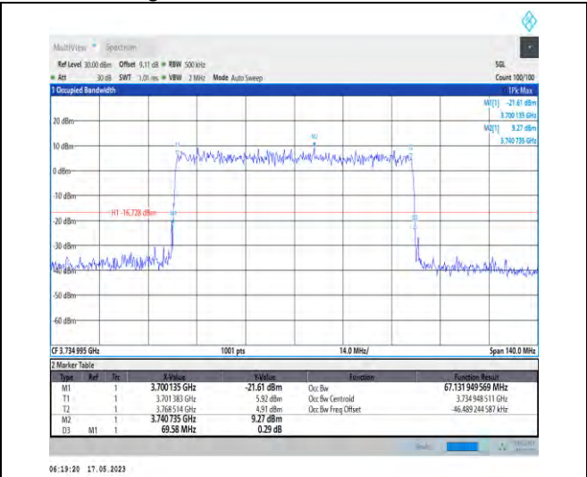
1-N78-3700-3800-PC1-30-70-L-9-CP-256QAM-Outer_Full-189@0-Ant1-67.132-69.580-≤70-PASS
