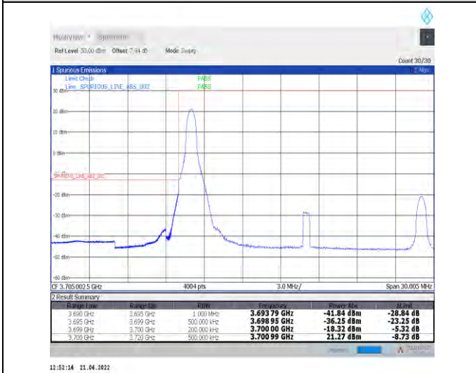
1-N78-3700-3800--30-20-L-4-CP-QPSK-Edge_1RB_L_eff-1@0-Ant1-PASS-see graph
