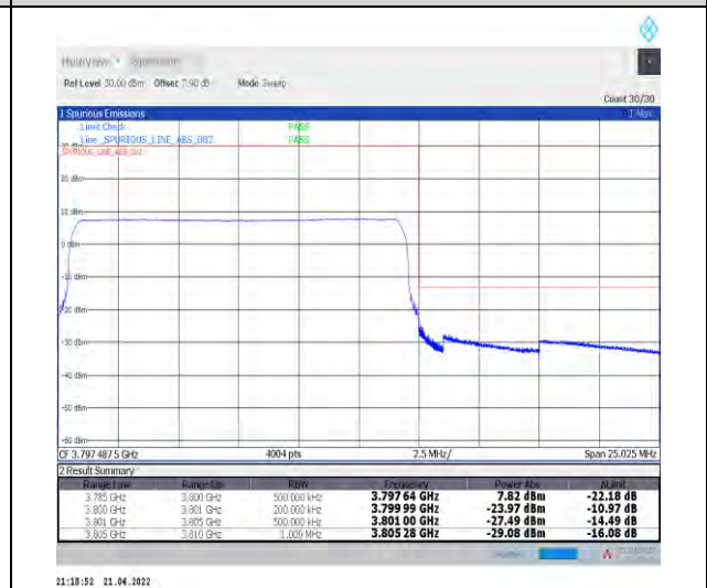
1-N78-3700-3800--30-15-H-6-CP-QPSK-Outer_Fu ll-38@0-Ant1-PASS-see graph
