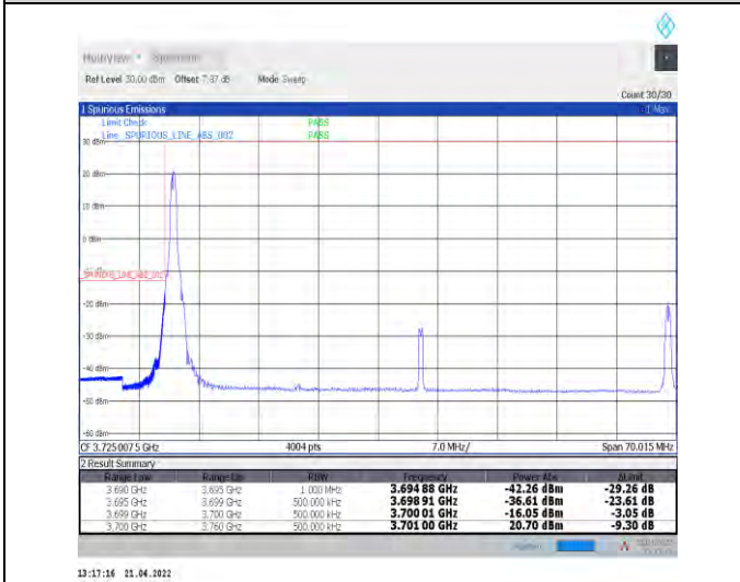
1-N78-3700-3800--30-60-L-4-CP-QPSK-Edge_1RB_L_eff-1@0-Ant1-PASS-see graph
