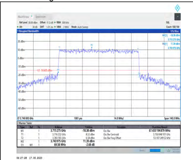
1-N78-3700-3800-PC1-30-70-M-8-CP-64QAM-Outer _Full-189@0-Ant1-67.433-69.580-≤70-PASS
