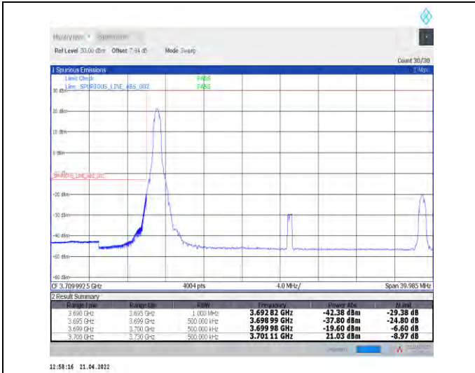
1-N78-3700-3800--30-30-L-1-DFT-PI2BPSK-Edge_1R_B_Left-1@0-Ant1-PASS-see graph
