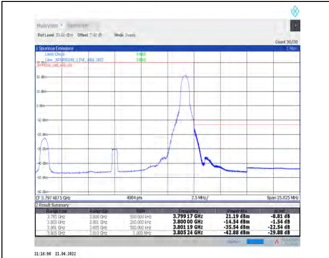
1-N78-3700-3800--30-15-H-2-DFT-PI2BPSK-Edge_1R_B_Right-1@37-Ant1-PASS-see graph
