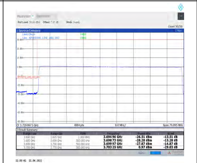
1-N78-3700-3800--30-70-L-6-CP-QPSK-Outer_Ful I-189@0-Ant1-PASS-see graph
