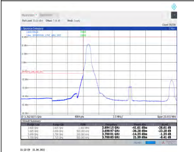
1-N78-3700-3800--30-15-L-4-CP-QPSK-Edge_1RB_L_eff-1@0-Ant1-PASS-see graph
