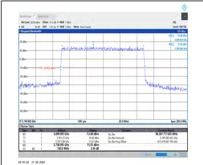
1-N78-3700-3800-PC1-30-100-L-3-DFT-16QAM-Out er_Full-270@0-Ant1-96.308-100.000-≤100-PASS
