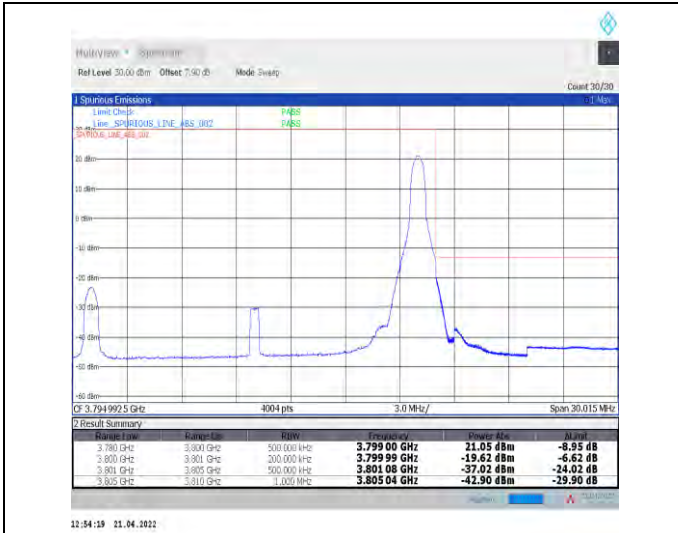
1-N78-3700-3800--30-20-H-2-DFT-PI2BPSK-Edge_1R_B_Right-1@50-Ant1-PASS-see graph
