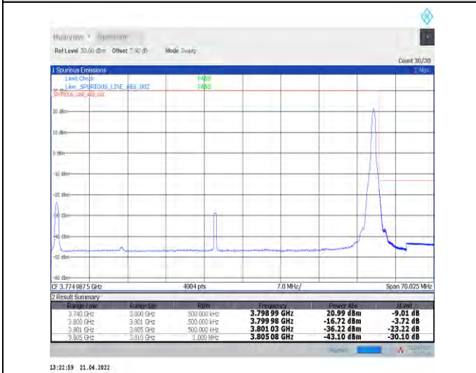
1-N78-3700-3800--30-60-H-5-CP-QPSK-Edge_1RB_R ight-1@161-Ant1-PASS-see graph
