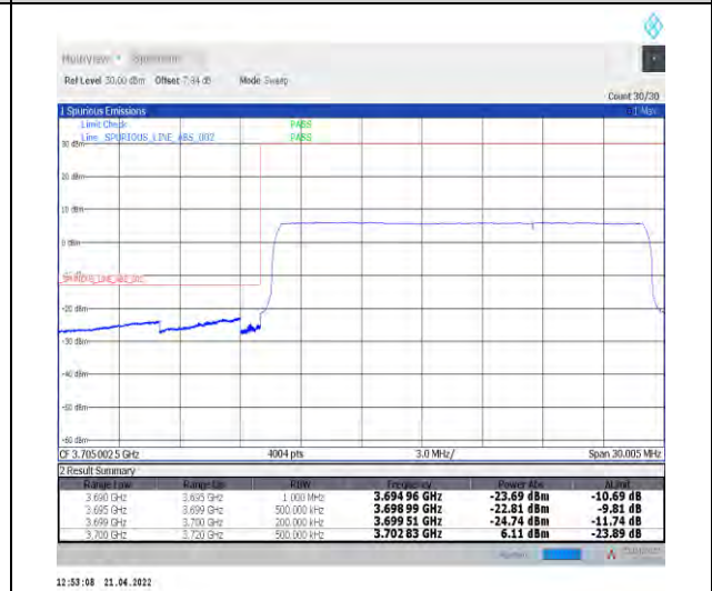
1-N78-3700-3800--30-20-L-6-CP-QPSK-Outer_Ful-I-51@0-Ant1-PASS-see graph
