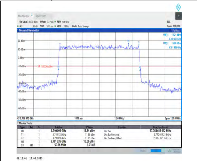
1-N78-3700-3800-PC1-30-60-H-2-DFT-PI2BPSK-Outer_Full-162@0-Ant1-57.764-59.760-≤60-PASS
