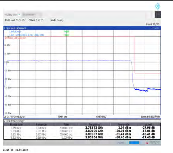
1-N78-3700-3800--30-50-H-6-CP-QPSK-Outer_Fu ll-133@0-Ant1-PASS-see graph
