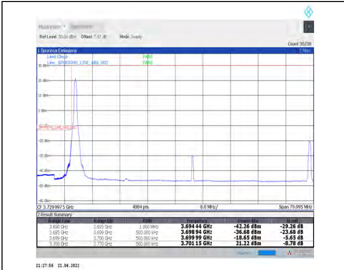
1-N78-3700-3800--30-70-L-1-DFT-PI2BPSK-Edge_1R_B_Left-1@0-Ant1-PASS-see graph
