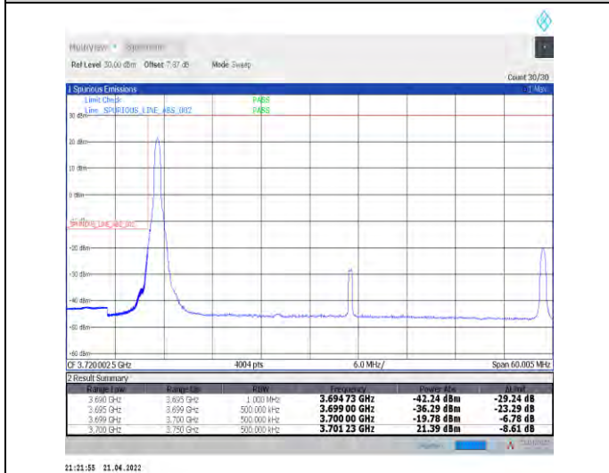
1-N78-3700-3800--30-50-L-4-CP-QPSK-Edge_1RB_L_eff-1@0-Ant1-PASS-see graph
