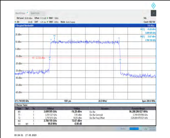
1-N78-3700-3800-PC1-30-100-M-5-DFT-256QAM-Out uter_Full-270@0-Ant1-96.288-99.800-≤100-PASS
