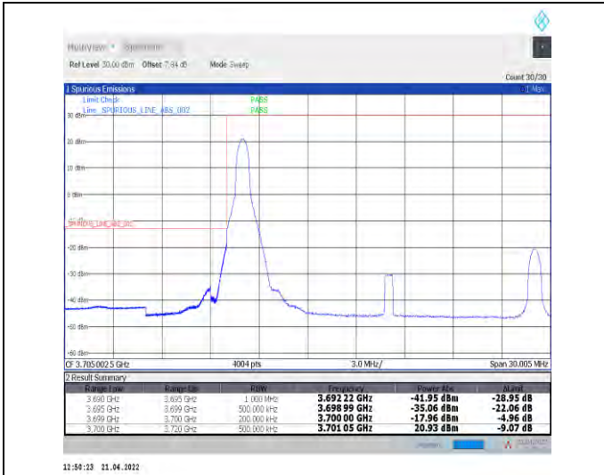
1-N78-3700-3800--30-20-L-1-DFT-PI2BPSK-Edge_1R_B_Left-1@0-Ant1-PASS-see graph
