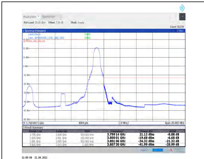
1-N78-3700-3800--30-10-H-2-DFT-PI2BPSK-Edge_1R_B_Right-1@23-Ant1-PASS-see graph
