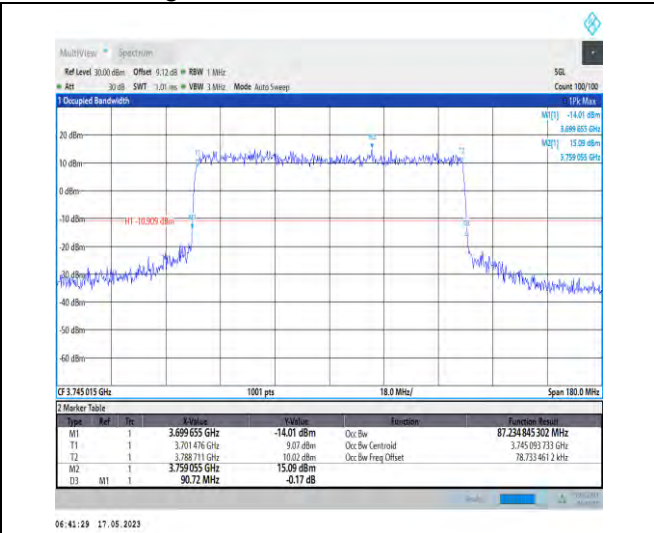
1-N78-3700-3800-PC1-30-90-L-7-CP-16QAM-Outer_Full-245@0-Ant1-87.235-90.720≤90-PASS
