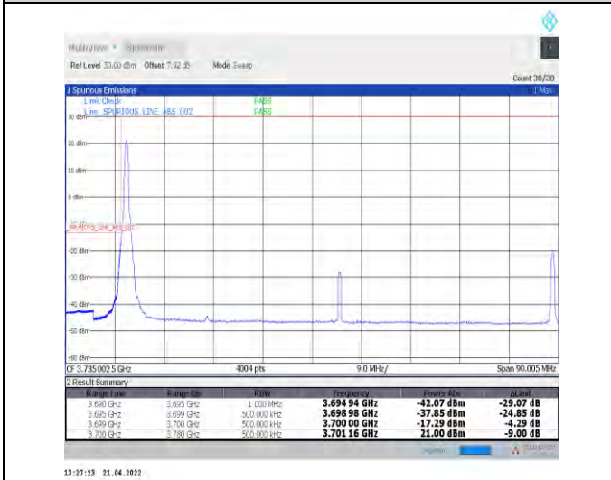
1-N78-3700-3800--30-80-L-4-CP-QPSK-Edge_1RB_L_eff-1@0-Ant1-PASS-see graph
