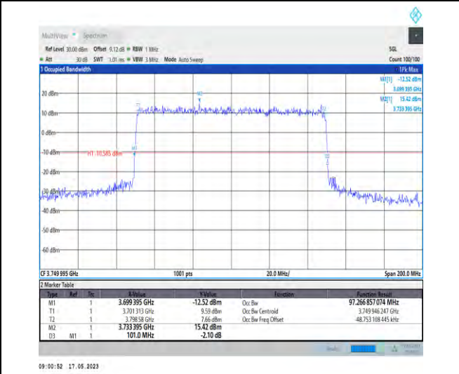
1-N78-3700-3800-PC1-30-100-L-6-CP-QPSK-Outer _Full-273@0-Ant1-97.267-101.000-≤100-PASS
