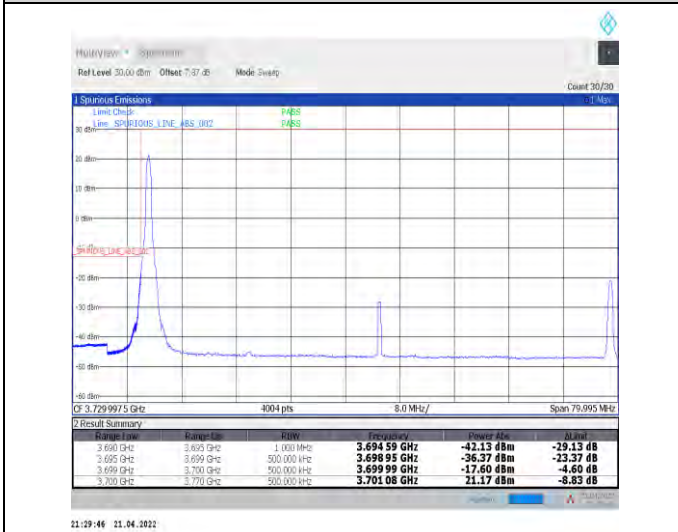
1-N78-3700-3800--30-70-L-4-CP-QPSK-Edge_1RB_L_eff-1@0-Ant1-PASS-see graph
