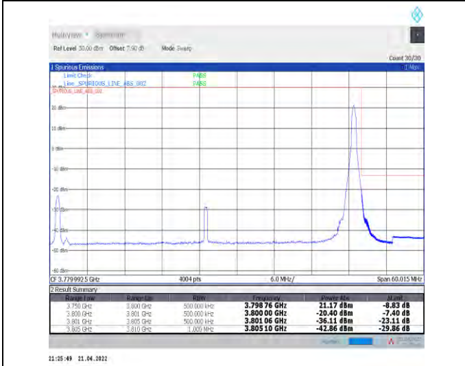
1-N78-3700-3800--30-50-H-5-CP-QPSK-Edge_1RB_R ight-1@132-Ant1-PASS-see graph
