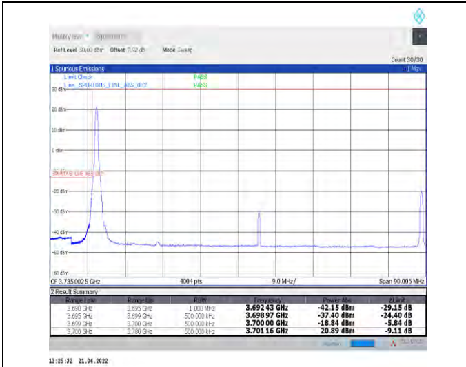
1-N78-3700-3800--30-80-L-1-DFT-PI2BPSK-Edge_1R_B_Left-1@0-Ant1-PASS-see graph
