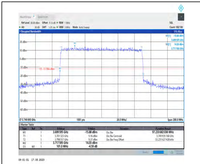
1-N78-3700-3800-PC1-30-100-L-7-CP-16QAM-Outer_Full-273@0-Ant1-97.234-101.000-≤100-PASS
