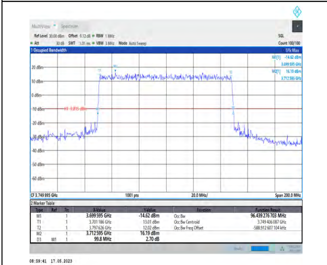
1-N78-3700-3800-PC1-30-100-L-1-DFT-QPSK-Outer_Full-270@0-Ant1-96.439-99.800-≤100-PASS
