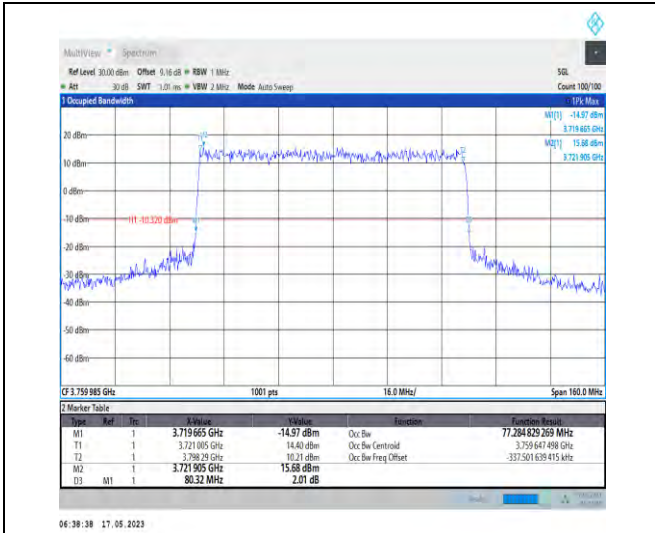
1-N78-3700-3800-PC1-30-80-H-3-DFT-16QAM-Outer_Full-216@0-Ant1-77.285-80.320-≤80-PASS
