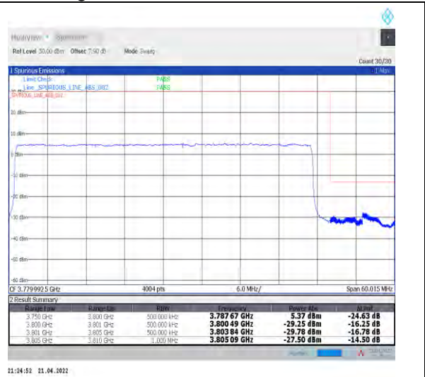
1-N78-3700-3800--30-50-H-3-DFT-PI2BPSK-Outer_Full-128@0-Ant1-PASS-see graph
