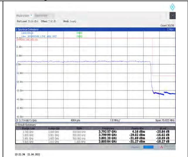
1-N78-3700-3800--30-60-H-3-DFT-PI2BPSK-Outer_Full-162@0-Ant1-PASS-see graph
