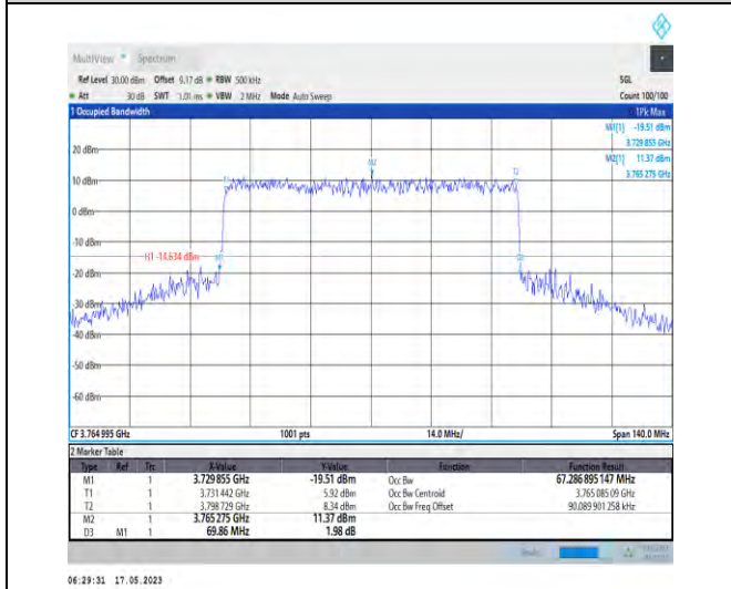
1-N78-3700-3800-PC1-30-70-H-8-CP-64QAM-Outer_Full-189@0-Ant1-67.287-69.860-≤70-PASS
