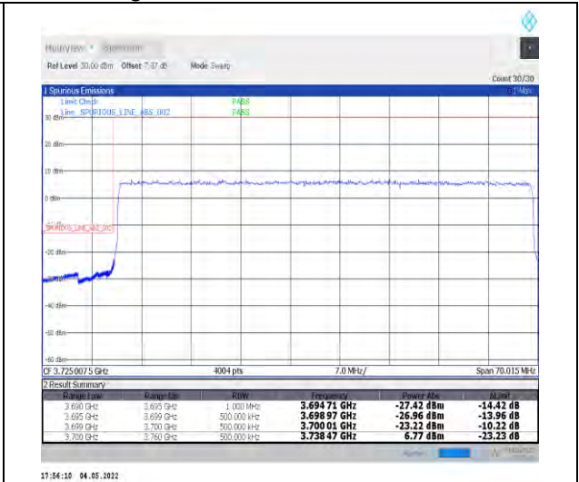
1-N78-3700-3800--30-60-L-3-DFT-PI2BPSK-Outer_Full-162@0-Ant1-PASS-see graph
