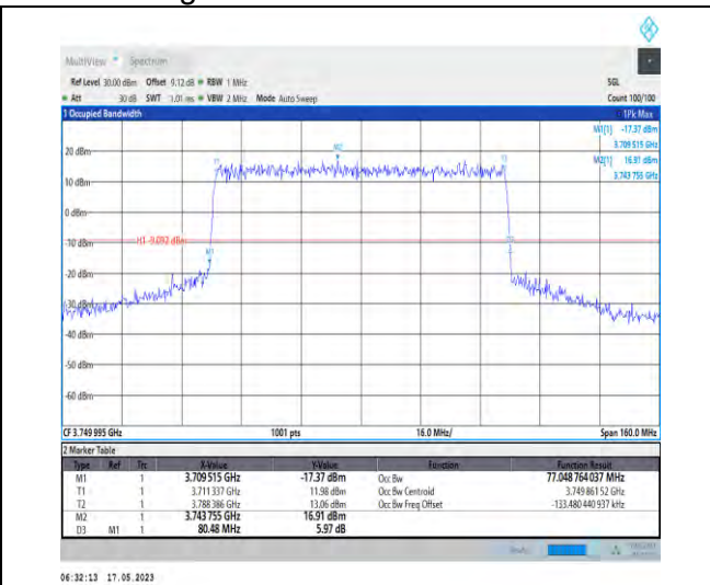
1-N78-3700-3800-PC1-30-80-M-1-DFT-QPSK-Outer_Full-216@0-Ant1-77.049-80.480-≤80-PASS
