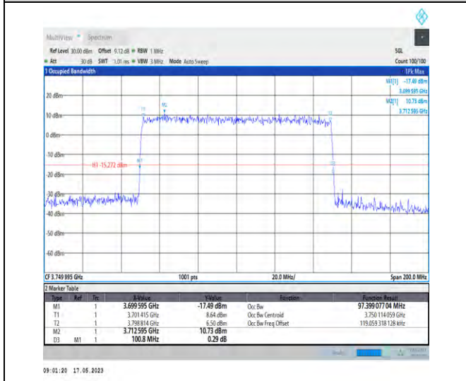
1-N78-3700-3800-PC1-30-100-L-9-CP-256QAM-Outer_Full-273@0-Ant1-97.399-100.800-≤100-PASS
