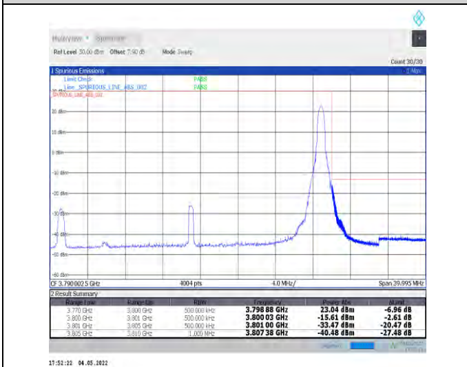
1-N78-3700-3800--30-30-H-5-CP-QPSK-Edge_1RB_R ight-1@77-Ant1-PASS-see graph
