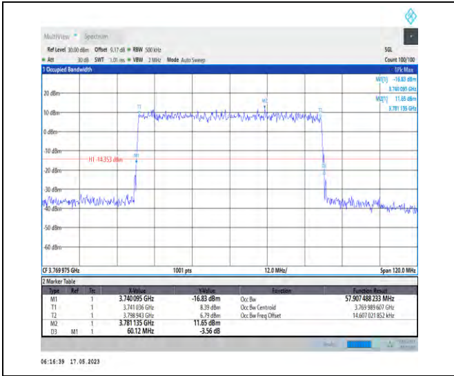
1-N78-3700-3800-PC1-30-60-H-5-DFT-256QAM-Out er_Full-162@0-Ant1-57.907-60.120-≤60-PASS
