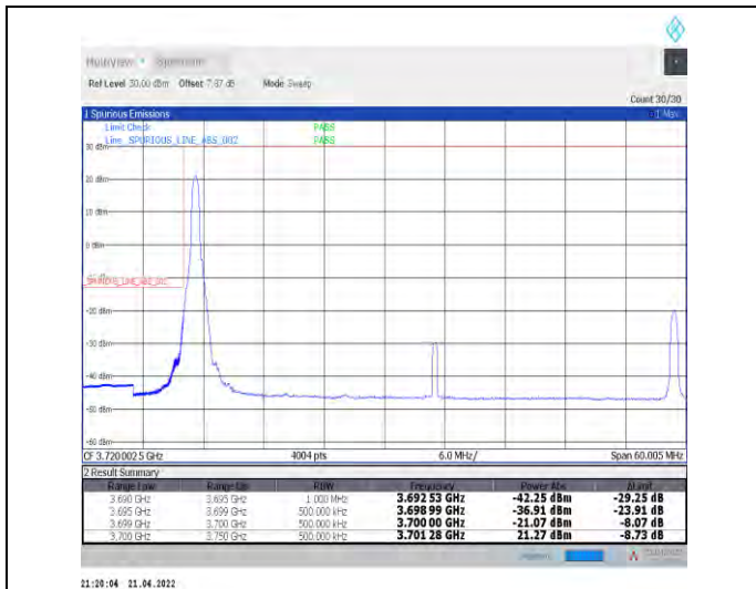
1-N78-3700-3800--30-50-L-1-DFT-PI2BPSK-Edge_1R_B_Left-1@0-Ant1-PASS-see graph
