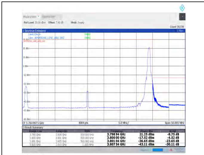
1-N78-3700-3800--30-40-H-2-DFT-PI2BPSK-Edge_1R_B_Right-1@105-Ant1-PASS-see graph
