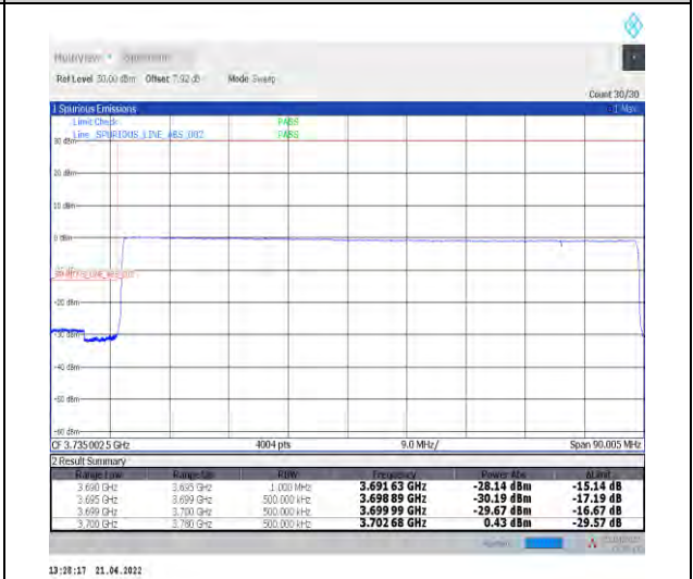
1-N78-3700-3800--30-80-L-6-CP-QPSK-Outer_Ful_I-217@0-Ant1-PASS-see graph
