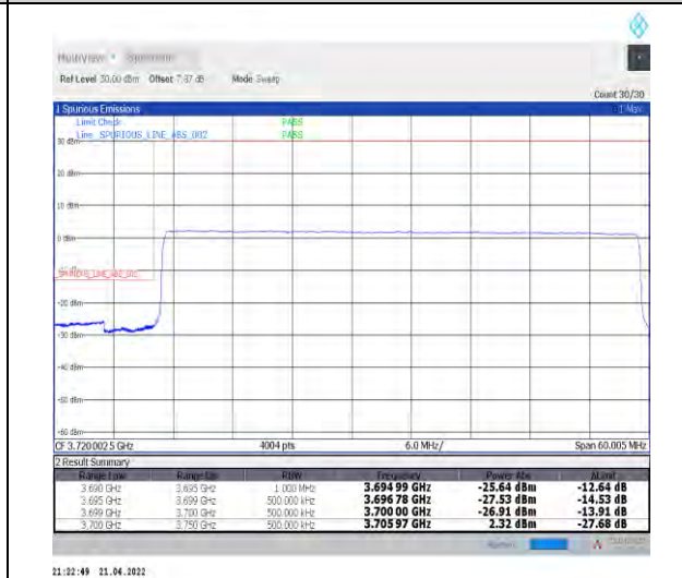
1-N78-3700-3800--30-50-L-6-CP-QPSK-Outer_Ful_I-133@0-Ant1-PASS-see graph
