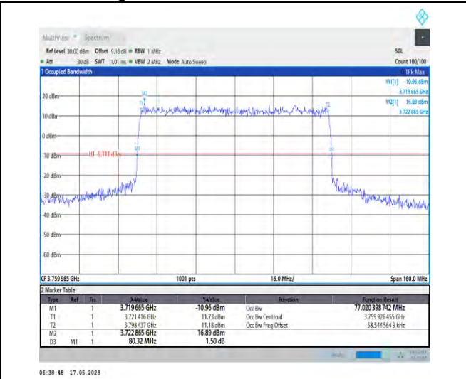
1-N78-3700-3800-PC1-30-80-H-4-DFT-64QAM-Outer_Full-216@0-Ant1-77.02-80.320-≤80-PASS
