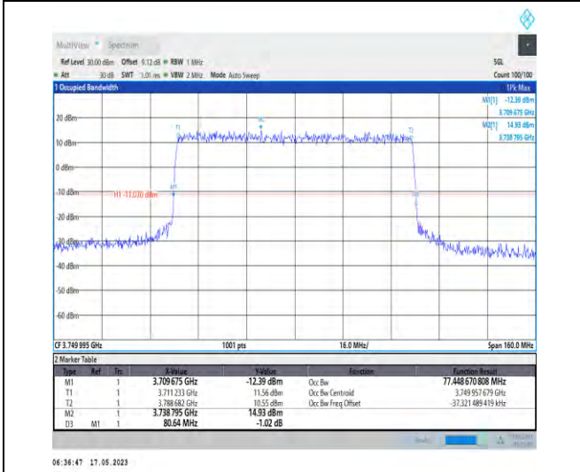
1-N78-3700-3800-PC1-30-80-M-6-CP-QPSK-Outer_Full-217@0-Ant1-77.449-80.640-≤80-PASS
