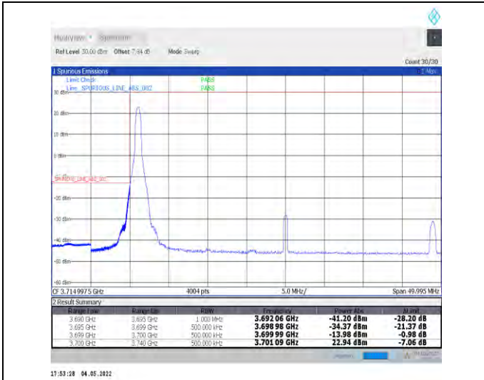
1-N78-3700-3800--30-40-L-1-DFT-PI2BPSK-Edge_1R_B_Left-1@0-Ant1-PASS-see graph
