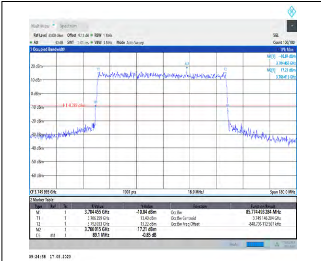
1-N78-3700-3800-PC1-30-90-M-1-DFT-QPSK-Outer_Full-240@0-Ant1-85.774-89.100-≤90-PASS
