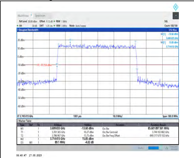
1-N78-3700-3800-PC1-30-90-L-3-DFT-16QAM-Outer_Full-240@0-Ant1-85.602-89.100-<=90-PASS
