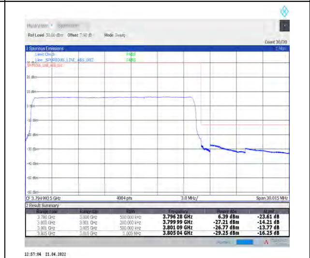
1-N78-3700-3800--30-20-H-6-CP-QPSK-Outer_Fu ll-51@0-Ant1-PASS-see graph
