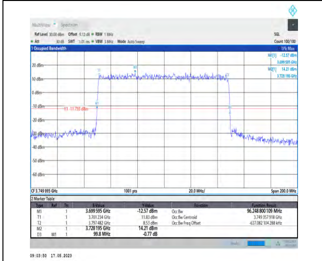
1-N78-3700-3800-PC1-30-100-M-4-DFT-64QAM-Out er_Full-270@0-Ant1-96.249-99.800-≤100-PASS
