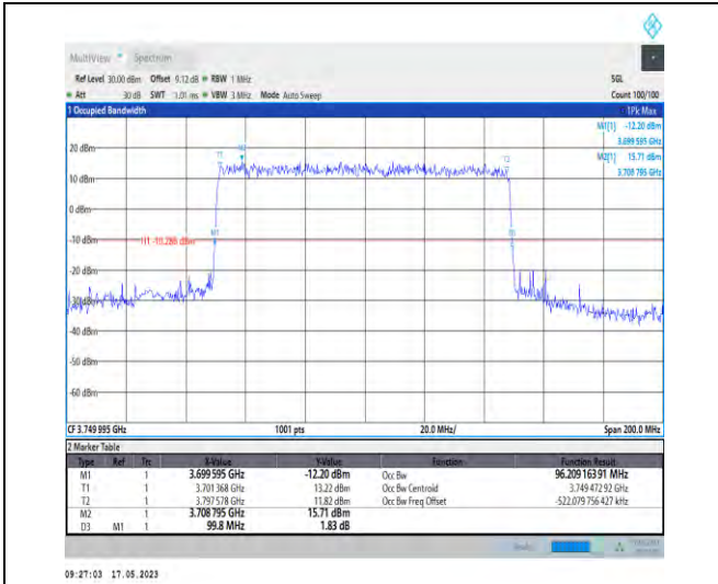
1-N78-3700-3800-PC1-30-100-H-1-DFT-QPSK-Outer_Full-270@0-Ant1-96.209-99.800-≤100-PASS
