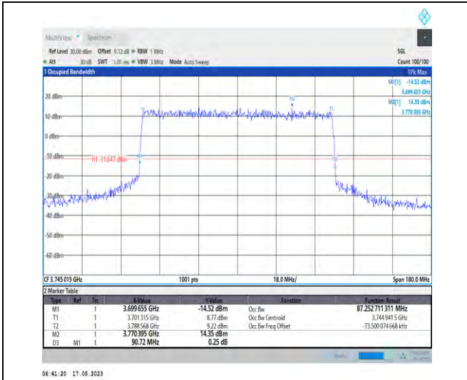
1-N78-3700-3800-PC1-30-90-L-6-CP-QPSK-Outer_Full-245@0-Ant1-87.253-90.720≤90-PASS
