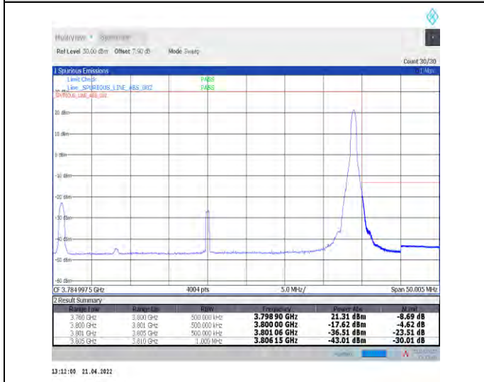
1-N78-3700-3800--30-40-H-5-CP-QPSK-Edge_1RB_Right-1@105-Ant1-PASS-see graph
