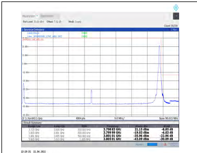
1-N78-3700-3800--30-80-H-2-DFT-PI2BPSK-Edge_1R_B_Right-1@216-Ant1-PASS-see graph
