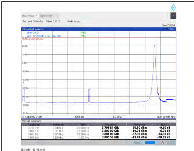
1-N78-3700-3800--30-70-H-2-DFT-PI2BPSK-Edge_1R_B_Right-1@188-Ant1-PASS-see graph
