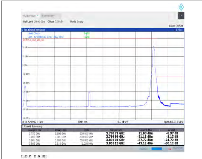
1-N78-3700-3800--30-50-H-2-DFT-PI2BPSK-Edge_1R_B_Right-1@132-Ant1-PASS-see graph
