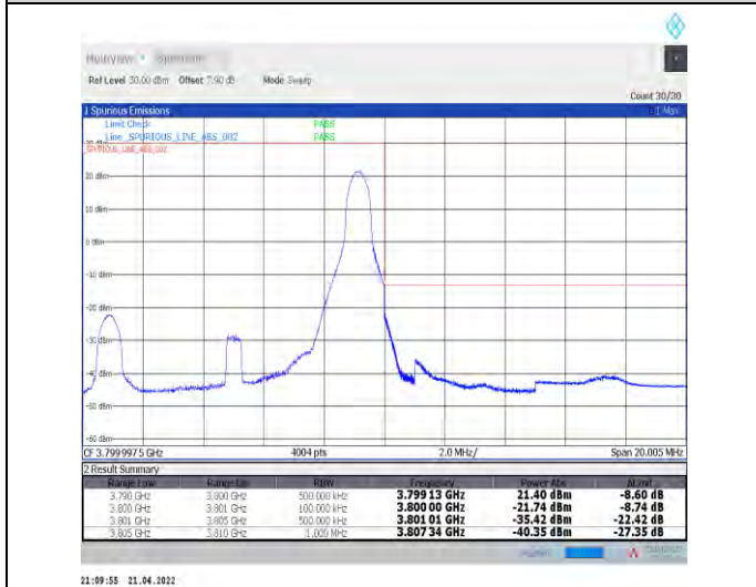
1-N78-3700-3800--30-10-H-5-CP-QPSK-Edge_1RB_R ight-1@23-Ant1-PASS-see graph
