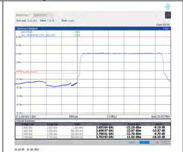
1-N78-3700-3800--30-15-L-3-DFT-PI2BPSK-Outer_Full-36@0-Ant1-PASS-see graph
