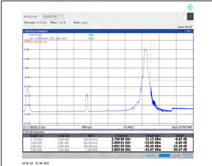
1-N78-3700-3800--30-30-H-2-DFT-PI2BPSK-Edge_1R_B_Right-1@77-Ant1-PASS-see graph
