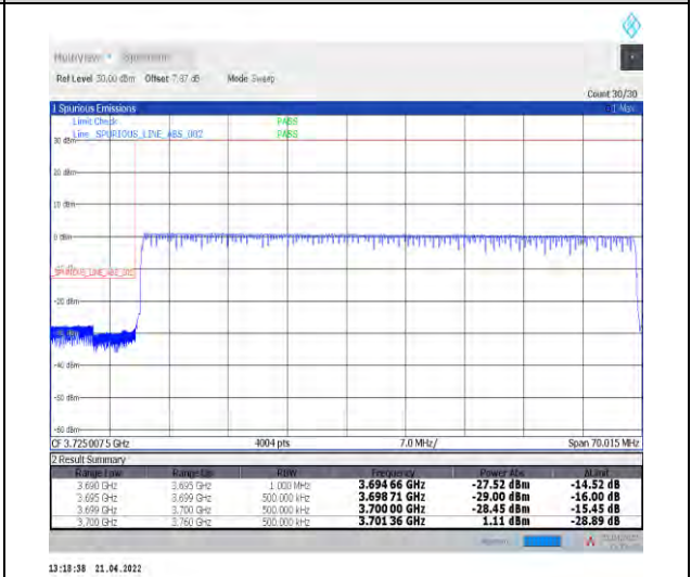
1-N78-3700-3800--30-60-L-6-CP-QPSK-Outer_Ful I-162@0-Ant1-PASS-see graph
