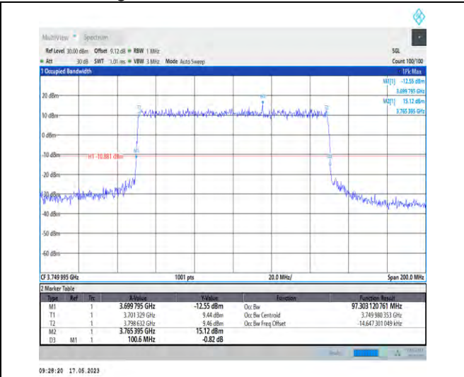
1-N78-3700-3800-PC1-30-100-H-6-CP-QPSK-Outer_Full-273@0-Ant1-97.303-100.600-≤100-PASS
