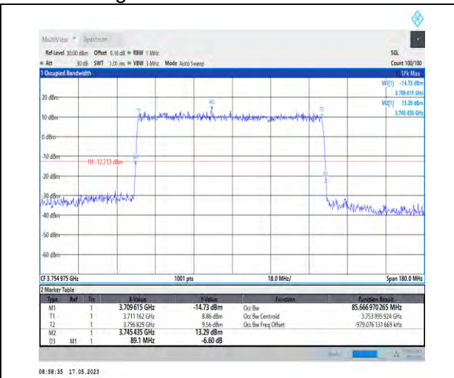
1-N78-3700-3800-PC1-30-90-H-5-DFT-256QAM-Outer_Full-240@0-Ant1-85.667-89.100-≤90-PASS
