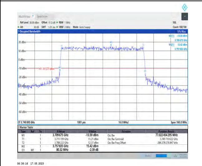
1-N78-3700-3800-PC1-30-80-M-3-DFT-16QAM-Outer_Full-216@0-Ant1-77.022-80.320-≤80-PASS
