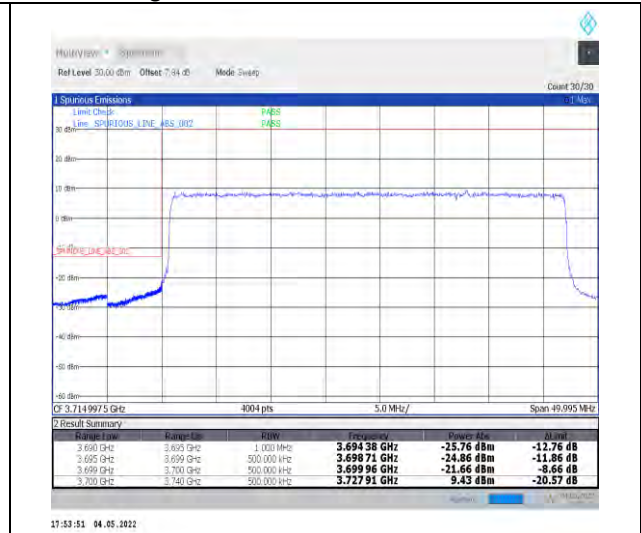
1-N78-3700-3800--30-40-L-3-DFT-PI2BPSK-Outer_Full-100@0-Ant1-PASS-see graph
