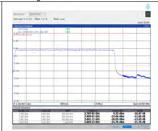
1-N78-3700-3800--30-40-H-3-DFT-PI2BPSK-Outer_Full-100@0-Ant1-PASS-see graph
