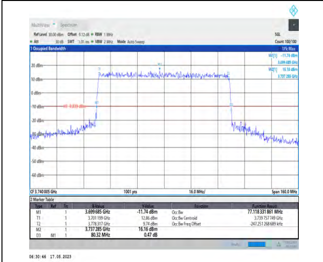
1-N78-3700-3800-PC1-30-80-L-3-DFT-16QAM-Outer_Full-216@0-Ant1-77.118-80.320-≤80-PASS
