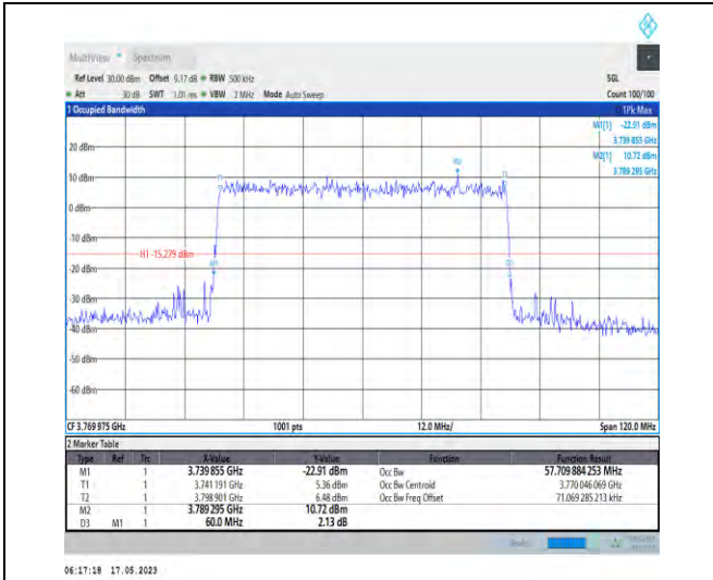
1-N78-3700-3800-PC1-30-60-H-9-CP-256QAM-Outer_Full-162@0-Ant1-57.71-60.000-≤60-PASS
