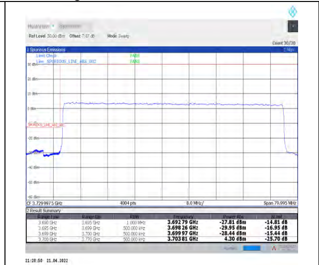
1-N78-3700-3800--30-70-L-3-DFT-PI2BPSK-Outer_Full-180@0-Ant1-PASS-see graph
