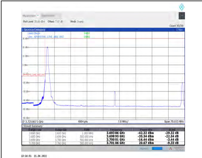
1-N78-3700-3800--30-60-L-1-DFT-PI2BPSK-Edge_1R_B_Left-1@0-Ant1-PASS-see graph
