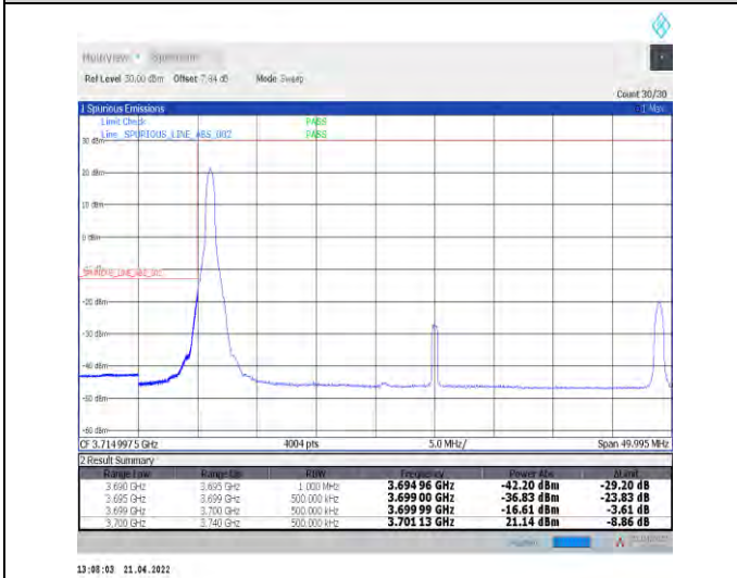
1-N78-3700-3800--30-40-L-4-CP-QPSK-Edge_1RB_L_eff-1@0-Ant1-PASS-see graph
