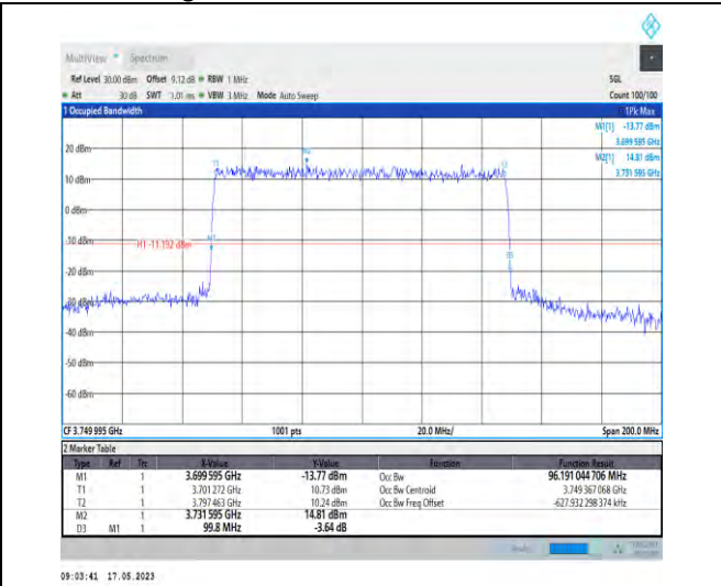
1-N78-3700-3800-PC1-30-100-M-3-DFT-16QAM-Out er_Full-270@0-Ant1-96.191-99.800-≤100-PASS
