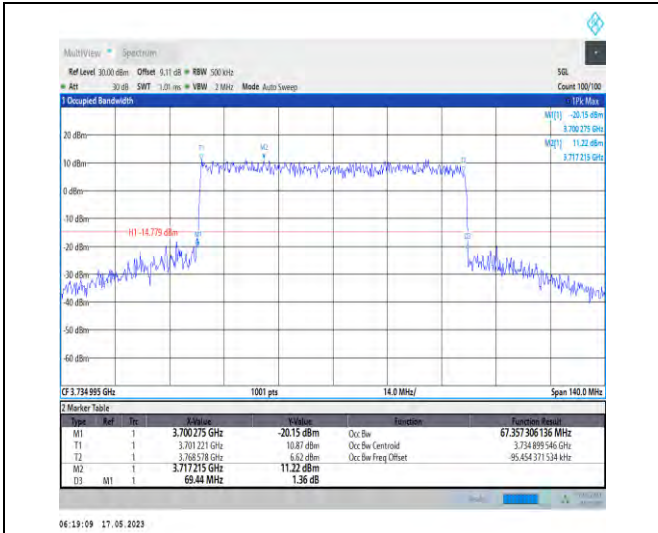
1-N78-3700-3800-PC1-30-70-L-8-CP-64QAM-Outer_Full-189@0-Ant1-67.357-69.440-≤70-PASS
