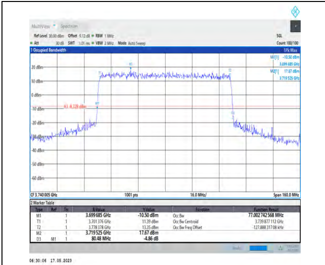
1-N78-3700-3800-PC1-30-80-L-1-DFT-QPSK-Outer_Full-216@0-Ant1-77.003-80.480-≤80-PASS
