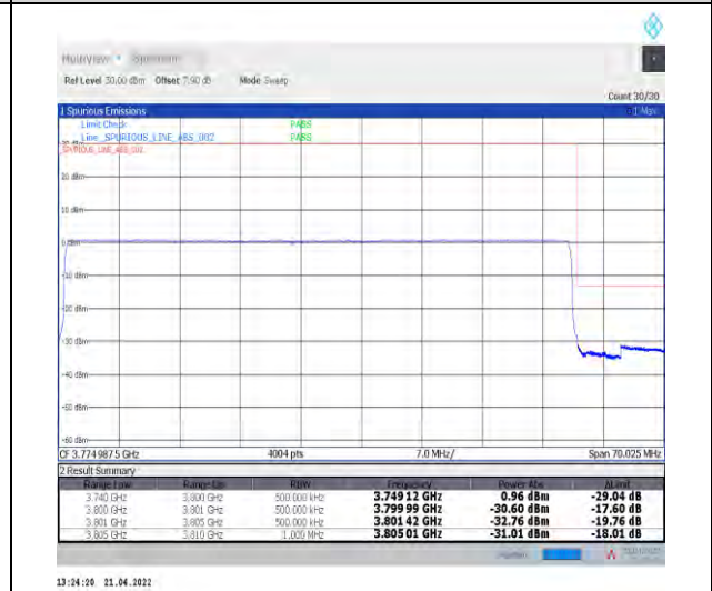
1-N78-3700-3800--30-60-H-6-CP-QPSK-Outer_Fu ll-162@0-Ant1-PASS-see graph
