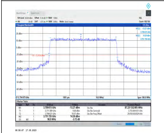
1-N78-3700-3800-PC1-30-90-H-6-CP-QPSK-Outer_Full-245@0-Ant1-87.232-90.900-≤90-PASS
