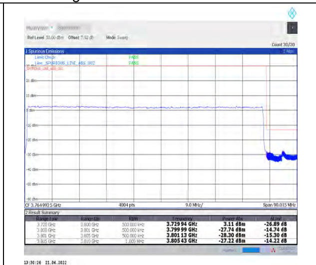
1-N78-3700-3800--30-80-H-3-DFT-PI2BPSK-Outer_Full-216@0-Ant1-PASS-see graph
