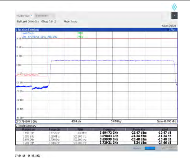
1-N78-3700-3800--30-40-L-6-CP-QPSK-Outer_Ful I-106@0-Ant1-PASS-see graph
