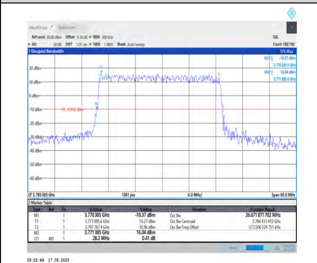
1-N78-3700-3800-PC1-30-30-H-1-DFT-QPSK-Outer _Full-75@0-Ant1-26.672-28.200-≤30-PASS
