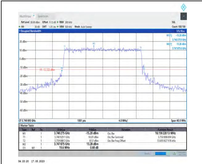
1-N78-3700-3800-PC1-30-20-M-6-CP-QPSK-Outer_Full-51@0-Ant1-18.159-19.600-≤20-PASS
