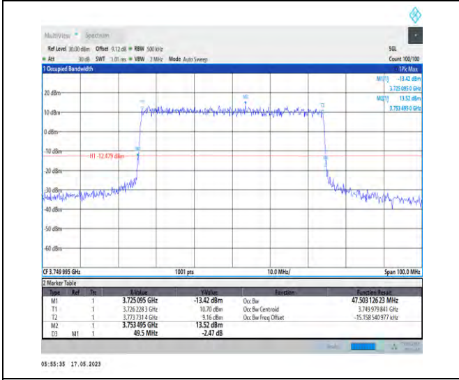
1-N78-3700-3800-PC1-30-50-M-7-CP-16QAM-Outer_Full-133@0-Ant1-47.503-49.500-≤50-PASS
