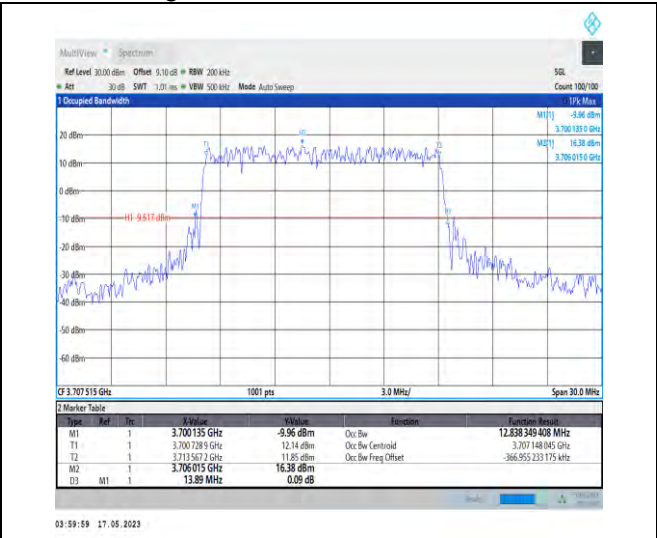
1-N78-3700-3800-PC1-30-15-L-3-DFT-16QAM-Out er_Full-36@0-Ant1-12.838-13.890-≤15-PASS
