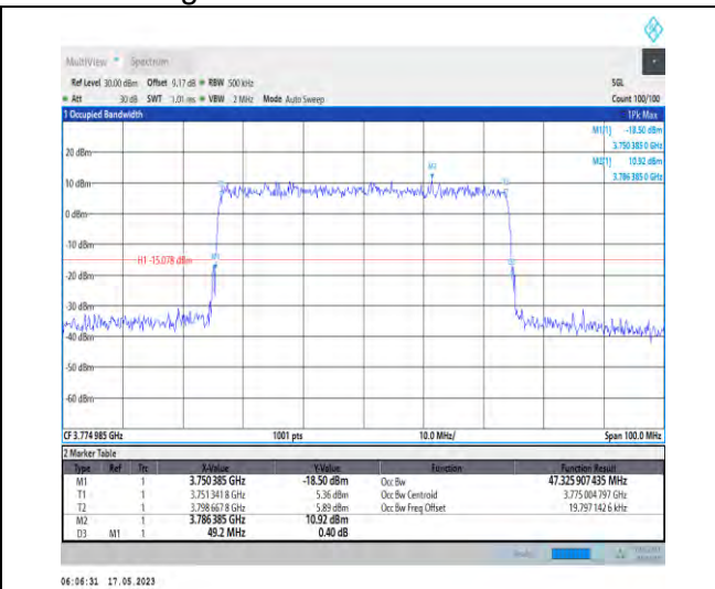
1-N78-3700-3800-PC1-30-50-H-9-CP-256QAM-Outer_Full-133@0-Ant1-47.326-49.200-≤50-PASS
