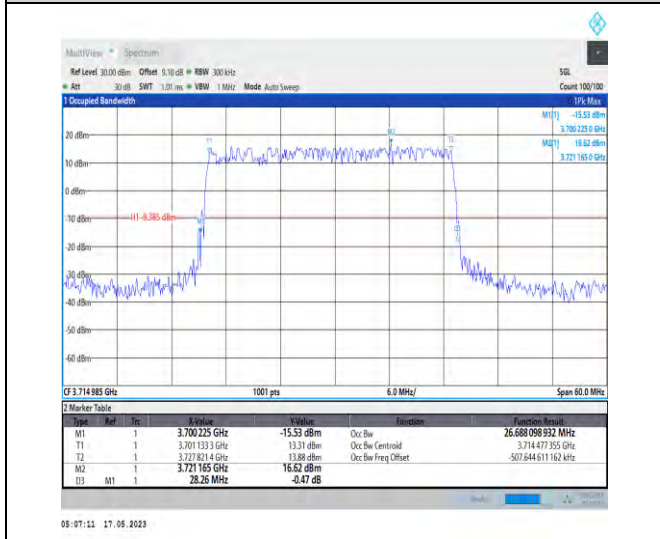
1-N78-3700-3800-PC1-30-30-L-2-DFT-PI2BPSK-Outer_Full-75@0-Ant1-26.688-28.260-≤30-PASS
