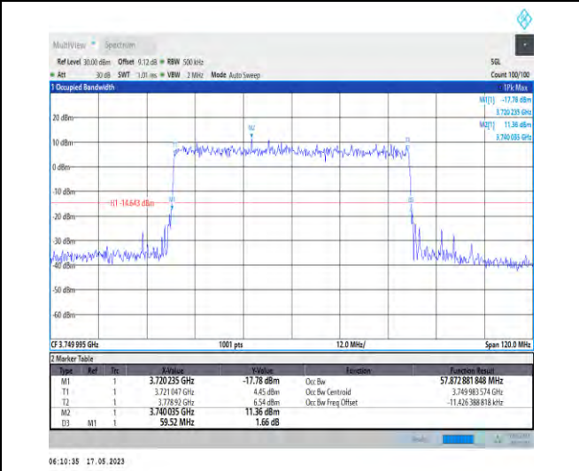
1-N78-3700-3800-PC1-30-60-M-9-CP-256QAM-Outer_Full-162@0-Ant1-57.873-59.520-≤60-PASS
