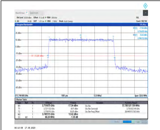
1-N78-3700-3800-PC1-30-60-M-6-CP-QPSK-Outer_Full-162@0-Ant1-57.784-60.240-≤60-PASS
