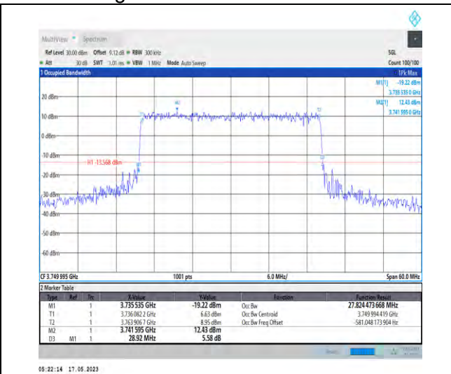
1-N78-3700-3800-PC1-30-30-M-8-CP-64QAM-Outer _Full-78@0-Ant1-27.824-28.920-≤30-PASS
