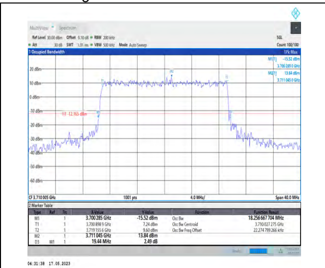
1-N78-3700-3800-PC1-30-20-L-8-CP-64QAM-Outer_Full-51@0-Ant1-18.257-19.440-≤20-PASS
