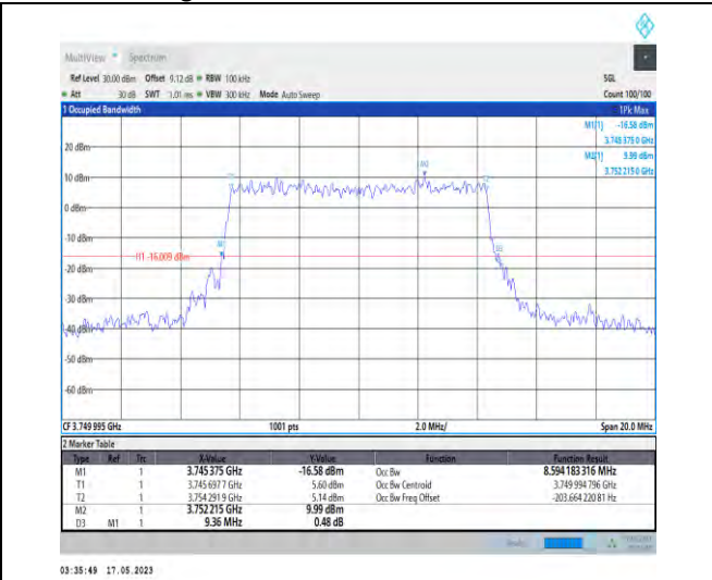
1-N78-3700-3800-PC1-30-10-M-9-CP-256QAM-Outer_Full-24@0-Ant1-8.594-9.360-≤10-PASS
