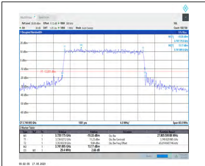
1-N78-3700-3800-PC1-30-30-M-7-CP-16QAM-Outer _Full-78@0-Ant1-27.806-29.400-≤30-PASS
