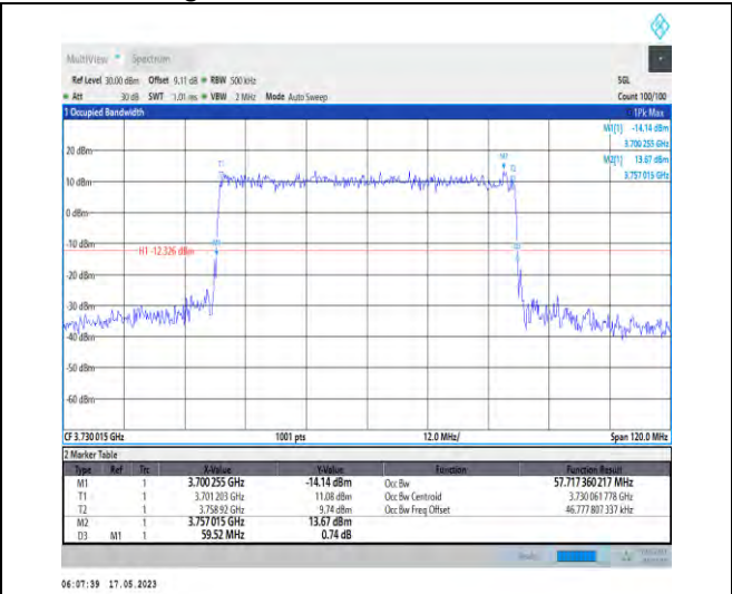
1-N78-3700-3800-PC1-30-60-L-4-DFT-64QAM-Outer_Full-162@0-Ant1-57.717-59.520-≤60-PASS
