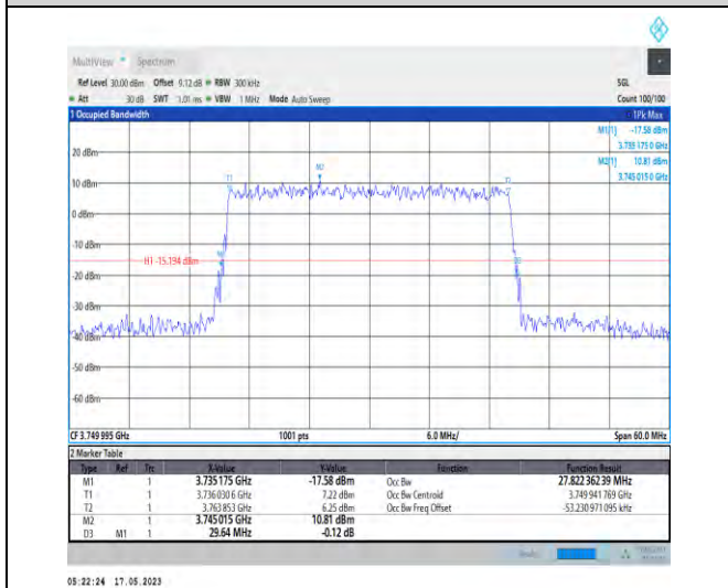
1-N78-3700-3800-PC1-30-30-M-9-CP-256QAM-Outer _Full-78@0-Ant1-27.822-29.640-≤30-PASS
