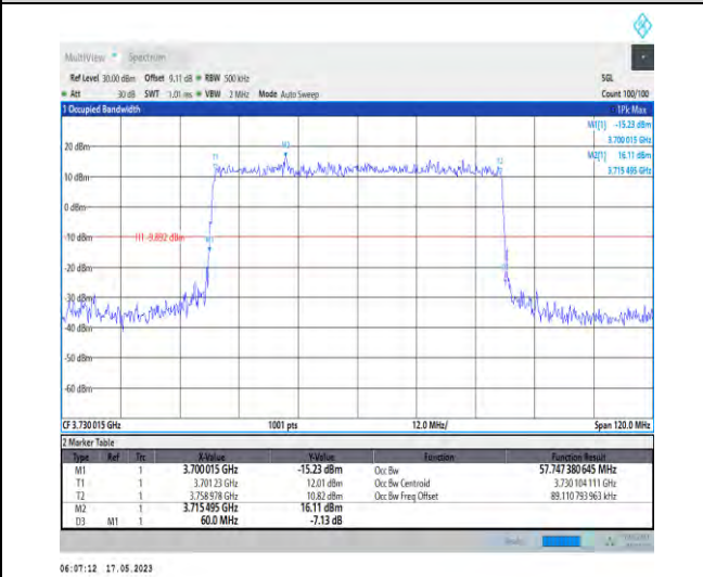
1-N78-3700-3800-PC1-30-60-L-2-DFT-PI2BPSK-Outer_Full-162@0-Ant1-57.747-60.000-≤60-PASS
