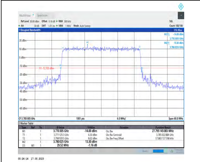
1-N78-3700-3800-PC1-30-30-H-8-CP-64QAM-Outer_Full-78@0-Ant1-27.795-29.520-≤30-PASS
