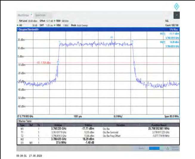
1-N78-3700-3800-PC1-30-40-H-2-DFT-PI2BPSK-Outer_Full-100@0-Ant1-35.799-37.600-≤40-PASS
