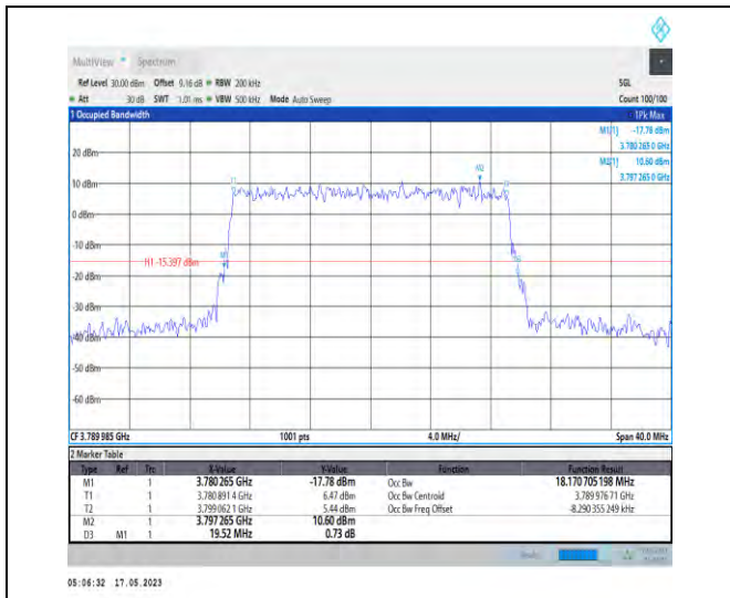
1-N78-3700-3800-PC1-30-20-H-9-CP-256QAM-Oute_r_Full-51@0-Ant1-18.171-19.520-≤20-PASS
