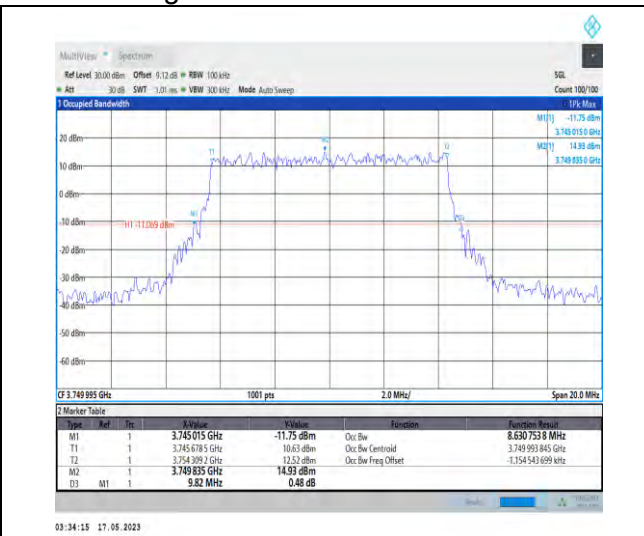
1-N78-3700-3800-PC1-30-10-M-1-DFT-QPSK-Outer_Full-24@0-Ant1-8.631-9.820-≤10-PASS
