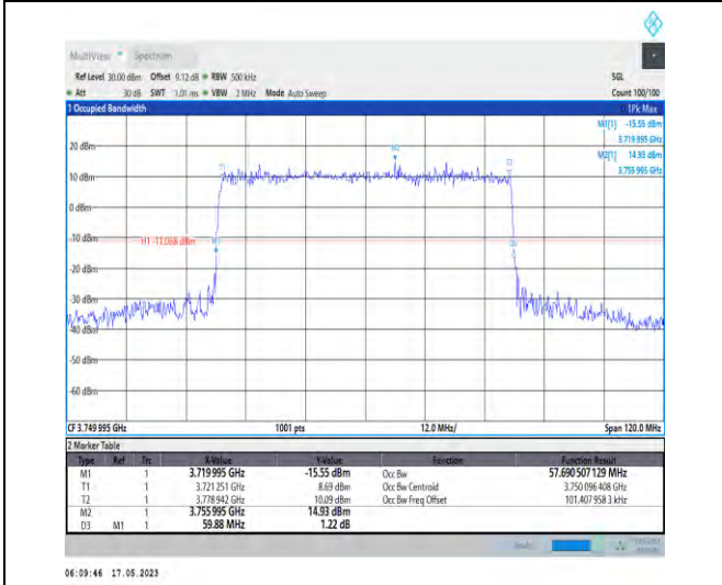
1-N78-3700-3800-PC1-30-60-M-4-DFT-64QAM-Outer_r_Full-162@0-Ant1-57.691-59.880-≤60-PASS
