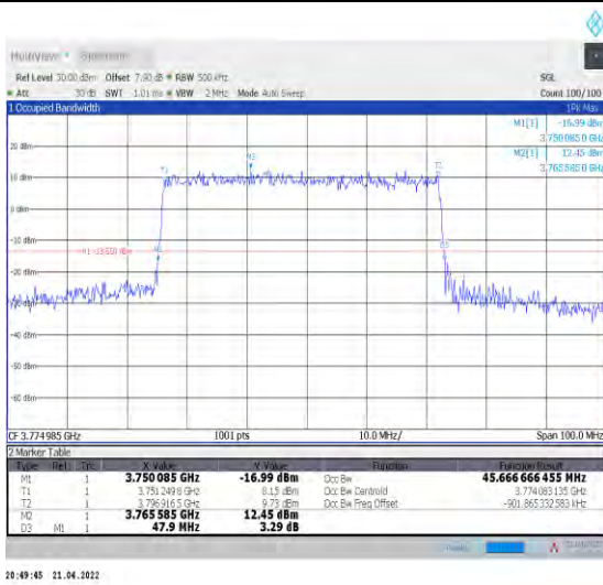
1-N78-3700-3800--30-50-H-4-DFT-64QAM-Outer_Fu II-128@0-Ant1-45.667-47.900-≤50-PASS
