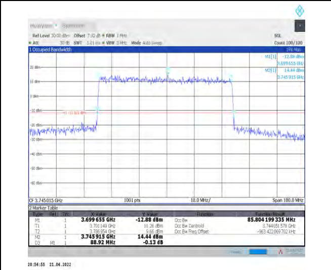
1-N78-3700-3800--30-90-L-1-DFT-QPSK-Outer_Full- 240@0-Ant1-85.804-88.920-≤90-PASS
