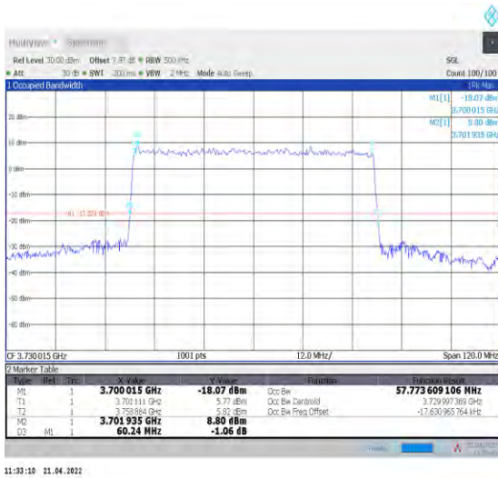
1-N78-3700-3800--30-60-L-9-CP-256QAM-Outer_Fu II-162@0-Ant1-57.774-60.240-≤60-PASS
