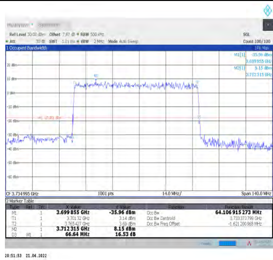
1-N78-3700-3800--30-70-L-5-DFT-256QAM-Outer_Full ull-180@0-Ant1-64.107-66.640-≤70-PASS
