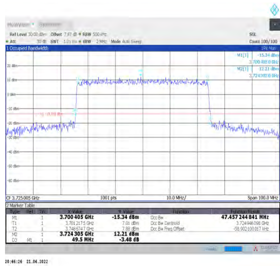
1-N78-3700-3800--30-50-L-7-CP-16QAM-Outer_Full -133@0-Ant1-47.457-49.500-≤50-PASS
