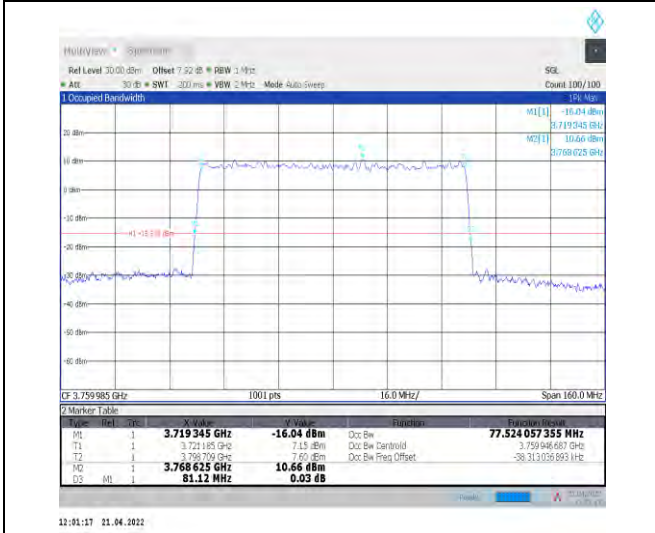
1-N78-3700-3800--30-80-H-9-CP-256QAM-Outer_Fu ll-217@0-Ant1-77.524-81.120-≤80-PASS
