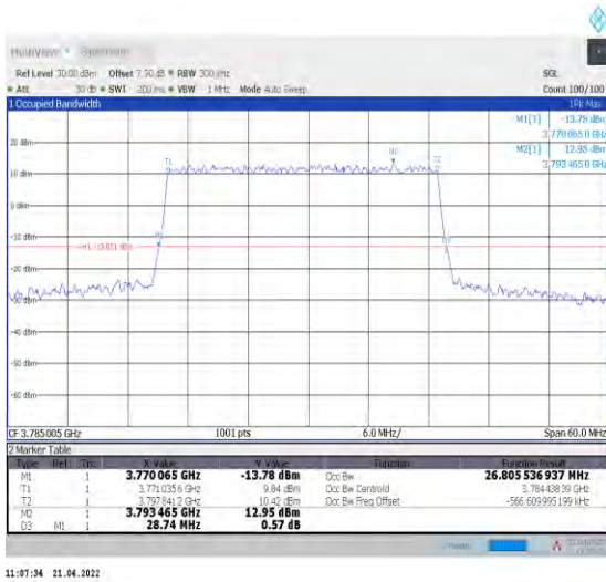
1-N78-3700-3800--30-30-H-4-DFT-64QAM-Outer_Fu II-75@0-Ant1-26.806-28.740-<math>\leq 30</math>-PASS
