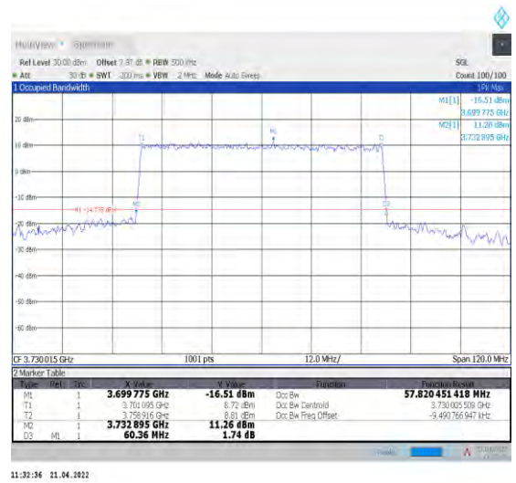
1-N78-3700-3800--30-60-L-8-CP-64QAM-Outer_Full -162@0-Ant1-57.82-60.360-≤60-PASS
