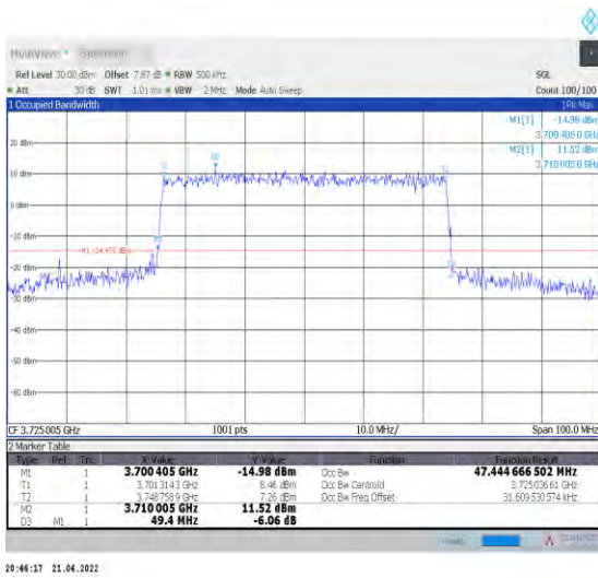
1-N78-3700-3800--30-50-L-6-CP-QPSK-Outer_Full-1 33@0-Ant1-47.445-49.400-≤50-PASS
