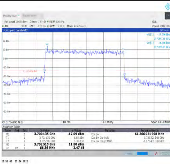
1-N78-3700-3800--30-70-L-4-DFT-64QAM-Outer_Full I-180@0-Ant1-64.366-66.360-≤70-PASS
