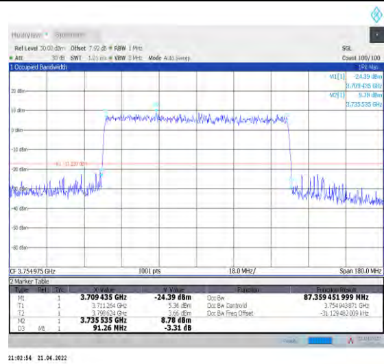
1-N78-3700-3800--30-90-H-9-CP-256QAM-Outer_F ull-245@0-Ant1-87.359-91.260-<=90-PASS
