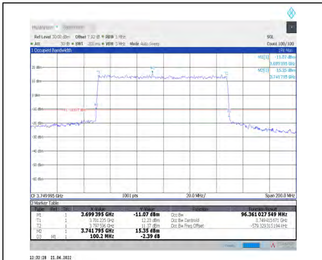
1-N78-3700-3800--30-100-H-1-DFT-QPSK-Outer_Fu II-270@0-Ant1-96.361-100.200-≤100-PASS
