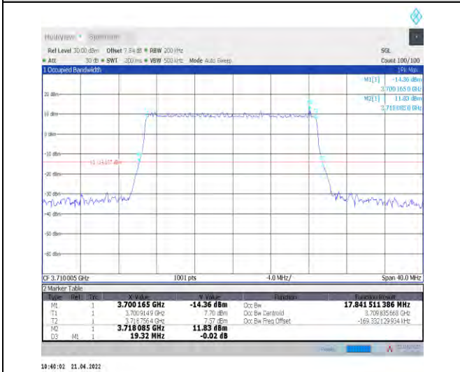
1-N78-3700-3800--30-20-L-5-DFT-256QAM-Outer_Full-50@0-Ant1-17.842-19.320-<=20-PASS
