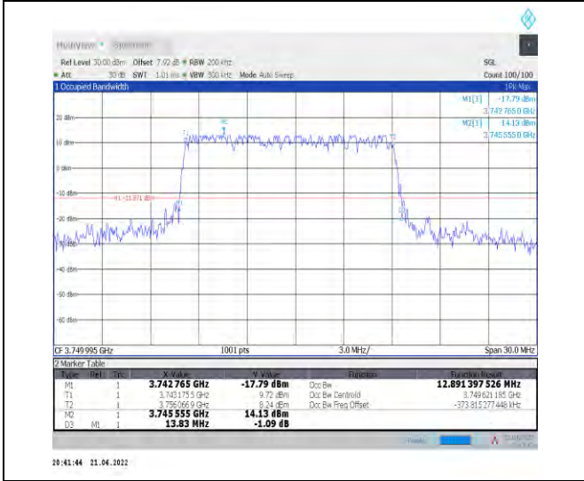
1-N78-3700-3800--30-15-M-3-DFT-16QAM-Outer_Full ull-36@0-Ant1-12.891-13.830-≤15-PASS
