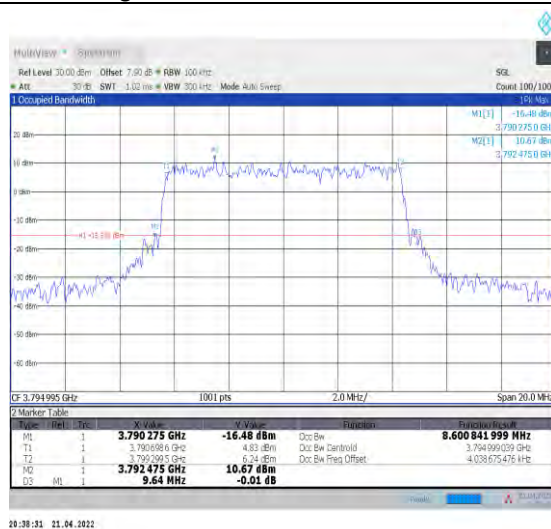
1-N78-3700-3800--30-10-H-8-CP-64QAM-Outer_Full -24@0-Ant1-8.601-9.640-≤10-PASS
