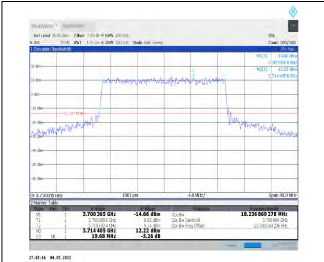
1-N78-3700-3800--30-20-L-7-CP-16QAM-Outer_Full -51@0-Ant1-18.237-19.680-<=20-PASS
