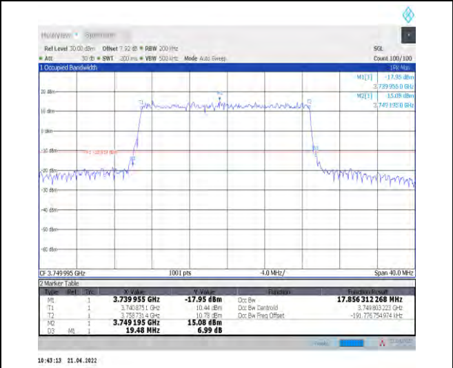
1-N78-3700-3800--30-20-M-1-DFT-QPSK-Outer_Full -50@0-Ant1-17.856-19.480-<=20-PASS
