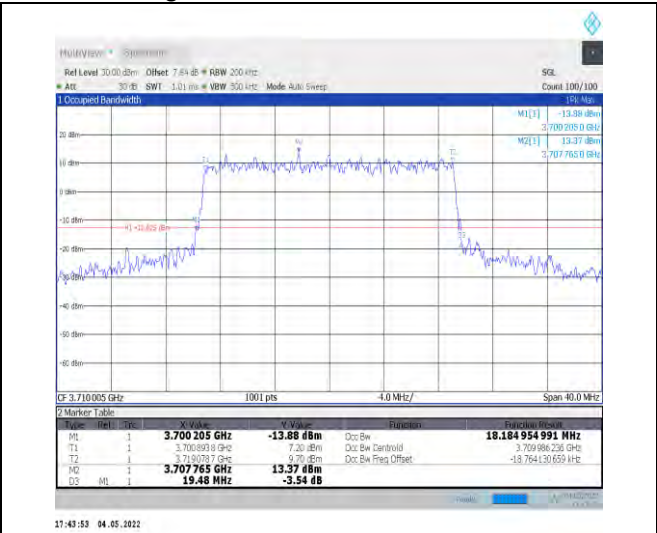
1-N78-3700-3800--30-20-L-8-CP-64QAM-Outer_Full -51@0-Ant1-18.185-19.480-<=20-PASS
