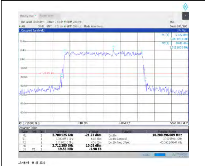
1-N78-3700-3800--30-20-L-9-CP-256QAM-Outer_Fu II-51@0-Ant1-18.208-19.560-<=20-PASS
