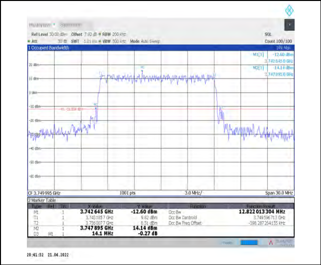
1-N78-3700-3800--30-15-M-4-DFT-64QAM-Outer_Full ull-36@0-Ant1-12.822-14.100-≤15-PASS
