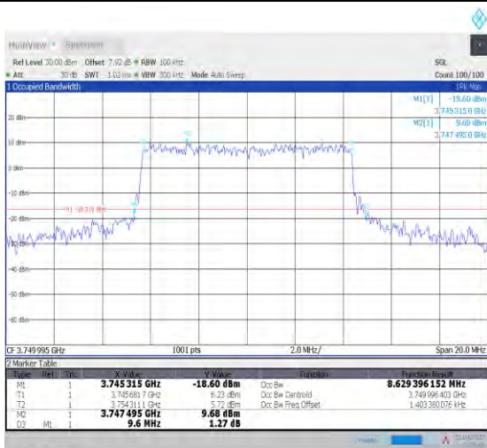
1-N78-3700-3800--30-10-M-4-DFT-64QAM-Outer_Full-24@0-Ant1-8.563-9.660-≤10-PASS
