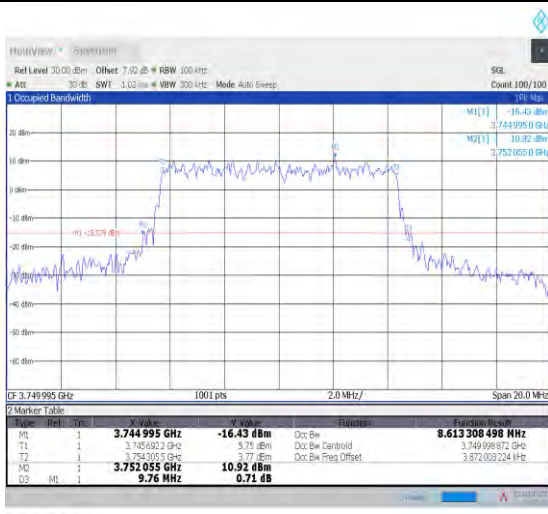
1-N78-3700-3800--30-10-M-8-CP-64QAM-Outer_Full -24@0-Ant1-8.613-9.760-≤10-PASS
