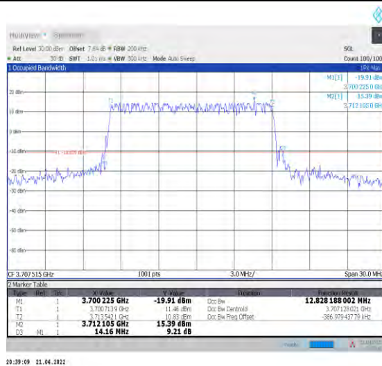
1-N78-3700-3800--30-15-L-1-DFT-QPSK-Outer_Full- 36@0-Ant1-12.828-14.160-≤15-PASS
