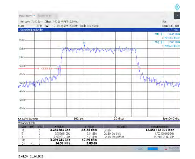
1-N78-3700-3800--30-15-H-8-CP-64QAM-Outer_Full -38@0-Ant1-13.551-14.970-≤15-PASS
