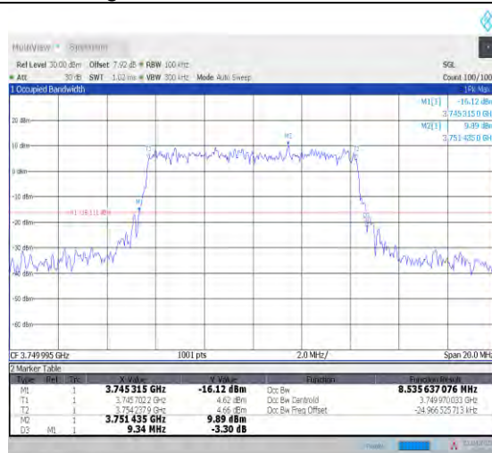
1-N78-3700-3800--30-10-M-5-DFT-256QAM-Outer_Full-24@0-Ant1-8.536-9.340-≤10-PASS
