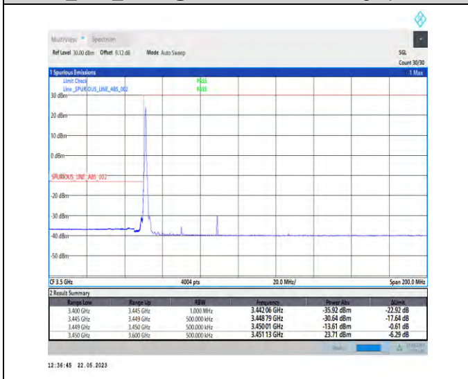
1-N78-3450-3550-PC1-30-40-L-4-CP-QPSK-Edge_1RB_Left-1@0-Ant1-1--PASS-see graph
