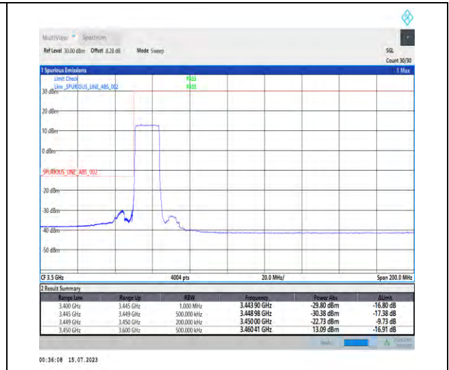
1-N78-3450-3550-PC1-30-15-L-3-DFT-PI2BPSK-Outer_Full-36@0-Ant1-1--PASS-see graph
