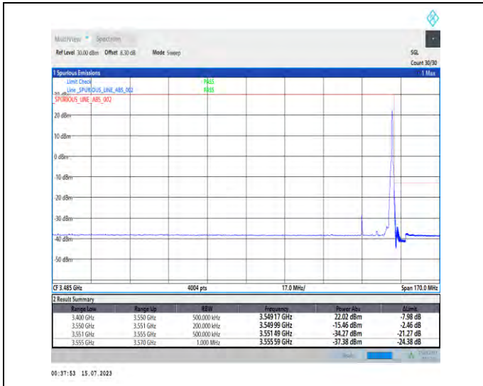
1-N78-3450-3550-PC1-30-15-H-2-DFT-PI2BPSK-Edge_1RB_Right-1@37-Ant1-1--PASS-see graph
