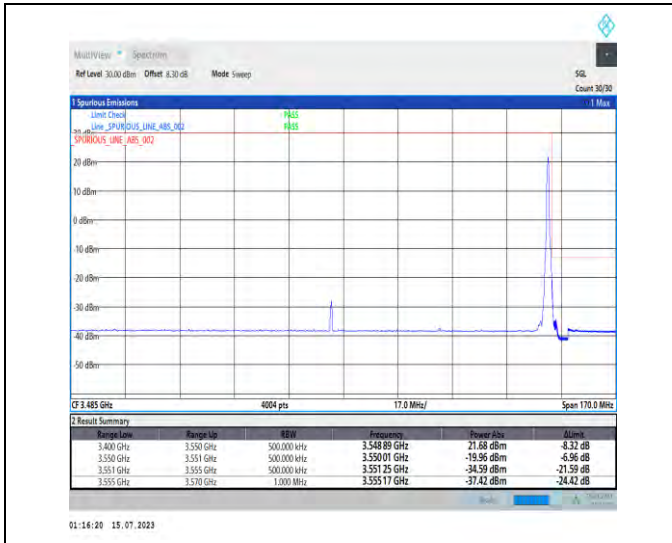
1-N78-3450-3550-PC1-30-70-H-2-DFT-PI2BPSK-Edge_1RB_Right-1@188-Ant1-1--PASS-see graph
