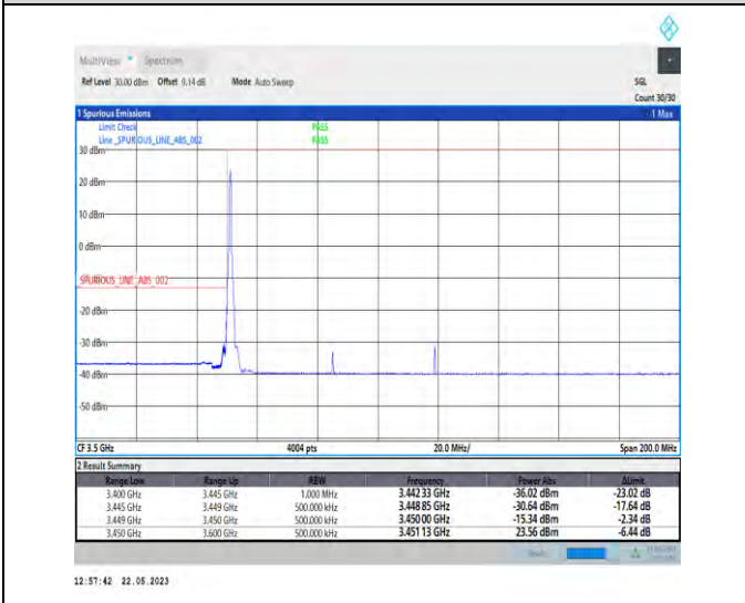
1-N78-3450-3550-PC1-30-70-L-4-CP-QPSK-Edge_1RB_Left-1@0-Ant1-1--PASS-see graph
