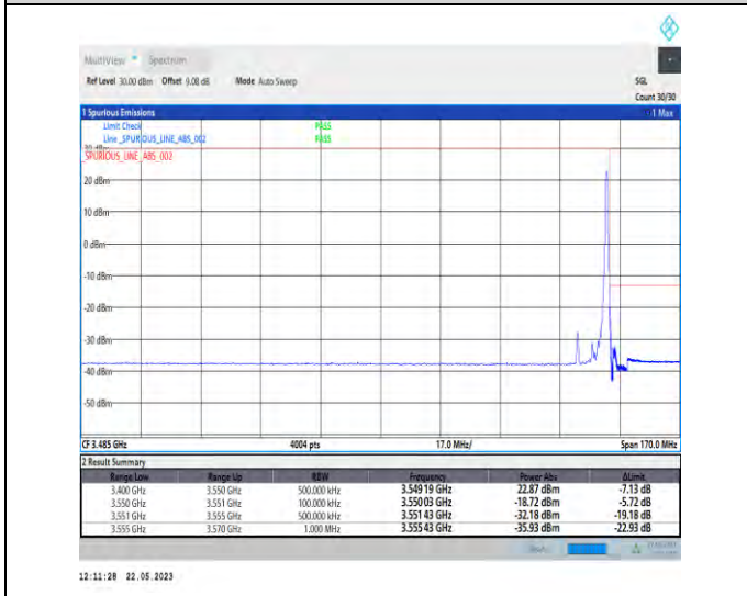
1-N78-3450-3550-PC1-30-10-H-5-CP-QPSK-Edge_1RB_Right-1@23-Ant1-1--PASS-see graph
