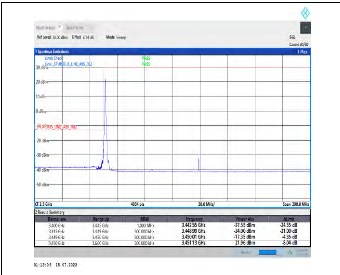
1-N78-3450-3550-PC1-30-70-L-1-DFT-PI2BPSK-Edge_1RB_Left-1@0-Ant1-1--PASS-see graph
