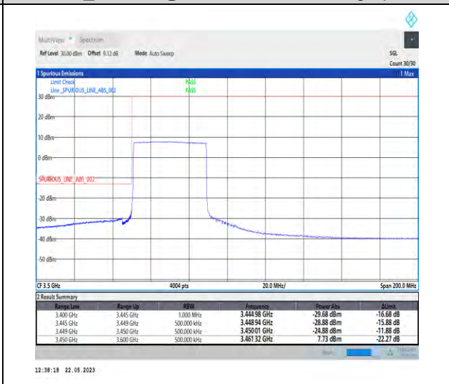
1-N78-3450-3550-PC1-30-40-L-6-CP-QPSK-Outer_Full-106@0-Ant1-1--PASS-see graph
