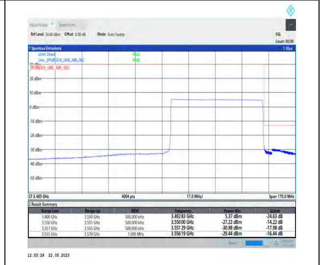
1-N78-3450-3550-PC1-30-60-H-6-CP-QPSK-Outer_Full-162@0-Ant1-1--PASS-see graph
