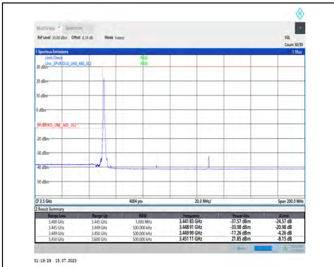
1-N78-3450-3550-PC1-30-80-L-1-DFT-PI2BPSK-Edge_1RB_Left-1@0-Ant1-1--PASS-see graph
