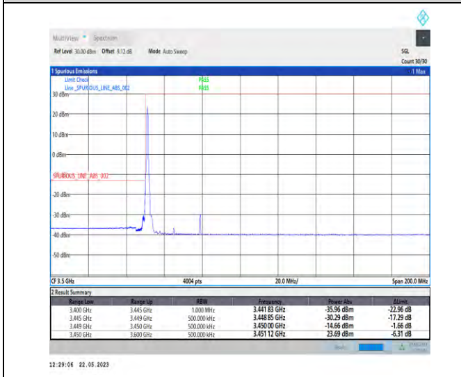
1-N78-3450-3550-PC1-30-30-L-4-CP-QPSK-Edge_1_RB_Left-1@0-Ant1-1--PASS-see graph
