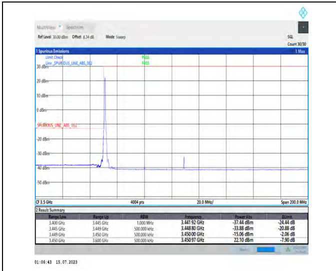
1-N78-3450-3550-PC1-30-60-L-1-DFT-PI2BPSK-Edge_1RB_Left-1@0-Ant1-1--PASS-see graph
