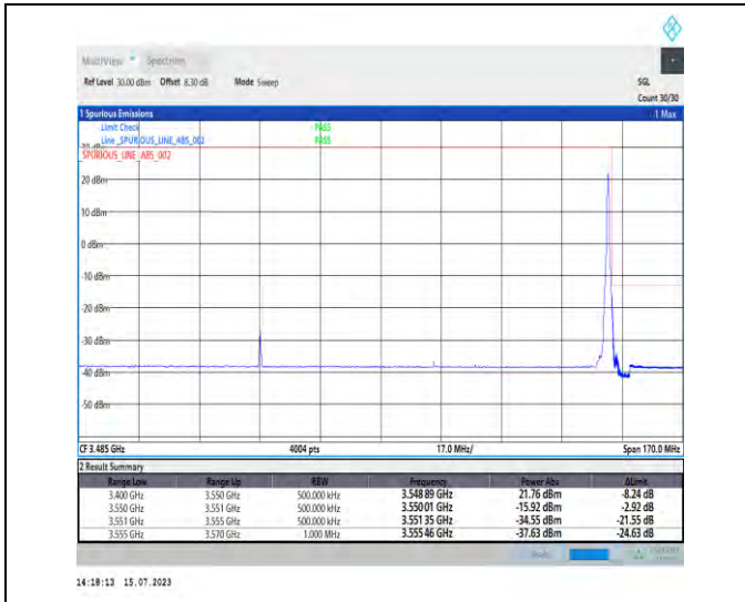
1-N78-3450-3550-PC1-30-100-H-2-DFT-PI2BPSK-Edge_1RB_Right-1@272-Ant1-1--PASS-see graph
