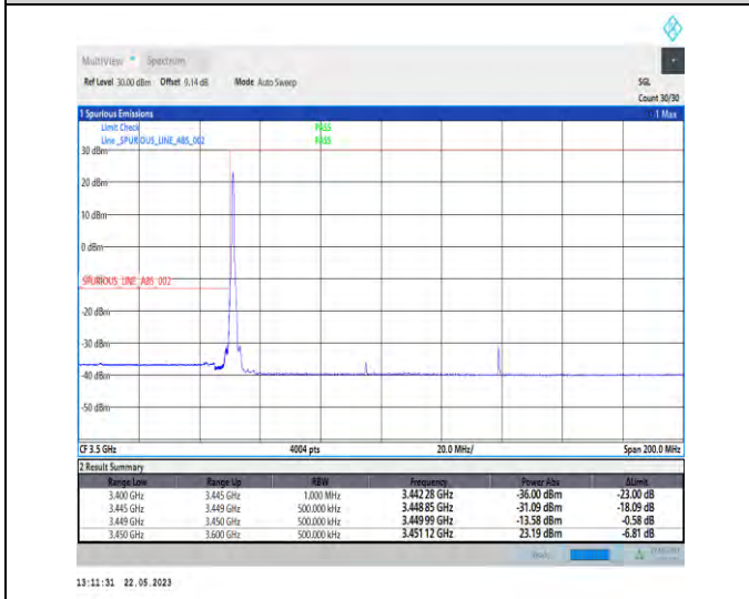
1-N78-3450-3550-PC1-30-90-L-4-CP-QPSK-Edge_1RB_Left-1@0-Ant1-1--PASS-see graph
