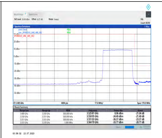
1-N78-3450-3550-PC1-30-40-H-3-DFT-PI2BPSK-Outer_Full-100@0-Ant1-1--PASS-see graph
