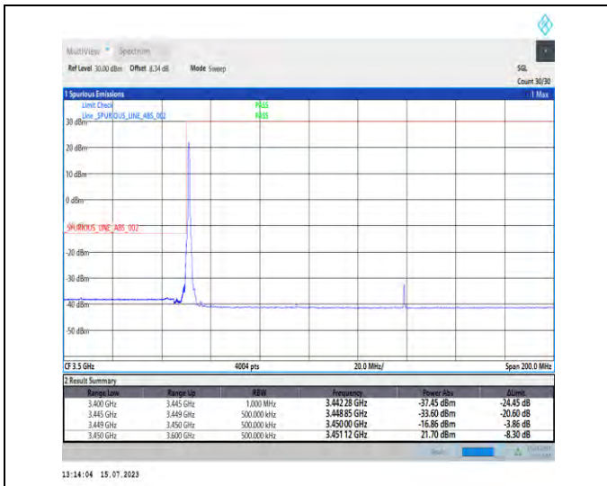
1-N78-3450-3550-PC1-30-90-L-1-DFT-PI2BPSK-Edge_1RB_Left-1@0-Ant1-1--PASS-see graph
