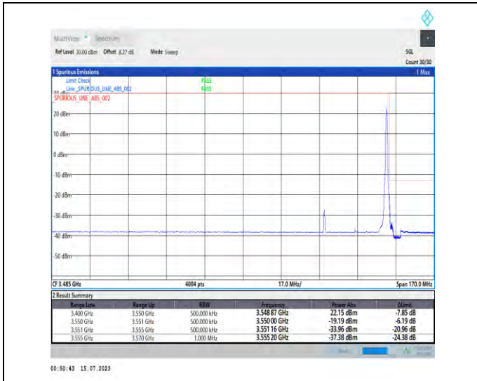
1-N78-3450-3550-PC1-30-30-H-2-DFT-PI2BPSK-Edge_1RB_Right-1@77-Ant1-1--PASS-see graph
