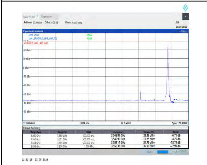
1-N78-3450-3550-PC1-30-30-H-5-CP-QPSK-Edge_1RB_Right-1@77-Ant1-1--PASS-see graph
