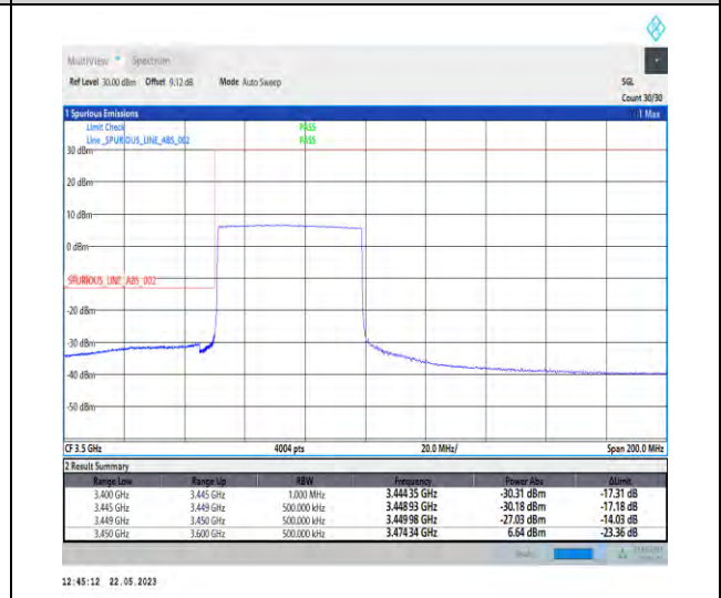
1-N78-3450-3550-PC1-30-50-L-6-CP-QPSK-Outer_Full-133@0-Ant1-1--PASS-see graph
