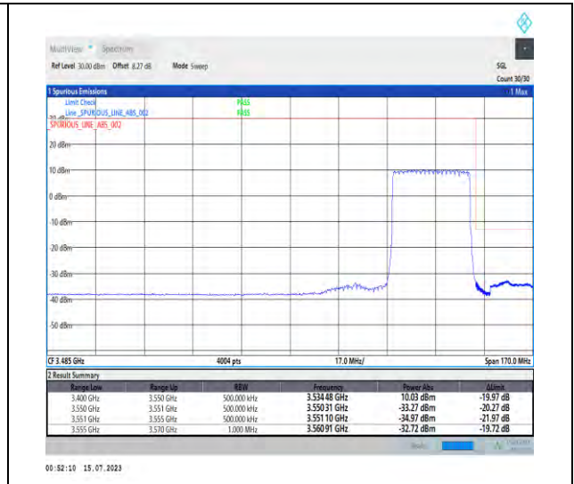
1-N78-3450-3550-PC1-30-30-H-3-DFT-PI2BPSK-Outer_Full-75@0-Ant1-1--PASS-see graph
