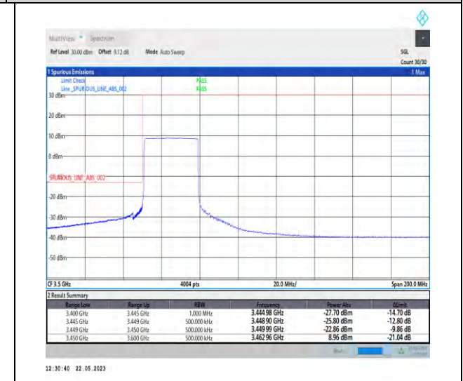
1-N78-3450-3550-PC1-30-30-L-6-CP-QPSK-Outer_Full-78@0-Ant1-1--PASS-see graph
