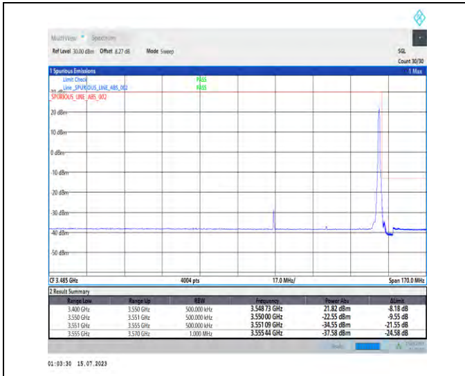
1-N78-3450-3550-PC1-30-50-H-2-DFT-PI2BPSK-Edge_1RB_Right-1@132-Ant1-1--PASS-see graph
