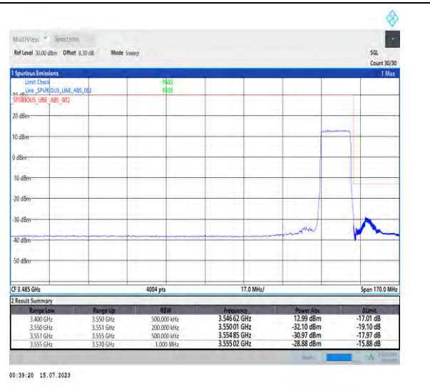
1-N78-3450-3550-PC1-30-15-H-3-DFT-PI2BPSK-Outer_Full-36@0-Ant1-1--PASS-see graph
