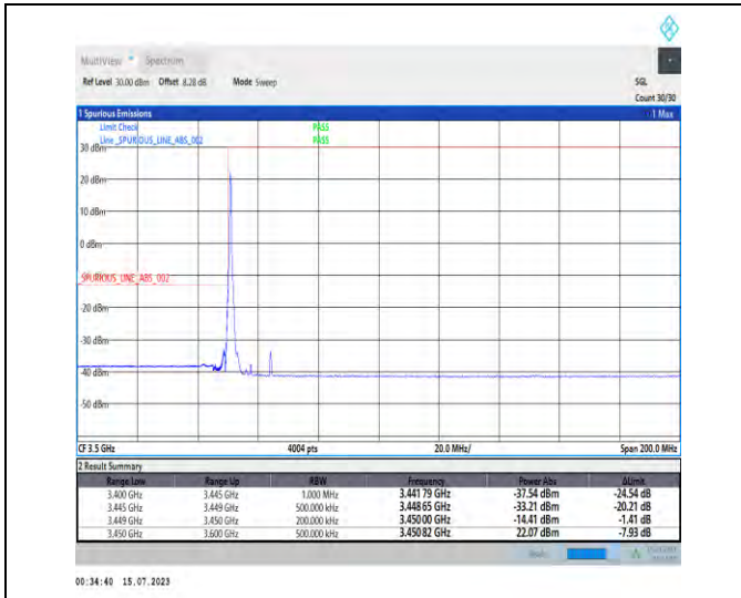
1-N78-3450-3550-PC1-30-15-L-1-DFT-PI2BPSK-Edge_1_RB_Left-1@0-Ant1-1--PASS-see graph
