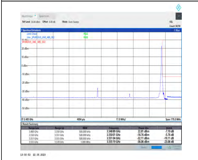
1-N78-3450-3550-PC1-30-70-H-5-CP-QPSK-Edge_1RB_Right-1@188-Ant1-1--PASS-see graph
