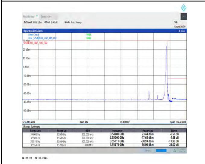
1-N78-3450-3550-PC1-30-20-H-5-CP-QPSK-Edge_1RB_Right-1@50-Ant1-1--PASS-see graph
