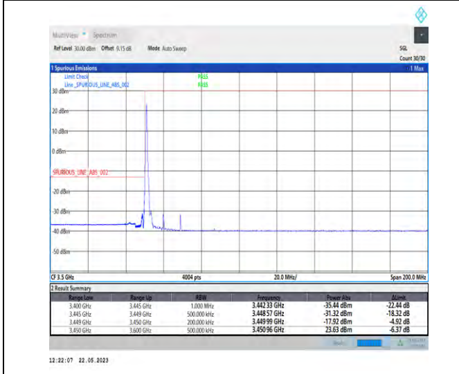
1-N78-3450-3550-PC1-30-20-L-4-CP-QPSK-Edge_1_RB_Left-1@0-Ant1-1--PASS-see graph
