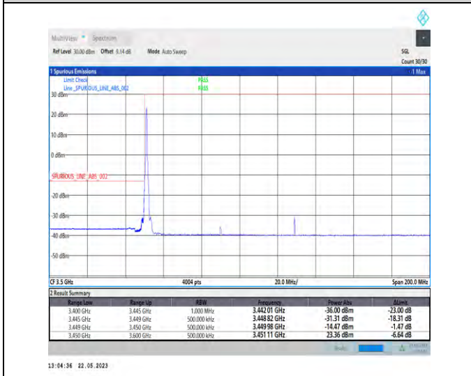
1-N78-3450-3550-PC1-30-80-L-4-CP-QPSK-Edge_1RB_Left-1@0-Ant1-1--PASS-see graph
