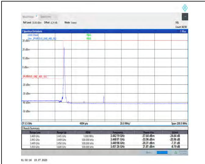
1-N78-3450-3550-PC1-30-50-L-1-DFT-PI2BPSK-Edge_1RB_Left-1@0-Ant1-1--PASS-see graph
