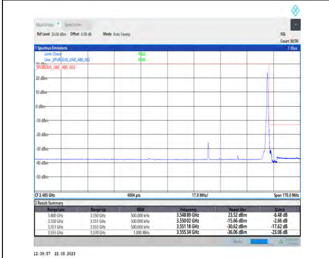
1-N78-3450-3550-PC1-30-40-H-5-CP-QPSK-Edge_1RB_Right-1@105-Ant1-1--PASS-see graph
