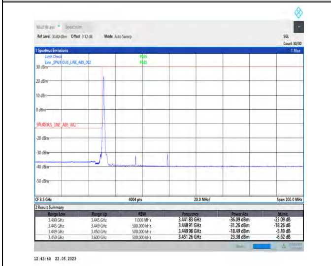
1-N78-3450-3550-PC1-30-50-L-4-CP-QPSK-Edge_1RB_Left-1@0-Ant1-1--PASS-see graph
