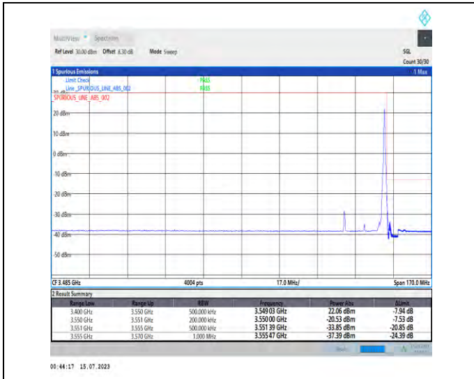
1-N78-3450-3550-PC1-30-20-H-2-DFT-PI2BPSK-Edge_1RB_Right-1@50-Ant1-1--PASS-see graph
