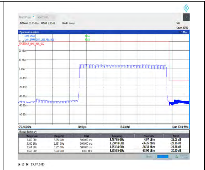
1-N78-3450-3550-PC1-30-90-H-3-DFT-PI2BPSK-Outer_Full-240@0-Ant1-1--PASS-see graph
