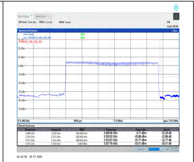
1-N78-3450-3550-PC1-30-100-H-3-DFT-PI2BPSK-Outer_Full-270@0-Ant1-1--PASS-see graph
