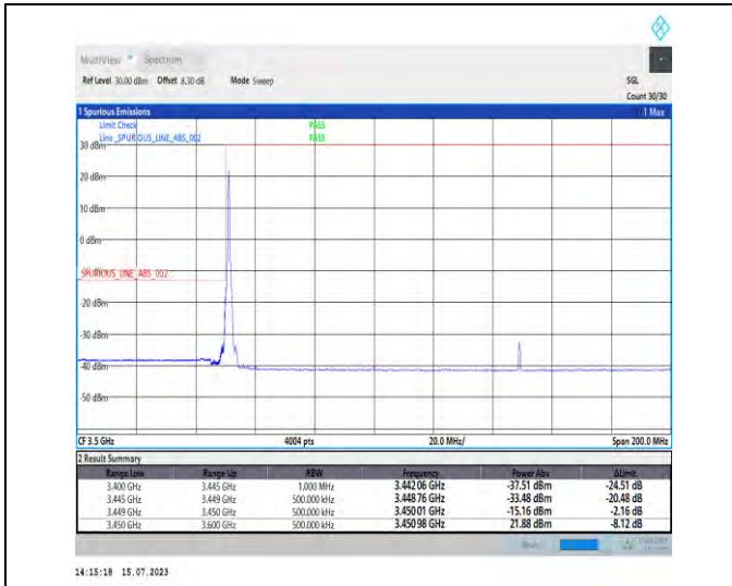
1-N78-3450-3550-PC1-30-100-L-1-DFT-PI2BPSK-Edge_1RB_Left-1@0-Ant1-1--PASS-see graph
