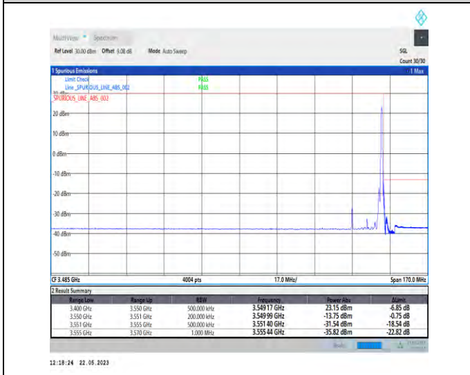
1-N78-3450-3550-PC1-30-15-H-5-CP-QPSK-Edge_1RB_Right-1@37-Ant1-1--PASS-see graph
