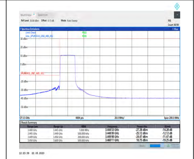
1-N78-3450-3550-PC1-30-20-L-6-CP-QPSK-Outer_Full-51@0-Ant1-1--PASS-see graph
