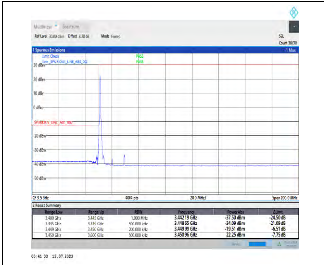
1-N78-3450-3550-PC1-30-20-L-1-DFT-PI2BPSK-Edge_1_RB_Left-1@0-Ant1-1--PASS-see graph
