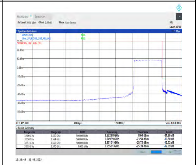
1-N78-3450-3550-PC1-30-30-H-6-CP-QPSK-Outer_Full-78@0-Ant1-1--PASS-see graph
