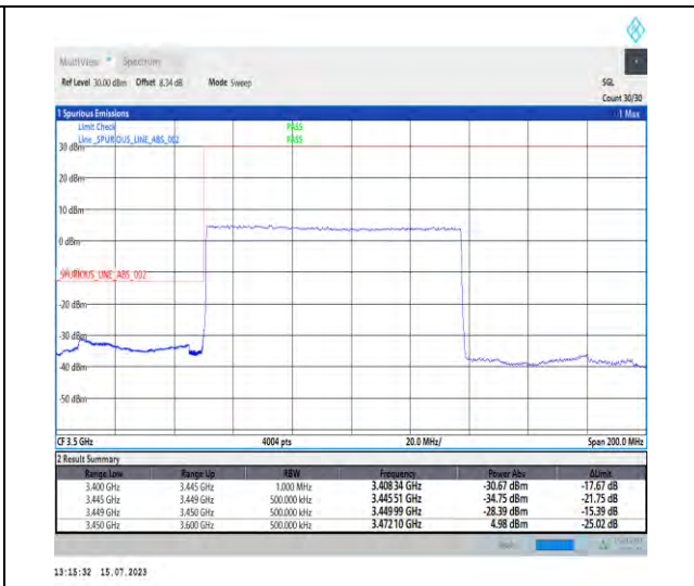
1-N78-3450-3550-PC1-30-90-L-3-DFT-PI2BPSK-Outer_Full-240@0-Ant1-1--PASS-see graph
