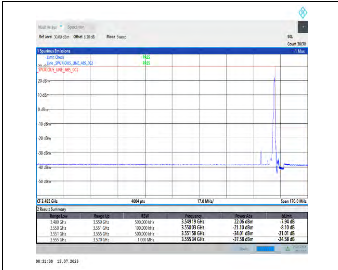
1-N78-3450-3550-PC1-30-10-H-2-DFT-PI2BPSK-Edge_1RB_Right-1@23-Ant1-1--PASS-see graph
