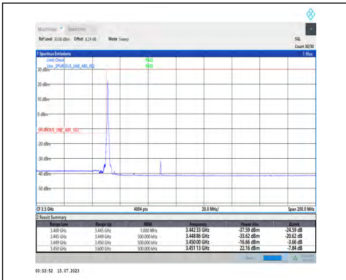
1-N78-3450-3550-PC1-30-40-L-1-DFT-PI2BPSK-Edge_1RB_Left-1@0-Ant1-1--PASS-see graph
