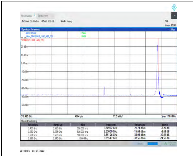
1-N78-3450-3550-PC1-30-60-H-2-DFT-PI2BPSK-Edge_1RB_Right-1@161-Ant1-1--PASS-see graph
