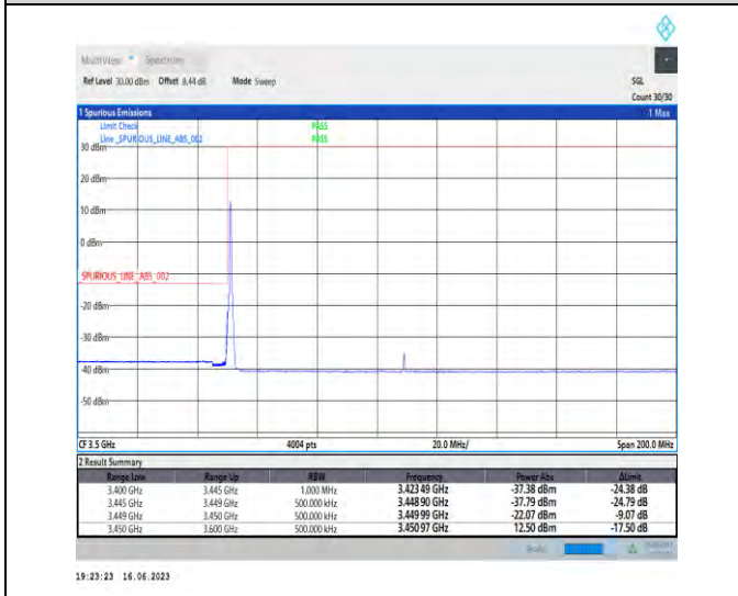
1-N78-3450-3550-PC1-30-60-L-4-CP-QPSK-Edge_1RB_Left-1@0-Ant1-1--PASS-see graph
