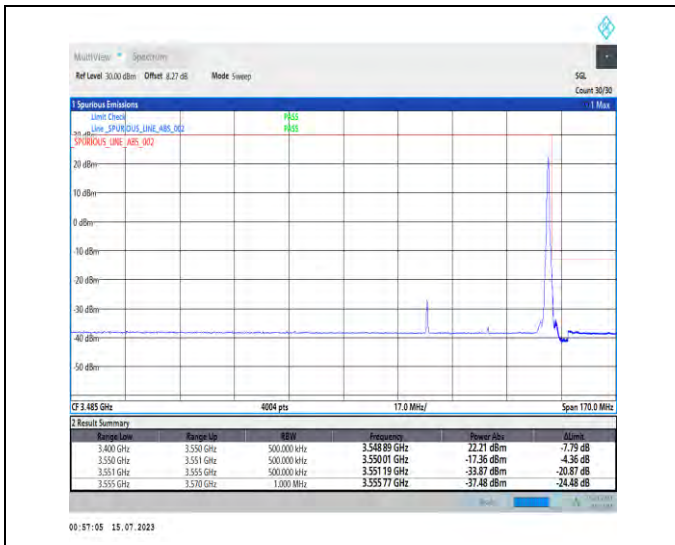
1-N78-3450-3550-PC1-30-40-H-2-DFT-PI2BPSK-Edge_1RB_Right-1@105-Ant1-1--PASS-see graph
