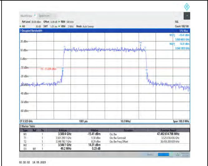
1-N78-3450-3550-PC1-30-50-H-7-CP-16QAM-Outer_Full-133@0-Ant1-47.493-49.200-≤50-PASS
