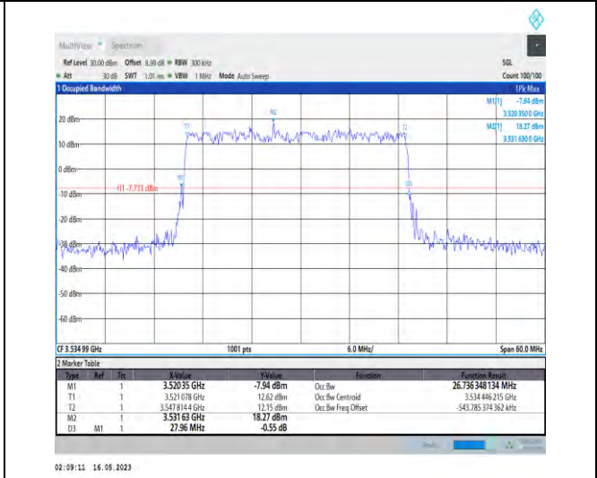
1-N78-3450-3550-PC1-30-30-H-1-DFT-QPSK-Outer_Full-75@0-Ant1-26.736-27.960-≤30-PASS
