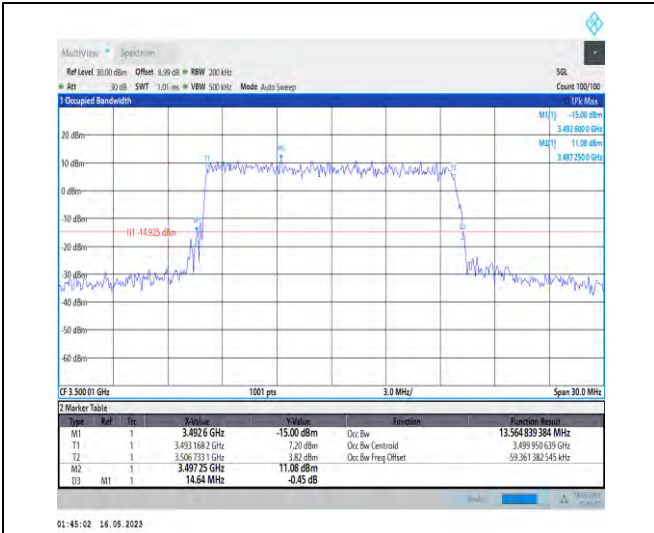
1-N78-3450-3550-PC1-30-15-M-9-CP-256QAM-Out er_Full-38@0-Ant1-13.565-14.640-≤15-PASS
