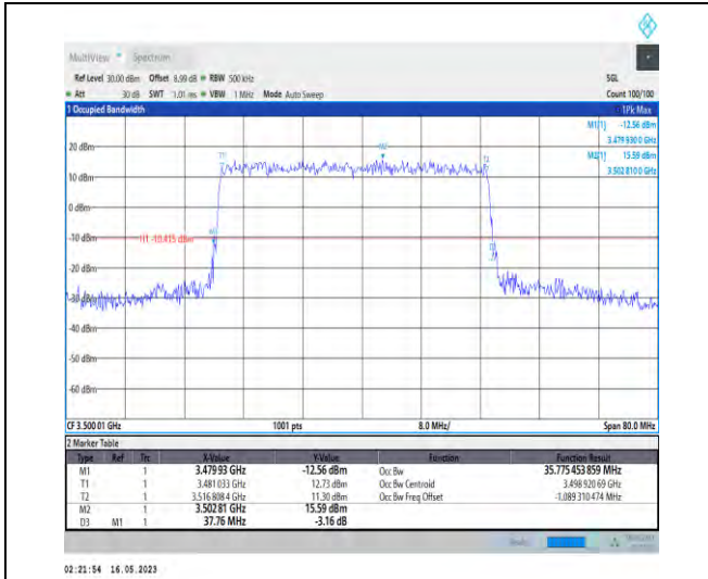
1-N78-3450-3550-PC1-30-40-M-4-DFT-64QAM-Out er_Full-100@0-Ant1-35.775-37.760-≤40-PASS
