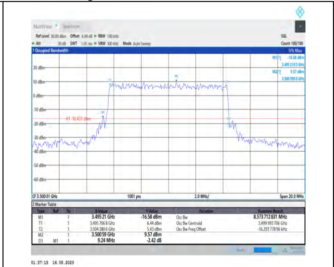
1-N78-3450-3550-PC1-30-10-M-9-CP-256QAM-Outer_Full-24@0-Ant1-8.574-9.240-≤10-PASS
