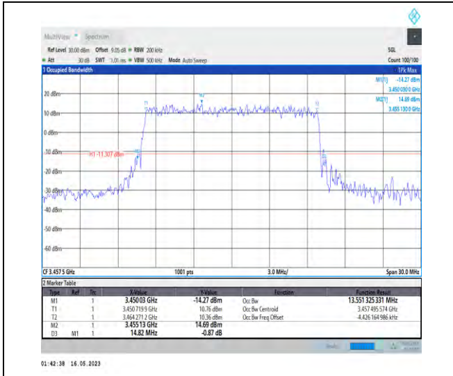
1-N78-3450-3550-PC1-30-15-L-6-CP-QPSK-Outer_Full-38@0-Ant1-13.551-14.820-≤15-PASS
