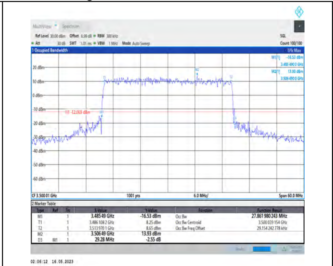
1-N78-3450-3550-PC1-30-30-M-8-CP-64QAM-Outer_Full-78@0-Ant1-27.862-29.280-≤30-PASS
