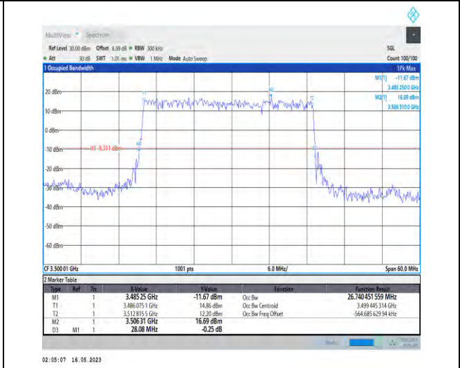
1-N78-3450-3550-PC1-30-30-M-2-DFT-PI2BPSK-Outer _Full-75@0-Ant1-26.74-28.080-≤30-PASS
