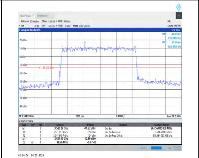
1-N78-3450-3550-PC1-30-30-H-5-DFT-256QAM-Outer_Full-75@0-Ant1-26.756-28.260-≤30-PASS
