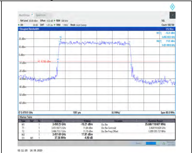
1-N78-3450-3550-PC1-30-40-L-2-DFT-PI2BPSK-Out_er_Full-100@0-Ant1-35.686-37.360-≤40-PASS
