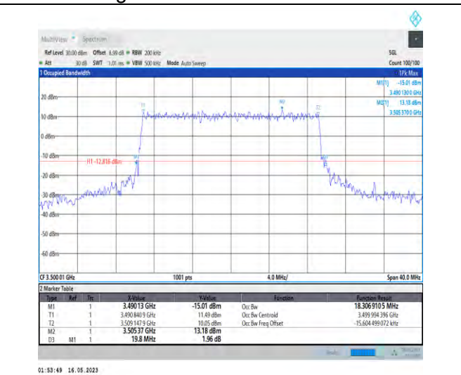
1-N78-3450-3550-PC1-30-20-M-7-CP-16QAM-Outer_Full-51@0-Ant1-18.307-19.800-≤20-PASS
