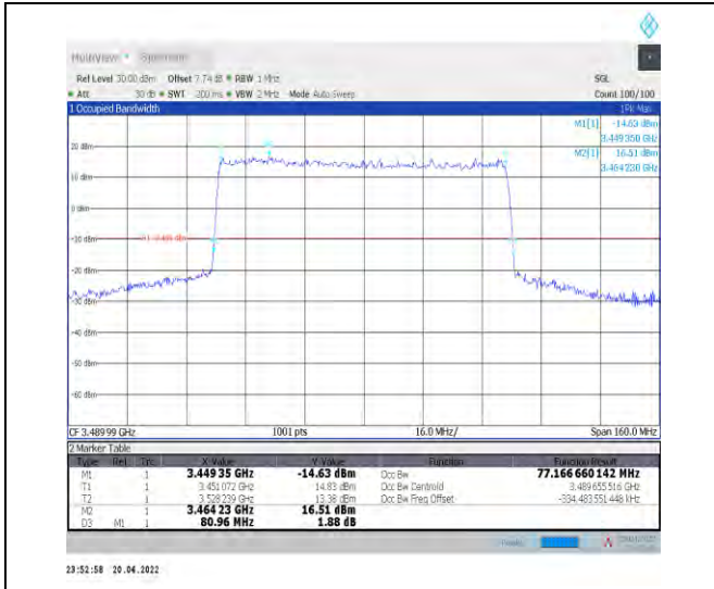
1-N78-3450-3550--30-80-L-1-DFT-QPSK-Outer_Full-216@0-Ant1-77.167-80.960-<math>\leq 80</math>-PASS
