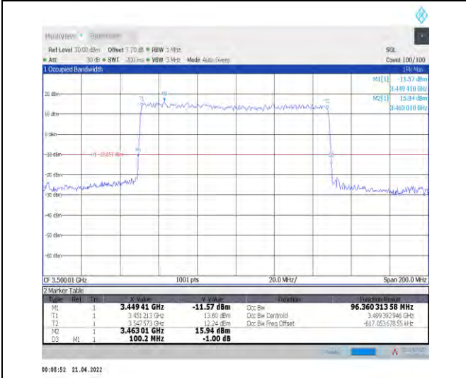
1-N78-3450-3550--30-100-L-1-DFT-QPSK-Outer_Full I-270@0-Ant1-96.36-100.200-≤100-PASS
