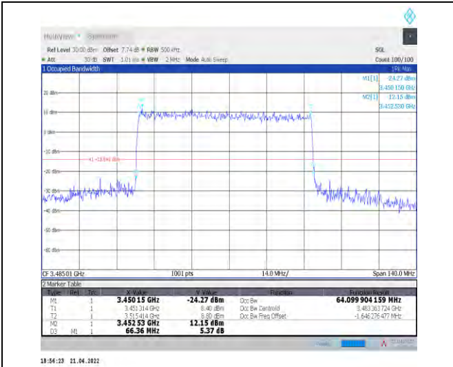
1-N78-3450-3550--30-70-L-4-DFT-64QAM-Outer_Full-180@0-Ant1-64.1-66.360-<math>\leq</math>70-PASS
