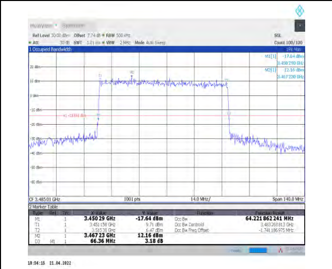
1-N78-3450-3550--30-70-L-3-DFT-16QAM-Outer_Full-180@0-Ant1-64.222-66.360-<=70-PASS
