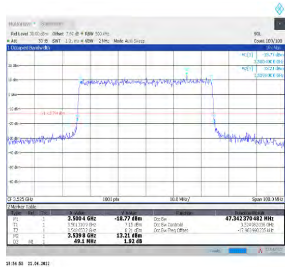
1-N78-3450-3550--30-50-H-7-CP-16QAM-Outer_Full -133@0-Ant1-47.342-49.100-≤50-PASS
