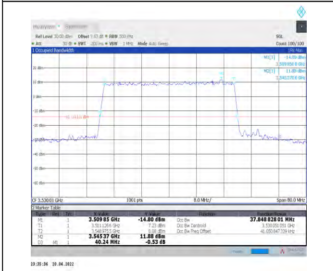
1-N78-3450-3550--30-40-H-9-CP-256QAM-Outer_Fu ll-106@0-Ant1-37.849-40.240-≤40-PASS
