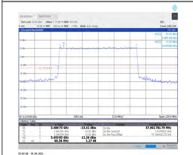
1-N78-3450-3550--30-60-H-7-CP-16QAM-Outer_Full-162@0-Ant1-57.903-60.360-≤60-PASS
