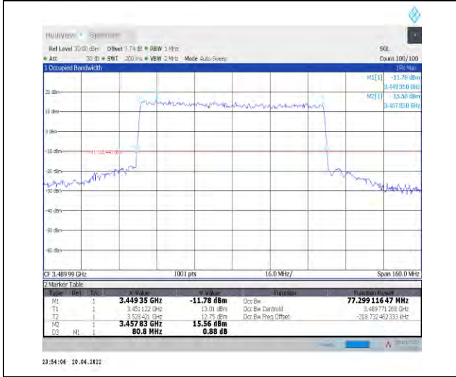
1-N78-3450-3550--30-80-L-3-DFT-16QAM-Outer_Ful-I-216@0-Ant1-77.299-80.800-<math>\leq 80</math>-PASS
