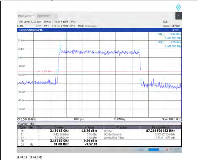
1-N78-3450-3550--30-90-H-9-CP-256QAM-Outer_Full -245@0-Ant1-87.285-91.080-≤90-PASS
