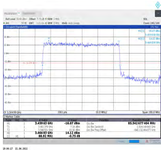
1-N78-3450-3550--30-90-H-3-DFT-16QAM-Outer_Full-240@0-Ant1-85.543-88.920-<=90-PASS
