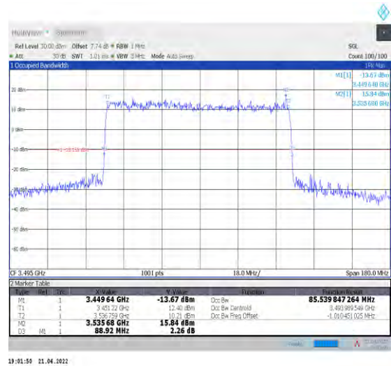
1-N78-3450-3550--30-90-L-1-DFT-QPSK-Outer_Full- 240@0-Ant1-85.54-88.920-≤90-PASS
