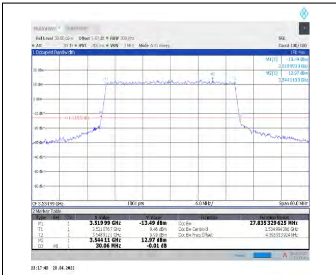
1-N78-3450-3550--30-30-H-6-CP-QPSK-Outer_Full-78@0-Ant1-27.835-30.060-<30-PASS
