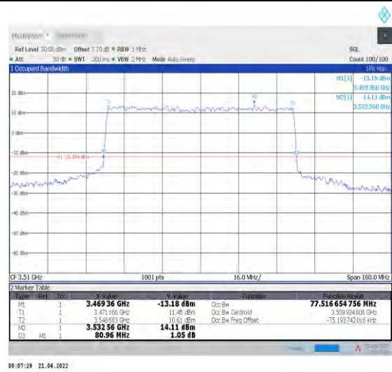
1-N78-3450-3550--30-80-H-8-CP-64QAM-Outer_Full -217@0-Ant1-77.517-80.960-≤80-PASS
