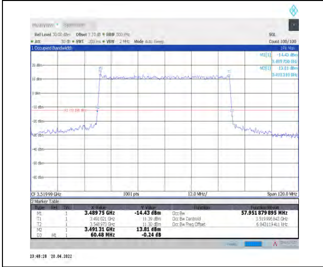
1-N78-3450-3550--30-60-H-3-DFT-16QAM-Outer_Fu II-162@0-Ant1-57.952-60.480-≤60-PASS
