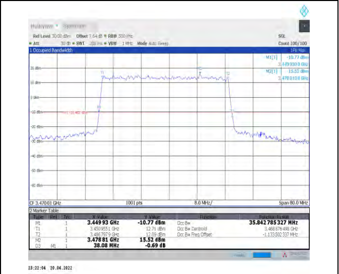
1-N78-3450-3550--30-40-L-4-DFT-64QAM-Outer_Fu ll-100@0-Ant1-35.843-38.080-<math>\leq 40</math>-PASS
