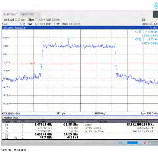
1-N78-3450-3550--30-50-M-3-DFT-16QAM-Outer_Full Full-128@0-Ant1-45.541-47.700-≤50-PASS
