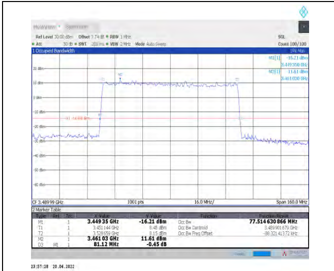
1-N78-3450-3550--30-80-L-9-CP-256QAM-Outer_Fu ll-217@0-Ant1-77.515-81.120≤80-PASS
