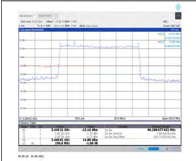
1-N78-3450-3550--30-100-H-3-DFT-16QAM-Outer_Full-270@0-Ant1-96.289-100.600-≤100-PASS
