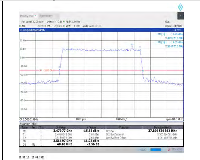
1-N78-3450-3550--30-40-M-9-CP-256QAM-Outer_Full-106@0-Ant1-37.9-40.480-<math>\leq 40</math>-PASS
