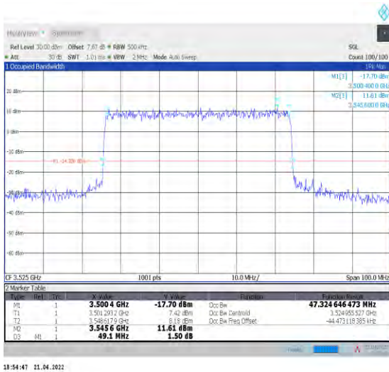
1-N78-3450-3550--30-50-H-6-CP-QPSK-Outer_Full- 133@0-Ant1-47.325-49.100-≤50-PASS
