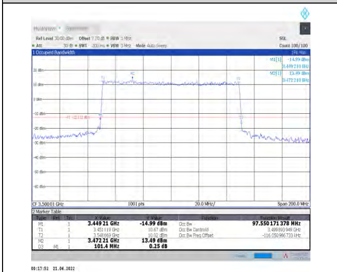
1-N78-3450-3550--30-100-M-8-CP-64QAM-Outer_Full -273@0-Ant1-97.55-101.400-≤100-PASS
