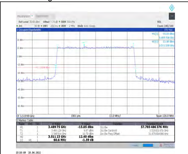
1-N78-3450-3550--30-60-H-6-CP-QPSK-Outer_Full-162@0-Ant1-57.785-60.600-≤60-PASS
