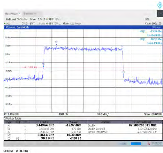
1-N78-3450-3550--30-90-L-9-CP-256QAM-Outer_Fu ll-245@0-Ant1-87.58-90.900≤90-PASS
