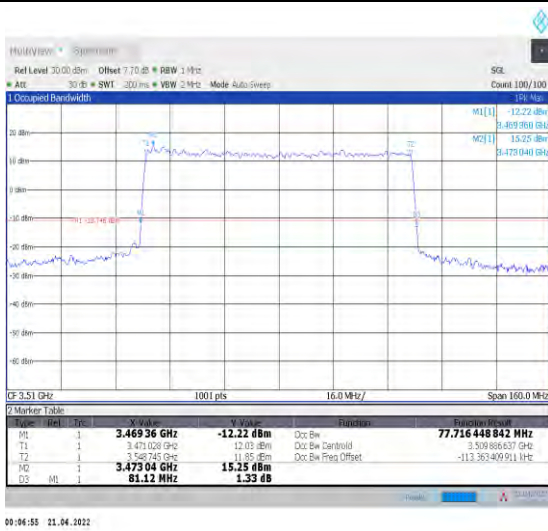
1-N78-3450-3550--30-80-H-7-CP-16QAM-Outer_Full -217@0-Ant1-77.716-81.120-≤80-PASS
