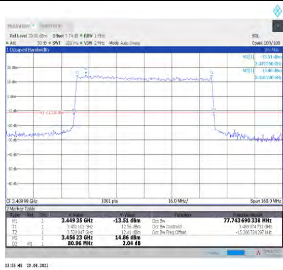
1-N78-3450-3550--30-80-L-6-CP-QPSK-Outer_Full-217@0-Ant1-77.744-80.960-<math>\leq 80</math>-PASS
