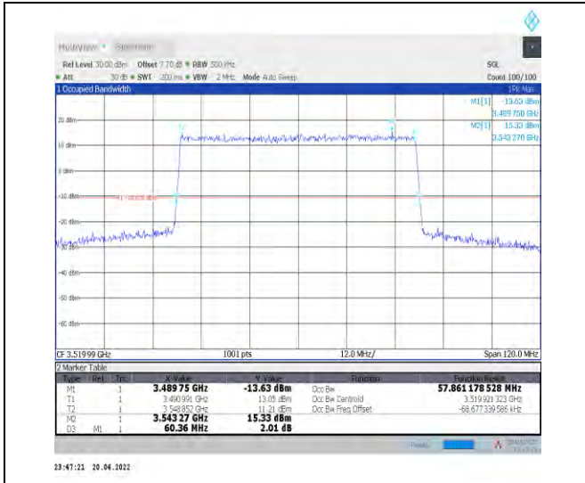
1-N78-3450-3550--30-60-H-1-DFT-QPSK-Outer_Full -162@0-Ant1-57.861-60.360-≤60-PASS
