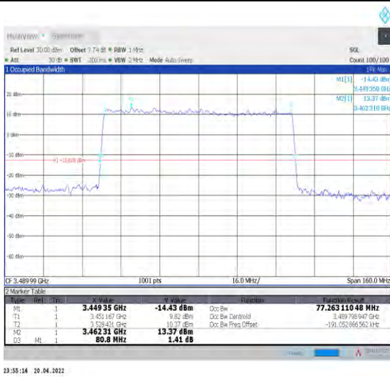
1-N78-3450-3550--30-80-L-5-DFT-256QAM-Outer_Full-216@0-Ant1-77.263-80.800-<math>\leq 80</math>-PASS
