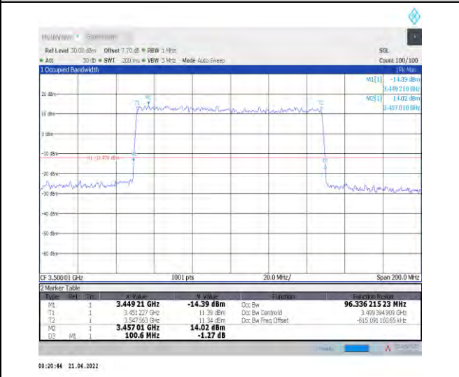
1-N78-3450-3550--30-100-H-4-DFT-64QAM-Outer_Full-270@0-Ant1-96.336-100.600-≤100-PASS
