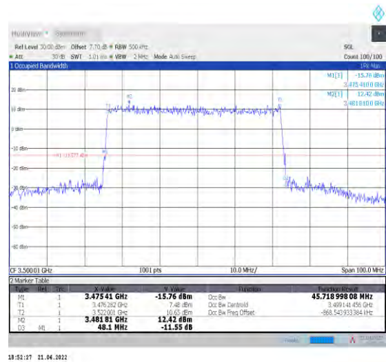
1-N78-3450-3550--30-50-M-4-DFT-64QAM-Outer_Full Full-128@0-Ant1-45.719-48.100-≤50-PASS
