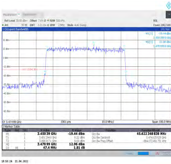
1-N78-3450-3550--30-50-L-4-DFT-64QAM-Outer_Ful l-128@0-Ant1-45.622-47.400-<math>\leq 50</math>-PASS
