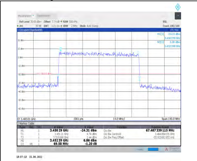
1-N78-3450-3550--30-70-L-9-CP-256QAM-Outer_Fu II-189@0-Ant1-67.487-69.580-≤70-PASS
