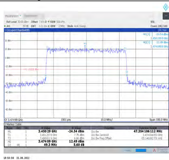
1-N78-3450-3550--30-50-L-7-CP-16QAM-Outer_Full -133@0-Ant1-47.354-49.300-≤50-PASS
