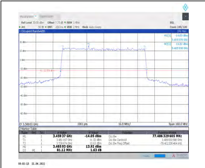
1-N78-3450-3550--30-80-M-8-CP-64QAM-Outer_Full -217@0-Ant1-77.486-81.120-≤80-PASS
