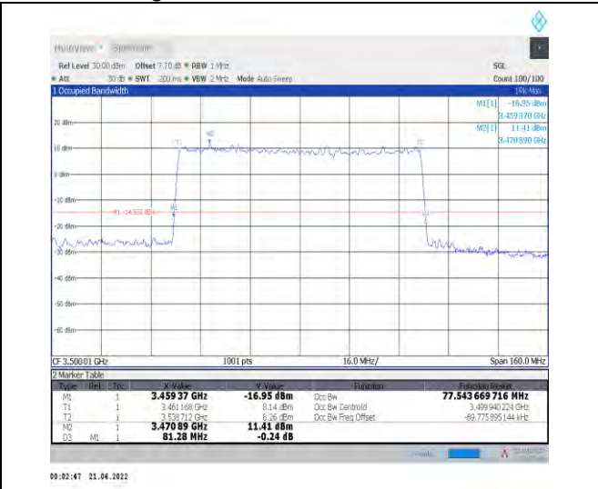
1-N78-3450-3550--30-80-M-9-CP-256QAM-Outer_Full -217@0-Ant1-77.544-81.280-≤80-PASS
