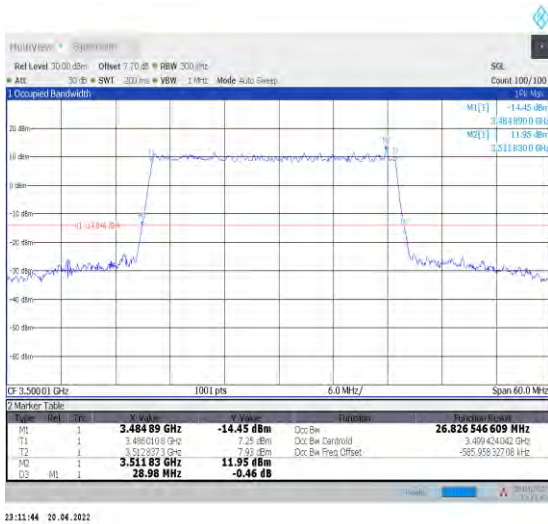
1-N78-3450-3550--30-30-M-5-DFT-256QAM-Outer_Full-75@0-Ant1-26.827-28.980-<=30-PASS
