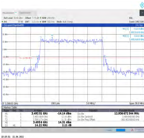
1-N78-3450-3550--30-15-M-3-DFT-16QAM-Outer_Full Full-36@0-Ant1-12.937-14.220-≤15-PASS
