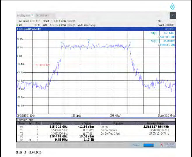
1-N78-3450-3550--30-10-H-2-DFT-PI2BPSK-Outer_Full -24@0-Ant1-8.569-9.480-≤10-PASS
