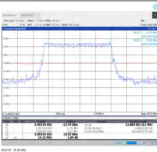
1-N78-3450-3550--30-15-M-1-DFT-QPSK-Outer_Full -36@0-Ant1-12.885-14.220-≤15-PASS
