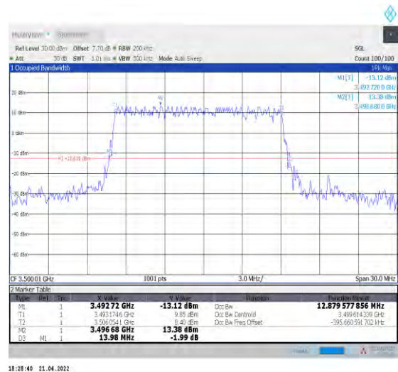
1-N78-3450-3550--30-15-M-4-DFT-64QAM-Outer_Full Full-36@0-Ant1-12.88-13.980-≤15-PASS
