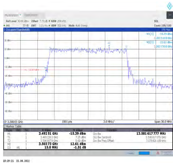
1-N78-3450-3550--30-15-M-8-CP-64QAM-Outer_Full-38@0-Ant1-13.582-15.000-≤15-PASS
