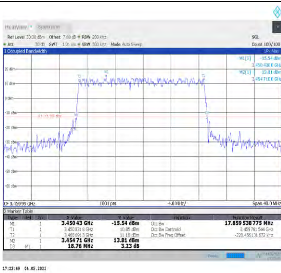
1-N78-3450-3550--30-20-L-3-DFT-16QAM-Outer_Full-50@0-Ant1-17.86-18.760-≤20-PASS
