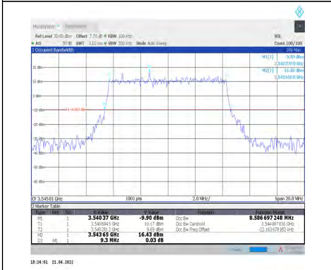
1-N78-3450-3550--30-10-H-1-DFT-QPSK-Outer_Full -24@0-Ant1-8.587-9.300-≤10-PASS
