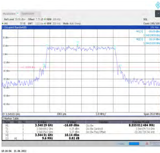
1-N78-3450-3550--30-10-H-5-DFT-256QAM-Outer_F ull-24@0-Ant1-8.555-9.600-≤10-PASS
