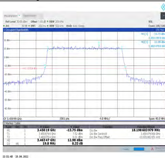
1-N78-3450-3550--30-20-L-8-CP-64QAM-Outer_Full -51@0-Ant1-18.199-19.800-<=20-PASS
