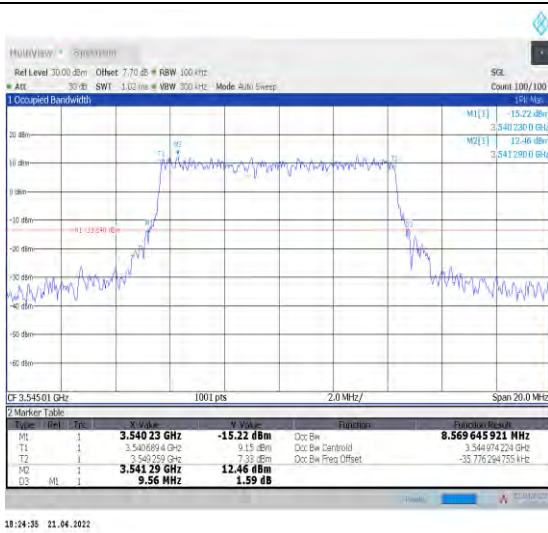
1-N78-3450-3550--30-10-H-3-DFT-16QAM-Outer_Fu Il-24@0-Ant1-8.57-9.560-≤10-PASS
