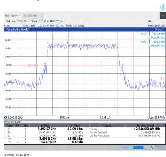
1-N78-3450-3550--30-15-M-2-DFT-PI2BPSK-Outer_Full Full-36@0-Ant1-12.846-14.430-≤15-PASS
