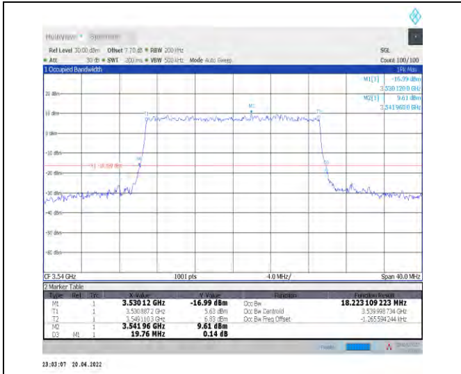
1-N78-3450-3550--30-20-H-9-CP-256QAM-Outer_Fu II-51@0-Ant1-18.223-19.760-≤20-PASS
