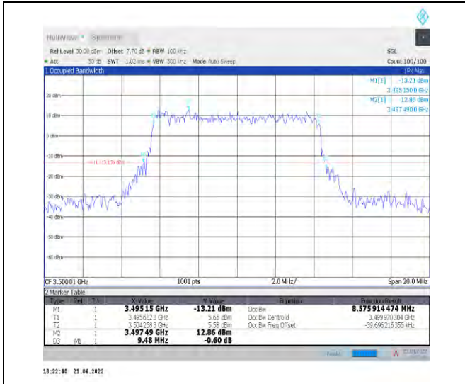
1-N78-3450-3550--30-10-M-4-DFT-64QAM-Outer_F ull-24@0-Ant1-8.576-9.480-<=10-PASS
