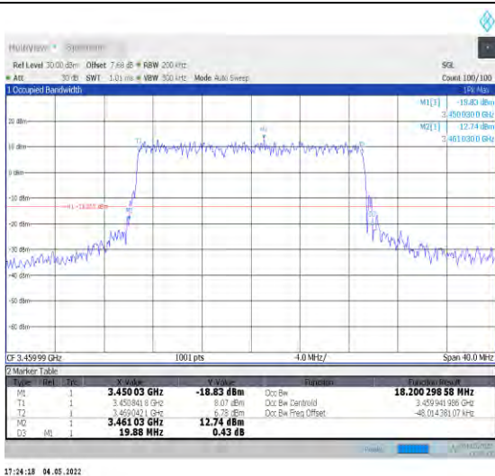
1-N78-3450-3550--30-20-L-7-CP-16QAM-Outer_Full -51@0-Ant1-18.2-19.880-<=20-PASS
