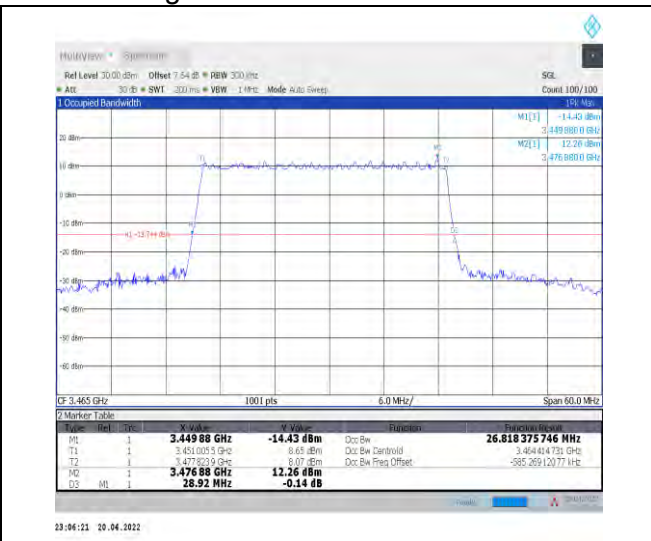
1-N78-3450-3550--30-30-L-5-DFT-256QAM-Outer_Full ull-75@0-Ant1-26.818-28.920-≤30-PASS
