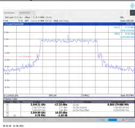
1-N78-3450-3550--30-10-H-8-CP-64QAM-Outer_Full -24@0-Ant1-8.569-9.780-≤10-PASS
