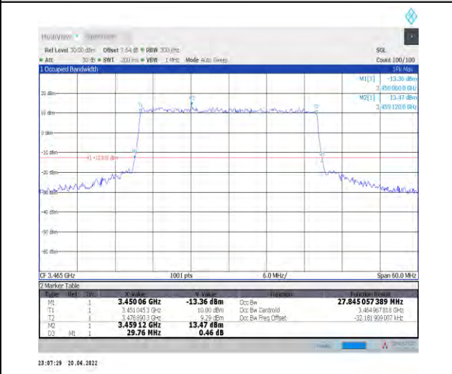
1-N78-3450-3550--30-30-L-7-CP-16QAM-Outer_Full -78@0-Ant1-27.845-29.760-≤30-PASS
