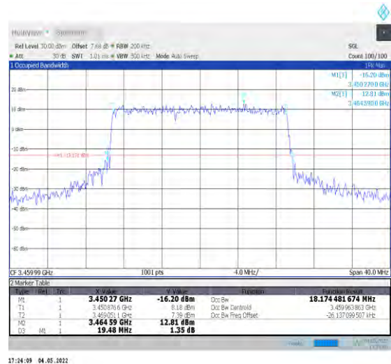
1-N78-3450-3550--30-20-L-6-CP-QPSK-Outer_Full-51@0-Ant1-18.174-19.480-≤20-PASS
