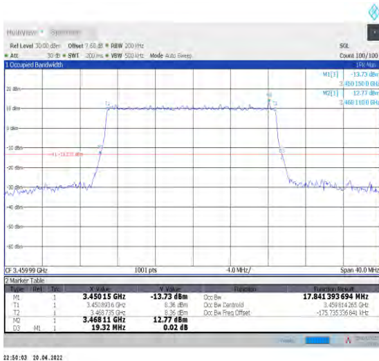
1-N78-3450-3550--30-20-L-5-DFT-256QAM-Outer_Full-50@0-Ant1-17.841-19.320-≤20-PASS
