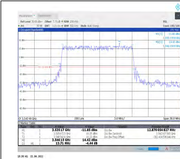
1-N78-3450-3550--30-15-H-4-DFT-64QAM-Outer_Fu ll-36@0-Ant1-12.87-13.710-≤15-PASS
