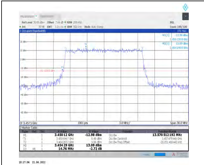
1-N78-3450-3550--30-15-L-6-CP-QPSK-Outer_Full_38@0-Ant1-13.571-14.760-<math>\leq 15</math>-PASS
