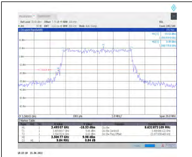
1-N78-3450-3550--30-10-M-8-CP-64QAM-Outer_Full -24@0-Ant1-8.633-9.840-≤10-PASS
