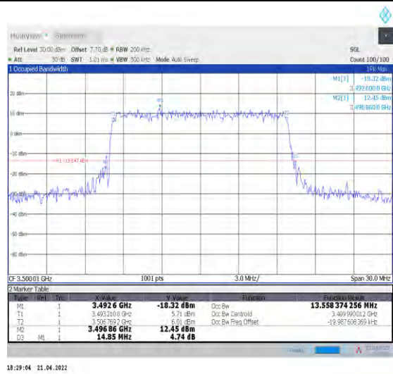
1-N78-3450-3550--30-15-M-6-CP-QPSK-Outer_Full-38@0-Ant1-13.558-14.850-≤15-PASS
