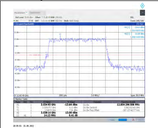
1-N78-3450-3550--30-15-H-5-DFT-256QAM-Outer_F ull-36@0-Ant1-12.854-14.130-≤15-PASS
