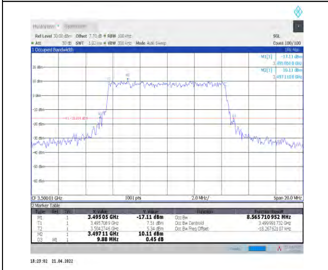
1-N78-3450-3550--30-10-M-6-CP-QPSK-Outer_F ull-24@0-Ant1-8.566-9.880-<=10-PASS
