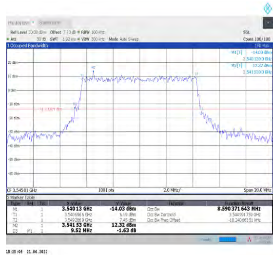
1-N78-3450-3550--30-10-H-6-CP-QPSK-Outer_Full- 24@0-Ant1-8.59-9.520-≤10-PASS
