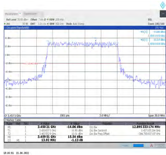
1-N78-3450-3550--30-15-L-1-DFT-QPSK-Outer_Full- 36@0-Ant1-12.895-13.920-≤15-PASS
