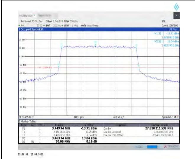
1-N78-3450-3550--30-30-L-6-CP-QPSK-Outer_Full-7 8@0-Ant1-27.83-30.060-≤30-PASS
