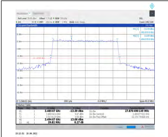
1-N78-3450-3550--30-30-M-7-CP-16QAM-Outer_Full -78@0-Ant1-27.87-29.820-≤30-PASS
