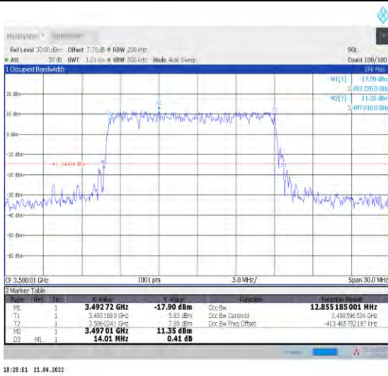
1-N78-3450-3550--30-15-M-5-DFT-256QAM-Outer_Full-36@0-Ant1-12.855-14.010-≤15-PASS
