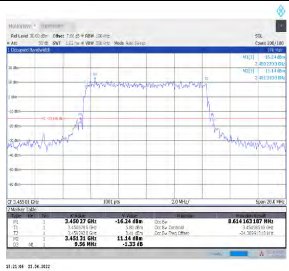
1-N78-3450-3550--30-10-L-6-CP-QPSK-Outer_Full-24@0-Ant1-8.614-9.560-≤10-PASS
