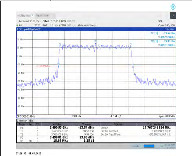
1-N78-3450-3550--30-20-M-3-DFT-16QAM-Outer_Full-50@0-Ant1-17.767-18.640-≤20-PASS
