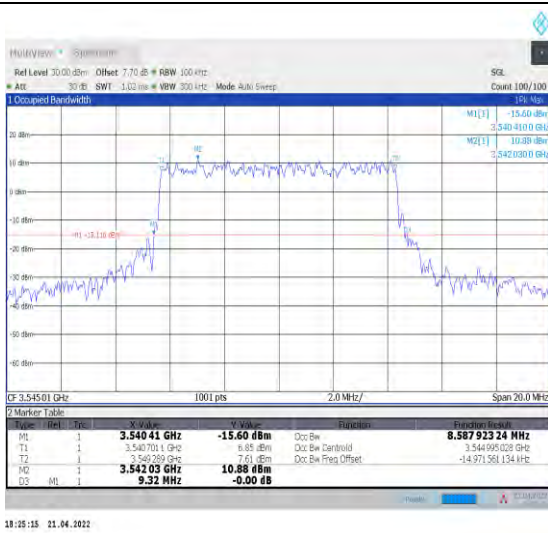
1-N78-3450-3550--30-10-H-7-CP-16QAM-Outer_Full -24@0-Ant1-8.588-9.320-≤10-PASS
