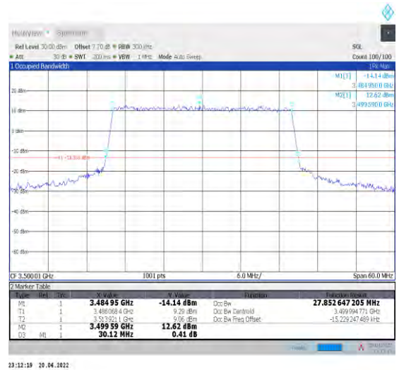
1-N78-3450-3550--30-30-M-6-CP-QPSK-Outer_Full-78@0-Ant1-27.853-30.120-<=30-PASS
