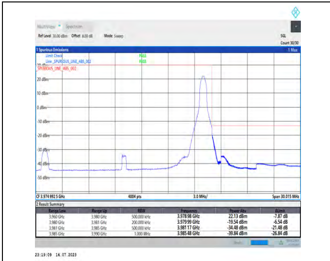
1-N77-3700-3980-PC1-30-20-H-2-DFT-PI2BPSK-Edge_1RB_Right-1@50-Ant1-1--PASS-see graph
