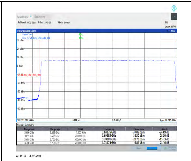
1-N77-3700-3980-PC1-30-60-L-3-DFT-PI2BPSK-Outer_Full-162@0-Ant1-1--PASS-see graph
