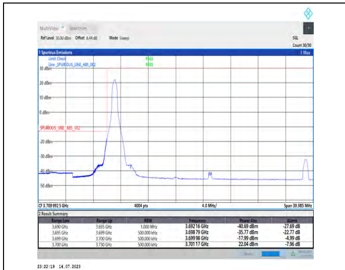
1-N77-3700-3980-PC1-30-30-L-1-DFT-PI2BPSK-Edge_1RB_Left-1@0-Ant1-1--PASS-see graph
