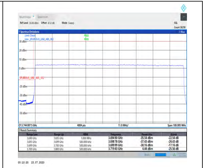
1-N77-3700-3980-PC1-30-100-L-3-DFT-PI2BPSK-Outer_Full-270@0-Ant1-1--PASS-see graph
