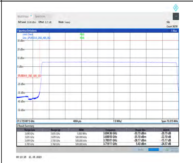
1-N77-3700-3980-PC1-30-60-L-6-CP-QPSK-Outer_Full-162@0-Ant1-1--PASS-see graph
