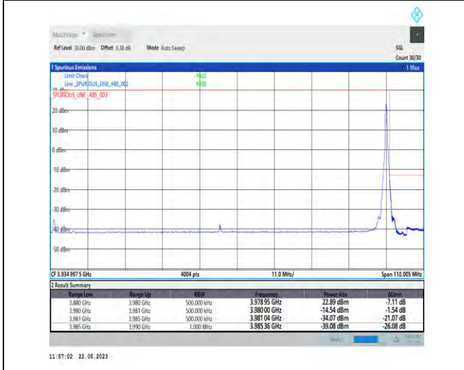
1-N77-3700-3980-PC1-30-100-H-5-CP-QPSK-Edge_1RB_Right-1@272-Ant1-1--PASS-see graph
