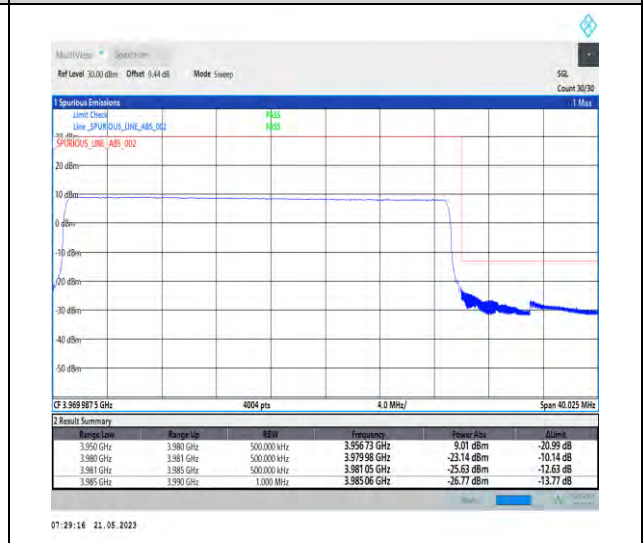
1-N77-3700-3980-PC1-30-30-H-6-CP-QPSK-Outer_Full-78@0-Ant1-1--PASS-see graph
