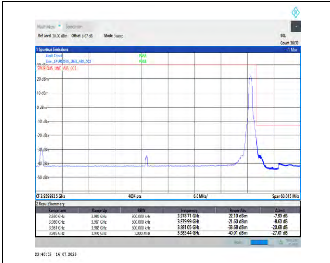
1-N77-3700-3980-PC1-30-50-H-2-DFT-PI2BPSK-Edge_1RB_Right-1@132-Ant1-1--PASS-see graph
