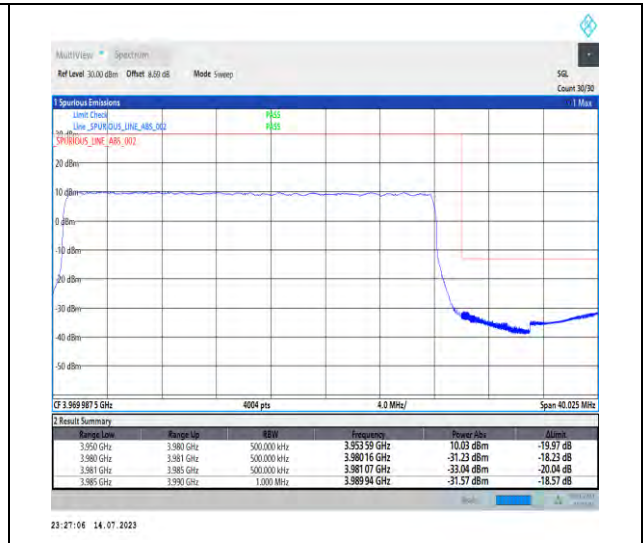
1-N77-3700-3980-PC1-30-30-H-3-DFT-PI2BPSK-Outer_Full-75@0-Ant1-1--PASS-see graph
