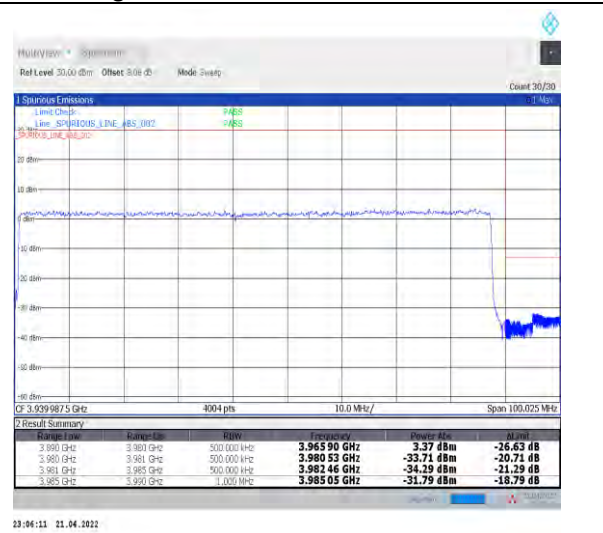
1-N77-3700-3980--30-90-H-3-DFT-PI2BPSK-Outer_Full-240@0-Ant1-PASS-see graph
