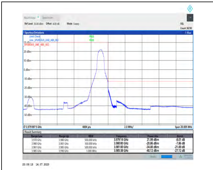
1-N77-3700-3980-PC1-30-10-H-2-DFT-PI2BPSK-Edge_1RB_Right-1@23-Ant1-1--PASS-see graph
