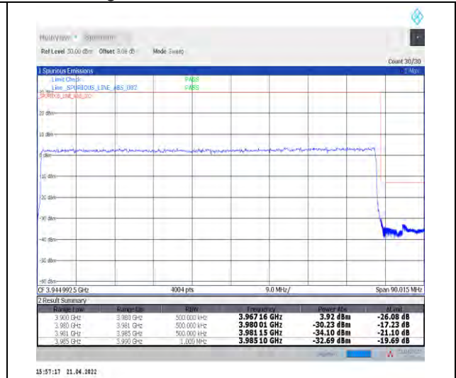
1-N77-3700-3980--30-80-H-3-DFT-PI2BPSK-Outer_Full-216@0-Ant1-PASS-see graph
