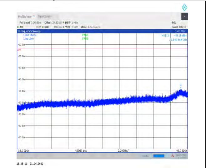
1-N77-3700-3980--30-100-H-1-DFT-PI2BPSK-Inner_ 1RB_Left-1@1-18000-40000-Ant1--48.18--13-PASS
