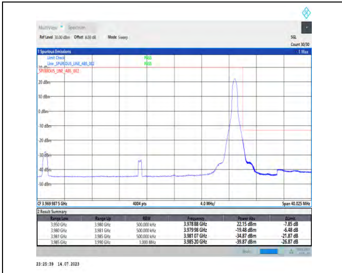
1-N77-3700-3980-PC1-30-30-H-2-DFT-PI2BPSK-Edge_1RB_Right-1@77-Ant1-1--PASS-see graph
