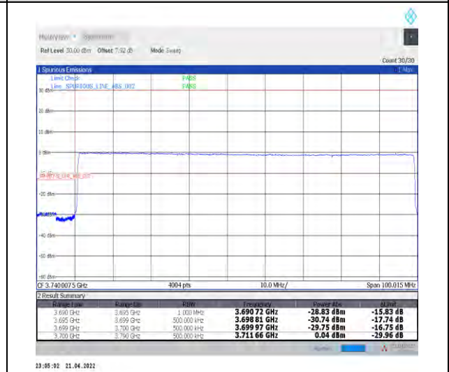
1-N77-3700-3980--30-90-L-6-CP-QPSK-Outer_Ful_I-245@0-Ant1-PASS-see graph
