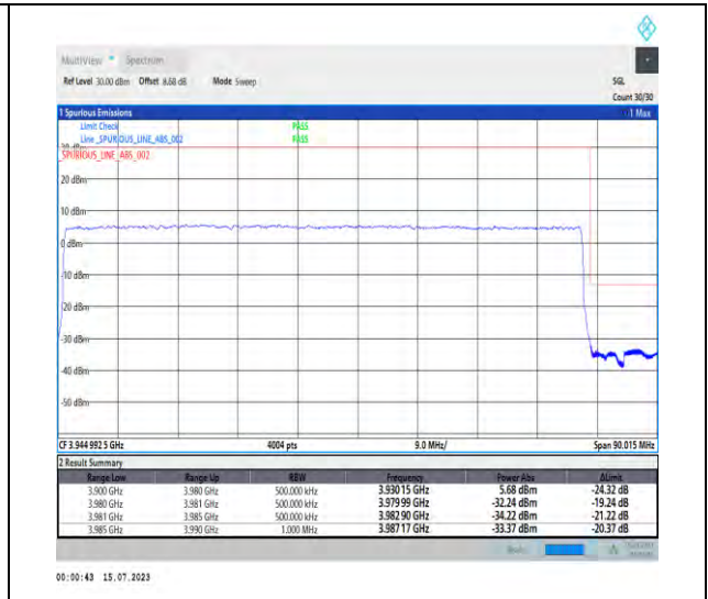
1-N77-3700-3980-PC1-30-80-H-3-DFT-PI2BPSK-Outer_Full-216@0-Ant1-1--PASS-see graph
