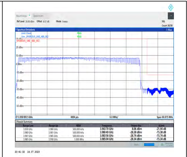
1-N77-3700-3980-PC1-30-50-H-3-DFT-PI2BPSK-Outer_Full-128@0-Ant1-1--PASS-see graph
