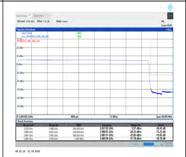
1-N77-3700-3980-PC1-30-60-H-6-CP-QPSK-Outer_Full-162@0-Ant1-1--PASS-see graph
