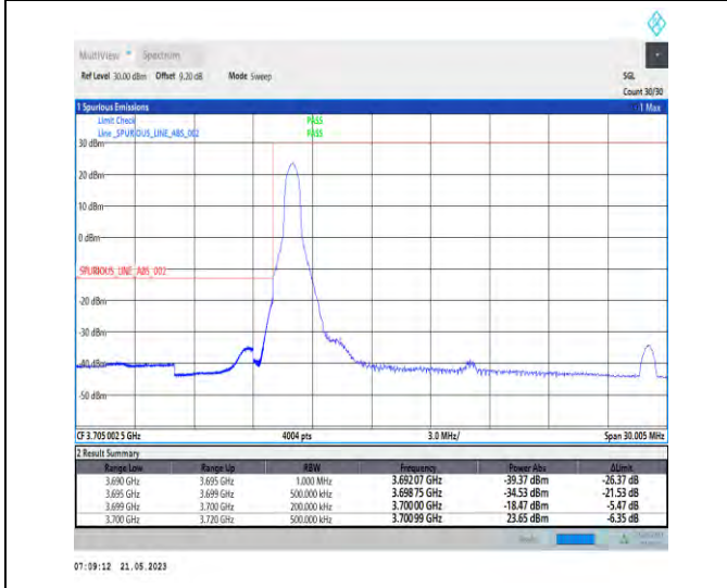
1-N77-3700-3980-PC1-30-20-L-4-CP-QPSK-Edge_1RB_Left-1@0-Ant1-1--PASS-see graph
