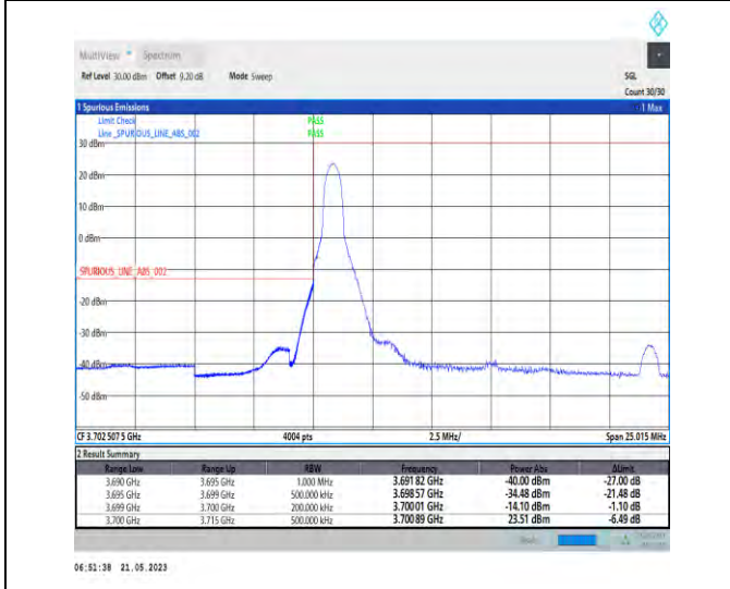
1-N77-3700-3980-PC1-30-15-L-4-CP-QPSK-Edge_1_RB_Left-1@0-Ant1-1--PASS-see graph
