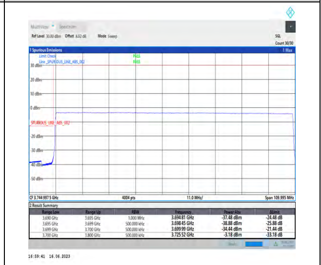
1-N77-3700-3980-PC1-30-100-L-6-CP-QPSK-Outer_Full-273@0-Ant1-1--PASS-see graph
