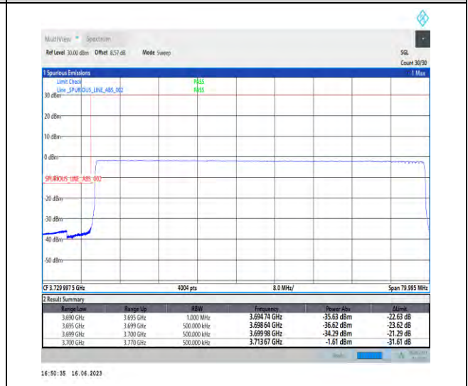
1-N77-3700-3980-PC1-30-70-L-6-CP-QPSK-Outer_Full-189@0-Ant1-1--PASS-see graph
