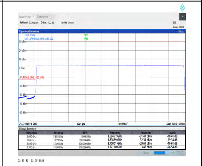
1-N77-3700-3980-PC1-30-90-L-6-CP-QPSK-Outer_Full-245@0-Ant1-1--PASS-see graph
