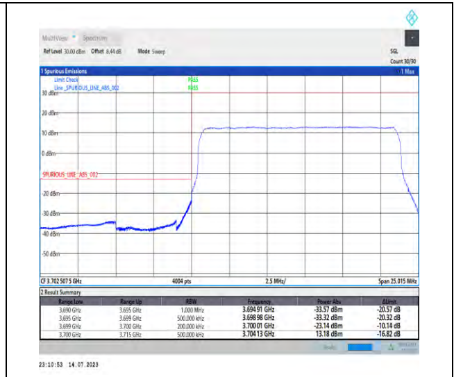
1-N77-3700-3980-PC1-30-15-L-3-DFT-PI2BPSK-Outer_Full-36@0-Ant1-1--PASS-see graph
