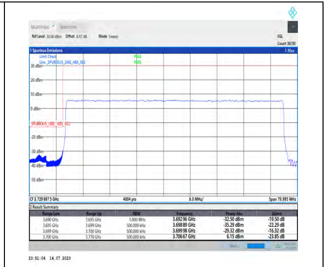
1-N77-3700-3980-PC1-30-70-L-3-DFT-PI2BPSK-Outer_Full-180@0-Ant1-1--PASS-see graph
