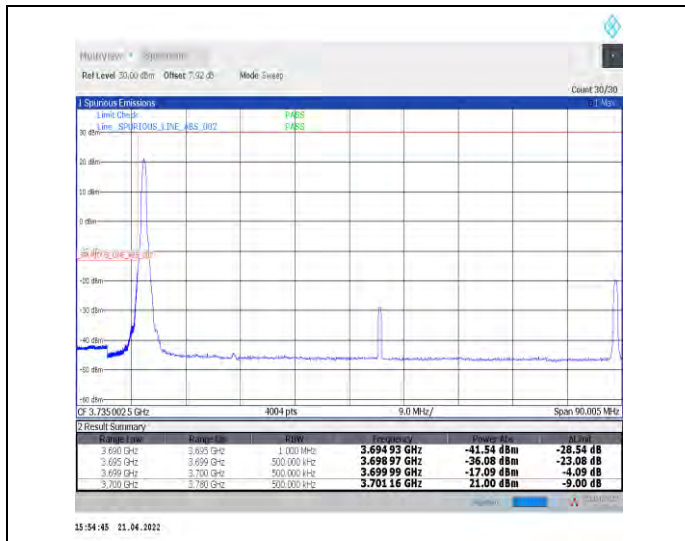
1-N77-3700-3980--30-80-L-1-DFT-PI2BPSK-Edge_1R_B_Left-1@0-Ant1-PASS-see graph
