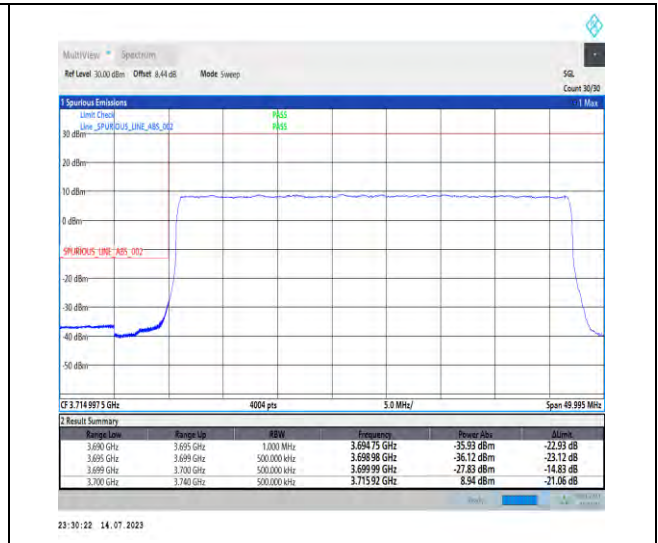
1-N77-3700-3980-PC1-30-40-L-3-DFT-PI2BPSK-Outer_Full-100@0-Ant1-1--PASS-see graph
