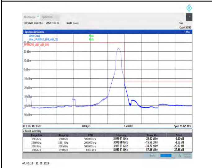
1-N77-3700-3980-PC1-30-15-H-5-CP-QPSK-Edge_1RB_Right-1@37-Ant1-1--PASS-see graph
