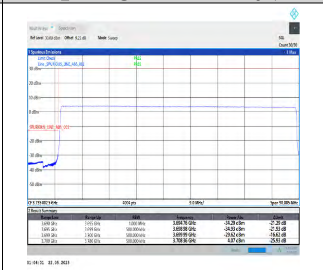
1-N77-3700-3980-PC1-30-80-L-6-CP-QPSK-Outer_Full-217@0-Ant1-1--PASS-see graph
