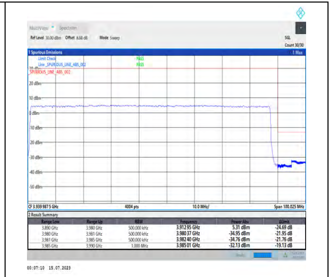
1-N77-3700-3980-PC1-30-90-H-3-DFT-PI2BPSK-Outer_Full-240@0-Ant1-1--PASS-see graph
