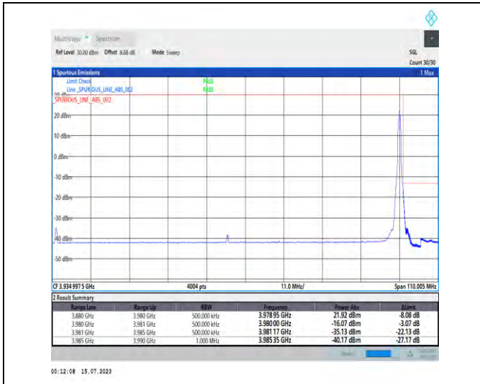
1-N77-3700-3980-PC1-30-100-H-2-DFT-PI2BPSK-Edge_e_1RB_Right-1@272-Ant1-1--PASS-see graph
