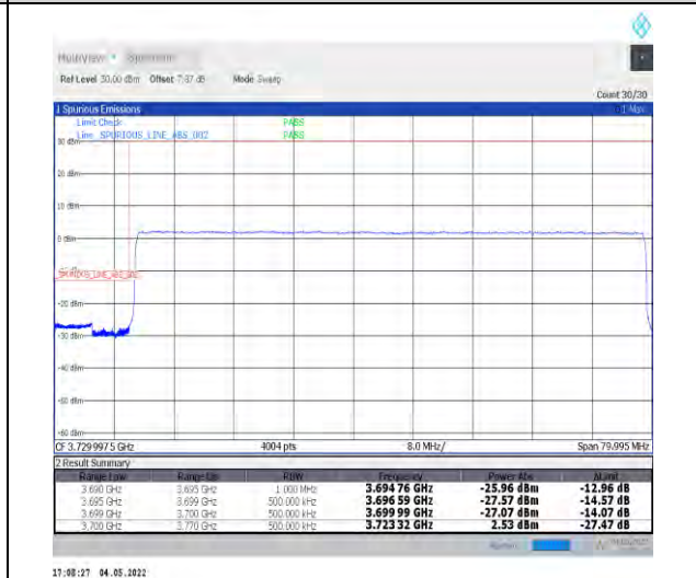
1-N77-3700-3980--30-70-L-6-CP-QPSK-Outer_Ful I-189@0-Ant1-PASS-see graph
