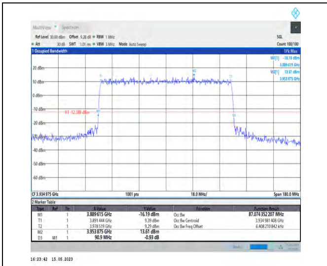
1-N77-3700-3980-PC1-30-90-H-8-CP-64QAM-Outer_Full-245@0-Ant1-87.074-90.900-≤90-PASS
