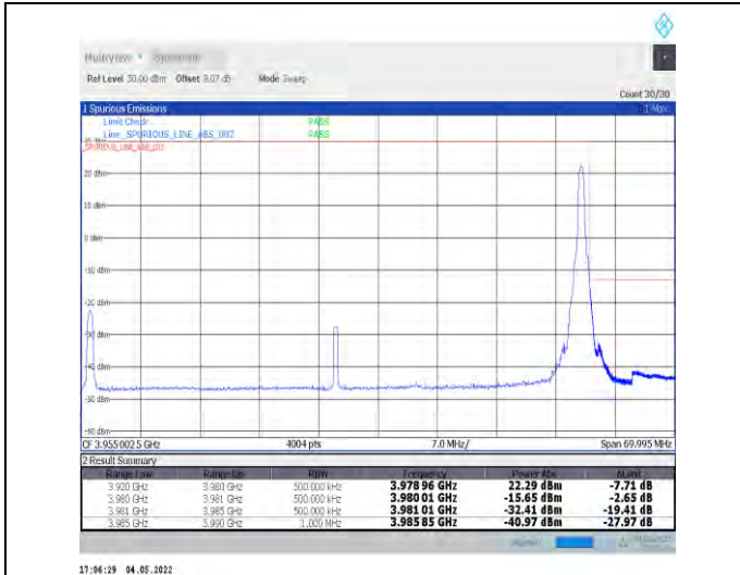
1-N77-3700-3980--30-60-H-2-DFT-PI2BPSK-Edge_1R_B_Right-1@161-Ant1-PASS-see graph
