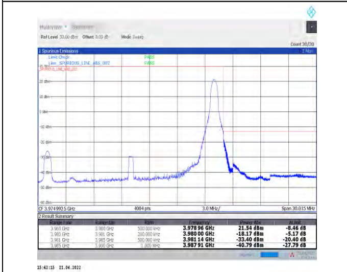
1-N77-3700-3980--30-20-H-5-CP-QPSK-Edge_1RB_R ight-1@50-Ant1-PASS-see graph
