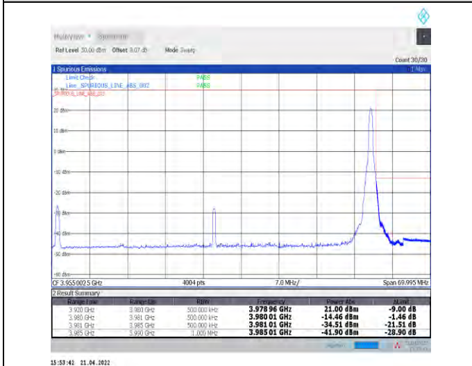
1-N77-3700-3980--30-60-H-5-CP-QPSK-Edge_1RB_Right-1@161-Ant1-PASS-see graph
