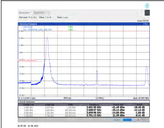
1-N77-3700-3980--30-40-L-4-CP-QPSK-Edge_1RB_L eft-1@0-Ant1-PASS-see graph
