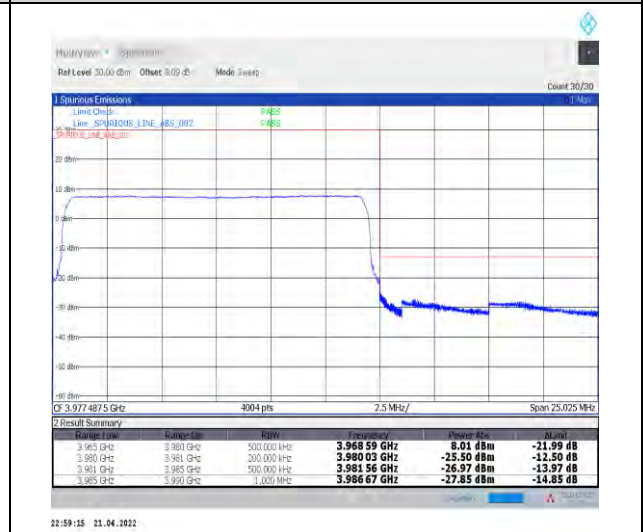
1-N77-3700-3980--30-15-H-6-CP-QPSK-Outer_Fu ll-38@0-Ant1-PASS-see graph
