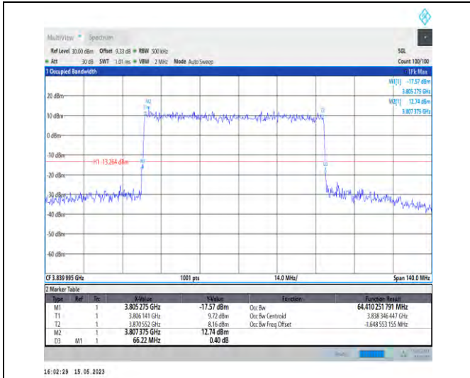
1-N77-3700-3980-PC1-30-70-M-3-DFT-16QAM-Outer_Full-180@0-Ant1-64.41-66.220-≤70-PASS
