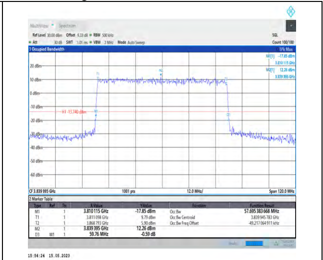
1-N77-3700-3980-PC1-30-60-M-7-CP-16QAM-Outer_Full-162@0-Ant1-57.695-59.760-≤60-PASS
