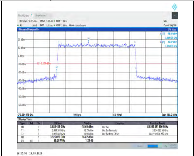
1-N77-3700-3980-PC1-30-90-H-1-DFT-QPSK-Outer_Full-240@0-Ant1-85.586-89.280-≤90-PASS
