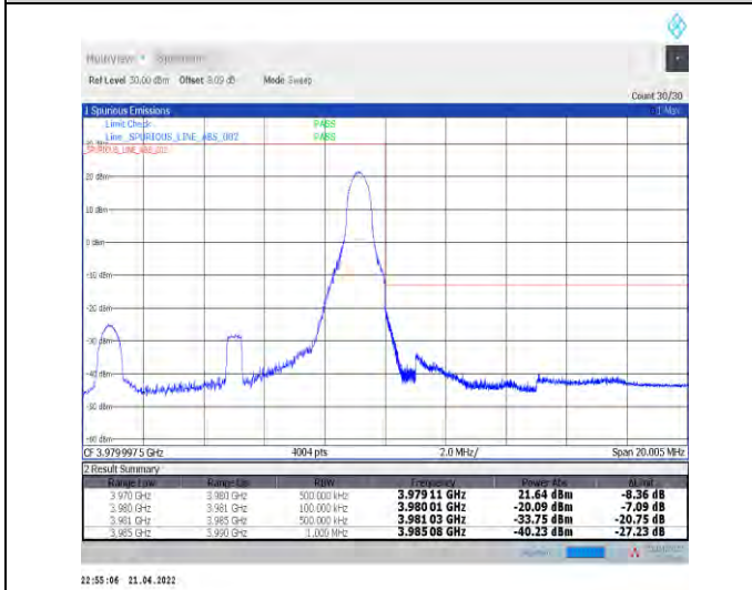
1-N77-3700-3980--30-10-H-5-CP-QPSK-Edge_1RB_R ight-1@23-Ant1-PASS-see graph
