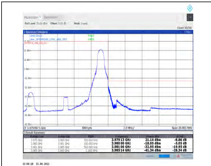
1-N77-3700-3980--30-10-H-2-DFT-PI2BPSK-Edge_1R_B_Right-1@23-Ant1-PASS-see graph
