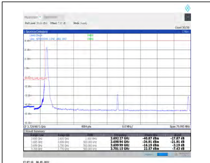
1-N77-3700-3980--30-70-L-1-DFT-PI2BPSK-Edge_1R_B_Left-1@0-Ant1-PASS-see graph
