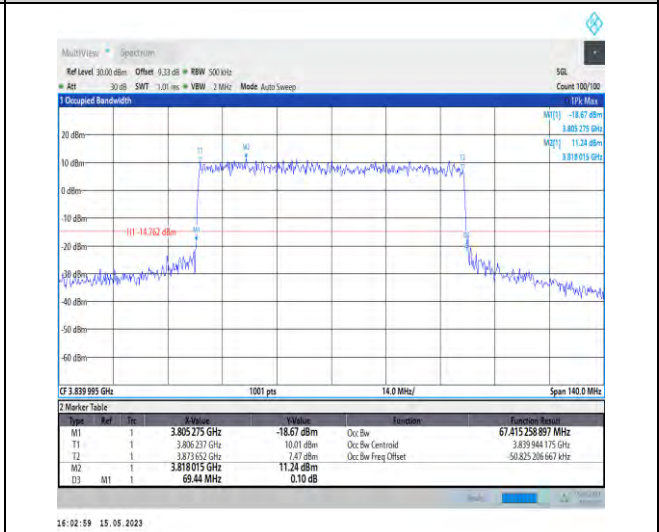
1-N77-3700-3980-PC1-30-70-M-6-CP-QPSK-Outer_Full-189@0-Ant1-67.415-69.440-≤70-PASS
