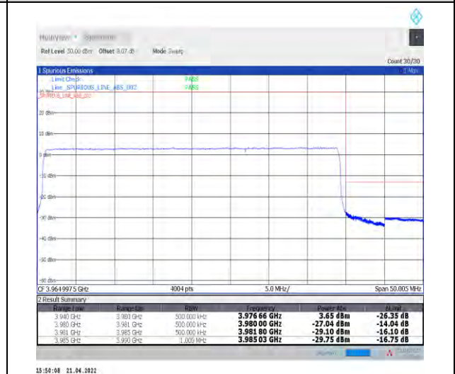
1-N77-3700-3980--30-40-H-6-CP-QPSK-Outer_Fu ll-106@0-Ant1-PASS-see graph
