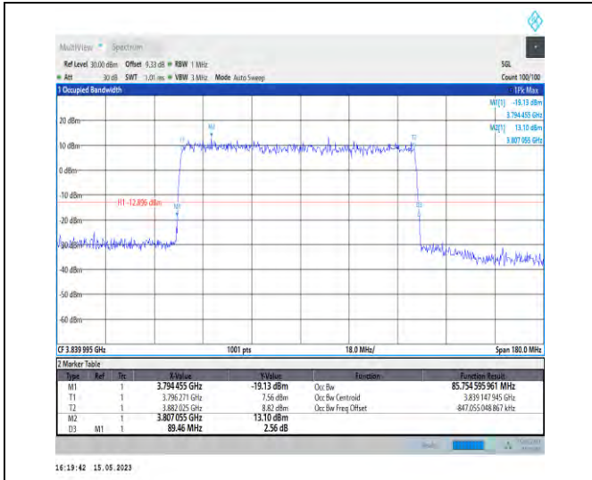
1-N77-3700-3980-PC1-30-90-M-5-DFT-256QAM-Outer_Full-240@0-Ant1-85.755-89.460-≤90-PASS
