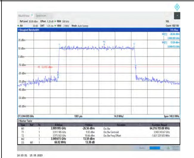
1-N77-3700-3980-PC1-30-70-H-1-DFT-QPSK-Outer_Full-180@0-Ant1-64.317-66.920-≤70-PASS
