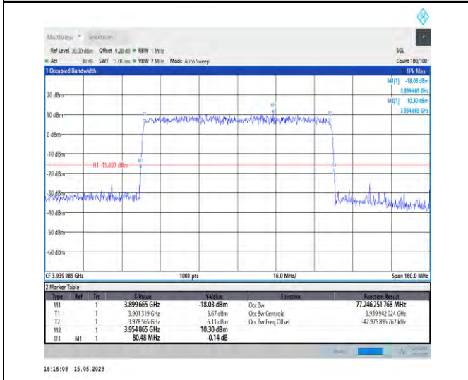
1-N77-3700-3980-PC1-30-80-H-9-CP-256QAM-Outer_Full-217@0-Ant1-77.246-80.480-≤80-PASS
