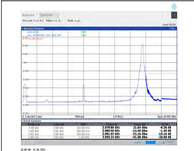
1-N77-3700-3980--30-40-H-5-CP-QPSK-Edge_1RB_R ight-1@105-Ant1-PASS-see graph
