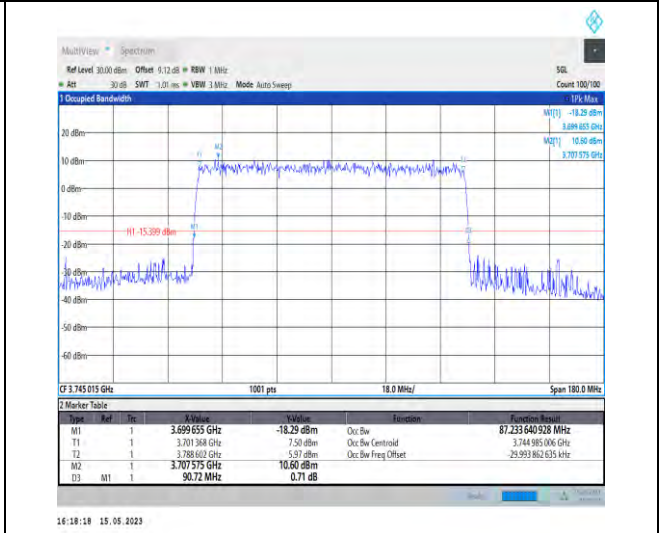
1-N77-3700-3980-PC1-30-90-L-9-CP-256QAM-Outer_Full-245@0-Ant1-87.234-90.720-<=90-PASS
