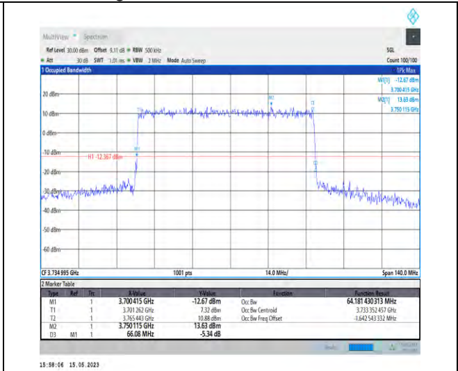
1-N77-3700-3980-PC1-30-70-L-1-DFT-QPSK-Outer_Full-180@0-Ant1-64.181-66.080-≤70-PASS
