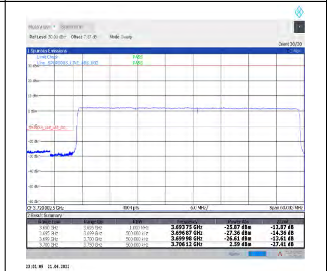
1-N77-3700-3980--30-50-L-6-CP-QPSK-Outer_Ful_I-133@0-Ant1-PASS-see graph
