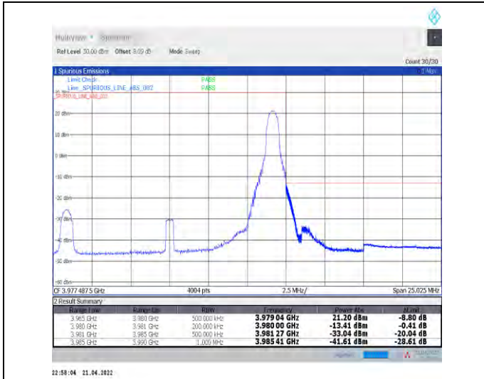
1-N77-3700-3980--30-15-H-2-DFT-PI2BPSK-Edge_1R_B_Right-1@37-Ant1-PASS-see graph
