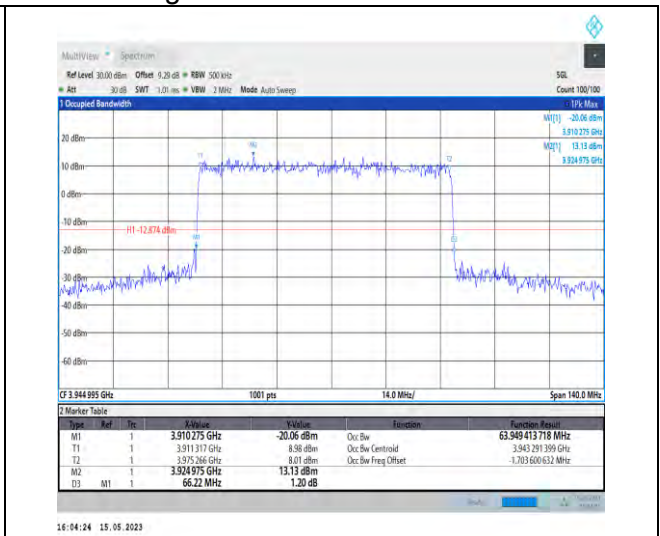
1-N77-3700-3980-PC1-30-70-H-3-DFT-16QAM-Out er_Full-180@0-Ant1-63.949-66.220-≤70-PASS
