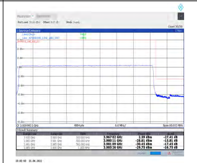
1-N77-3700-3980--30-50-H-6-CP-QPSK-Outer_Fu ll-133@0-Ant1-PASS-see graph
