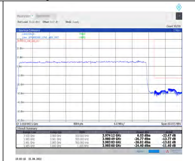
1-N77-3700-3980--30-50-H-3-DFT-PI2BPSK-Outer_Full-128@0-Ant1-PASS-see graph
