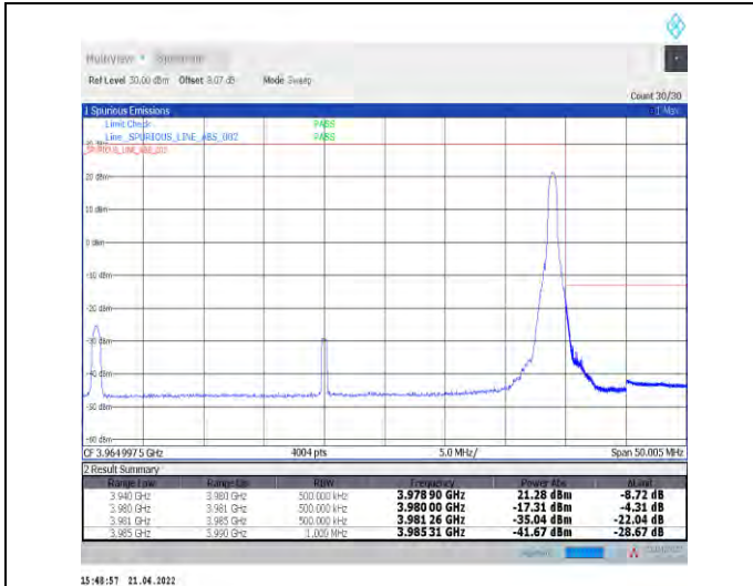
1-N77-3700-3980--30-40-H-2-DFT-PI2BPSK-Edge_1R_B_Right-1@105-Ant1-PASS-see graph
