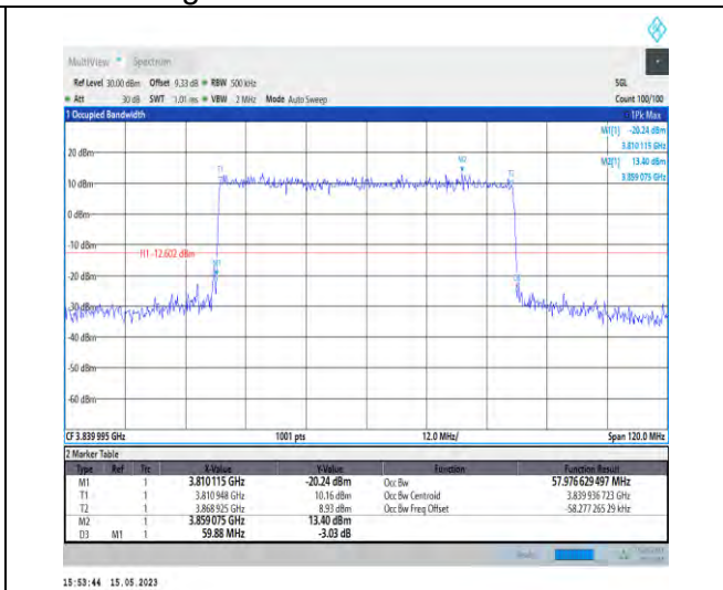
1-N77-3700-3980-PC1-30-60-M-3-DFT-16QAM-Out_Full-162@0-Ant1-57.977-59.880-≤60-PASS
