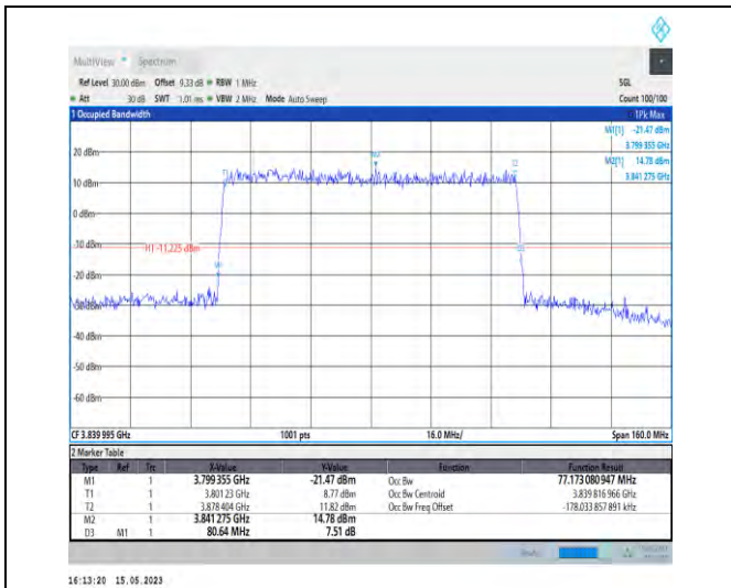
1-N77-3700-3980-PC1-30-80-M-4-DFT-64QAM-Outer_Full-216@0-Ant1-77.173-80.640-≤80-PASS
