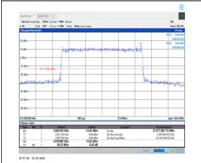
1-N77-3700-3980-PC1-30-60-H-7-CP-16QAM-Outer_Full-162@0-Ant1-57.677-59.520-≤60-PASS
