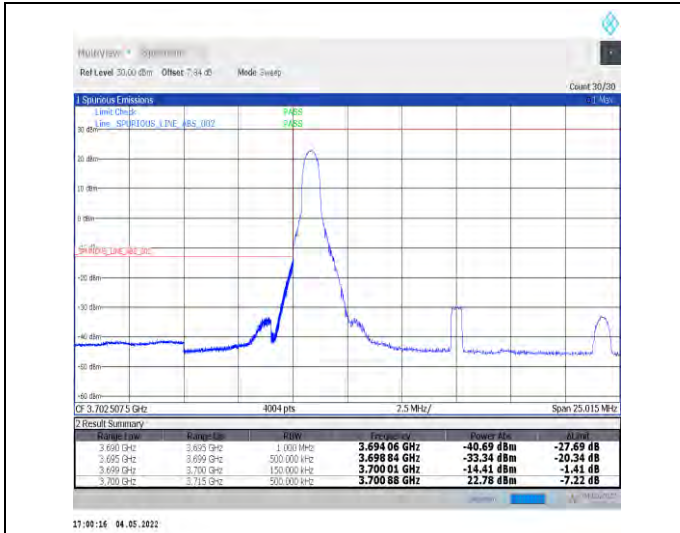
1-N77-3700-3980--30-15-L-1-DFT-PI2BPSK-Edge_1R_B_Left-1@0-Ant1-PASS-see graph
