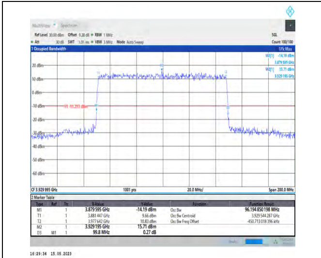
1-N77-3700-3980-PC1-30-100-H-1-DFT-QPSK-Outer_Full-270@0-Ant1-96.195-99.800-≤100-PASS
