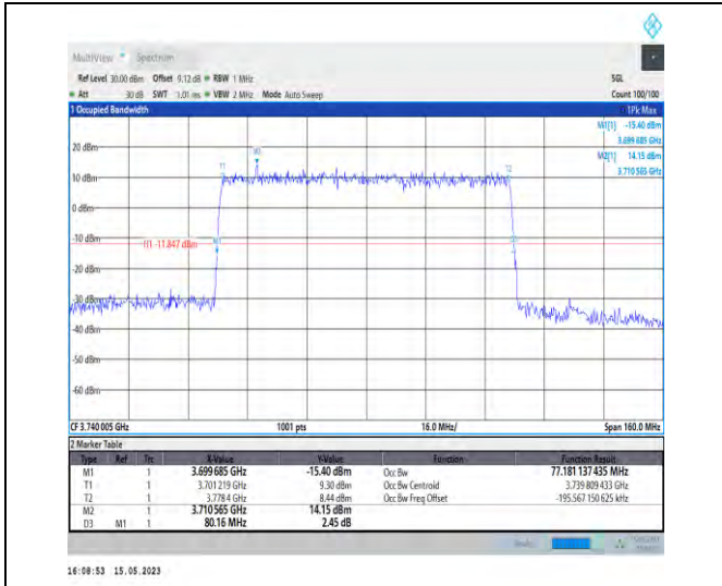
1-N77-3700-3980-PC1-30-80-L-5-DFT-256QAM-Out er_Full-216@0-Ant1-77.181-80.160-≤80-PASS
