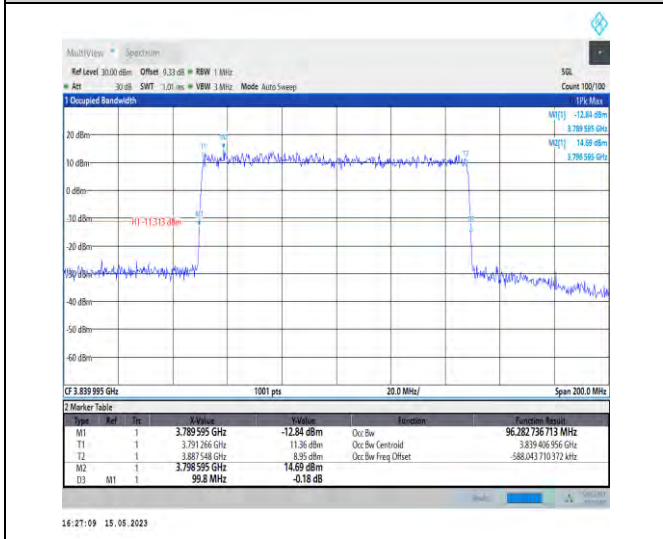
1-N77-3700-3980-PC1-30-100-M-4-DFT-64QAM-Out er_Full-270@0-Ant1-96.283-99.800-≤100-PASS
