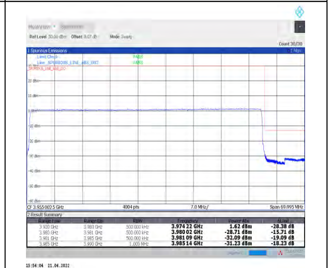
1-N77-3700-3980--30-60-H-6-CP-QPSK-Outer_Full-162@0-Ant1-PASS-see graph
