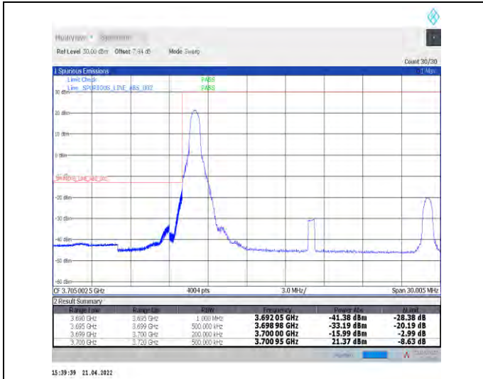
1-N77-3700-3980--30-20-L-1-DFT-PI2BPSK-Edge_1R_B_Left-1@0-Ant1-PASS-see graph
