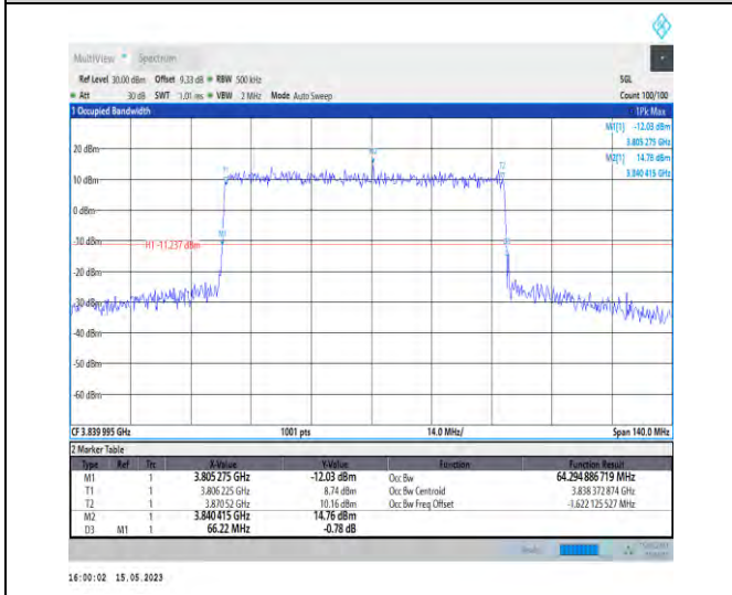
1-N77-3700-3980-PC1-30-70-M-1-DFT-QPSK-Outer_Full-180@0-Ant1-64.295-66.220-≤70-PASS
