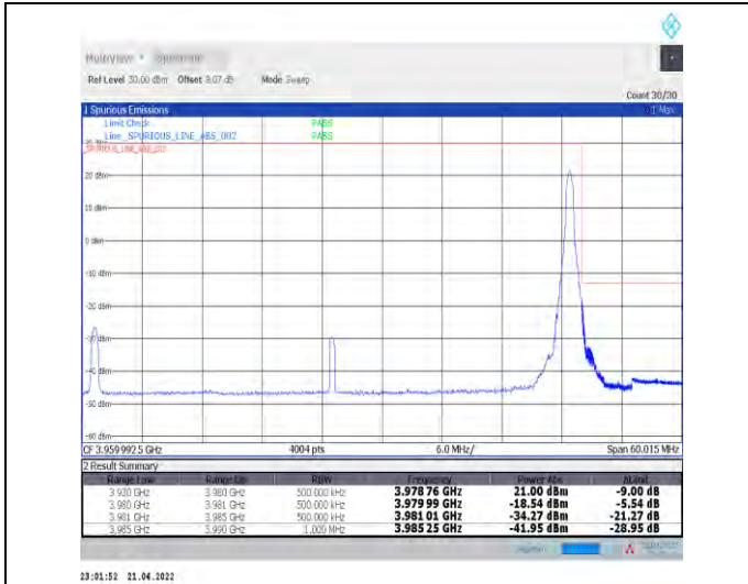
1-N77-3700-3980--30-50-H-2-DFT-PI2BPSK-Edge_1R_B_Right-1@132-Ant1-PASS-see graph
