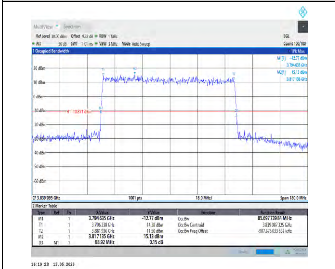
1-N77-3700-3980-PC1-30-90-M-3-DFT-16QAM-Outer_Full-240@0-Ant1-85.698-88.920-≤90-PASS
