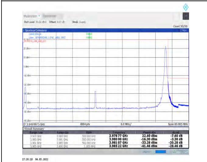
1-N77-3700-3980--30-70-H-5-CP-QPSK-Edge_1RB_R ight-1@188-Ant1-PASS-see graph
