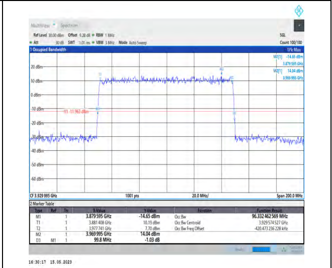
1-N77-3700-3980-PC1-30-100-H-4-DFT-64QAM-Outer_Full-270@0-Ant1-96.332-99.800-≤100-PASS
