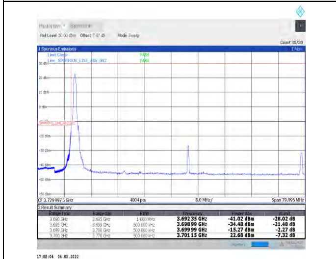
1-N77-3700-3980--30-70-L-4-CP-QPSK-Edge_1RB_L_eff-1@0-Ant1-PASS-see graph
