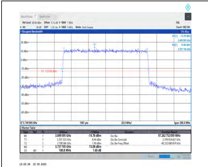
1-N77-3700-3980-PC1-30-100-L-7-CP-16QAM-Outer_Full-273@0-Ant1-97.263-100.800-≤100-PASS
