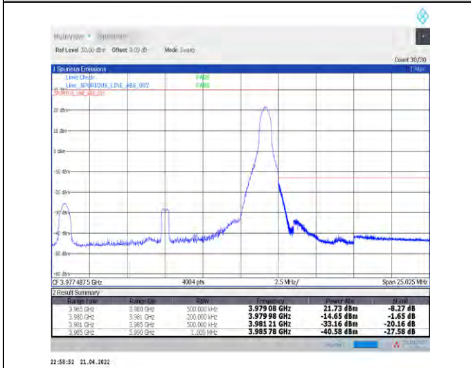
1-N77-3700-3980--30-15-H-5-CP-QPSK-Edge_1RB_R ight-1@37-Ant1-PASS-see graph
