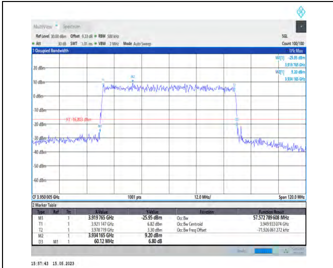
1-N77-3700-3980-PC1-30-60-H-9-CP-256QAM-Outer_Full-162@0-Ant1-57.573-60.120-≤60-PASS
