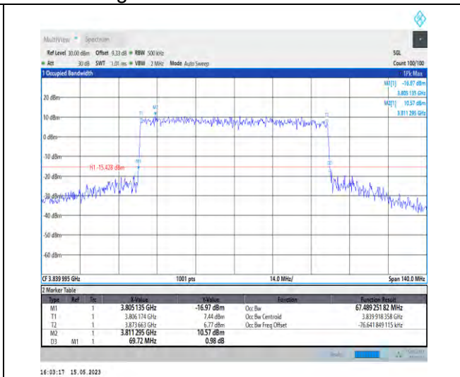
1-N77-3700-3980-PC1-30-70-M-8-CP-64QAM-Outer_Full-189@0-Ant1-67.489-69.720-≤70-PASS
