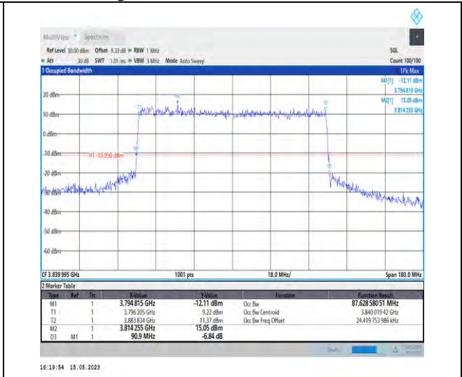
1-N77-3700-3980-PC1-30-90-M-6-CP-QPSK-Outer_Full-245@0-Ant1-87.629-90.900-≤90-PASS
