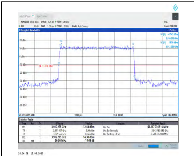
1-N77-3700-3980-PC1-30-70-H-2-DFT-PI2BPSK-Out er_Full-180@0-Ant1-64.148-66.360-≤70-PASS
