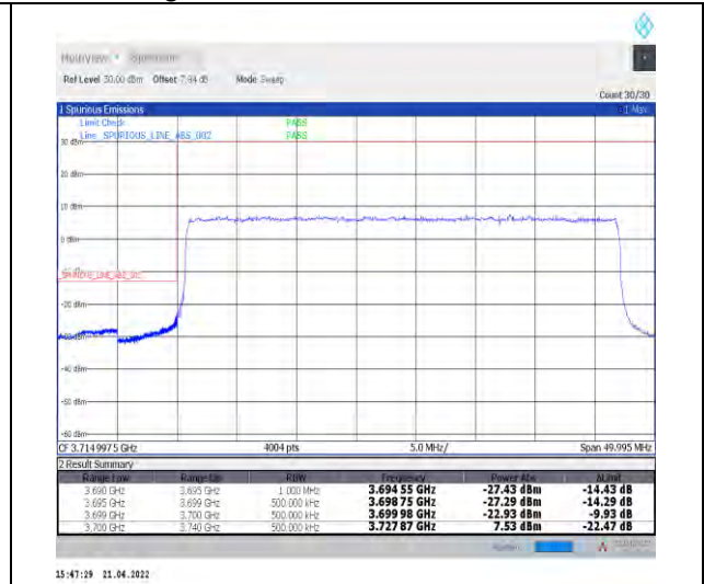
1-N77-3700-3980--30-40-L-3-DFT-PI2BPSK-Outer _Full-100@0-Ant1-PASS-see graph
