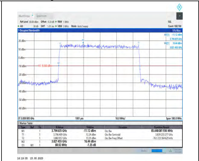
1-N77-3700-3980-PC1-30-90-M-2-DFT-PI2BPSK-Outer_Full-240@0-Ant1-85.648-88.920-≤90-PASS
