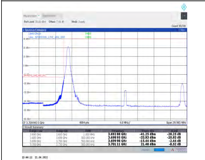
1-N77-3700-3980--30-30-L-4-CP-QPSK-Edge_1RB_L_eft-1@0-Ant1-PASS-see graph
