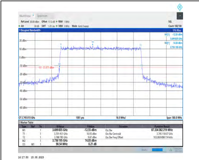
1-N77-3700-3980-PC1-30-90-L-6-CP-QPSK-Outer_Full-245@0-Ant1-87.334-90.540-<=90-PASS
