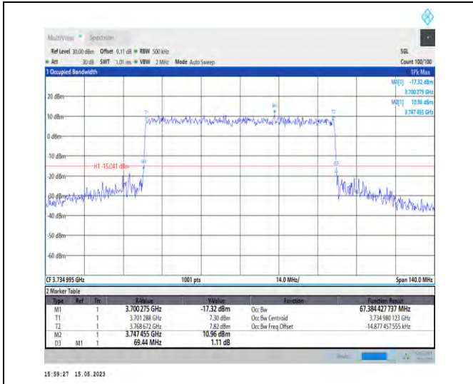
1-N77-3700-3980-PC1-30-70-L-8-CP-64QAM-Outer_Full-189@0-Ant1-67.384-69.440-≤70-PASS
