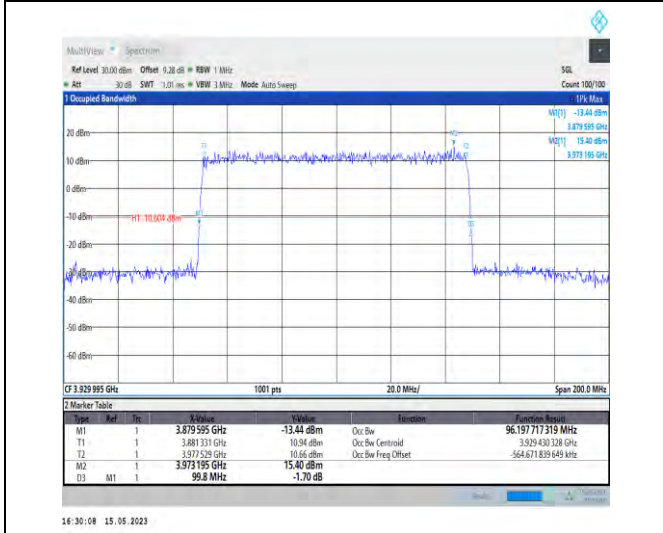
1-N77-3700-3980-PC1-30-100-H-3-DFT-16QAM-Outer_Full-270@0-Ant1-96.198-99.800-≤100-PASS
