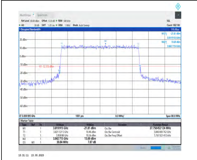
1-N77-3700-3980-PC1-30-40-M-6-CP-QPSK-Outer_Full-106@0-Ant1-37.758-39.840-≤40-PASS
