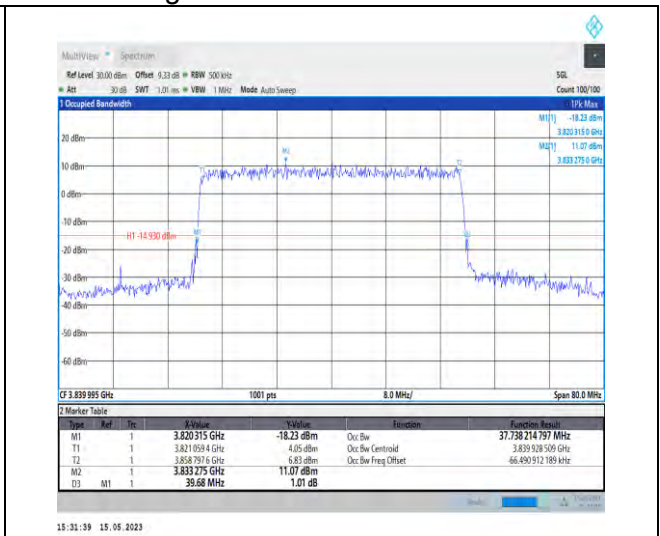
1-N77-3700-3980-PC1-30-40-M-9-CP-256QAM-Outer_Full-106@0-Ant1-37.738-39.680-≤40-PASS
