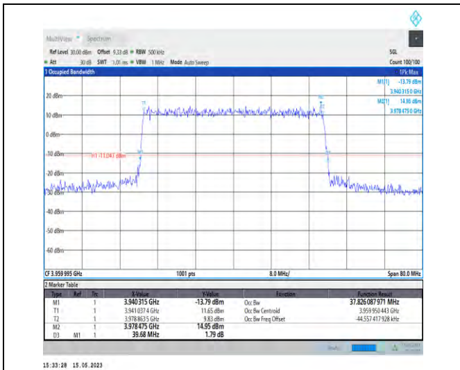
1-N77-3700-3980-PC1-30-40-H-7-CP-16QAM-Outer_Full-106@0-Ant1-37.826-39.680-≤40-PASS
