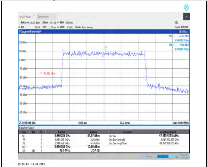
1-N77-3700-3980-PC1-30-50-H-9-CP-256QAM-Outer_Full-133@0-Ant1-47.415-49.600-≤50-PASS
