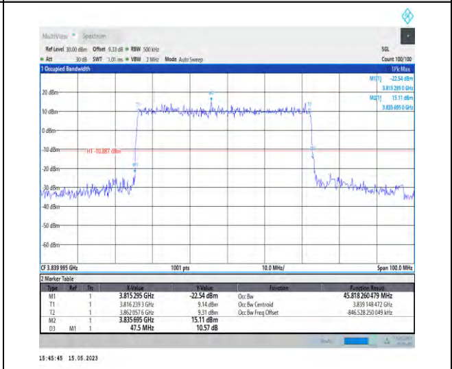
1-N77-3700-3980-PC1-30-50-M-4-DFT-64QAM-Outer_Full-128@0-Ant1-45.818-47.500-≤50-PASS
