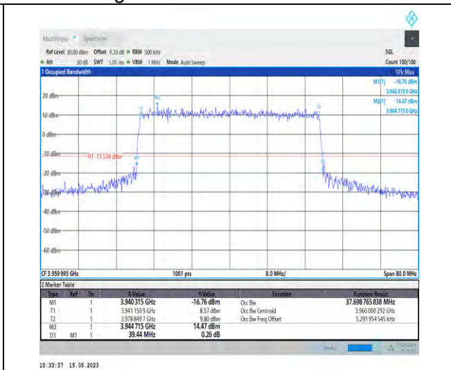
1-N77-3700-3980-PC1-30-40-H-8-CP-64QAM-Outer_Full-106@0-Ant1-37.699-39.440-≤40-PASS
