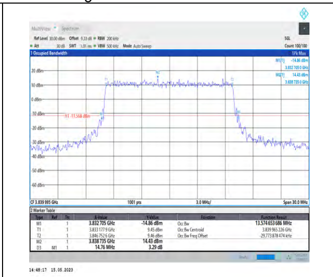
1-N77-3700-3980-PC1-30-15-M-6-CP-QPSK-Outer_Full-38@0-Ant1-13.575-14.760-≤15-PASS
