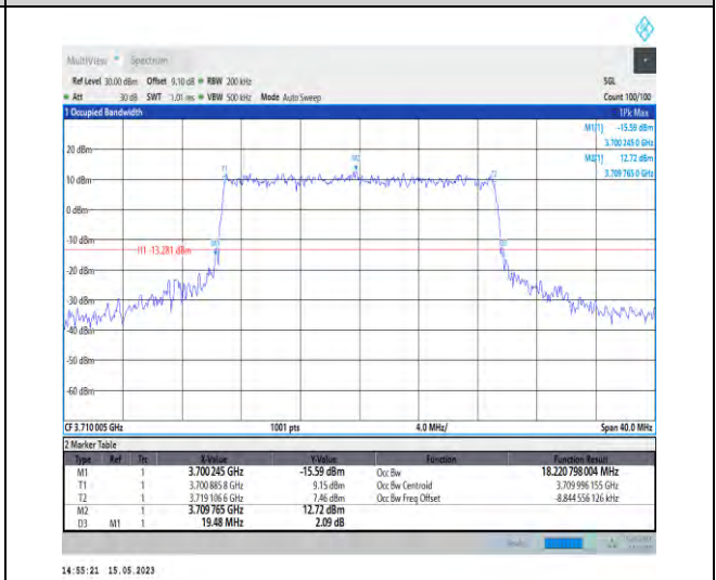
1-N77-3700-3980-PC1-30-20-L-6-CP-QPSK-Outer_Full-51@0-Ant1-18.221-19.480-≤20-PASS
