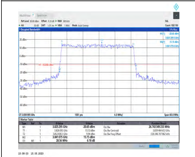
1-N77-3700-3980-PC1-30-30-M-1-DFT-QPSK-Outer_Full-75@0-Ant1-26.743-28.560-≤30-PASS
