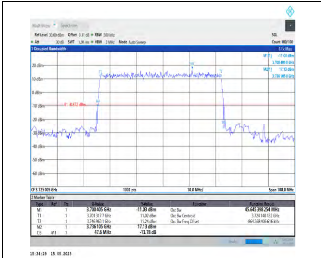
1-N77-3700-3980-PC1-30-50-L-2-DFT-PI2BPSK-Out er_Full-128@0-Ant1-45.645-47.600-<math>\leq 50</math>-PASS
