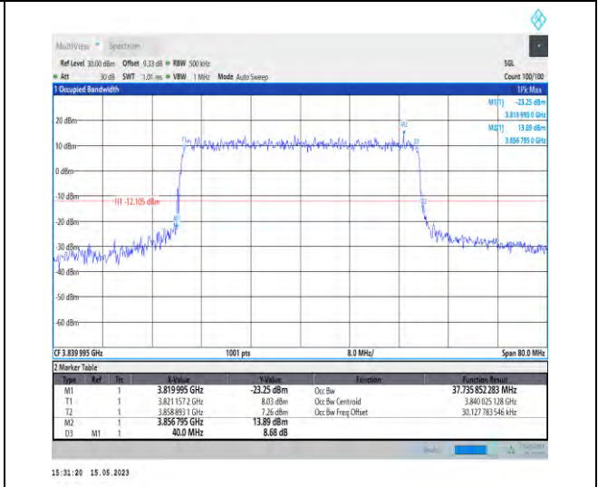
1-N77-3700-3980-PC1-30-40-M-7-CP-16QAM-Outer_Full-106@0-Ant1-37.736-40.000-≤40-PASS
