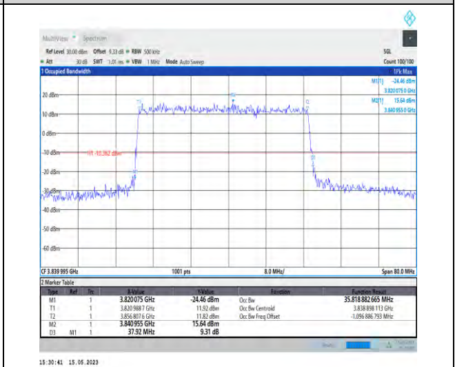
1-N77-3700-3980-PC1-30-40-M-3-DFT-16QAM-Outer_Full-100@0-Ant1-35.819-37.920-≤40-PASS
