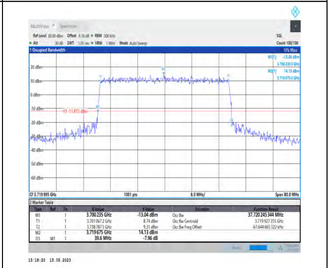
1-N77-3700-3980-PC1-30-40-L-8-CP-64QAM-Outer_Full-106@0-Ant1-37.72-39.600-≤40-PASS
