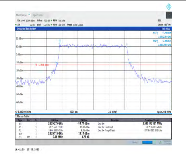
1-N77-3700-3980-PC1-30-10-M-3-DFT-16QAM-Outer_Full-24@0-Ant1-8.596-9.480-≤10-PASS
