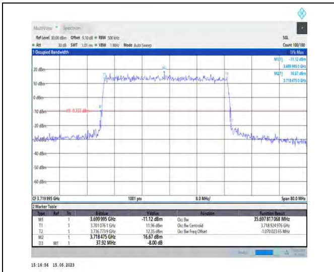
1-N77-3700-3980-PC1-30-40-L-1-DFT-QPSK-Outer_Full-100@0-Ant1-35.698-37.920-≤40-PASS
