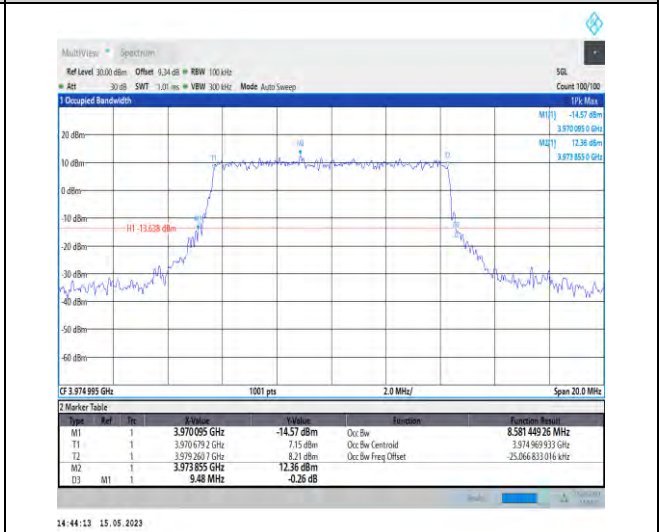
1-N77-3700-3980-PC1-30-10-H-6-CP-QPSK-Outer_Full-24@0-Ant1-8.581-9.480-≤10-PASS
