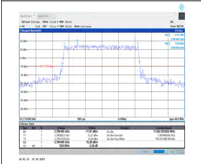
1-N77-3700-3980-PC1-30-20-L-1-DFT-QPSK-Outer_Full-50@0-Ant1-17.832-18.800-≤20-PASS
