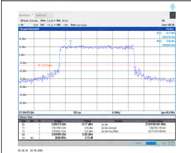
1-N77-3700-3980-PC1-30-30-H-8-CP-64QAM-Outer_Full-78@0-Ant1-27.811-28.860-≤30-PASS
