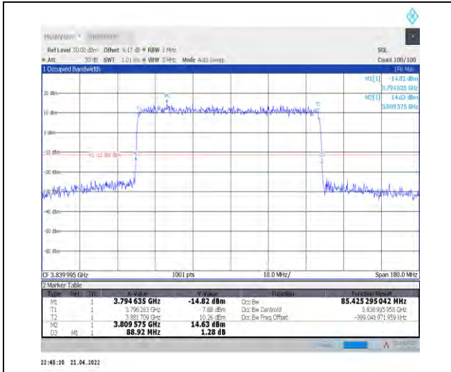
1-N77-3700-3980--30-90-M-1-DFT-QPSK-Outer_Full -240@0-Ant1-85.425-88.920-≤90-PASS
