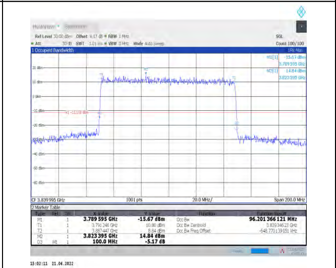
1-N77-3700-3980--30-100-M-1-DFT-QPSK-Outer_Fu I1-270@0-Ant1-96.201-100.000-≤100-PASS
