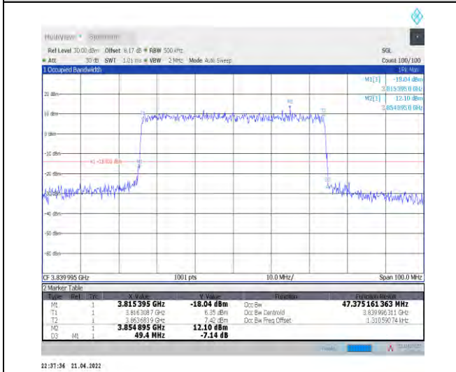
1-N77-3700-3980--30-50-M-7-CP-16QAM-Outer_Ful I-133@0-Ant1-47.375-49.400-≤50-PASS
