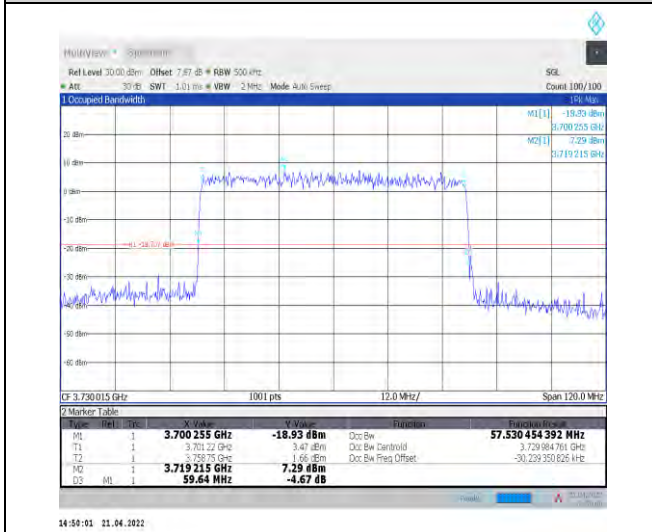
1-N77-3700-3980--30-60-L-9-CP-256QAM-Outer_Fu ll-162@0-Ant1-57.53-59.640-≤60-PASS
