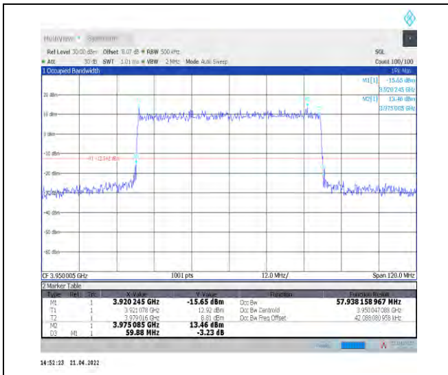
1-N77-3700-3980--30-60-H-1-DFT-QPSK-Outer_Full -162@0-Ant1-57.938-59.880-≤60-PASS
