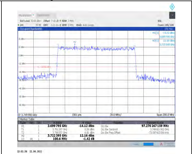
1-N77-3700-3980--30-100-L-8-CP-64QAM-Outer_Ful I-273@0-Ant1-97.27-100.600-≤100-PASS
