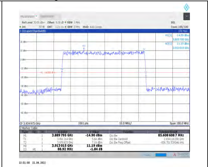
1-N77-3700-3980--30-90-H-5-DFT-256QAM-Outer_Full-240@0-Ant1-85.609-88.920-<=90-PASS
