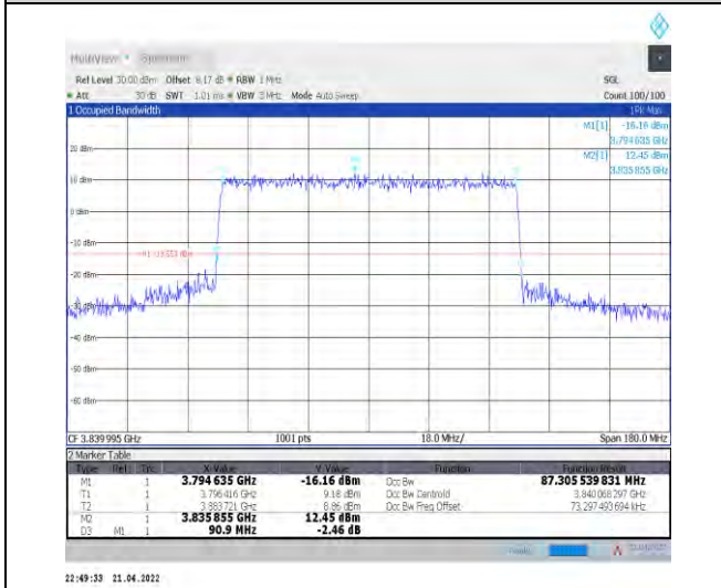
1-N77-3700-3980--30-90-M-7-CP-16QAM-Outer_Ful I-245@0-Ant1-87.306-90.900-≤90-PASS
