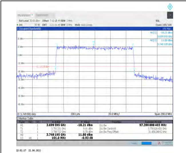
1-N77-3700-3980--30-100-L-7-CP-16QAM-Outer_Fu I1-273@0-Ant1-97.391-101.000-≤100-PASS
