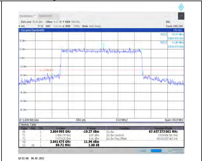
1-N77-3700-3980--30-70-M-8-CP-64QAM-Outer_Full -189@0-Ant1-67.457-69.720-≤70-PASS
