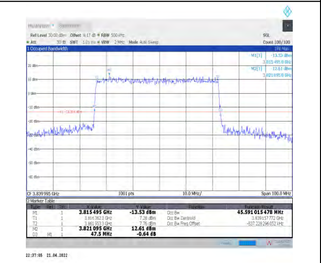
1-N77-3700-3980--30-50-M-4-DFT-64QAM-Outer_Full Full-128@0-Ant1-45.591-47.500-≤50-PASS
