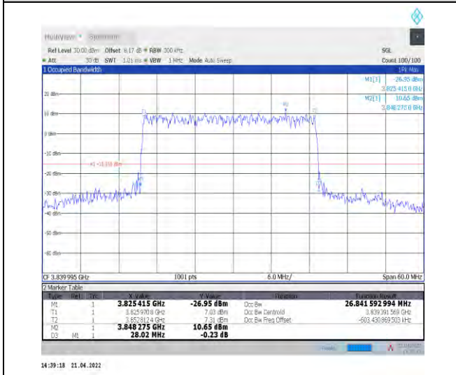
1-N77-3700-3980--30-30-M-5-DFT-256QAM-Outer_Full-75@0-Ant1-26.842-28.020-≤30-PASS
