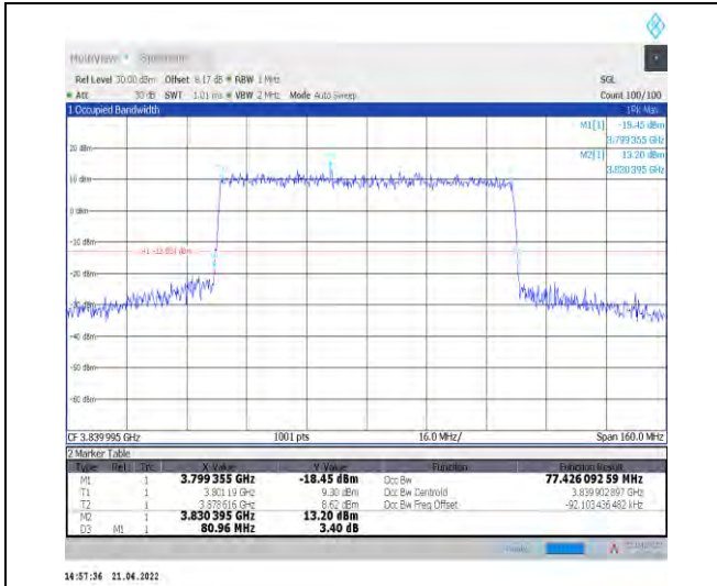
1-N77-3700-3980--30-80-M-8-CP-64QAM-Outer_Full I-217@0-Ant1-77.426-80.960-≤80-PASS
