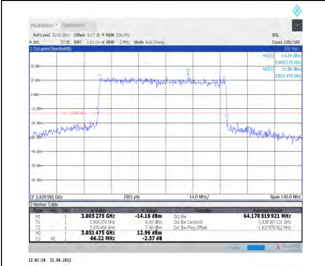
1-N77-3700-3980--30-70-M-1-DFT-QPSK-Outer_Full -180@0-Ant1-64.179-66.220-<math>\leq 70</math>-PASS
