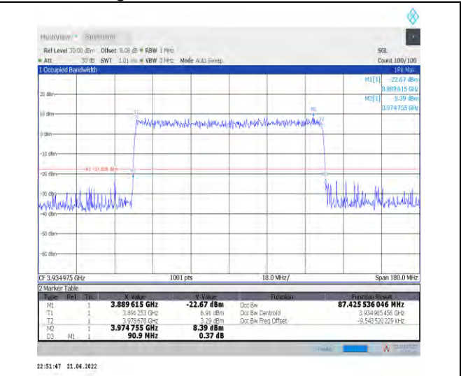
1-N77-3700-3980--30-90-H-9-CP-256QAM-Outer_Fu ll-245@0-Ant1-87.426-90.900-<=90-PASS
