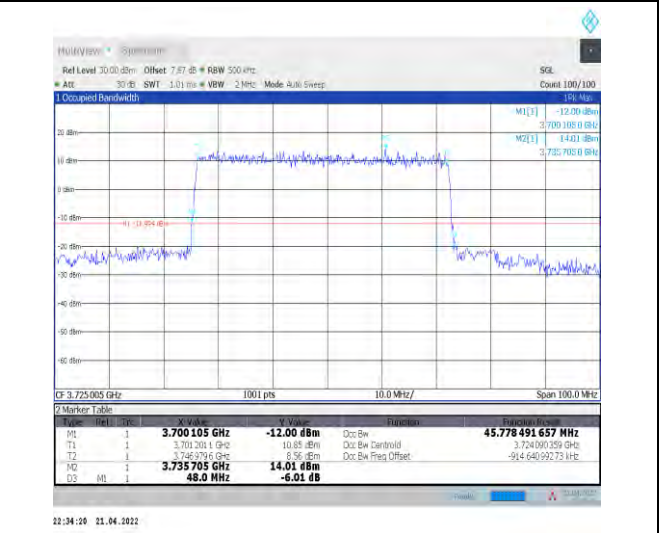
1-N77-3700-3980--30-50-L-1-DFT-QPSK-Outer_Full -128@0-Ant1-45.778-48.000≤50-PASS
