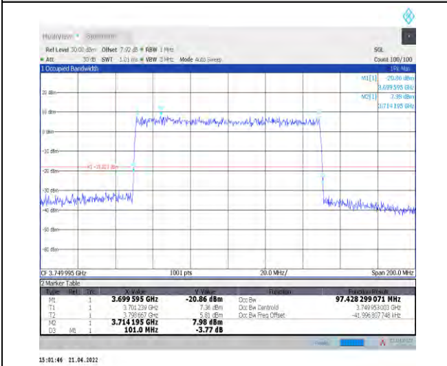
1-N77-3700-3980--30-100-L-9-CP-256QAM-Outer_F ull-273@0-Ant1-97.428-101.000-≤100-PASS
