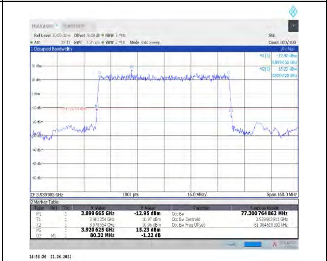
1-N77-3700-3980--30-80-H-2-DFT-PI2BPSK-Outer_Full Full-216@0-Ant1-77.301-80.320-≤80-PASS
