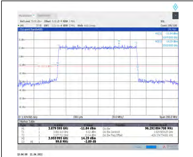
1-N77-3700-3980--30-100-H-1-DFT-QPSK-Outer_Fu II-270@0-Ant1-96.293-99.800-≤100-PASS
