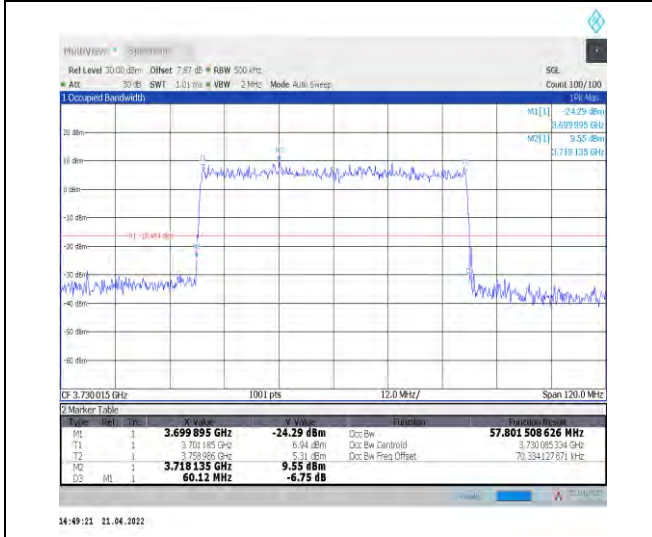
1-N77-3700-3980--30-60-L-5-DFT-256QAM-Outer_F ull-162@0-Ant1-57.802-60.120-≤60-PASS
