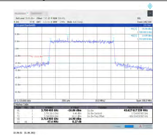
1-N77-3700-3980--30-50-L-3-DFT-16QAM-Outer_Full-128@0-Ant1-45.628-47.400-<math>\leq 50</math>-PASS
