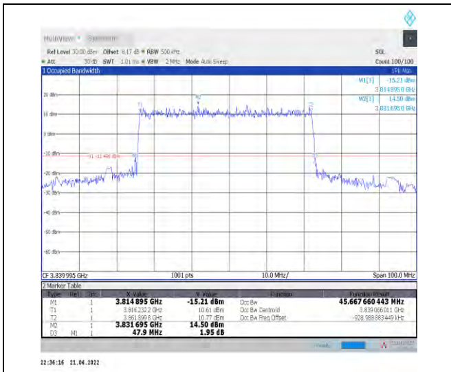
1-N77-3700-3980--30-50-M-1-DFT-QPSK-Outer_Full -128@0-Ant1-45.668-47.900-≤50-PASS
