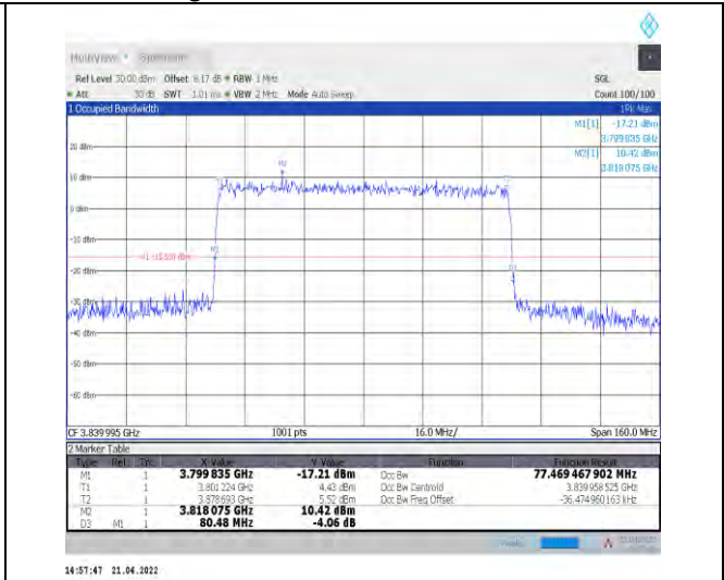
1-N77-3700-3980--30-80-M-9-CP-256QAM-Outer_Full ull-217@0-Ant1-77.469-80.480-≤80-PASS
