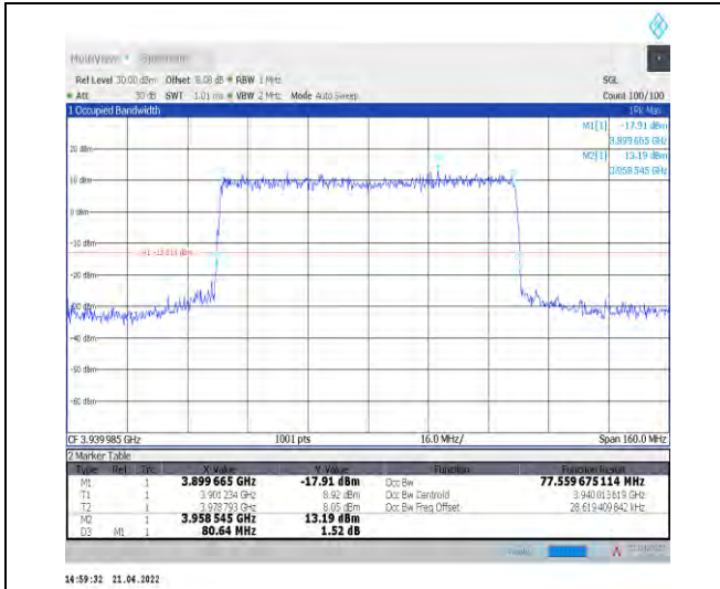
1-N77-3700-3980--30-80-H-7-CP-16QAM-Outer_Full -217@0-Ant1-77.56-80.640≤80-PASS
