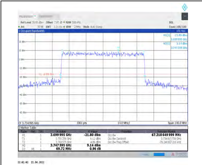
1-N77-3700-3980--30-70-L-8-CP-64QAM-Outer_Full -189@0-Ant1-67.319-69.720-<math>\leq 70</math>-PASS
