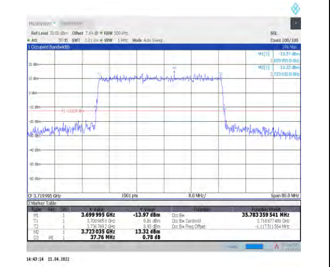
1-N77-3700-3980--30-40-L-4-DFT-64QAM-Outer_Full -100@0-Ant1-35.791-37.760-≤40-PASS
