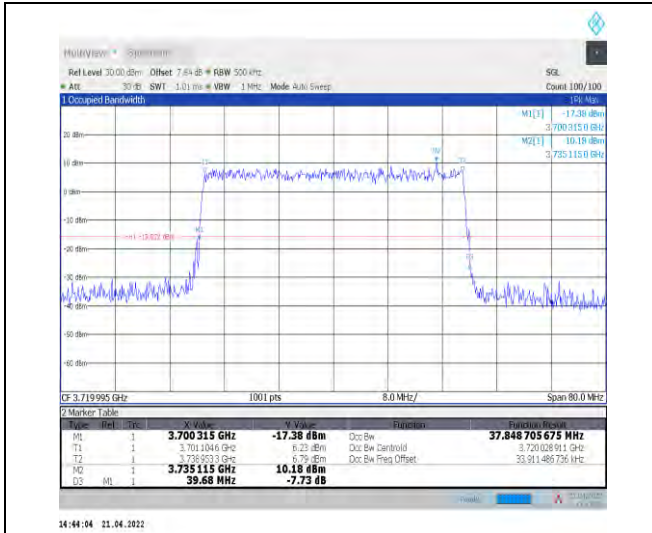
1-N77-3700-3980--30-40-L-9-CP-256QAM-Outer_Fu II-106@0-Ant1-37.853-39.680-≤40-PASS
