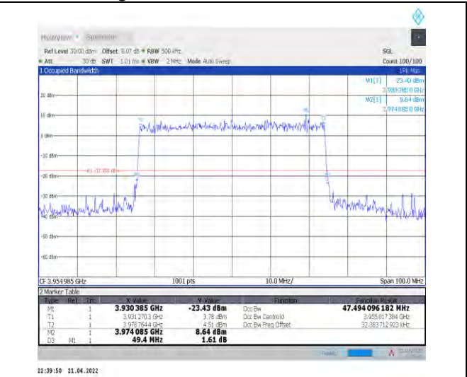
1-N77-3700-3980--30-50-H-9-CP-256QAM-Outer_Fu ll-133@0-Ant1-47.494-49.400-≤50-PASS
