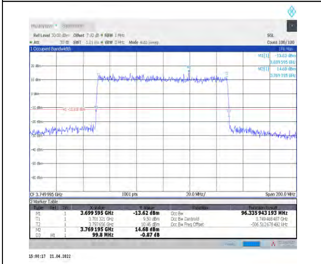
1-N77-3700-3980--30-100-L-1-DFT-QPSK-Outer_Fu ll-270@0-Ant1-96.336-99.800-<=100-PASS
