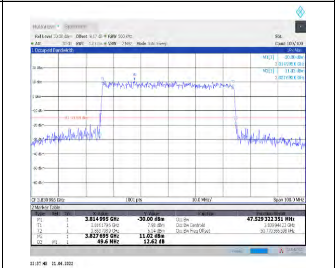
1-N77-3700-3980--30-50-M-8-CP-64QAM-Outer_Full -133@0-Ant1-47.529-49.600-≤50-PASS
