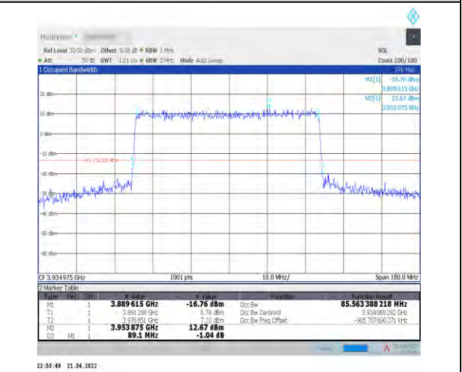
1-N77-3700-3980--30-90-H-3-DFT-16QAM-Outer_Full-240@0-Ant1-85.563-89.100-<math>\leq 90</math>-PASS
