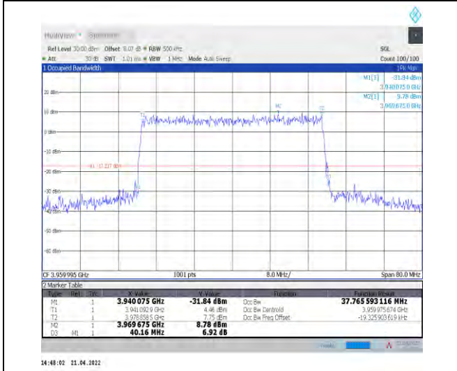
1-N77-3700-3980--30-40-H-9-CP-256QAM-Outer_Full -106@0-Ant1-37.692-40.160≤40-PASS
