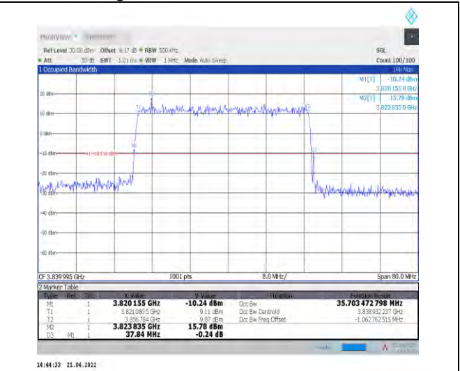
1-N77-3700-3980--30-40-M-1-DFT-QPSK-Outer_Full -100@0-Ant1-35.718-37.840-≤40-PASS
