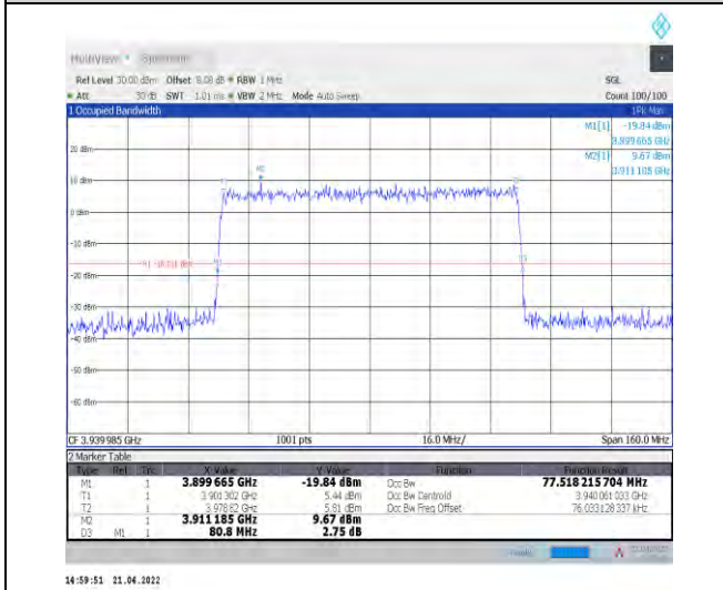
1-N77-3700-3980--30-80-H-9-CP-256QAM-Outer_Full -217@0-Ant1-77.518-80.800≤80-PASS
