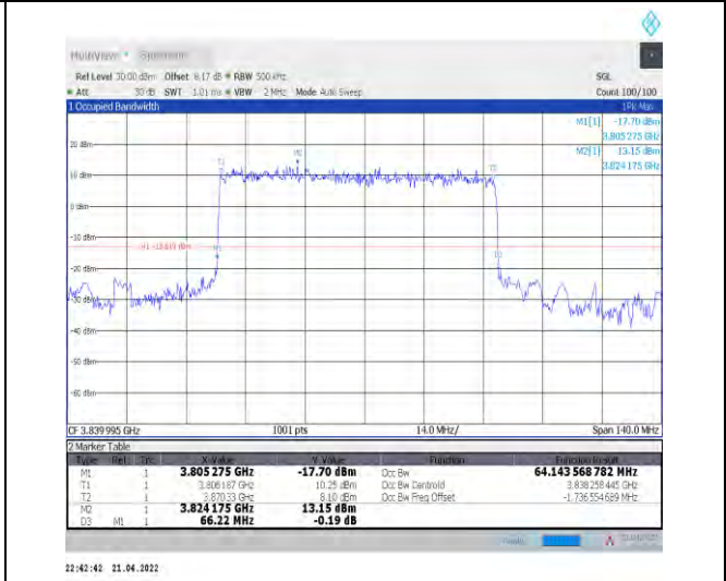
1-N77-3700-3980--30-70-M-2-DFT-PI2BPSK-Outer_Full Full-180@0-Ant1-64.144-66.220-<math>\leq 70</math>-PASS
