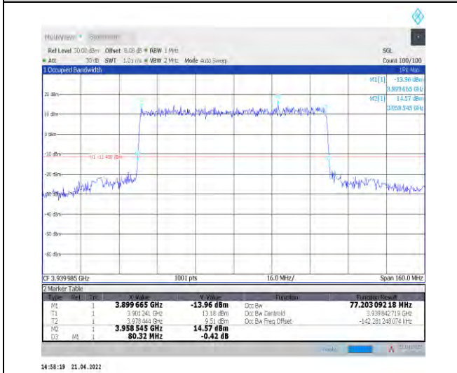
1-N77-3700-3980--30-80-H-1-DFT-QPSK-Outer_Full -216@0-Ant1-77.203-80.320-≤80-PASS
