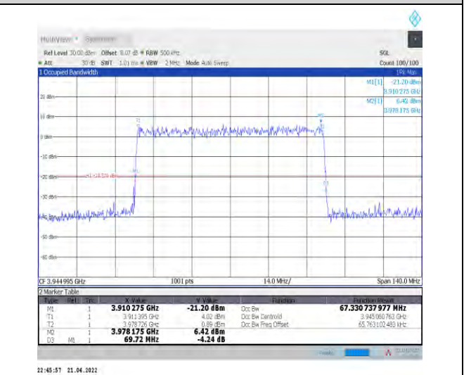
1-N77-3700-3980--30-70-H-9-CP-256QAM-Outer_Fu ll-189@0-Ant1-67.331-69.720-<=70-PASS
