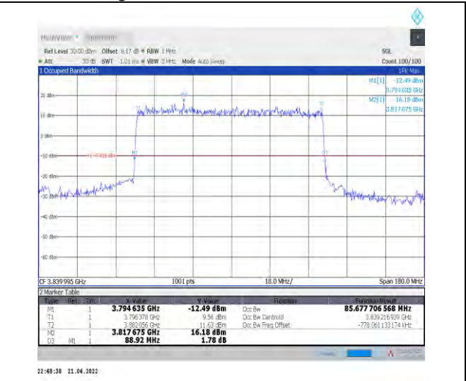
1-N77-3700-3980--30-90-M-2-DFT-PI2BPSK-Outer_Full -240@0-Ant1-85.678-88.920-≤90-PASS
