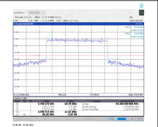
1-N77-3700-3980--30-70-L-3-DFT-16QAM-Outer_Full-180@0-Ant1-64.386-66.360-≤70-PASS
