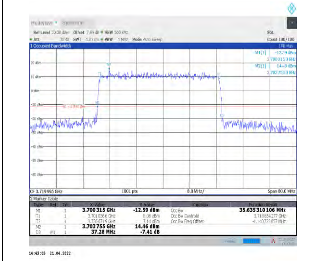
1-N77-3700-3980--30-40-L-3-DFT-16QAM-Outer_Full -100@0-Ant1-35.643-37.280-≤40-PASS
