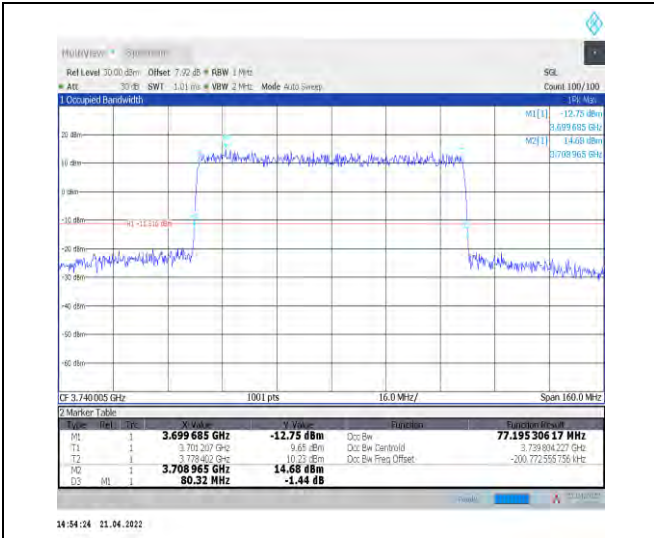
1-N77-3700-3980--30-80-L-1-DFT-QPSK-Outer_Full -216@0-Ant1-77.195-80.320-≤80-PASS
