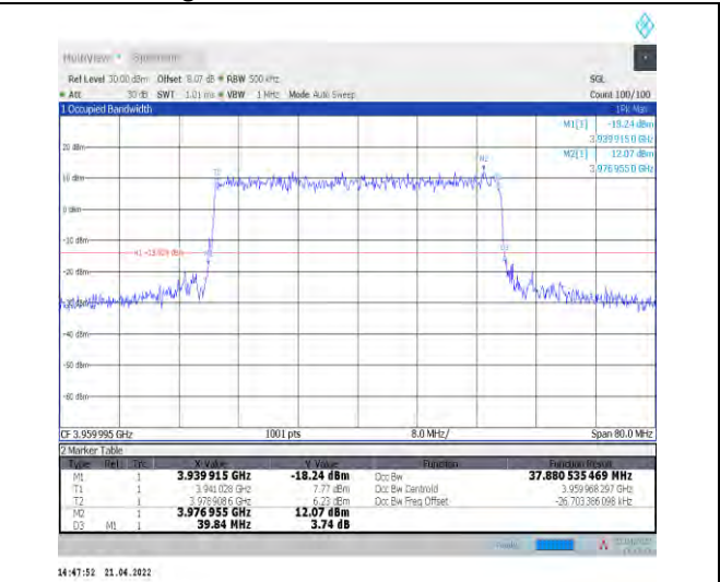
1-N77-3700-3980--30-40-H-8-CP-64QAM-Outer_Full -106@0-Ant1-37.892-39.840≤40-PASS
