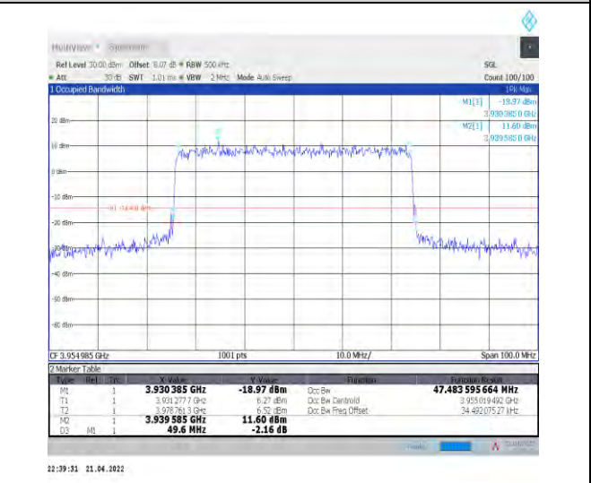
1-N77-3700-3980--30-50-H-7-CP-16QAM-Outer_Full-133@0-Ant1-47.484-49.600-<=50-PASS
