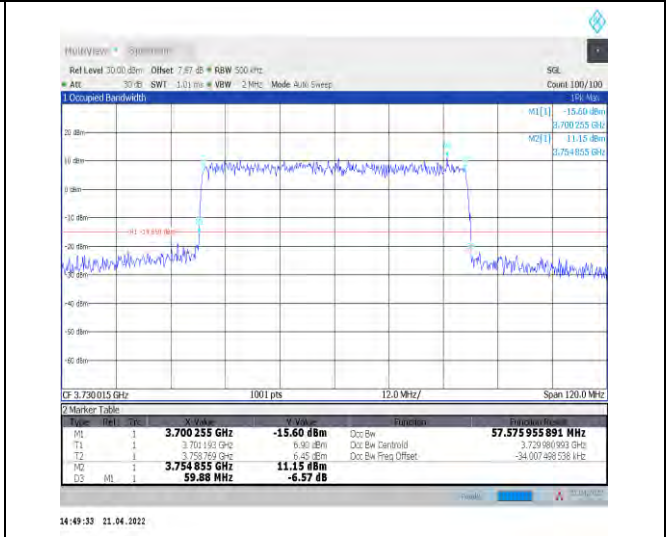
1-N77-3700-3980--30-60-L-6-CP-QPSK-Outer_Full-1 62@0-Ant1-57.576-59.880-≤60-PASS
