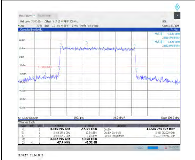
1-N77-3700-3980--30-50-M-3-DFT-16QAM-Outer_Full Full-128@0-Ant1-45.588-47.400-≤50-PASS
