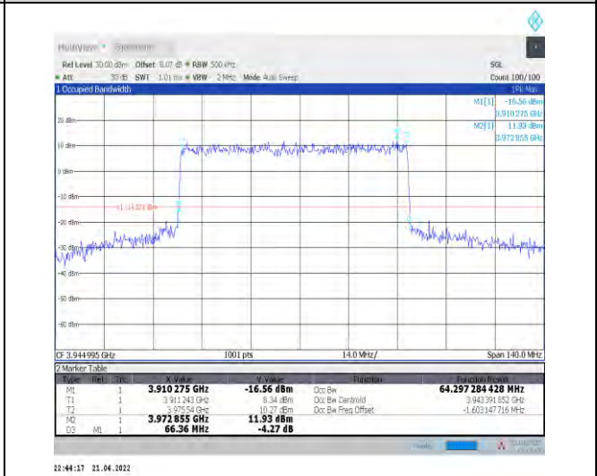
1-N77-3700-3980--30-70-H-1-DFT-QPSK-Outer_Full -180@0-Ant1-64.297-66.360-≤70-PASS
