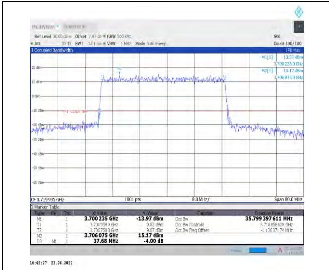
1-N77-3700-3980--30-40-L-1-DFT-QPSK-Outer_Full -100@0-Ant1-35.818-37.680-≤40-PASS
