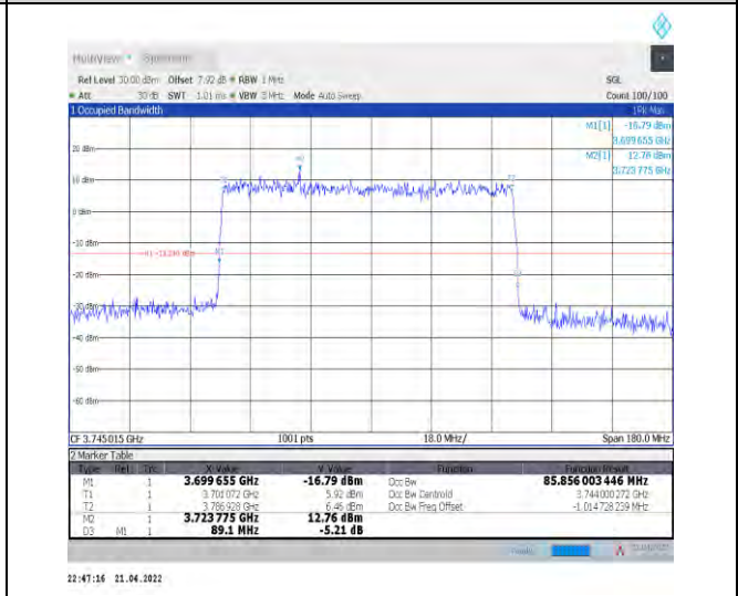
1-N77-3700-3980--30-90-L-5-DFT-256QAM-Outer_Full-240@0-Ant1-85.856-89.100-<=90-PASS
