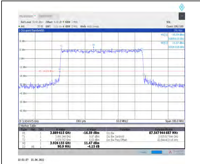
1-N77-3700-3980--30-90-H-8-CP-64QAM-Outer_Full -245@0-Ant1-87.548-90.900-<=90-PASS
