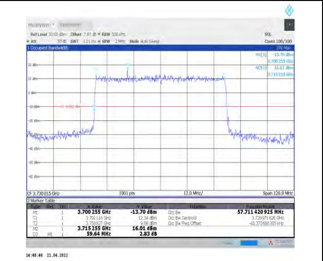
1-N77-3700-3980--30-60-L-2-DFT-PI2BPSK-Outer_F ull-162@0-Ant1-57.711-59.640-≤60-PASS
