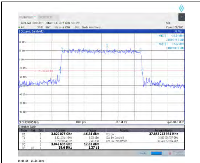
1-N77-3700-3980--30-40-M-8-CP-64QAM-Outer_Full-I-106@0-Ant1-37.826-39.600-≤40-PASS
