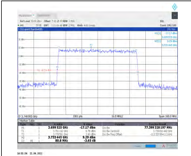
1-N77-3700-3980--30-80-L-9-CP-256QAM-Outer_Fu II-217@0-Ant1-77.399-80.800-<math>\leq 80</math>-PASS
