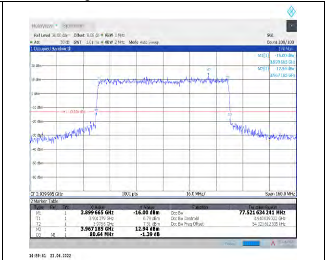
1-N77-3700-3980--30-80-H-8-CP-64QAM-Outer_Full -217@0-Ant1-77.522-80.640≤80-PASS
