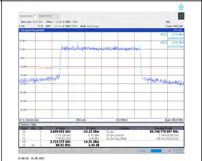
1-N77-3700-3980--30-90-L-1-DFT-QPSK-Outer_Full -240@0-Ant1-85.747-88.920≤90-PASS
