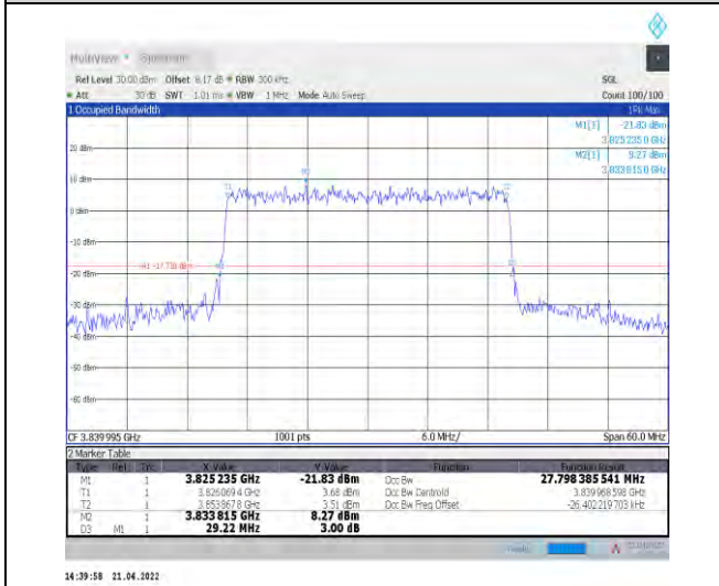
1-N77-3700-3980--30-30-M-9-CP-256QAM-Outer_Full I-78@0-Ant1-27.798-29.220-<30-PASS
