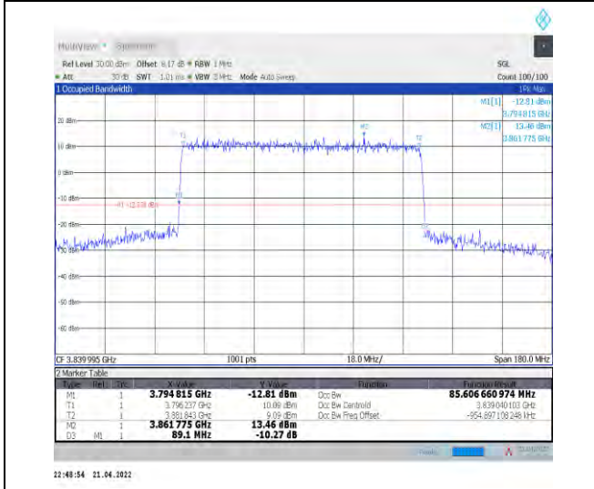
1-N77-3700-3980--30-90-M-3-DFT-16QAM-Outer_Full -240@0-Ant1-85.607-89.100-≤90-PASS
