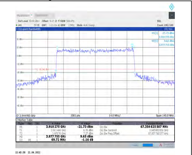
1-N77-3700-3980--30-70-H-7-CP-16QAM-Outer_Full-189@0-Ant1-67.355-69.720-<=70-PASS
