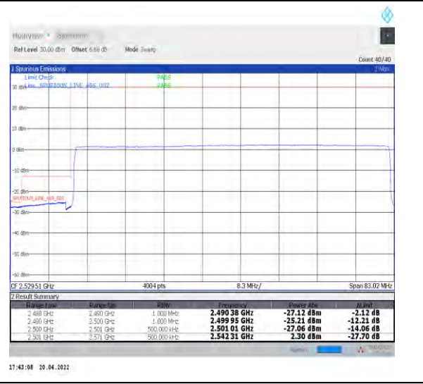
1-N41--30-70-L-6-CP-QPSK-Outer_Full-189@0-Ant1-PASS-see graph
