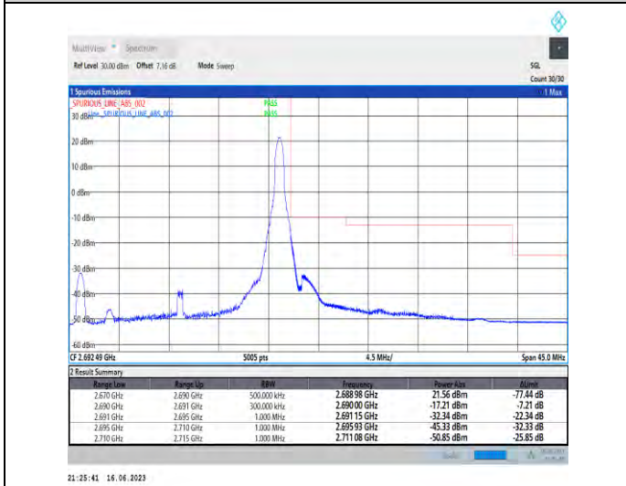
1-N41-PC1-30-20-H-5-CP-QPSK-Edge_1RB_Righ t-1@50-Ant1-1--PASS-see graph
