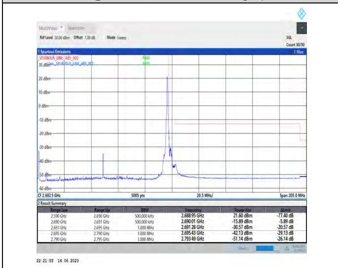
1-N41-PC1-30-100-H-5-CP-QPSK-Edge_1RB_Right-1 @272-Ant1-1--PASS-see graph
