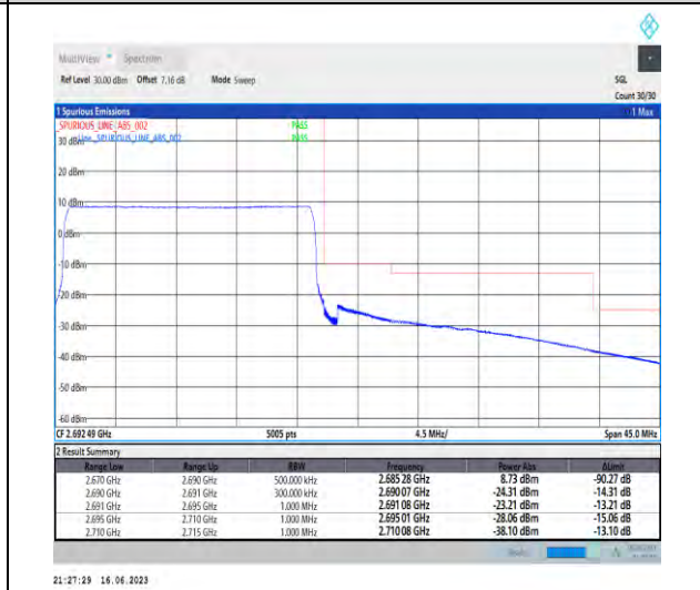
1-N41-PC1-30-20-H-6-CP-QPSK-Outer_Full-51 @0-Ant1-1--PASS-see graph
