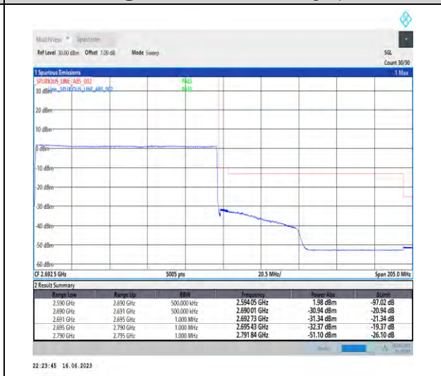
1-N41-PC1-30-100-H-6-CP-QPSK-Outer_Full-273 @0-Ant1-1--PASS-see graph
