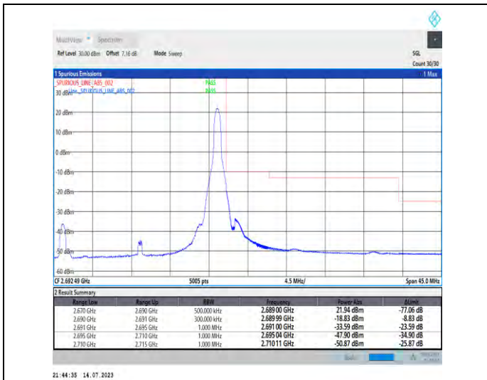
1-N41-PC1-30-20-H-2-DFT-PI2BPSK-Edge_1RB_Righ t-1@50-Ant1-1--PASS-see graph
