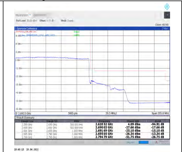
1-N41--30-100-H-3-DFT-PI2BPSK-Outer_Full-270 @0-Ant1-PASS-see graph
