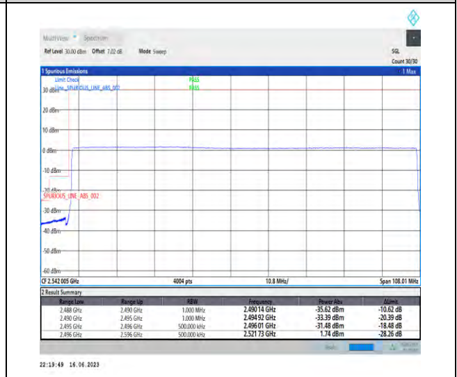
1-N41-PC1-30-100-L-6-CP-QPSK-Outer_Full-273@ 0-Ant1-1--PASS-see graph
