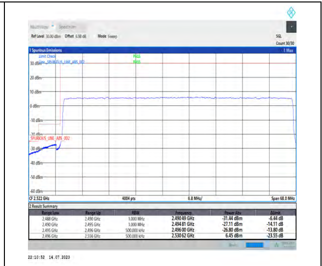
1-N41-PC1-30-60-L-3-DFT-PI2BPSK-Outer_Full-16 2@0-Ant1-1--PASS-see graph
