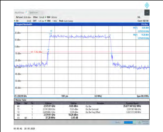
1-N41-PC1-30-40-M-1-DFT-QPSK-Outer_Full-100@ 0-Ant1-35.677-37.280-≤40-PASS
