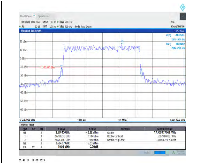
1-N41-PC1-30-20-H-3-DFT-16QAM-Outer_Full-50@ 0-Ant1-17.959-19.040-≤20-PASS
