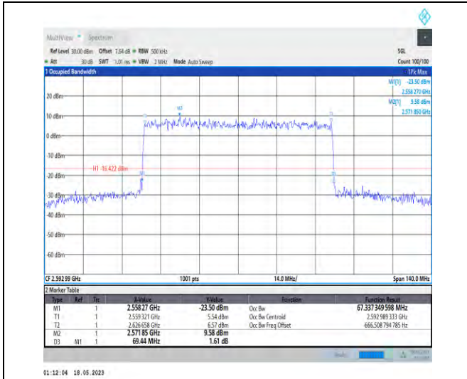
1-N41-PC1-30-70-M-9-CP-256QAM-Outer_Full-189 @0-Ant1-67.337-69.440-≤70-PASS
