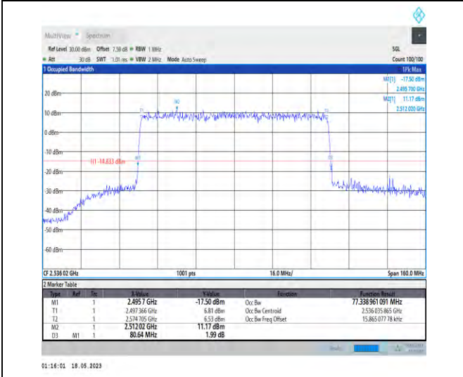
1-N41-PC1-30-80-L-9-CP-256QAM-Outer_Full-217 @0-Ant1-77.339-80.640-≤80-PASS
