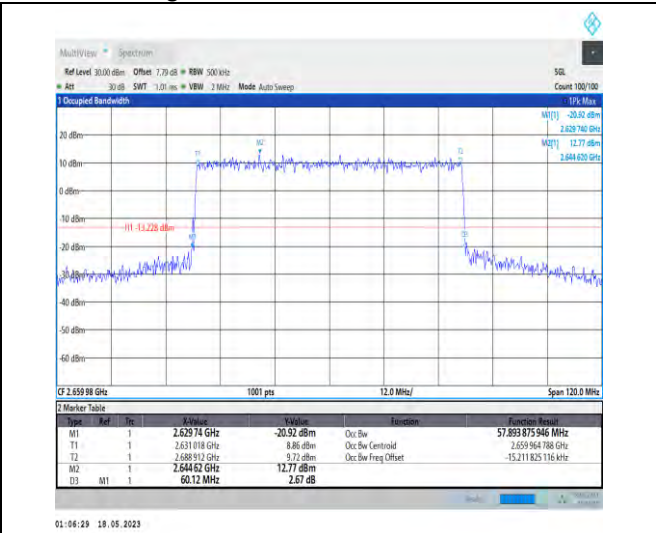
1-N41-PC1-30-60-H-8-CP-64QAM-Outer_Full-162@ 0-Ant1-57.894-60.120-≤60-PASS
