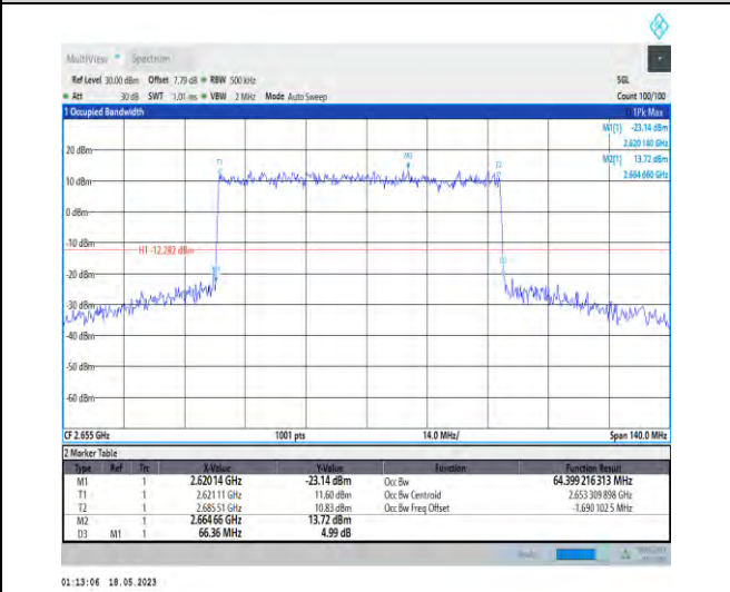
1-N41-PC1-30-70-H-3-DFT-16QAM-Outer_Full-180 @0-Ant1-64.399-66.360-≤70-PASS
