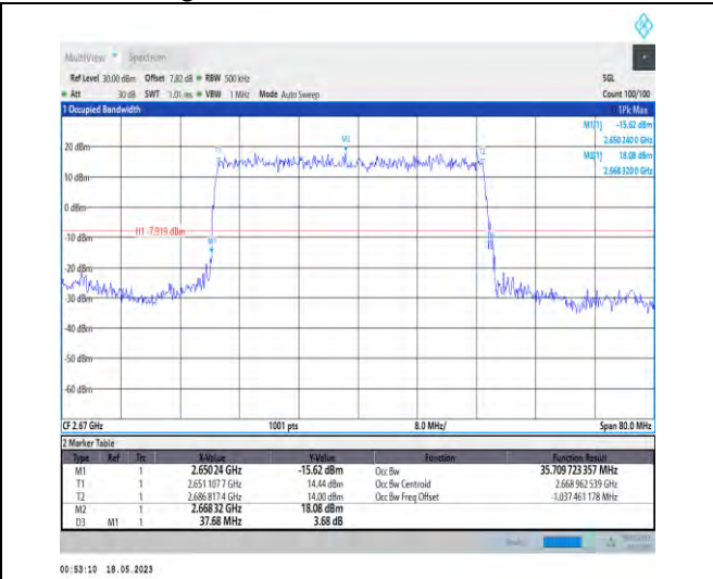
1-N41-PC1-30-40-H-2-DFT-PI2BPSK-Outer_Full-100@ 0-Ant1-35.71-37.680-≤40-PASS
