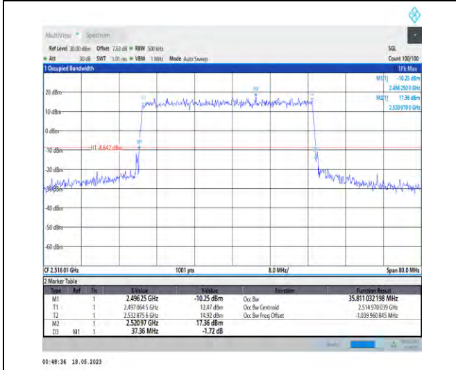
1-N41-PC1-30-40-L-1-DFT-QPSK-Outer_Full-100@0 -Ant1-35.811-37.360-≤40-PASS
