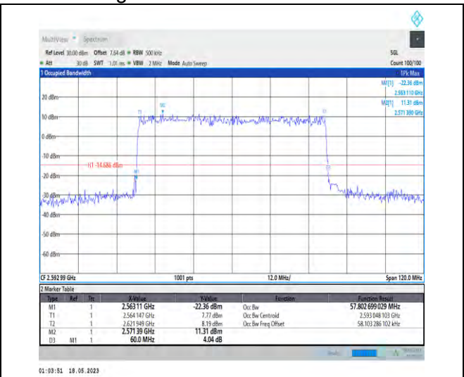
1-N41-PC1-30-60-M-5-DFT-256QAM-Outer_Full-162 @0-Ant1-57.803-60.000-≤60-PASS
