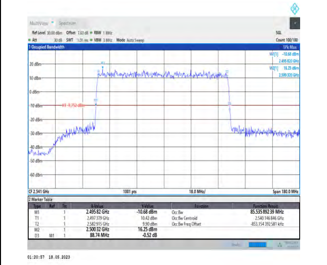
1-N41-PC1-30-90-L-3-DFT-16QAM-Outer_Full-240 @0-Ant1-85.536-88.740-≤90-PASS
