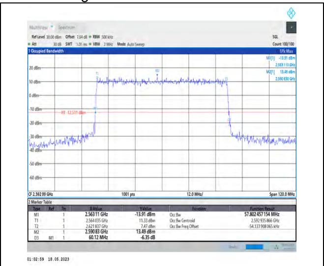
1-N41-PC1-30-60-M-1-DFT-QPSK-Outer_Full-162 @0-Ant1-57.802-60.120-≤60-PASS
