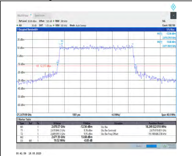
1-N41-PC1-30-20-H-8-CP-64QAM-Outer_Full-51@0 -Ant1-18.249-19.520-≤20-PASS
