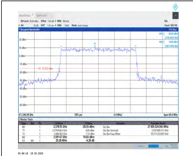
1-N41-PC1-30-30-M-9-CP-256QAM-Outer_Full-78@ 0-Ant1-27.905-29.280-≤30-PASS
