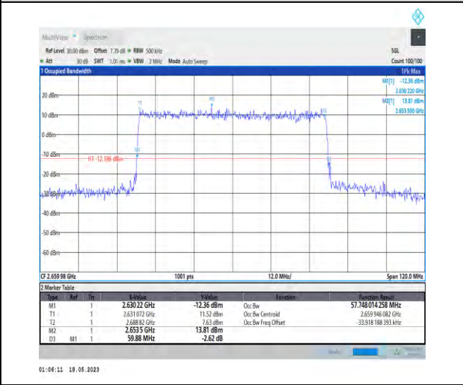
1-N41-PC1-30-60-H-6-CP-QPSK-Outer_Full-162@0-Ant1-57.748-59.880-≤60-PASS
