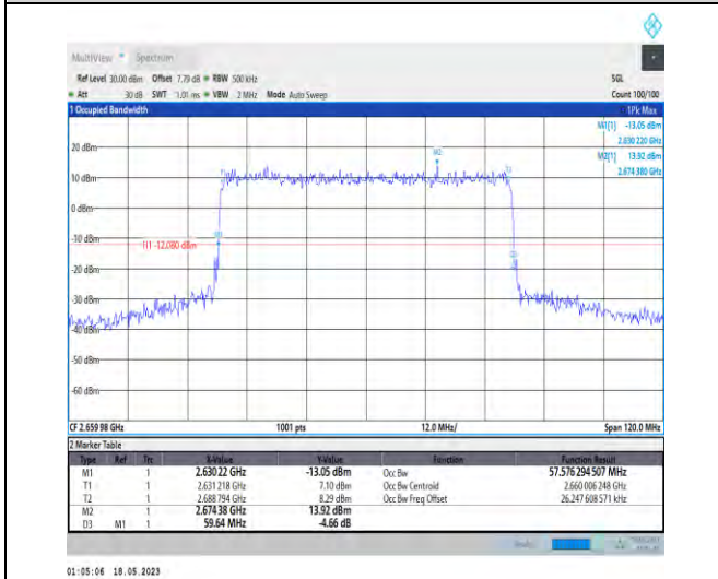
1-N41-PC1-30-60-H-1-DFT-QPSK-Outer_Full-162@ 0-Ant1-57.576-59.640-≤60-PASS
