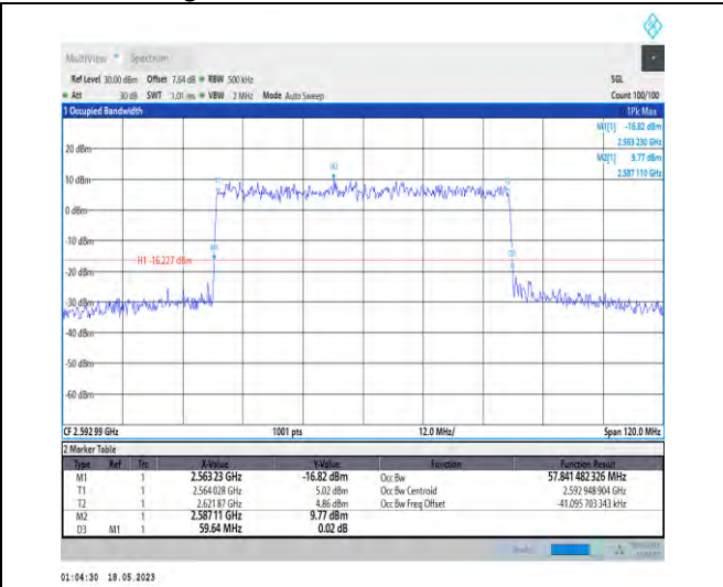
1-N41-PC1-30-60-M-9-CP-256QAM-Outer_Full-162 @0-Ant1-57.841-59.640-≤60-PASS
