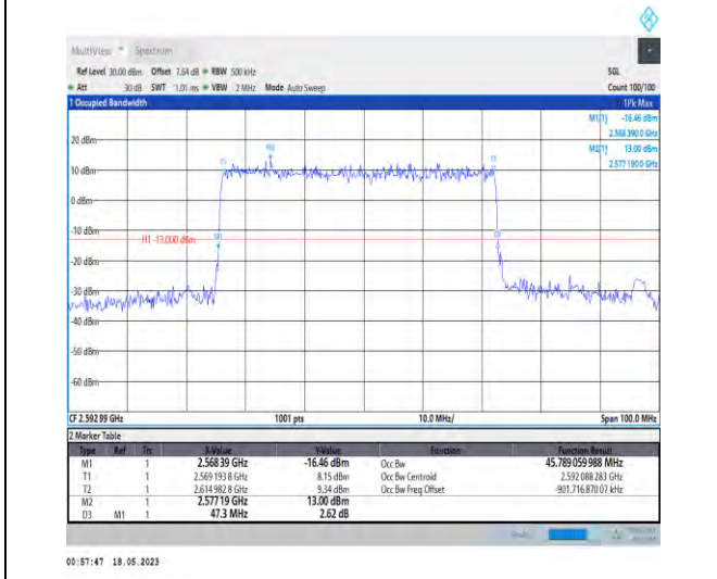
1-N41-PC1-30-50-M-5-DFT-256QAM-Outer_Full-128 @0-Ant1-45.789-47.300-≤50-PASS
