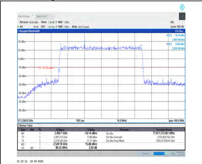
1-N41-PC1-30-80-L-4-DFT-64QAM-Outer_Full-216 @0-Ant1-77.011-80.320-≤80-PASS
