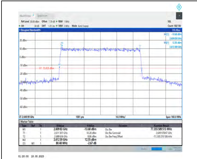
1-N41-PC1-30-80-H-9-CP-256QAM-Outer_Full-217 @0-Ant1-77.356-80.480-≤80-PASS
