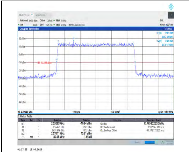
1-N41-PC1-30-80-M-6-CP-QPSK-Outer_Full-217@0 -Ant1-77.466-80.480-≤80-PASS
