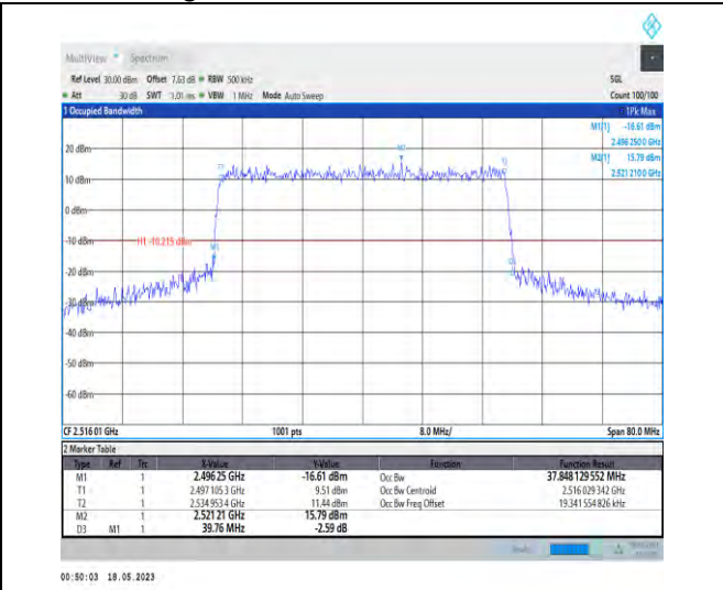
1-N41-PC1-30-40-L-8-CP-64QAM-Outer_Full-106@ 0-Ant1-37.848-39.760-≤40-PASS
