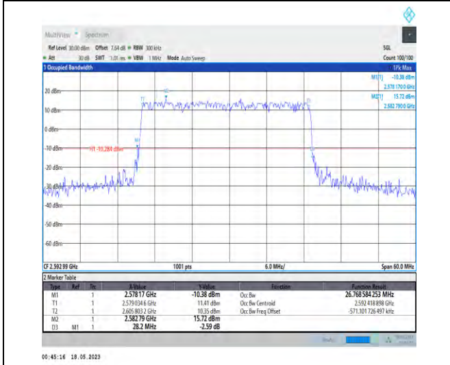
1-N41-PC1-30-30-M-3-DFT-16QAM-Outer_Full-75@0 0-Ant1-26.769-28.200-≤30-PASS
