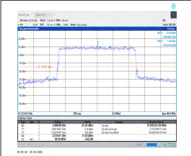
1-N41-PC1-30-40-L-9-CP-256QAM-Outer_Full-106 @0-Ant1-37.878-39.760-≤40-PASS
