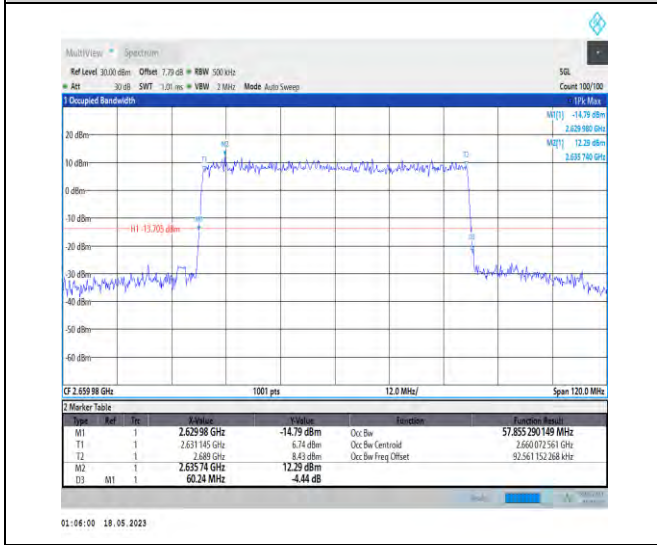
1-N41-PC1-30-60-H-5-DFT-256QAM-Outer_Full-162 @0-Ant1-57.855-60.240-≤60-PASS
