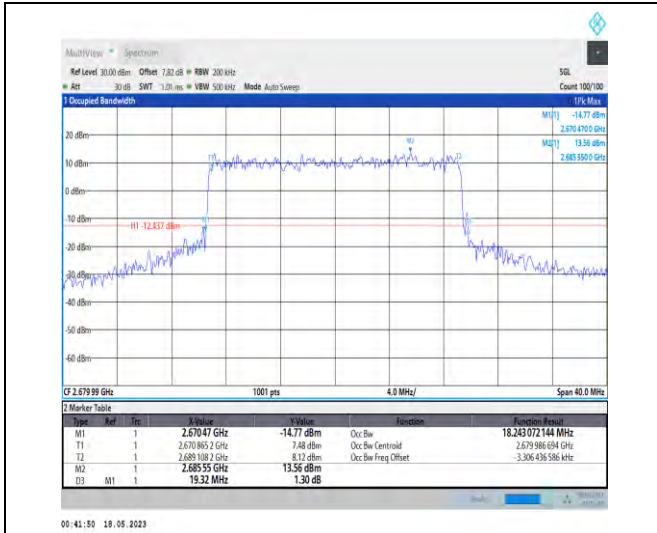
1-N41-PC1-30-20-H-7-CP-16QAM-Outer_Full-51@0 -Ant1-18.243-19.320-≤20-PASS
