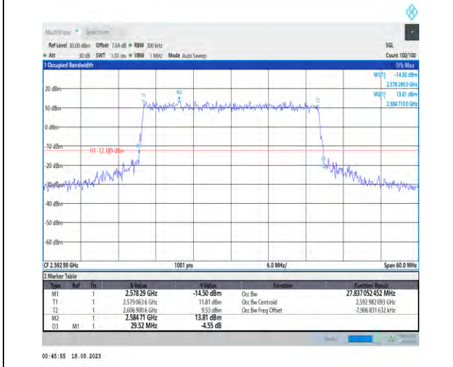
1-N41-PC1-30-30-M-7-CP-16QAM-Outer_Full-78@0 -Ant1-27.837-29.520-≤30-PASS
