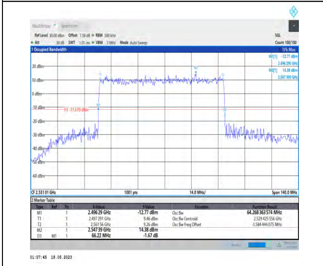
1-N41-PC1-30-70-L-4-DFT-64QAM-Outer_Full-180 @0-Ant1-64.268-66.220-≤70-PASS
