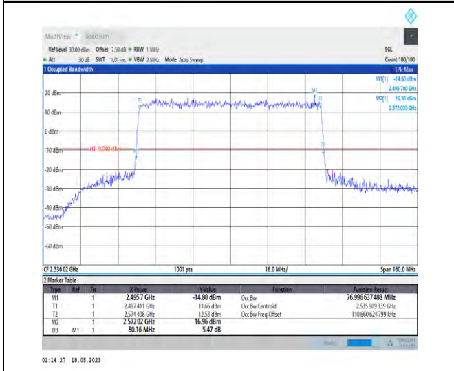
1-N41-PC1-30-80-L-1-DFT-QPSK-Outer_Full-216@0 -Ant1-76.997-80.160-≤80-PASS
