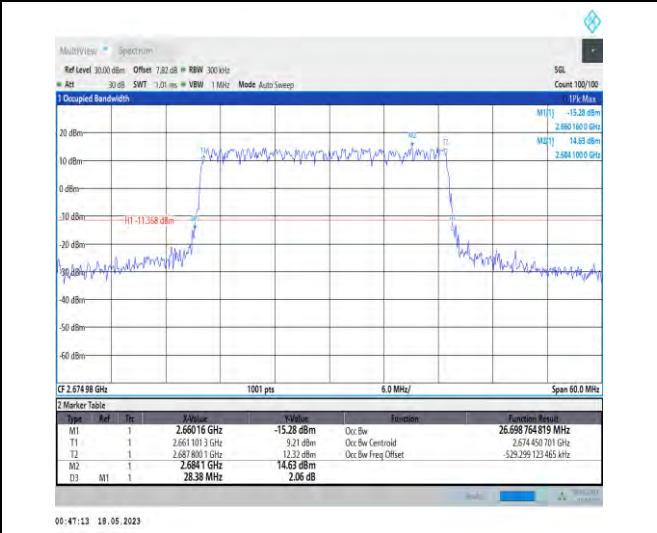
1-N41-PC1-30-30-H-3-DFT-16QAM-Outer_Full-75@ 0-Ant1-26.699-28.380-≤30-PASS
