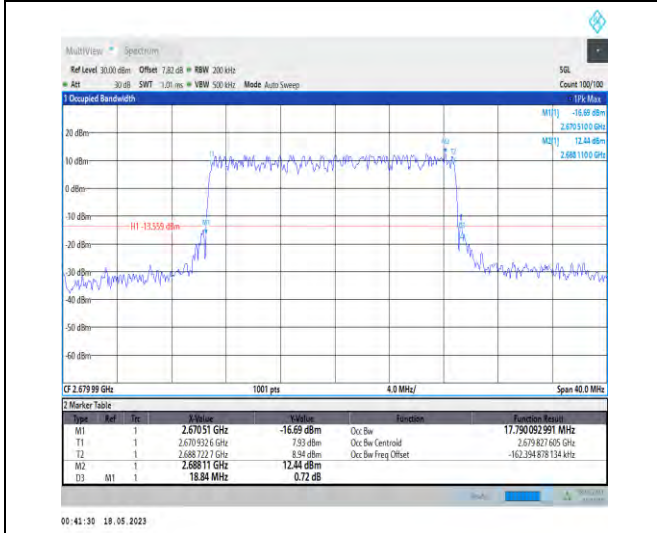
1-N41-PC1-30-20-H-5-DFT-256QAM-Outer_Full-50 @0-Ant1-17.79-18.840-≤20-PASS
