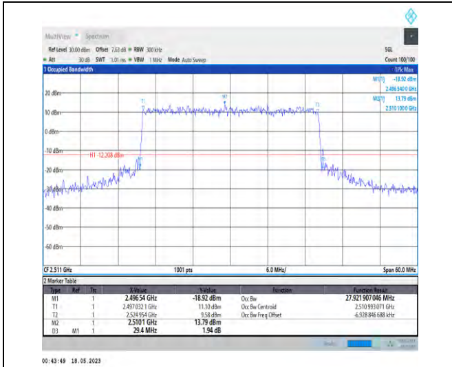
1-N41-PC1-30-30-L-6-CP-QPSK-Outer_Full-78@0-A Ant1-27.922-29.400-≤30-PASS
