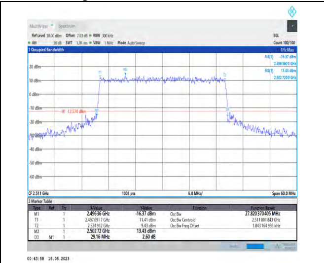
1-N41-PC1-30-30-L-7-CP-16QAM-Outer_Full-78@0-A Ant1-27.82-29.160-≤30-PASS
