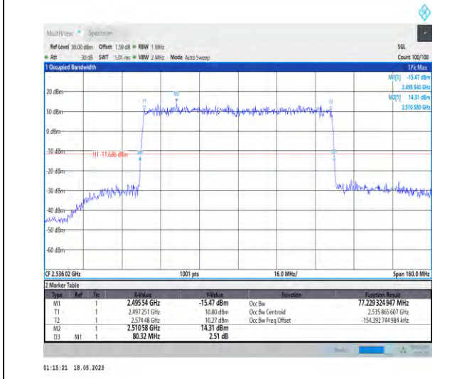
1-N41-PC1-30-80-L-5-DFT-256QAM-Outer_Full-216 @0-Ant1-77.229-80.320-≤80-PASS
