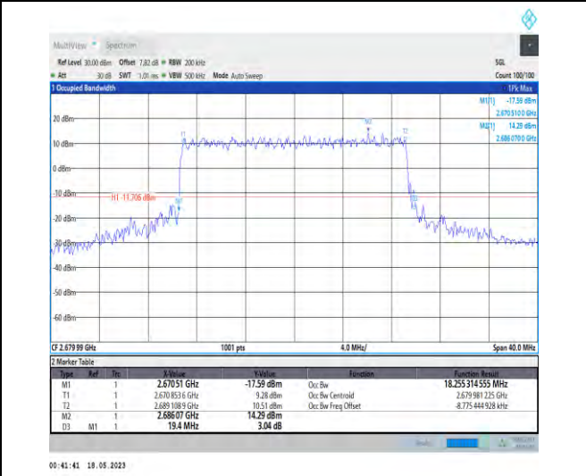
1-N41-PC1-30-20-H-6-CP-QPSK-Outer_Full-51@0- Ant1-18.255-19.400-≤20-PASS
