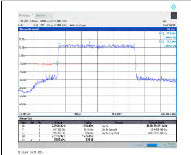
1-N41-PC1-30-90-L-4-DFT-64QAM-Outer_Full-240 @0-Ant1-85.565-88.920-≤90-PASS
