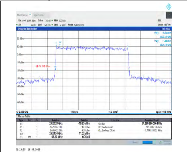
1-N41-PC1-30-70-H-5-DFT-256QAM-Outer_Full-180 @0-Ant1-64.28-66.220-≤70-PASS
