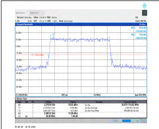
1-N41-PC1-30-30-M-5-DFT-256QAM-Outer_Full-75 @0-Ant1-26.873-28.380-≤30-PASS
