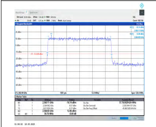
1-N41-PC1-30-60-M-6-CP-QPSK-Outer_Full-162@0 -Ant1-57.764-59.760-≤60-PASS
