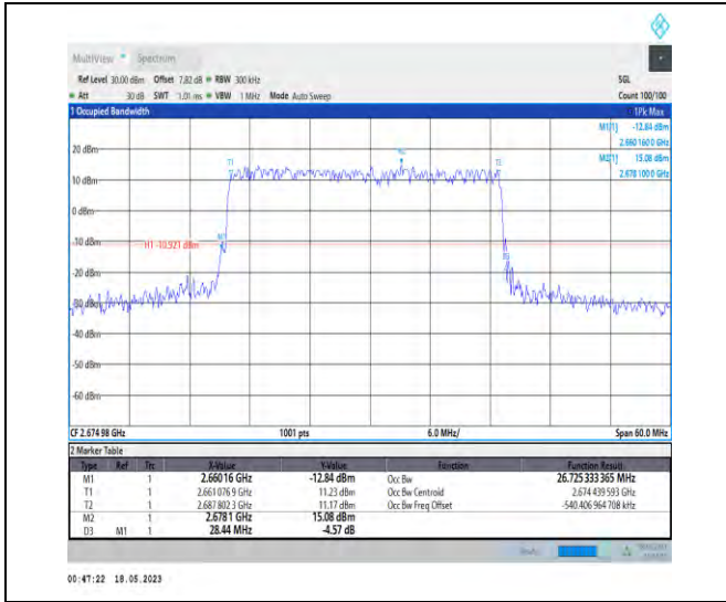
1-N41-PC1-30-30-H-4-DFT-64QAM-Outer_Full-75@ 0-Ant1-26.725-28.440-≤30-PASS
