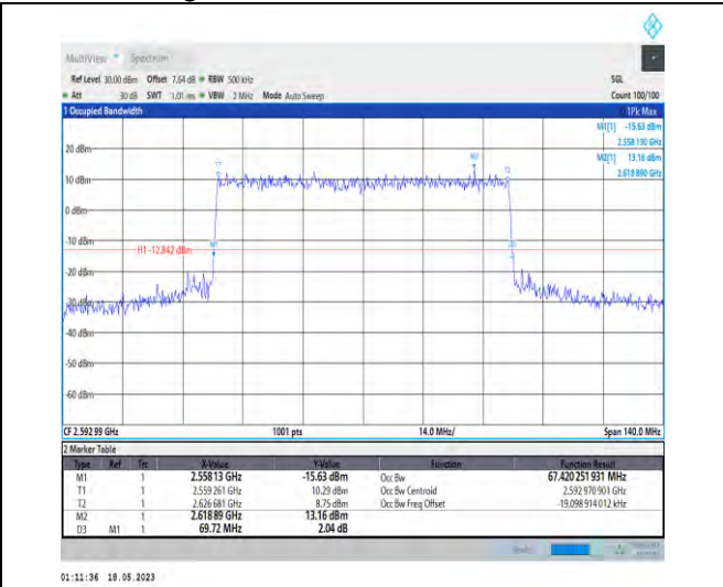
1-N41-PC1-30-70-M-6-CP-QPSK-Outer_Full-189@0 -Ant1-67.42-69.720-≤70-PASS
