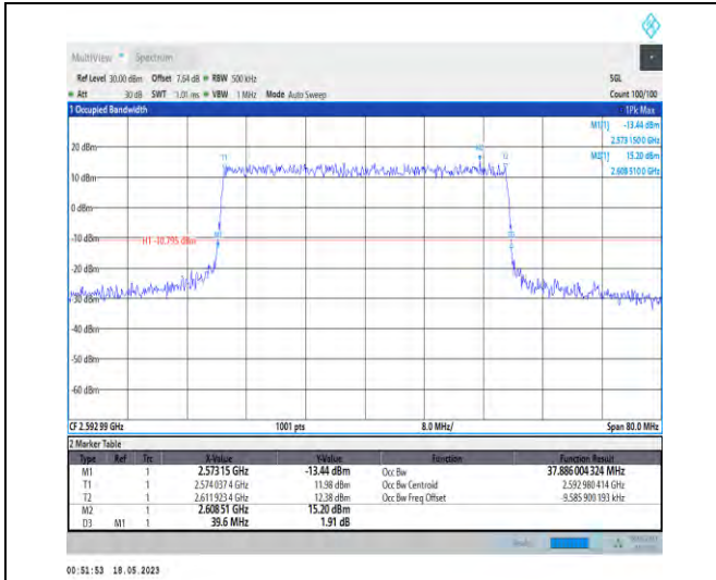
1-N41-PC1-30-40-M-6-CP-QPSK-Outer_Full-106@0 -Ant1-37.886-39.600-≤40-PASS
