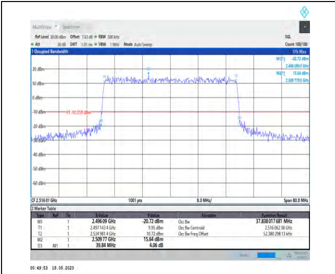
1-N41-PC1-30-40-L-7-CP-16QAM-Outer_Full-106@ 0-Ant1-37.838-39.840-≤40-PASS
