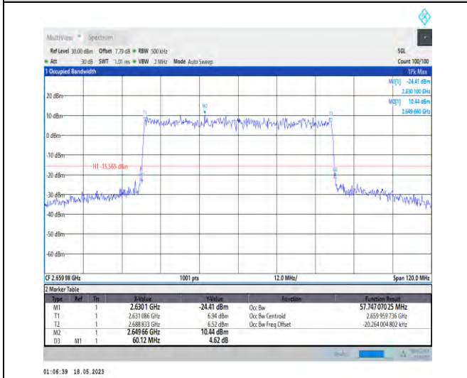
1-N41-PC1-30-60-H-9-CP-256QAM-Outer_Full-162 @0-Ant1-57.747-60.120-≤60-PASS
