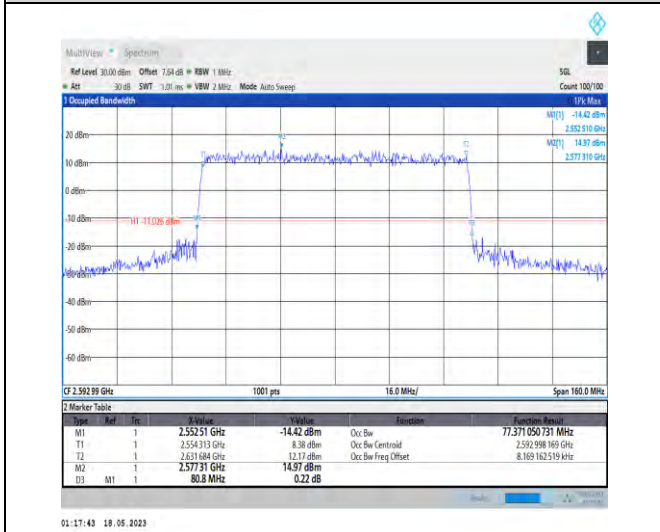
1-N41-PC1-30-80-M-8-CP-64QAM-Outer_Full-217@0 -Ant1-77.371-80.800-≤80-PASS
