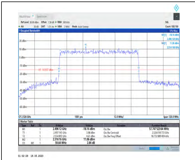
1-N41-PC1-30-60-L-9-CP-256QAM-Outer_Full-162 @0-Ant1-57.748-59.640-≤60-PASS
