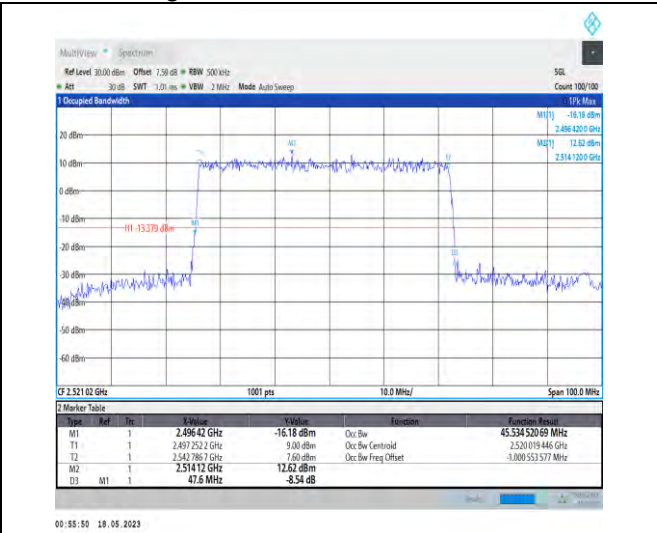
1-N41-PC1-30-50-L-5-DFT-256QAM-Outer_Full-128 @0-Ant1-45.535-47.600-≤50-PASS
