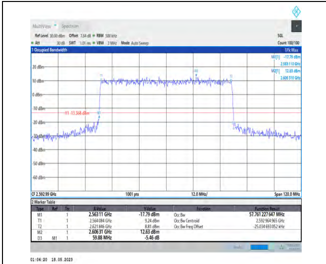
1-N41-PC1-30-60-M-8-CP-64QAM-Outer_Full-162@ 0-Ant1-57.761-59.880-≤60-PASS
