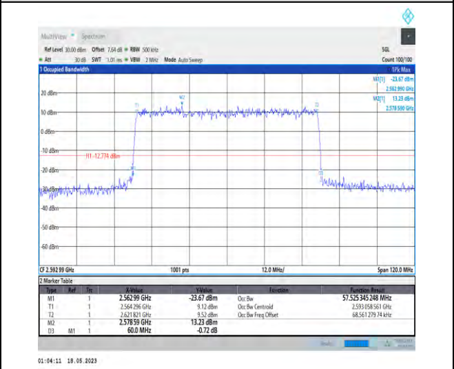
1-N41-PC1-30-60-M-7-CP-16QAM-Outer_Full-162@0 -Ant1-57.525-60.000-≤60-PASS
