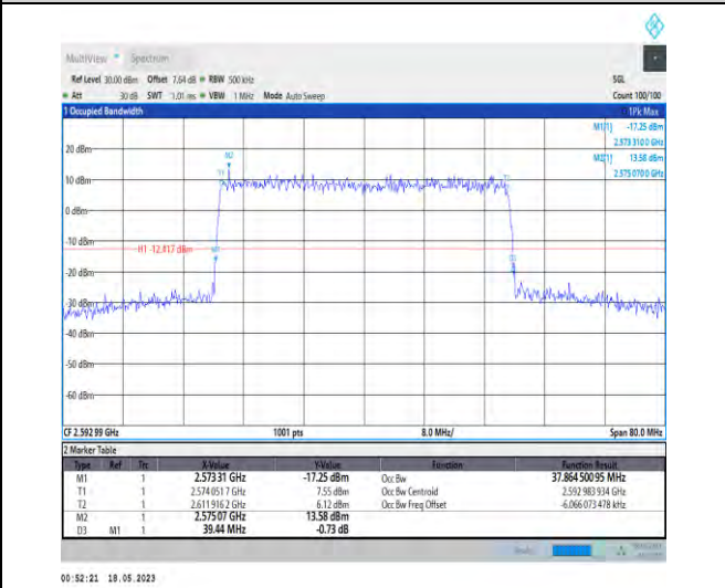
1-N41-PC1-30-40-M-9-CP-256QAM-Outer_Full-106@0 @0-Ant1-37.865-39.440-≤40-PASS
