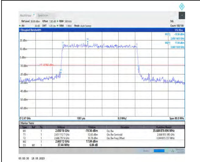
1-N41-PC1-30-40-H-3-DFT-16QAM-Outer_Full-100@ 0-Ant1-35.685-37.440-≤40-PASS
