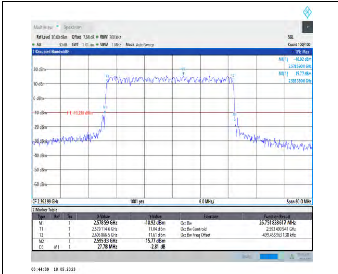
1-N41-PC1-30-30-M-1-DFT-QPSK-Outer_Full-75@0 -Ant1-26.752-27.780-≤30-PASS
