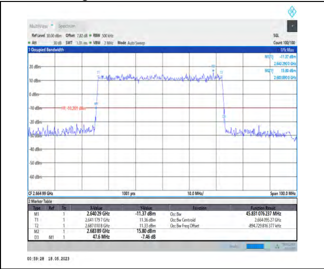
1-N41-PC1-30-50-H-3-DFT-16QAM-Outer_Full-128 @0-Ant1-45.831-47.600-≤50-PASS
