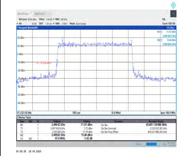
1-N41-PC1-30-50-L-3-DFT-16QAM-Outer_Full-128 @0-Ant1-45.601-47.400-≤50-PASS
