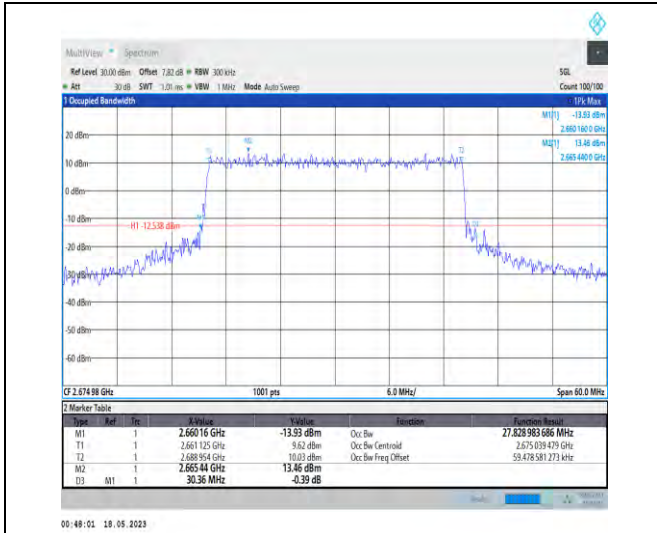
1-N41-PC1-30-30-H-8-CP-64QAM-Outer_Full-78@0 -Ant1-27.829-30.360-≤30-PASS
