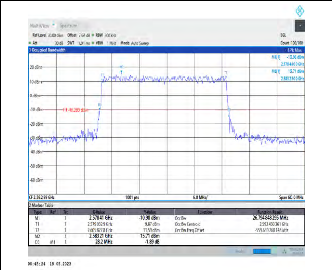
1-N41-PC1-30-30-M-4-DFT-64QAM-Outer_Full-75@0 0-Ant1-26.795-28.200-≤30-PASS
