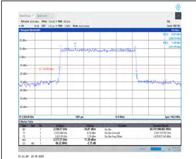
1-N41-PC1-30-70-M-5-DFT-256QAM-Outer_Full-180 @0-Ant1-64.142-66.220-≤70-PASS
