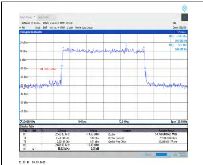
1-N41-PC1-30-60-M-4-DFT-64QAM-Outer_Full-162 @0-Ant1-57.779-59.520-≤60-PASS
