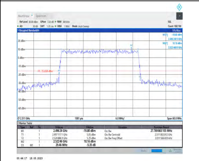
1-N41-PC1-30-30-L-9-CP-256QAM-Outer_Full-78@0-A Ant1-27.77-29.460-≤30-PASS
