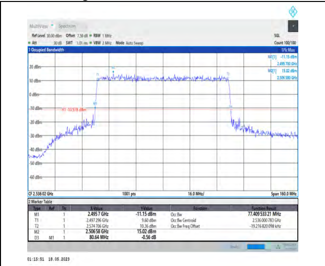
1-N41-PC1-30-80-L-8-CP-64QAM-Outer_Full-217@ 0-Ant1-77.41-80.640-≤80-PASS
