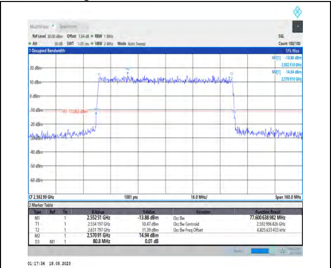
1-N41-PC1-30-80-M-7-CP-16QAM-Outer_Full-217@0 -Ant1-77.601-80.800-≤80-PASS
