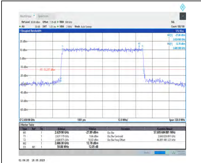
1-N41-PC1-30-60-H-7-CP-16QAM-Outer_Full-162@ 0-Ant1-57.696-59.880-≤60-PASS
