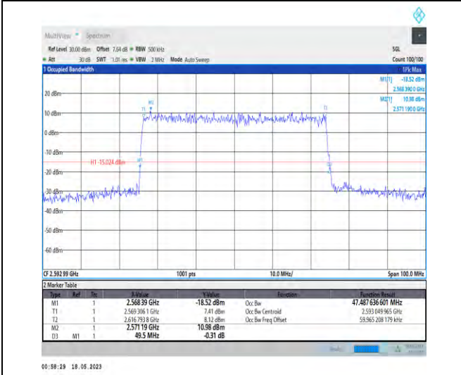
1-N41-PC1-30-50-M-9-CP-256QAM-Outer_Full-133 @0-Ant1-47.488-49.500-≤50-PASS
