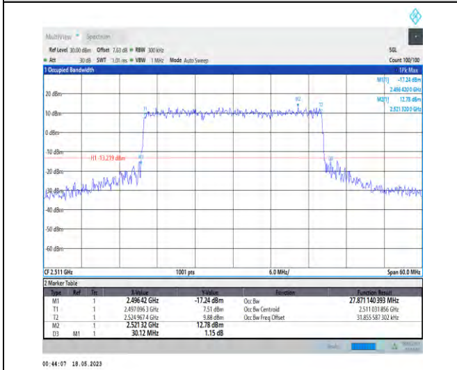
1-N41-PC1-30-30-L-8-CP-64QAM-Outer_Full-78@0-A Ant1-27.871-30.120-≤30-PASS
