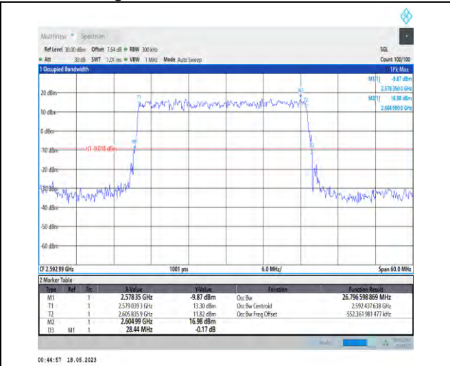
1-N41-PC1-30-30-M-2-DFT-PI2BPSK-Outer_Full-75@0 @0-Ant1-26.797-28.440-≤30-PASS
