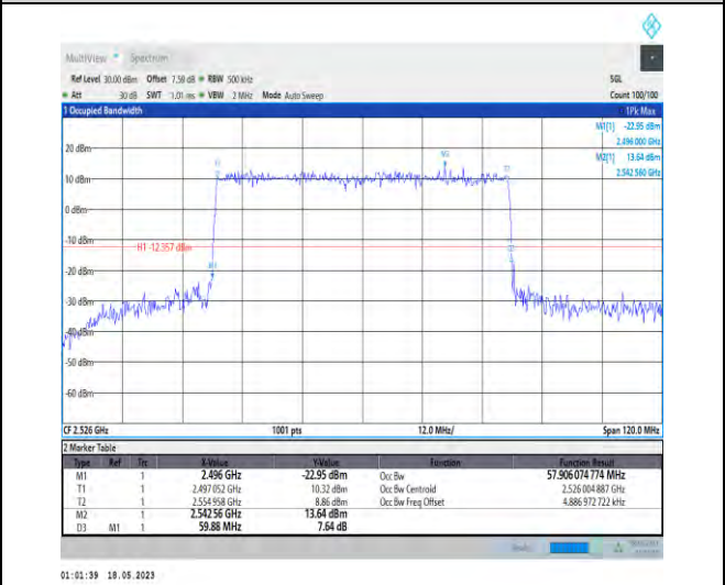
1-N41-PC1-30-60-L-4-DFT-64QAM-Outer_Full-162 @0-Ant1-57.906-59.880-≤60-PASS
