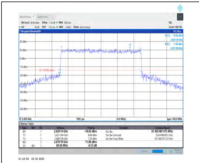
1-N41-PC1-30-70-H-8-CP-64QAM-Outer_Full-189@ 0-Ant1-67.492-69.580-≤70-PASS
