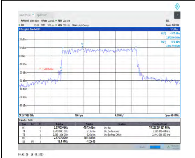
1-N41-PC1-30-20-H-9-CP-256QAM-Outer_Full-51@0 -Ant1-18.226-19.400-≤20-PASS
