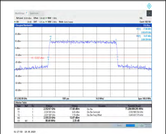
1-N41-PC1-30-80-M-9-CP-256QAM-Outer_Full-217@0 -Ant1-77.206-80.640-≤80-PASS
