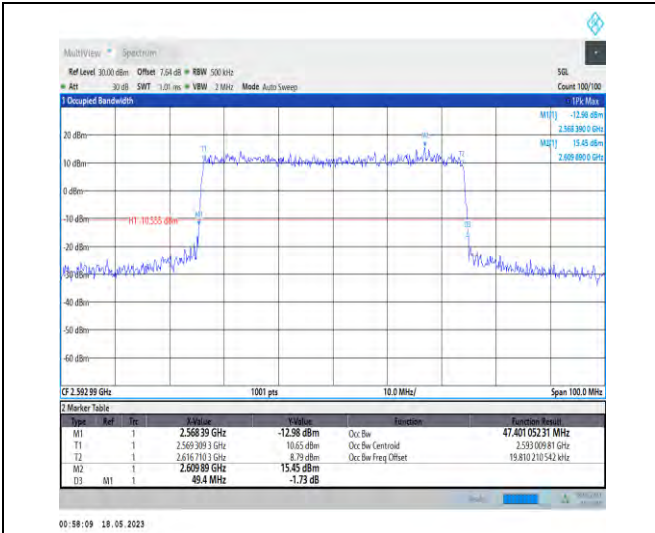
1-N41-PC1-30-50-M-7-CP-16QAM-Outer_Full-133@ 0-Ant1-47.401-49.400-≤50-PASS
