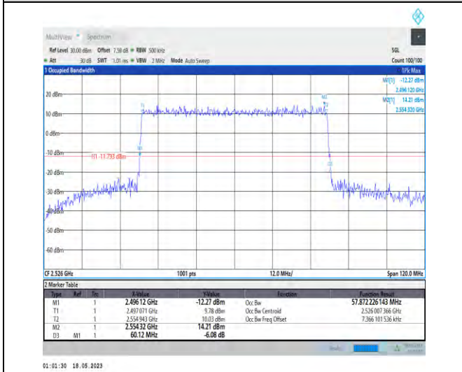
1-N41-PC1-30-60-L-3-DFT-16QAM-Outer_Full-162 @0-Ant1-57.872-60.120-≤60-PASS
