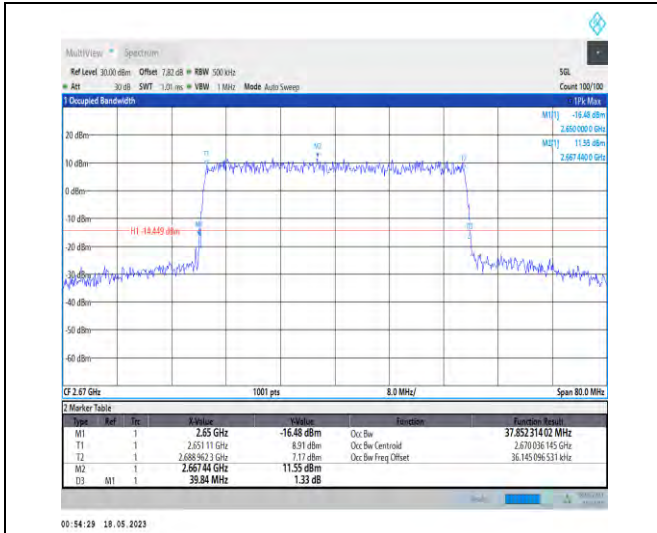
1-N41-PC1-30-40-H-9-CP-256QAM-Outer_Full-106 @0-Ant1-37.852-39.840-≤40-PASS
