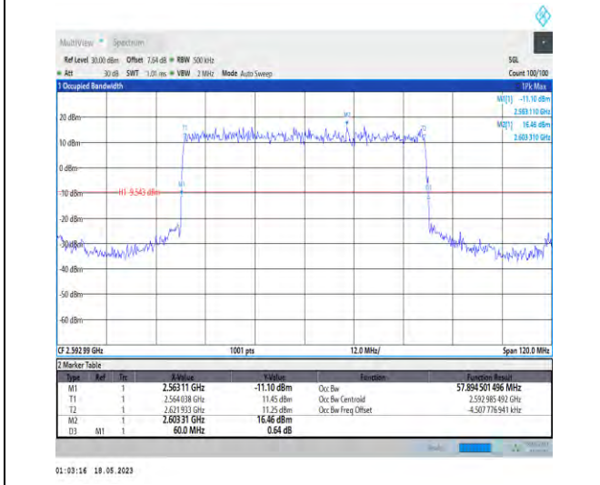
1-N41-PC1-30-60-M-2-DFT-PI2BPSK-Outer_Full-162 @0-Ant1-57.895-60.000-≤60-PASS
