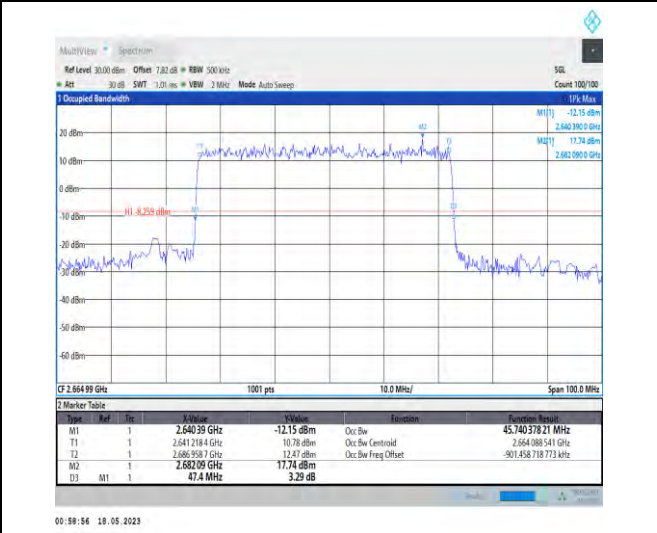
1-N41-PC1-30-50-H-1-DFT-QPSK-Outer_Full-128@ 0-Ant1-45.74-47.400-≤50-PASS
