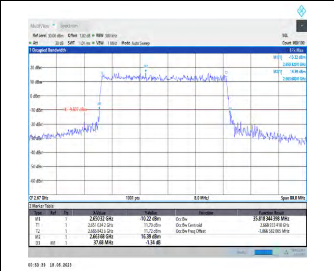
1-N41-PC1-30-40-H-4-DFT-64QAM-Outer_Full-100@ 0-Ant1-35.818-37.680-≤40-PASS
