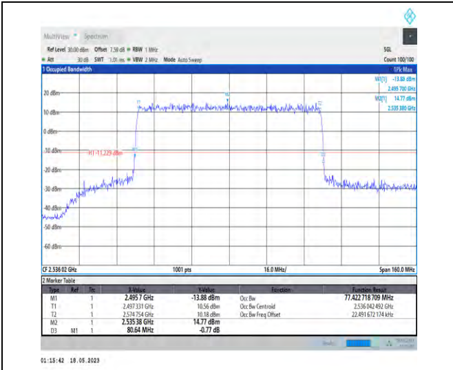
1-N41-PC1-30-80-L-7-CP-16QAM-Outer_Full-217@ 0-Ant1-77.423-80.640-≤80-PASS
