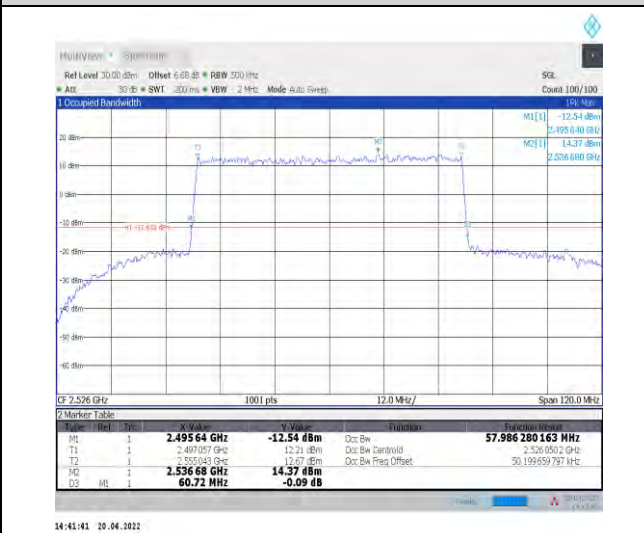
1-N41--30-60-L-4-DFT-64QAM-Outer_Full-162@0-A nt1-57.986-60.720-≤60-PASS
