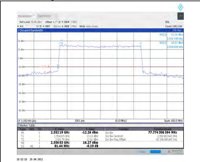
1-N41--30-80-M-7-CP-16QAM-Outer_Full-217@0-Ant 1-77.774-81.440-<80-PASS
