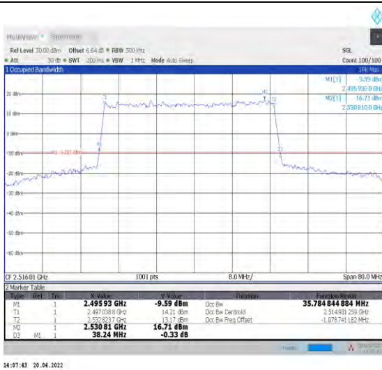
1-N41--30-40-L-3-DFT-16QAM-Outer_Full-100@0-A nt1-35.785-38.240-<math>\leq 40</math>-PASS
