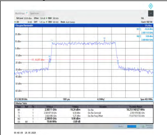
1-N41-PC1-30-20-M-9-CP-256QAM-Outer_Full-51@0 -Ant1-18.213-19.640-≤20-PASS
