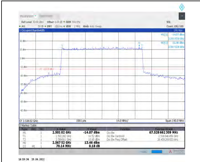
1-N41--30-70-L-6-CP-QPSK-Outer_Full-189@0-Ant1 -67.529-70.140-≤70-PASS
