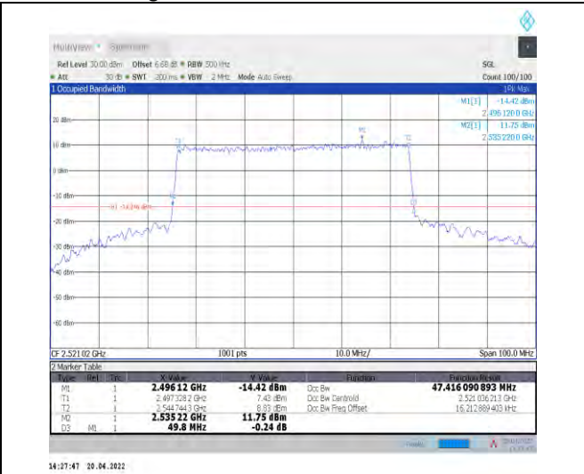
1-N41--30-50-L-9-CP-256QAM-Outer_Full-133@0-Ant 1-47.416-49.800-≤50-PASS
