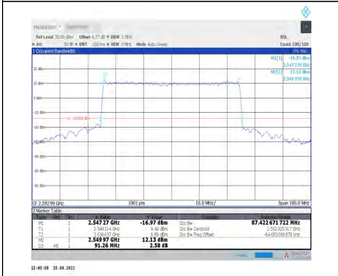
1-N41--30-90-M-9-CP-256QAM-Outer_Full-245@0-A nt1-87.423-91.260-<=90-PASS
