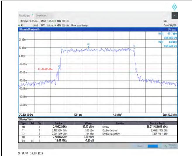
1-N41-PC1-30-20-L-9-CP-256QAM-Outer_Full-51@ 0-Ant1-18.211-19.440-≤20-PASS
