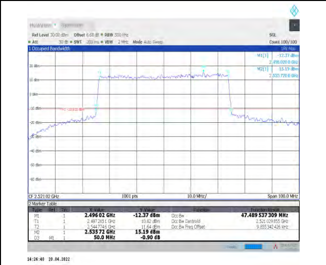
1-N41--30-50-L-7-CP-16QAM-Outer_Full-133@0-Ant t1-47.49-50.000-<math>\leq 50</math>-PASS
