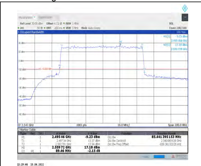
1-N41--30-90-L-1-DFT-QPSK-Outer_Full-240@0-Ant 1-85.441-89.460-≤90-PASS
