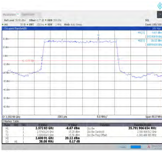
1-N41--30-40-M-2-DFT-PI2BPSK-Outer_Full-100@0-Ant1-35.792-38.080-≤40-PASS
