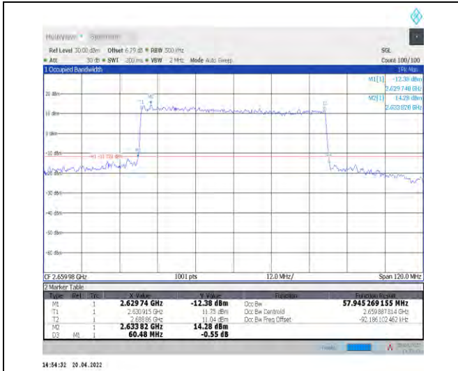
1-N41--30-60-H-7-CP-16QAM-Outer_Full-162@0-An t1-57.945-60.480-≤60-PASS
