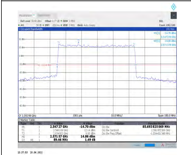
1-N41--30-90-M-5-DFT-256QAM-Outer_Full-240@0-A Ant1-85.694-89.460-≤90-PASS
