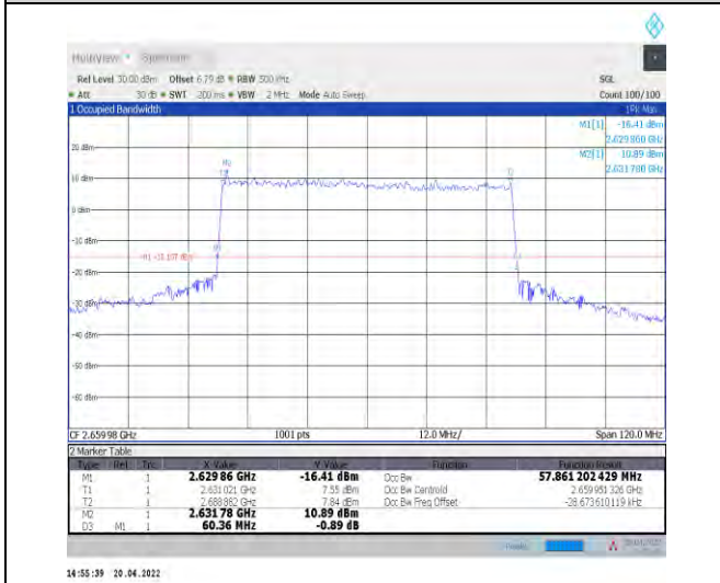
1-N41--30-60-H-9-CP-256QAM-Outer_Full-162@0-A nt1-57.861-60.360-≤60-PASS
