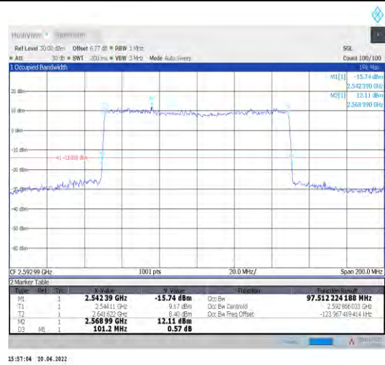
1-N41--30-100-M-9-CP-256QAM-Outer_Full-273@0- Ant1-97.512-101.200-≤100-PASS
