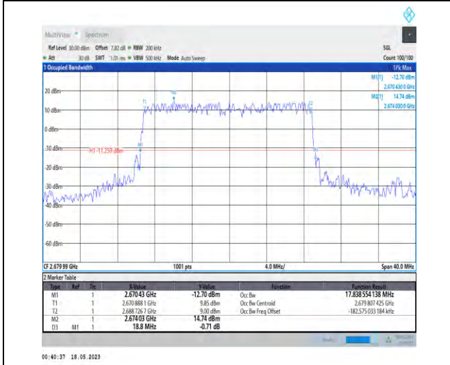
1-N41-PC1-30-20-H-1-DFT-QPSK-Outer_Full-50@0- Ant1-17.839-18.800-≤20-PASS
