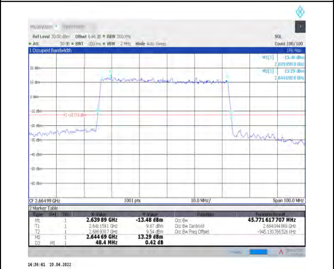
1-N41--30-50-H-5-DFT-256QAM-Outer_Full-128@0-Ant1-45.772-48.400-≤50-PASS
