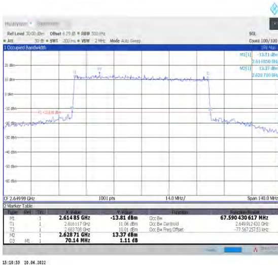
1-N41--30-70-H-6-CP-QPSK-Outer_Full-189@0-Ant 1-67.59-70.140-≤70-PASS
