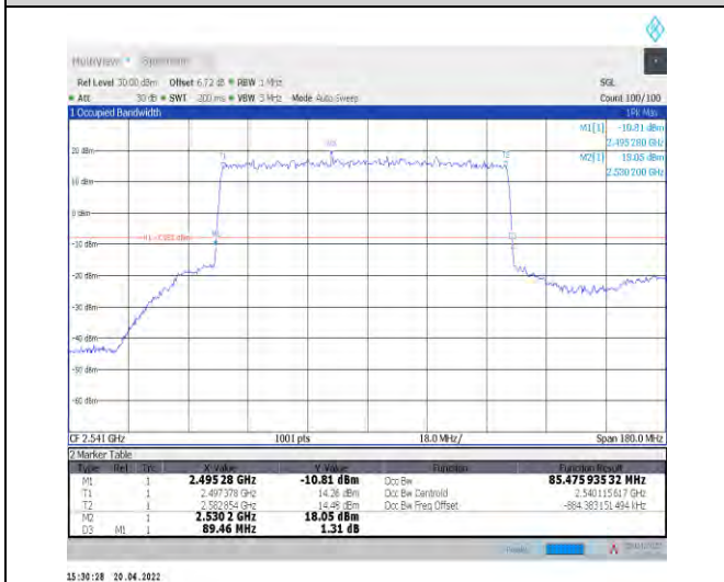
1-N41--30-90-L-2-DFT-PI2BPSK-Outer_Full-240@0-Ant1 Ant1-85.476-89.460-≤90-PASS
