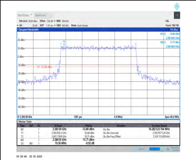
1-N41-PC1-30-20-M-7-CP-16QAM-Outer_Full-51@0- Ant1-18.283-19.360-<=20-PASS
