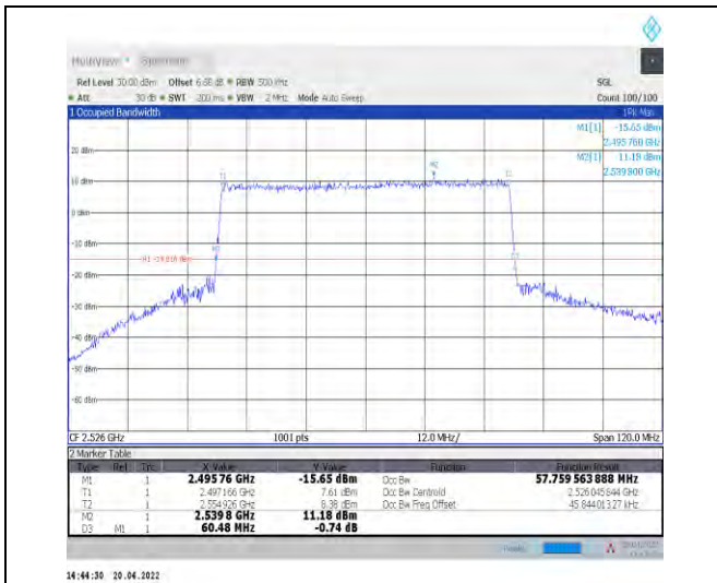
1-N41--30-60-L-9-CP-256QAM-Outer_Full-162@0-A nt1-57.76-60.480-≤60-PASS
