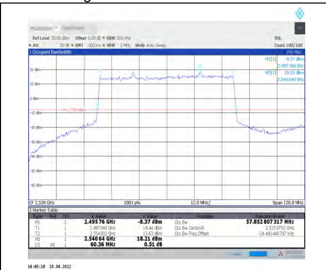
1-N41--30-60-L-2-DFT-PI2BPSK-Outer_Full-162@0-Ant 1-57.853-60.360-≤60-PASS
