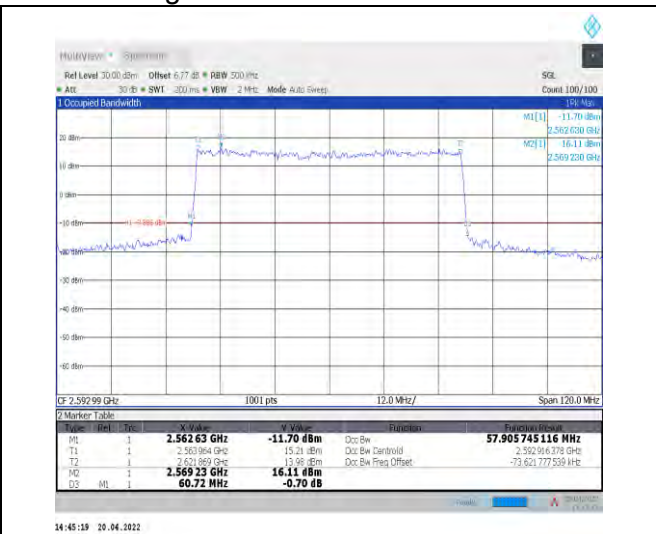
1-N41--30-60-M-1-DFT-QPSK-Outer_Full-162@0-An t1-57.906-60.720-≤60-PASS
