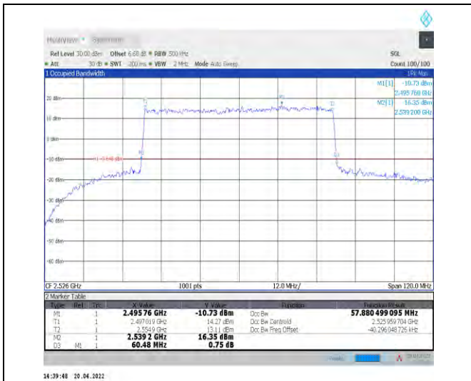
1-N41--30-60-L-1-DFT-QPSK-Outer_Full-162@0-Ant 1-57.88-60.480-≤60-PASS
