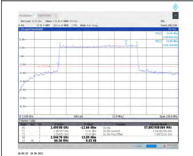
1-N41--30-60-L-7-CP-16QAM-Outer_Full-162@0-Ant 1-57.894-60.360-≤60-PASS
