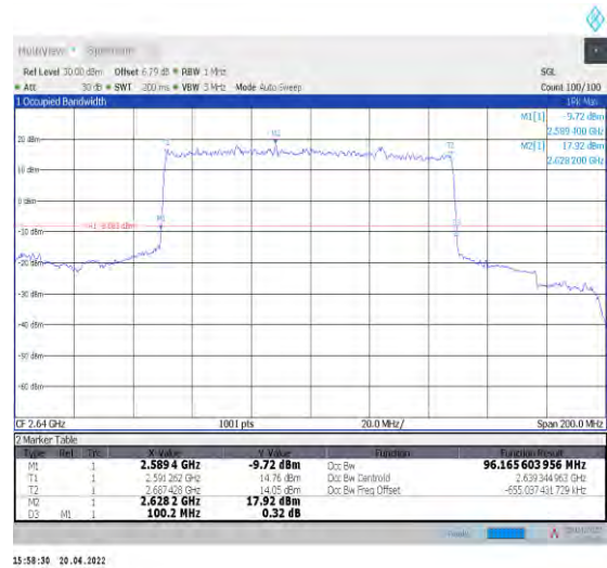
1-N41--30-100-H-2-DFT-PI2BPSK-Outer_Full-270@ 0-Ant1-96.166-100.200-≤100-PASS
