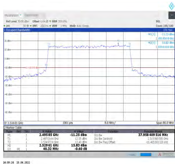
1-N41--30-40-L-6-CP-QPSK-Outer_Full-106@0-Ant 1-37.958-40.320-<math>\leq 40</math>-PASS
