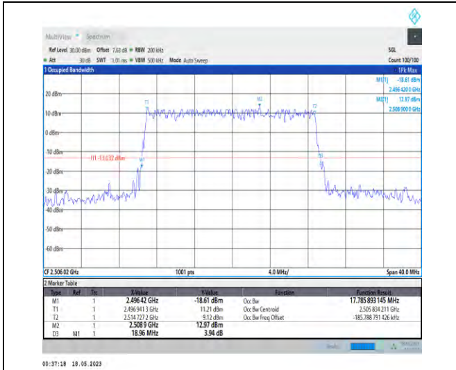
1-N41-PC1-30-20-L-5-DFT-256QAM-Outer_Full-50@0-Ant1-17.786-18.960-≤20-PASS
