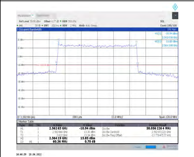
1-N41--30-60-M-3-DFT-16QAM-Outer_Full-162@0- Ant1-58.056-60.360-≤60-PASS
