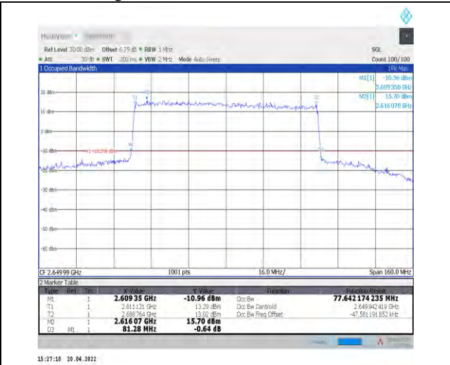
1-N41--30-80-H-6-CP-QPSK-Outer_Full-217@0-Ant 1-77.642-81.280-<math>\leq 80</math>-PASS
