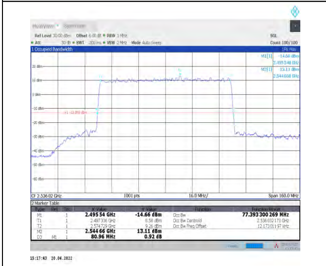
1-N41--30-80-L-9-CP-256QAM-Outer_Full-217@0-A nt1-77.393-80.960-≤80-PASS
