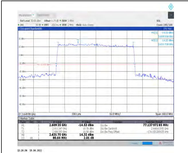
1-N41--30-80-H-5-DFT-256QAM-Outer_Full-216@0-Ant1-77.138-80.640-<math>\leq 80</math>-PASS
