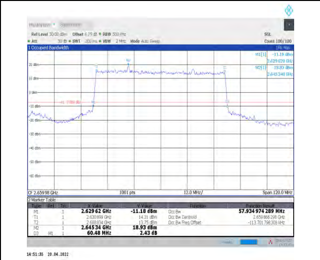
1-N41--30-60-H-2-DFT-PI2BPSK-Outer_Full-162@0-Ant1-57.935-60.480-≤60-PASS
