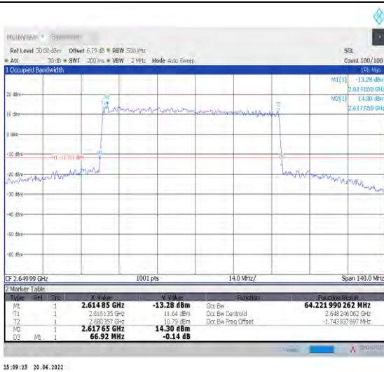
1-N41--30-70-H-4-DFT-64QAM-Outer_Full-180@0-A nt1-64.222-66.920-≤70-PASS
