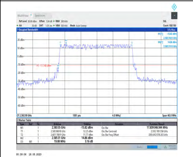
1-N41-PC1-30-20-M-3-DFT-16QAM-Outer_Full-50@ 0-Ant1-17.839-19.080-≤20-PASS
