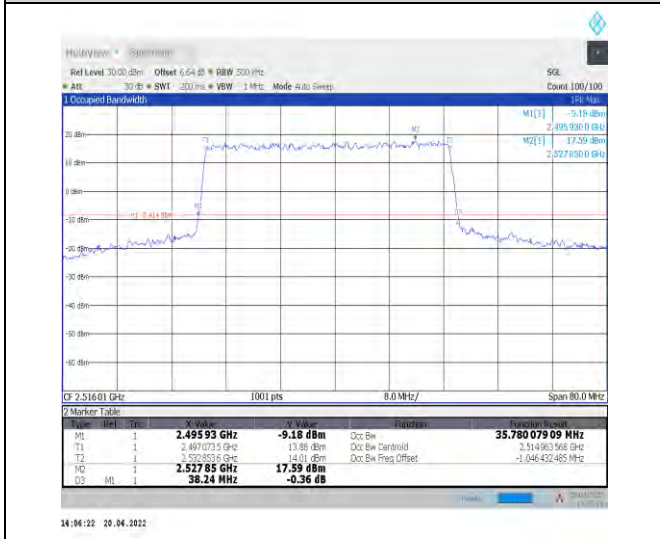
1-N41--30-40-L-1-DFT-QPSK-Outer_Full-100@0-Ant 1-35.78-38.240-≤40-PASS
