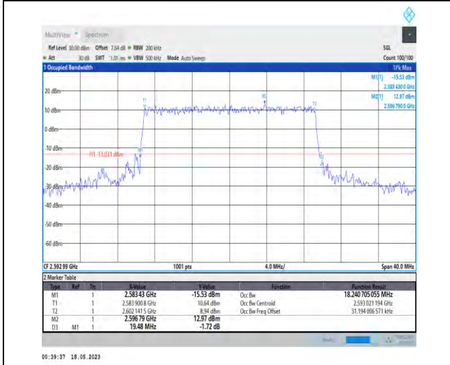
1-N41-PC1-30-20-M-6-CP-QPSK-Outer_Full-51@0- Ant1-18.241-19.480-<=20-PASS
