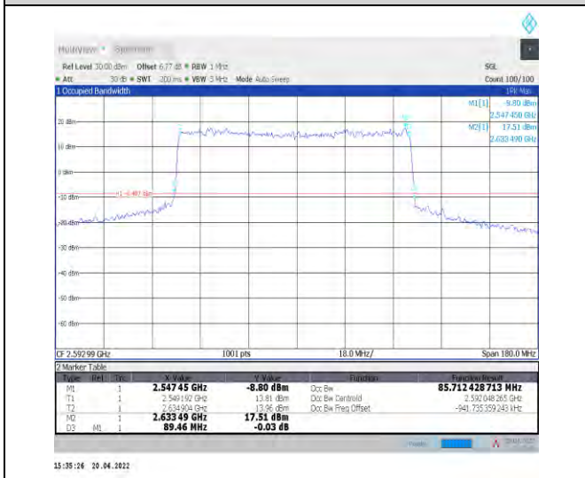
1-N41--30-90-M-1-DFT-QPSK-Outer_Full-240@0-Ant 1-85.712-89.460-≤90-PASS
