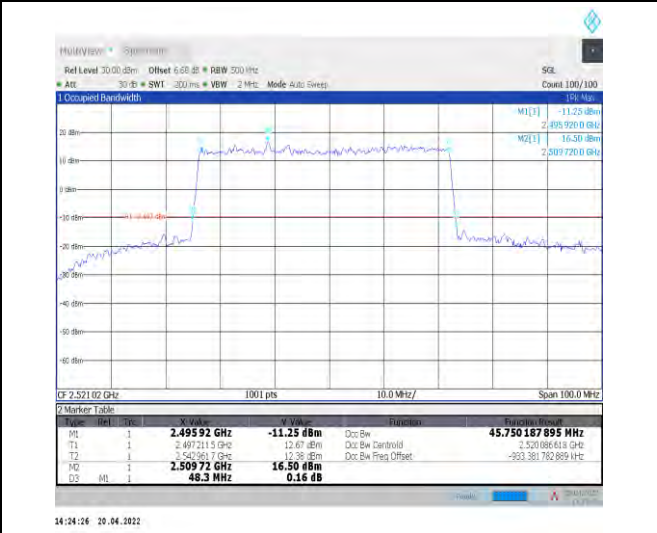
1-N41--30-50-L-3-DFT-16QAM-Outer_Full-128@0-A nt1-45.75-48.300-≤50-PASS
