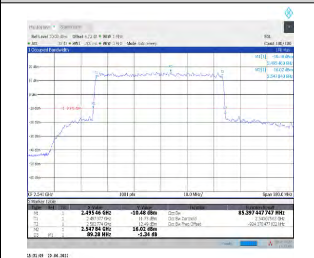
1-N41--30-90-L-3-DFT-16QAM-Outer_Full-240@0-A nt1-85.397-89.280-≤90-PASS
