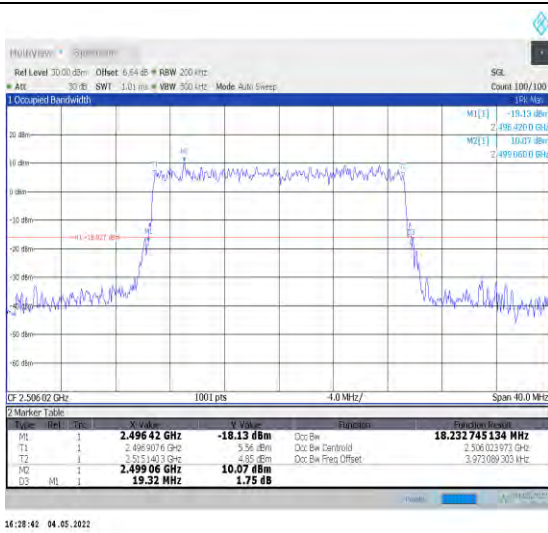
1-N41--30-20-L-9-CP-256QAM-Outer_Full-51@0-Ant 1-18.233-19.320-≤20-PASS
