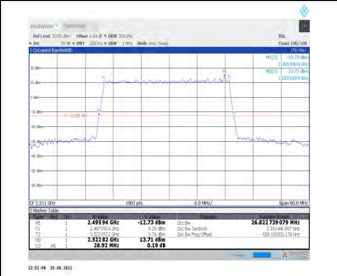
1-N41--30-30-L-5-DFT-256QAM-Outer_Full-75@0-A nt1-26.823-28.920-≤30-PASS
