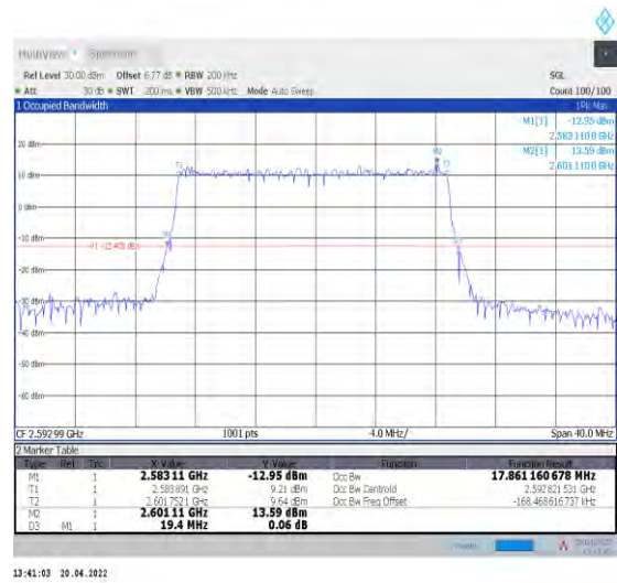
1-N41--30-20-M-5-DFT-256QAM-Outer_Full-50@0-Ant1-17.861-19.400-<=20-PASS
