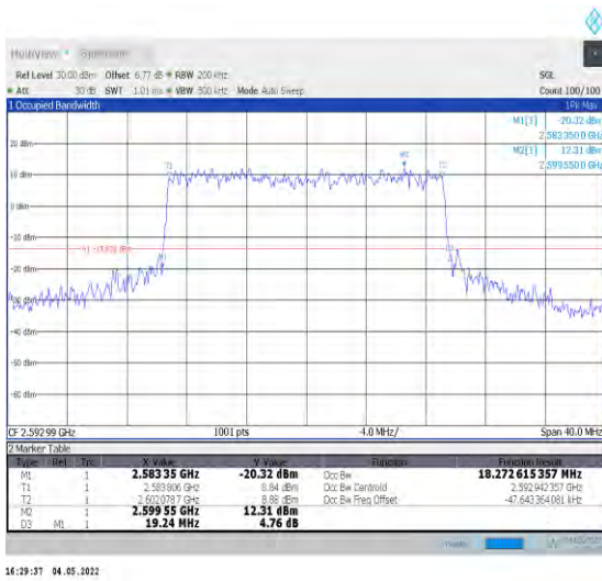
1-N41--30-20-M-8-CP-64QAM-Outer_Full-51@0-Ant 1-18.273-19.240-≤20-PASS
