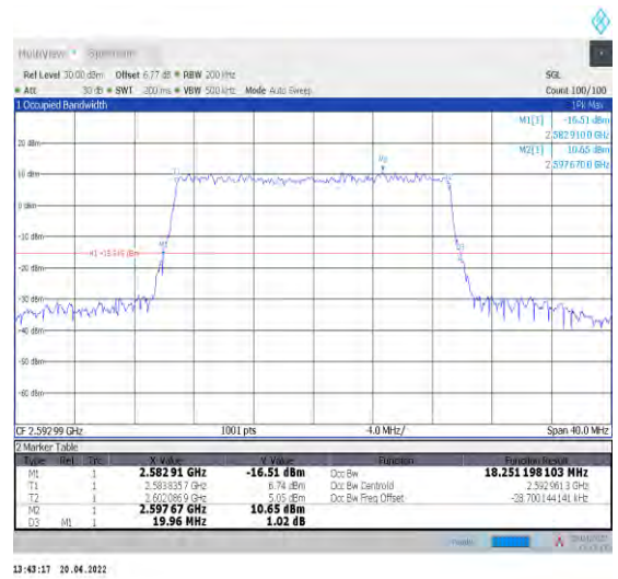
1-N41--30-20-M-9-CP-256QAM-Outer_Full-51@0-Ant 1-18.251-19.960-≤20-PASS
