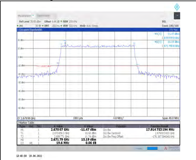
1-N41--30-20-H-4-DFT-64QAM-Outer_Full-50@0-An t1-17.915-19.600-≤20-PASS
