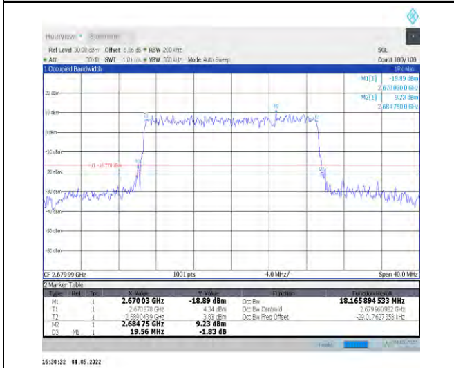
1-N41--30-20-H-9-CP-256QAM-Outer_Full-51@0-Ant t1-18.166-19.560-≤20-PASS
