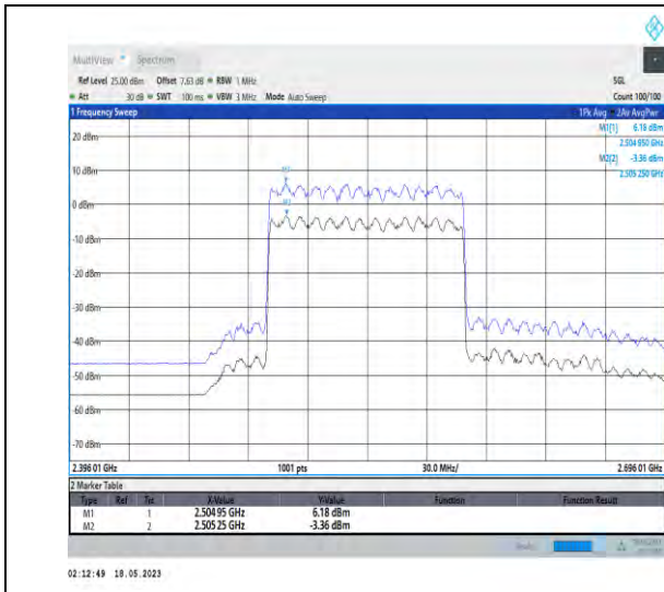
1-N41-PC1-30-100-L-1-DFT-256QAM-Outer_Full-270@0-Ant1-9.54-19.56%-7.09-2.45-PASS-≤13
