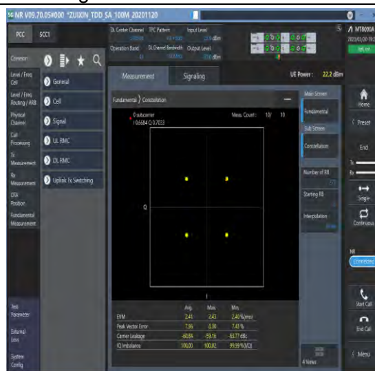
1-N41-30-100-M-6-CP-QPSK-Outer_Full-273@0-Ant1-see graph-PASS
