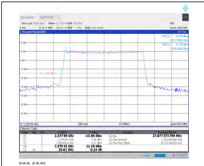
1-N41--30-30-M-9-CP-256QAM-Outer_Full-78@0-Ant t1-27.877-29.820-≤30-PASS
