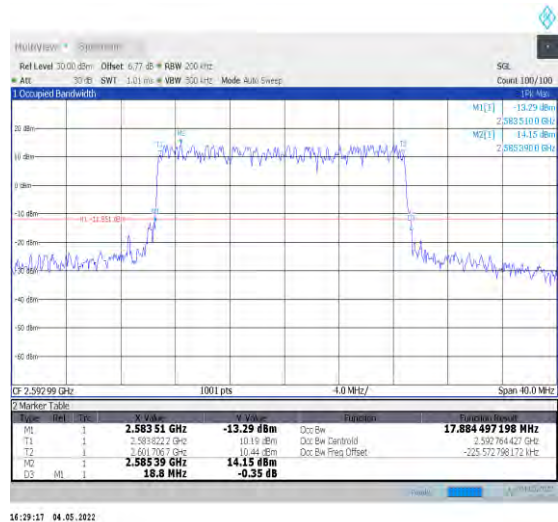
1-N41--30-20-M-3-DFT-16QAM-Outer_Full-50@0-Ant 1-17.884-18.800-≤20-PASS
