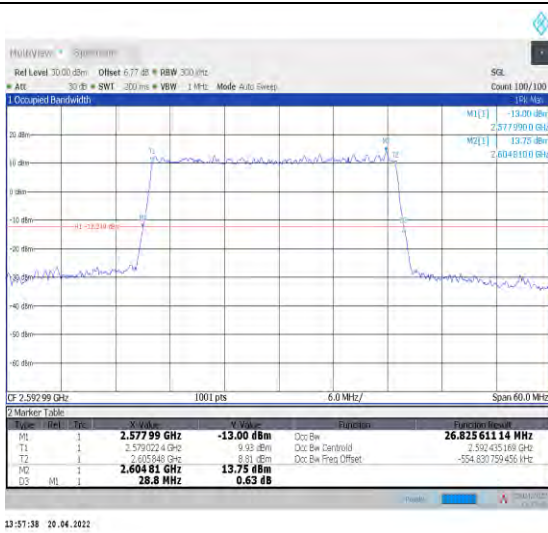
1-N41--30-30-M-5-DFT-256QAM-Outer_Full-75@0-A nt1-26.826-28.800-≤30-PASS
