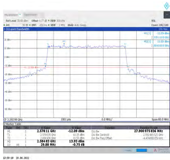
1-N41--30-30-M-8-CP-64QAM-Outer_Full-78@0-Ant 1-27.901-29.880-≤30-PASS
