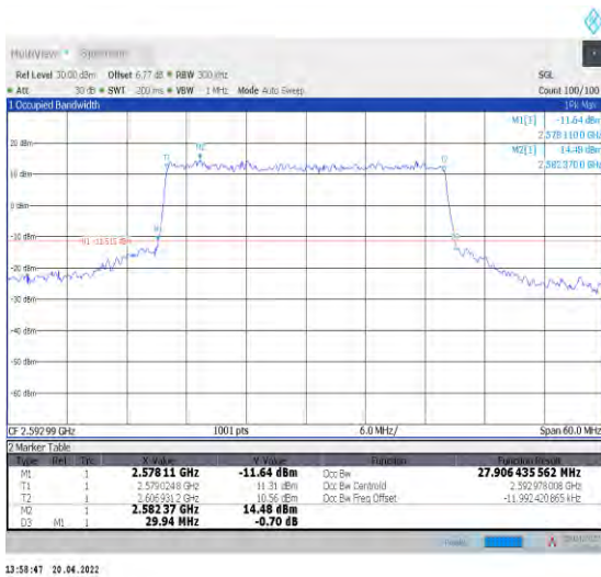
1-N41--30-30-M-7-CP-16QAM-Outer_Full-78@0-Ant 1-27.906-29.940-≤30-PASS
