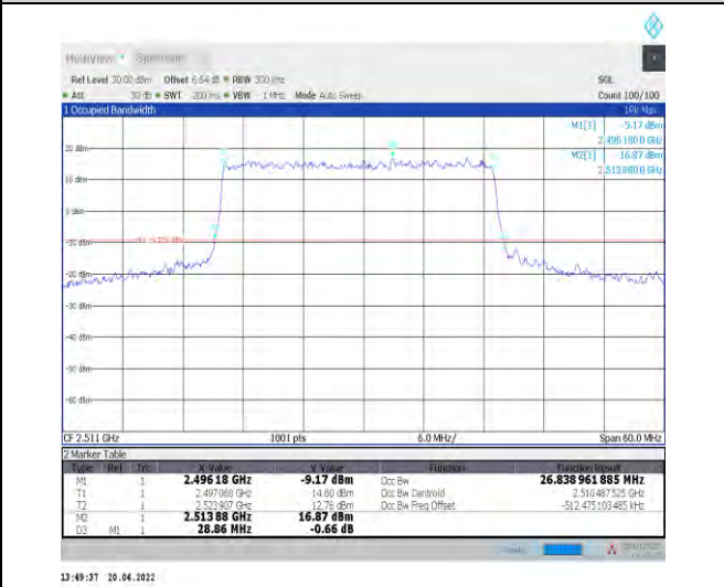
1-N41--30-30-L-1-DFT-QPSK-Outer_Full-75@0-Ant1 -26.839-28.860-≤30-PASS
