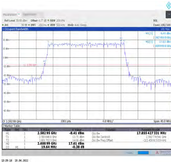
1-N41--30-20-M-2-DFT-PI2BPSK-Outer_Full-50@0-Ant 1-17.855-19.640-≤20-PASS
