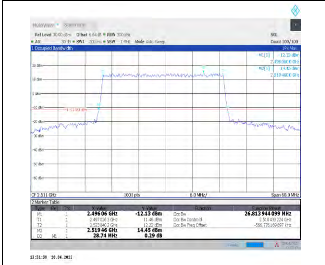
1-N41--30-30-L-4-DFT-64QAM-Outer_Full-75@0-Ant 1-26.814-28.740-≤30-PASS
