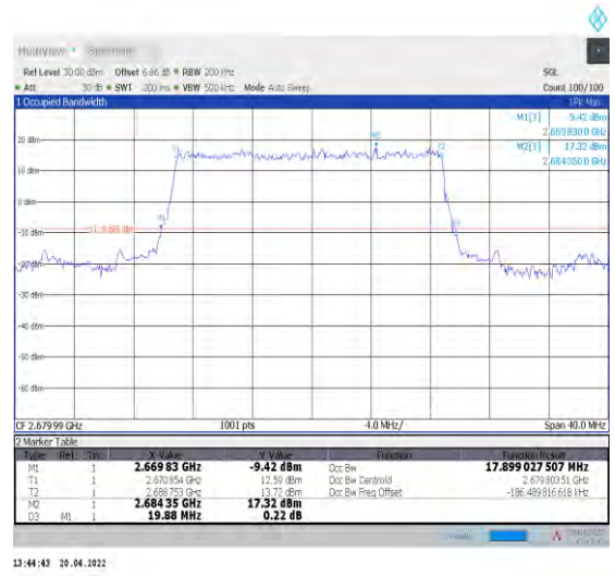
1-N41--30-20-H-2-DFT-PI2BPSK-Outer_Full-50@0-Ant 1-17.899-19.880-≤20-PASS
