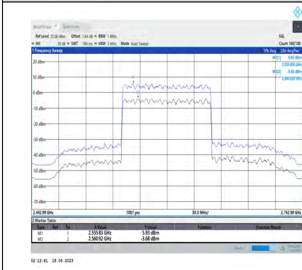
1-N41-PC1-30-100-M-1-DFT-256QAM-Outer_Full-270@0-Ant1-9.61-19.56%-7.09-2.52-PASS-≤13
