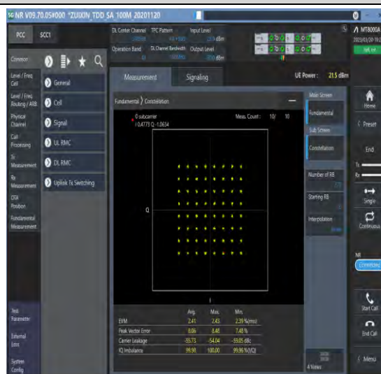
1-N41-30-100-M-8-CP-64QAM-Outer_Full-273@0-Ant1-see graph-PASS
