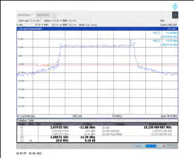
1-N41--30-20-H-6-CP-QPSK-Outer_Full-51@0-Ant1- 18.25-20.000-≤20-PASS
