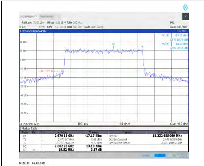
1-N41--30-20-H-7-CP-16QAM-Outer_Full-51@0-Ant 1-18.232-19.520-≤20-PASS
