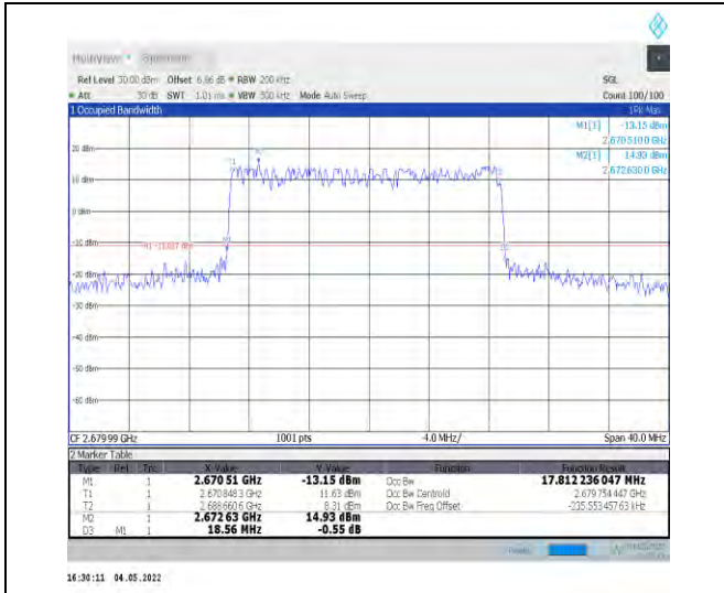
1-N41--30-20-H-3-DFT-16QAM-Outer_Full-50@0-An t1-17.812-18.560-≤20-PASS
