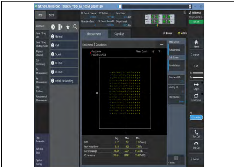
1-N41-30-100-M-9-CP-256QAM-Outer_Full-273@0-Ant1-see graph-PASS
