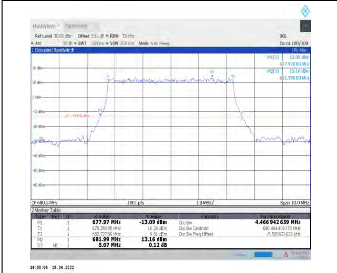
1-N71--15-5-M-2-DFT-PI2BPSK-Outer_Full-25@0-A nt1-4.467-5.070-≤5-PASS
