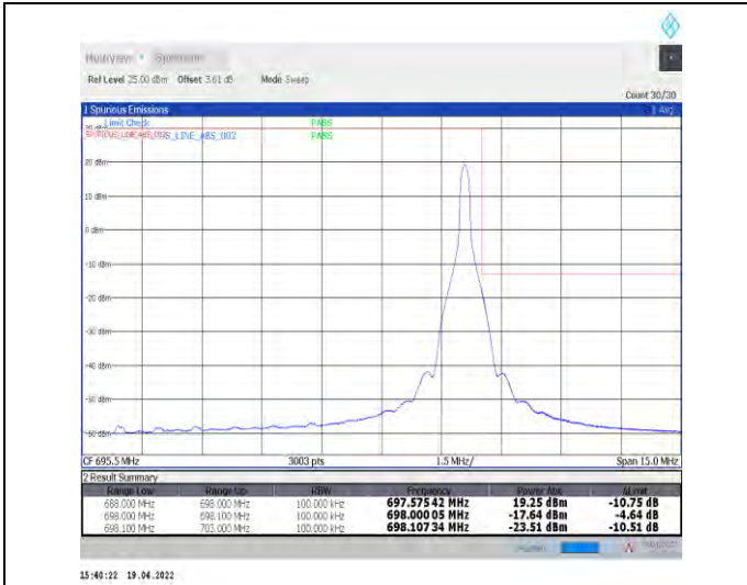
1-N71--15-10-H-2-DFT-PI2BPSK-Edge_1RB_Right-1@ 51-Ant1-PASS-see graph
