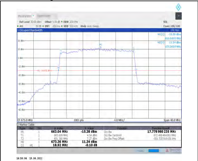
1-N71--15-20-L-5-DFT-256QAM-Outer_Full-100@0-Ant1-17.779-18.920-≤20-PASS
