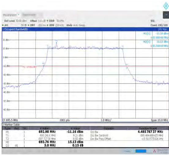
1-N71--15-5-H-1-DFT-QPSK-Outer_Full-25@0-Ant1- 4.486-5.000-≤5-PASS
