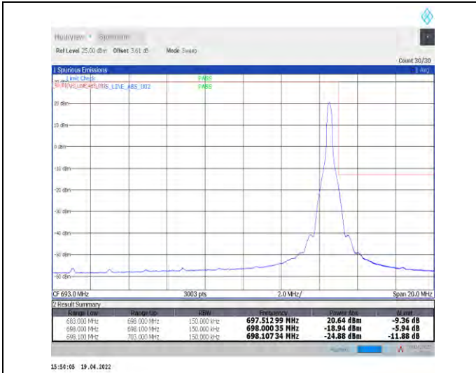
1-N71--15-15-H-2-DFT-PI2BPSK-Edge_1RB_Right-1@78-Ant1-PASS-see graph
