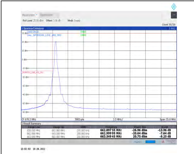
1-N71--15-20-L-1-DFT-PI2BPSK-Edge_1RB_Left-1@0-Ant1-PASS-see graph
