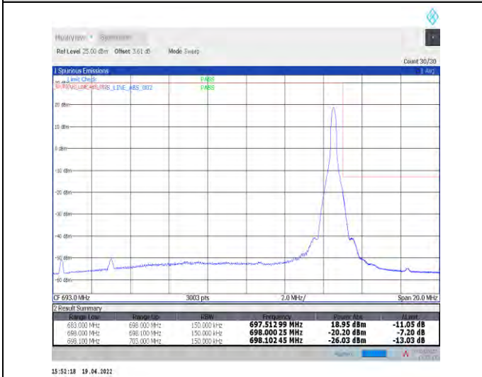
1-N71--15-15-H-5-CP-QPSK-Edge_1RB_Right-1@78-Ant1-PASS-see graph
