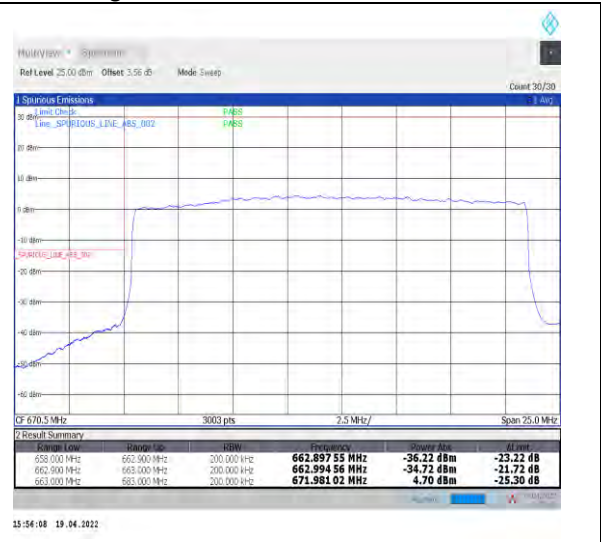
1-N71--15-20-L-3-DFT-PI2BPSK-Outer_Full-100@0-Ant1-PASS-see graph
