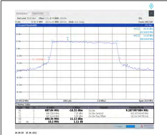
1-N71--15-10-H-8-CP-64QAM-Outer_Full-52@0-Ant 1-9.288-10.200-≤10-PASS
