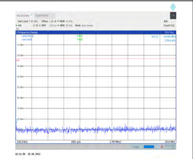
1-N71--15-20-M-1-DFT-PI2BPSK-Inner_1RB_Left-1 @1-0.15-30-Ant1--84.08--23-PASS
