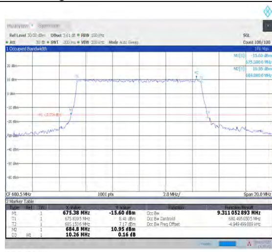
1-N71--15-10-M-6-CP-QPSK-Outer_Full-52@0-Ant1 -9.311-10.260-≤10-PASS
