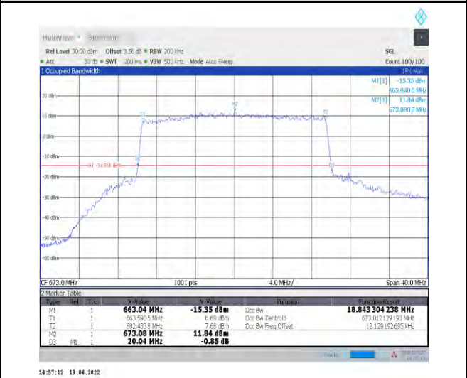
1-N71--15-20-L-7-CP-16QAM-Outer_Full-106@0-Ant1-18.843-20.040-≤20-PASS
