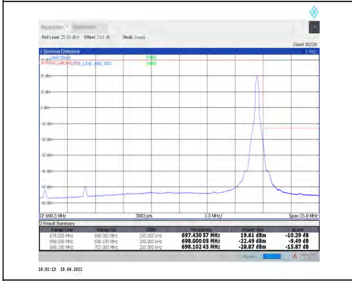
1-N71--15-20-H-5-CP-QPSK-Edge_1RB_Right-1@105-Ant1-PASS-see graph
