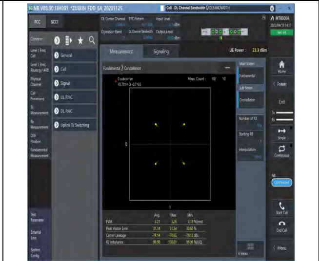
1-N71--15-20-M-2-DFT-QPSK-Outer_Full-100@0-A Ant1-see graph-PASS
