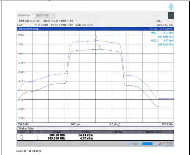
1-N71--15-20-H-2-CP-256QAM-Outer_Full-106@0-Ant1-9.44-100%-0.00-9.44-PASS-≤13
