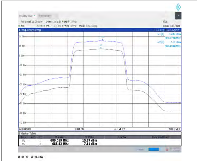
1-N71--15-20-H-1-DFT-256QAM-Outer_Full-100@0-Ant1-8.76-100%-0.00-8.76-PASS-≤13
