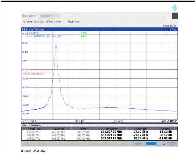
1-N71--15-20-L-4-CP-QPSK-Edge_1RB_Left-1@0-Ant1-PASS-see graph
