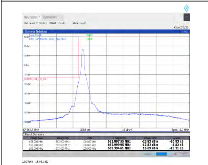
1-N71--15-10-L-4-CP-QPSK-Edge_1RB_Left-1@0-Ant1-PASS-see graph
