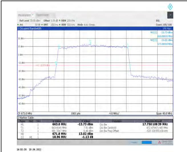
1-N71--15-20-L-4-DFT-64QAM-Outer_Full-100@0-A nt1-17.75-18.960-≤20-PASS
