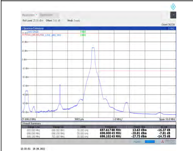
1-N71--15-5-H-5-CP-QPSK-Edge_1RB_Right-1@24-Ant1-PASS-see graph
