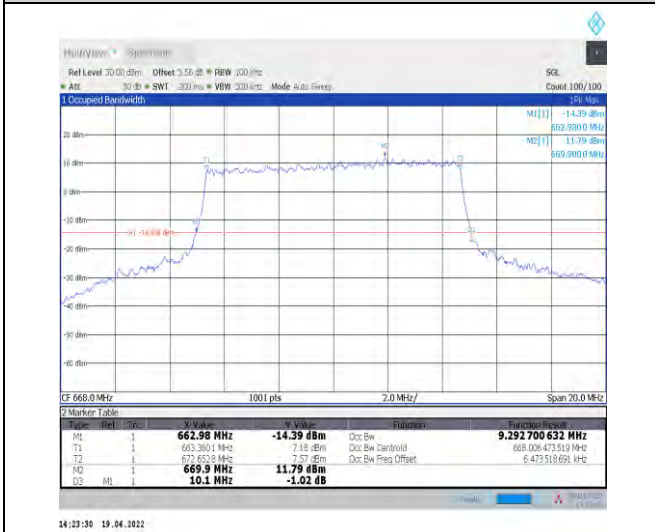
1-N71--15-10-L-8-CP-64QAM-Outer_Full-52@0-Ant1-9.293-10.100-≤10-PASS
