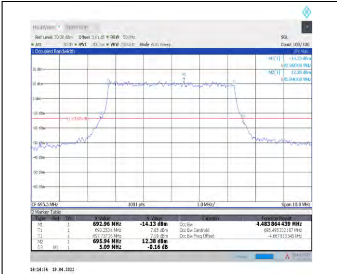
1-N71--15-5-H-3-DFT-16QAM-Outer_Full-25@0-Ant 1-4.484-5.090-≤5-PASS
