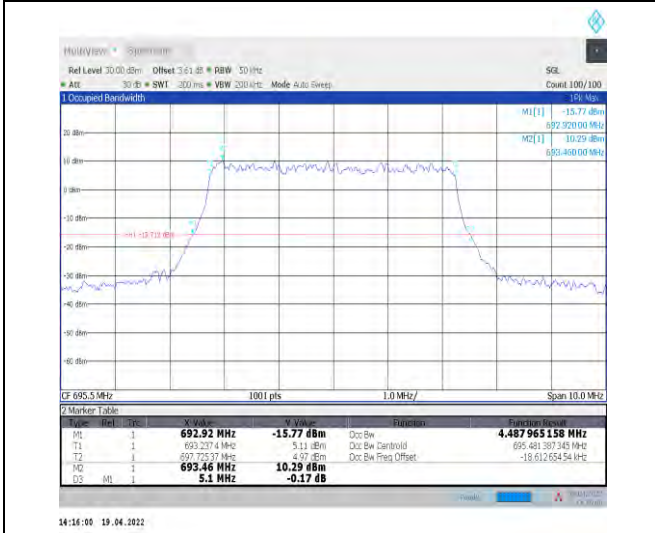
1-N71--15-5-H-5-DFT-256QAM-Outer_Full-25@0-Ant t1-4.488-5.100-≤5-PASS
