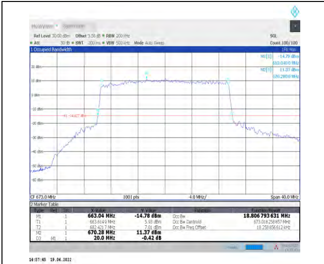
1-N71--15-20-L-8-CP-64QAM-Outer_Full-106@0-Ant 1-18.807-20.000-≤20-PASS
