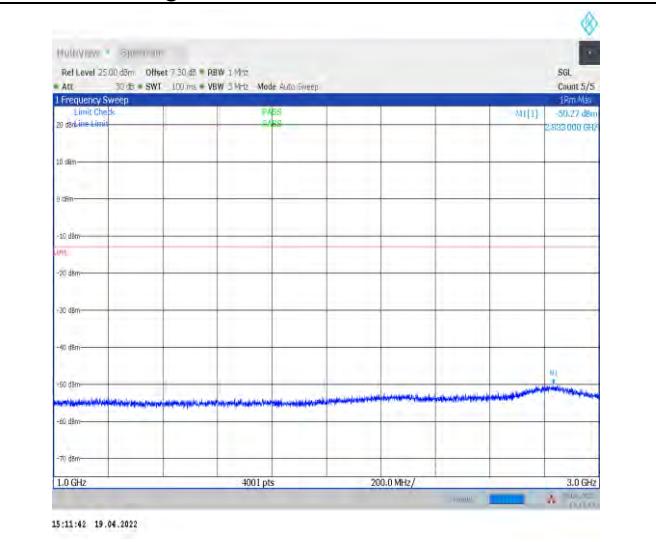
1-N71--15-20-M-1-DFT-PI2BPSK-Inner_1RB_Left-1 @1-1000-3000-Ant1--50.27--13-PASS
