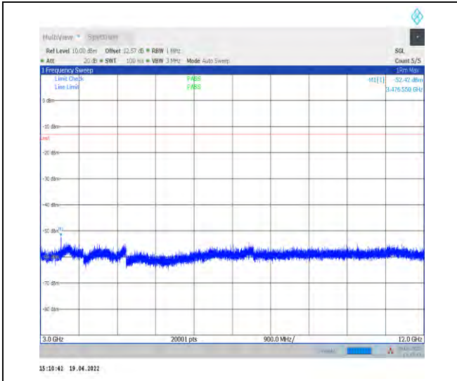
1-N71--15-20-L-1-DFT-PI2BPSK-Inner_1RB_Left-1 @1-3000-12000-Ant1--52.42--13-PASS
