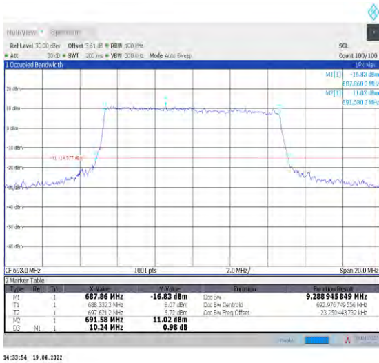
1-N71--15-10-H-6-CP-QPSK-Outer_Full-52@0-Ant1- 9.289-10.240-≤10-PASS
