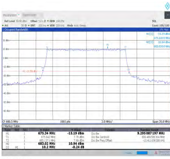
1-N71--15-10-M-7-CP-16QAM-Outer_Full-52@0-Ant 1-9.295-10.200-≤10-PASS
