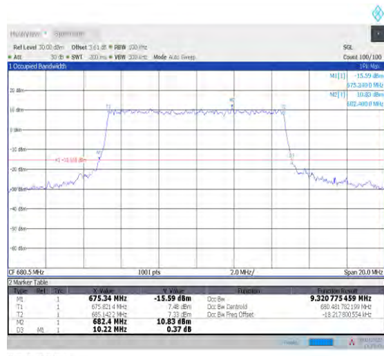
1-N71--15-10-M-8-CP-64QAM-Outer_Full-52@0-Ant 1-9.321-10.220-≤10-PASS
