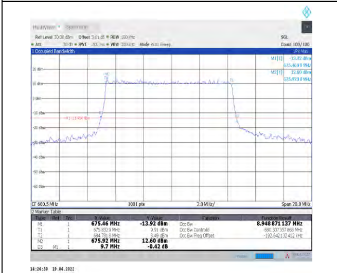
1-N71--15-10-M-3-DFT-16QAM-Outer_Full-50@0-Ant t1-8.949-9.700-≤10-PASS
