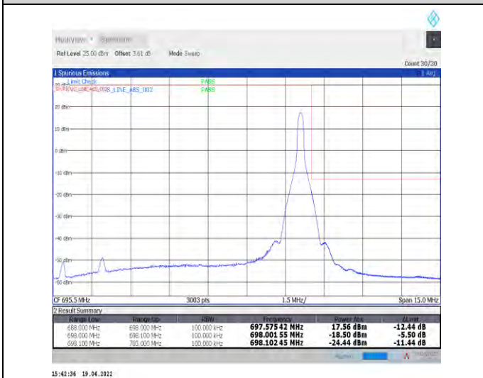
1-N71--15-10-H-5-CP-QPSK-Edge_1RB_Right-1@51- Ant1-PASS-see graph
