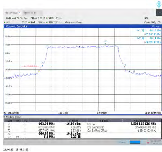
1-N71--15-5-L-6-CP-QPSK-Outer_Full-25@0-Ant1-4 .501-5.200-≤5-PASS
