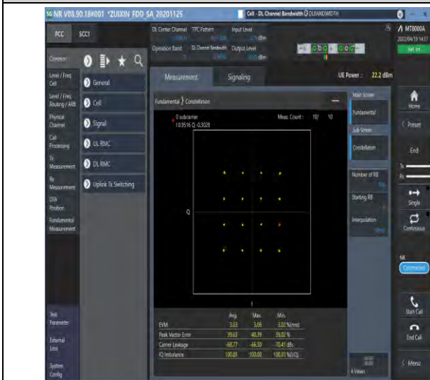
1-N71--15-20-M-3-DFT-16QAM-Outer_Full-100@0-A Ant1-see graph-PASS
