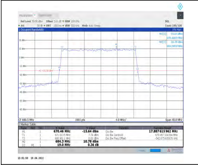
1-N71--15-20-M-5-DFT-256QAM-Outer_Full-100@0-Ant1-17.888-19.000-≤20-PASS
