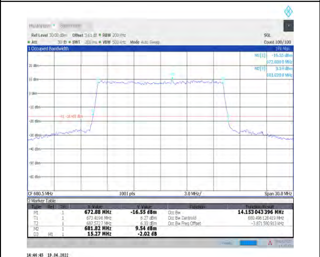
1-N71--15-15-M-9-CP-256QAM-Outer_Full-79@0-Ant-14.153-15.270-≤15-PASS
