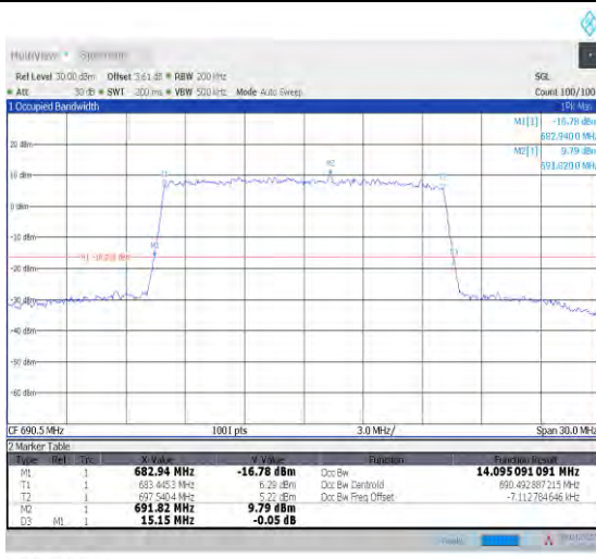
1-N71--15-15-H-9-CP-256QAM-Outer_Full-79@0-Ant t1-14.095-15.150-<=15-PASS
