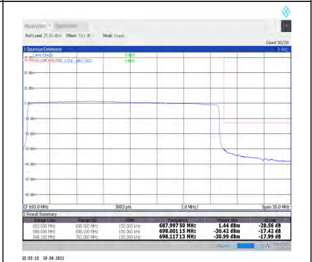
1-N71--15-15-H-6-CP-QPSK-Outer_Full-79@0-Ant1-PASS-see graph
