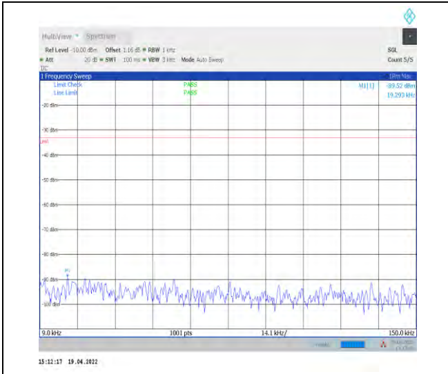
1-N71--15-20-H-1-DFT-PI2BPSK-Inner_1RB_Left-1 @1-0.009-0.15-Ant1--89.52--33-PASS
