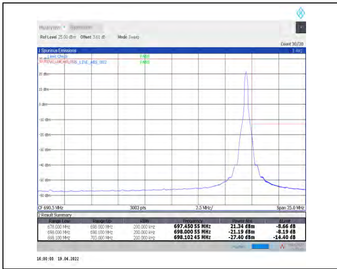
1-N71--15-20-H-2-DFT-PI2BPSK-Edge_1RB_Right-1@105-Ant1-PASS-see graph
