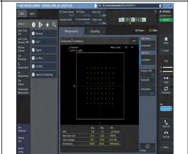
1-N71--15-20-M-4-DFT-64QAM-Outer_Full-100@0-A Ant1-see graph-PASS
