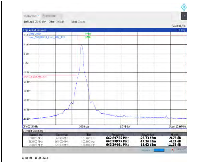
1-N71--15-10-L-1-DFT-PI2BPSK-Edge_1RB_Left-1@0-Ant1-PASS-see graph
