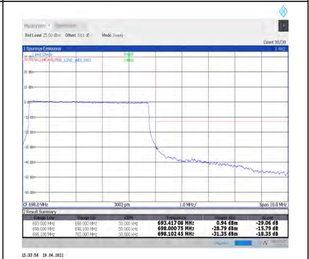
1-N71--15-5-H-6-CP-QPSK-Outer_Full-25@0-Ant1-PASS-see graph
