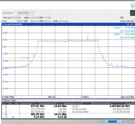
1-N71--15-5-M-8-CP-64QAM-Outer_Full-25@0-Ant1 -4.493-5.190-≤5-PASS
