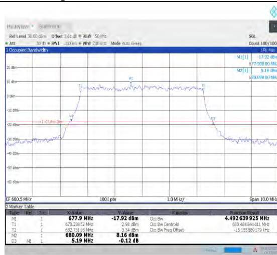
1-N71--15-5-M-9-CP-256QAM-Outer_Full-25@0-Ant 1-4.493-5.190-≤5-PASS
