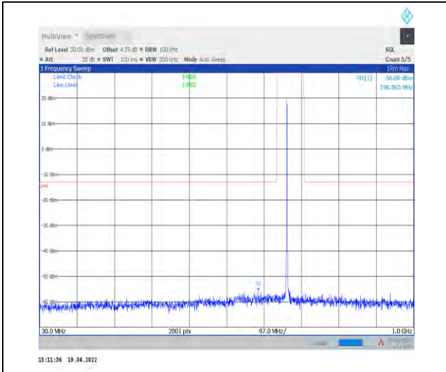
1-N71--15-20-M-1-DFT-PI2BPSK-Inner_1RB_Left-1 @1-30-1000-Ant1--56.06--13-PASS
