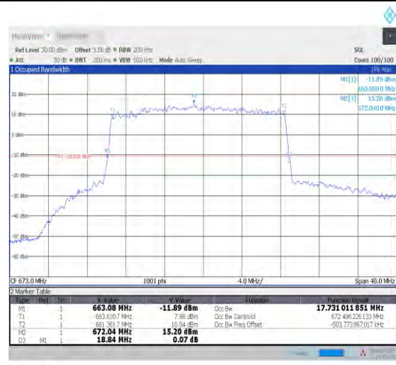
1-N71--15-20-L-1-DFT-QPSK-Outer_Full-100@0-Ant 1-17.731-18.840-<=20-PASS
