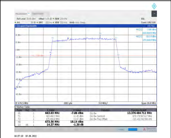
1-N71--15-15-L-2-DFT-PI2BPSK-Outer_Full-75@0-Ant1 -13.376-14.370-≤15-PASS
