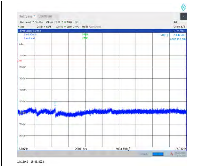
1-N71--15-20-H-1-DFT-PI2BPSK-Inner_1RB_Left-1 @1-3000-12000-Ant1--54.42--13-PASS
