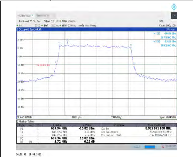
1-N71--15-10-H-1-DFT-QPSK-Outer_Full-50@0-Ant 1-8.93-9.720≤10-PASS
