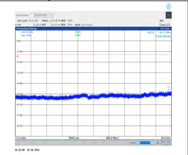
1-N71--15-20-L-1-DFT-PI2BPSK-Inner_1RB_Left-1 @1-12000-20000-Ant1--46.79--13-PASS
