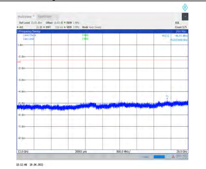
1-N71--15-20-H-1-DFT-PI2BPSK-Inner_1RB_Left-1 @1-12000-20000-Ant1--46.91--13-PASS
