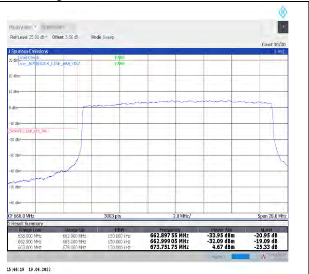
1-N71--15-15-L-3-DFT-PI2BPSK-Outer_Full-75@0-Ant1-PASS-see graph
