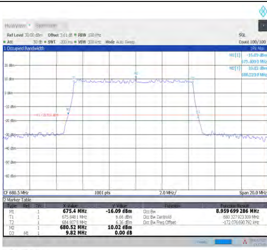
1-N71--15-10-M-5-DFT-256QAM-Outer_Full-50@0-A nt1-8.96-9.820-≤10-PASS
