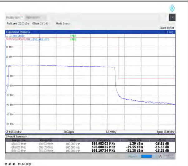
1-N71--15-10-H-6-CP-QPSK-Outer_Full-52@0-An t1-PASS-see graph
