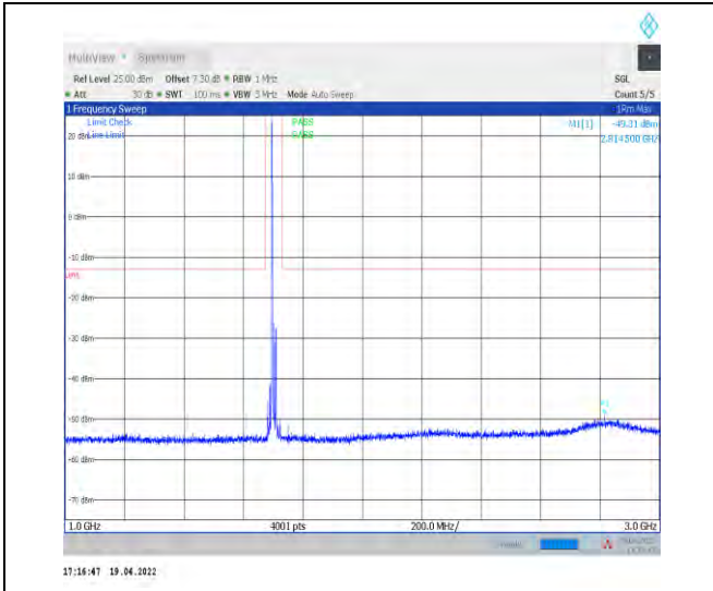
1-N70--15-15-M-1-DFT-PI2BPSK-Inner_1RB_Left-1 @1-1000-3000-Ant1--49.31--13-PASS
