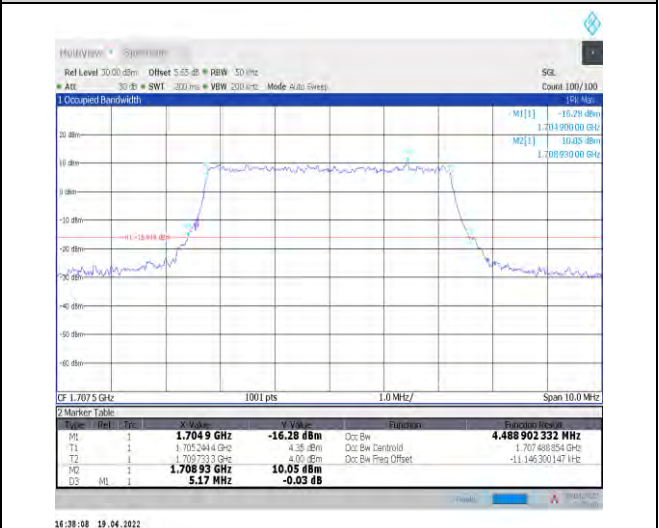
1-N70--15-5-H-6-CP-QPSK-Outer_Full-25@0-Ant1-4 .489-5.170-≤5-PASS
