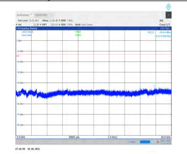
1-N70--15-15-M-1-DFT-PI2BPSK-Inner_1RB_Left-1 @1-3000-18000-Ant1--43.64--13-PASS
