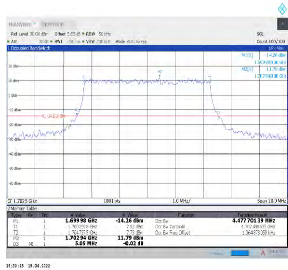
1-N70--15-5-M-3-DFT-16QAM-Outer_Full-25@0-Ant1 1-4.478-5.050-≤5-PASS
