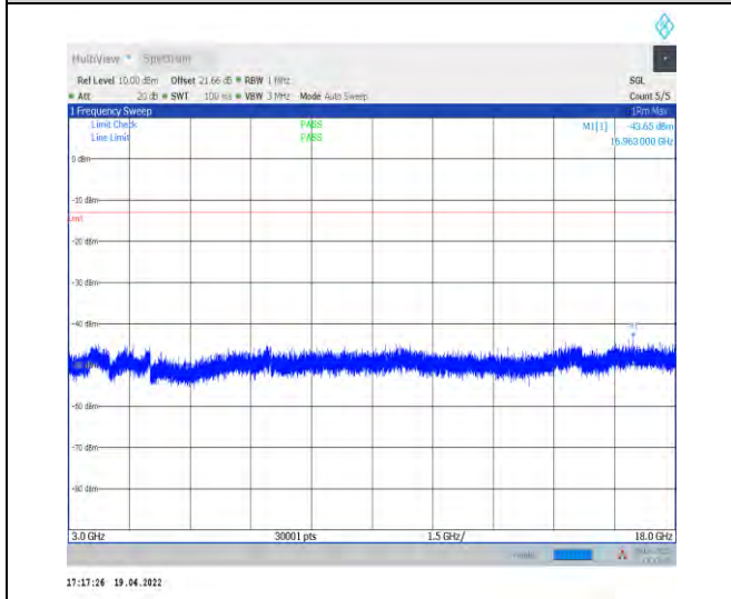
1-N70--15-15-H-1-DFT-PI2BPSK-Inner_1RB_Left-1 @1-3000-18000-Ant1--43.65--13-PASS
