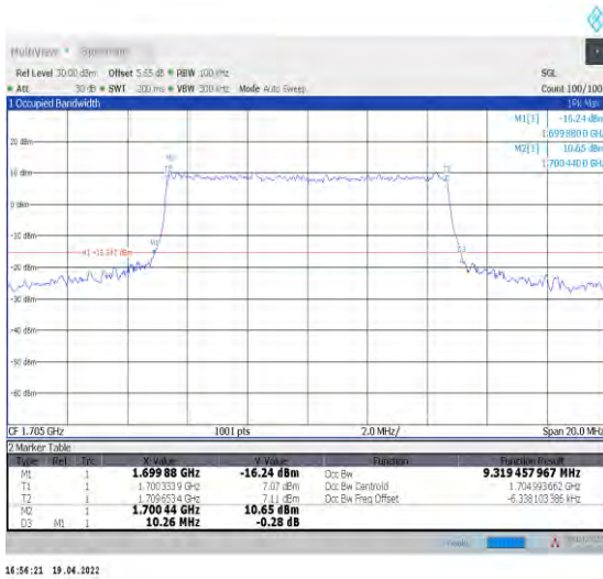
1-N70--15-10-H-6-CP-QPSK-Outer_Full-52@0-Ant1- 9.319-10.260-≤10-PASS
