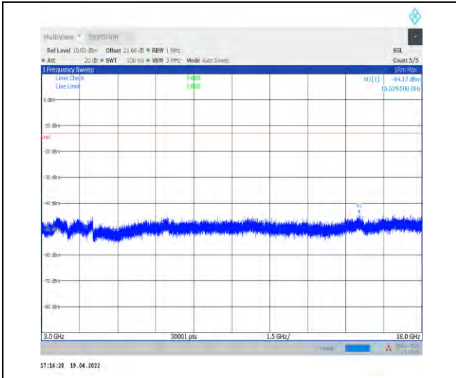
1-N70--15-15-L-1-DFT-PI2BPSK-Inner_1RB_Left-1 @1-3000-18000-Ant1--44.17--13-PASS
