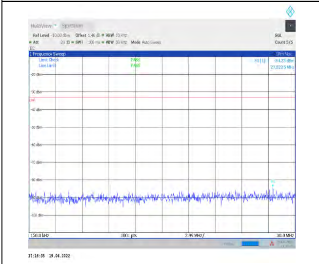
1-N70--15-15-M-1-DFT-PI2BPSK-Inner_1RB_Left-1 @1-0.15-30-Ant1--84.23--33-PASS
