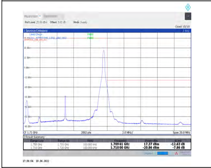
1-N70--15-10-H-5-CP-QPSK-Edge_1RB_Right-1@51-Ant1-seegraph-PASS-see graph
