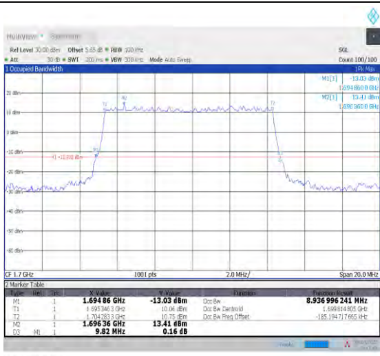
1-N70--15-10-L-2-DFT-PI2BPSK-Outer_Full-50@0-A nt1-8.937-9.820-≤10-PASS
