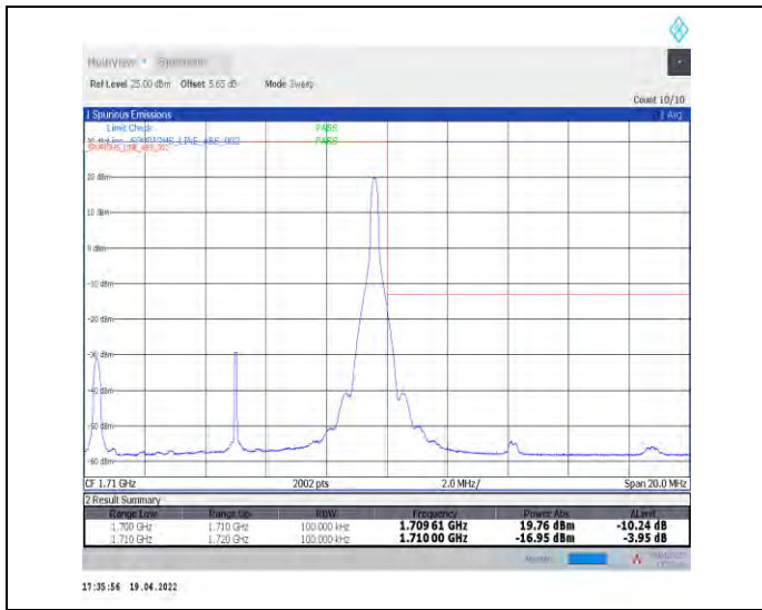
1-N70--15-10-H-2-DFT-PI2BPSK-Edge_1RB_Right-1@51-Ant1-seegraph-PASS-see graph
