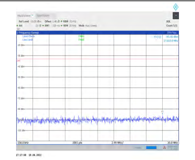
1-N70--15-15-H-1-DFT-PI2BPSK-Inner_1RB_Left-1 @1-0.15-30-Ant1--85.45--33-PASS
