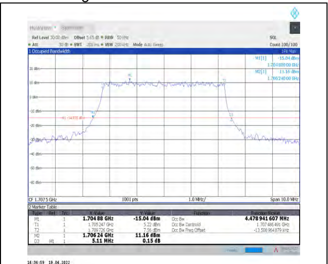
1-N70--15-5-H-4-DFT-64QAM-Outer_Full-25@0-Ant 1-4.479-5.110-≤5-PASS
