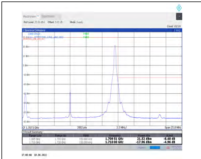
1-N70--15-15-H-2-DFT-PI2BPSK-Edge_1RB_Right-1@78-Ant1-seegraph-PASS-see graph
