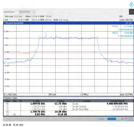
1-N70--15-5-M-1-DFT-QPSK-Outer_Full-25@0-Ant1 -4.487-5.030-≤5-PASS
