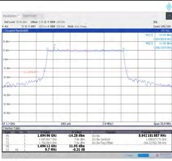
1-N70--15-10-L-4-DFT-64QAM-Outer_Full-50@0-Ant 1-8.942-9.700-≤10-PASS
