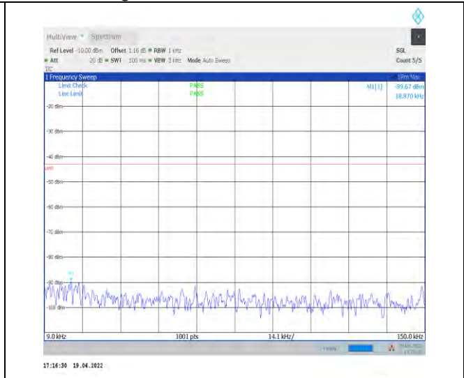
1-N70--15-15-M-1-DFT-PI2BPSK-Inner_1RB_Left-1 @1-0.009-0.15-Ant1--89.67--43-PASS
