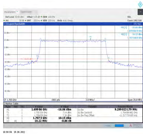
1-N70--15-10-H-7-CP-16QAM-Outer_Full-52@0-Ant 1-9.299-10.220-≤10-PASS
