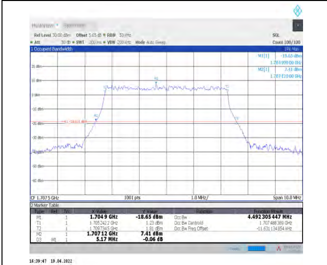
1-N70--15-5-H-9-CP-256QAM-Outer_Full-25@0-Ant 1-4.492-5.170-≤5-PASS
