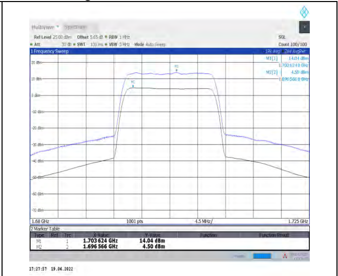
1-N70--15-15-H-2-CP-256QAM-Outer_Full-79@0-A nt1-9.54-100%-0.00-9.54-PASS-≤13
