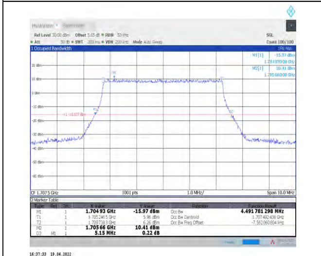
1-N70--15-5-H-5-DFT-256QAM-Outer_Full-25@0-Ant t1-4.492-5.150-≤5-PASS
