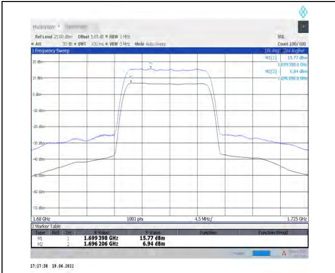
1-N70--15-15-H-1-DFT-256QAM-Outer_Full-75@0-A nt1-8.83-100%-0.00-8.83-PASS-≤13
