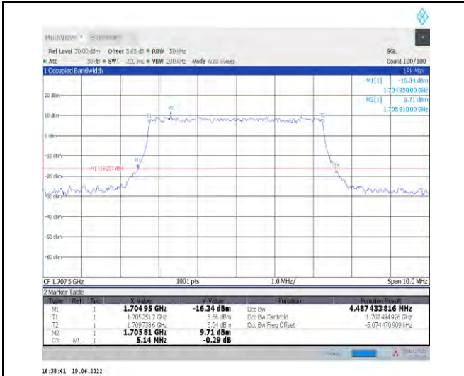
1-N70--15-5-H-7-CP-16QAM-Outer_Full-25@0-Ant1 4.487-5.140-≤5-PASS
