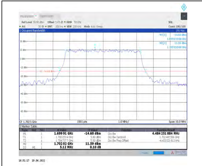
1-N70--15-5-M-4-DFT-64QAM-Outer_Full-25@0-Ant 1-4.484-5.120-≤5-PASS
