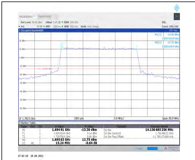
1-N70--15-15-L-7-CP-16QAM-Outer_Full-79@0-Ant1 -14.137-15.240-≤15-PASS
