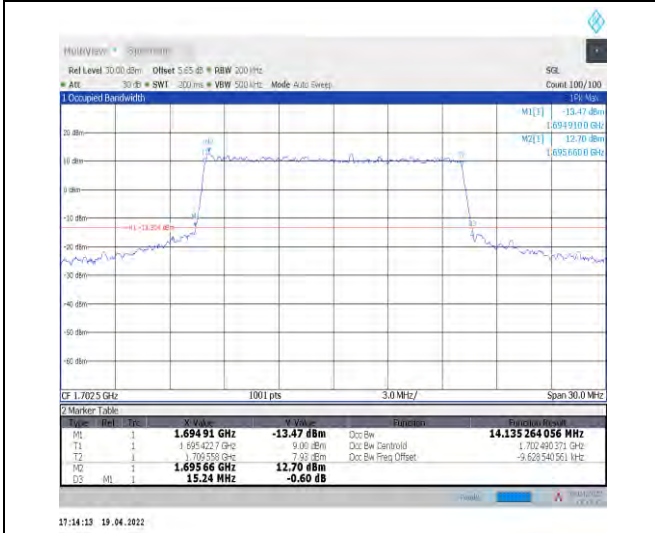
1-N70--15-15-H-7-CP-16QAM-Outer_Full-79@0-Ant 1-14.135-15.240-≤15-PASS
