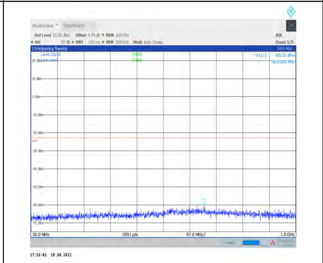
1-N70--15-15-M-1-DFT-PI2BPSK-Inner_1RB_Left-1 @1-30-1000-Ant1--60.33--23-PASS
