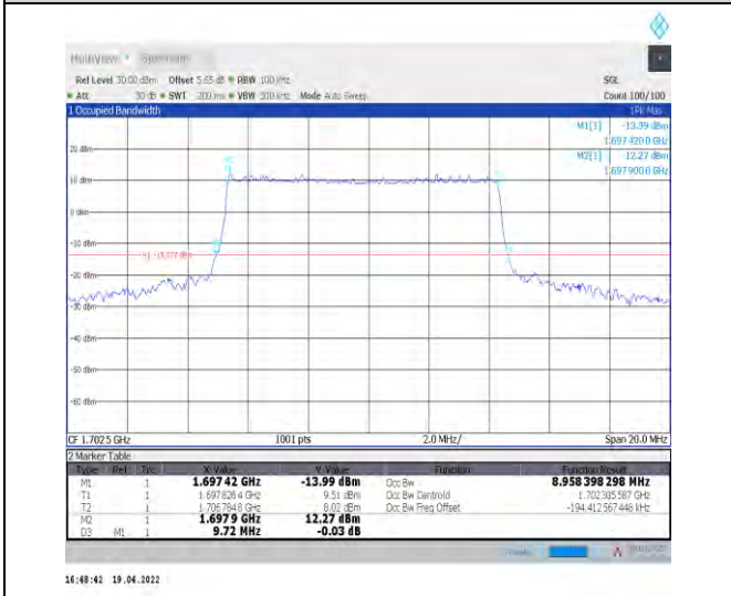
1-N70--15-10-M-3-DFT-16QAM-Outer_Full-50@0-Ant t1-8.958-9.720-≤10-PASS
