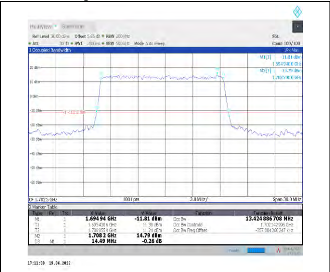
1-N70--15-15-H-2-DFT-PI2BPSK-Outer_Full-75@0-Ant1-13.425-14.490-≤15-PASS
