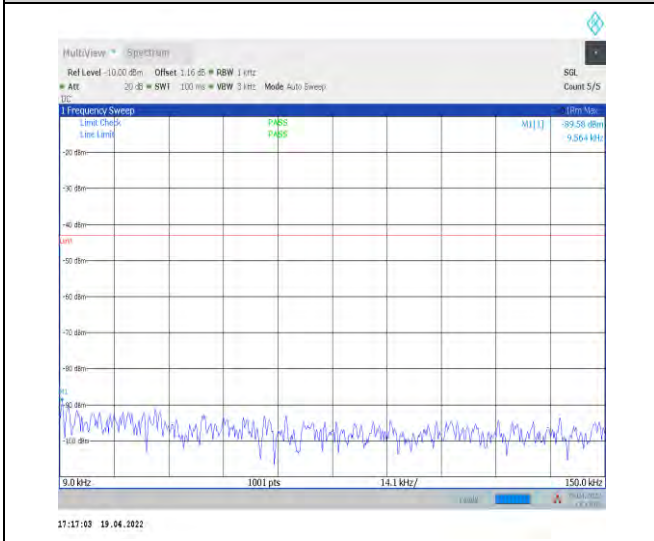
1-N70--15-15-H-1-DFT-PI2BPSK-Inner_1RB_Left-1 @1-0.009-0.15-Ant1--89.58--43-PASS
