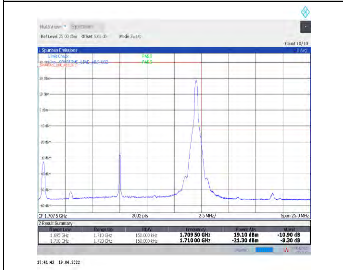
1-N70--15-15-H-5-CP-QPSK-Edge_1RB_Right-1@78-Ant1-seegraph-PASS-see graph
