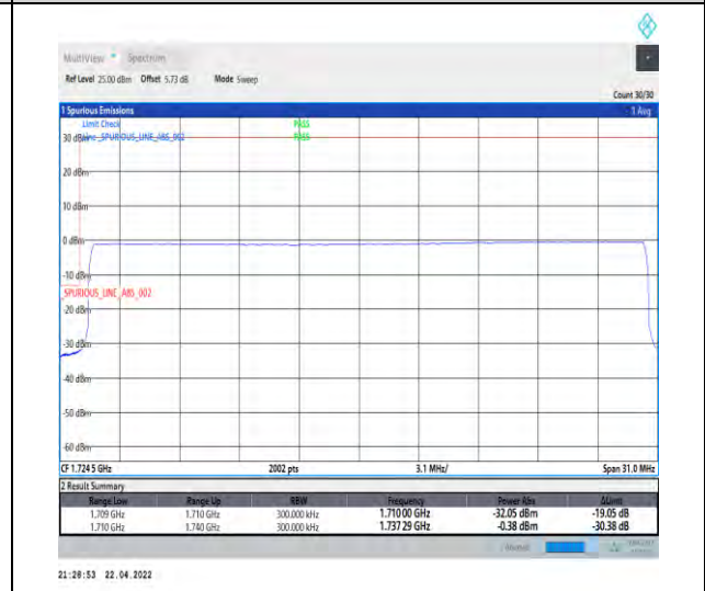
1-N66-PC3-15-30-L-6-CP-QPSK-Outer_Full-160@0-Ant1-seegraph-PASS-see graph
