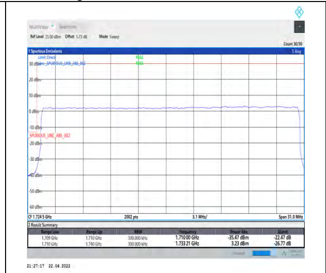
1-N66-PC3-15-30-L-3-DFT-PI2BPSK-Outer_Full-160@0-Ant1-seegraph-PASS-see graph
