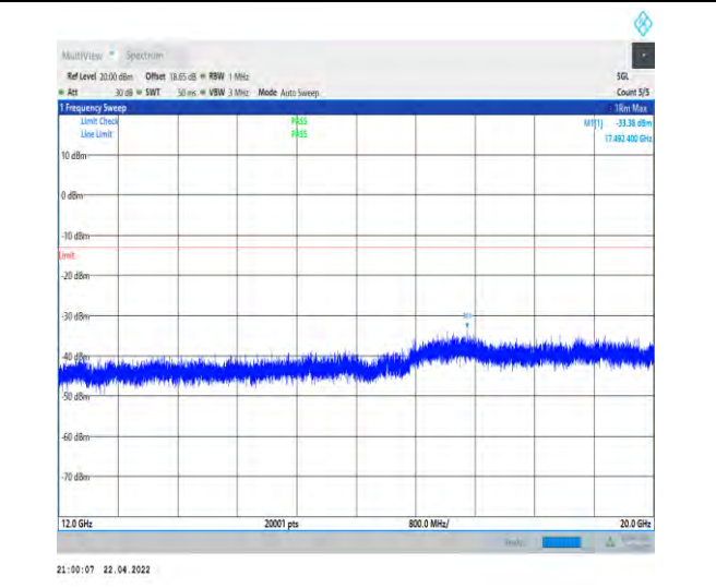
1-N66-PC3-15-40-M-1-DFT-PI2BPSK-Inner_1RB_Le ft-1@1-12000-20000-Ant1--33.38--13-PASS
