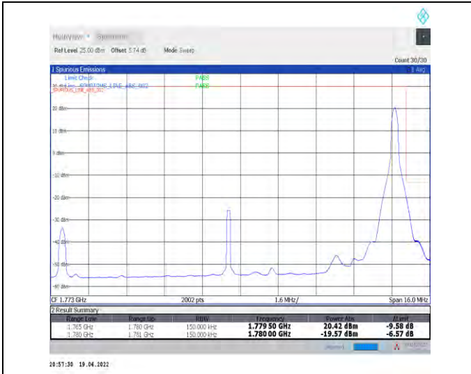
1-N66-PC3-15-15-H-2-DFT-PI2BPSK-Edge_1RB_Right-t-1@78-Ant1-seegraph-PASS-see graph
