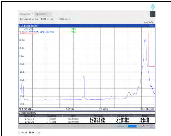
1-N66-PC3-15-20-H-2-DFT-PI2BPSK-Edge_1RB_Right-t-1@105-Ant1-seegraph-PASS-see graph
