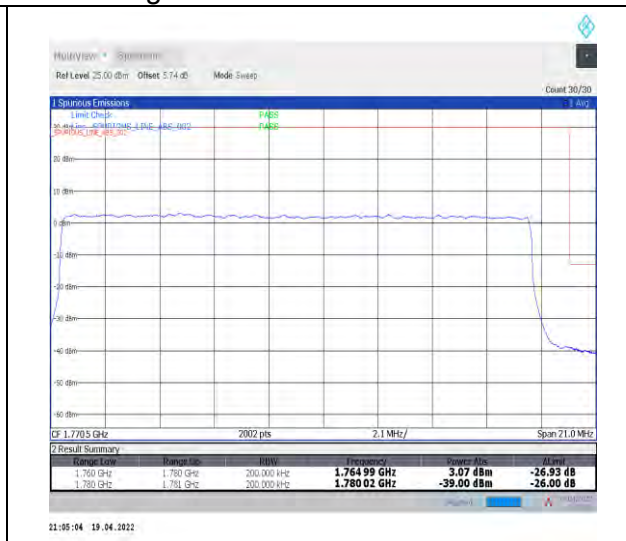
1-N66-PC3-15-20-H-3-DFT-PI2BPSK-Outer_Full-100@0-Ant1-seegraph-PASS-see graph
