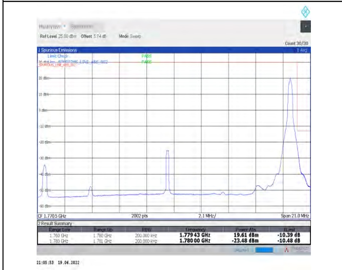
1-N66-PC3-15-20-H-5-CP-QPSK-Edge_1RB_Right-1@105-Ant1-seegraph-PASS-see graph
