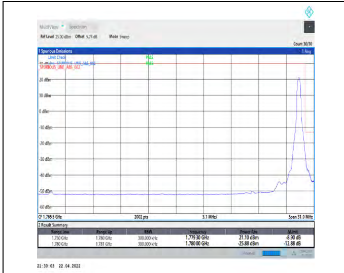
1-N66-PC3-15-30-H-2-DFT-PI2BPSK-Edge_1RB_Right-t1@159-Ant1-seegraph-PASS-see graph
