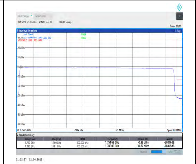
1-N66-PC3-15-30-H-6-CP-QPSK-Outer_Full-160@0-Ant1-seegraph-PASS-see graph
