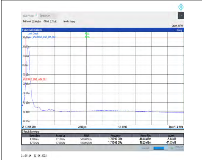
1-N66-PC3-15-40-L-4-CP-QPSK-Edge_1RB_Left-1@0-Ant1-seegraph-PASS-see graph
