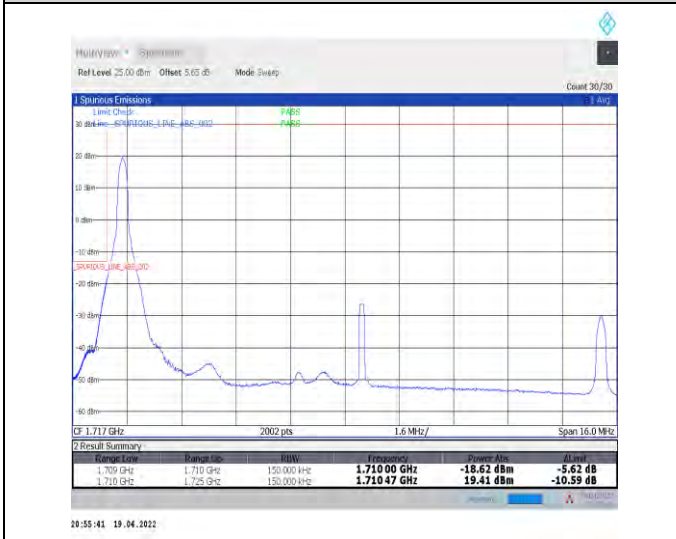
1-N66-PC3-15-15-L-4-CP-QPSK-Edge_1RB_Left-1@0-Ant1-seegraph-PASS-see graph
