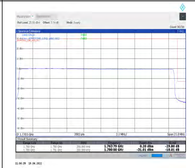
1-N66-PC3-15-20-H-6-CP-QPSK-Outer_Full-106@0-Ant1-seegraph-PASS-see graph
