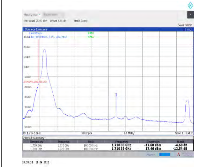
1-N66-PC3-15-10-L-4-CP-QPSK-Edge_1RB_Left-1@0-Ant1-seegraph-PASS-see graph
