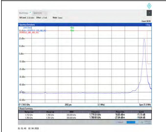
1-N66-PC3-15-30-H-5-CP-QPSK-Edge_1RB_Right-1@159-Ant1-seegraph-PASS-see graph
