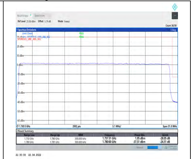
1-N66-PC3-15-30-H-3-DFT-PI2BPSK-Outer_Full-160@0-Ant1-seegraph-PASS-see graph
