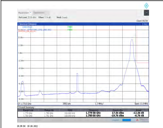
1-N66-PC3-15-10-H-5-CP-QPSK-Edge_1RB_Right-1@51-Ant1-seegraph-PASS-see graph
