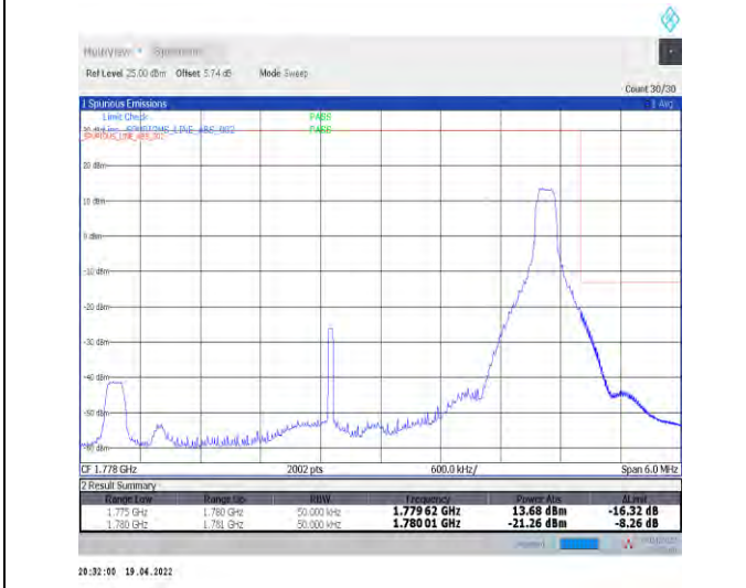
1-N66-PC3-15-5-H-5-CP-QPSK-Edge_1RB_Right-1@24-Ant1-seegraph-PASS-see graph
