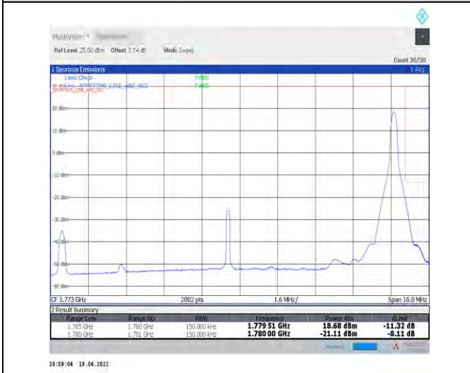
1-N66-PC3-15-15-H-5-CP-QPSK-Edge_1RB_Right-1@78-Ant1-seegraph-PASS-see graph
