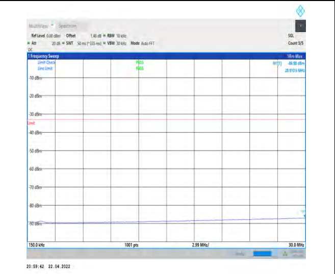
1-N66-PC3-15-40-M-1-DFT-PI2BPSK-Inner_1RB_Le ft-1@1-0.15-30-Ant1--86.88--33-PASS
