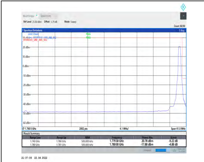
1-N66-PC3-15-40-H-2-DFT-PI2BPSK-Edge_1RB_Right-t1@215-Ant1-seegraph-PASS-see graph
