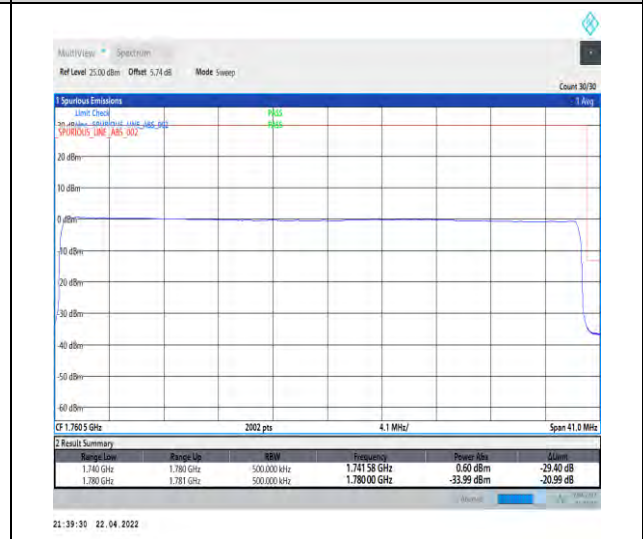
1-N66-PC3-15-40-H-6-CP-QPSK-Outer_Full-216@0-Ant1-seegraph-PASS-see graph
