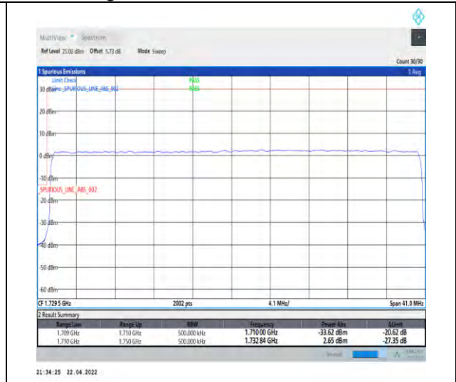
1-N66-PC3-15-40-L-3-DFT-PI2BPSK-Outer_Full-216@0-Ant1-seegraph-PASS-see graph
