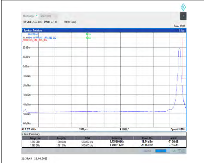
1-N66-PC3-15-40-H-5-CP-QPSK-Edge_1RB_Right-1@215-Ant1-seegraph-PASS-see graph
