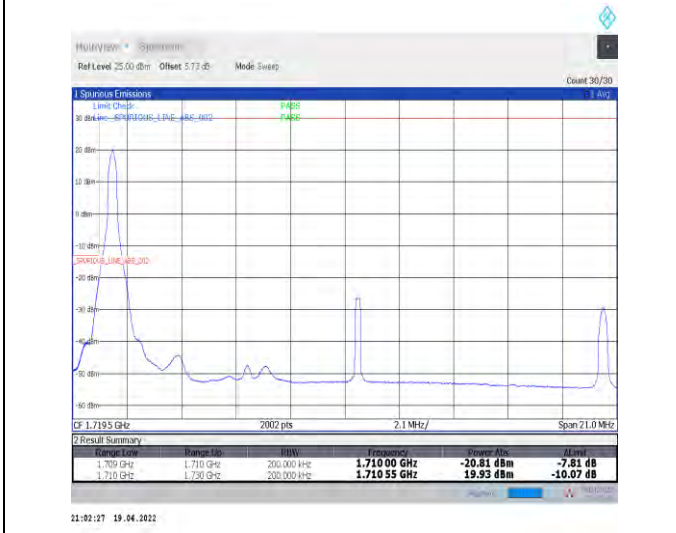
1-N66-PC3-15-20-L-4-CP-QPSK-Edge_1RB_Left-1@0-Ant1-seegraph-PASS-see graph
