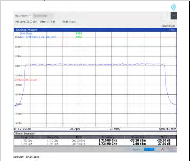
1-N66-PC3-15-20-L-3-DFT-PI2BPSK-Outer_Full-100@0-Ant1-seegraph-PASS-see graph
