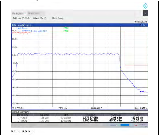
1-N66-PC3-15-5-H-3-DFT-PI2BPSK-Outer_Full-25@0-Ant1-seegraph-PASS-see graph
