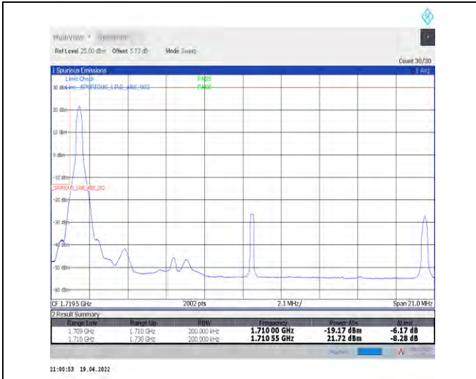
1-N66-PC3-15-20-L-1-DFT-PI2BPSK-Edge_1RB_Left-1@0-Ant1-seegraph-PASS-see graph
