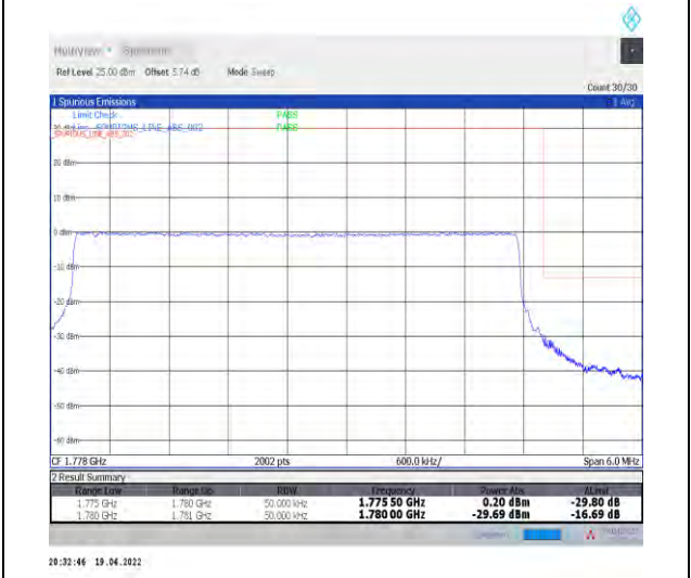
1-N66-PC3-15-5-H-6-CP-QPSK-Outer_Full-25@0-Ant1-seegraph-PASS-see graph
