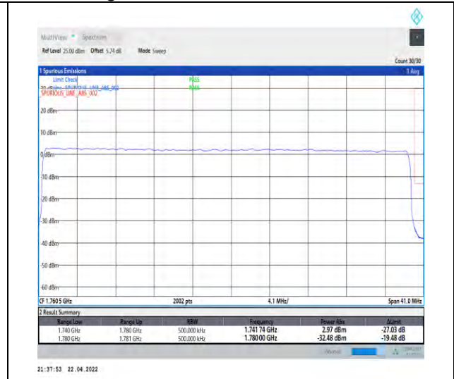
1-N66-PC3-15-40-H-3-DFT-PI2BPSK-Outer_Full-216@0-Ant1-seegraph-PASS-see graph
