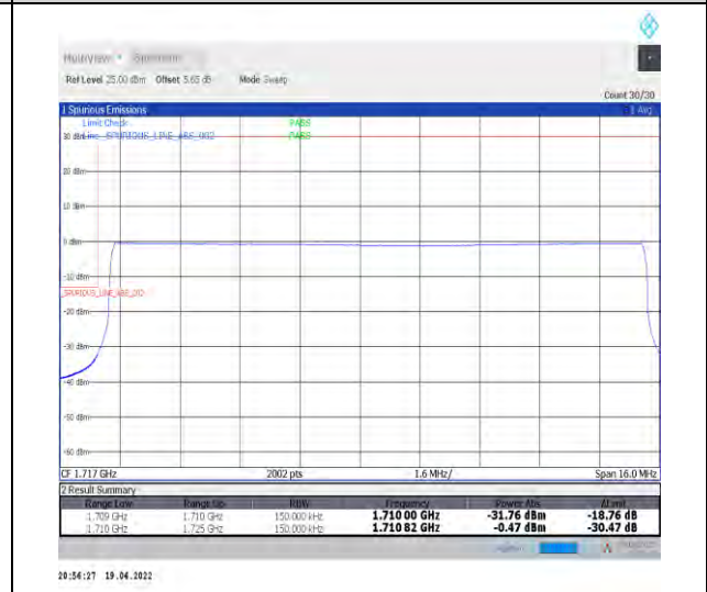
1-N66-PC3-15-15-L-6-CP-QPSK-Outer_Full-79@0-Ant1-seegraph-PASS-see graph
