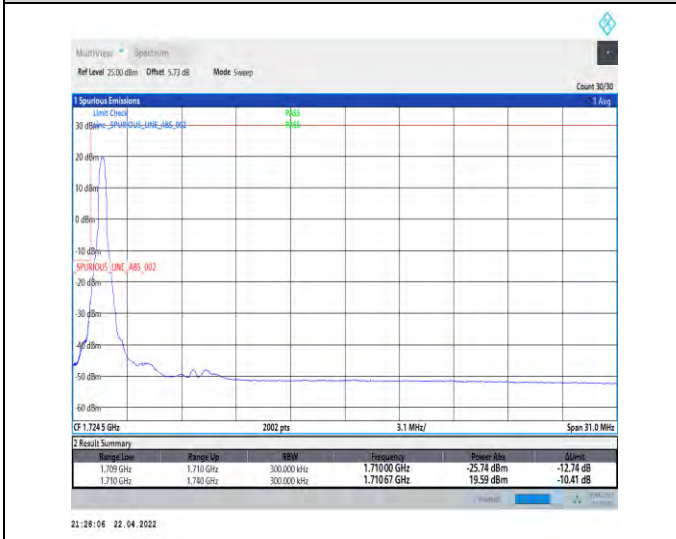
1-N66-PC3-15-30-L-4-CP-QPSK-Edge_1RB_Left-1@0-Ant1-seegraph-PASS-see graph
