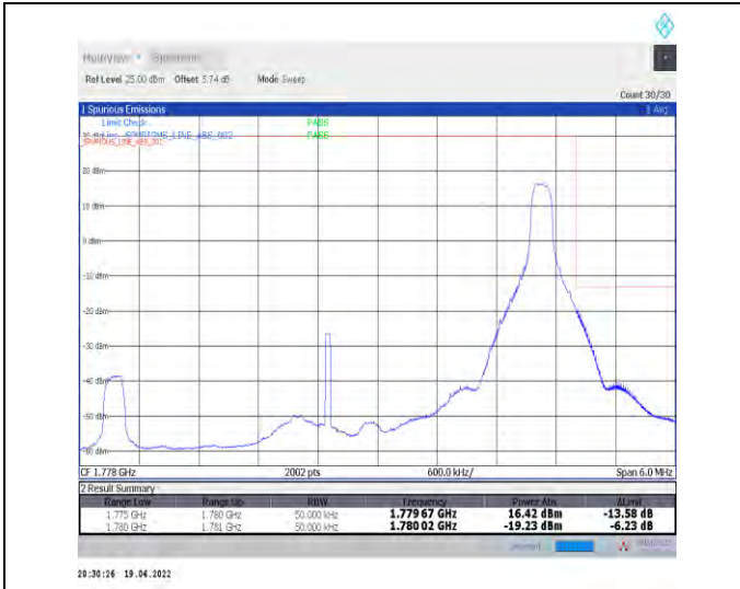
1-N66-PC3-15-5-H-2-DFT-PI2BPSK-Edge_1RB_Right-1@24-Ant1-seegraph-PASS-see graph
