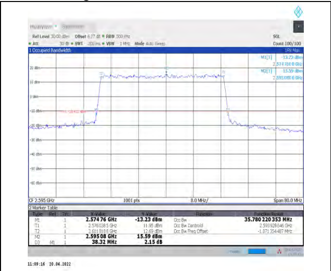
1-N38--30-40-M-1-DFT-QPSK-Outer_Full-100@0-An t1-35.78-38.320-<40-PASS
