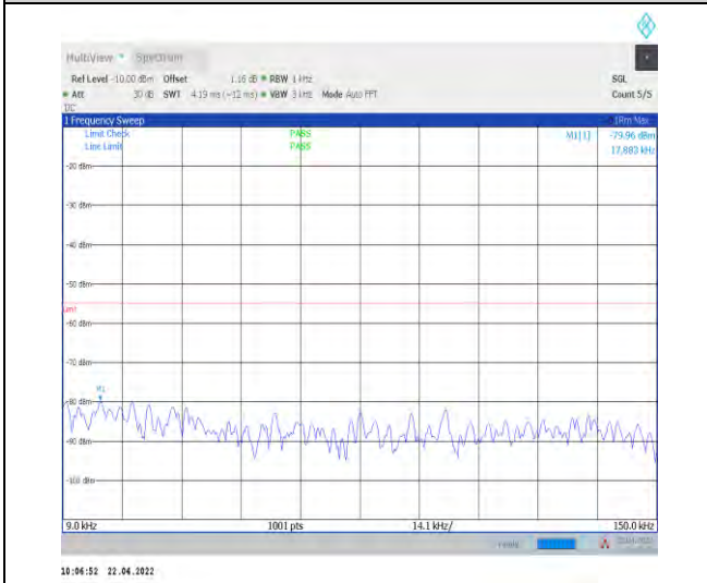
1-N38--30-40-M-1-DFT-PI2BPSK-Inner_1RB_Left-1 @1-0.009-0.15-Ant1--79.96--55-PASS
