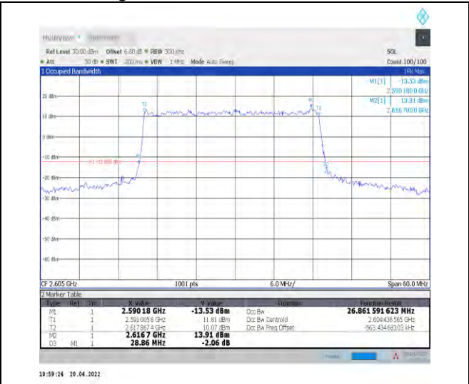
1-N38--30-30-H-3-DFT-16QAM-Outer_Full-75@0-An t1-26.862-28.860-<=30-PASS
