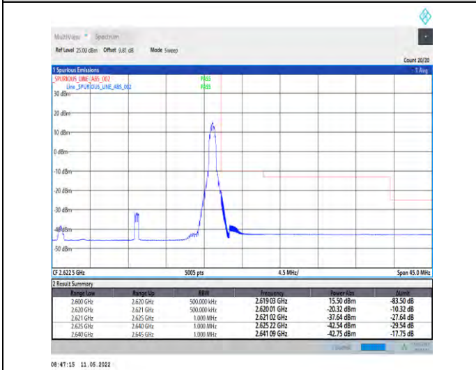
1-N38-PC2-30-20-H-5-CP-QPSK-Edge_1RB_Right-1@50-Ant1-PASS-see graph
