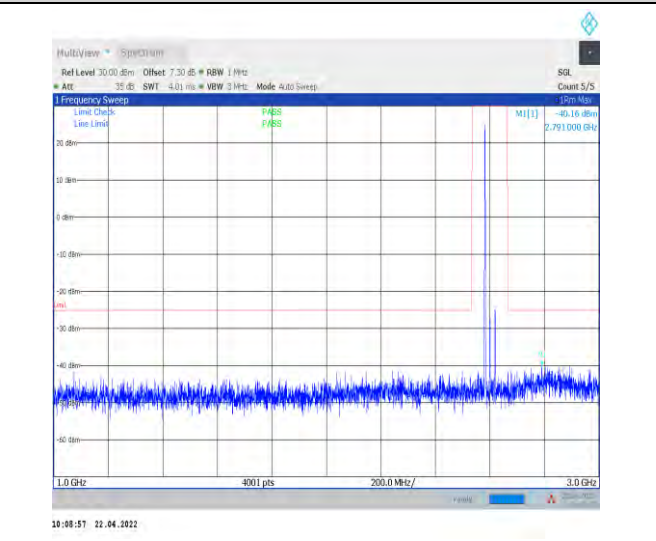
1-N38--30-40-H-1-DFT-PI2BPSK-Inner_1RB_Left-1 @1-1000-3000-Ant1--40.16--25-PASS
