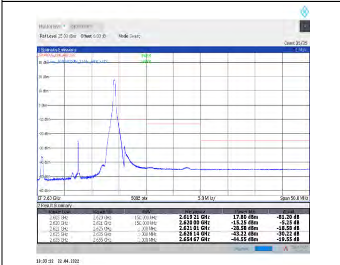
1-N38--30-15-H-5-CP-QPSK-Edge_1RB_Right-1@37-Ant1-PASS-see graph
