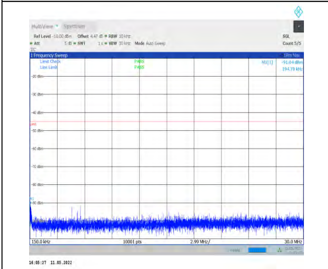
1-N38-PC2-30-40-H-1-DFT-QPSK-Edge_1RB_Left-1 @0-0.15-30-Ant1--91.04--45-PASS
