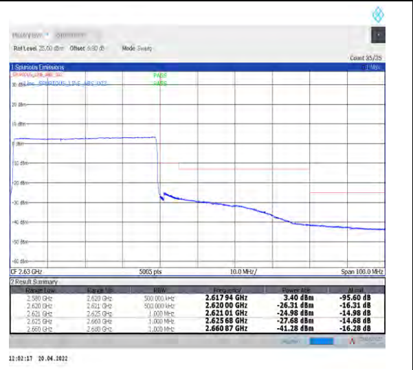
1-N38--30-40-H-6-CP-QPSK-Outer_Full-106@0-Ant1-PASS-see graph
