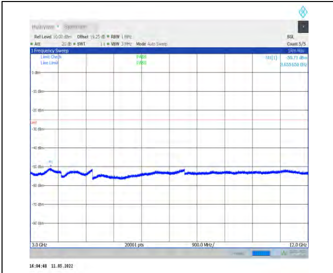
1-N38-PC2-30-40-M-1-DFT-QPSK-Edge_1RB_Left-1 @0-3000-12000-Ant1--50.71--25-PASS
