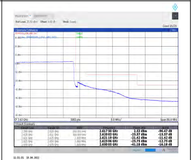
1-N38--30-30-H-6-CP-QPSK-Outer_Full-78@0-Ant1-PASS-see graph
