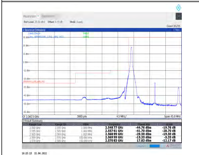
1-N38--30-15-L-4-CP-QPSK-Edge_1RB_Left-1@0-Ant1-PASS-see graph
