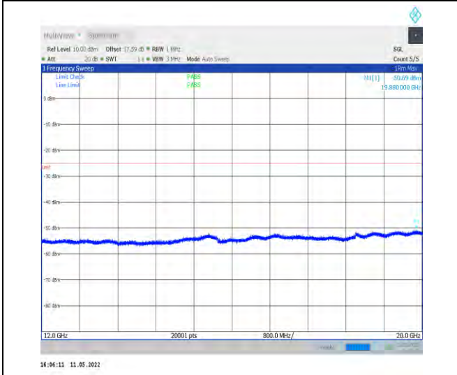
1-N38-PC2-30-40-H-1-DFT-QPSK-Edge_1RB_Left-1 @0-12000-20000-Ant1--50.69--25-PASS
