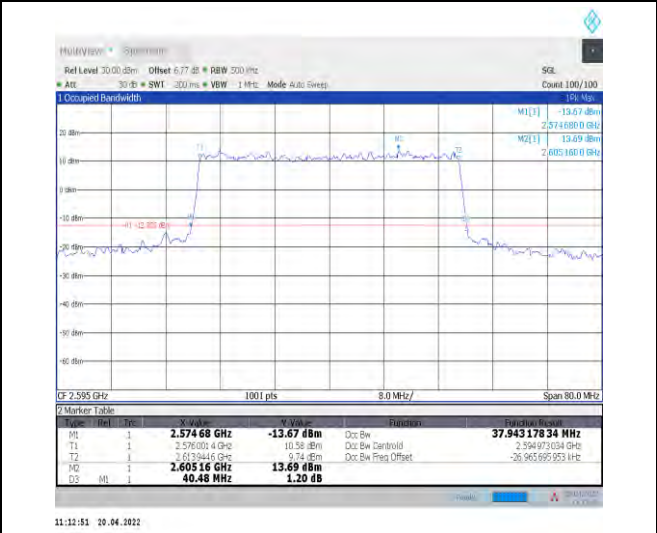
1-N38--30-40-M-7-CP-16QAM-Outer_Full-106@0-A nt1-37.943-40.480-≤40-PASS
