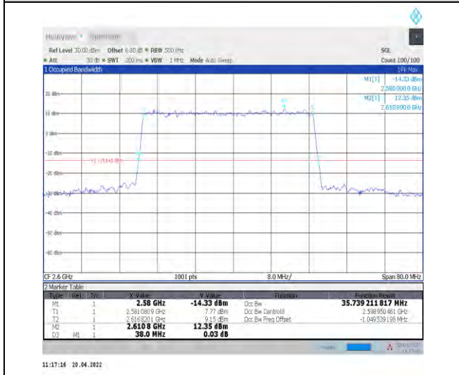
1-N38--30-40-H-5-DFT-256QAM-Outer_Full-100@0-A Ant1-35.739-38.000-≤40-PASS
