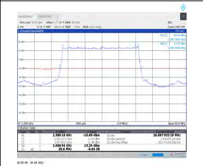
1-N38--30-30-M-2-DFT-PI2BPSK-Outer_Full-75@0-Ant1 1-26.898-28.800-≤30-PASS
