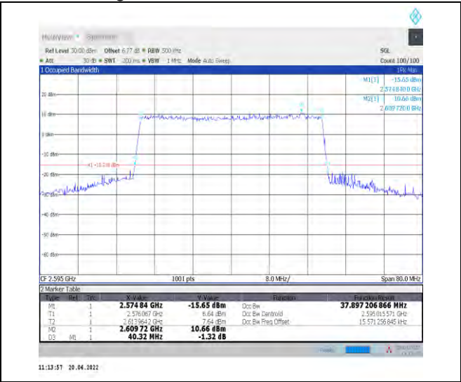
1-N38--30-40-M-9-CP-256QAM-Outer_Full-106@0-Ant1-37.897-40.320-<math>\leq 40</math>-PASS
