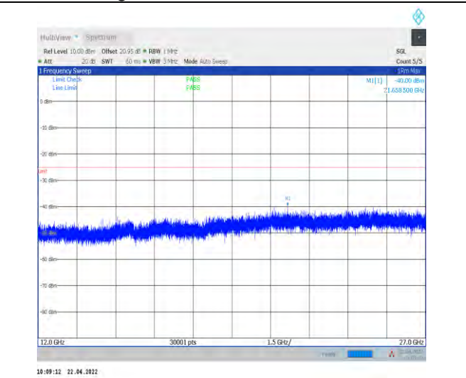
1-N38--30-40-H-1-DFT-PI2BPSK-Inner_1RB_Left-1 @1-12000-27000-Ant1--40.00--25-PASS
