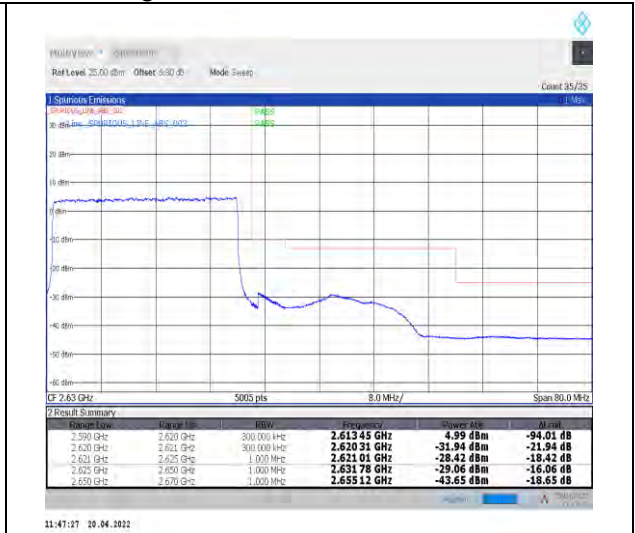
1-N38--30-30-H-3-DFT-PI2BPSK-Outer_Full-75@0-Ant1-PASS-see graph
