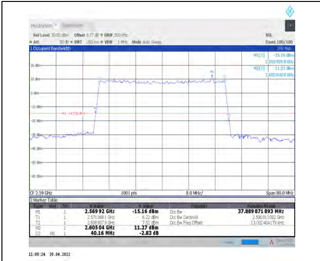
1-N38--30-40-L-9-CP-256QAM-Outer_Full-106@0-A nt1-37.89-40.160-<40-PASS
