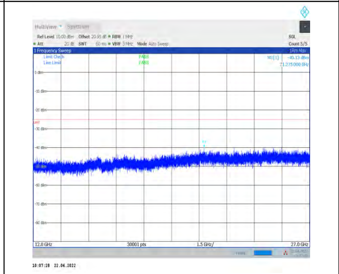
1-N38--30-40-M-1-DFT-PI2BPSK-Inner_1RB_Left-1 @1-12000-27000-Ant1--40.13--25-PASS
