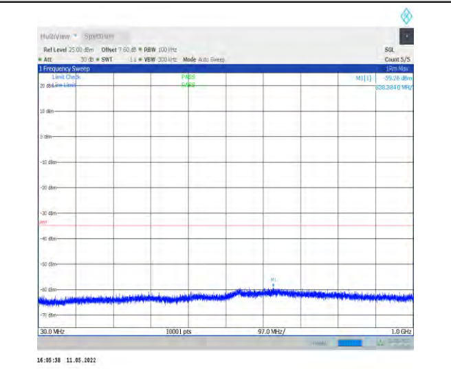
1-N38-PC2-30-40-H-1-DFT-QPSK-Edge_1RB_Left-1 @0-30-1000-Ant1--59.26--35-PASS
