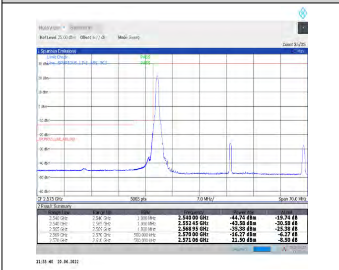
1-N38--30-40-L-4-CP-QPSK-Edge_1RB_Left-1@0-Ant1-PASS-see graph
