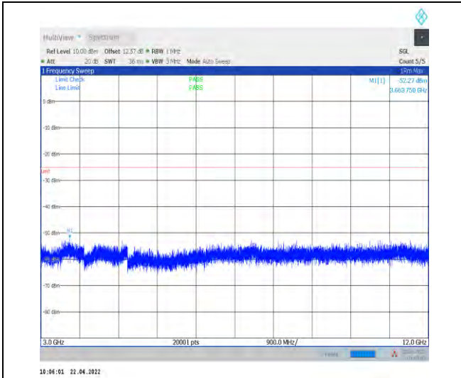
1-N38--30-40-L-1-DFT-PI2BPSK-Inner_1RB_Left-1 @1-3000-12000-Ant1--52.27--25-PASS
