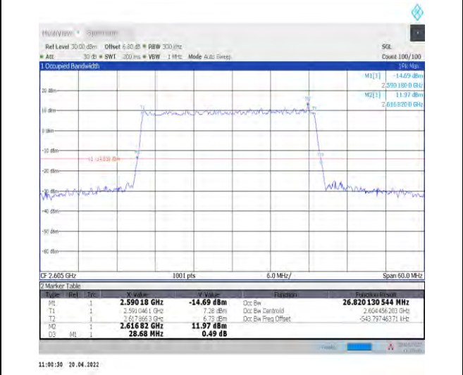
1-N38--30-30-H-5-DFT-256QAM-Outer_Full-75@0-A nt1-26.82-28.680-<=30-PASS
