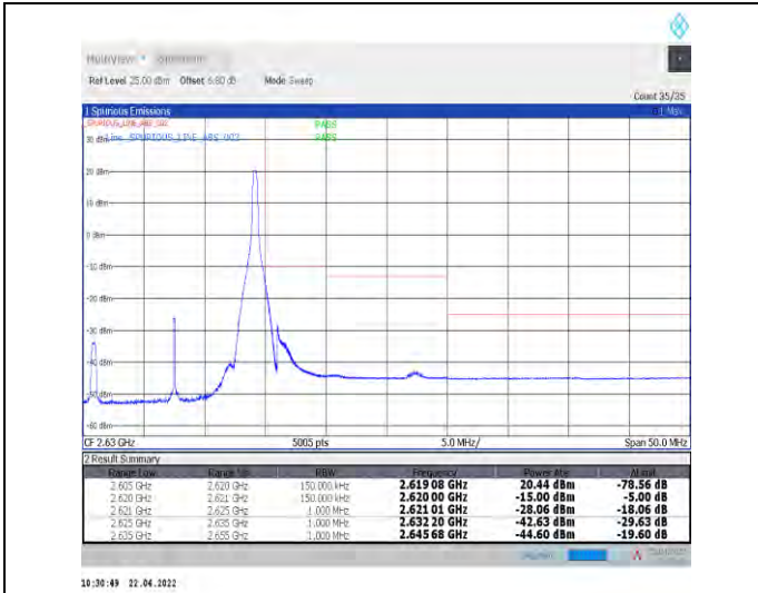
1-N38--30-15-H-2-DFT-PI2BPSK-Edge_1RB_Right-1@37-Ant1-PASS-see graph
