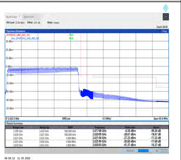
1-N38-PC2-30-30-H-6-CP-QPSK-Outer_Full-78@0-Ant1-PASS-see graph
