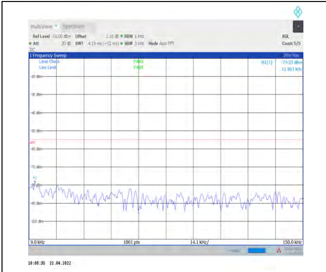
1-N38--30-40-H-1-DFT-PI2BPSK-Inner_1RB_Left-1 @1-0.009-0.15-Ant1--79.23--55-PASS
