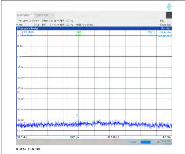
1-N38--30-40-H-1-DFT-PI2BPSK-Inner_1RB_Left-1 @1-30-1000-Ant1--58.44--35-PASS
