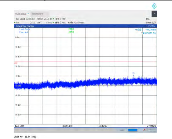
1-N38--30-40-L-1-DFT-PI2BPSK-Inner_1RB_Left-1@ 1-12000-27000-Ant1--40.23--25-PASS
