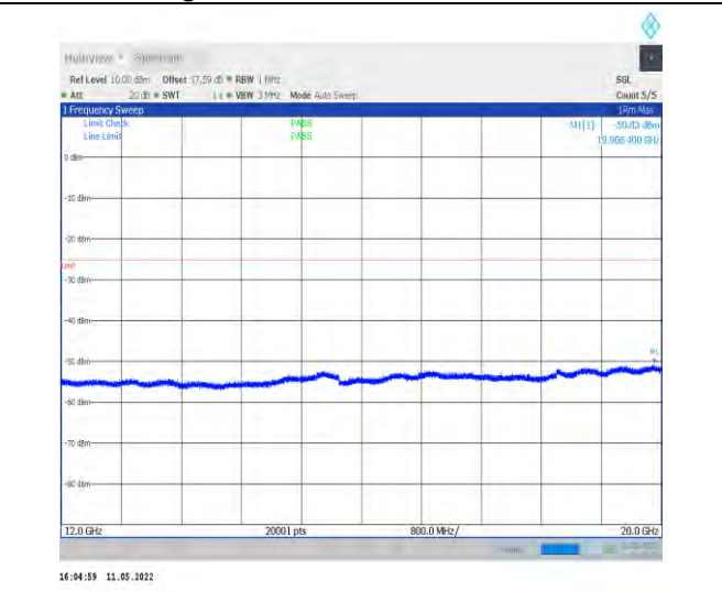
1-N38-PC2-30-40-M-1-DFT-QPSK-Edge_1RB_Left-1 @0-12000-20000-Ant1--50.83--25-PASS
