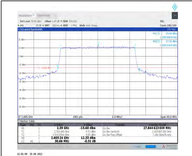
1-N38--30-30-H-6-CP-QPSK-Outer_Full-78@0-Ant1-27.845-30.660-<=30-PASS
