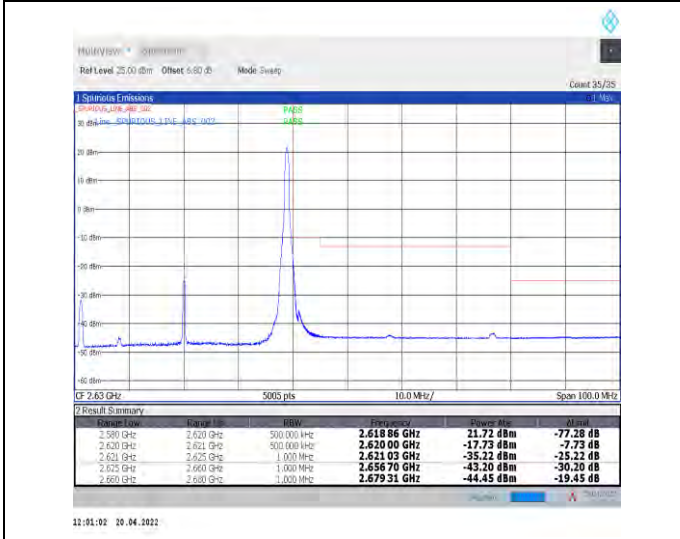
1-N38--30-40-H-5-CP-QPSK-Edge_1RB_Right-1@105-Ant1-PASS-see graph
