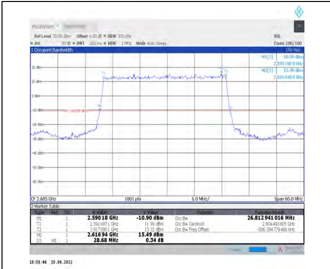
1-N38--30-30-H-2-DFT-PI2BPSK-Outer_Full-75@0-Ant1-26.813-28.680-<=30-PASS
