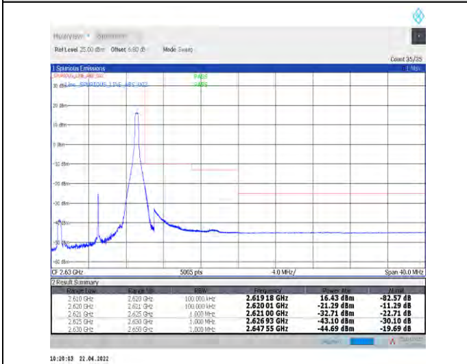
1-N38--30-10-H-5-CP-QPSK-Edge_1RB_Right-1@23-Ant1-PASS-see graph
