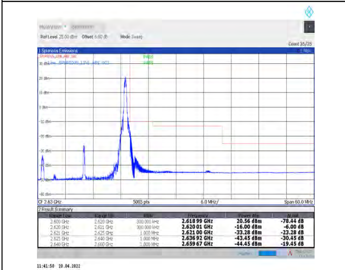
1-N38--30-20-H-5-CP-QPSK-Edge_1RB_Right-1@50-Ant1-PASS-see graph
