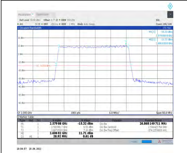
1-N38--30-30-M-5-DFT-256QAM-Outer_Full-75@0-Ant1-26.868-28.920-≤30-PASS
