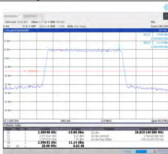
1-N38--30-30-L-5-DFT-256QAM-Outer_Full-75@0-Ant 1-26.819-28.980-≤30-PASS
