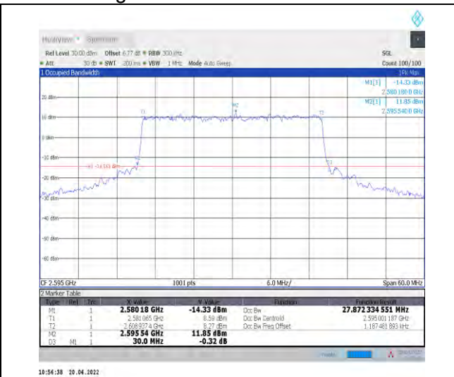
1-N38--30-30-M-8-CP-64QAM-Outer_Full-78@0-Ant 1-27.872-30.000-≤30-PASS
