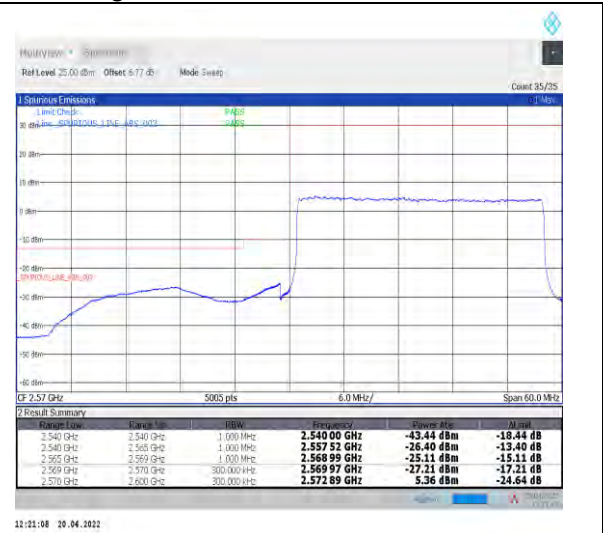
1-N38--30-30-L-3-DFT-PI2BPSK-Outer_Full-75@0-Ant1-PASS-see graph
