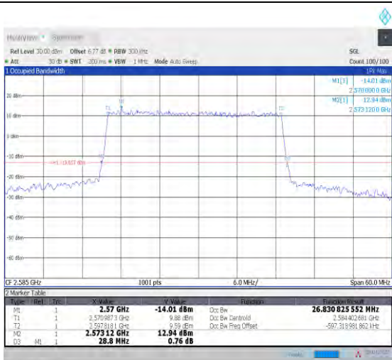
1-N38--30-30-L-4-DFT-64QAM-Outer_Full-75@0-Ant 1-26.831-28.800-≤30-PASS
