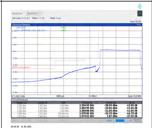
1-N38--30-15-L-6-CP-QPSK-Outer_Full-38@0-Ant1-PASS-see graph
