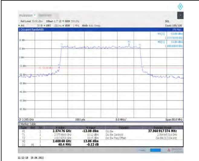
1-N38--30-40-M-6-CP-QPSK-Outer_Full-106@0-Ant 1-37.961-40.400-≤40-PASS
