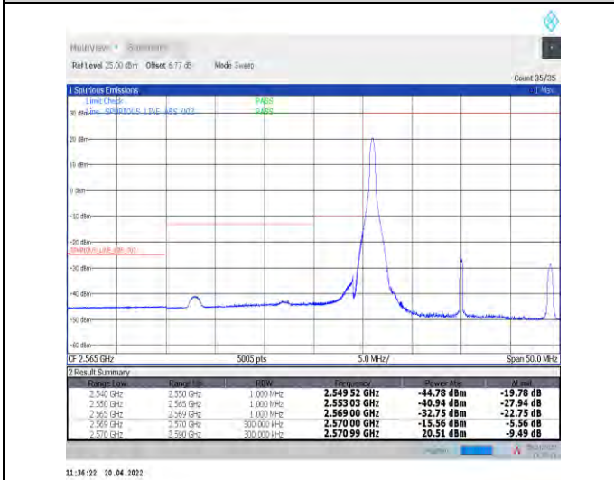
1-N38--30-20-L-4-CP-QPSK-Edge_1RB_Left-1@0-Ant1-PASS-see graph
