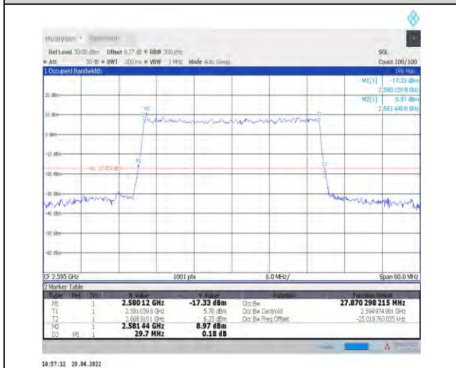
1-N38--30-30-M-9-CP-256QAM-Outer_Full-78@0-Ant t1-27.87-29.700-≤30-PASS
