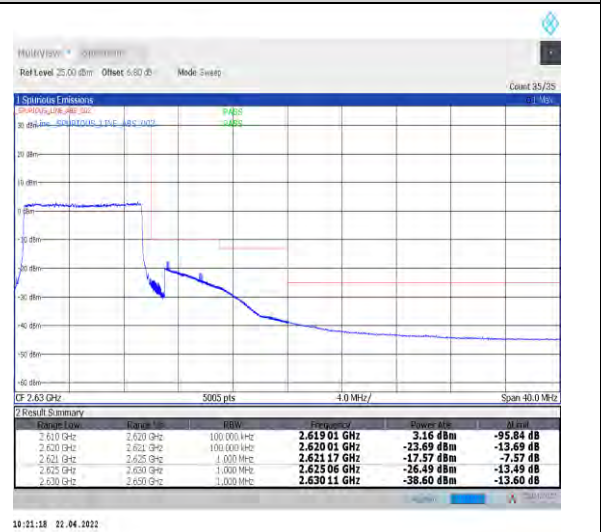
1-N38--30-10-H-6-CP-QPSK-Outer_Full-24@0-Ant1-PASS-see graph
