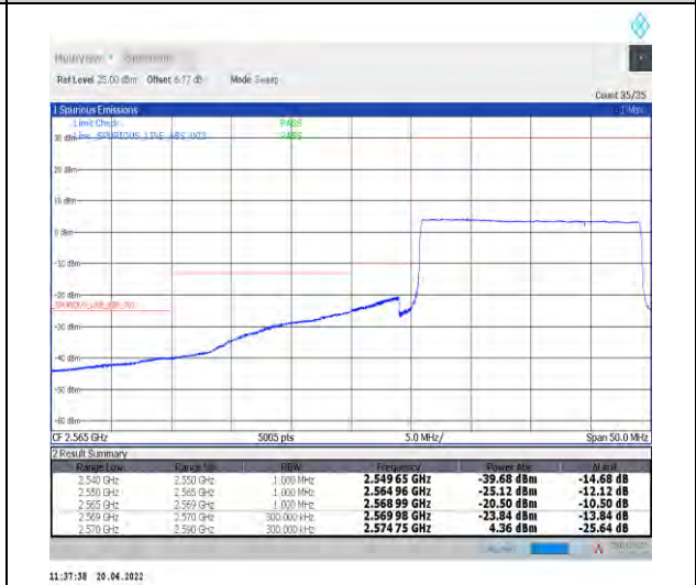
1-N38--30-20-L-6-CP-QPSK-Outer_Full-51@0-Ant1-PASS-see graph
