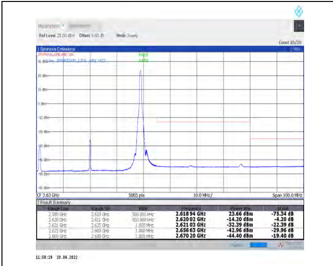
1-N38--30-40-H-2-DFT-PI2BPSK-Edge_1RB_Right-1@105-Ant1-PASS-see graph
