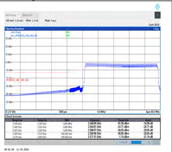
1-N38-PC2-30-30-L-6-CP-QPSK-Outer_Full-78@0-Ant1-PASS-see graph
