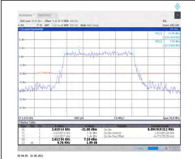
1-N38--30-10-H-9-CP-256QAM-Outer_Full-24@0-Ant t1-8.595-9.760-≤10-PASS
