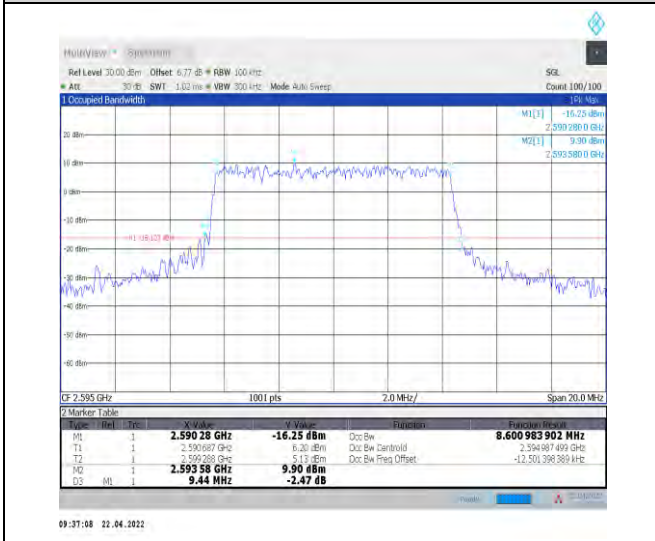
1-N38--30-10-M-6-CP-QPSK-Outer_Full-24@0-Ant1-8.601-9.440-≤10-PASS
