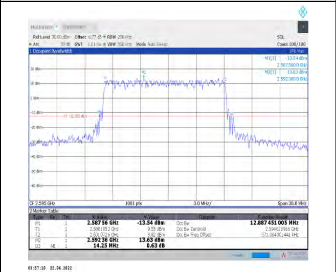
1-N38--30-15-M-4-DFT-64QAM-Outer_Full-36@0-Ant t1-12.887-14.250-≤15-PASS
