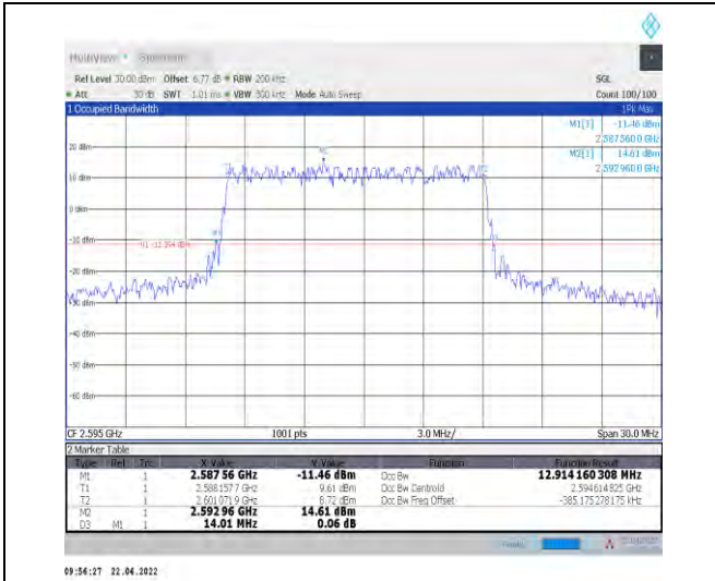
1-N38--30-15-M-1-DFT-QPSK-Outer_Full-36@0-Ant 1-12.914-14.010-≤15-PASS
