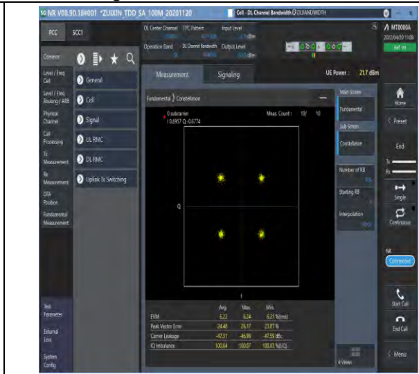
1-N38--30-40-M-6-CP-QPSK-Outer_Full-106@0-Ant1-see graph-PASS
