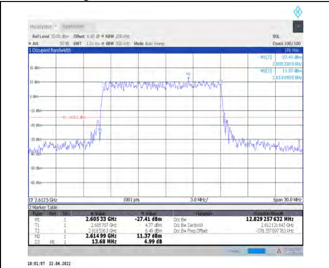
1-N38--30-15-H-5-DFT-256QAM-Outer_Full-36@0-Ant nt1-12.829-13.680-≤15-PASS
