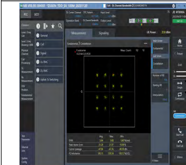
1-N38--30-40-M-7-CP-16QAM-Outer_Full-106@0-Ant1-see graph-PASS
