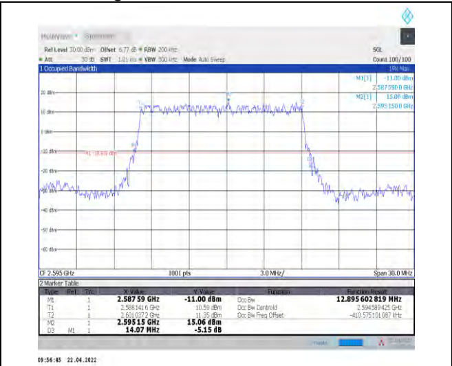
1-N38--30-15-M-2-DFT-PI2BPSK-Outer_Full-36@0-Ant 1-12.896-14.070-≤15-PASS
