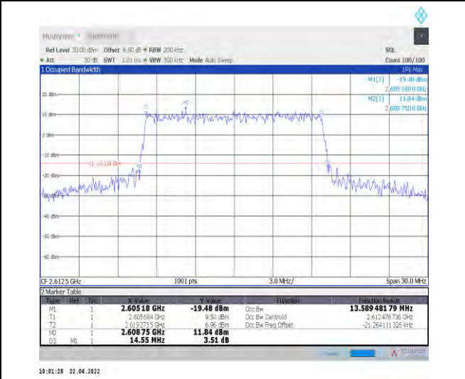
1-N38--30-15-H-7-CP-16QAM-Outer_Full-38@0-Ant 1-13.589-14.550-≤15-PASS
