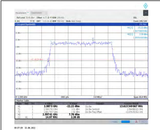
1-N38--30-15-M-9-CP-256QAM-Outer_Full-38@0-An t1-13.615-14.970-<=15-PASS
