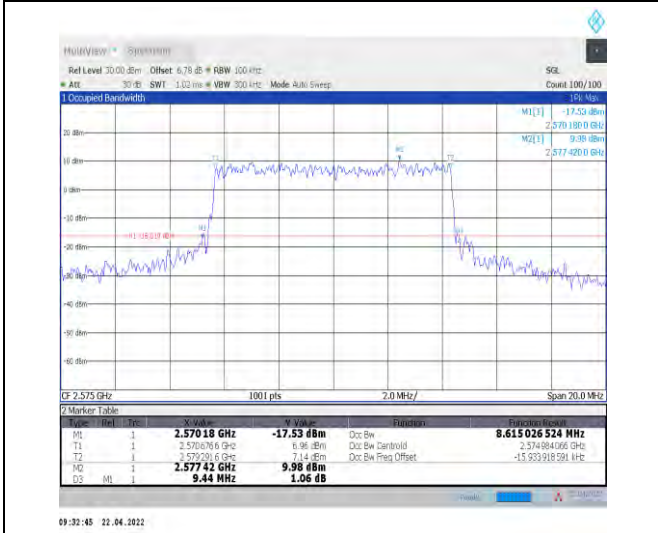
1-N38--30-10-L-7-CP-16QAM-Outer_Full-24@0-Ant1 -8.615-9.440-<=10-PASS
