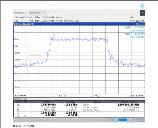
1-N38--30-10-M-1-DFT-QPSK-Outer_Full-24@0-Ant 1-8.595-9.860-≤10-PASS
