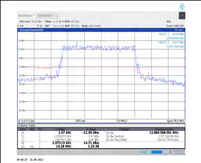
1-N38--30-15-L-1-DFT-QPSK-Outer_Full-36@0-Ant1 -12.885-14.280-≤15-PASS
