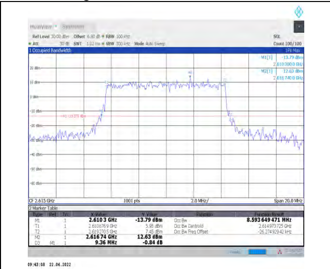
1-N38--30-10-H-4-DFT-64QAM-Outer_Full-24@0-An t1-8.594-9.360-≤10-PASS
