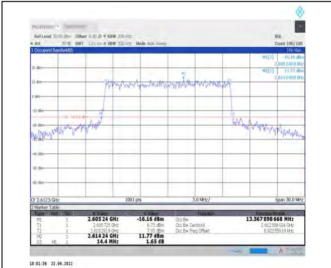
1-N38--30-15-H-8-CP-64QAM-Outer_Full-38@0-Ant 1-13.568-14.400-≤15-PASS
