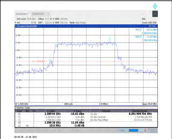
1-N38--30-10-M-3-DFT-16QAM-Outer_Full-24@0-Ant nt1-8.592-10.000-≤10-PASS
