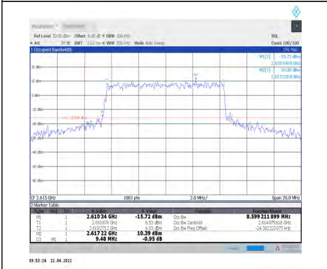
1-N38--30-10-H-1-DFT-QPSK-Outer_Full-24@0-Ant 1-8.599-9.480-≤10-PASS
