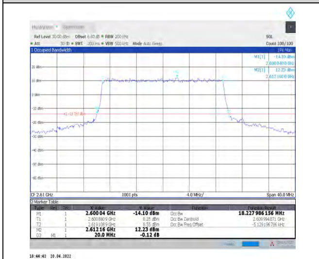
1-N38--30-20-H-7-CP-16QAM-Outer_Full-51@0-Ant 1-18.228-20.000-≤20-PASS
