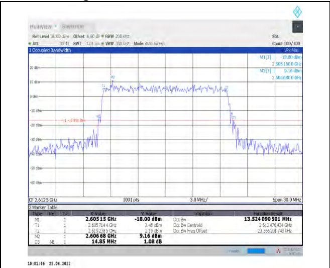
1-N38--30-15-H-9-CP-256QAM-Outer_Full-38@0-An t1-13.524-14.850-≤15-PASS
