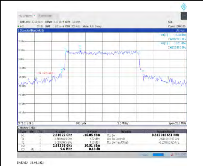
1-N38--30-10-H-6-CP-QPSK-Outer_Full-24@0-Ant1- 8.615-9.600-≤10-PASS
