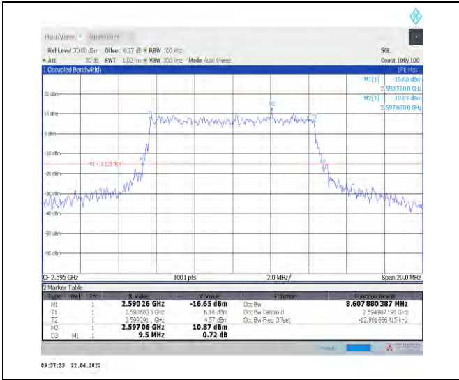
1-N38--30-10-M-8-CP-64QAM-Outer_Full-24@0-Ant 1-8.608-9.500-≤10-PASS
