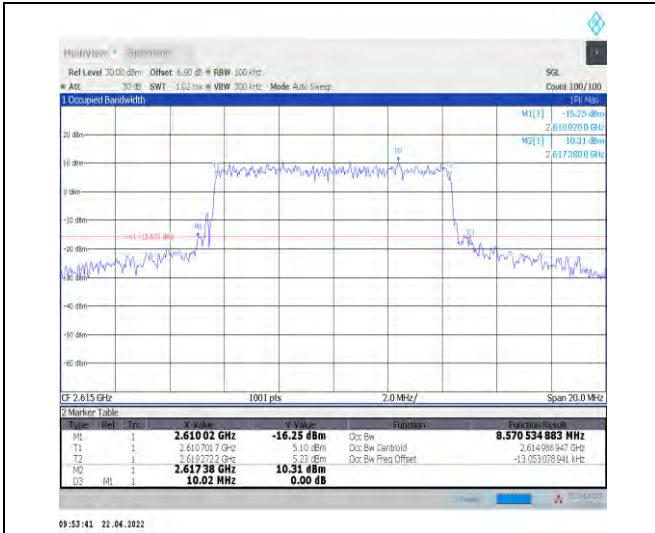
1-N38--30-10-H-7-CP-16QAM-Outer_Full-24@0-Ant 1-8.571-10.020-≤10-PASS
