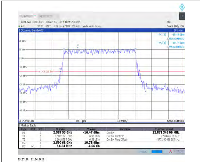
1-N38--30-15-M-5-DFT-256QAM-Outer_Full-36@0-A nt1-12.871-14.340-≤15-PASS
