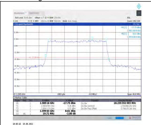
1-N38--30-20-M-7-CP-16QAM-Outer_Full-51@0-Ant-18.206-19.960-≤20-PASS
