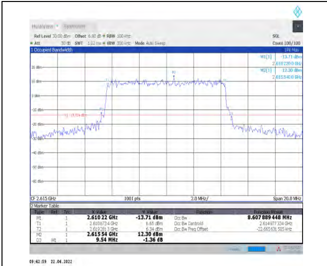
1-N38--30-10-H-3-DFT-16QAM-Outer_Full-24@0-An t1-8.608-9.540-≤10-PASS
