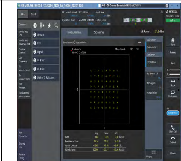
1-N38--30-40-M-8-CP-64QAM-Outer_Full-106@0-Ant1-see graph-PASS
