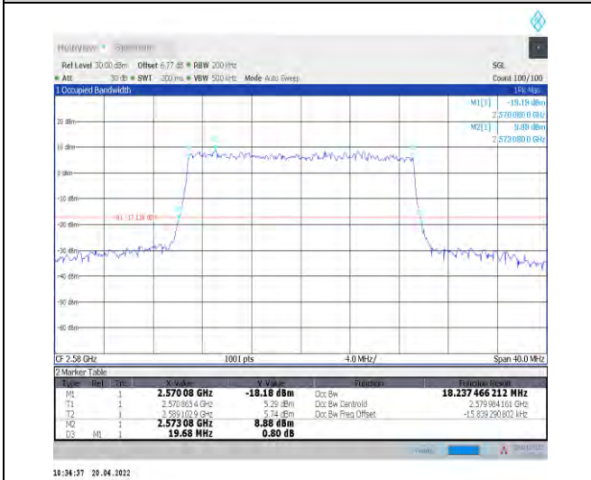
1-N38--30-20-L-9-CP-256QAM-Outer_Full-51@0-Ant 1-18.237-19.680-≤20-PASS
