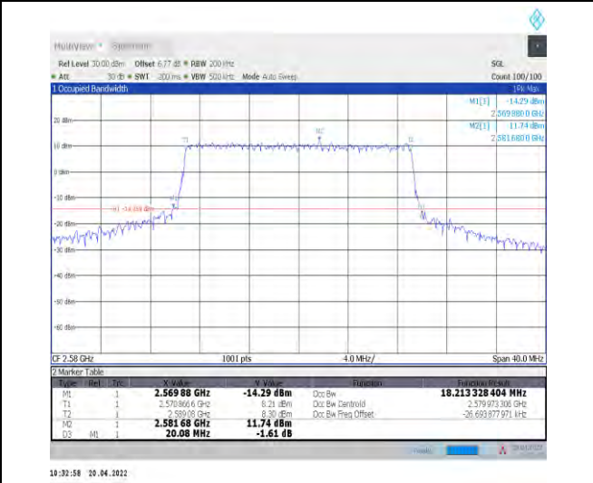
1-N38--30-20-L-6-CP-QPSK-Outer_Full-51@0-Ant1 18.213-20.080-≤20-PASS
