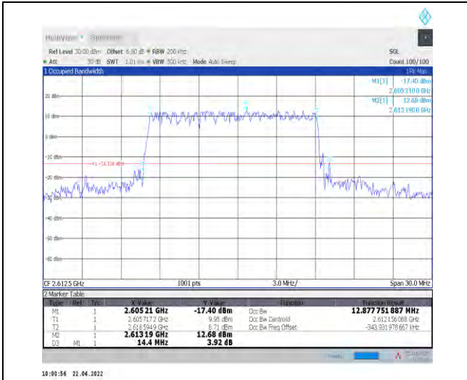
1-N38--30-15-H-4-DFT-64QAM-Outer_Full-36@0-Ant t1-12.878-14.400-≤15-PASS
