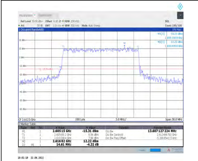
1-N38--30-15-H-6-CP-QPSK-Outer_Full-38@0-Ant1 13.607-14.610-≤15-PASS
