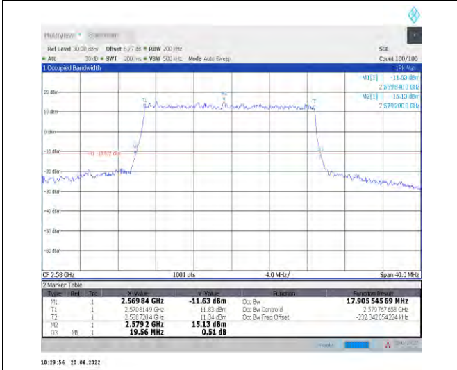
1-N38--30-20-L-1-DFT-QPSK-Outer_Full-50@0-Ant1 -17.906-19.560-≤20-PASS
