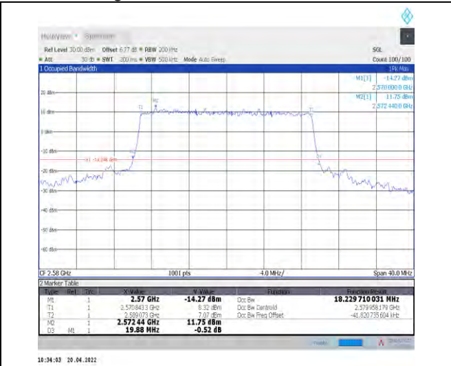
1-N38--30-20-L-8-CP-64QAM-Outer_Full-51@0-Ant 1-18.23-19.880-≤20-PASS
