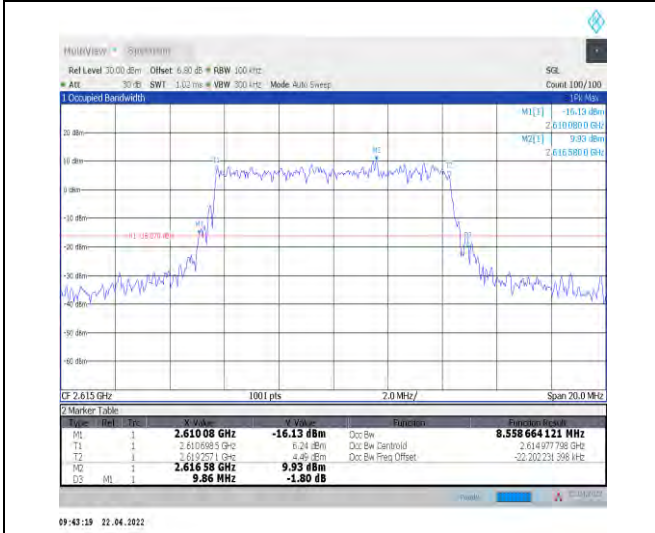
1-N38--30-10-H-5-DFT-256QAM-Outer_Full-24@0-A nt1-8.559-9.860-≤10-PASS
