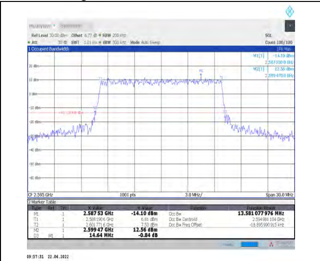
1-N38--30-15-M-6-CP-QPSK-Outer_Full-38@0-Ant1 -13.581-14.640-≤15-PASS
