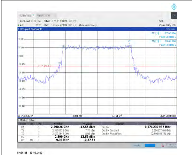
1-N38--30-10-M-2-DFT-PI2BPSK-Outer_Full-24@0-Ant Ant1-8.574-9.360-≤10-PASS
