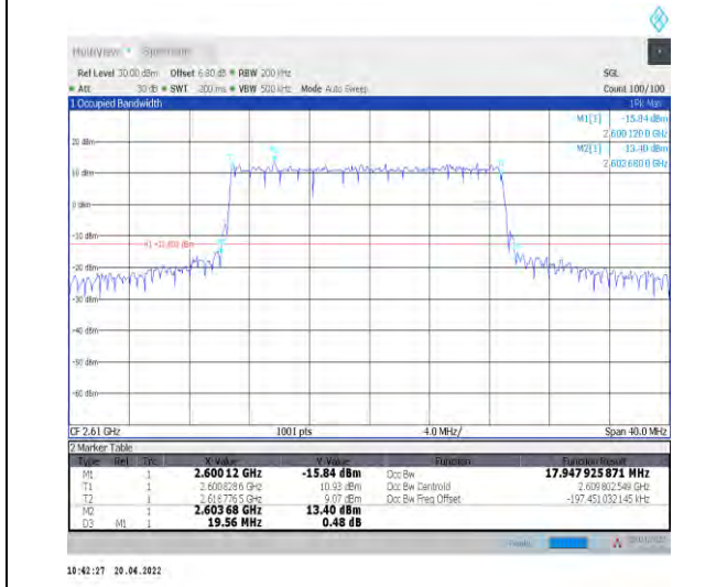
1-N38--30-20-H-3-DFT-16QAM-Outer_Full-50@0-An t1-17.948-19.560-≤20-PASS
