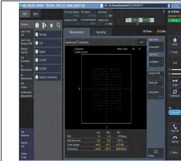
1-N38--30-40-M-5-DFT-256QAM-Outer_Full-100@0-Ant1-see graph-PASS
