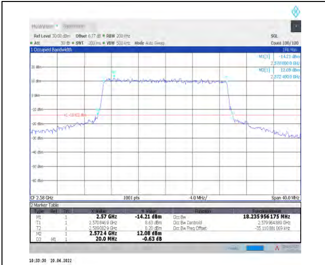
1-N38--30-20-L-7-CP-16QAM-Outer_Full-51@0-Ant1 -18.236-20.000-≤20-PASS
