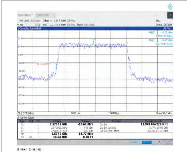
1-N38--30-15-L-2-DFT-PI2BPSK-Outer_Full-36@0-A nt1-12.949-14.040-≤15-PASS
