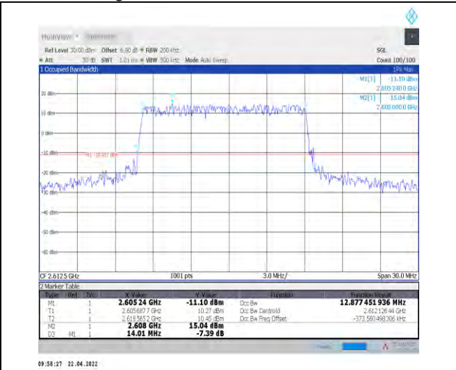
1-N38--30-15-H-1-DFT-QPSK-Outer_Full-36@0-Ant 1-12.877-14.010-<=15-PASS
