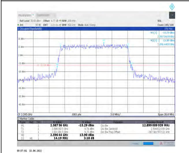
1-N38--30-15-M-3-DFT-16QAM-Outer_Full-36@0-Ant t1-12.899-14.190-≤15-PASS
