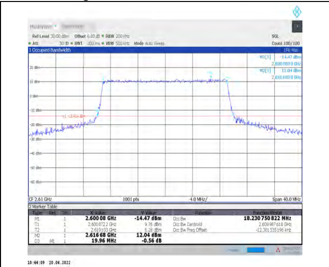
1-N38--30-20-H-6-CP-QPSK-Outer_Full-51@0-Ant1- 18.231-19.960-≤20-PASS
