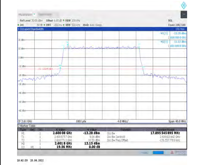
1-N38--30-20-H-4-DFT-64QAM-Outer_Full-50@0-An t1-17.896-19.560-≤20-PASS
