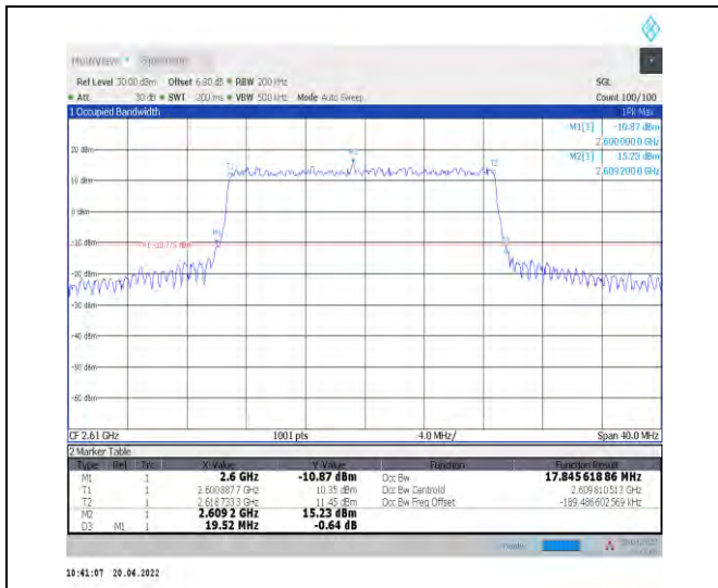
1-N38--30-20-H-1-DFT-QPSK-Outer_Full-50@0-Ant 1-17.846-19.520-≤20-PASS
