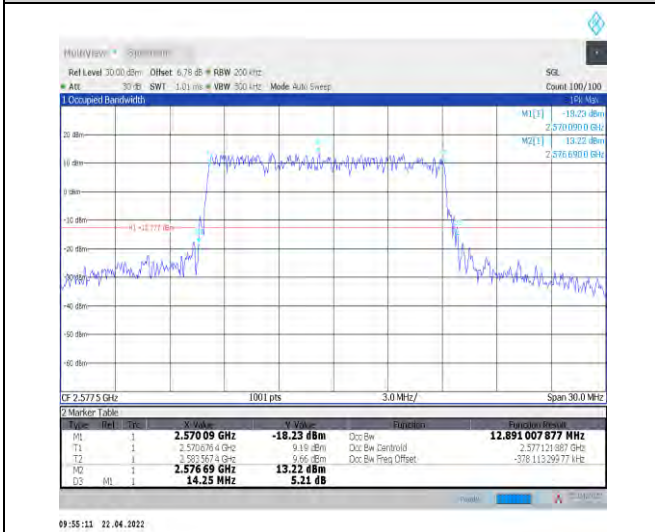
1-N38--30-15-L-4-DFT-64QAM-Outer_Full-36@0-Ant 1-12.891-14.250-≤15-PASS
