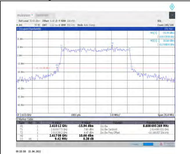
1-N38--30-10-H-8-CP-64QAM-Outer_Full-24@0-Ant 1-8.609-9.420-≤10-PASS
