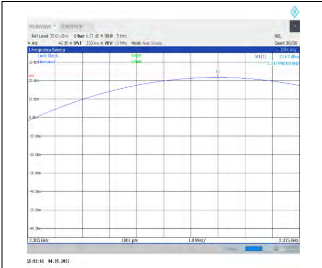
1-N30-PC3-15-5-M-2-DFT-PI2BPSK-Inner_1RB_Ri ght-1@23-2305-2315-Ant1-21.67-23.98-PASS
