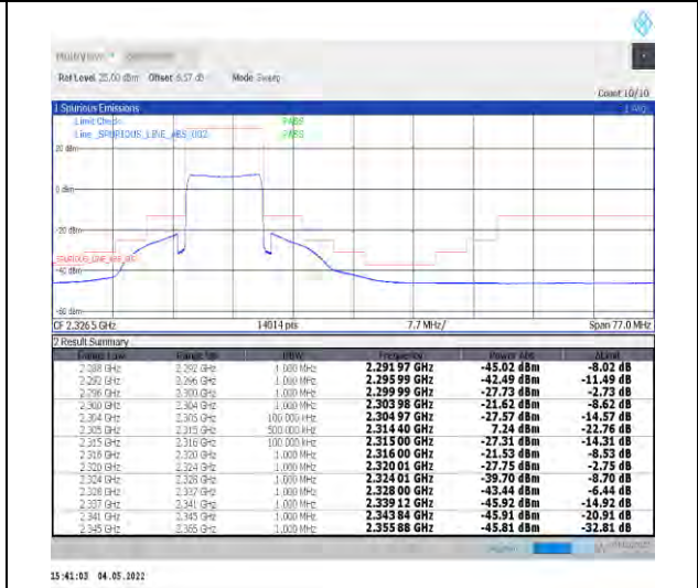
1-N30--15-10-H-6-CP-QPSK-Outer_Full-52@0-Ant1-PASS-see graph
