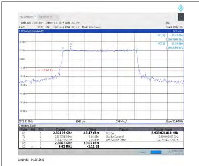
1-N30--15-10-M-1-DFT-QPSK-Outer_Full-50@0-Ant 1-8.933-9.620-≤10-PASS
