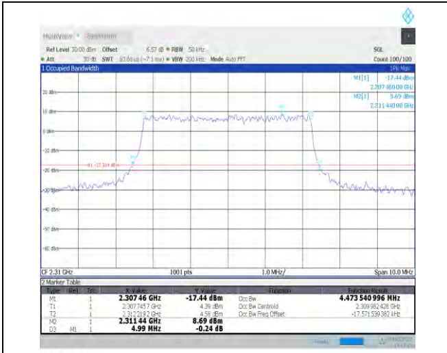
1-N30--15-5-M-8-CP-64QAM-Outer_Full-25@0-Ant1 -4.474-4.990-≤5-PASS
