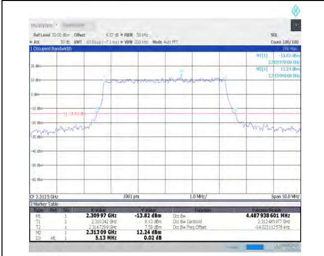
1-N30--15-5-H-1-DFT-QPSK-Outer_Full-25@0-Ant1- 4.488-5.130-≤5-PASS
