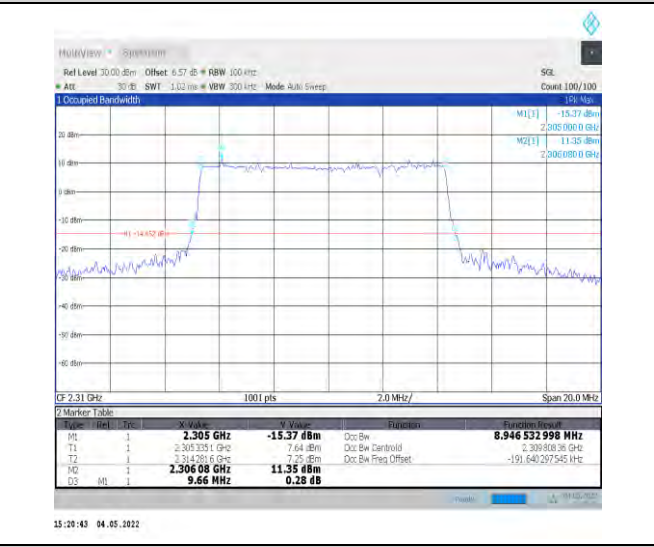
1-N30--15-10-M-4-DFT-64QAM-Outer_Full-50@0-Ant1-8.947-9.660-≤10-PASS
