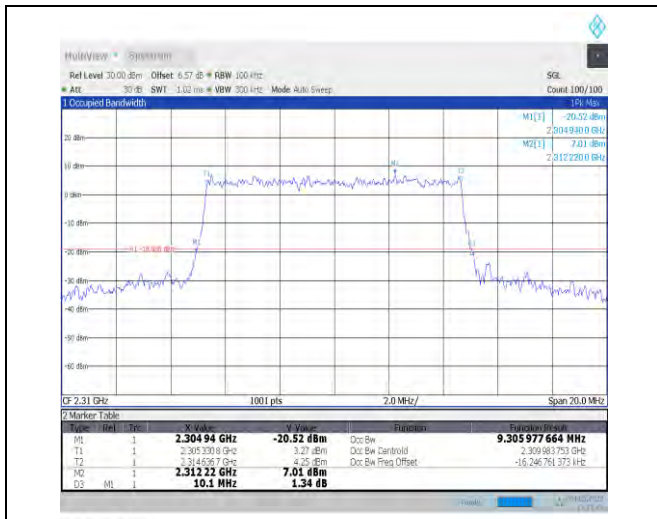
1-N30--15-10-M-9-CP-256QAM-Outer_Full-52@0-A nt1-9.306-10.100-≤10-PASS
