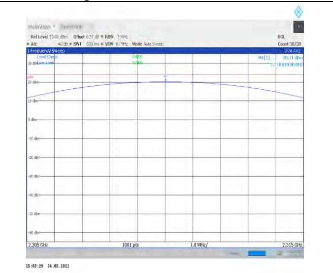
1-N30-PC3-15-5-M-3-DFT-PI2BPSK-Outer_Full-25@ 0-2305-2315-Ant1-20.11-23.98-PASS
