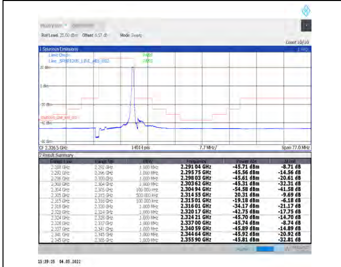
1-N30--15-10-H-5-CP-QPSK-Edge_1RB_Right-1@51-Ant1-PASS-see graph
