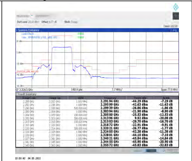
1-N30--15-10-L-3-DFT-PI2BPSK-Outer_Full-50@0-Ant1-PASS-see graph
