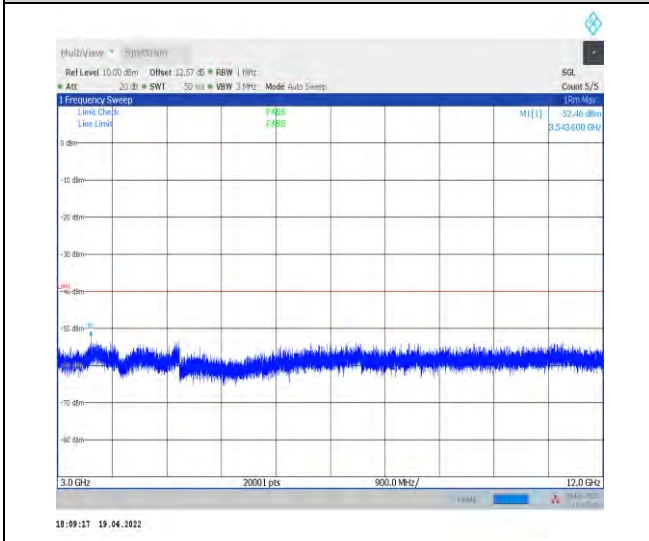
1-N30--15-10-M-1-DFT-PI2BPSK-Inner_1RB_Left-1 @1-3000-12000-Ant1--52.46--40-PASS
