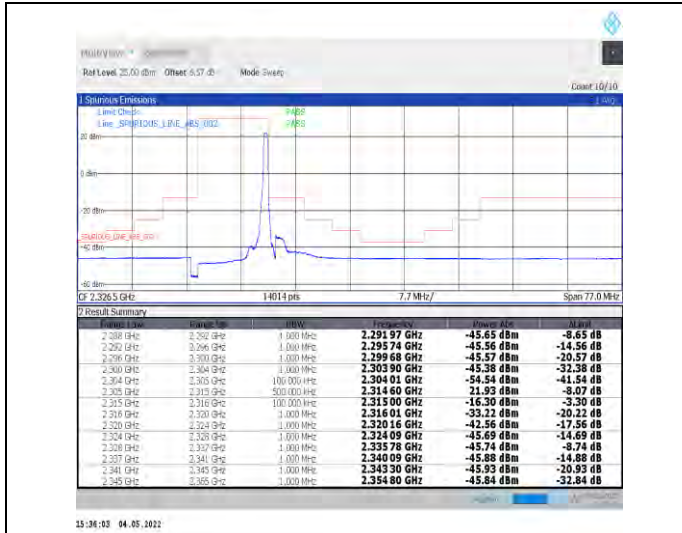
1-N30--15-10-H-2-DFT-PI2BPSK-Edge_1RB_Right-1@51-Ant1-PASS-see graph
