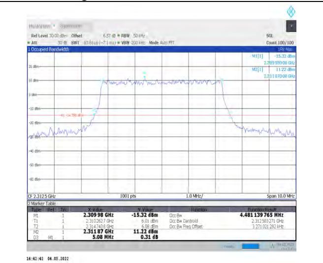
1-N30--15-5-H-4-DFT-64QAM-Outer_Full-25@0-Ant 1-4.481-5.080-≤5-PASS
