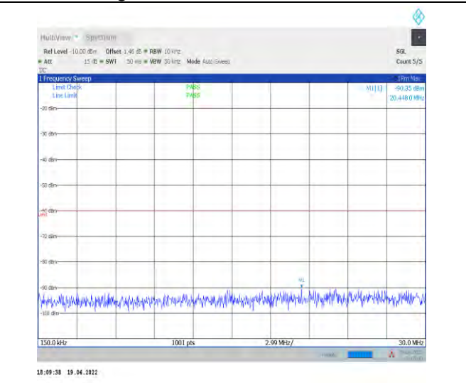
1-N30--15-10-H-1-DFT-PI2BPSK-Inner_1RB_Left-1 @1-0.15-30-Ant1--90.35--60-PASS
