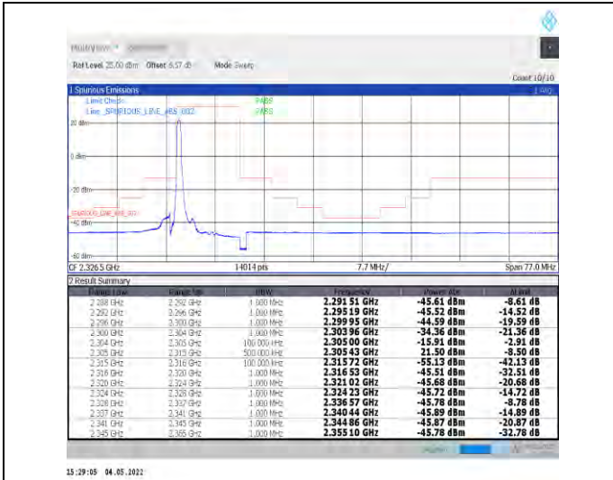
1-N30--15-10-L-1-DFT-PI2BPSK-Edge_1RB_Left-1@0-Ant1-PASS-see graph
