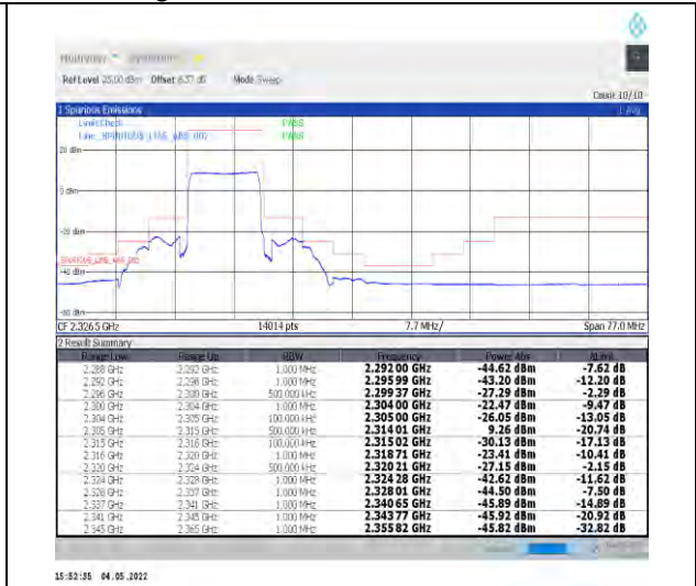
1-N30--15-10-H-3-DFT-PI2BPSK-Outer_Full-50@0-Ant1-PASS-see graph
