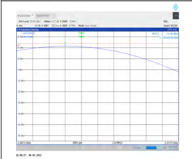
1-N30-PC3-15-5-H-1-DFT-PI2BPSK-Inner_1RB_Lef t-1@1-2307.5-2317.5-Ant1-21.50-23.98-PASS
