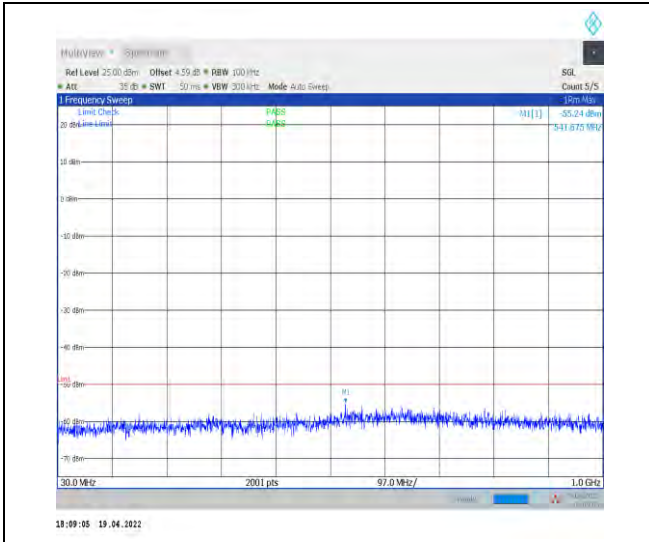
1-N30--15-10-M-1-DFT-PI2BPSK-Inner_1RB_Left-1 @1-30-1000-Ant1--55.24--50-PASS
