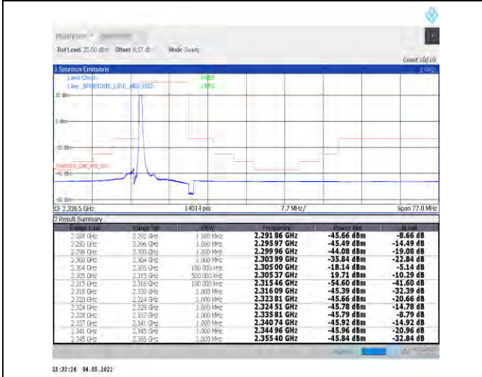
1-N30--15-10-L-4-CP-QPSK-Edge_1RB_Left-1@0-Ant1-PASS-see graph
