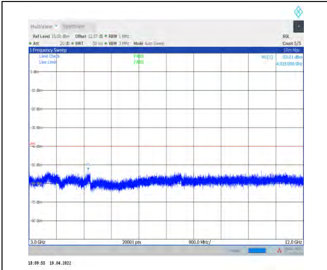
1-N30--15-10-H-1-DFT-PI2BPSK-Inner_1RB_Left-1 @1-3000-12000-Ant1--53.01--40-PASS
