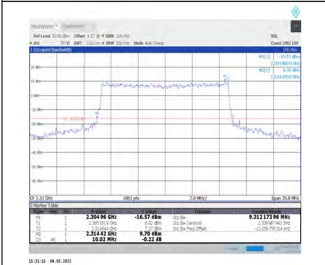
1-N30--15-10-M-7-CP-16QAM-Outer_Full-52@0-Ant1-9.312-10.020-≤10-PASS
