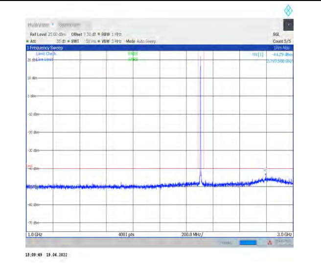
1-N30--15-10-H-1-DFT-PI2BPSK-Inner_1RB_Left-1 @1-1000-3000-Ant1--44.29--40-PASS
