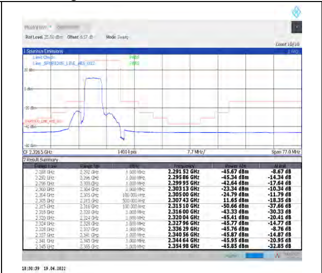
1-N30--30-10-L-3-DFT-PI2BPSK-Outer_Full-24@0-Ant1-PASS-see graph
