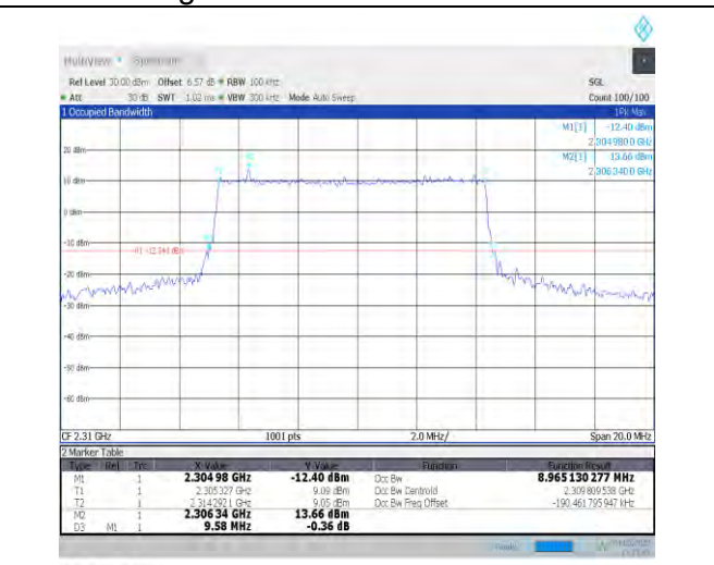
1-N30--15-10-H-1-DFT-QPSK-Outer_Full-50@0-Ant 1-8.965-9.580-≤10-PASS
