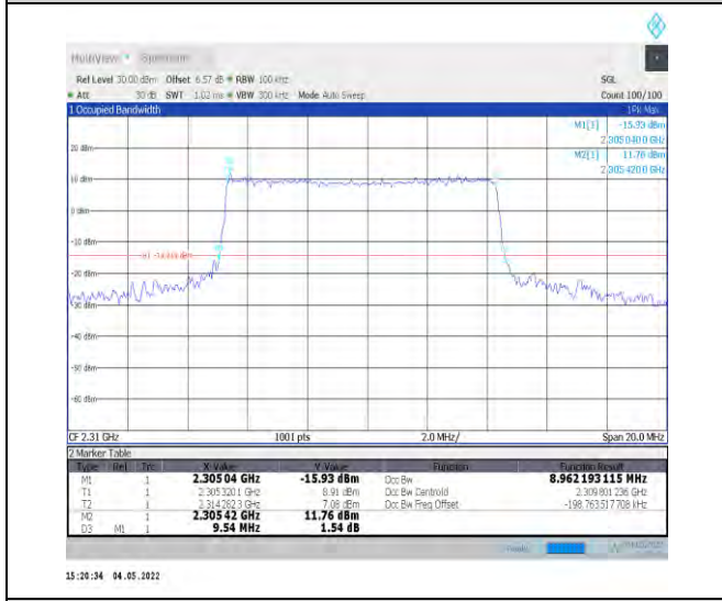
1-N30--15-10-M-3-DFT-16QAM-Outer_Full-50@0-Ant1-8.962-9.540-≤10-PASS
