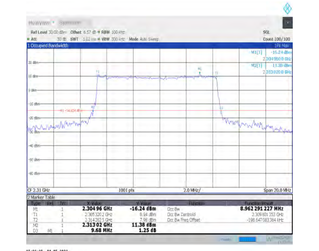
1-N30--15-10-H-3-DFT-16QAM-Outer_Full-50@0-Ant t1-8.962-9.680-≤10-PASS
