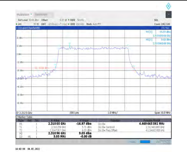
1-N30--15-5-H-6-CP-QPSK-Outer_Full-25@0-Ant1-4 .47-5.050-≤5-PASS
