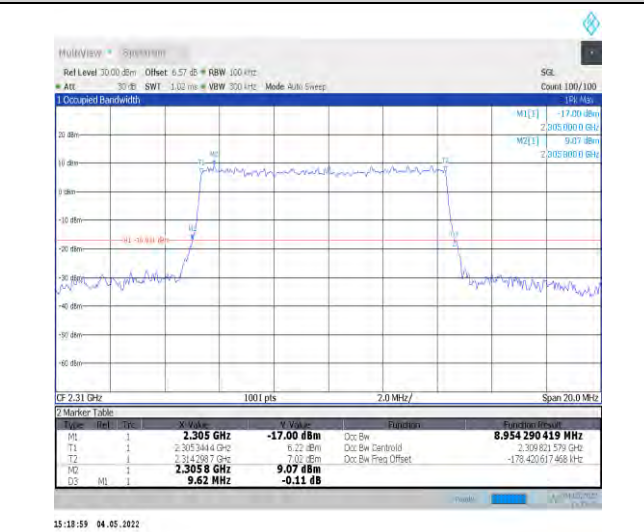
1-N30--15-10-L-5-DFT-256QAM-Outer_Full-50@0-A nt1-8.954-9.620-≤10-PASS
