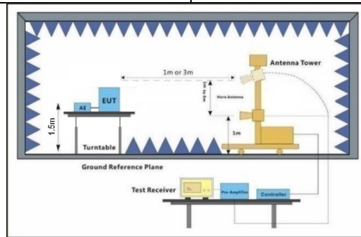
Figure 3. above 1GHz
