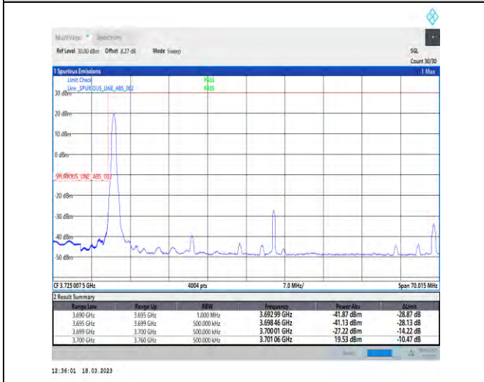
1-N78-3700-3800-30-60-L-4-CP-QPSK-Edge_1RB_Lef t-1@0-Ant1-1--PASS-see graph
