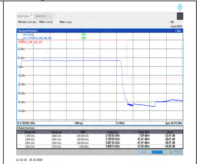
1-N78-3700-3800-30-20-H-3-DFT-PI2BPSK-Outer_Full-50@0-Ant1-1--PASS-see graph
