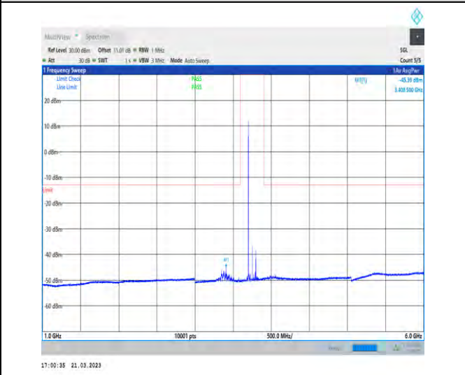
1-N78-3700-3800-30-100-H-1-DFT-QPSK-Edge_1RB _Left-1@0-1000-6000-Ant1-3408.50--45.39--13-PASS
