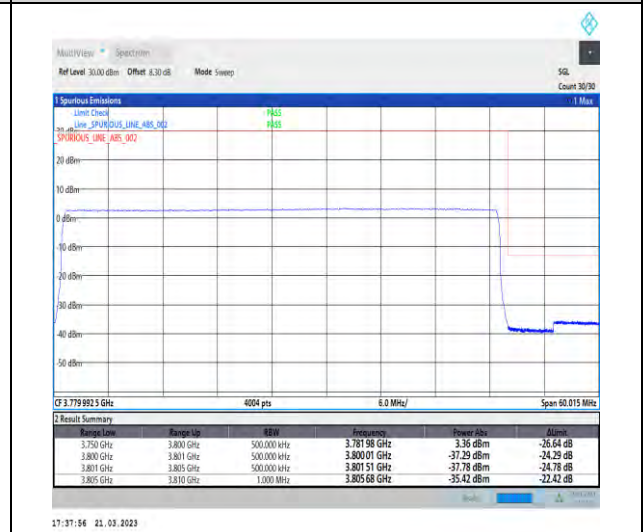
1-N78-3700-3800-30-50-H-6-CP-QPSK-Outer_Full -133@0-Ant1-1--PASS-see graph
