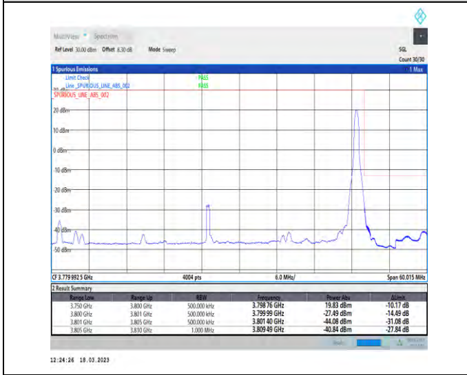
1-N78-3700-3800-30-50-H-5-CP-QPSK-Edge_1RB_Right-1@132-Ant1-1--PASS-see graph
