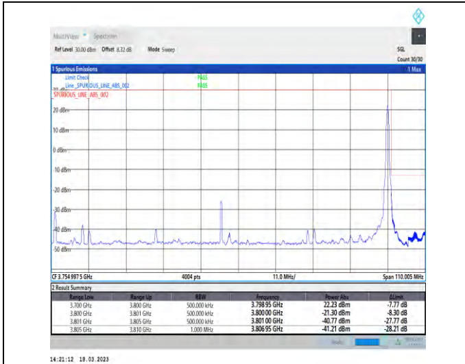
1-N78-3700-3800-30-100-H-2-DFT-PI2BPSK-Edge_1R_B_Right-1@272-Ant1-1--PASS-see graph
