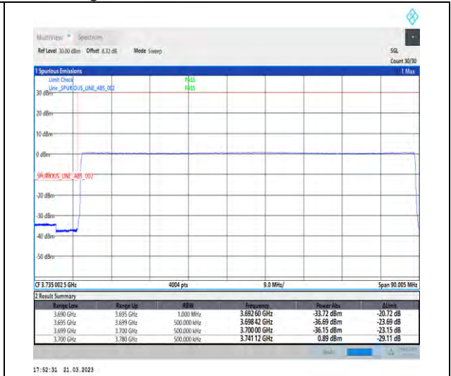
1-N78-3700-3800-30-80-L-6-CP-QPSK-Outer_Full -217@0-Ant1-1--PASS-see graph
