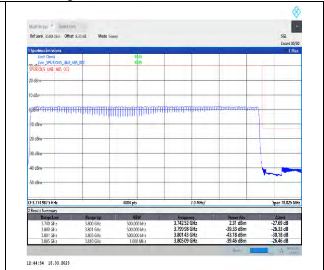
1-N78-3700-3800-30-60-H-3-DFT-PI2BPSK-Outer_Full-162@0-Ant1-1--PASS-see graph
