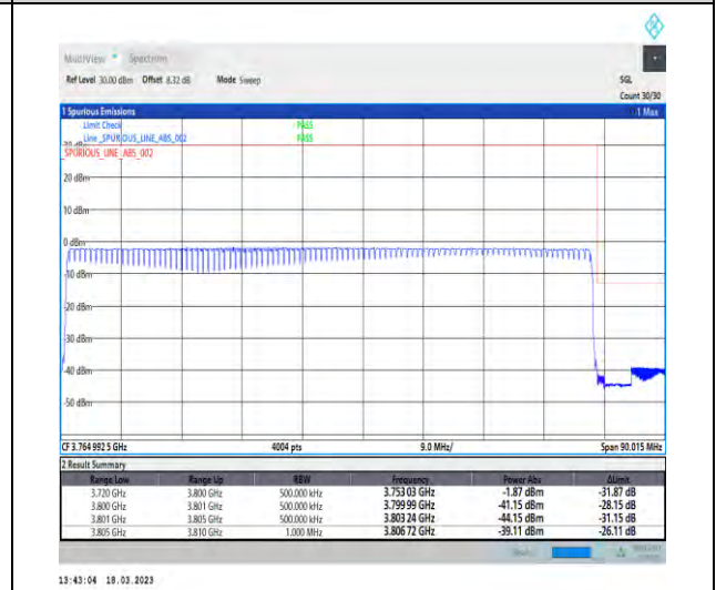
1-N78-3700-3800-30-80-H-6-CP-QPSK-Outer_Full-217@0-Ant1-1--PASS-see graph
