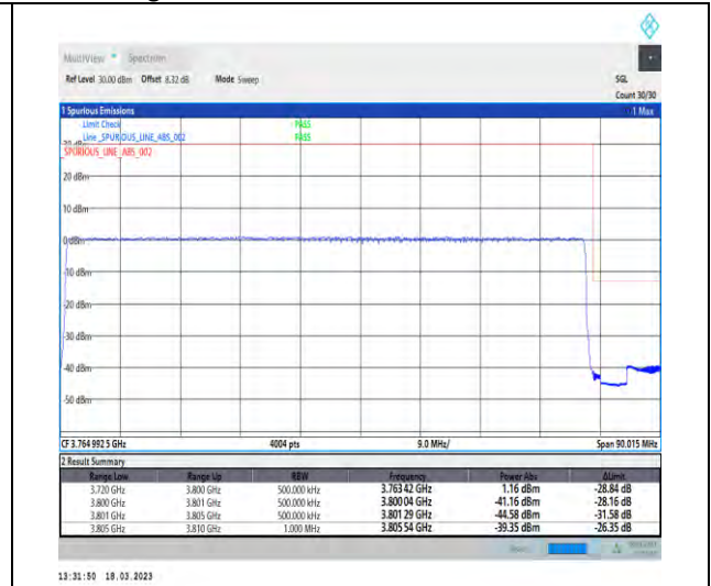
1-N78-3700-3800-30-80-H-3-DFT-PI2BPSK-Outer_Full-216@0-Ant1-1--PASS-see graph
