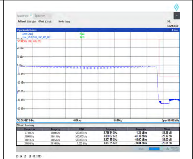
1-N78-3700-3800-30-70-H-6-CP-QPSK-Outer_Full-189@0-Ant1-1--PASS-see graph
