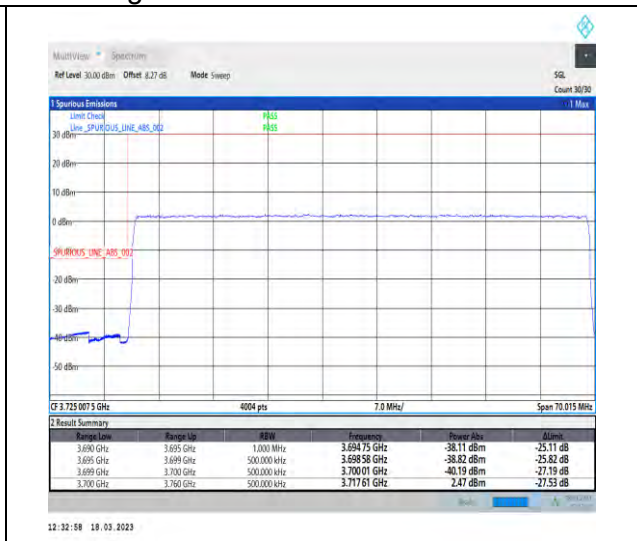
1-N78-3700-3800-30-60-L-3-DFT-PI2BPSK-Outer_Full-162@0-Ant1-1--PASS-see graph
