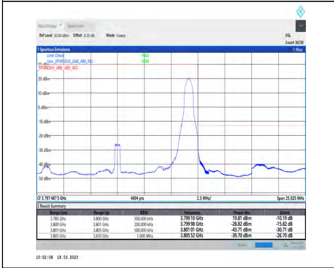
1-N78-3700-3800-30-15-H-5-CP-QPSK-Edge_1RB_Right-1@37-Ant1-1--PASS-see graph
