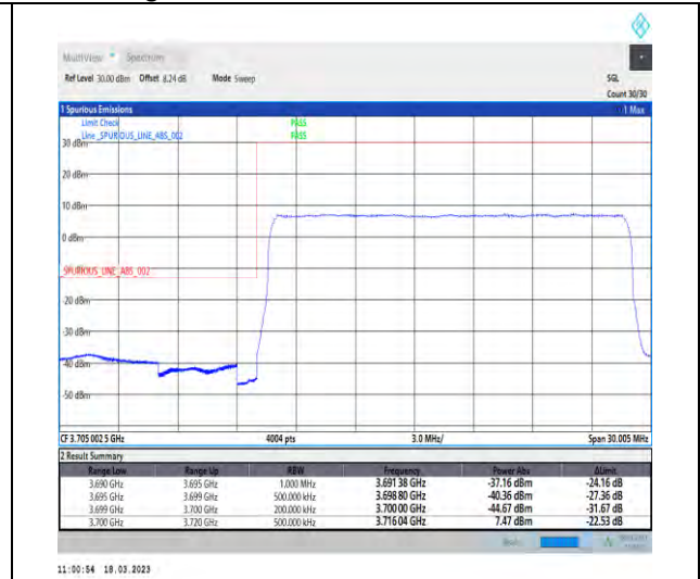
1-N78-3700-3800-30-20-L-3-DFT-PI2BPSK-Outer _Full-50@0-Ant1-1--PASS-see graph
