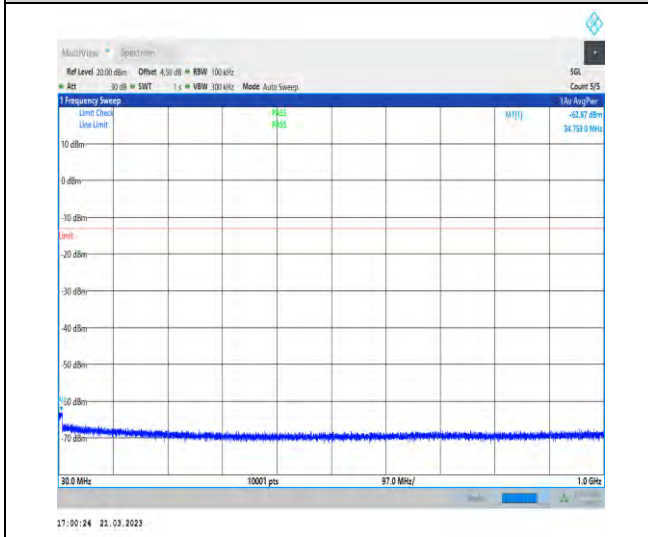
1-N78-3700-3800-30-100-H-1-DFT-QPSK-Edge_1R B_Left-1@0-0.009-0.15-Ant1-0.02--82.39--43-PASS
