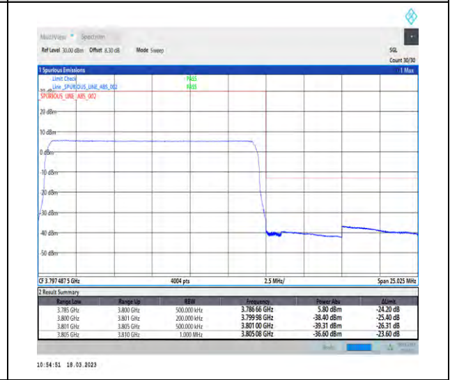
1-N78-3700-3800-30-15-H-6-CP-QPSK-Outer_Full-38@0-Ant1-1--PASS-see graph
