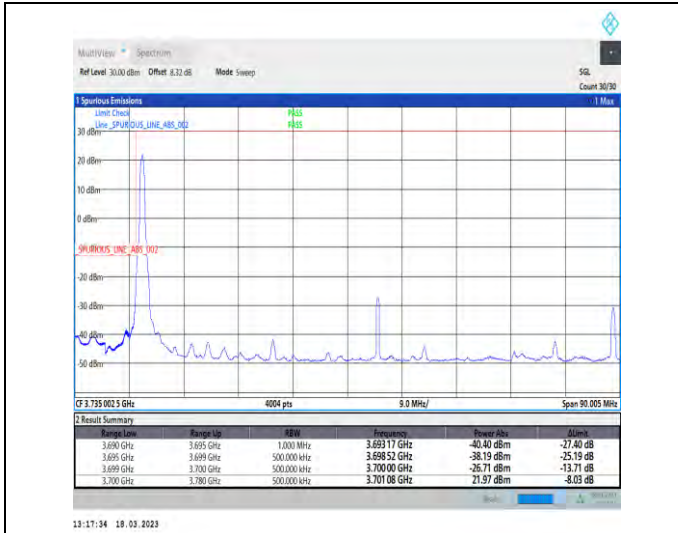
1-N78-3700-3800-30-80-L-1-DFT-PI2BPSK-Edge_1RB_Left-1@0-Ant1-1--PASS-see graph
