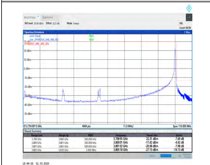
1-N78-3700-3800-30-100-H-5-CP-QPSK-Edge_1RB_Right-1@272-Ant1-1--PASS-see graph
