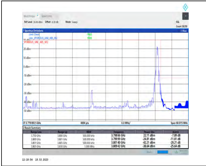
1-N78-3700-3800-30-50-H-2-DFT-PI2BPSK-Edge_1R B_Right-1@132-Ant1-1--PASS-see graph
