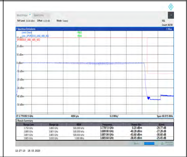
1-N78-3700-3800-30-50-H-6-CP-QPSK-Outer_Full-133@0-Ant1-1--PASS-see graph
