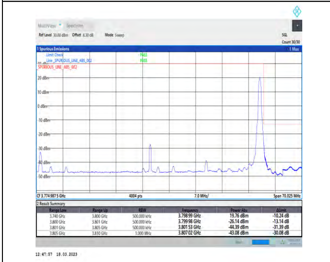
1-N78-3700-3800-30-60-H-5-CP-QPSK-Edge_1RB_Right-1@161-Ant1-1--PASS-see graph
