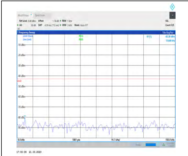
1-N78-3700-3800-30-100-H-1-DFT-QPSK-Edge_1R B_Left-1@0-0.009-0.15-Ant1-0.02--82.39--43-PASS
