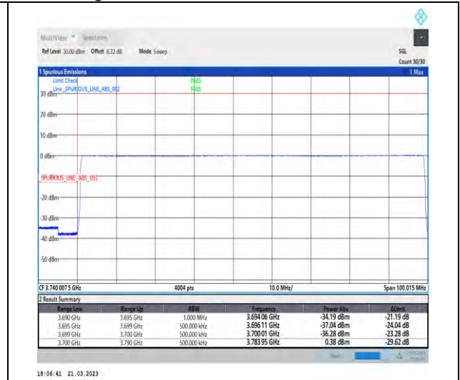
1-N78-3700-3800-30-90-L-6-CP-QPSK-Outer_Full -245@0-Ant1-1--PASS-see graph
