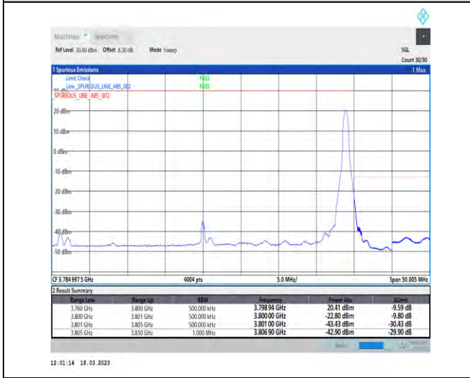
1-N78-3700-3800-30-40-H-5-CP-QPSK-Edge_1RB_Right-1@105-Ant1-1--PASS-see graph
