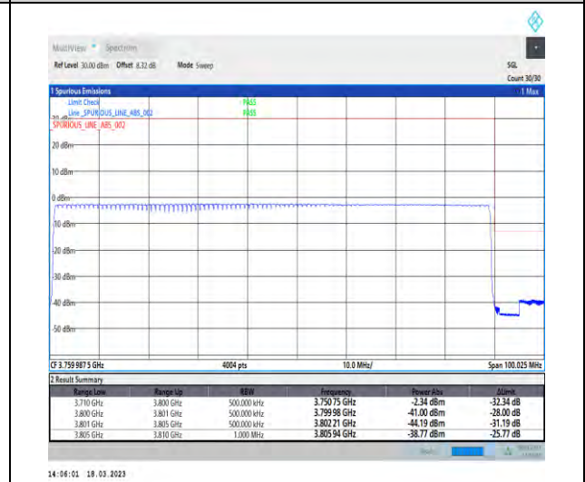
1-N78-3700-3800-30-90-H-6-CP-QPSK-Outer_Full-245@0-Ant1-1--PASS-see graph
