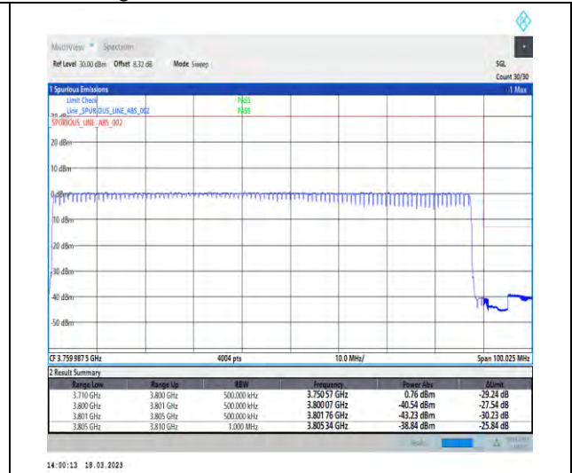
1-N78-3700-3800-30-90-H-3-DFT-PI2BPSK-Outer_Full-240@0-Ant1-1--PASS-see graph
