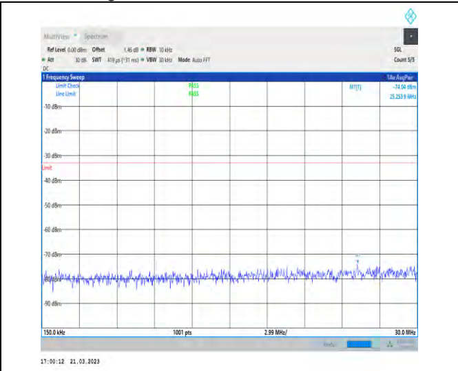
1-N78-3700-3800-30-100-H-1-DFT-QPSK-Edge_1RB _Left-1@0-0.15-30-Ant1-25.25--74.04--33-PASS
