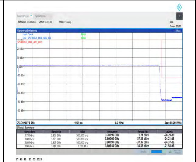
1-N78-3700-3800-30-70-H-6-CP-QPSK-Outer_Full -189@0-Ant1-1--PASS-see graph
