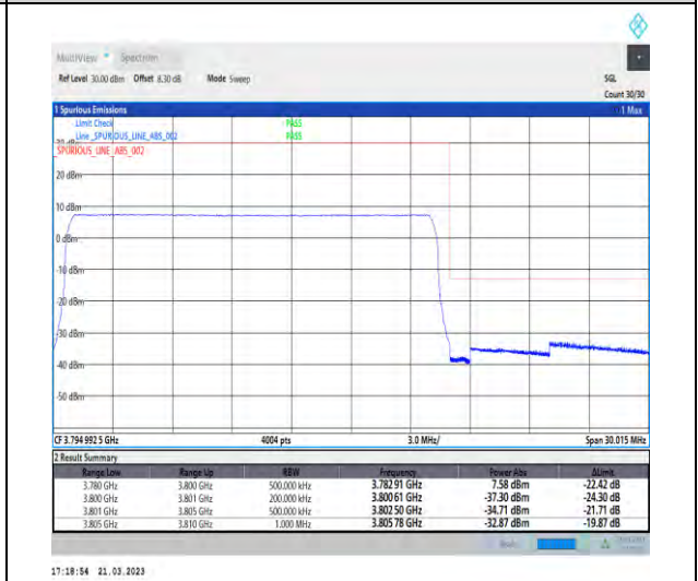
1-N78-3700-3800-30-20-H-6-CP-QPSK-Outer_Full -51@0-Ant1-1--PASS-see graph
