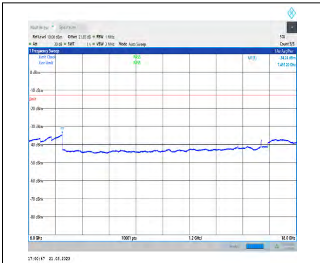
1-N78-3700-3800-30-100-H-1-DFT-QPSK-Edge_1R B_Left-1@0-6000-18000-Ant1-7495.20--34.24--13-P ASS
