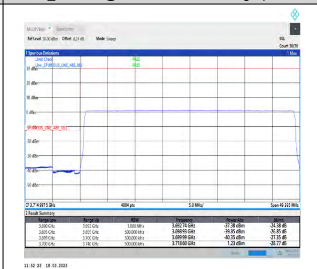
1-N78-3700-3800-30-40-L-6-CP-QPSK-Outer_Full -106@0-Ant1-1--PASS-see graph
