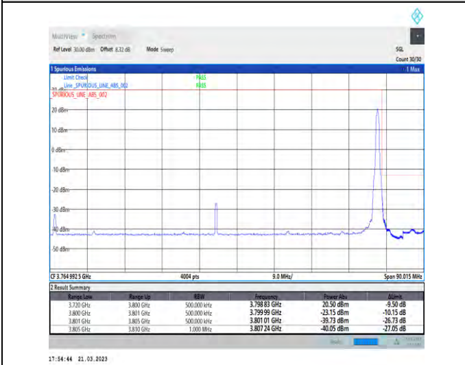
1-N78-3700-3800-30-80-H-5-CP-QPSK-Edge_1RB_Ri ght-1@216-Ant1-1--PASS-see graph
