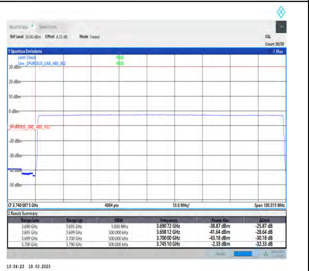
1-N78-3700-3800-30-90-L-6-CP-QPSK-Outer_Full -245@0-Ant1-1--PASS-see graph
