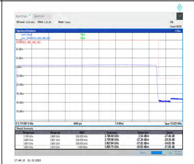
1-N78-3700-3800-30-60-H-6-CP-QPSK-Outer_Full -162@0-Ant1-1--PASS-see graph
