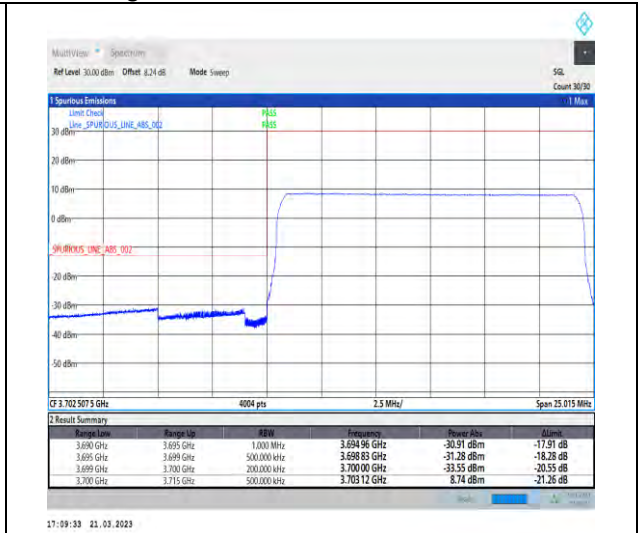
1-N78-3700-3800-30-15-L-6-CP-QPSK-Outer_Full -38@0-Ant1-1--PASS-see graph
