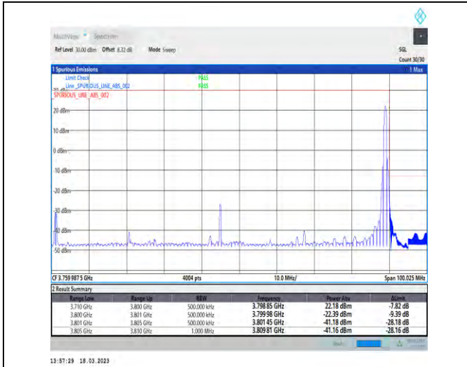
1-N78-3700-3800-30-90-H-2-DFT-PI2BPSK-Edge_1R_B_Right-1@244-Ant1-1--PASS-see graph
