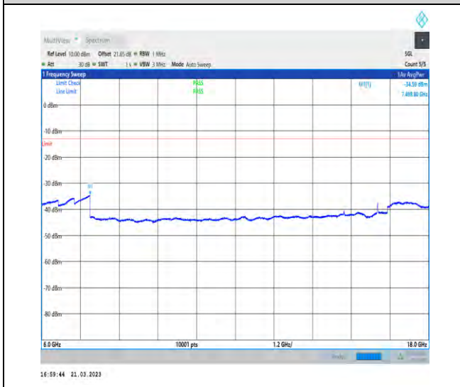
1-N78-3700-3800-30-100-M-1-DFT-QPSK-Edge_1R B_Left-1@0-6000-18000-Ant1-7498.80--34.59--13-P ASS
