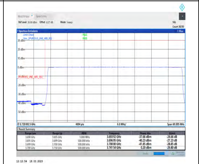
1-N78-3700-3800-30-50-L-6-CP-QPSK-Outer_Full -133@0-Ant1-1--PASS-see graph
