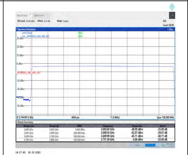
1-N78-3700-3800-30-100-L-6-CP-QPSK-Outer_Full-273@0-Ant1-1--PASS-see graph
