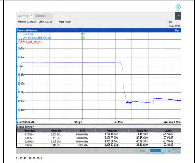
1-N78-3700-3800-30-20-H-6-CP-QPSK-Outer_Full-51@0-Ant1-1--PASS-see graph
