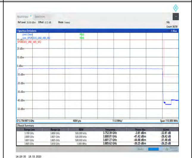
1-N78-3700-3800-30-100-H-6-CP-QPSK-Outer_Full-273@0-Ant1-1--PASS-see graph
