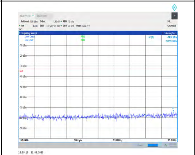
1-N78-3700-3800-30-100-M-1-DFT-QPSK-Edge_1R B_Left-1@0-0.15-30-Ant1-29.25--74.32--33-PASS
