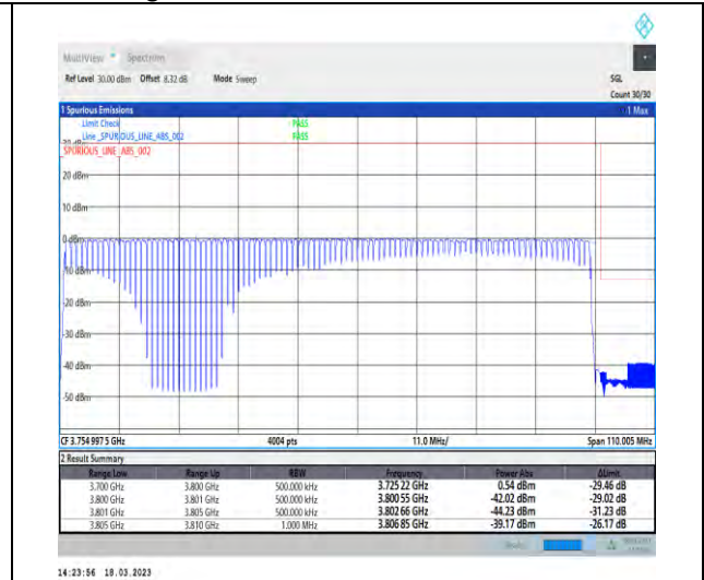
1-N78-3700-3800-30-100-H-3-DFT-PI2BPSK-Outer_Full-270@0-Ant1-1--PASS-see graph
