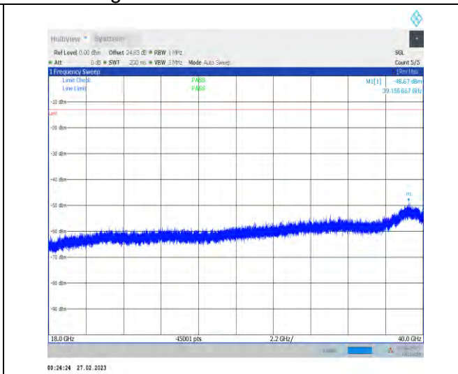
1-N78-3700-3800-30-100-H-1-DFT-PI2BPSK-Inner_1RB_Left-1@1-18000-40000-Ant1-18000.00--58.70--1 3-PASS
