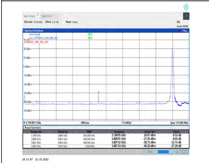
1-N78-3700-3800-30-100-H-5-CP-QPSK-Edge_1RB_R ight-1@272-Ant1-1--PASS-see graph
