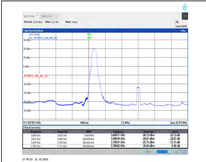
1-N78-3700-3800-30-15-L-4-CP-QPSK-Edge_1RB_Lef t-1@0-Ant1-1--PASS-see graph
