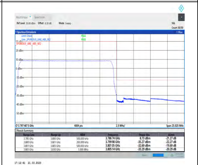
1-N78-3700-3800-30-15-H-6-CP-QPSK-Outer_Full -38@0-Ant1-1--PASS-see graph
