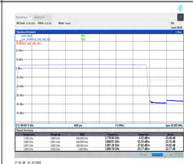
1-N78-3700-3800-30-40-H-6-CP-QPSK-Outer_Full -106@0-Ant1-1--PASS-see graph
