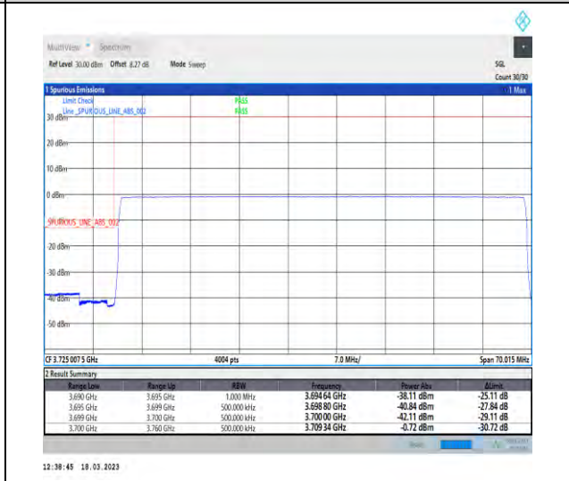
1-N78-3700-3800-30-60-L-6-CP-QPSK-Outer_Full -162@0-Ant1-1--PASS-see graph
