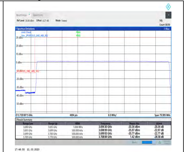
1-N78-3700-3800-30-70-L-6-CP-QPSK-Outer_Full -189@0-Ant1-1--PASS-see graph
