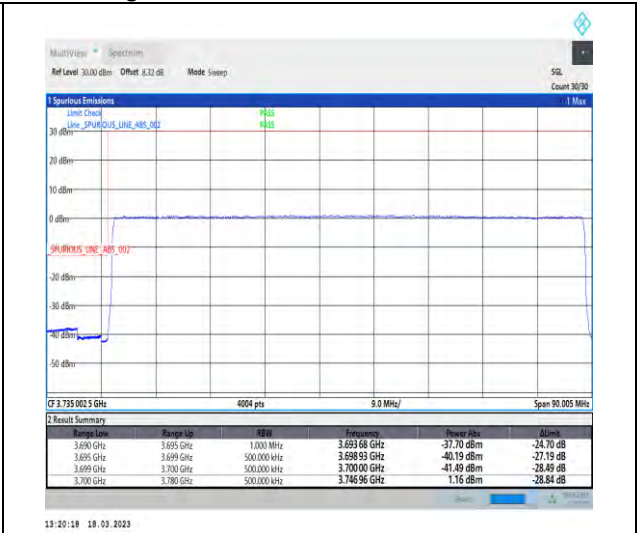
1-N78-3700-3800-30-80-L-3-DFT-PI2BPSK-Outer_Full-216@0-Ant1-1--PASS-see graph
