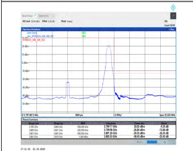
1-N78-3700-3800-30-15-H-5-CP-QPSK-Edge_1RB_Ri ght-1@37-Ant1-1--PASS-see graph
