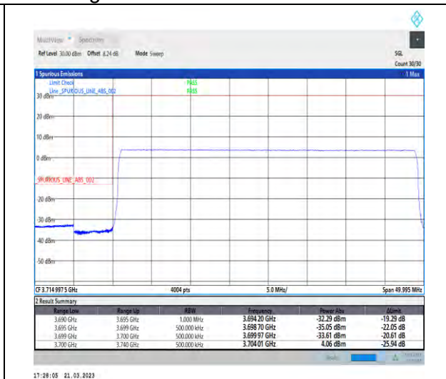
1-N78-3700-3800-30-40-L-6-CP-QPSK-Outer_Full -106@0-Ant1-1--PASS-see graph
