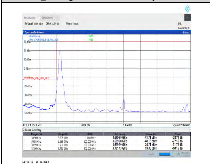
1-N78-3700-3800-30-40-L-4-CP-QPSK-Edge_1RB_Lef t-1@0-Ant1-1--PASS-see graph
