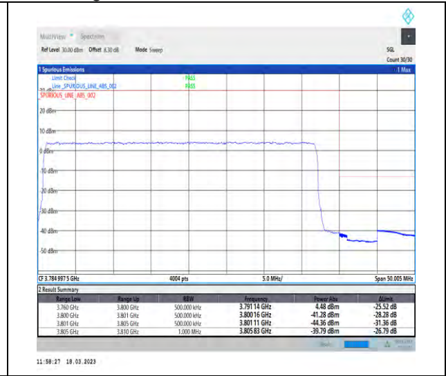
1-N78-3700-3800-30-40-H-3-DFT-PI2BPSK-Outer_Full-100@0-Ant1-1--PASS-see graph
