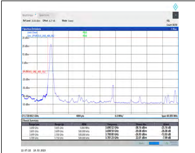
1-N78-3700-3800-30-50-L-1-DFT-PI2BPSK-Edge_1RB_Left-1@0-Ant1-1--PASS-see graph
