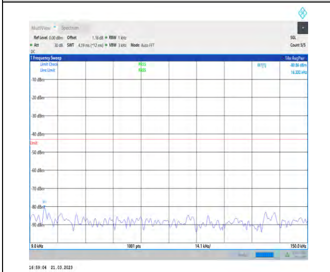
1-N78-3700-3800-30-100-M-1-DFT-QPSK-Edge_1R B_Left-1@0-0.009-0.15-Ant1-0.02--80.86--43-PASS
