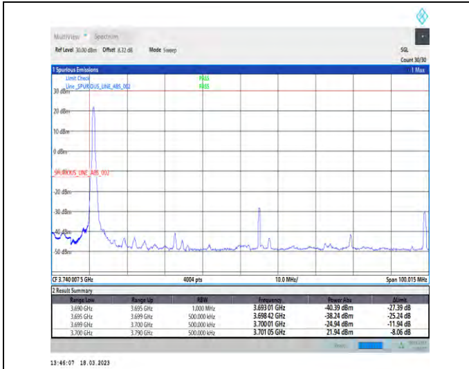
1-N78-3700-3800-30-90-L-1-DFT-PI2BPSK-Edge_1RB_Left-1@0-Ant1-1--PASS-see graph
