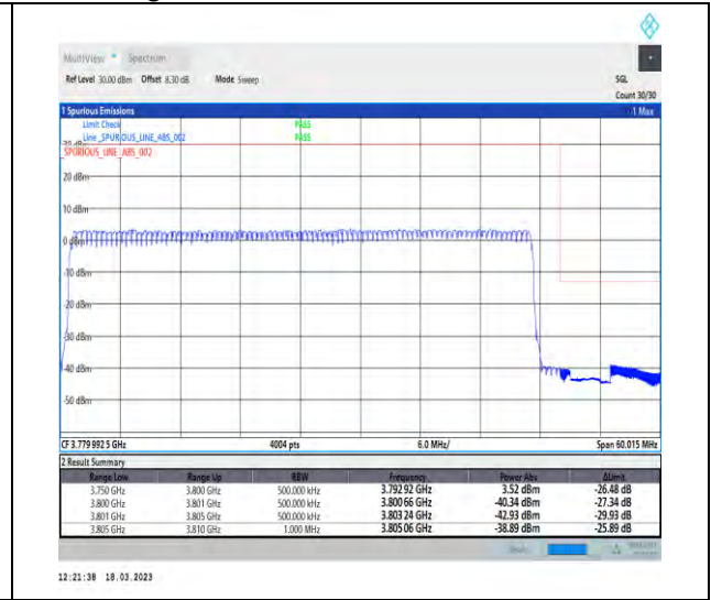
1-N78-3700-3800-30-50-H-3-DFT-PI2BPSK-Outer_Full-128@0-Ant1-1--PASS-see graph
