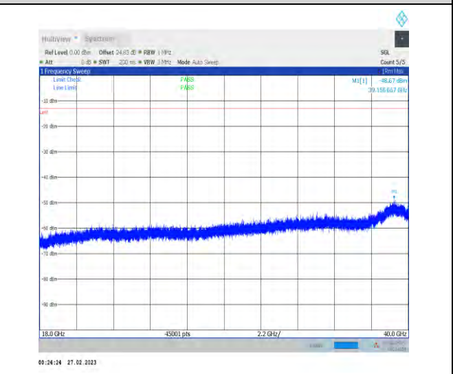
1-N78-3700-3800-30-100-M-1-DFT-QPSK-Edge_1R B_Left-1@0-18000-40000-Ant1-18000.00--38.63--13-P PASS
