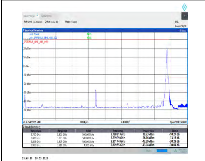
1-N78-3700-3800-30-80-H-5-CP-QPSK-Edge_1RB_Right-1@216-Ant1-1--PASS-see graph
