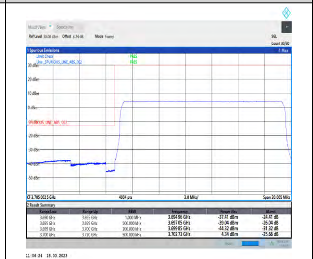
1-N78-3700-3800-30-20-L-6-CP-QPSK-Outer_Full -51@0-Ant1-1--PASS-see graph
