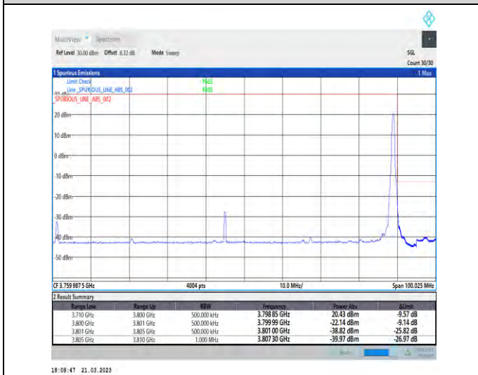
1-N78-3700-3800-30-90-H-5-CP-QPSK-Edge_1RB_Ri ght-1@244-Ant1-1--PASS-see graph
