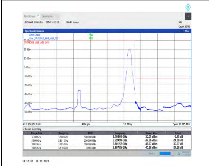
1-N78-3700-3800-30-20-H-5-CP-QPSK-Edge_1RB_Right-1@50-Ant1-1--PASS-see graph
