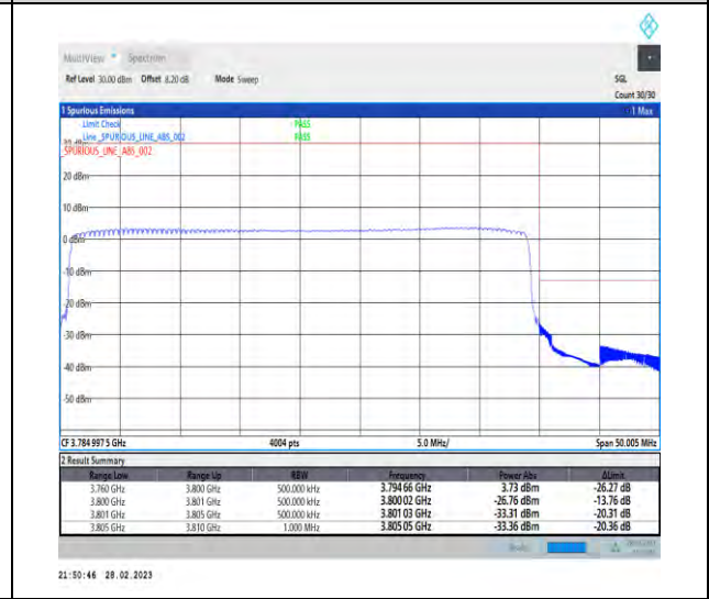
1-N78-3700-3800-30-40-H-6-CP-QPSK-Outer_Full-106@0-Ant1-1--PASS-see graph
