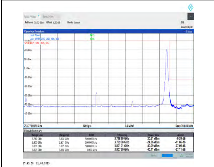
1-N78-3700-3800-30-60-H-5-CP-QPSK-Edge_1RB_Ri ght-1@161-Ant1-1--PASS-see graph
