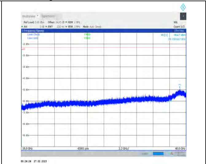
1-N78-3700-3800-30-100-L-1-DFT-QPSK-Edge_1RB _Left-1@0-18000-40000-Ant1-18000.00--38.62--13-P ASS
