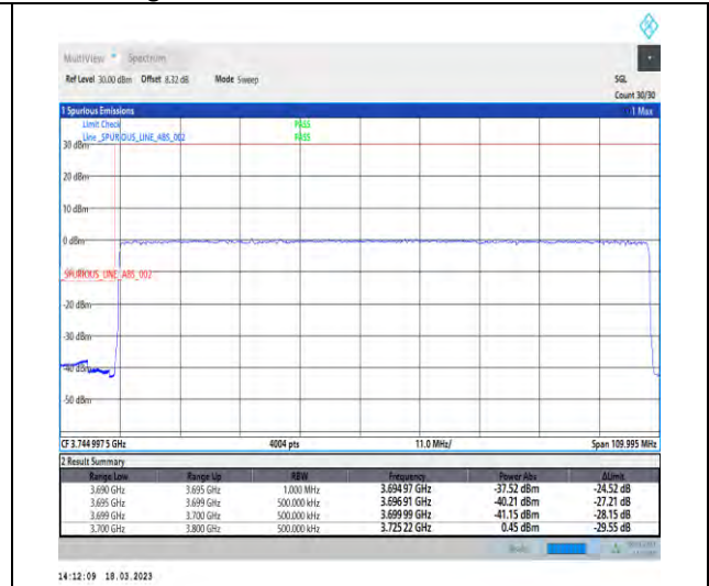
1-N78-3700-3800-30-100-L-3-DFT-PI2BPSK-Outer_Full-270@0-Ant1-1--PASS-see graph
