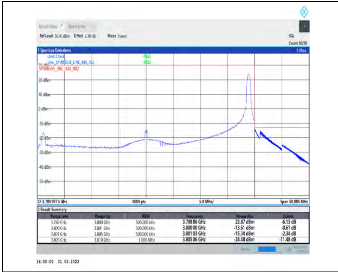
1-N78-3700-3800-30-40-H-2-DFT-PI2BPSK-Edge_1R_B_Right-1@105-Ant1-1--PASS-see graph
