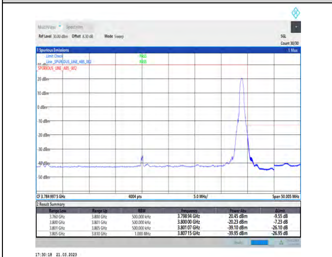
1-N78-3700-3800-30-40-H-5-CP-QPSK-Edge_1RB_Ri ght-1@105-Ant1-1--PASS-see graph
