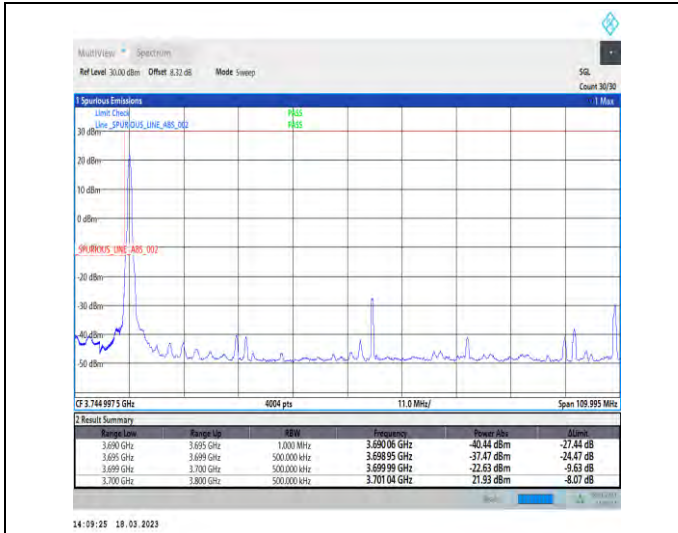
1-N78-3700-3800-30-100-L-1-DFT-PI2BPSK-Edge_1R_B_Left-1@0-Ant1-1--PASS-see graph
