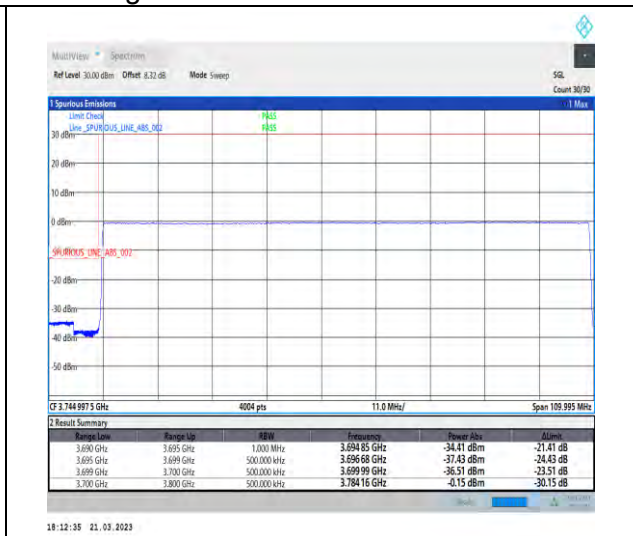
1-N78-3700-3800-30-100-L-6-CP-QPSK-Outer_Fu ll-273@0-Ant1-1--PASS-see graph
