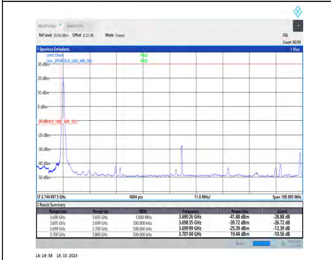
1-N78-3700-3800-30-100-L-4-CP-QPSK-Edge_1RB_Left-1@0-Ant1-1--PASS-see graph
