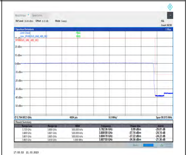
1-N78-3700-3800-30-80-H-6-CP-QPSK-Outer_Full -217@0-Ant1-1--PASS-see graph
