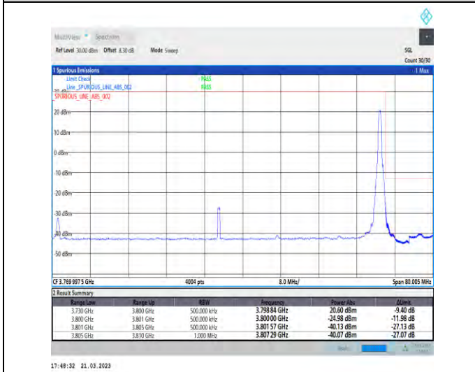
1-N78-3700-3800-30-70-H-5-CP-QPSK-Edge_1RB_Ri ght-1@188-Ant1-1--PASS-see graph
