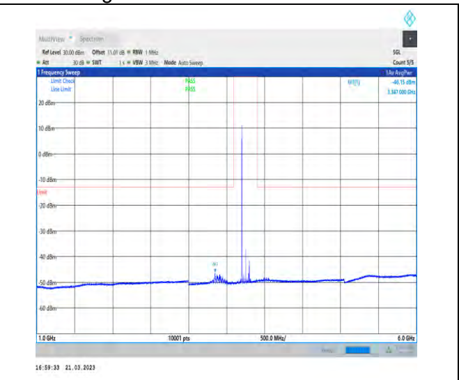
1-N78-3700-3800-30-100-M-1-DFT-QPSK-Edge_1R B_Left-1@0-1000-6000-Ant1-3347.00--46.15--13-PA SS
