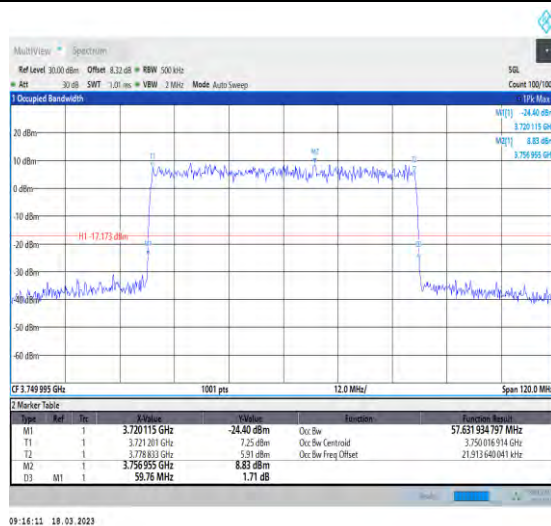
1-N78-3700-3800-30-60-M-7-CP-16QAM-Outer_Full-I-162@0-Ant1-57.632-59.760-≤60-PASS
