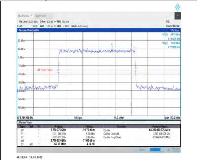
1-N78-3700-3800-30-70-H-1-DFT-QPSK-Outer_Full-180@0-Ant1-64.284-66.360-≤70-PASS
