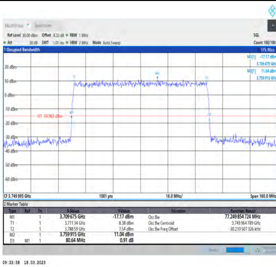
1-N78-3700-3800-30-80-M-6-CP-QPSK-Outer_Full-2 17@0-Ant1-77.25-80.640-≤80-PASS
