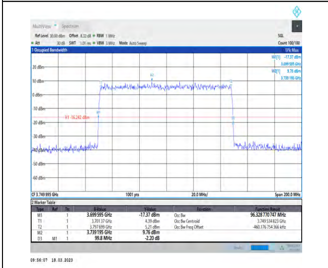
1-N78-3700-3800-30-100-H-5-DFT-256QAM-Outer_Full-270@0-Ant1-96.329-99.800-≤100-PASS
