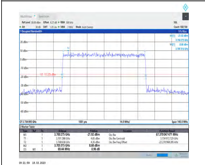
1-N78-3700-3800-30-70-L-8-CP-64QAM-Outer_Full-189@0-Ant1-67.37-69.440-≤70-PASS
