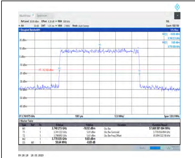
1-N78-3700-3800-30-60-H-3-DFT-16QAM-Outer_Ful I-162@0-Ant1-57.669-59.640-≤60-PASS
