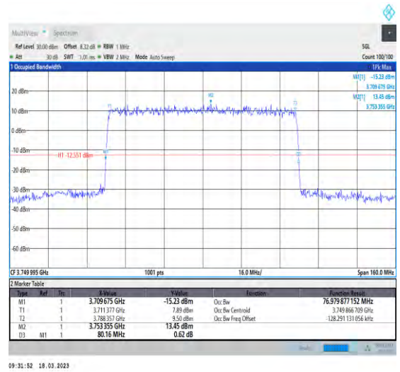
1-N78-3700-3800-30-80-M-1-DFT-QPSK-Outer_Full-216@0-Ant1-76.98-80.160-≤80-PASS
