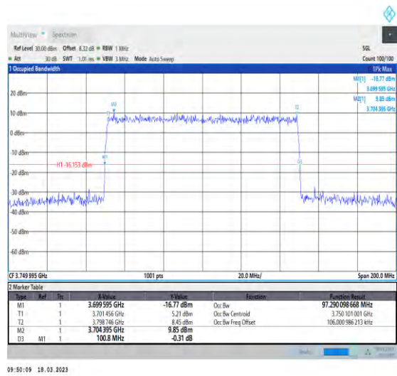
1-N78-3700-3800-30-100-L-6-CP-QPSK-Outer_Full-273@0-Ant1-97.29-100.800-≤100-PASS
