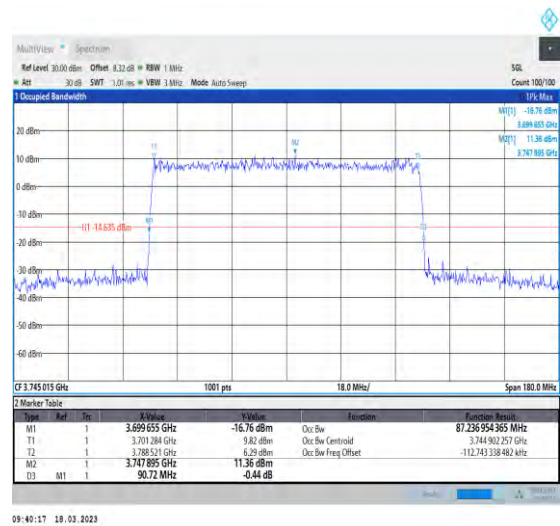
1-N78-3700-3800-30-90-L-7-CP-16QAM-Outer_Full-245@0-Ant1-87.237-90.720-≤90-PASS
