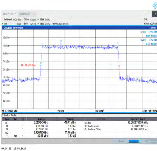
1-N78-3700-3800-30-80-L-7-CP-16QAM-Outer_Full-217@0-Ant1-77.363-80.480-≤80-PASS
