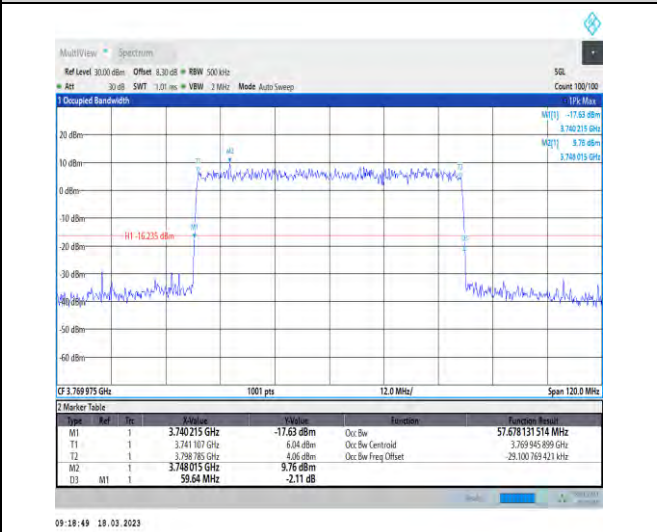
1-N78-3700-3800-30-60-H-6-CP-QPSK-Outer_Full-62@0-Ant1-57.678-59.640-≤60-PASS
