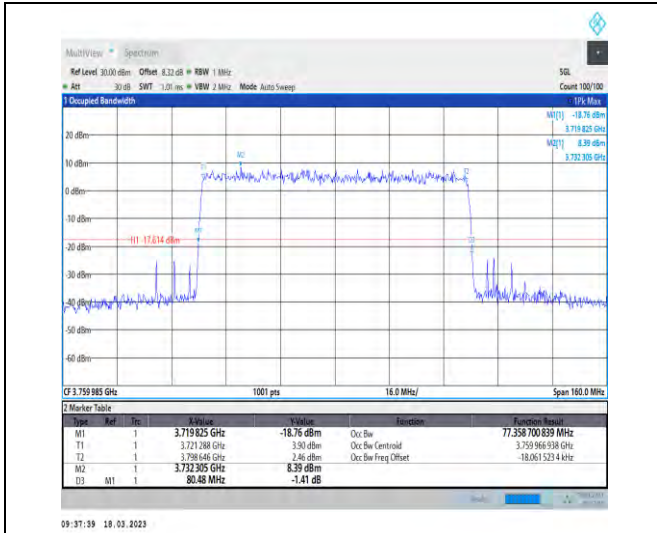
1-N78-3700-3800-30-80-H-9-CP-256QAM-Outer_Full-I-217@0-Ant1-77.359-80.480-≤80-PASS
