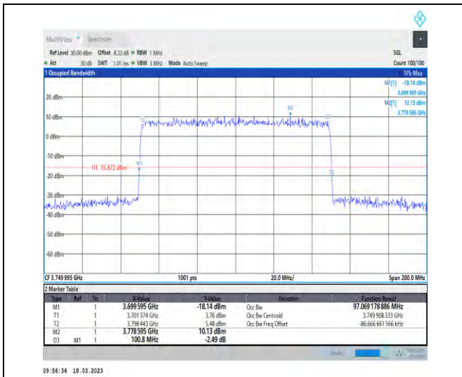
1-N78-3700-3800-30-100-H-7-CP-16QAM-Outer_Ful I-273@0-Ant1-97.069-100.800-≤100-PASS
