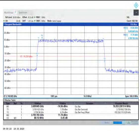
1-N78-3700-3800-30-80-L-4-DFT-64QAM-Outer_Full -216@0-Ant1-76.955-80.160-<80-PASS
