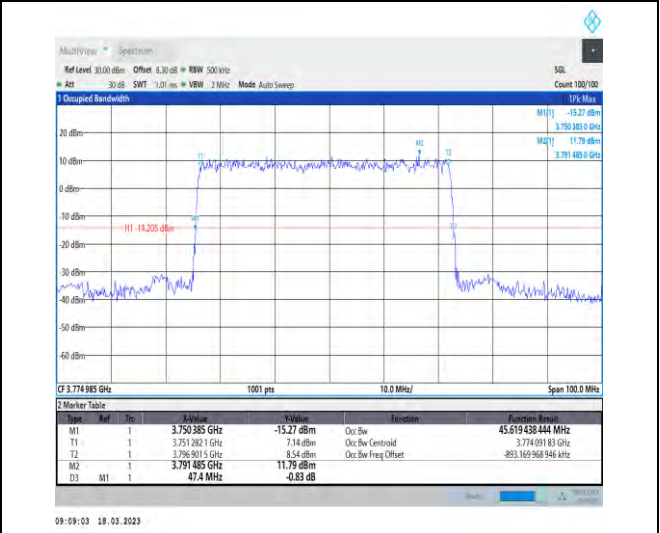
1-N78-3700-3800-30-50-H-1-DFT-QPSK-Outer_Full-128@0-Ant1-45.619-47.400-≤50-PASS
