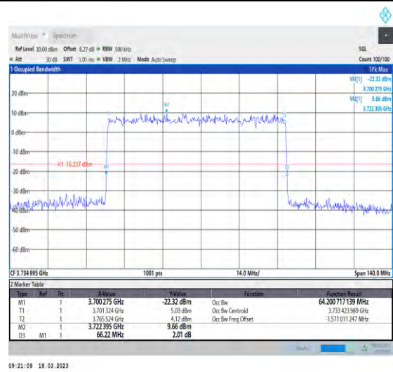
1-N78-3700-3800-30-70-L-3-DFT-16QAM-Outer_Full-180@0-Ant1-64.201-66.220-≤70-PASS
