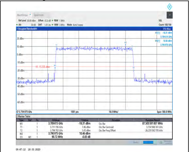
1-N78-3700-3800-30-90-H-7-CP-16QAM-Outer_Full-245@0-Ant1-87.506-90.720-≤90-PASS
