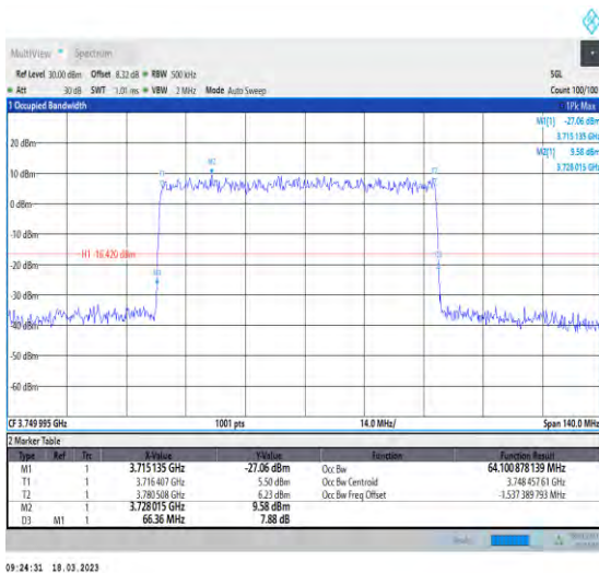
1-N78-3700-3800-30-70-M-3-DFT-16QAM-Outer_Full-180@0-Ant1-64.101-66.360-≤70-PASS
