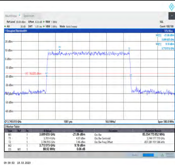
1-N78-3700-3800-30-90-L-5-DFT-256QAM-Outer_Full-240@0-Ant1-85.555-88.920-≤90-PASS
