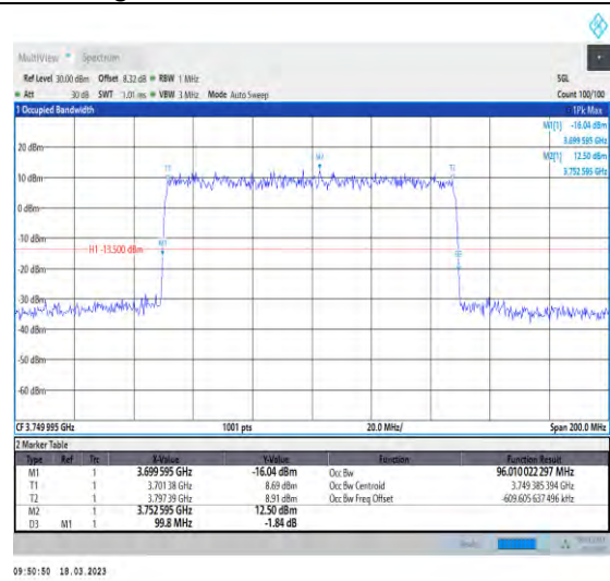
1-N78-3700-3800-30-100-M-1-DFT-QPSK-Outer_Ful I-270@0-Ant1-96.01-99.800-≤100-PASS
