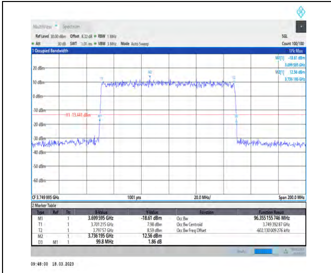
1-N78-3700-3800-30-100-L-1-DFT-QPSK-Outer_Full -270@0-Ant1-96.355-99.800-≤100-PASS
