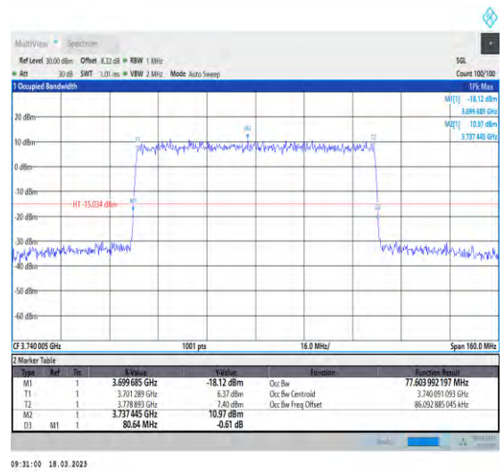
1-N78-3700-3800-30-80-L-8-CP-64QAM-Outer_Full-217@0-Ant1-77.604-80.640-≤80-PASS
