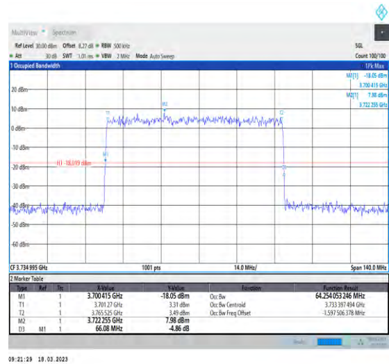
1-N78-3700-3800-30-70-L-5-DFT-256QAM-Outer_Full-180@0-Ant1-64.254-66.080-≤70-PASS
