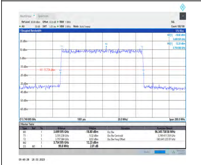
1-N78-3700-3800-30-100-L-3-DFT-16QAM-Outer_Fu ll-270@0-Ant1-96.346-99.800-≤100-PASS
