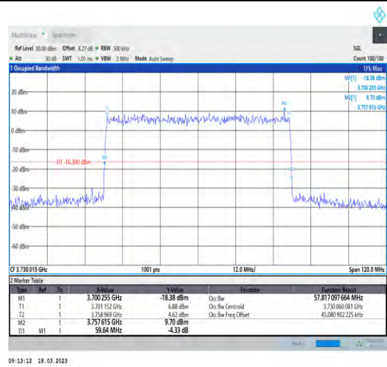
1-N78-3700-3800-30-60-L-6-CP-QPSK-Outer_Full-1 62@0-Ant1-57.817-59.640-≤60-PASS
