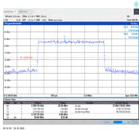
1-N78-3700-3800-30-60-L-8-CP-64QAM-Outer_Full-162@0-Ant1-57.856-59.640-≤60-PASS
