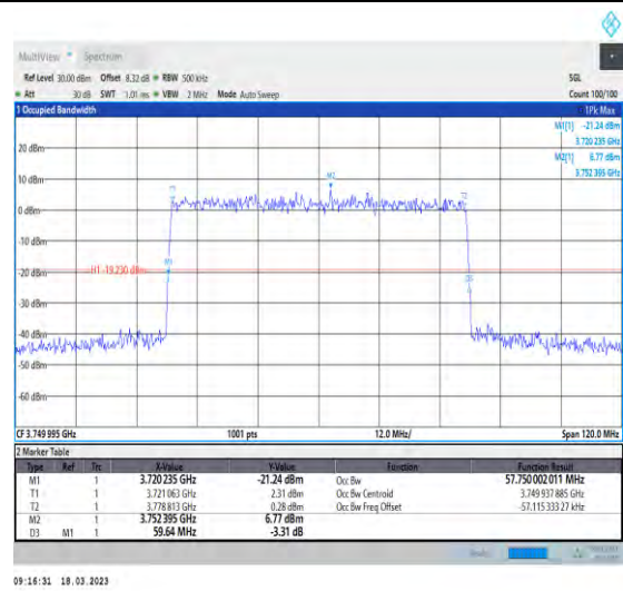
1-N78-3700-3800-30-60-M-9-CP-256QAM-Outer_Fu II-162@0-Ant1-57.75-59.640-≤60-PASS
