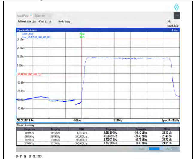
1-N78-3700-3800-30-15-L-3-DFT-PI2BPSK-Outer_Full-36@0-Ant1-1--PASS-see graph
