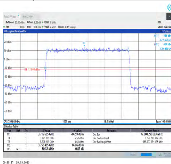
1-N78-3700-3800-30-80-H-2-DFT-PI2BPSK-Outer_Full-216@0-Ant1-77-80.320-≤80-PASS
