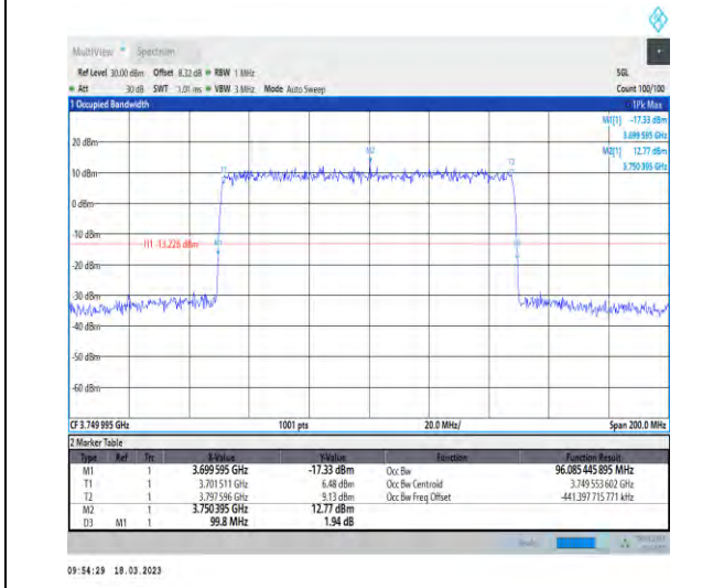
1-N78-3700-3800-30-100-H-1-DFT-QPSK-Outer_Full-I-270@0-Ant1-96.085-99.800-≤100-PASS
