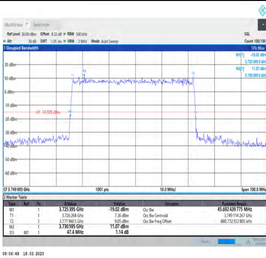
1-N78-3700-3800-30-50-M-3-DFT-16QAM-Outer_Full-128@0-Ant1-45.692-47.400-≤50-PASS
