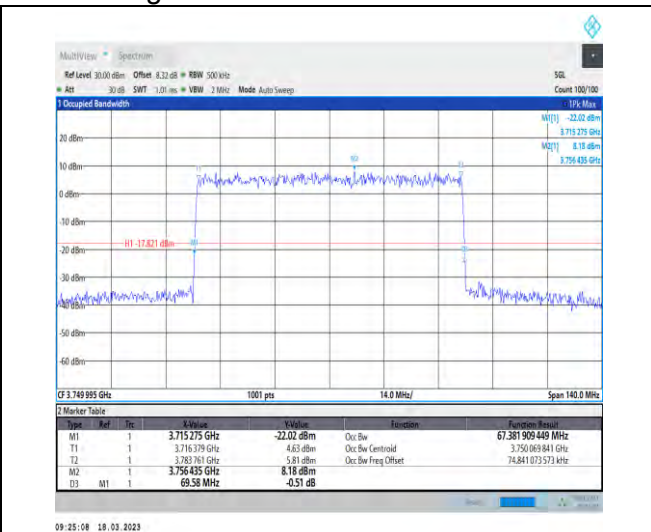
1-N78-3700-3800-30-70-M-6-CP-QPSK-Outer_Full-189@0-Ant1-67.382-69.580-≤70-PASS
