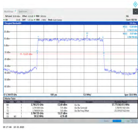
1-N78-3700-3800-30-60-H-2-DFT-PI2BPSK-Outer_Full-162@0-Ant1-57.776-59.520-≤60-PASS
