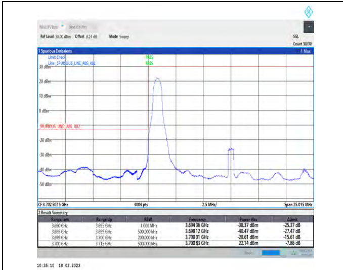
1-N78-3700-3800-30-15-L-1-DFT-PI2BPSK-Edge_1RB_Left-1@0-Ant1-1--PASS-see graph
