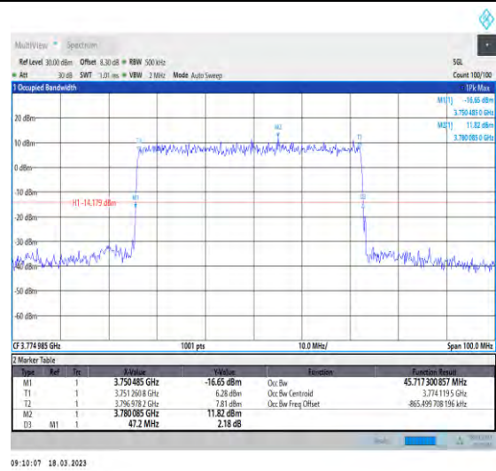
1-N78-3700-3800-30-50-H-3-DFT-16QAM-Outer_Full-128@0-Ant1-45.717-47.200-≤50-PASS
