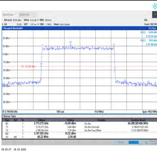
1-N78-3700-3800-30-70-M-1-DFT-QPSK-Outer_Full-180@0-Ant1-64.289-66.220-≤70-PASS
