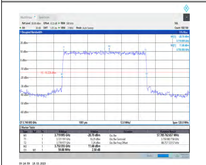
1-N78-3700-3800-30-60-M-2-DFT-PI2BPSK-Outer_Full -162@0-Ant1-57.786-59.880-≤60-PASS
