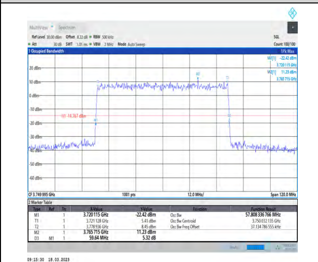
1-N78-3700-3800-30-60-M-3-DFT-16QAM-Outer_Full -162@0-Ant1-57.808-59.640-≤60-PASS
