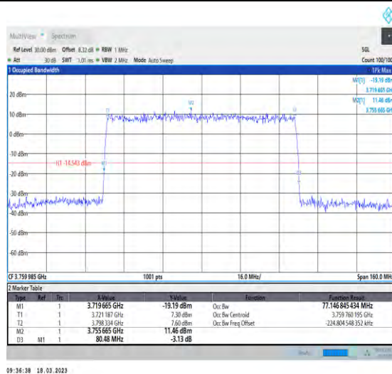
1-N78-3700-3800-30-80-H-4-DFT-64QAM-Outer_Full-216@0-Ant1-77.147-80.480-≤80-PASS
