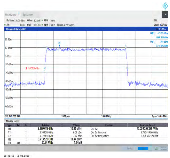
1-N78-3700-3800-30-80-L-6-CP-QPSK-Outer_Full-2 17@0-Ant1-77.258-80.640-<80-PASS
