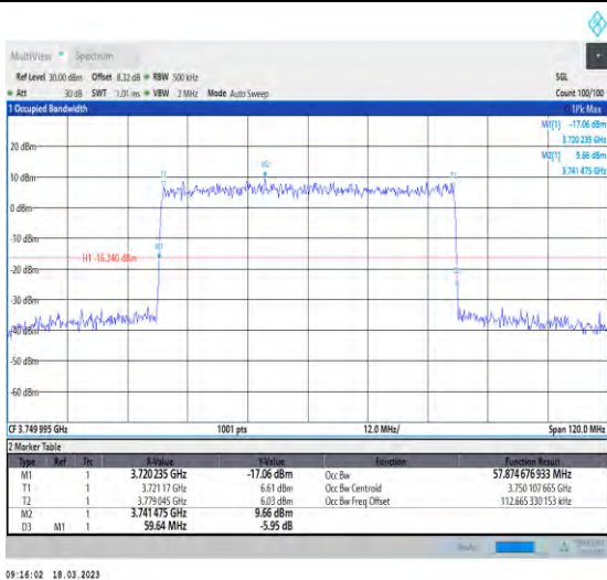
1-N78-3700-3800-30-60-M-6-CP-QPSK-Outer_Full-I-62@0-Ant1-57.875-59.640-≤60-PASS
