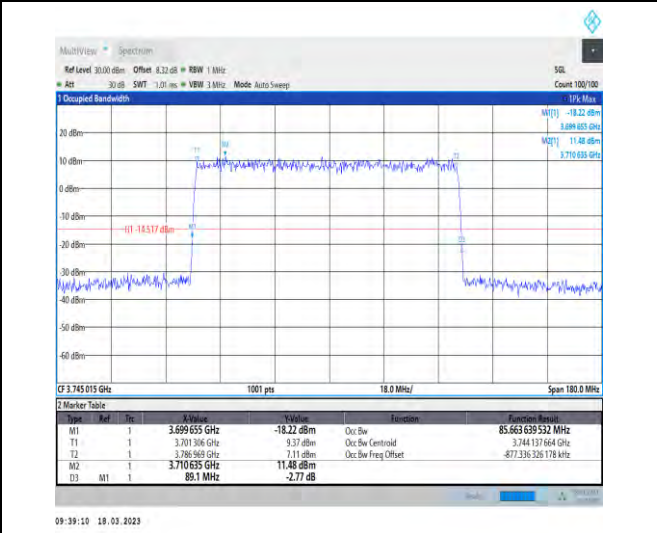
1-N78-3700-3800-30-90-L-3-DFT-16QAM-Outer_Full-240@0-Ant1-85.664-89.100-≤90-PASS
