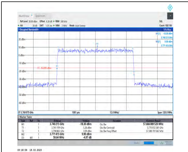
1-N78-3700-3800-30-60-H-7-CP-16QAM-Outer_Full-162@0-Ant1-57.666-59.640-≤60-PASS
