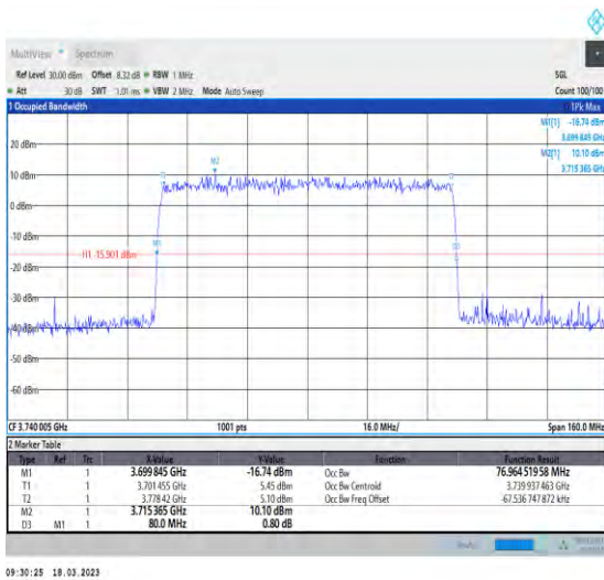
1-N78-3700-3800-30-80-L-5-DFT-256QAM-Outer_Fu ll-216@0-Ant1-76.965-80.000-<80-PASS
