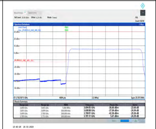
1-N78-3700-3800-30-15-L-6-CP-QPSK-Outer_Full -38@0-Ant1-1--PASS-see graph
