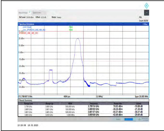
1-N78-3700-3800-30-10-H-5-CP-QPSK-Edge_1RB_Right-1@23-Ant1-1--PASS-see graph
