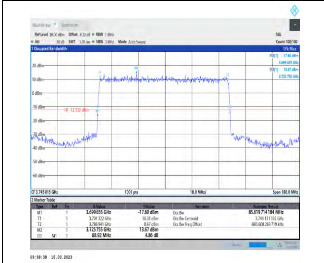
1-N78-3700-3800-30-90-L-2-DFT-PI2BPSK-Outer_Full-240@0-Ant1-85.62-88.920-≤90-PASS
