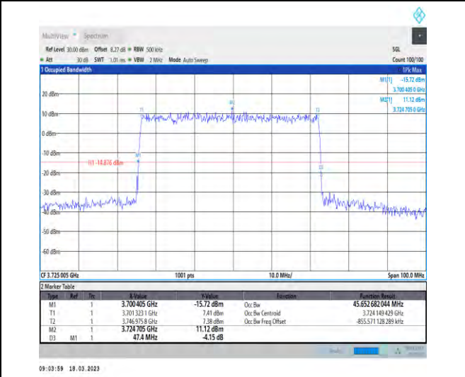
1-N78-3700-3800-30-50-L-3-DFT-16QAM-Outer_Full-128@0-Ant1-45.653-47.400-≤50-PASS
