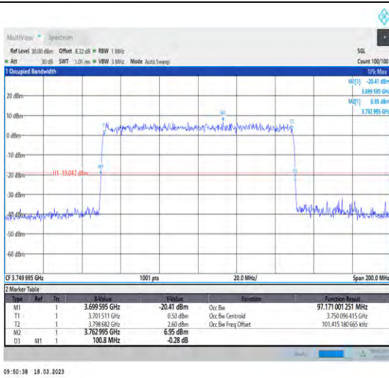
1-N78-3700-3800-30-100-L-9-CP-256QAM-Outer_F ull-273@0-Ant1-97.171-100.800-≤100-PASS
