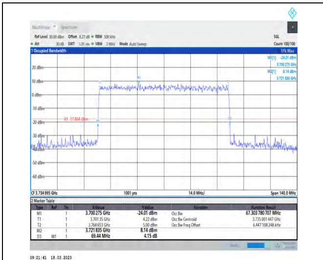
1-N78-3700-3800-30-70-L-6-CP-QPSK-Outer_Full-189@0-Ant1-67.304-69.440-≤70-PASS
