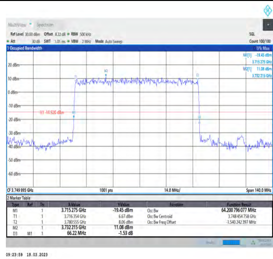
1-N78-3700-3800-30-70-M-2-DFT-PI2BPSK-Outer_Full-180@0-Ant1-64.201-66.220-≤70-PASS
