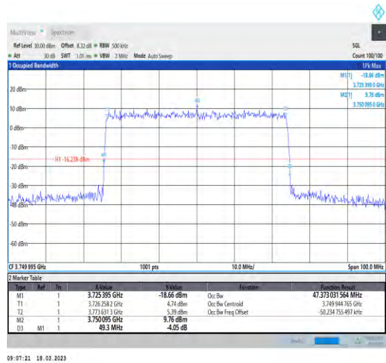
1-N78-3700-3800-30-50-M-6-CP-QPSK-Outer_Full-128@0-Ant1-47.373-49.300-≤50-PASS
