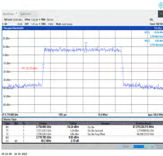
1-N78-3700-3800-30-50-H-8-CP-64QAM-Outer_Full-133@0-Ant1-47.319-49.200-≤50-PASS
