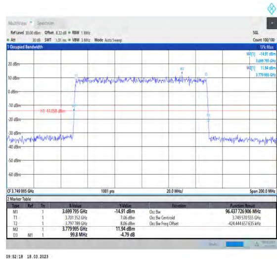
1-N78-3700-3800-30-100-M-3-DFT-16QAM-Outer_F ull-270@0-Ant1-96.438-99.800-≤100-PASS
