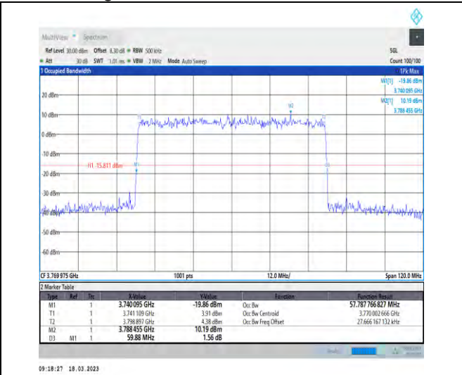
1-N78-3700-3800-30-60-H-4-DFT-64QAM-Outer_Ful I-162@0-Ant1-57.788-59.880-≤60-PASS
