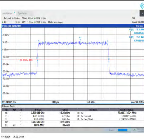
1-N78-3700-3800-30-80-L-3-DFT-16QAM-Outer_Full -216@0-Ant1-77.09-80.160-<80-PASS
