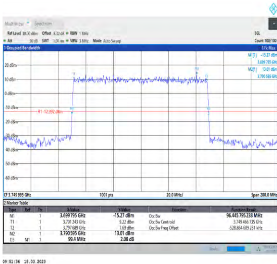
1-N78-3700-3800-30-100-M-2-DFT-PI2BPSK-Outer_ Full-270@0-Ant1-96.446-99.400-≤100-PASS
