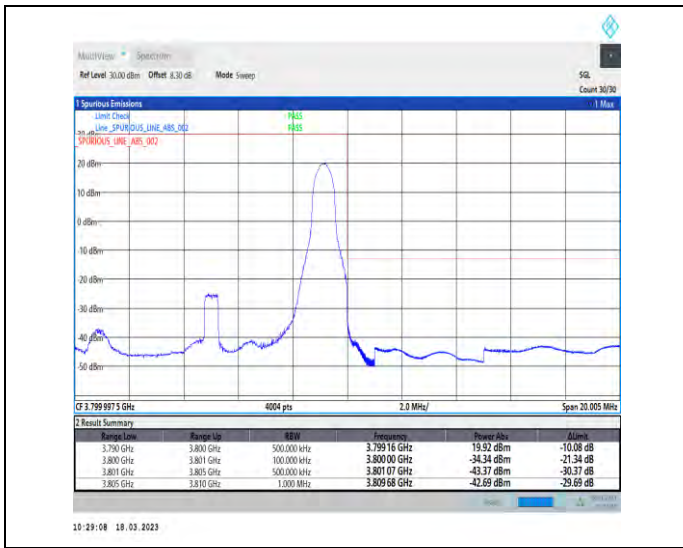
1-N78-3700-3800-30-10-H-2-DFT-PI2BPSK-Edge_1R_B_Right-1@23-Ant1-1--PASS-see graph
