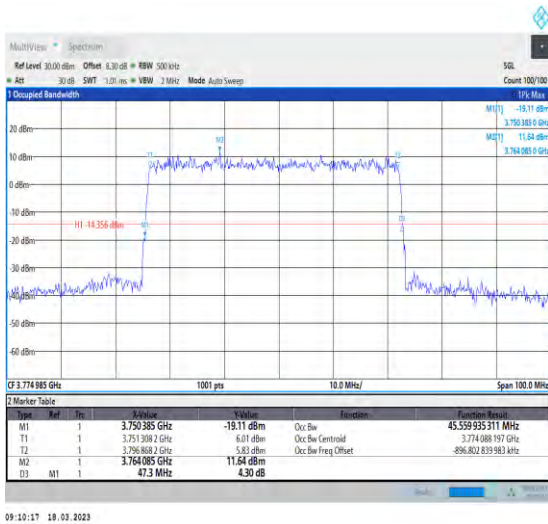
1-N78-3700-3800-30-50-H-4-DFT-64QAM-Outer_Full-128@0-Ant1-45.56-47.300-≤50-PASS
