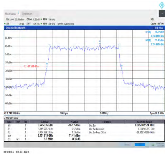
1-N78-3700-3800-30-10-M-3-DFT-16QAM-Outer_Full -24@0-Ant1-8.605-9.300-≤10-PASS
