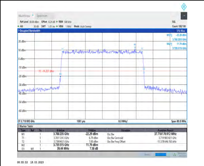
1-N78-3700-3800-30-40-L-6-CP-QPSK-Outer_Full-1 06@0-Ant1-37.718-39.440-≤40-PASS
