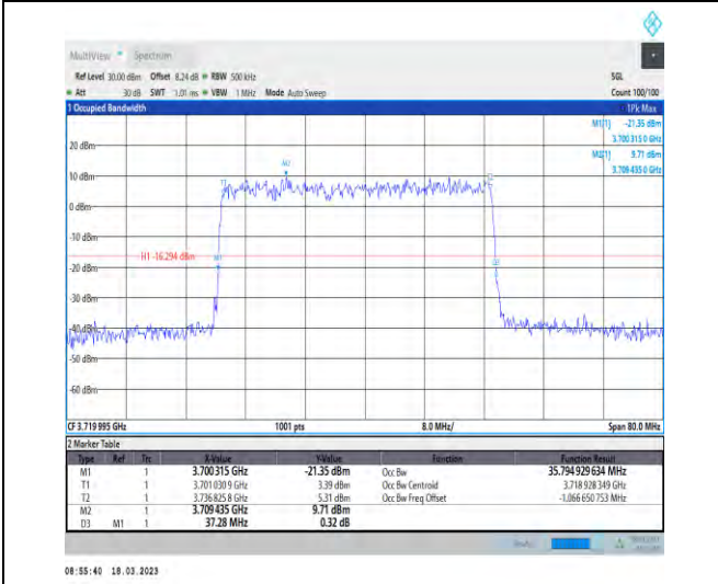
1-N78-3700-3800-30-40-L-5-DFT-256QAM-Outer_Fu II-100@0-Ant1-35.795-37.280-≤40-PASS
