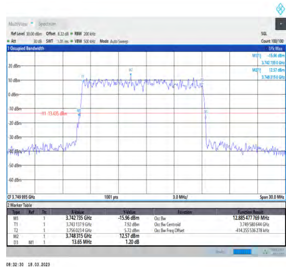
1-N78-3700-3800-30-15-M-4-DFT-64QAM-Outer_Full-36@0-Ant1-12.885-13.650-≤15-PASS
