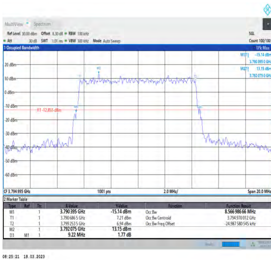
1-N78-3700-3800-30-10-H-1-DFT-QPSK-Outer_Full-24@0-Ant1-8.567-9.220-≤10-PASS
