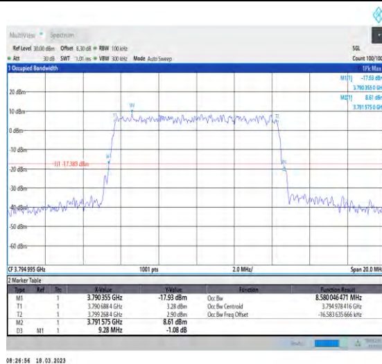
1-N78-3700-3800-30-10-H-6-CP-QPSK-Outer_Full-24@0-Ant1-8.58-9.280-≤10-PASS
