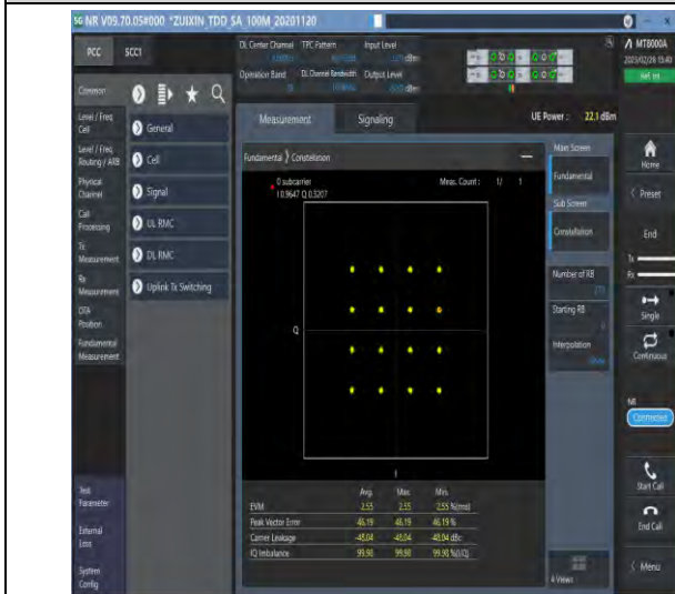
1-N78-3700-3800-30-100-M-7-CP-16QAM-Outer_Full-273@0-Ant1-see graph-PASS
