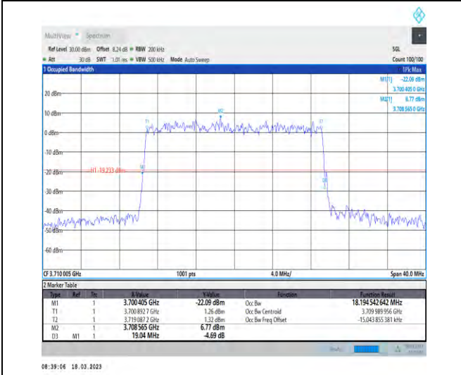
1-N78-3700-3800-30-20-L-9-CP-256QAM-Outer_Full-51@0-Ant1-18.195-19.040-≤20-PASS
