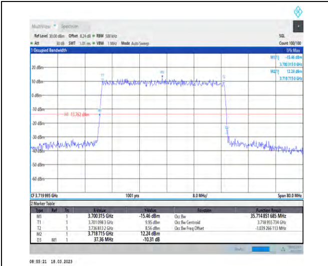
1-N78-3700-3800-30-40-L-3-DFT-16QAM-Outer_Full -100@0-Ant1-35.715-37.360-≤40-PASS
