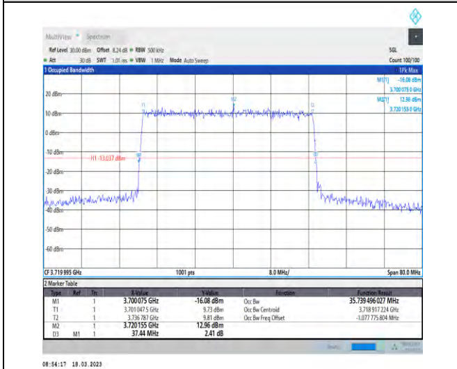
1-N78-3700-3800-30-40-L-1-DFT-QPSK-Outer_Full-100@0-Ant1-35.739-37.440-≤40-PASS
