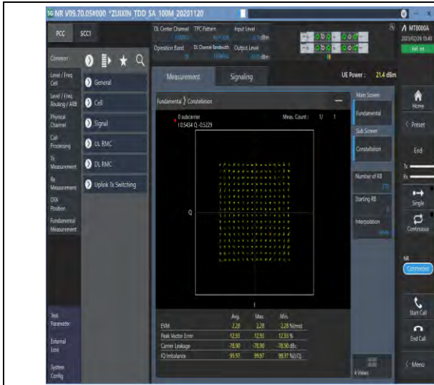
1-N78-3700-3800-30-100-M-5-DFT-256QAM-Outer_Full-270@0-Ant1-see graph-PASS
