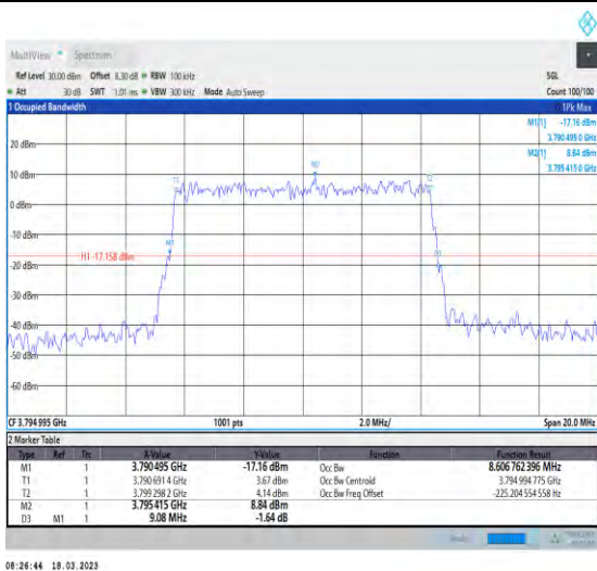
1-N78-3700-3800-30-10-H-5-DFT-256QAM-Outer_Full-24@0-Ant1-8.607-9.080-≤10-PASS
