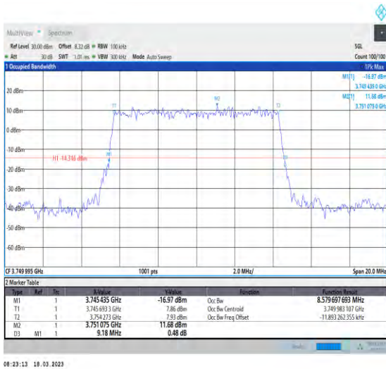
1-N78-3700-3800-30-10-M-2-DFT-PI2BPSK-Outer_Full -24@0-Ant1-8.58-9.180-≤10-PASS
