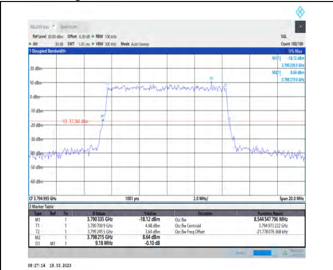
1-N78-3700-3800-30-10-H-8-CP-64QAM-Outer_Full-24@0-Ant1-8.545-9.180-≤10-PASS
