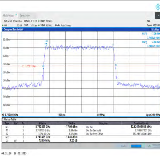
1-N78-3700-3800-30-15-M-1-DFT-QPSK-Outer_Full-36@0-Ant1-12.825-13.650-≤15-PASS
