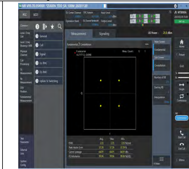
1-N78-3700-3800-30-100-M-6-CP-QPSK-Outer_Full-273@0-Ant1-see graph-PASS
