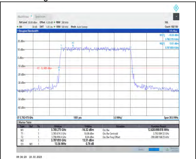
1-N78-3700-3800-30-15-H-1-DFT-QPSK-Outer_Full-36@0-Ant1-12.82-13.560-≤15-PASS
