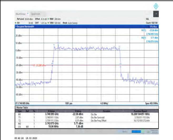
1-N78-3700-3800-30-20-M-9-CP-256QAM-Outer_Fu-51@0-Ant1-18.2-19.040-≤20-PASS
