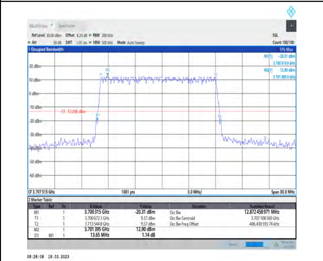
1-N78-3700-3800-30-15-L-1-DFT-QPSK-Outer_Full-36@0-Ant1-12.872-13.650-≤15-PASS
