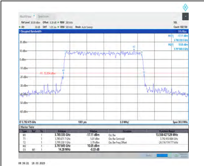
1-N78-3700-3800-30-15-H-8-CP-64QAM-Outer_Full-38@0-Ant1-13.558-14.280-≤15-PASS
