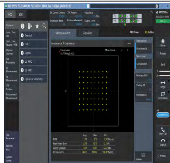
1-N78-3700-3800-30-100-M-4-DFT-64QAM-Outer_Full-270@0-Ant1-see graph-PASS
