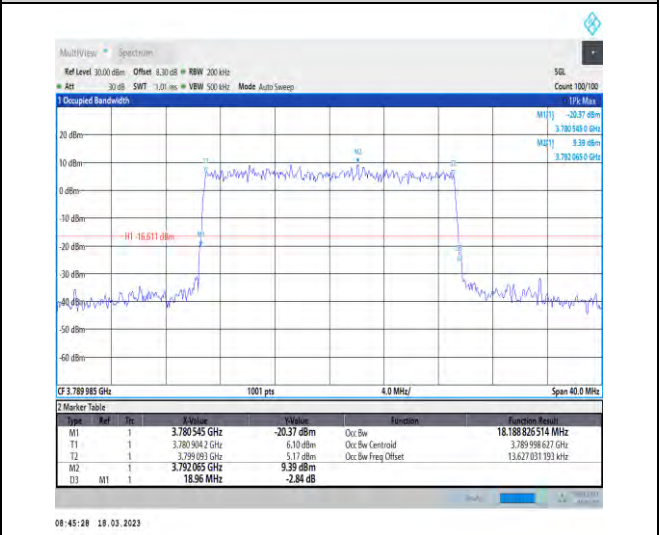
1-N78-3700-3800-30-20-H-8-CP-64QAM-Outer_Full-51@0-Ant1-18.189-18.960-≤20-PASS
