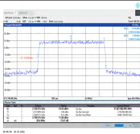
1-N78-3700-3800-30-40-M-7-CP-16QAM-Outer_Full-106@0-Ant1-37.828-39.600-≤40-PASS
