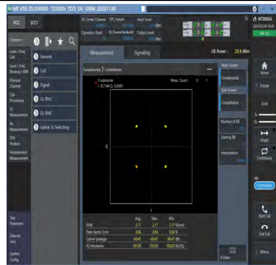
1-N78-3700-3800-30-100-M-2-DFT-QPSK-Outer_Full-270@0-Ant1-see graph-PASS
