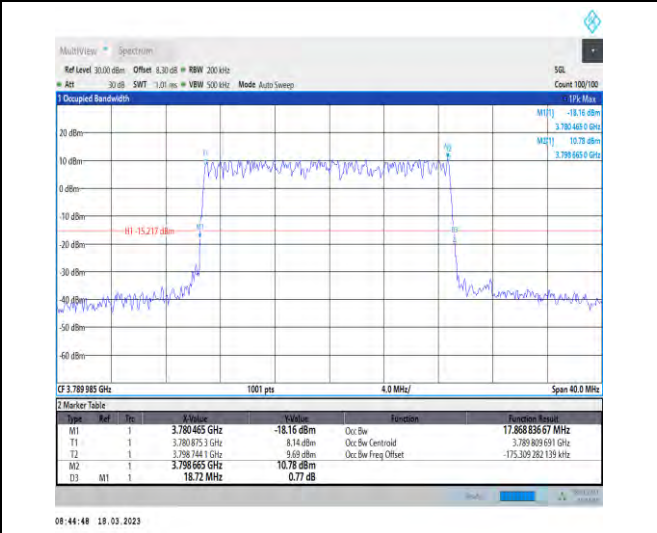
1-N78-3700-3800-30-20-H-4-DFT-64QAM-Outer_Full-50@0-Ant1-17.869-18.720-≤20-PASS
