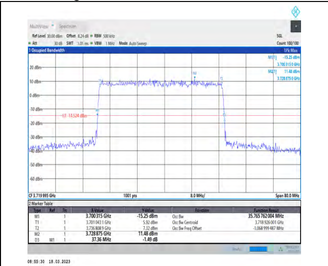
1-N78-3700-3800-30-40-L-4-DFT-64QAM-Outer_Full -100@0-Ant1-35.766-37.360-≤40-PASS
