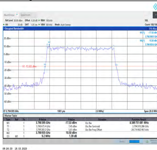
1-N78-3700-3800-30-10-H-4-DFT-64QAM-Outer_Ful I-24@0-Ant1-8.59-9.200-≤10-PASS
