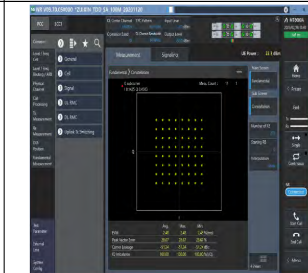
1-N78-3700-3800-30-100-M-8-CP-64QAM-Outer_Full-273@0-Ant1-see graph-PASS
